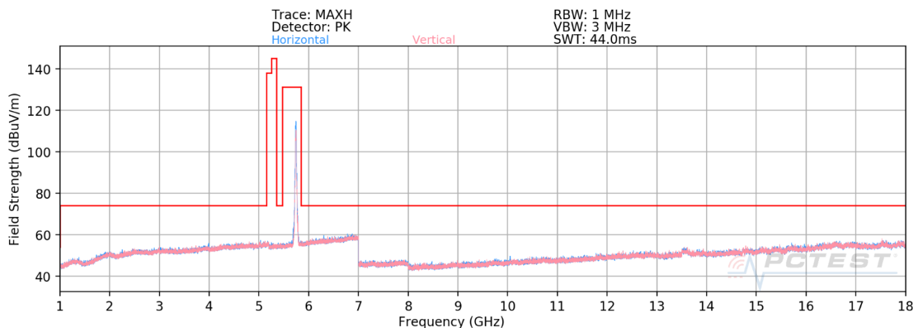
Plot 7-610. RSE above 1GHz Antenna 3b (11ax – Ch.149 – RU242)
