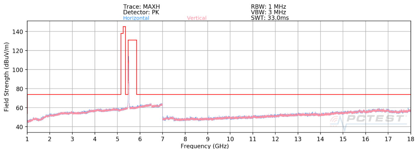
Plot 7-631. RSE above 1GHz Antenna 1b (11ax – Ch.100 – RU242)
