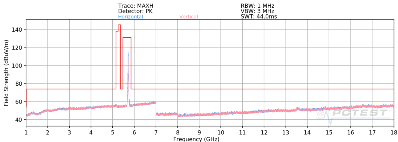
Plot 7-609. RSE above 1GHz Antenna 3b (11ax – Ch.144 – RU242)
