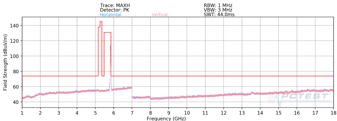
Plot 7-612. RSE above 1GHz Antenna 3b (11ax – Ch.165 – RU242)
