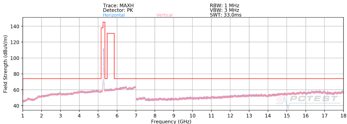
Plot 7-629. RSE above 1GHz Antenna 1b (11ax – Ch.56 – RU242)
