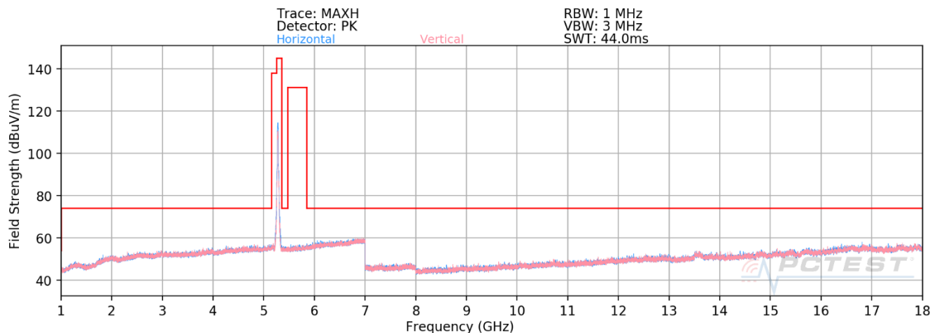
Plot 7-605. RSE above 1GHz Antenna 3b (11ax – Ch.56 – RU242)
