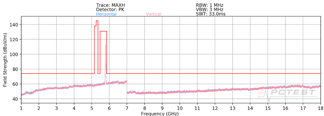
Plot 7-635. RSE above 1GHz Antenna 1b (11ax – Ch.157 – RU242)
