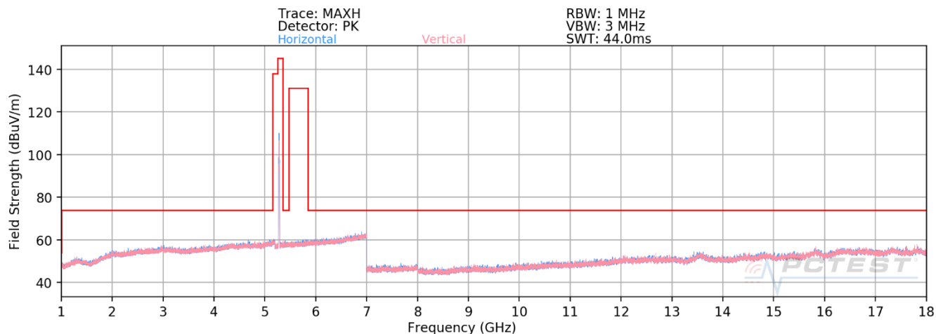
Plot 7-617. RSE above 1GHz Antenna 1b (11ax – Ch.56 – RU26)
