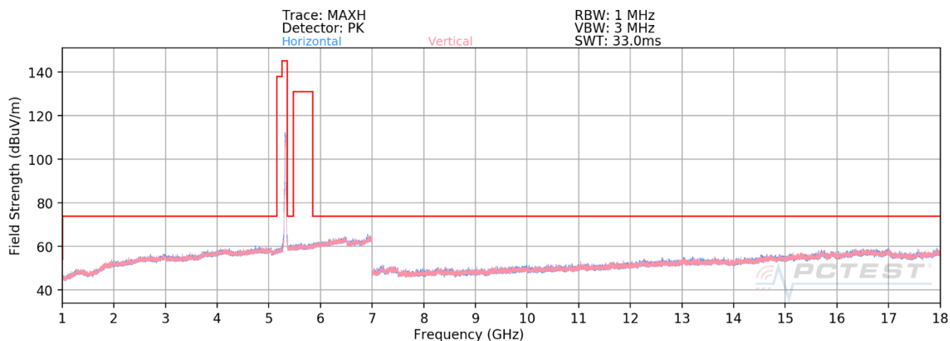
Plot 7-630. RSE above 1GHz Antenna 1b (11ax – Ch.64 – RU242)
