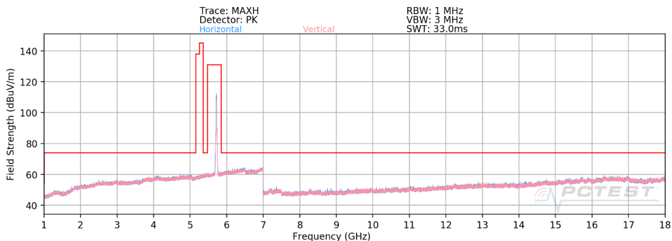
Plot 7-633. RSE above 1GHz Antenna 1b (11ax – Ch.144 – RU242)
