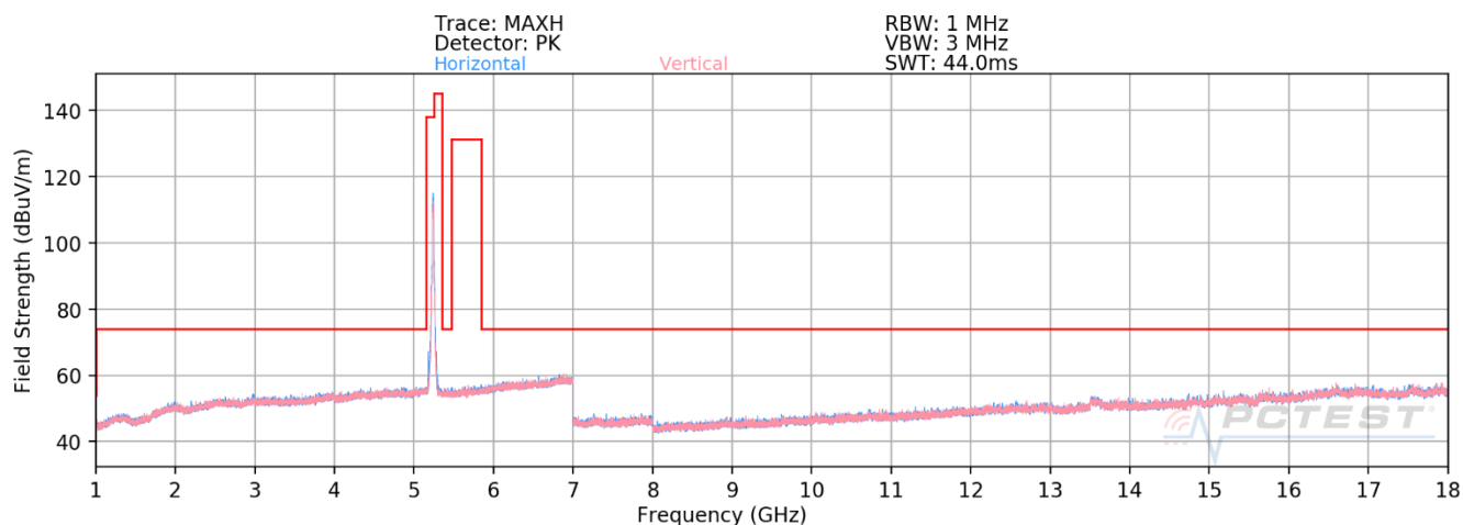
Plot 7-627. RSE above 1GHz Antenna 1b (11ax – Ch.48 – RU242)
