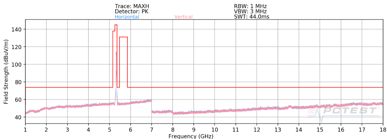
Plot 7-606. RSE above 1GHz Antenna 3b (11ax – Ch.64 – RU242)
