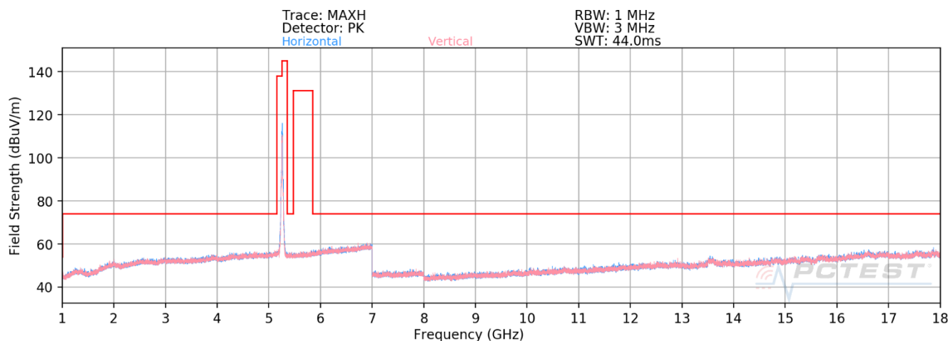
Plot 7-604. RSE above 1GHz Antenna 3b (11ax – Ch.52 – RU242)
