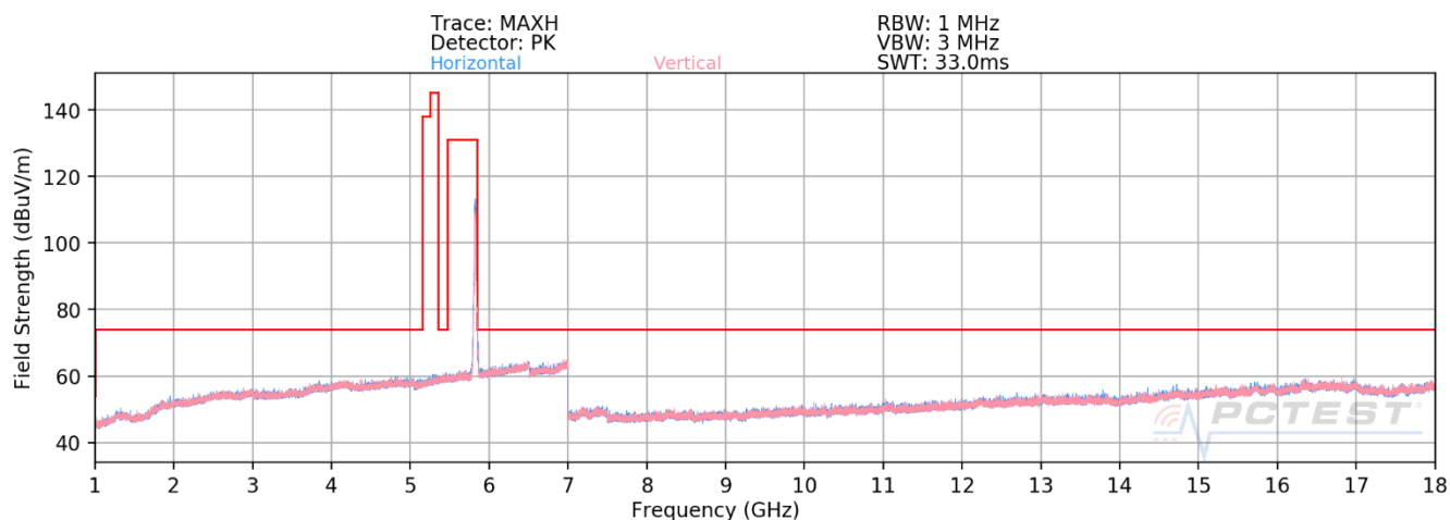
Plot 7-636. RSE above 1GHz Antenna 1b (11ax – Ch.165 – RU242)
