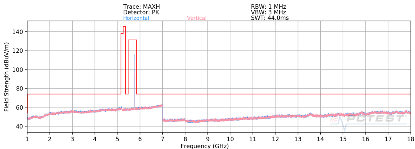
Plot 7-598. RSE above 1GHz Antenna 3b (11ax – Ch.149 – RU26)
