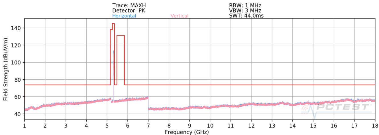
Plot 7-594. RSE above 1GHz Antenna 3b (11ax – Ch.64 – RU26)
