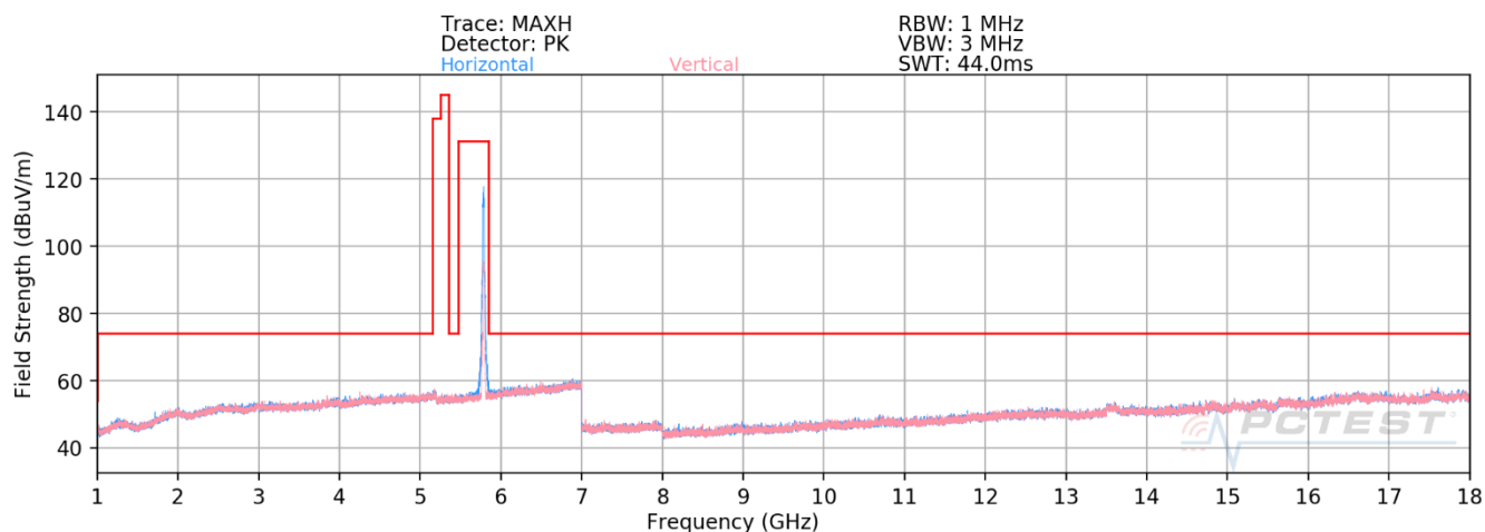
Plot 7-587. RSE above 1GHz Antenna 5T (11ax – Ch.157 – RU242)
