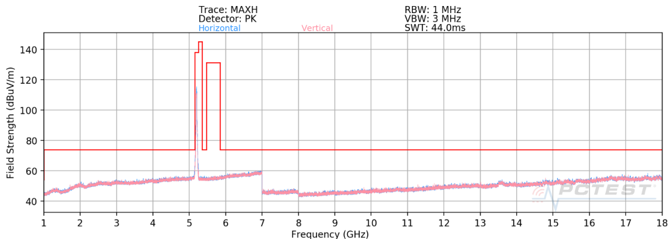
Plot 7-602. RSE above 1GHz Antenna 3b (11ax – Ch.40 – RU242)
