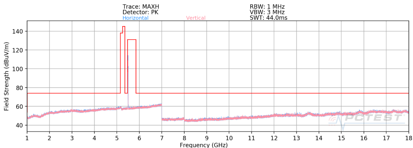
Plot 7-595. RSE above 1GHz Antenna 3b (11ax – Ch.100 – RU26)
