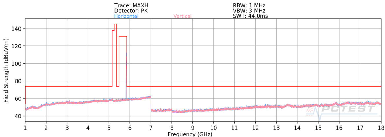
Plot 7-600. RSE above 1GHz Antenna 3b (11ax – Ch.165 – RU26)
