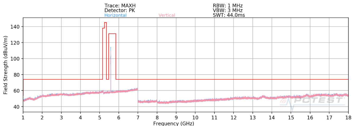
Plot 7-596. RSE above 1GHz Antenna 3b (11ax – Ch.116 – RU26)
