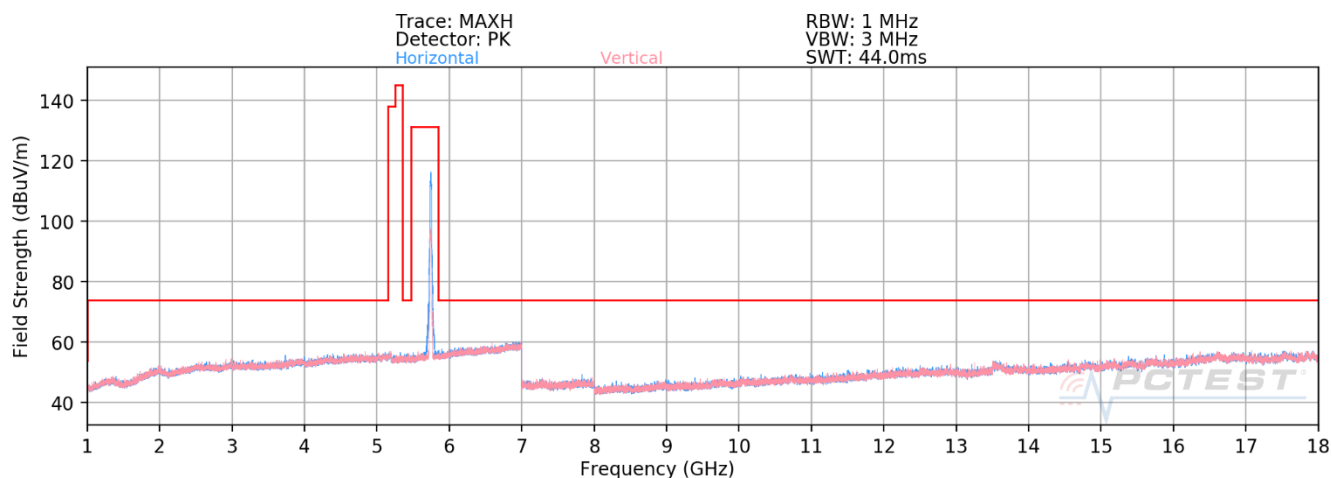
Plot 7-586. RSE above 1GHz Antenna 5T (11ax – Ch.149 – RU242)
