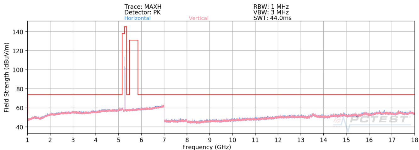
Plot 7-593. RSE above 1GHz Antenna 3b (11ax – Ch.56 – RU26)
