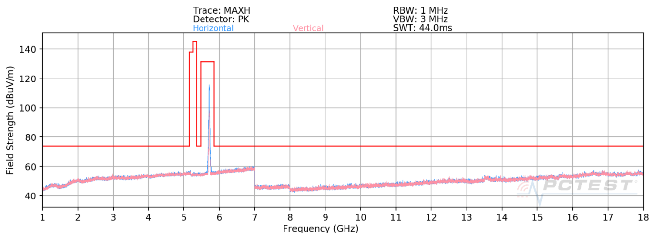
Plot 7-585. RSE above 1GHz Antenna 5T (11ax – Ch.144 – RU242)
