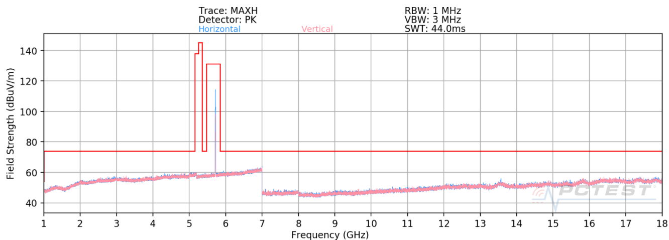
Plot 7-573. RSE above 1GHz Antenna 5T (11ax – Ch.144 – RU26)
