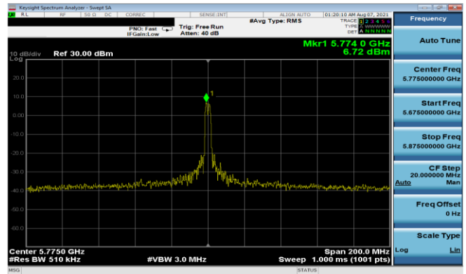
Plot 7-190. PSD Antenna 5T (80MHz BW 11ax Index 18 - RU26 - Ch.155)
