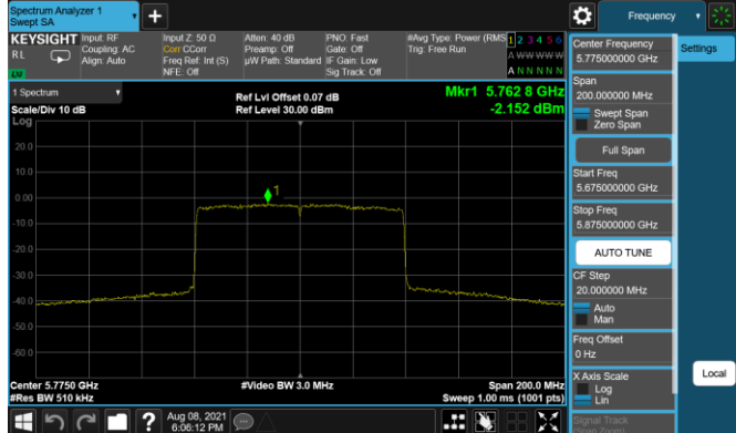
Plot 7-192. PSD Antenna 5T (80MHz BW 11ax - RU996 - Ch.155)
