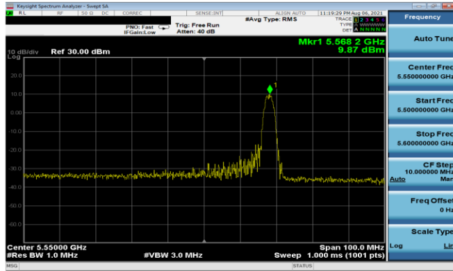
Plot 7-175. PSD Antenna 5T (40MHz BW 11ax Index 17 – RU26 – Ch.110)
