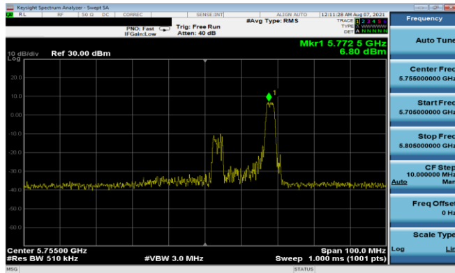
Plot 7-187. PSD Antenna 5T (40MHz BW 11ax Index 17 - RU26 - Ch.151)
