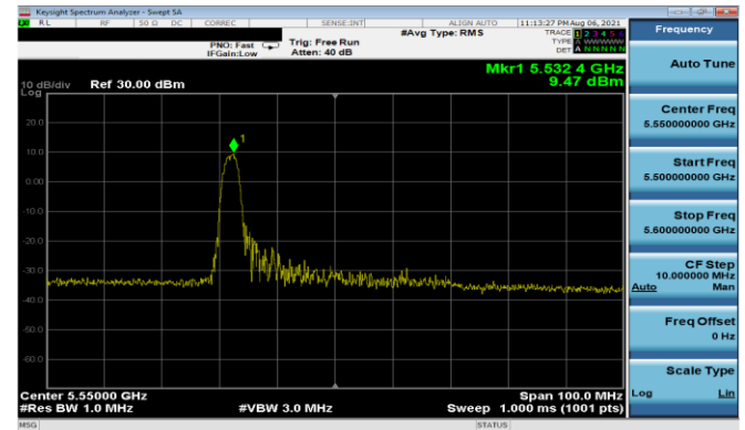
Plot 7-173. PSD Antenna 5T (40MHz BW 11ax Index 0 – RU26 – Ch.110)
