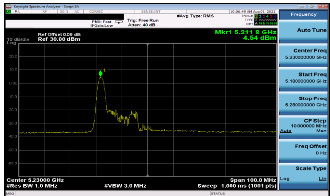
Plot 7-197. ISED PSD Antenna 5T (40MHz BW 11ax Index 0 – RU26 – Ch.46)
