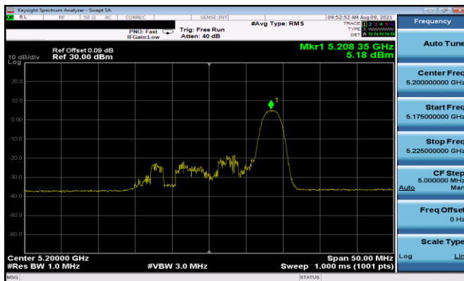
Plot 7-195. ISED PSD Antenna 5T (20MHz BW 11ax Index 8– RU26 – Ch.40)
