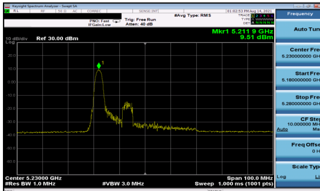
Plot 7-209. PSD Antenna 3b (40MHz BW 11ax Index 0 - RU26 - Ch.46)
