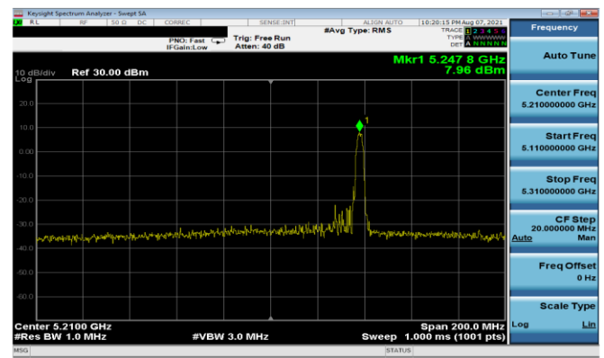
Plot 7-215. PSD Antenna 3b (80MHz BW 11ax Index 36 – RU26 – Ch.42)
