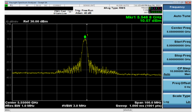
Plot 7-174. PSD Antenna 5T (40MHz BW 11ax Index 8 – RU26 – Ch.110)
