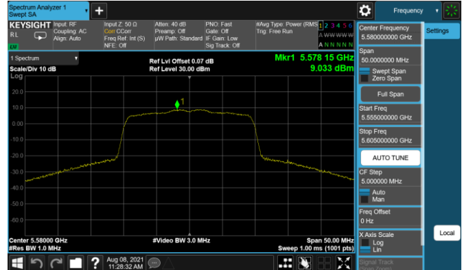
Plot 7-172. PSD Antenna 5T (20MHz BW 11ax– RU242 – Ch.116)
