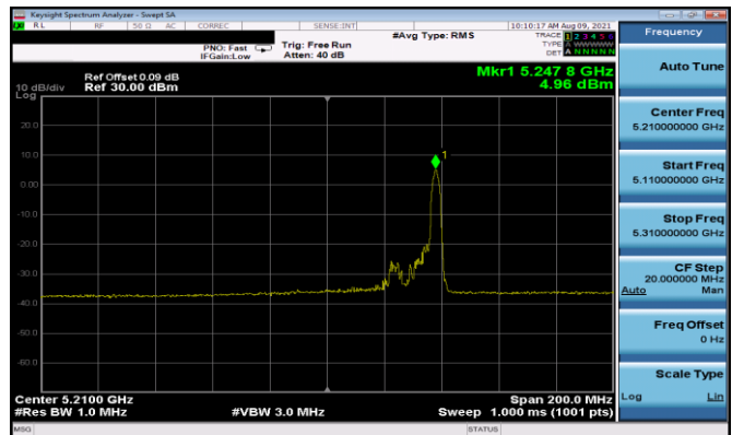
Plot 7-203. ISED PSD Antenna 5T (80MHz BW 11ax Index 36 - RU26 - Ch.42)
