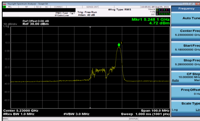
Plot 7-199. ISED PSD Antenna 5T (40MHz BW 11ax Index 17 - RU26 - Ch.46)
