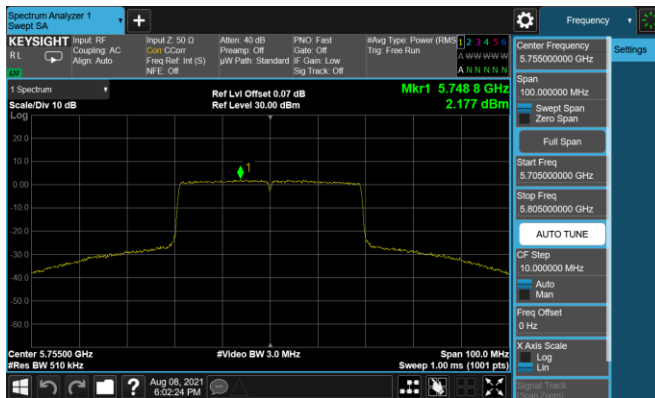
Plot 7-188. PSD Antenna 5T (40MHz BW 11ax - RU484 - Ch.151)
