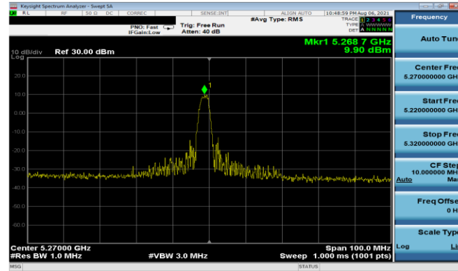
Plot 7-162. PSD Antenna 5T (40MHz BW 11ax Index 8 - RU26 - Ch.54)
