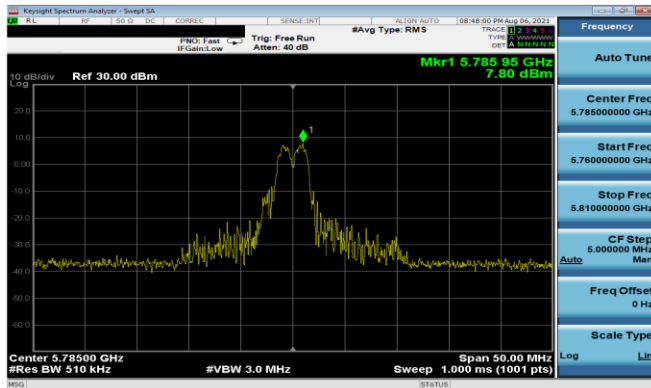
Plot 7-182. PSD Antenna 5T (20MHz BW 11ax Index 4 – RU26 – Ch.157)
