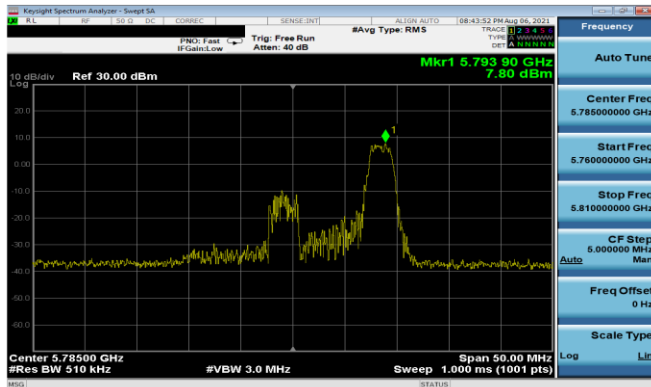
Plot 7-183. PSD Antenna 5T (20MHz BW 11ax Index 8– RU26 – Ch.157)
