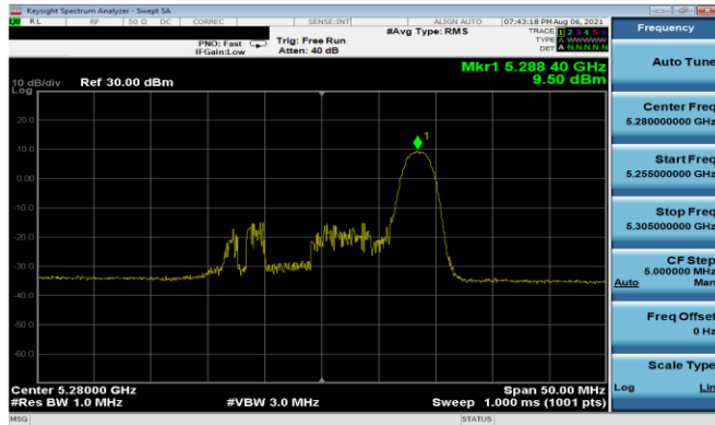
Plot 7-159. PSD Antenna 5T (20MHz BW 11ax Index 8- RU26 - Ch.56)
