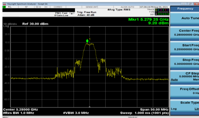
Plot 7-158. PSD Antenna 5T (20MHz BW 11ax Index 4 - RU26 - Ch.56)
