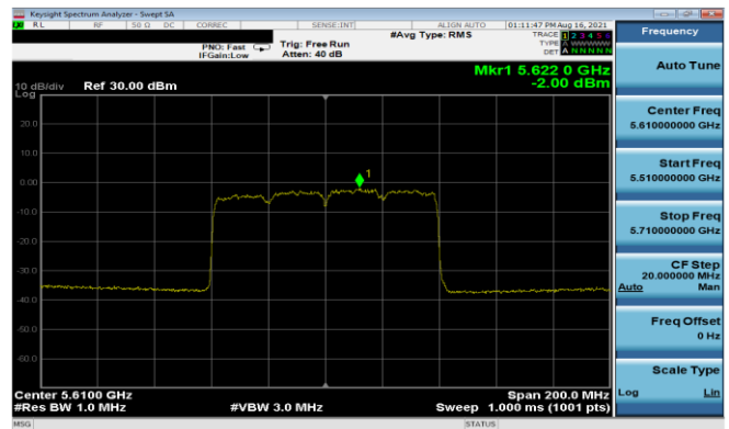
Plot 7-180. PSD Antenna 5T (80MHz BW 11ax – RU996 – Ch.122)
