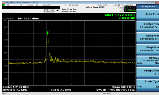
Plot 7-213. PSD Antenna 3b (80MHz BW 11ax Index 0 – RU26 – Ch.42)
