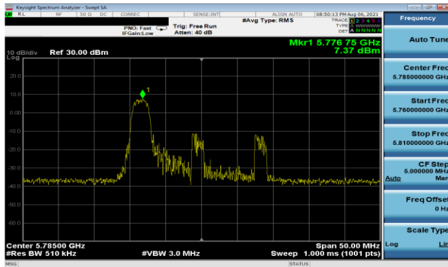
Plot 7-181. PSD Antenna 5T (20MHz BW 11ax Index 0 – RU26 – Ch.157)
