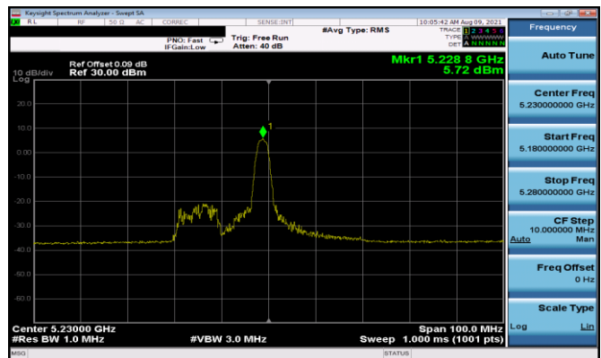
Plot 7-198. ISED PSD Antenna 5T (40MHz BW 11ax Index 8 – RU26 – Ch.46)
