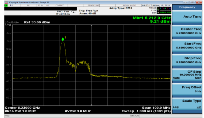
Plot 7-149. PSD Antenna 5T (40MHz BW 11ax Index 0 – RU26 – Ch.46)
