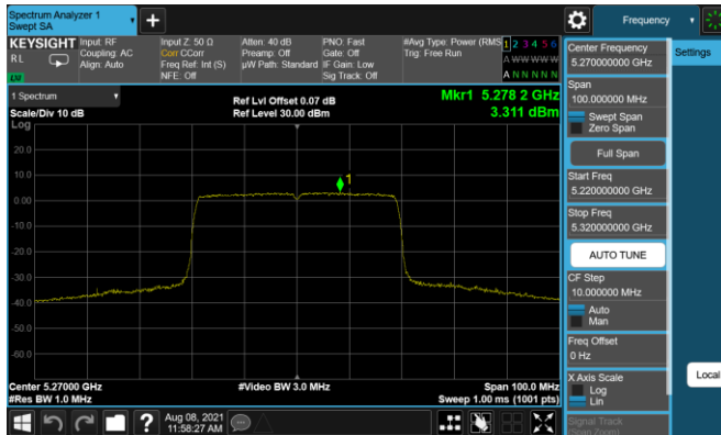
Plot 7-164. PSD Antenna 5T (40MHz BW 11ax - RU484 - Ch.54)
