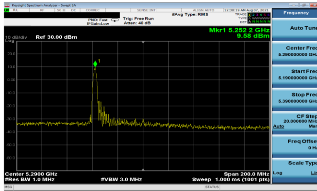
Plot 7-165. PSD Antenna 5T (80MHz BW 11ax Index 0 - RU26 - Ch.58)
