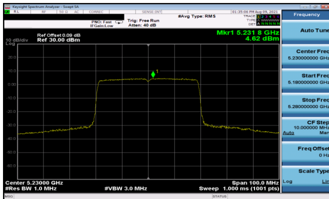
Plot 7-200. ISED PSD Antenna 5T (40MHz BW 11ax - RU484 - Ch.46)
