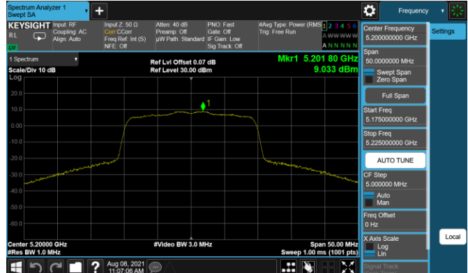
Plot 7-148. PSD Antenna 5T (20MHz BW 11ax– RU242 – Ch.40)
