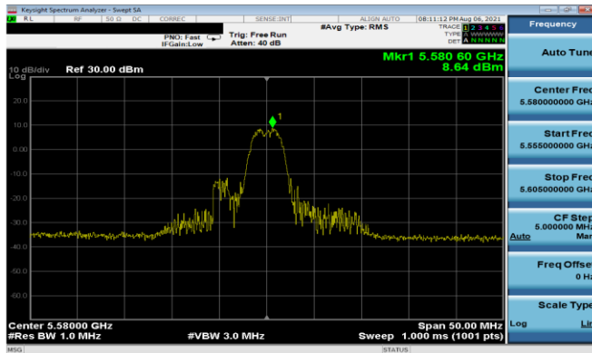
Plot 7-170. PSD Antenna 5T (20MHz BW 11ax Index 4 – RU26 – Ch.116)
