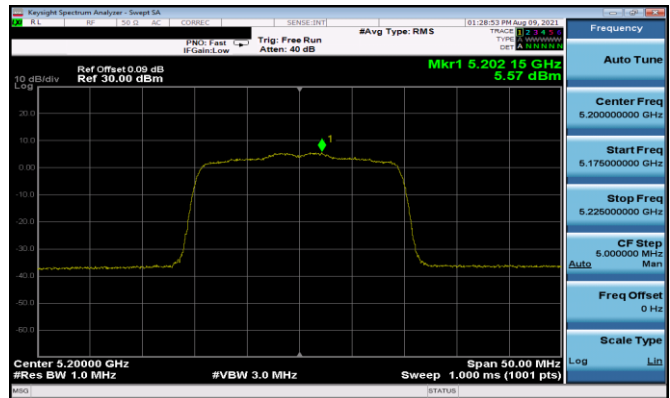
Plot 7-196. ISED PSD Antenna 5T (20MHz BW 11ax– RU242 – Ch.40)
