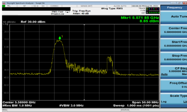
Plot 7-169. PSD Antenna 5T (20MHz BW 11ax Index 0 – RU26 – Ch.116)
