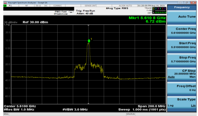
Plot 7-178. PSD Antenna 5T (80MHz BW 11ax Index 18 – RU26 – Ch.122)
