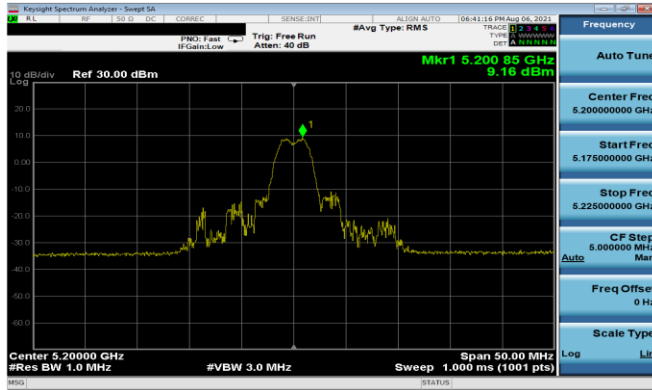
Plot 7-146. PSD Antenna 5T (20MHz BW 11ax Index 4 – RU26 – Ch.40)
