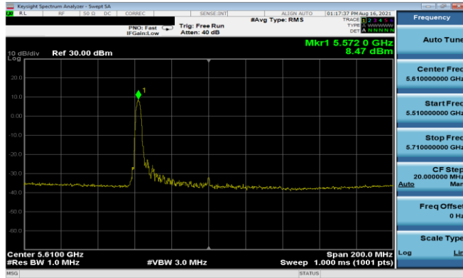
Plot 7-177. PSD Antenna 5T (80MHz BW 11ax Index 0 – RU26 – Ch.122)
