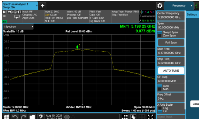
Plot 7-208. PSD Antenna 3b (20MHz BW 11ax- RU242 - Ch.40)
