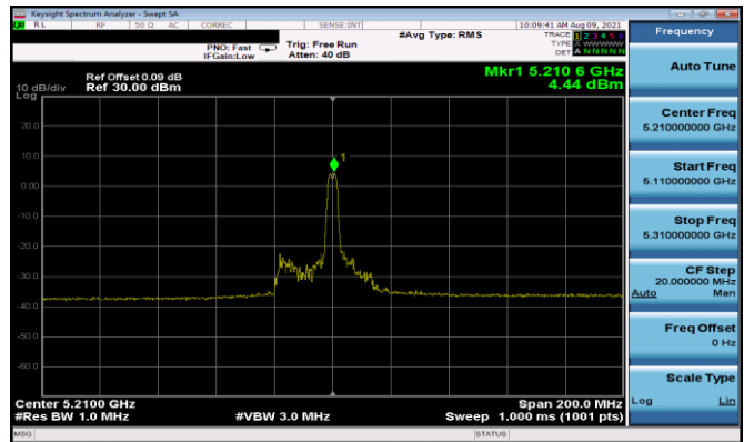
Plot 7-202. ISED PSD Antenna 5T (80MHz BW 11ax Index 18 - RU26 - Ch.42)
