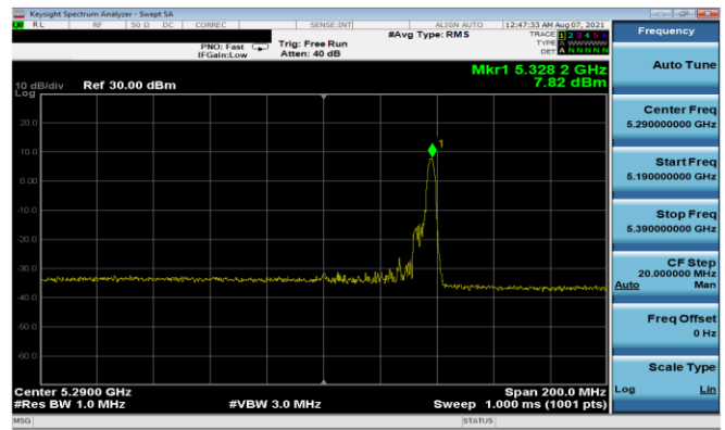
Plot 7-167. PSD Antenna 5T (80MHz BW 11ax Index 36 - RU26 - Ch.58)
