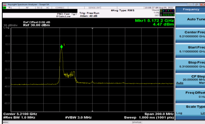
Plot 7-201. ISED PSD Antenna 5T (80MHz BW 11ax Index 0 - RU26 - Ch.42)
