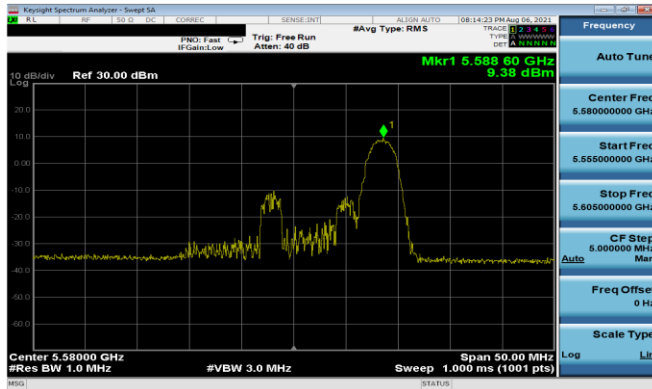
Plot 7-171. PSD Antenna 5T (20MHz BW 11ax Index 8– RU26 – Ch.116)
