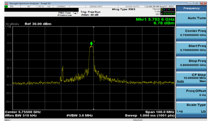
Plot 7-186. PSD Antenna 5T (40MHz BW 11ax Index 8 – RU26 – Ch.151)
