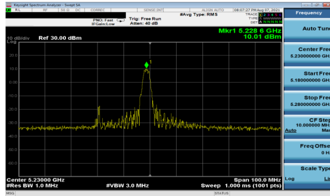
Plot 7-210. PSD Antenna 3b (40MHz BW 11ax Index 8 - RU26 - Ch.46)
