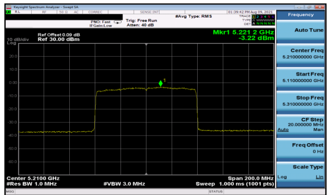
Plot 7-204. ISED PSD Antenna 5T (80MHz BW 11ax - RU996 - Ch.42)
