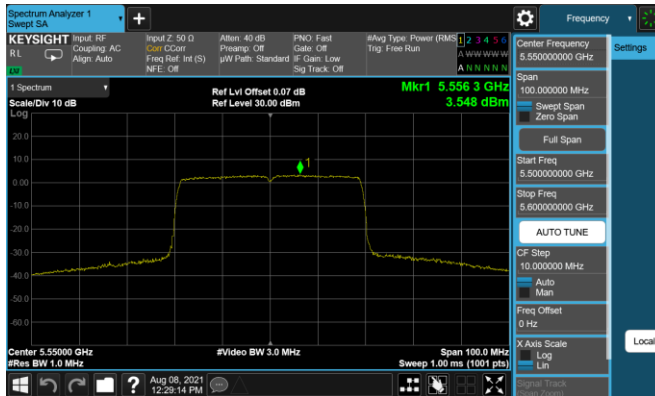
Plot 7-176. PSD Antenna 5T (40MHz BW 11ax – RU484 – Ch.110)
