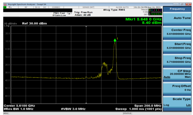
Plot 7-179. PSD Antenna 5T (80MHz BW 11ax Index 36 – RU26 – Ch.122)
