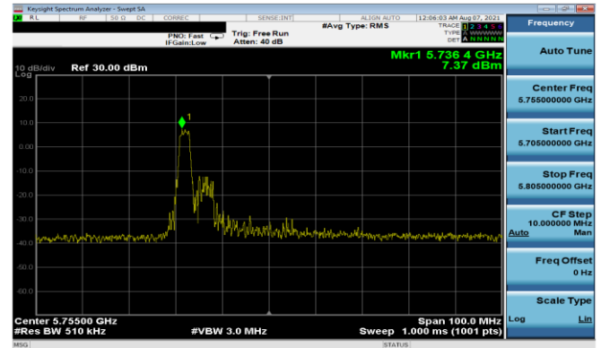
Plot 7-185. PSD Antenna 5T (40MHz BW 11ax Index 0 – RU26 – Ch.151)
