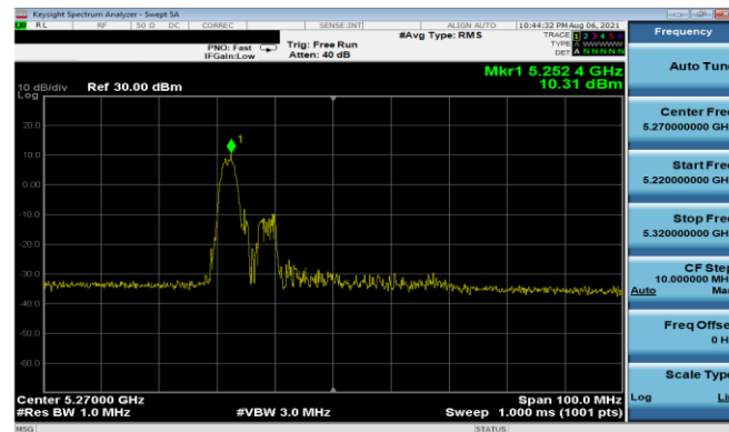
Plot 7-161. PSD Antenna 5T (40MHz BW 11ax Index 0 - RU26 - Ch.54)
