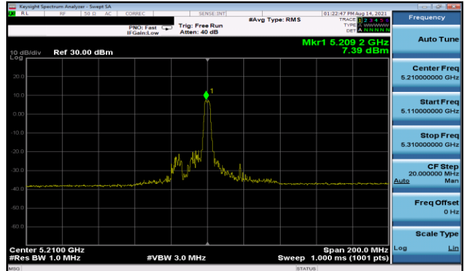
Plot 7-214. PSD Antenna 3b (80MHz BW 11ax Index 18 – RU26 – Ch.42)
