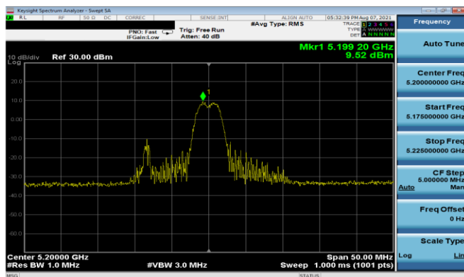
Plot 7-206. PSD Antenna 3b (20MHz BW 11ax Index 4 - RU26 - Ch.40)
