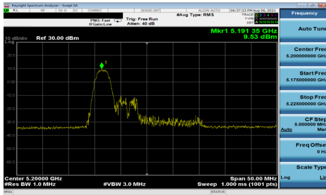
Plot 7-145. PSD Antenna 5T (20MHz BW 11ax Index 0 – RU26 – Ch.40)
