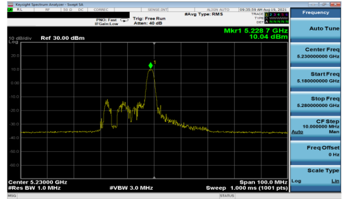
Plot 7-150. PSD Antenna 5T (40MHz BW 11ax Index 8 – RU26 – Ch.46)
