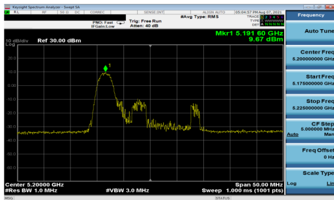
Plot 7-205. PSD Antenna 3b (20MHz BW 11ax Index 0 - RU26 - Ch.40)
