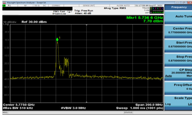
Plot 7-189. PSD Antenna 5T (80MHz BW 11ax Index 0 - RU26 - Ch.155)
