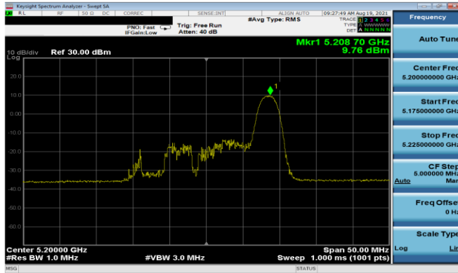
Plot 7-147. PSD Antenna 5T (20MHz BW 11ax Index 8– RU26 – Ch.40)
