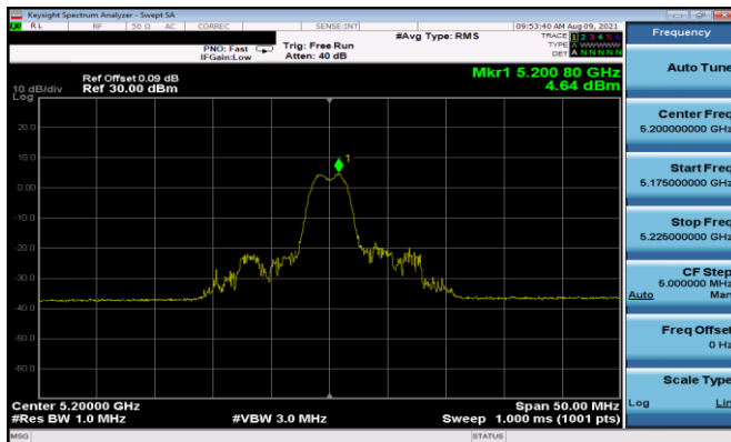
Plot 7-194. ISED PSD Antenna 5T (20MHz BW 11ax Index 4 – RU26 – Ch.40)
