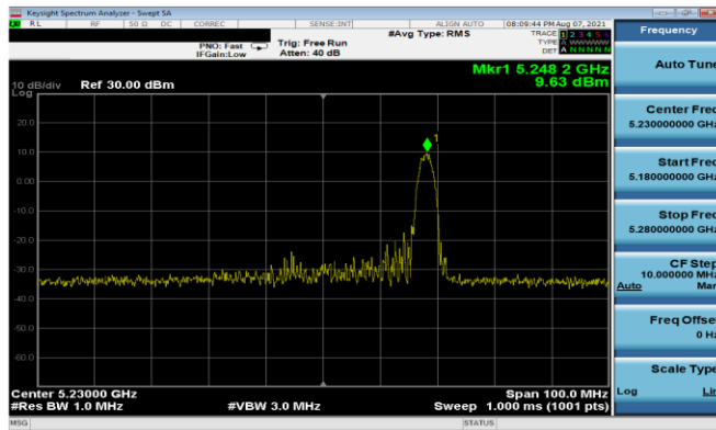
Plot 7-211. PSD Antenna 3b (40MHz BW 11ax Index 17 – RU26 – Ch.46)
