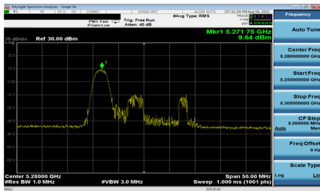
Plot 7-157. PSD Antenna 5T (20MHz BW 11ax Index 0 - RU26 - Ch.56)
