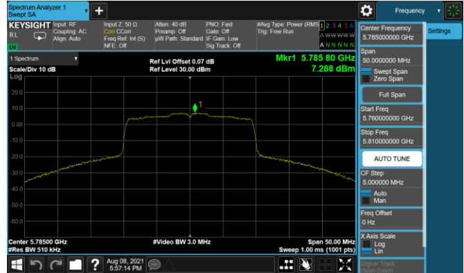
Plot 7-184. PSD Antenna 5T (20MHz BW 11ax– RU242 – Ch.157)
