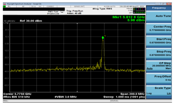
Plot 7-191. PSD Antenna 5T (80MHz BW 11ax Index 36 - RU26 - Ch.155)
