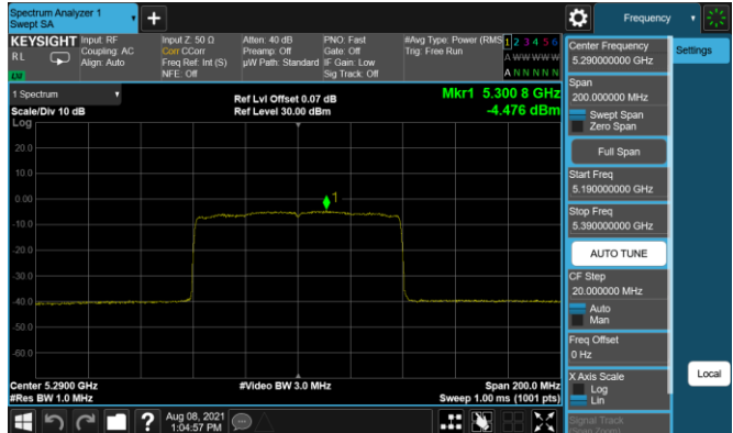
Plot 7-168. PSD Antenna 5T (80MHz BW 11ax - RU996 - Ch.58)
