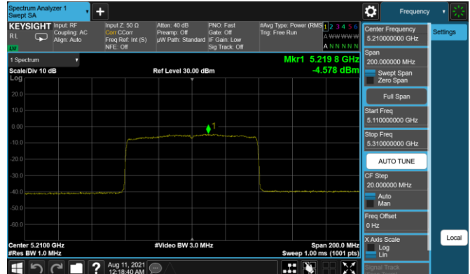
Plot 7-216. PSD Antenna 3b (80MHz BW 11ax – RU996 – Ch.42)
