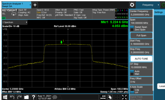
Plot 7-212. PSD Antenna 3b (40MHz BW 11ax – RU484 – Ch.46)
