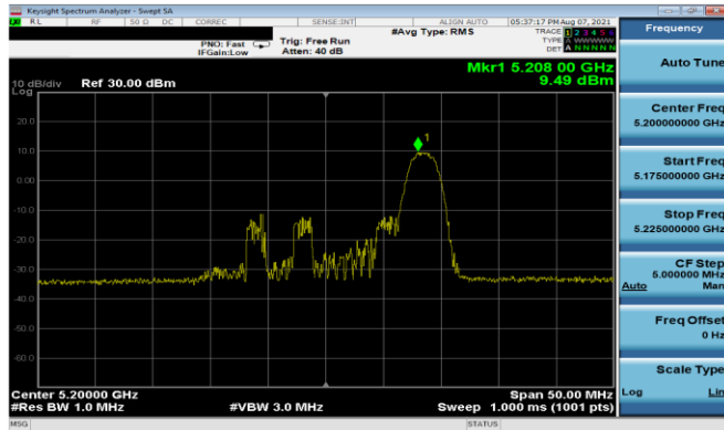
Plot 7-207. PSD Antenna 3b (20MHz BW 11ax Index 8- RU26 - Ch.40)
