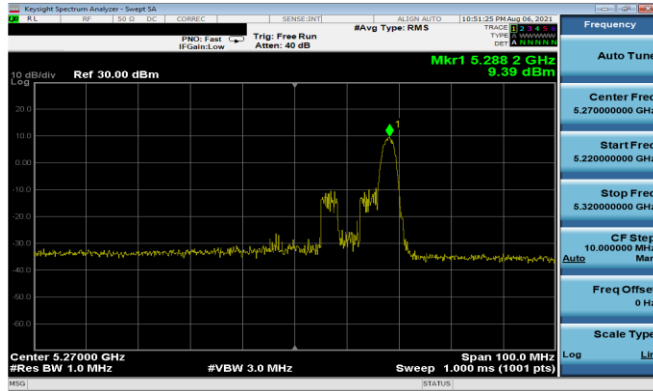
Plot 7-163. PSD Antenna 5T (40MHz BW 11ax Index 17 - RU26 - Ch.54)
