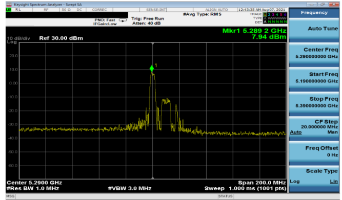
Plot 7-166. PSD Antenna 5T (80MHz BW 11ax Index 18 - RU26 - Ch.58)
