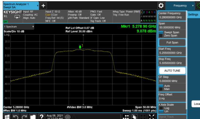
Plot 7-160. PSD Antenna 5T (20MHz BW 11ax- RU242 - Ch.56)
