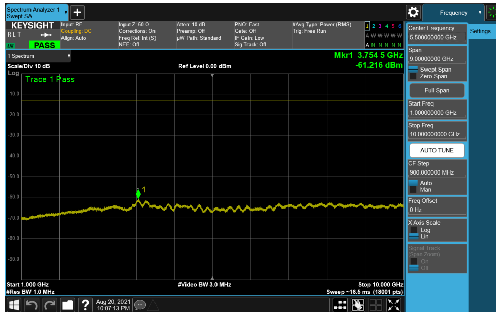
Plot 7-42. Conducted Spurious Plot (LTE Band 14 - 5MHz QPSK - RB Size 1, RB Offset 0 – High Channel)
