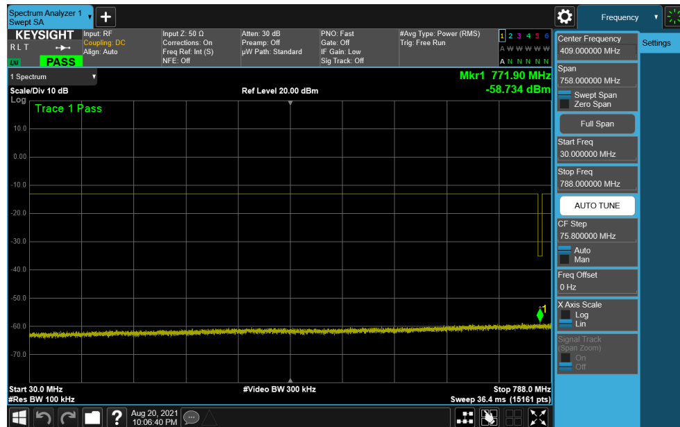
Plot 7-40. Conducted Spurious Plot (LTE Band 14 - 5MHz QPSK - RB Size 1, RB Offset 0 – High Channel)
