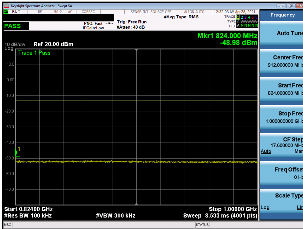
Plot 7-29. Conducted Spurious Plot (Band 26 - 10MHz QPSK - RB Size 1, RB Offset 0 - Mid Channel)
