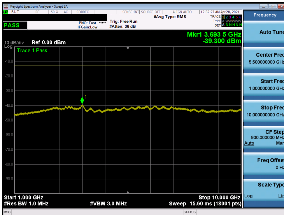
Plot 7-30. Conducted Spurious Plot (Band 26 - 10MHz QPSK - RB Size 1, RB Offset 0 - Mid Channel)
