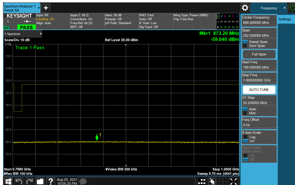
Plot 7-41. Conducted Spurious Plot (LTE Band 14 - 5MHz QPSK - RB Size 1, RB Offset 0 – High Channel)
