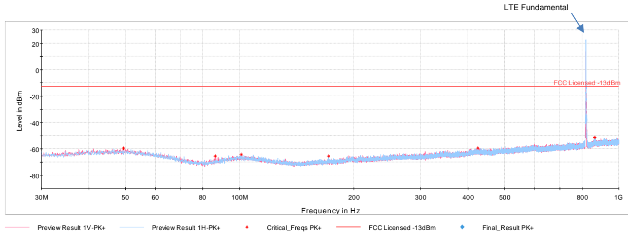
Plot 7-58. Antenna 4 Radiated Spurious Plot below 1GHz (LTE Band 26)
