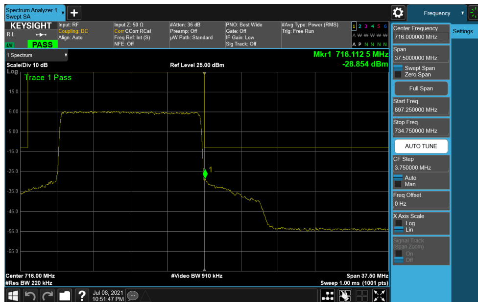
Plot 7-323. Upper Band Edge Plot (NR Band n12 – 15.0MHz DFT-s-OFDM \pi/2 BPSK - Full RB)
