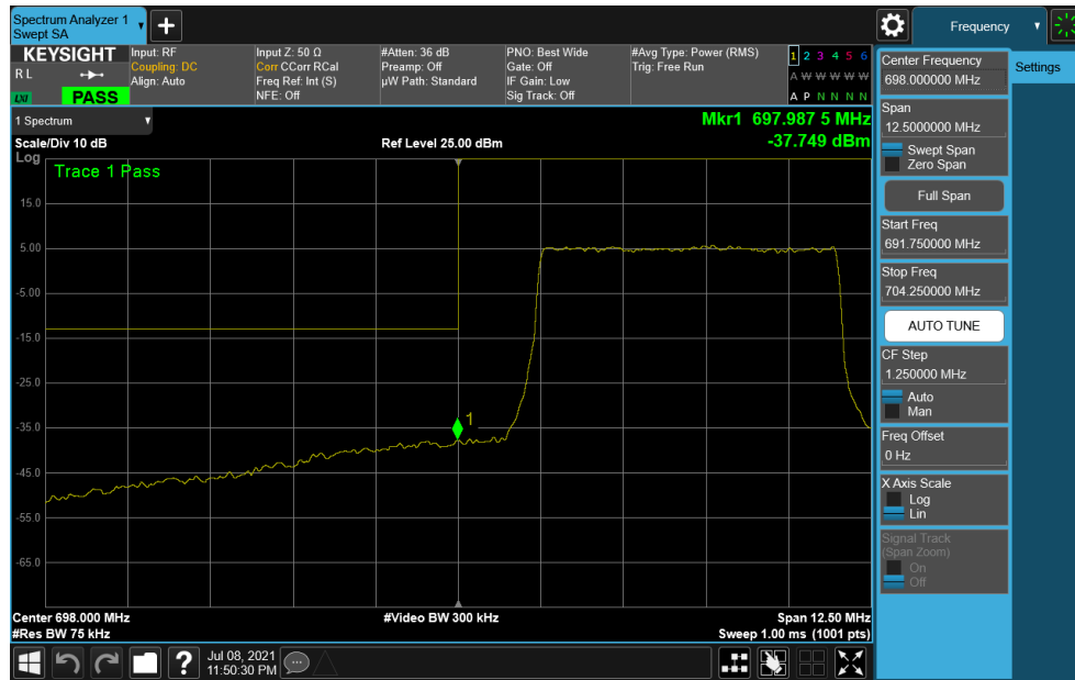
Plot 7-318. Lower Band Edge Plot (NR Band n12 – 5.0MHz DFT-s-OFDM \pi/2 BPSK - Full RB)
