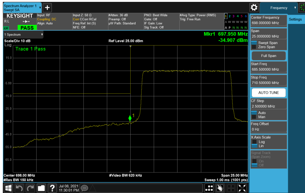
Plot 7-320. Lower Band Edge Plot (NR Band n12 – 10.0MHz DFT-s-OFDM \pi/2 BPSK - Full RB)
