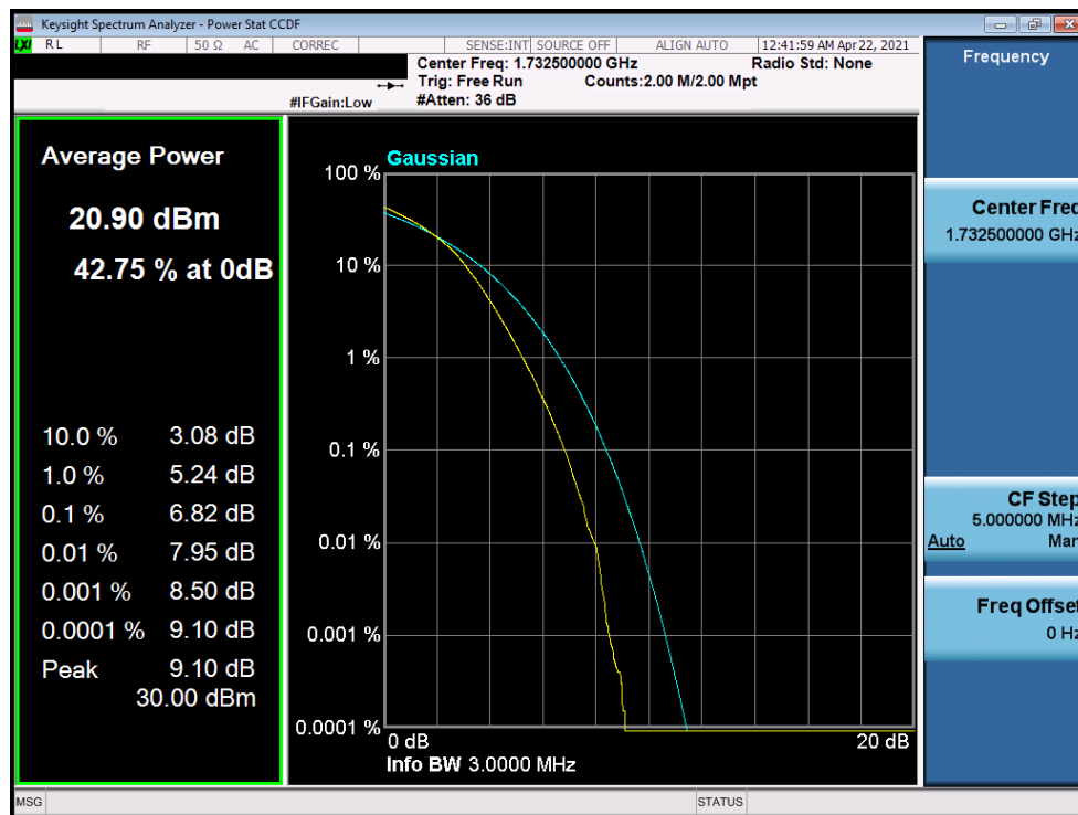
Plot 7-359. PAR Plot (LTE Band 4 - 3MHz 256-QAM - Full RB)
