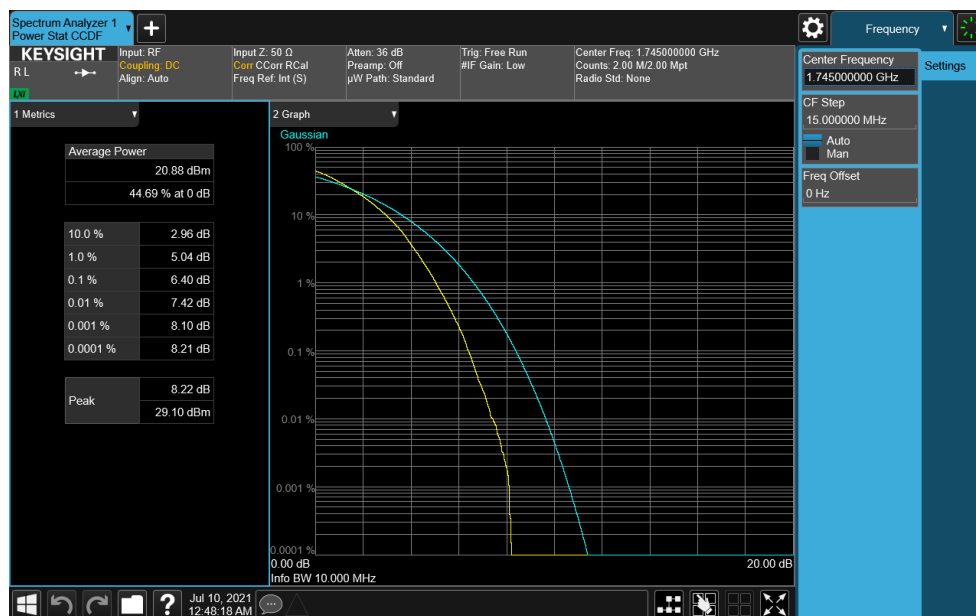
Plot 7-385. PAR Plot (NR Band n66- 10MHz DFT-s-OFDM 256-QAM - Full RB)
