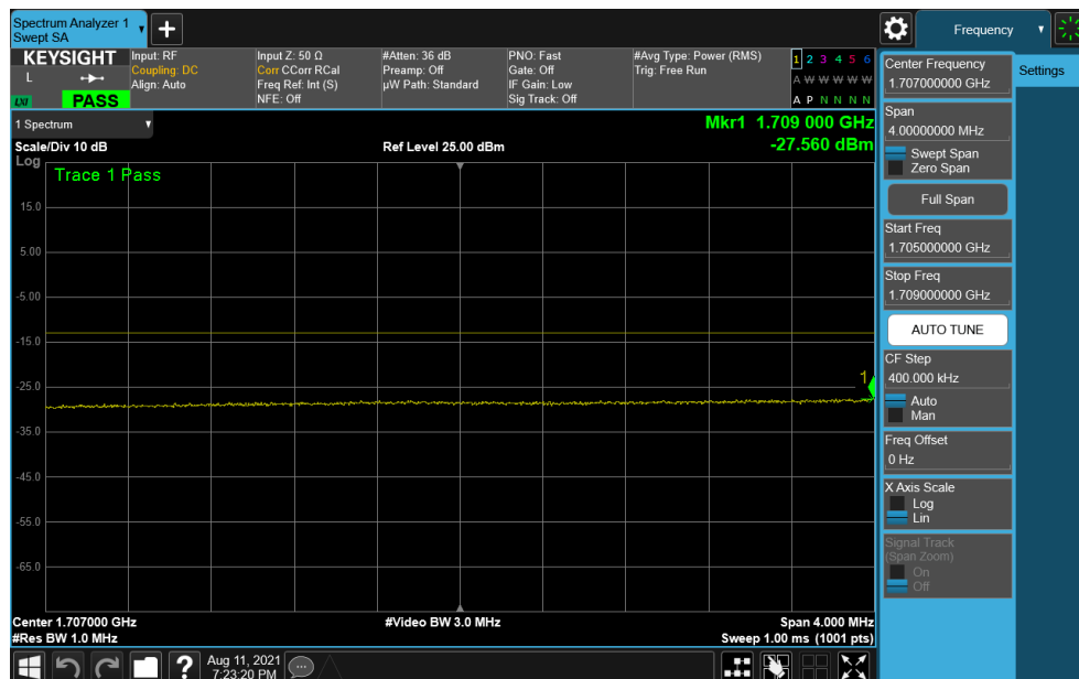
Plot 7-307. Lower Extended Band Edge Plot (NR Band n66 – 40.0MHz CP-OFDM QPSK - Full RB)
