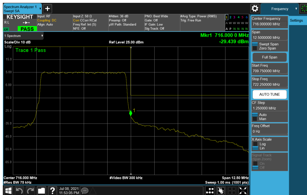
Plot 7-319. Upper Band Edge Plot (NR Band n12 – 5.0MHz DFT-s-OFDM \pi/2 BPSK - Full RB)
