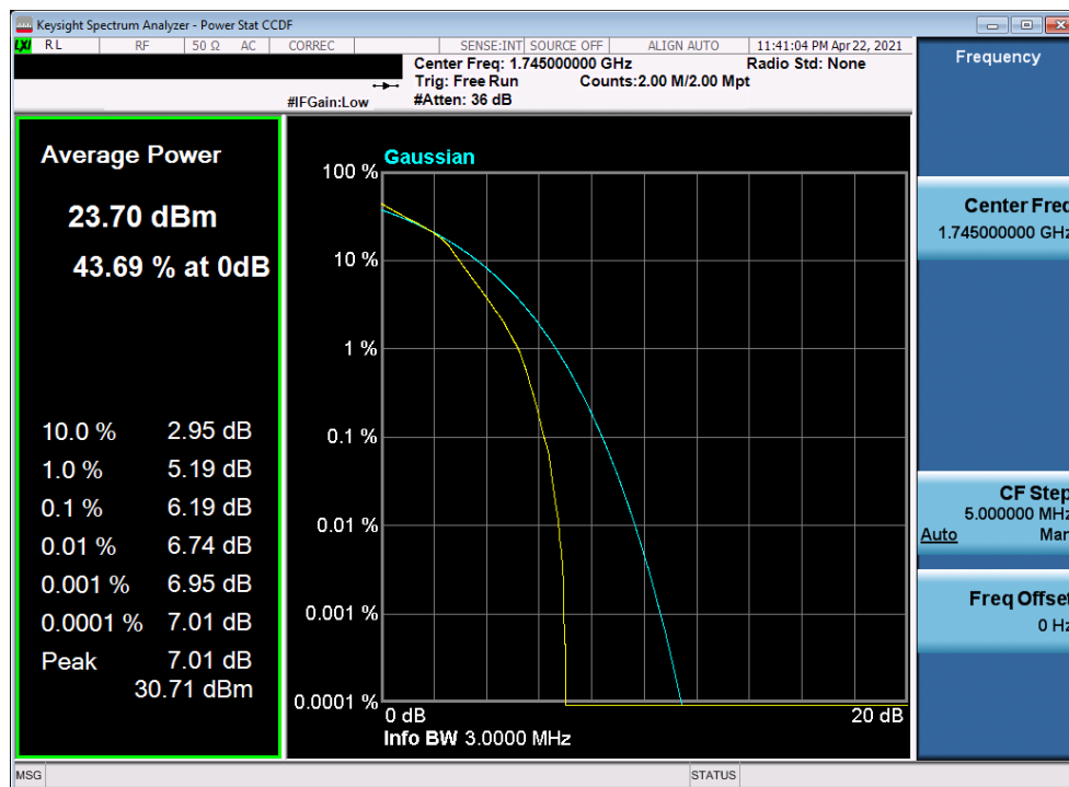
Plot 7-333. PAR Plot (LTE Band 66 - 3MHz 16-QAM - Full RB)
