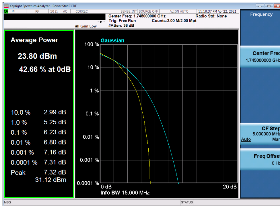
Plot 7-345. PAR Plot (LTE Band 66 - 15MHz 16-QAM - Full RB)
