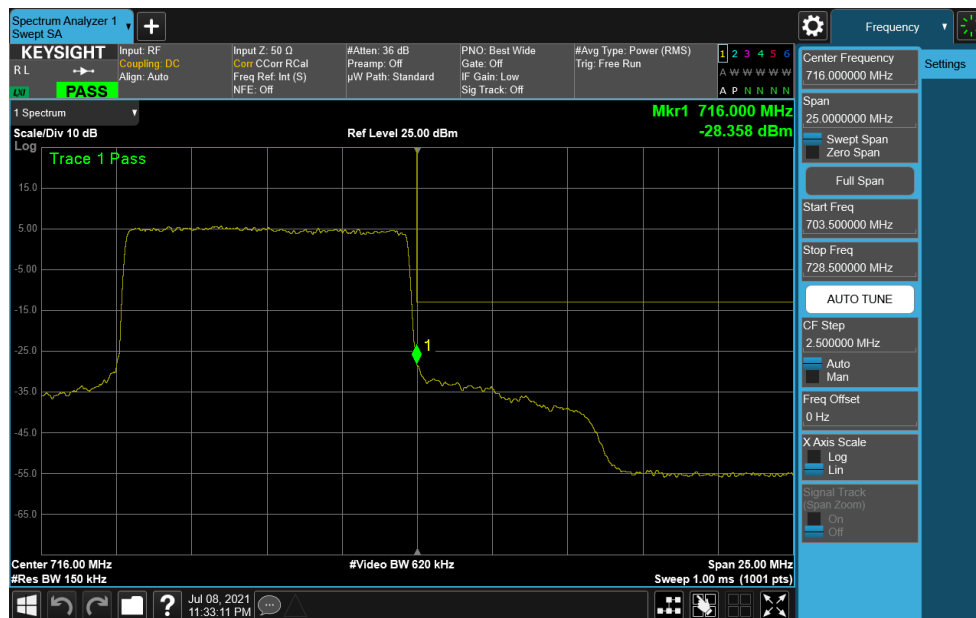
Plot 7-321. Upper Band Edge Plot (NR Band n12 – 10.0MHz DFT-s-OFDM \pi/2 BPSK - Full RB)
