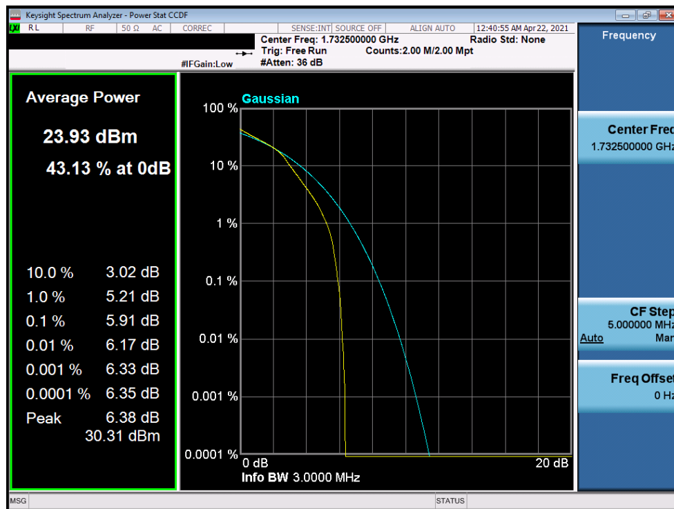
Plot 7-357. PAR Plot (LTE Band 4 - 3MHz 16-QAM - Full RB)
