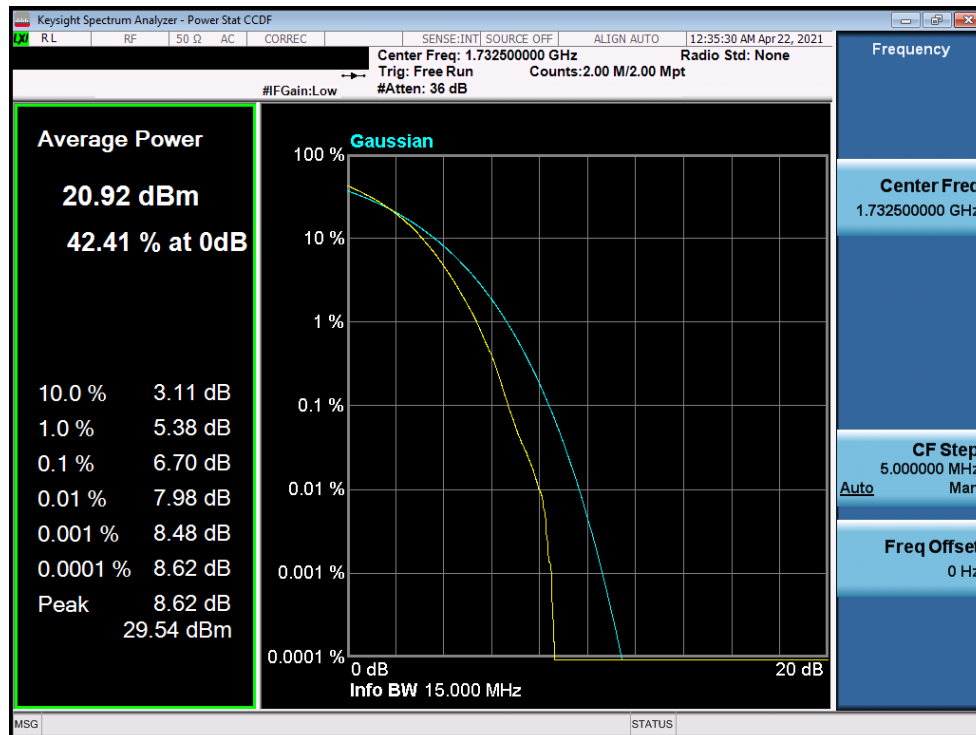
Plot 7-371. PAR Plot (LTE Band 4 - 15MHz 256-QAM - Full RB)
