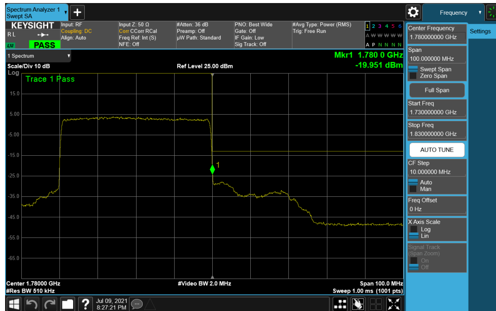
Plot 7-308. Upper Band Edge Plot (NR Band n66 – 40.0MHz DFT-s-OFDM \pi/2 BPSK - Full RB)
