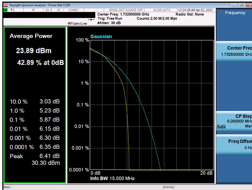
Plot 7-369. PAR Plot (LTE Band 4 - 15MHz 16-QAM - Full RB)
