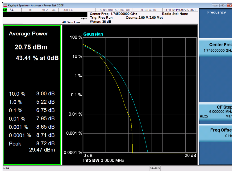
Plot 7-335. PAR Plot (LTE Band 66 - 3MHz 256-QAM - Full RB)
