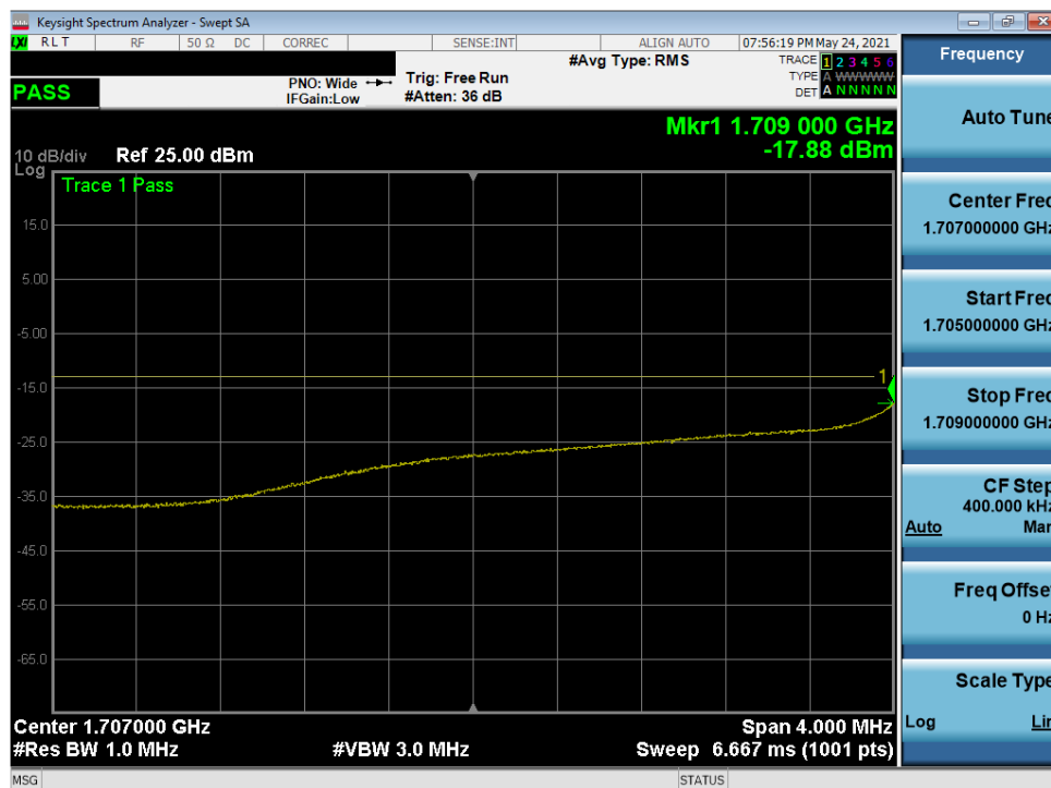
Plot 7-325. Lower Extended Band Edge Plot (WCDMA AWS – Ch. 1312)
