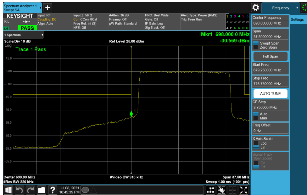
Plot 7-322. Lower Band Edge Plot (NR Band n12 – 15.0MHz DFT-s-OFDM \pi/2 BPSK - Full RB)
