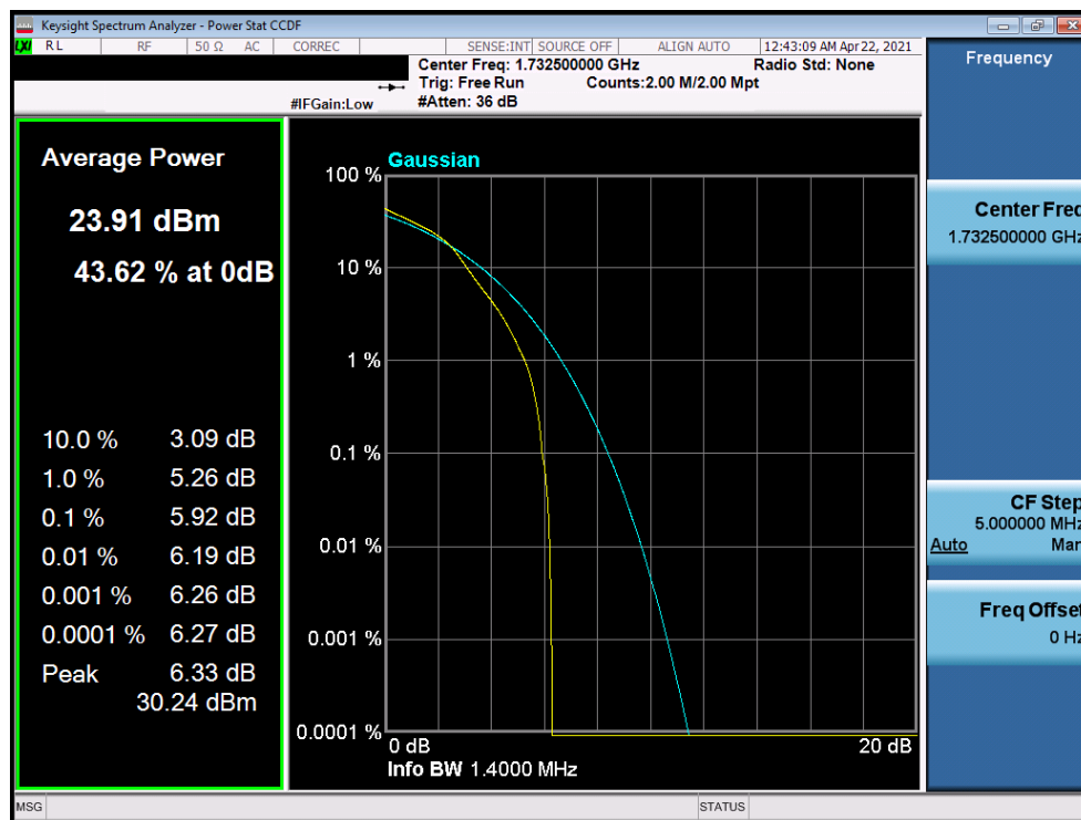
Plot 7-353. PAR Plot (LTE Band 4 - 1.4MHz 16-QAM - Full RB)
