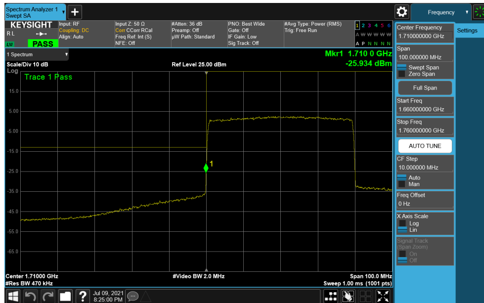
Plot 7-306. Lower Band Edge Plot (NR Band n66 – 40.0MHz CP-OFDM QPSK - Full RB)
