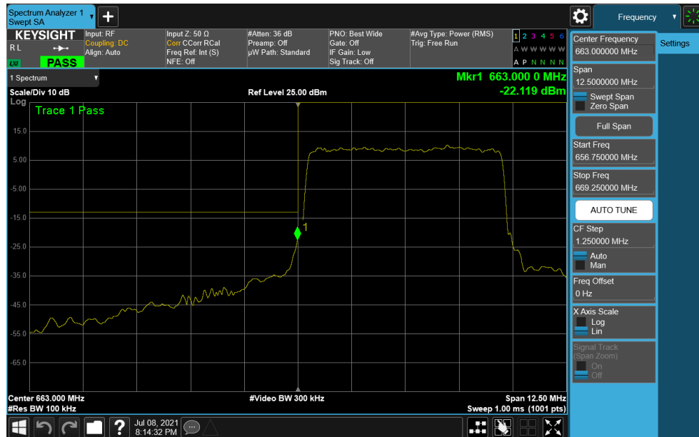
Plot 7-310. Lower Band Edge Plot (NR Band n71 – 5.0MHz DFT-s-OFDM \pi/2 BPSK - Full RB)
