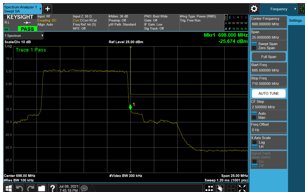
Plot 7-313. Upper Band Edge Plot (NR Band n71 – 10.0MHz CP-OFDM QPSK - Full RB)
