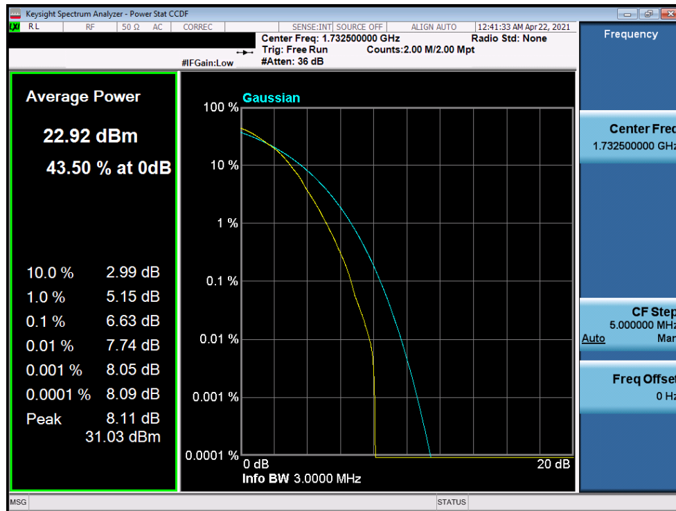
Plot 7-358. PAR Plot (LTE Band 4 - 3MHz 64-QAM - Full RB)
