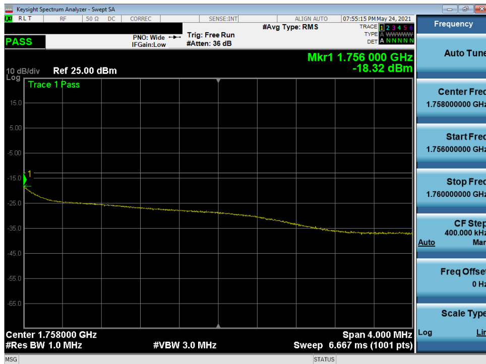
Plot 7-327. Upper Extended Band Edge Plot (WCDMA AWS – Ch. 1513)
