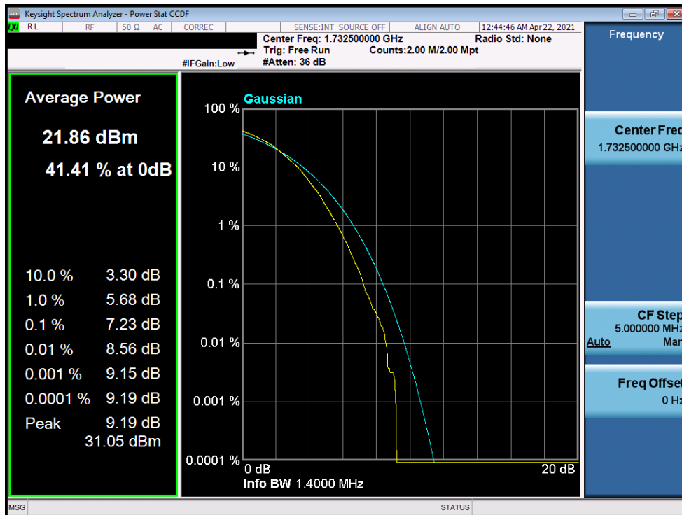
Plot 7-355. PAR Plot (LTE Band 4 - 1.4MHz 256-QAM - Full RB)
