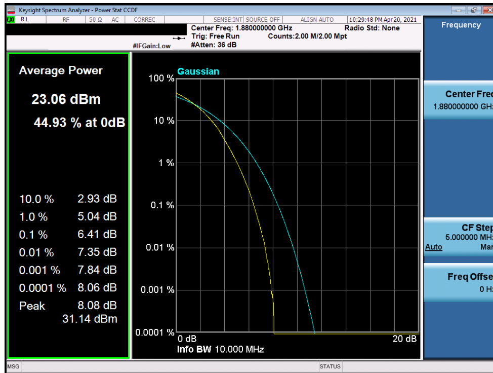
Plot 7-207. PAR Plot (LTE Band 2 - 10MHz 64-QAM - Full RB Configuration)
