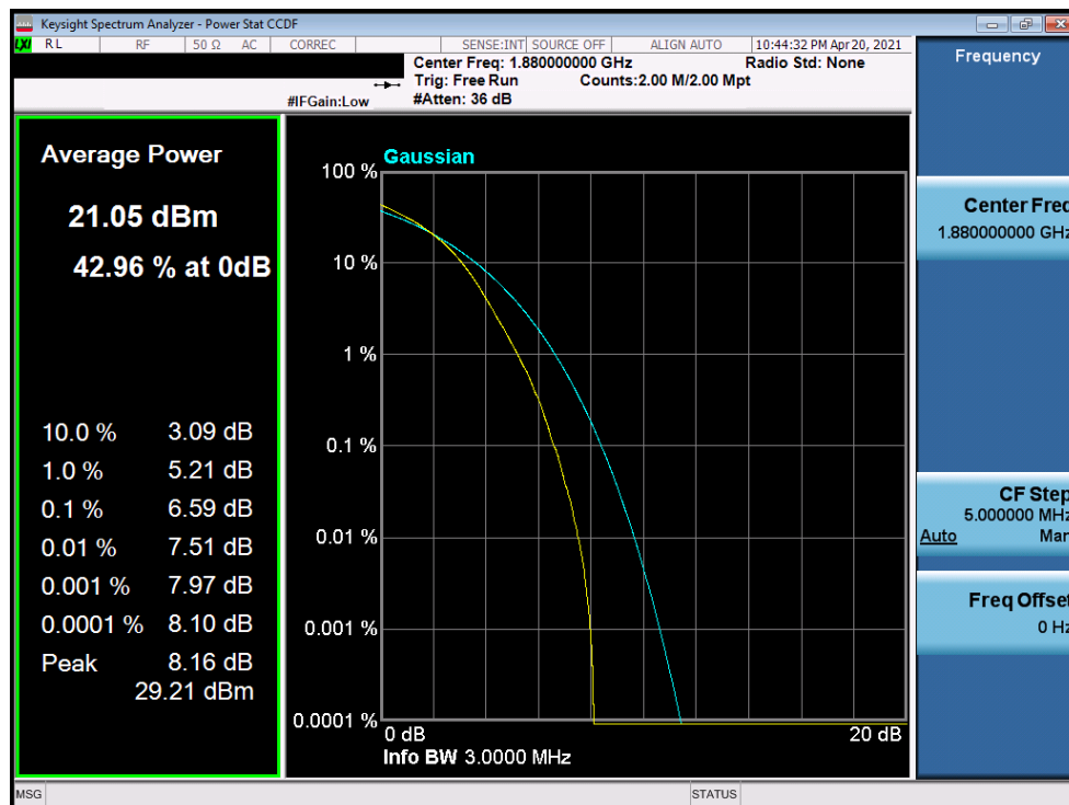
Plot 7-200. PAR Plot (LTE Band 2 - 3MHz 256-QAM - Full RB Configuration)
