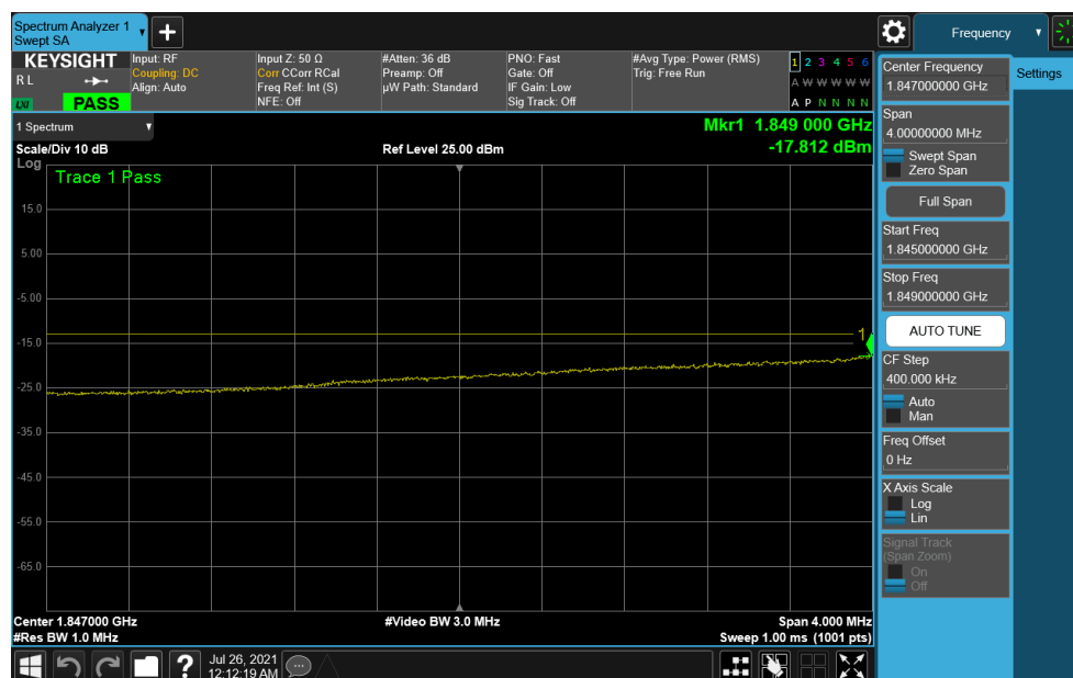
Plot 7-174. Extended Lower Band Edge Plot (NR Band n25 – 20MHz DFT-s-OFDM \pi/2 BPSK – Full RB Configuration)
