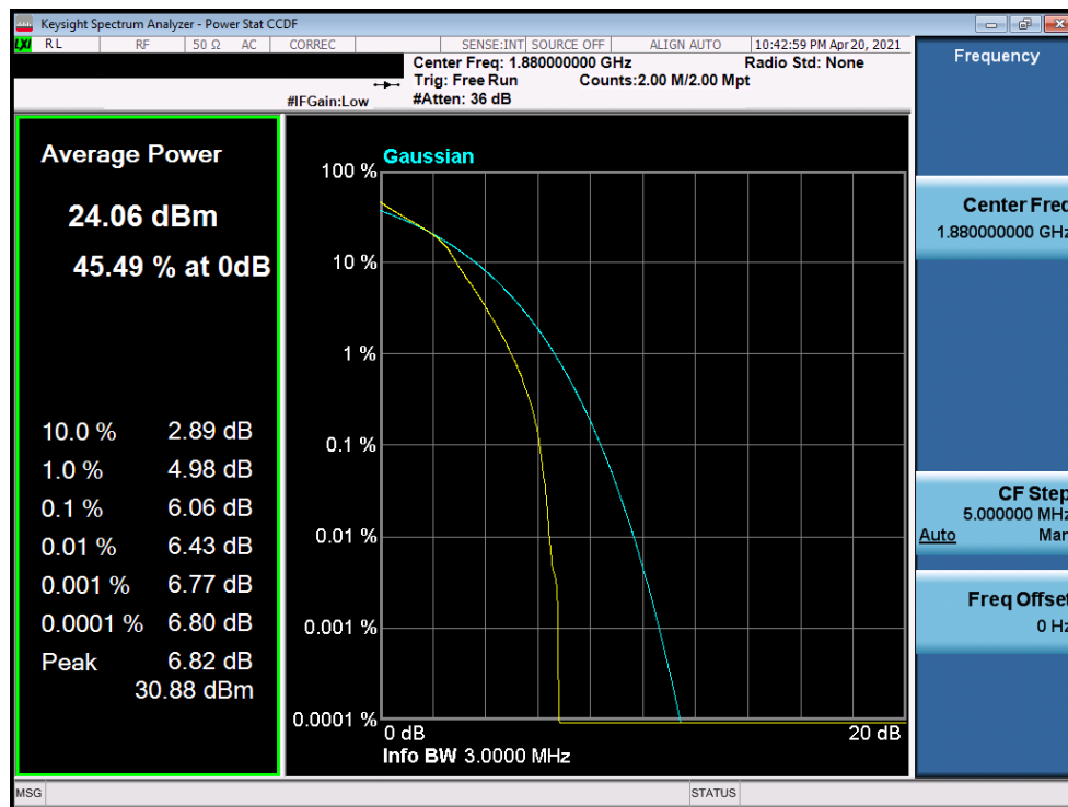
Plot 7-198. PAR Plot (LTE Band 2 - 3MHz 16-QAM - Full RB Configuration)
