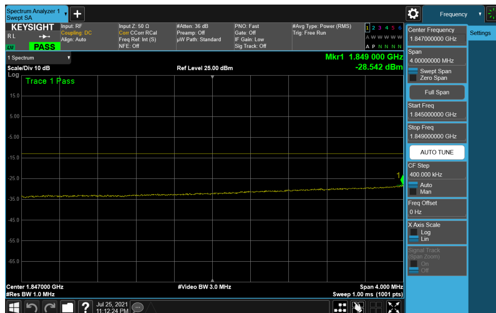
Plot 7-182. Extended Lower Band Edge Plot (NR Band n25 – 30MHz DFT-s-OFDM \pi/2 BPSK – Full RB Configuration)
