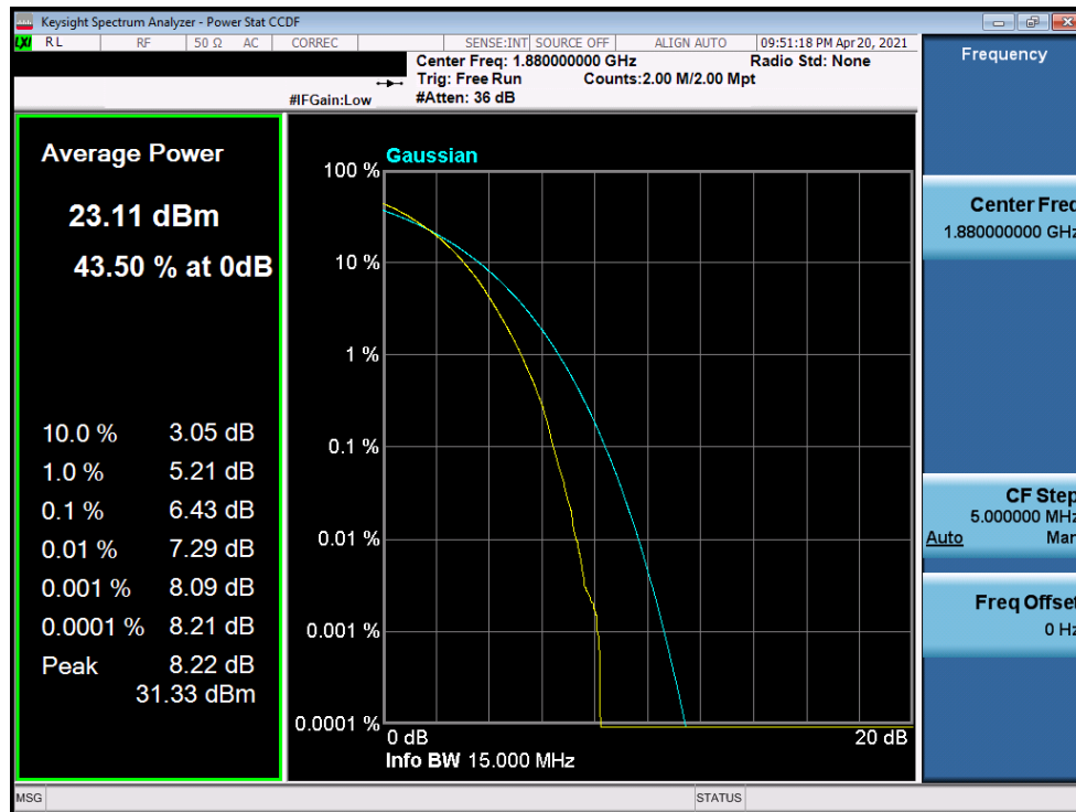
Plot 7-211. PAR Plot (LTE Band 2 - 15MHz 64-QAM - Full RB Configuration)
