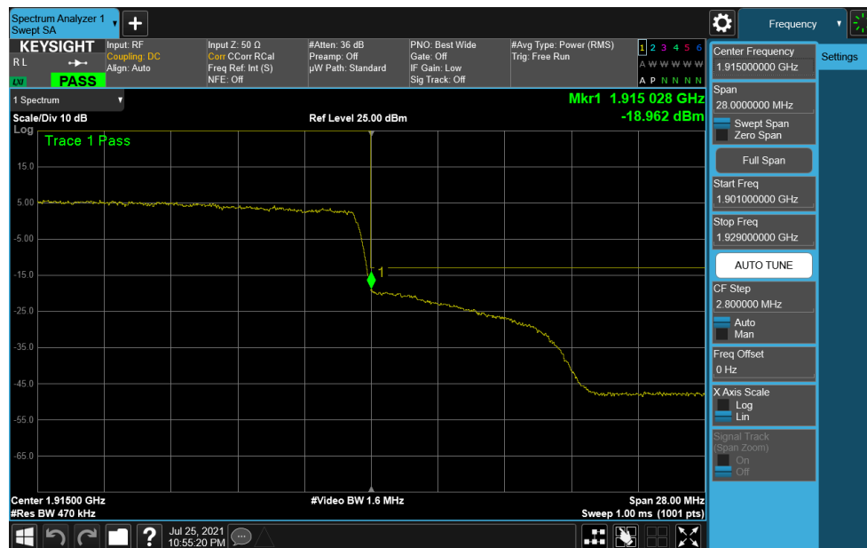
Plot 7-187. Upper Band Edge Plot (NR Band n25 – 40MHz DFT-s-OFDM \pi/2 BPSK – Full RB Configuration)
