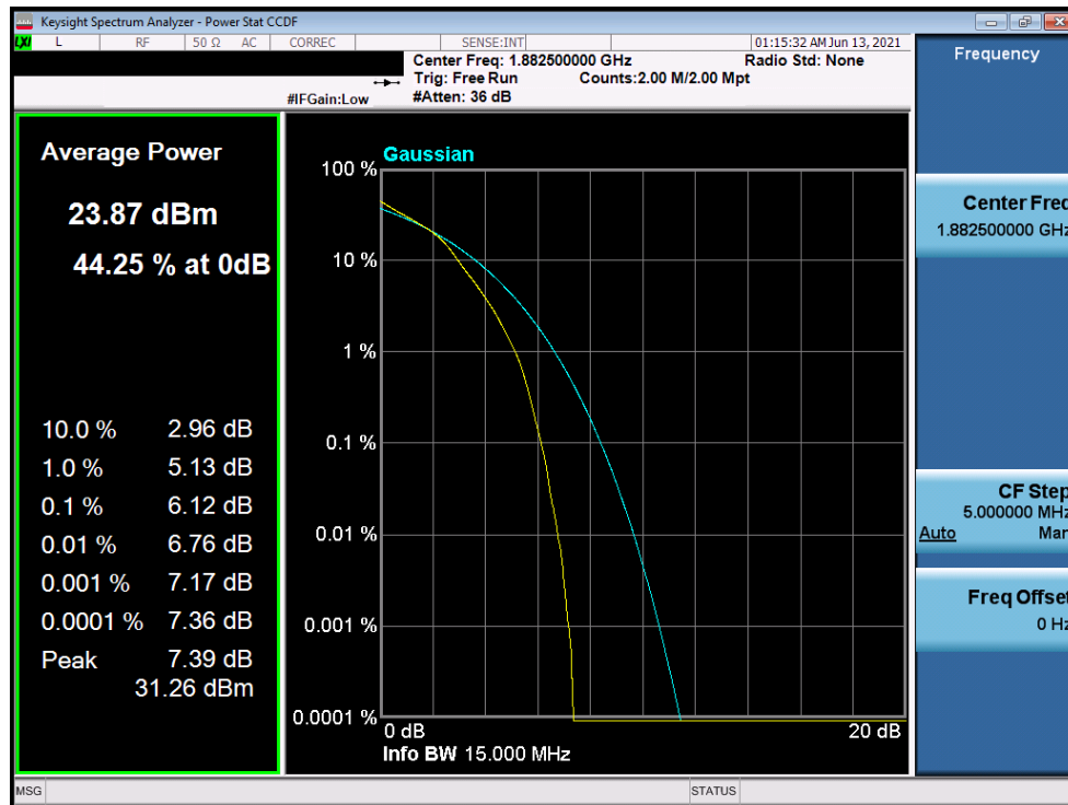
Plot 7-234. PAR Plot (LTE Band 25/2 - 15MHz 16-QAM - Full RB Configuration)
