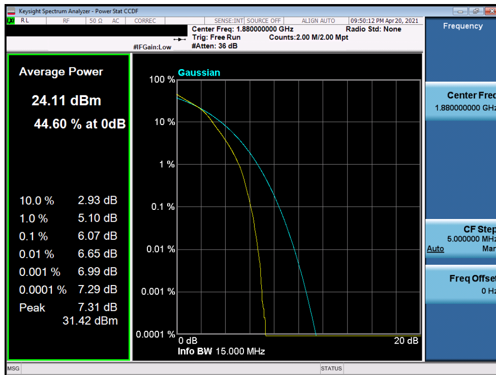
Plot 7-210. PAR Plot (LTE Band 2 - 15MHz 16-QAM - Full RB Configuration)
