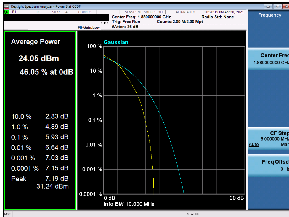
Plot 7-206. PAR Plot (LTE Band 2 - 10MHz 16-QAM - Full RB Configuration)
