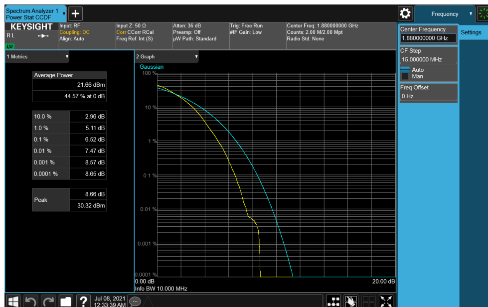
Plot 7-250. PAR Plot (NR Band n2 - 10.0MHz CP-OFDM 256-QAM - Full RB)
