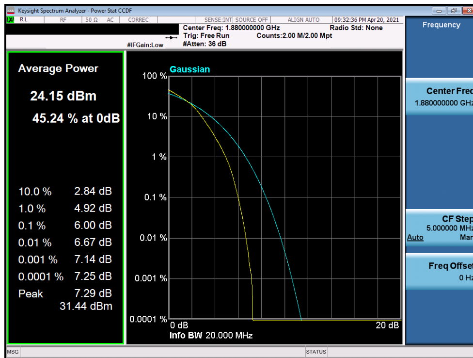
Plot 7-214. PAR Plot (LTE Band 2 - 20MHz 16-QAM - Full RB Configuration)
