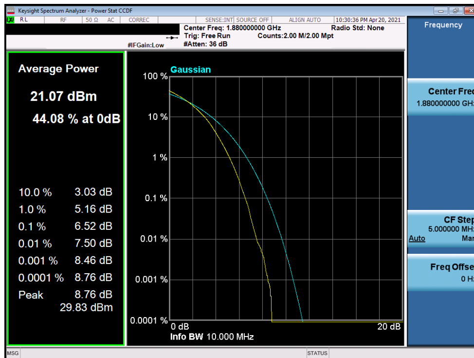
Plot 7-208. PAR Plot (LTE Band 2 - 10MHz 256-QAM - Full RB Configuration)
