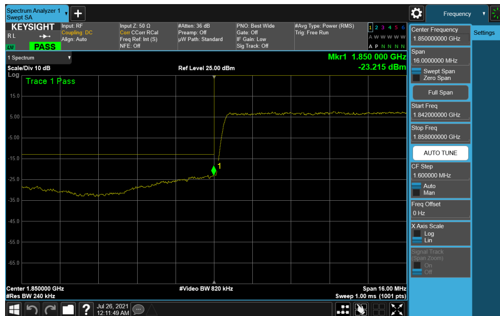
Plot 7-173. Lower Band Edge Plot (NR Band n25 – 20MHz DFT-s-OFDM \pi/2 BPSK – Full RB Configuration)
