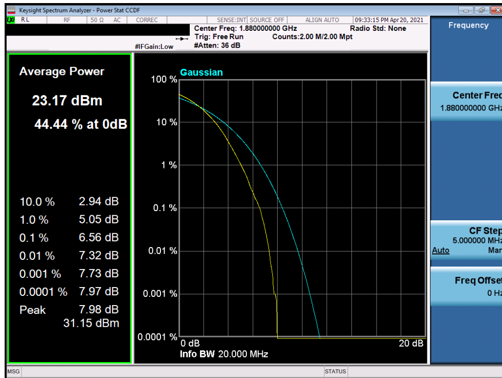
Plot 7-215. PAR Plot (LTE Band 2 - 20MHz 64-QAM - Full RB Configuration)
