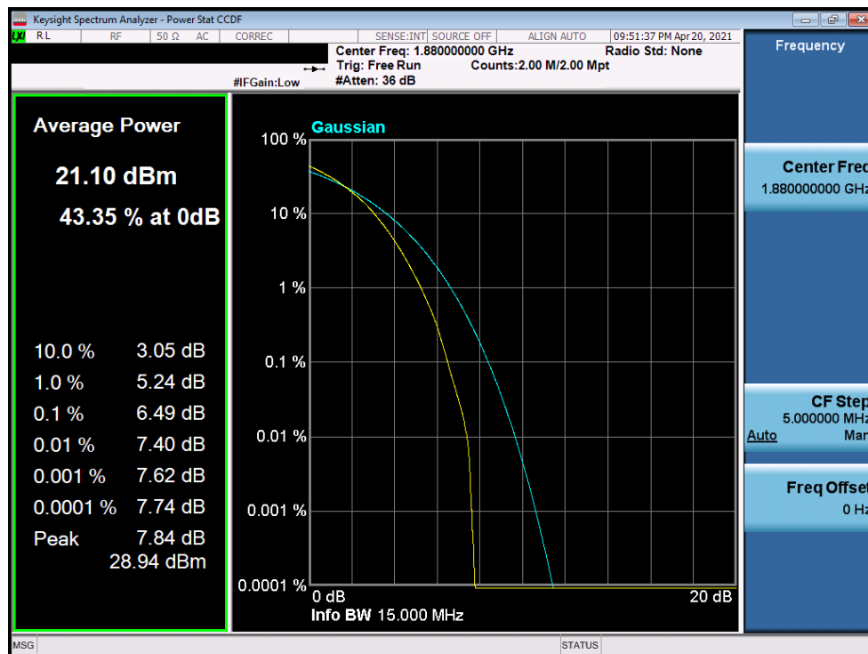
Plot 7-212. PAR Plot (LTE Band 2 - 15MHz 256-QAM - Full RB Configuration)
