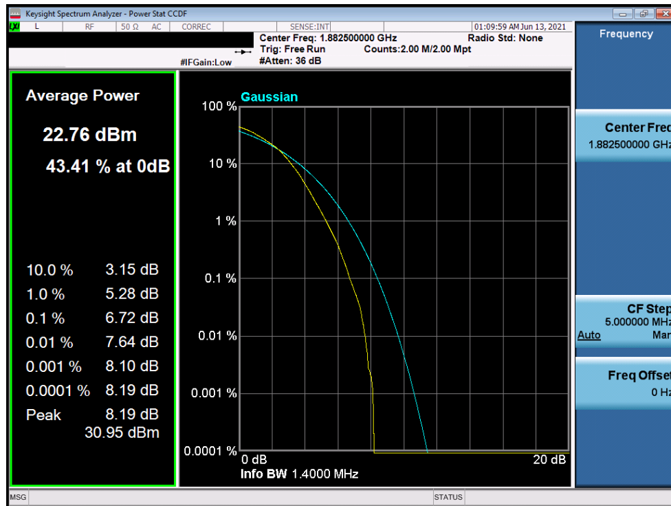
Plot 7-219. PAR Plot (LTE Band 25/2 - 1.4MHz 64-QAM - Full RB Configuration)
