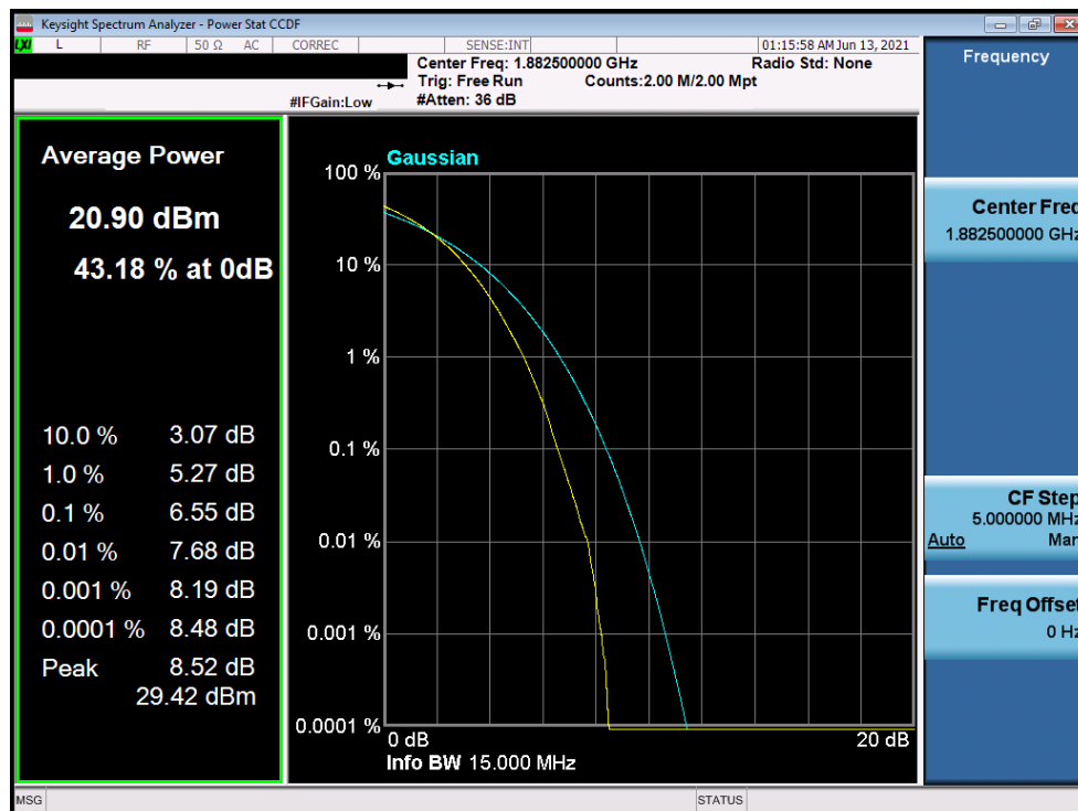
Plot 7-236. PAR Plot (LTE Band 25/2 - 15MHz 256-QAM - Full RB Configuration)
