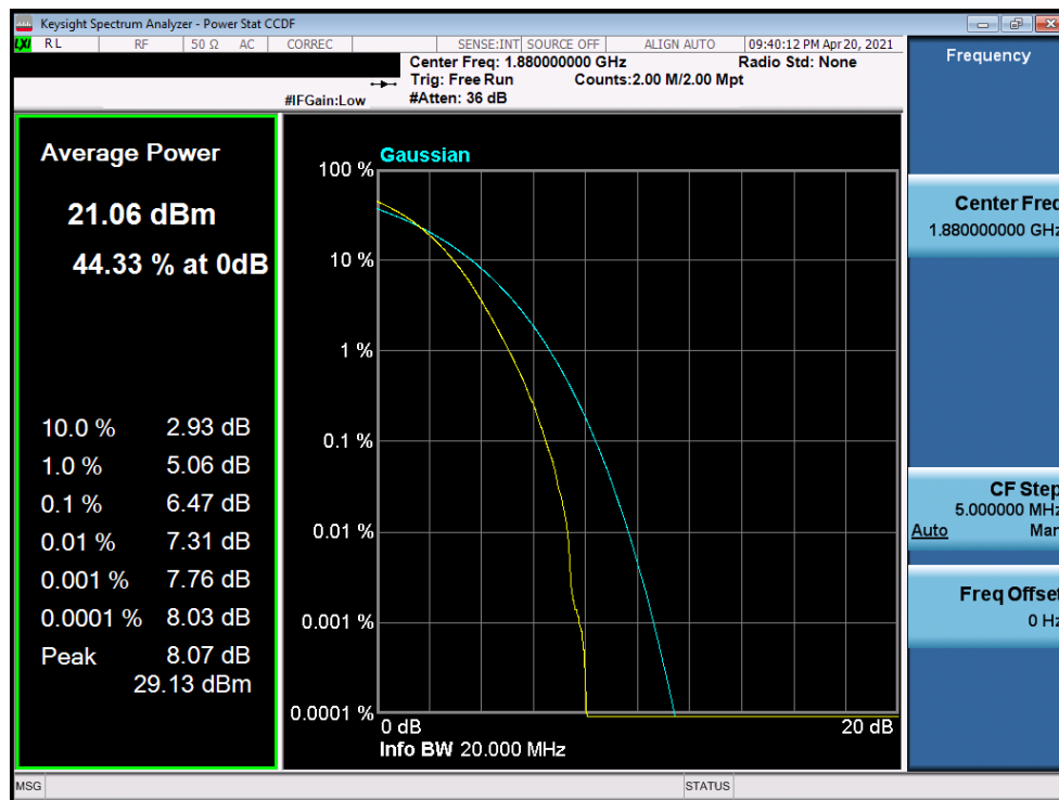
Plot 7-216. PAR Plot (LTE Band 2 - 20MHz 256-QAM - Full RB Configuration)
