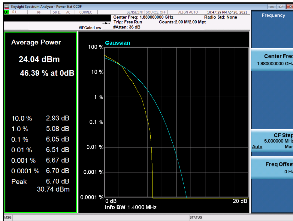
Plot 7-194. PAR Plot (LTE Band 2 - 1.4MHz 16-QAM - Full RB Configuration)
