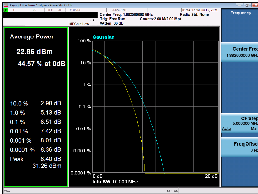
Plot 7-231. PAR Plot (LTE Band 25/2 - 10MHz 64-QAM - Full RB Configuration)
