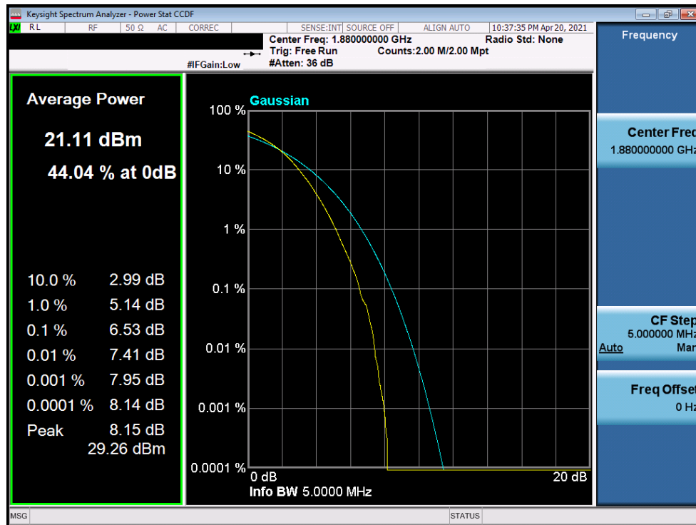
Plot 7-204. PAR Plot (LTE Band 2 - 5MHz 256-QAM - Full RB Configuration)
