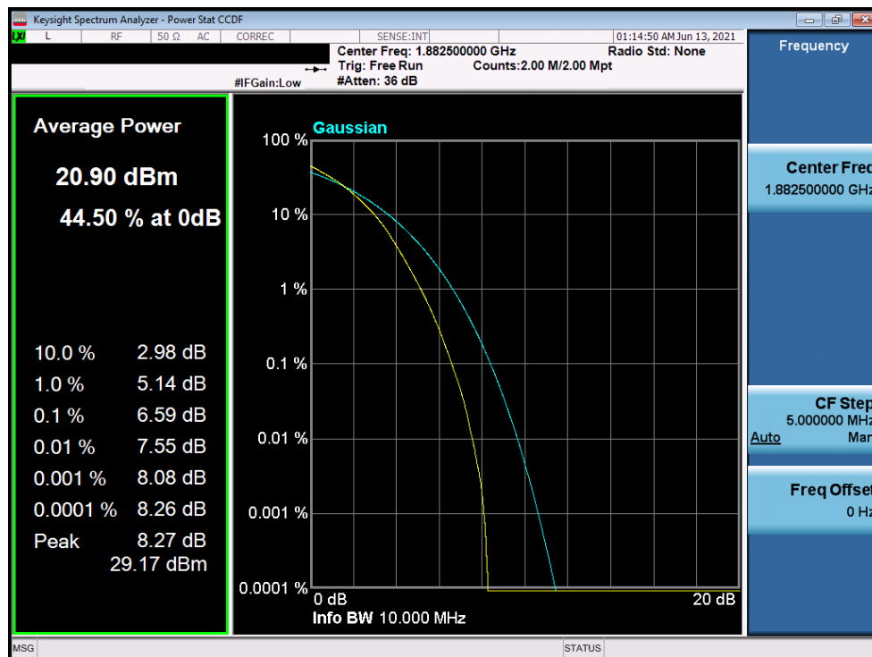
Plot 7-232. PAR Plot (LTE Band 25/2 - 10MHz 256-QAM - Full RB Configuration)
