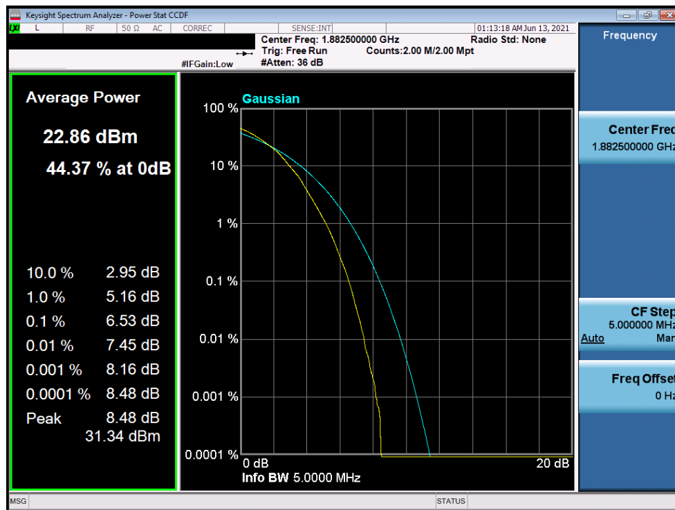
Plot 7-227. PAR Plot (LTE Band 25/2 - 5MHz 64-QAM - Full RB Configuration)
