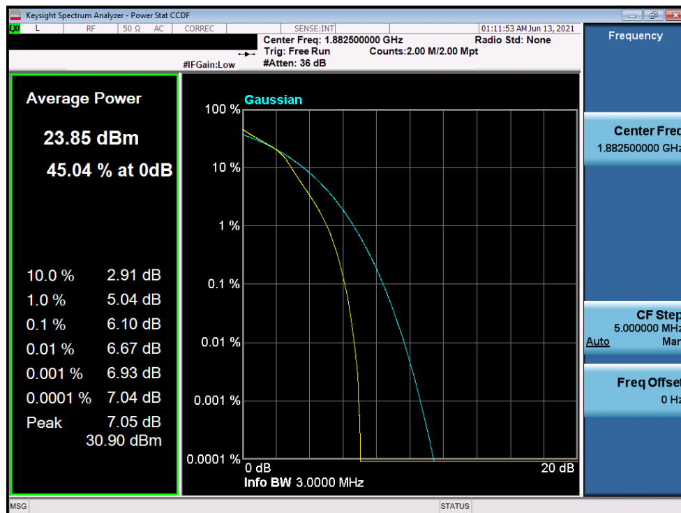
Plot 7-222. PAR Plot (LTE Band 25/2 - 3MHz 16-QAM - Full RB Configuration)
