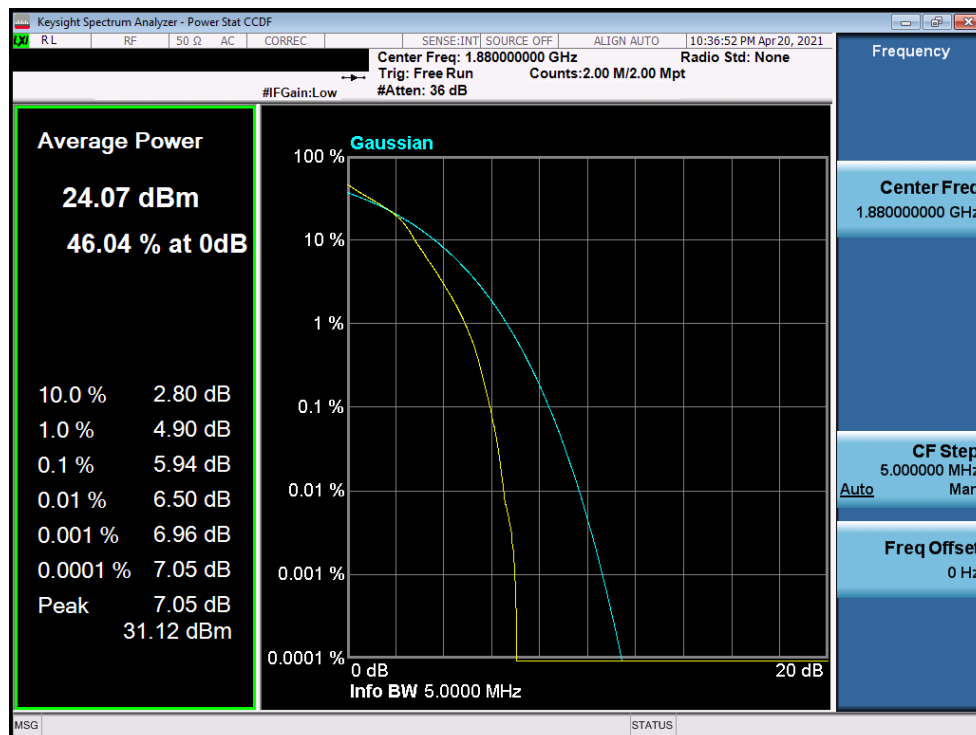
Plot 7-202. PAR Plot (LTE Band 2 - 5MHz 16-QAM - Full RB Configuration)
