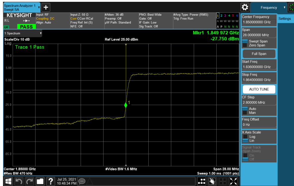
Plot 7-185. Lower Band Edge Plot (NR Band n25 – 40MHz DFT-s-OFDM \pi/2 BPSK – Full RB Configuration)
