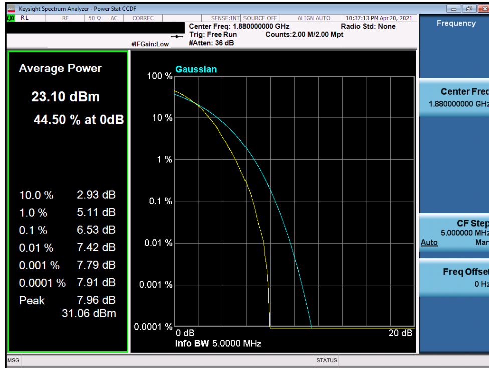
Plot 7-203. PAR Plot (LTE Band 2 - 5MHz 64-QAM - Full RB Configuration)
