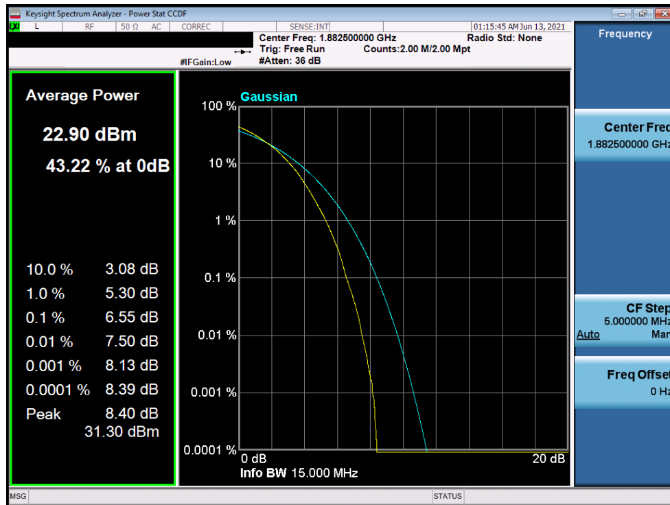
Plot 7-235. PAR Plot (LTE Band 25/2 - 15MHz 64-QAM - Full RB Configuration)
