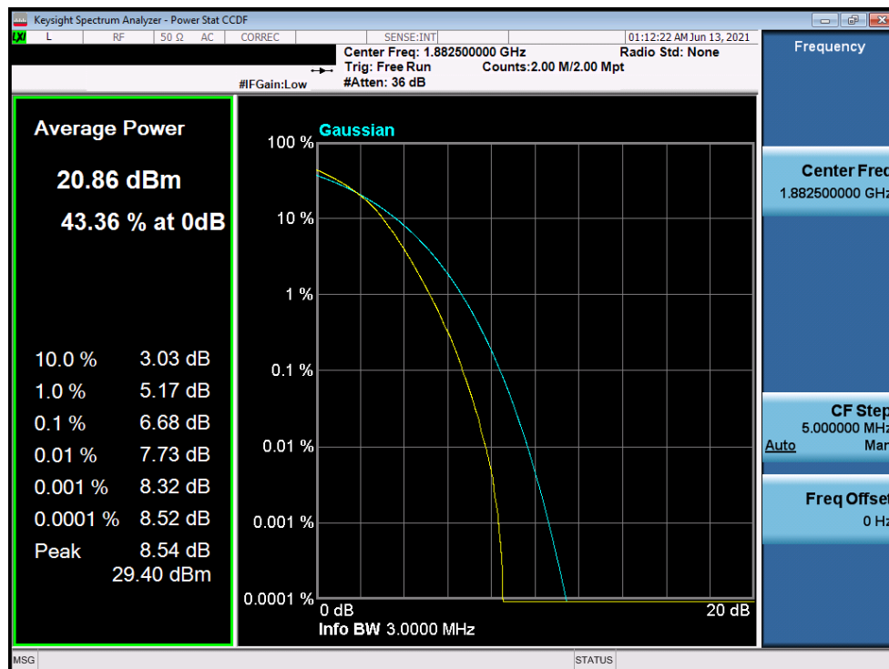
Plot 7-224. PAR Plot (LTE Band 25/2 - 3MHz 256-QAM - Full RB Configuration)
