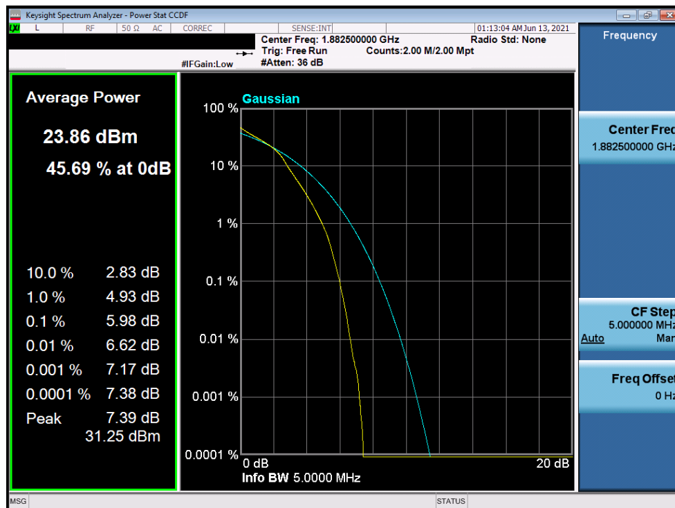
Plot 7-226. PAR Plot (LTE Band 25/2 - 5MHz 16-QAM - Full RB Configuration)
