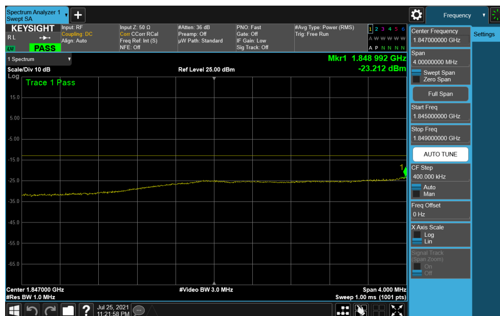
Plot 7-178. Extended Lower Band Edge Plot (NR Band n25 – 25MHz DFT-s-OFDM \pi/2 BPSK – Full RB Configuration)
