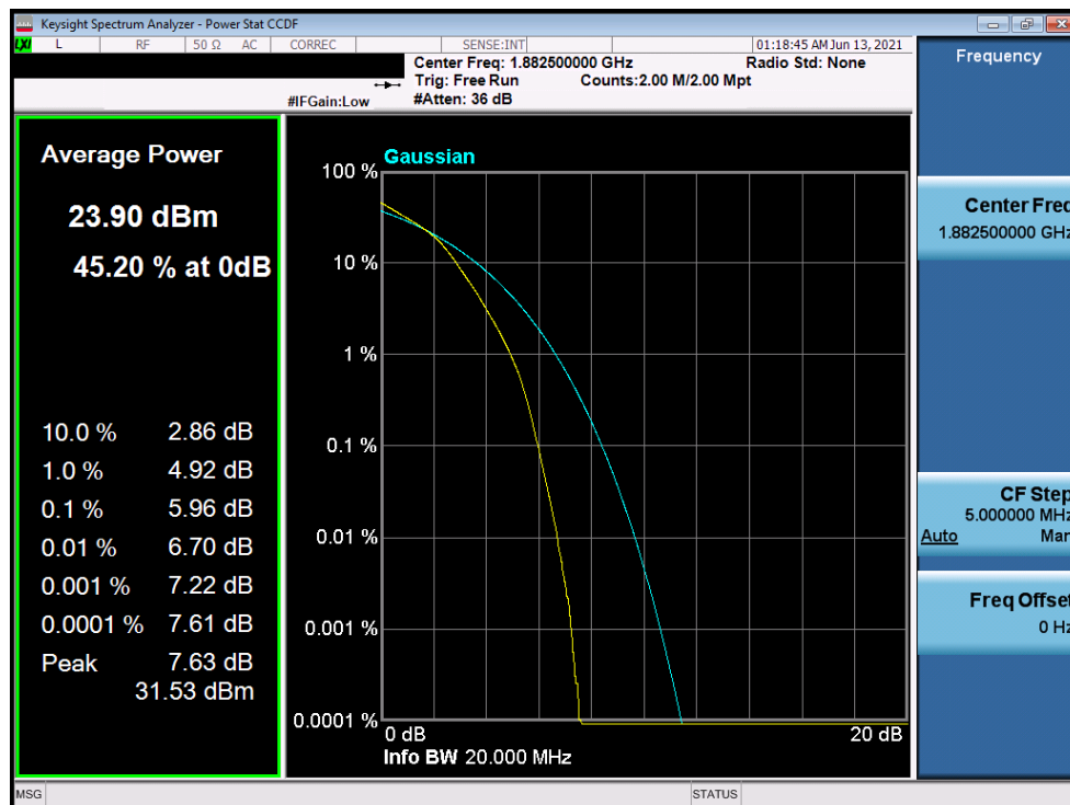
Plot 7-238. PAR Plot (LTE Band 25/2 - 20MHz 16-QAM - Full RB Configuration)
