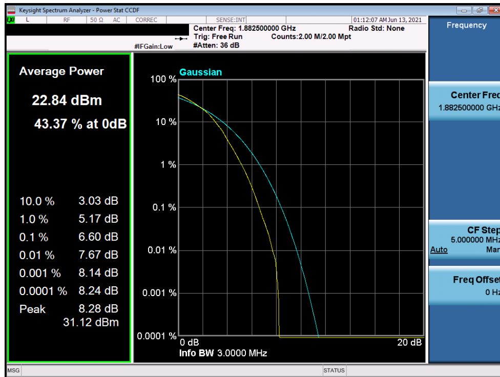
Plot 7-223. PAR Plot (LTE Band 25/2 - 3MHz 64-QAM - Full RB Configuration)
