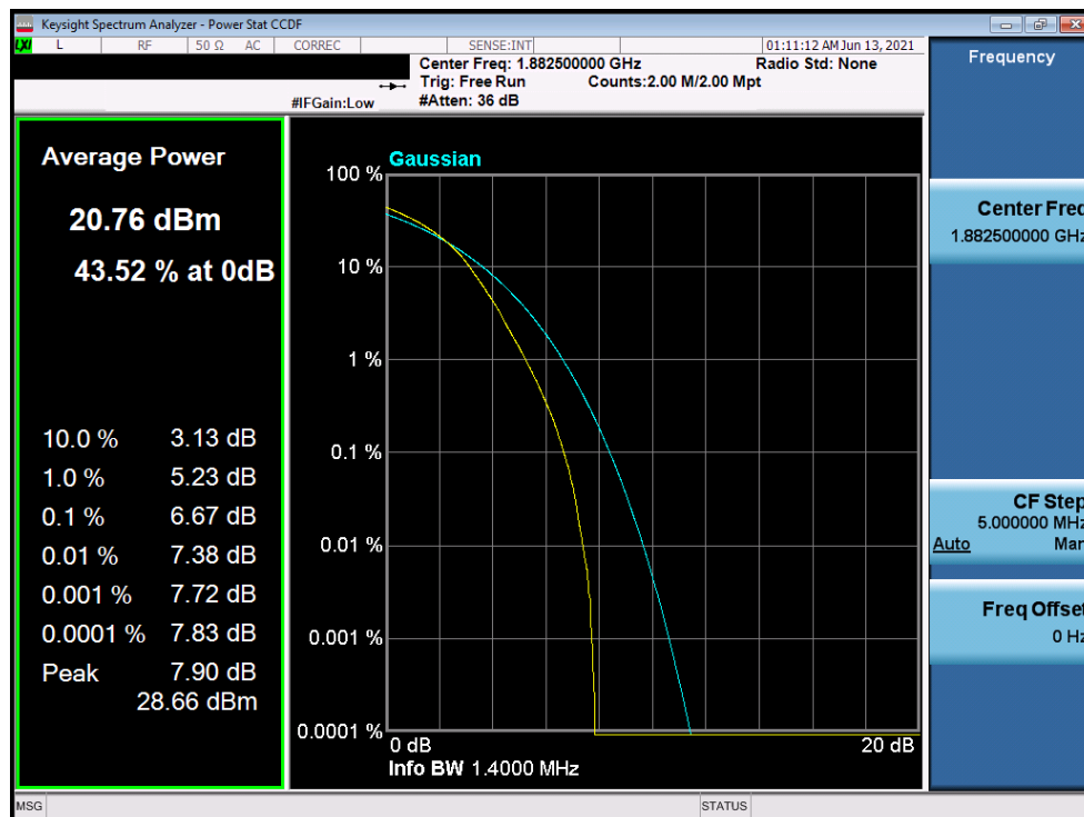
Plot 7-220. PAR Plot (LTE Band 25/2 - 1.4MHz 256-QAM - Full RB Configuration)
