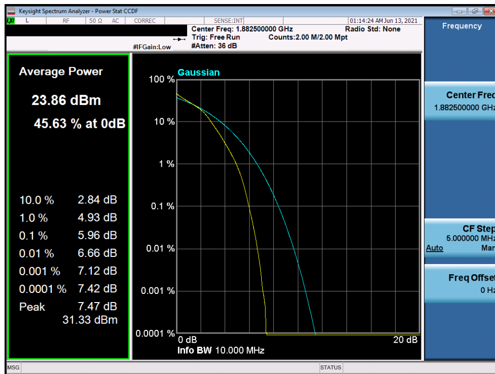
Plot 7-230. PAR Plot (LTE Band 25/2 - 10MHz 16-QAM - Full RB Configuration)
