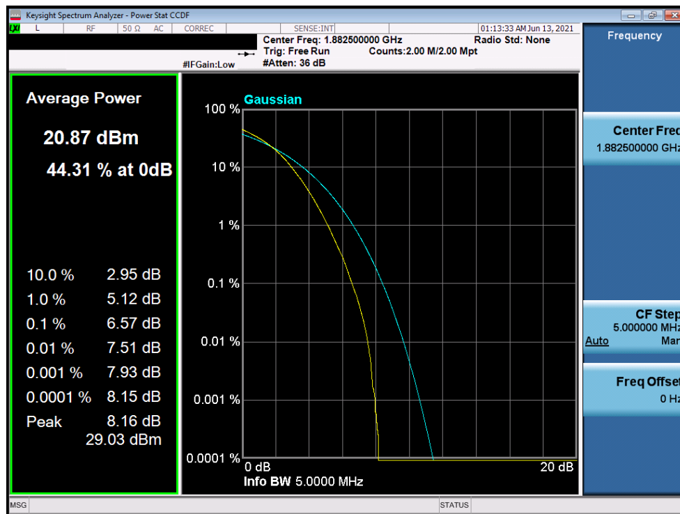
Plot 7-228. PAR Plot (LTE Band 25/2 - 5MHz 256-QAM - Full RB Configuration)
