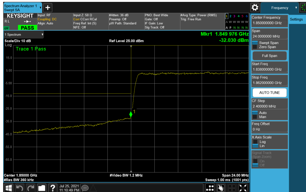
Plot 7-181. Lower Band Edge Plot (NR Band n25 – 30MHz DFT-s-OFDM \pi/2 BPSK – Full RB Configuration)
