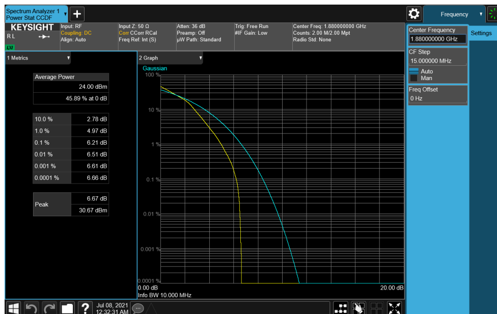
Plot 7-248. PAR Plot (NR Band n2 - 10.0MHz CP-OFDM 16-QAM - Full RB)
