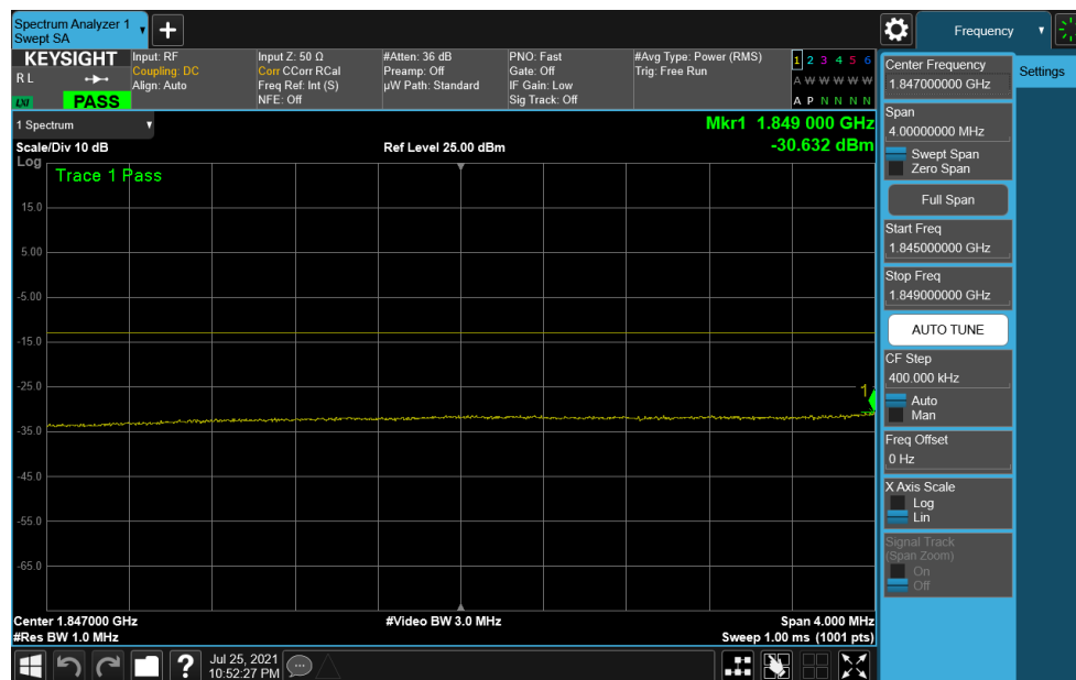
Plot 7-186. Extended Lower Band Edge Plot (NR Band n25 – 40MHz DFT-s-OFDM \pi/2 BPSK – Full RB Configuration)
