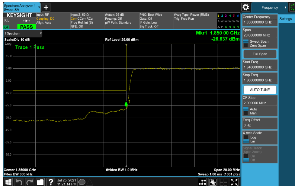
Plot 7-177. Lower Band Edge Plot (NR Band n25 – 25MHz DFT-s-OFDM \pi/2 BPSK – Full RB Configuration)
