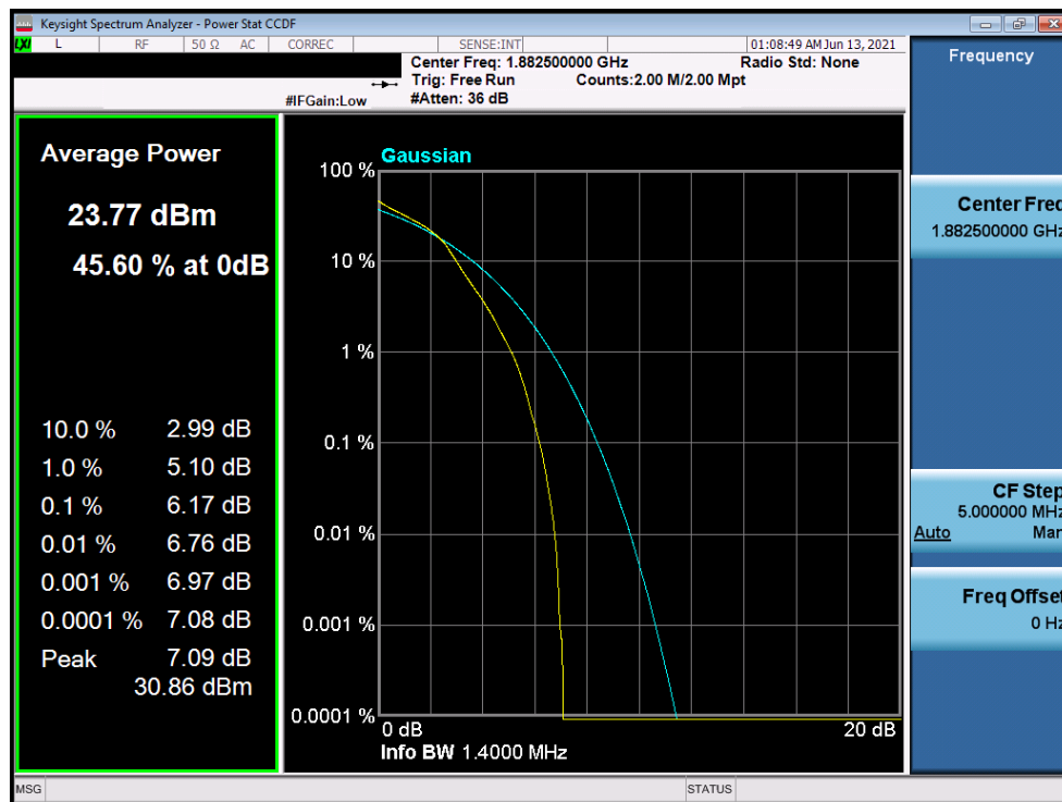
Plot 7-218. PAR Plot (LTE Band 25/2 - 1.4MHz 16-QAM - Full RB Configuration)
