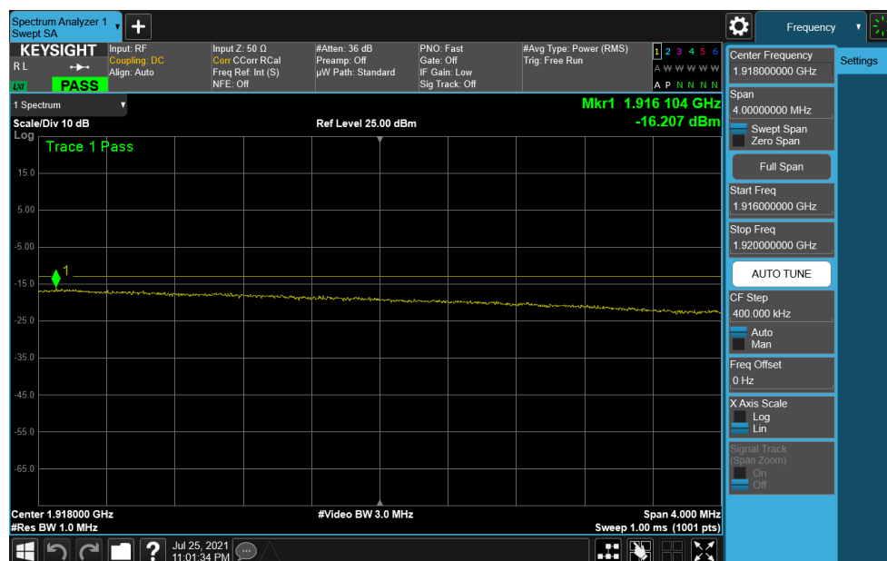
Plot 7-188. Extended Upper Band Edge Plot (NR Band n25 – 40MHz DFT-s-OFDM \pi/2 BPSK – Full RB Configuration)
