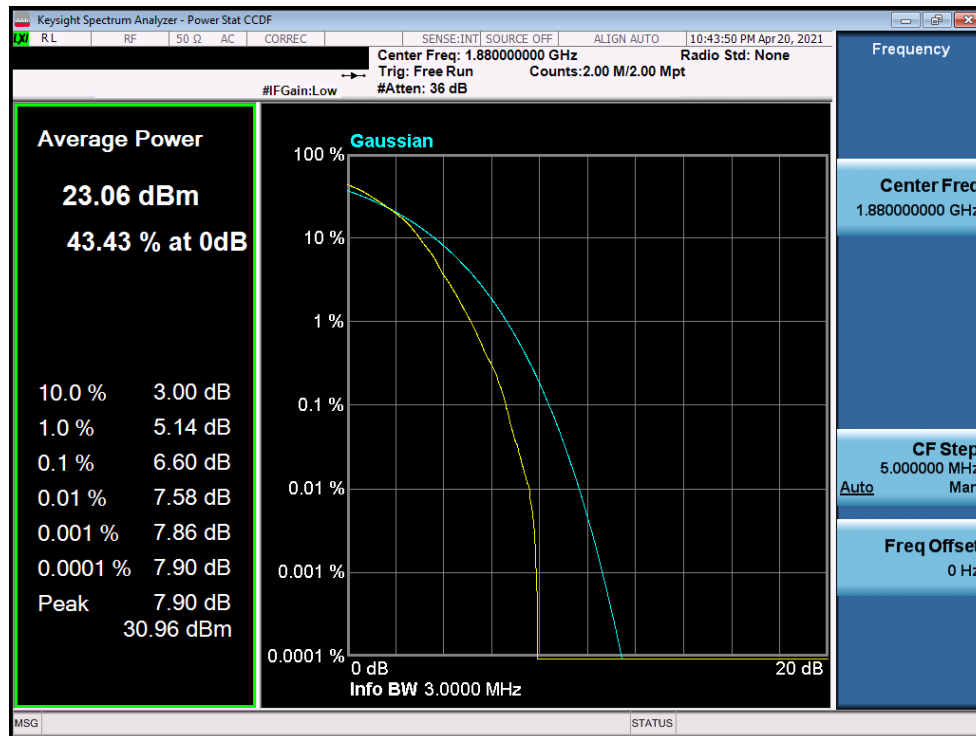
Plot 7-199. PAR Plot (LTE Band 2 - 3MHz 64-QAM - Full RB Configuration)
