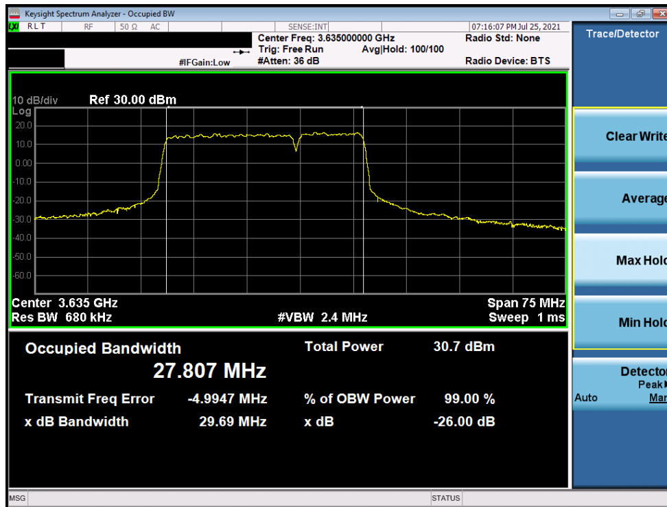
Plot 7-21. Occupied Bandwidth Plot (ULCA LTE Band 48 - 20+10MHz QPSK - Full RB Configuration)
