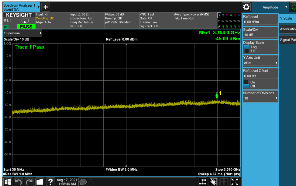
Plot 7-45. Conducted Spurious Plot (ULCA LTE Band 48 - 20+20MHz QPSK - Low Channel)
