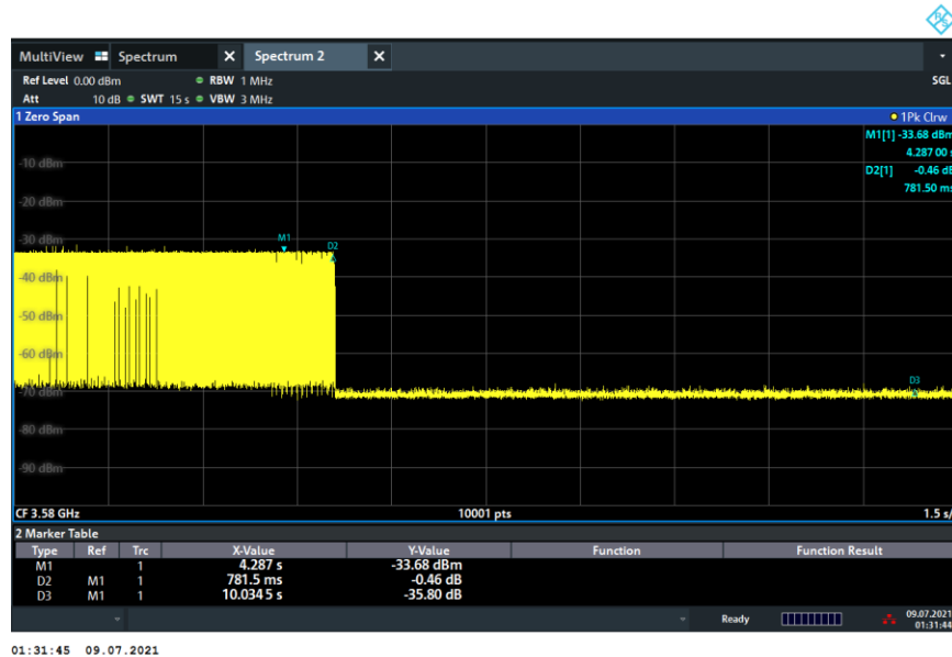
Plot 7-83. Run#1 End User Device Discontinues Operations within 10s
