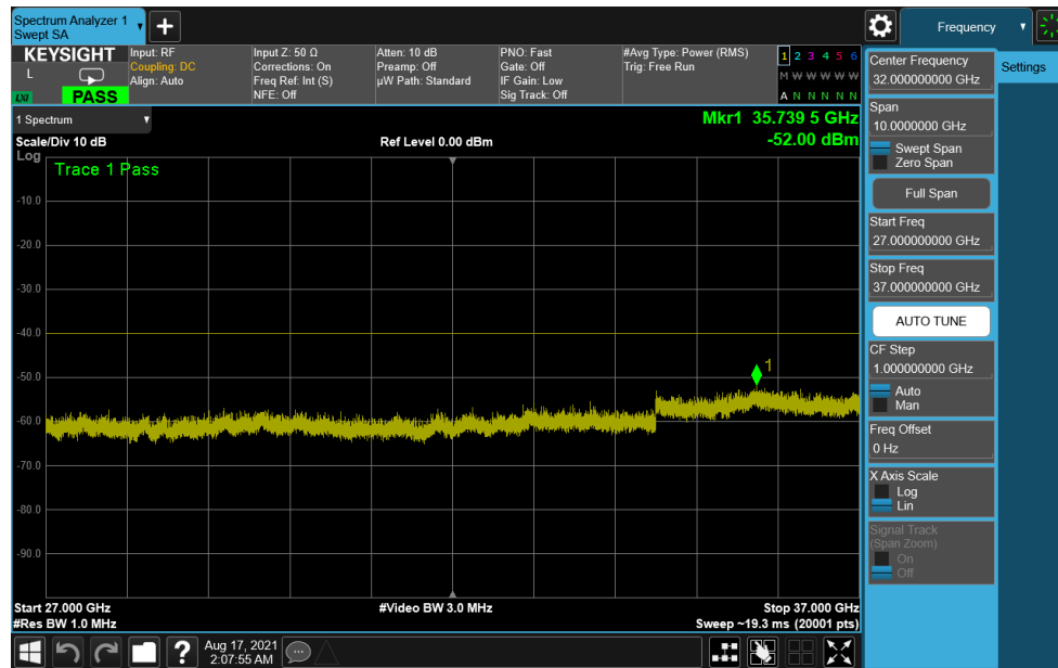
Plot 7-56. Conducted Spurious Plot (ULCA LTE Band 48 - 20+20MHz QPSK - High Channel)
