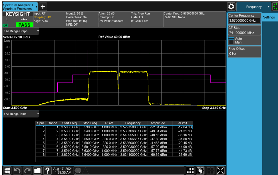
Plot 7-69. ACP Plot (LTE Band 48 – 20+20MHz QPSK - Low Channel)
