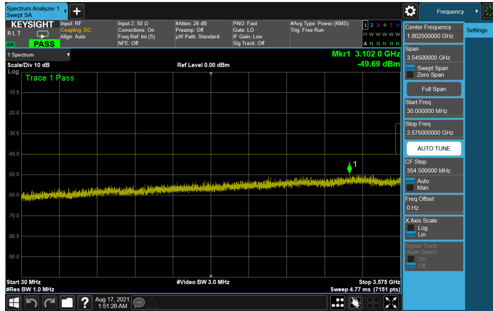
Plot 7-49. Conducted Spurious Plot (ULCA LTE Band 48 - 20+20MHz QPSK - Mid Channel)
