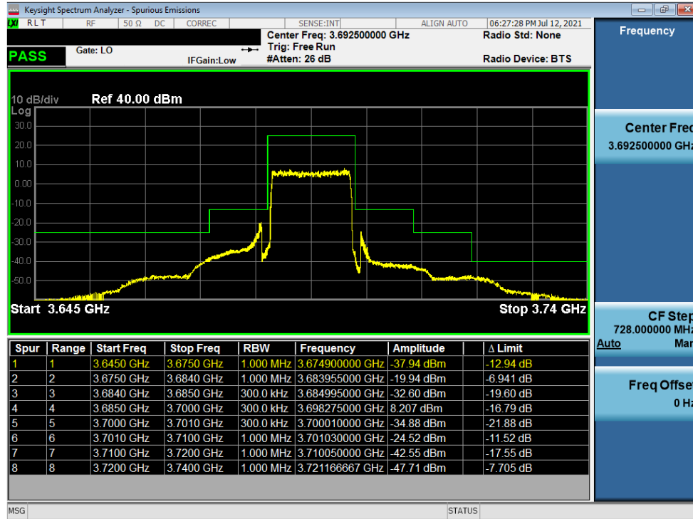
Plot 7-65. ACP Plot (LTE Band 48 - 15MHz QPSK - High Channel)
