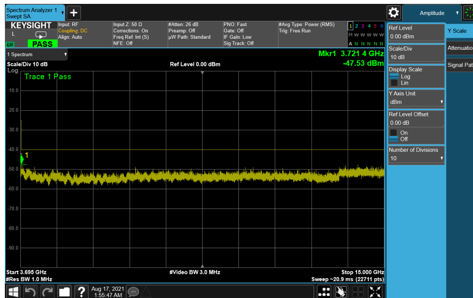
Plot 7-50. Conducted Spurious Plot (ULCA LTE Band 48 - 20+20MHz QPSK - Mid Channel)
