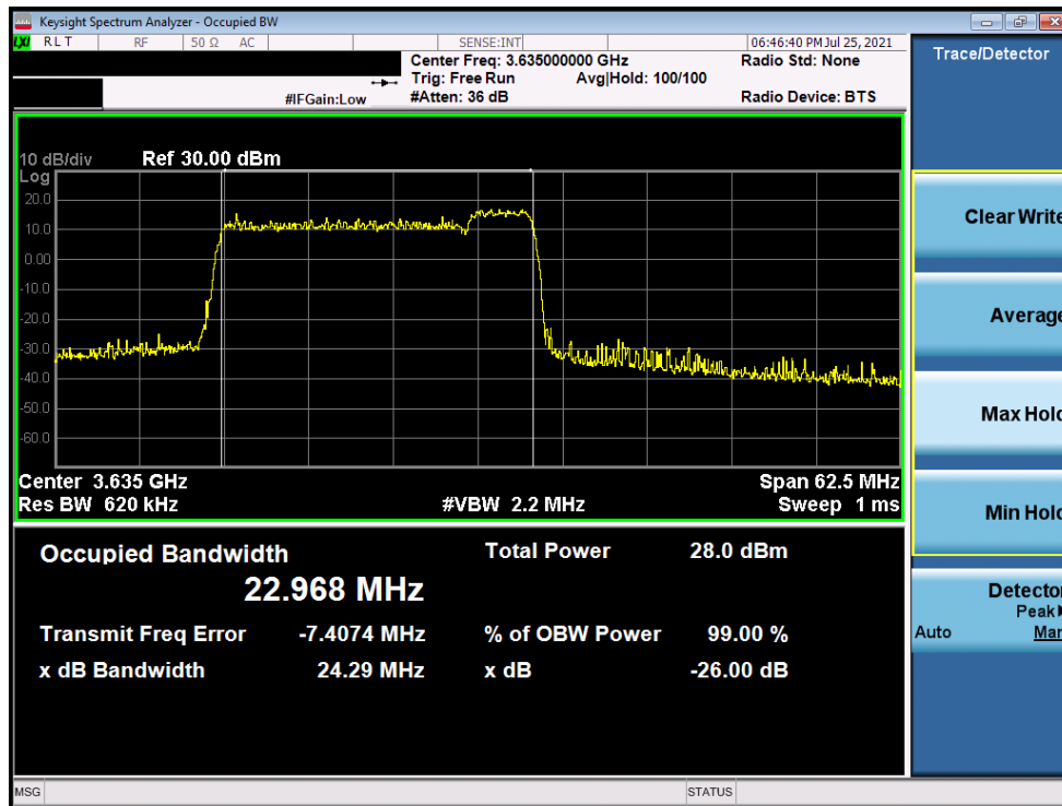
Plot 7-19. Occupied Bandwidth Plot (ULCA LTE Band 48 - 20+5MHz 64-QAM - Full RB Configuration)
