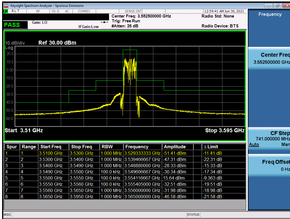
Plot 7-57. ACP Plot (LTE Band 48 - 5MHz QPSK - Low Channel)
