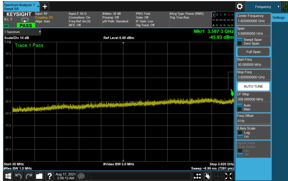
Plot 7-53. Conducted Spurious Plot (ULCA LTE Band 48 - 20+20MHz QPSK - High Channel)
