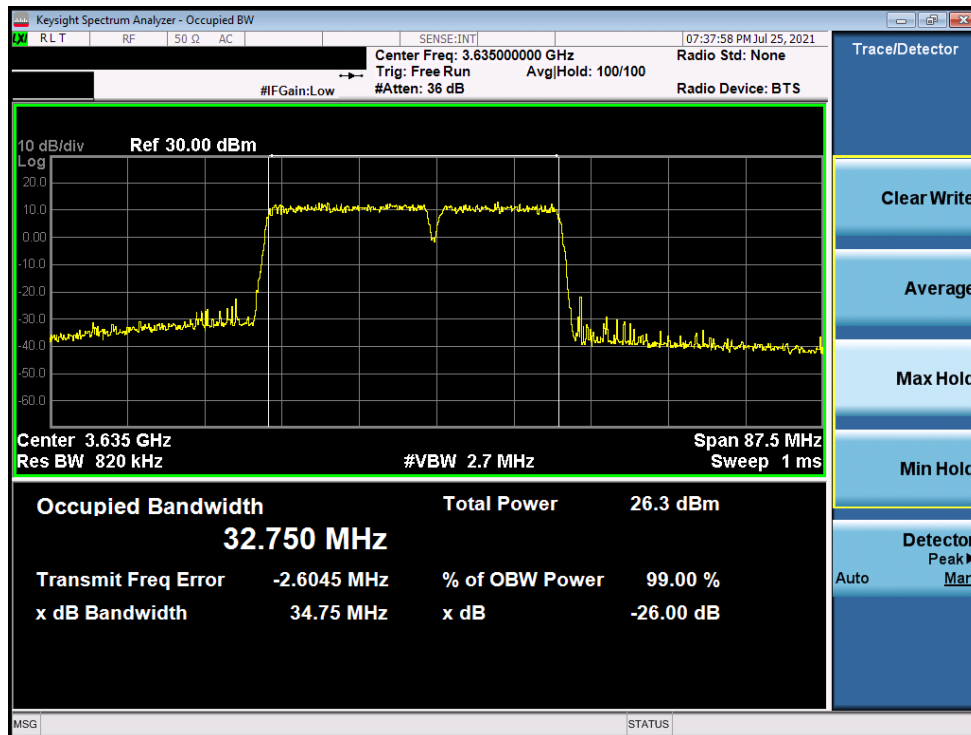
Plot 7-28. Occupied Bandwidth Plot (ULCA LTE Band 48 - 20+15MHz 256-QAM - Full RB Configuration)
