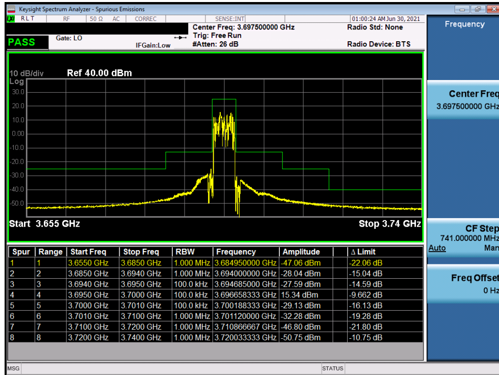
Plot 7-59. ACP Plot (LTE Band 48 - 5MHz QPSK - High Channel)
