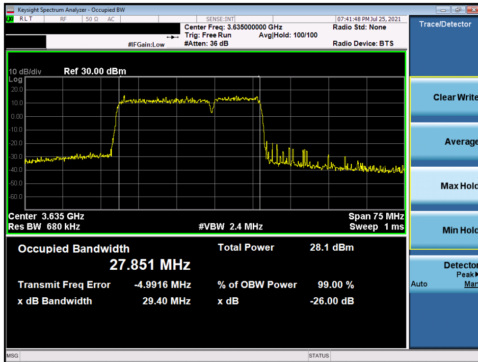
Plot 7-23. Occupied Bandwidth Plot (ULCA LTE Band 48 - 20+10MHz 64-QAM - Full RB Configuration)
