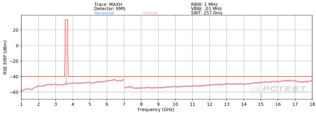
Plot 7-72. Radiated Spurious Plot 1 – 18GHz (LTE Band 48)
