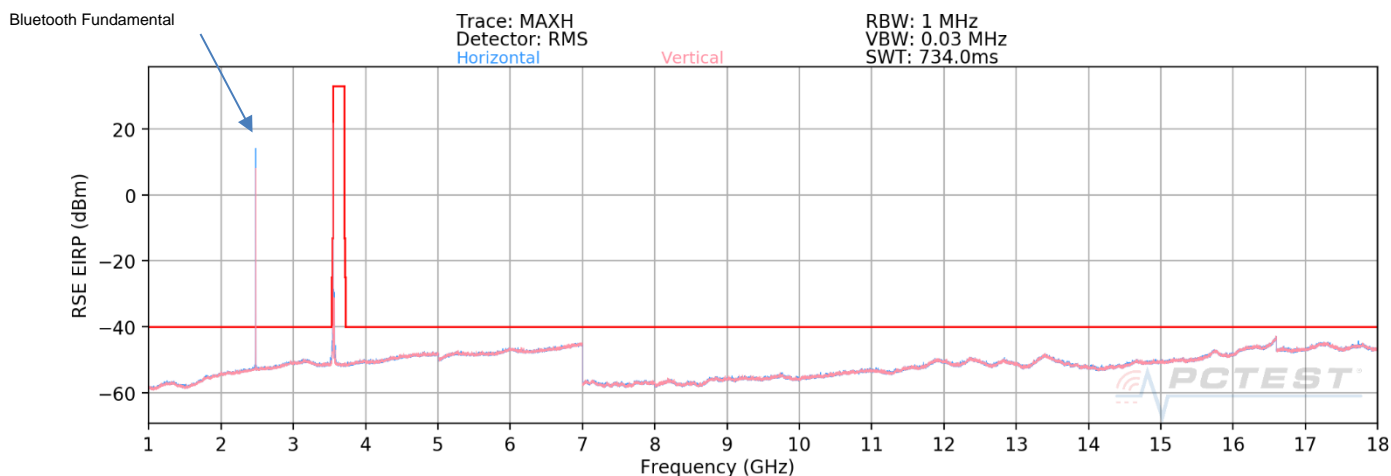
Plot 7-79. Radiated Spurious Emissions - Simultaneous Transmission 1-18GHz
