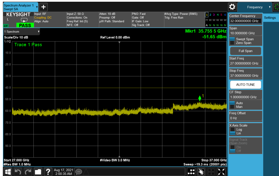
Plot 7-48. Conducted Spurious Plot (ULCA LTE Band 48 - 20+20MHz QPSK - Low Channel)
