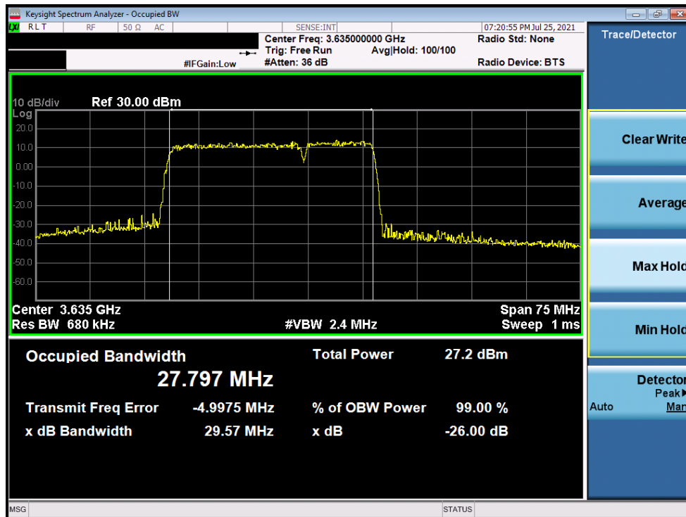
Plot 7-24. Occupied Bandwidth Plot (ULCA LTE Band 48 - 20+10MHz 256-QAM - Full RB Configuration)
