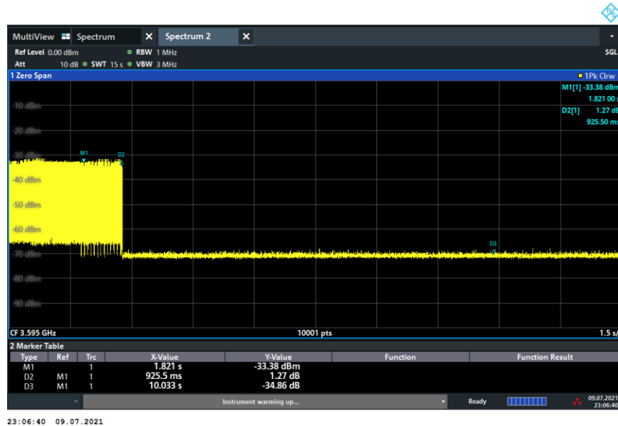
Plot 7-85. Run#2 End User Device Discontinues Operations within 10s
