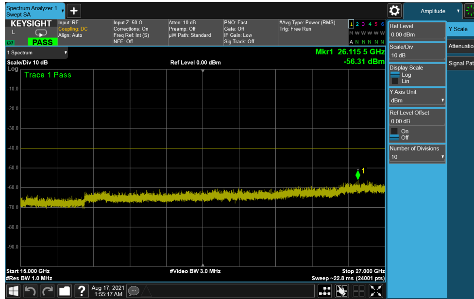
Plot 7-51. Conducted Spurious Plot (ULCA LTE Band 48 - 20+20MHz QPSK - Mid Channel)
