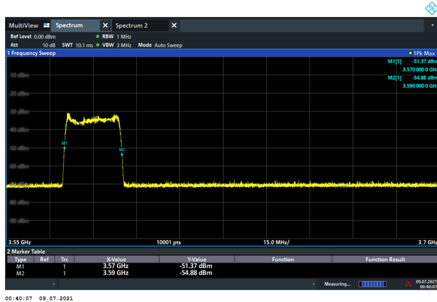
Plot 7-82. Run#1 End User Device Frequency of Operations
