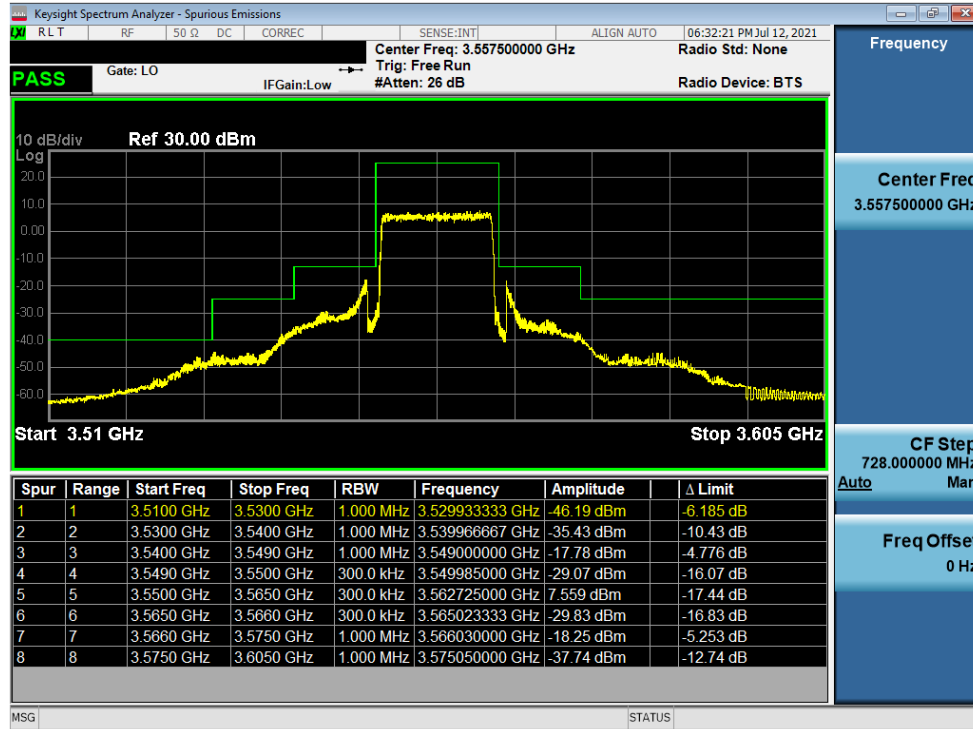
Plot 7-63. ACP Plot (LTE Band 48 - 15MHz QPSK - Low Channel)
