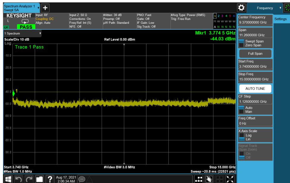
Plot 7-54. Conducted Spurious Plot (ULCA LTE Band 48 - 20+20MHz QPSK - High Channel)
