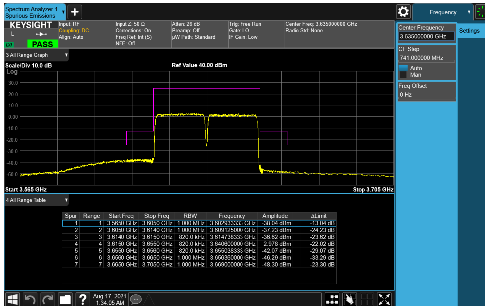
Plot 7-70. ACP Plot (LTE Band 48 – 20+20MHz QPSK - Mid Channel)
