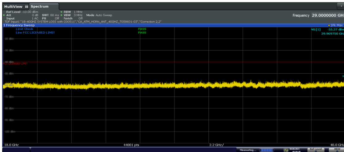
Plot 7-74. Radiated Spurious Plot 18 – 40GHz (LTE Band 48 – Ant. Pol V)
