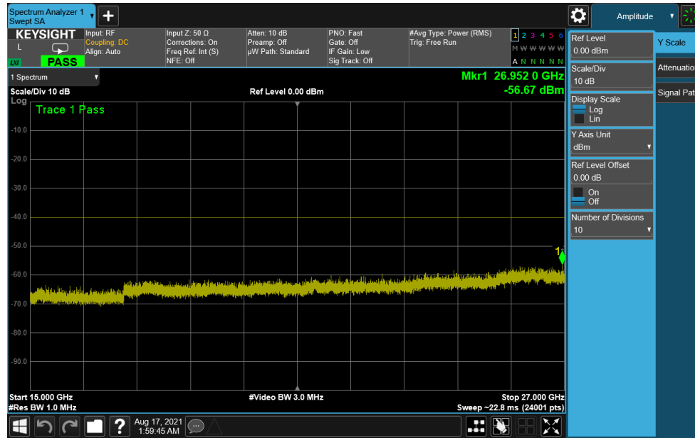
Plot 7-47. Conducted Spurious Plot (ULCA LTE Band 48 - 20+20MHz QPSK - Low Channel)
