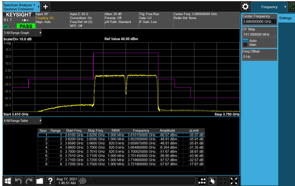
Plot 7-71. ACP Plot (LTE Band 48 – 20+20MHz QPSK - High Channel)
