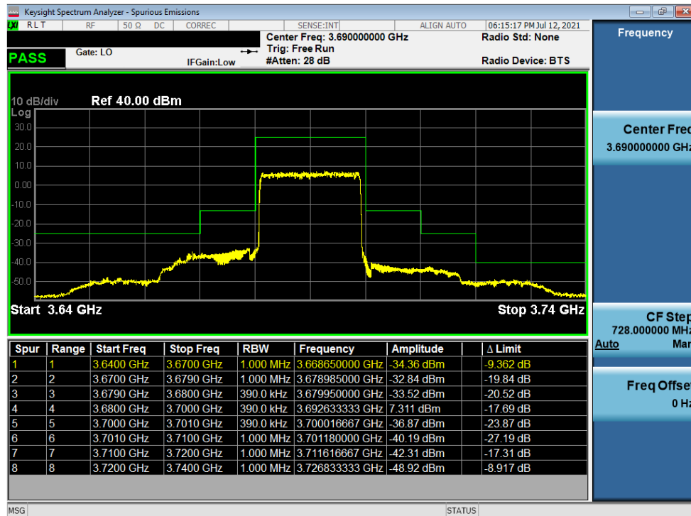
Plot 7-68. ACP Plot (LTE Band 48 - 20MHz QPSK - High Channel)
