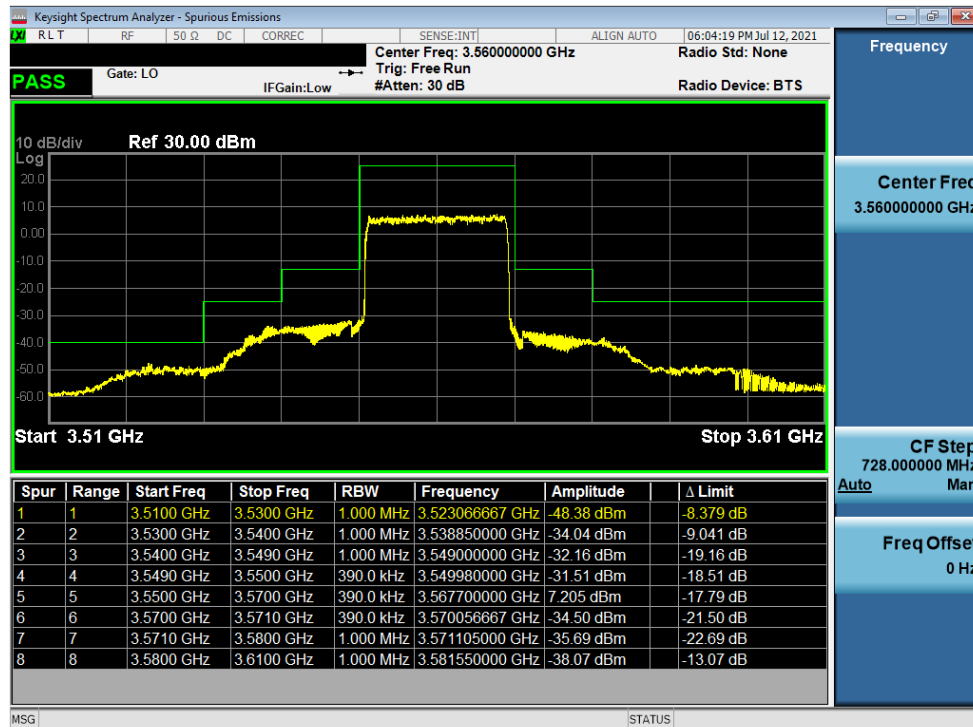
Plot 7-66. ACP Plot (LTE Band 48 - 20MHz QPSK - Low Channel)
