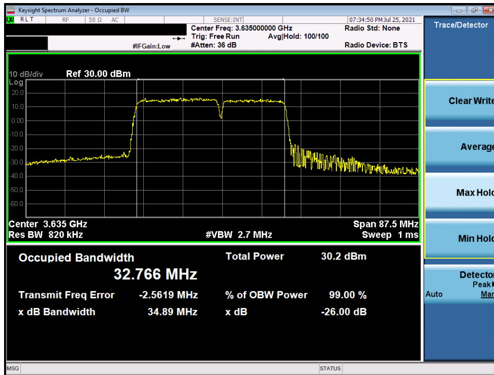
Plot 7-25. Occupied Bandwidth Plot (ULCA LTE Band 48 - 20+15MHz QPSK - Full RB Configuration)
