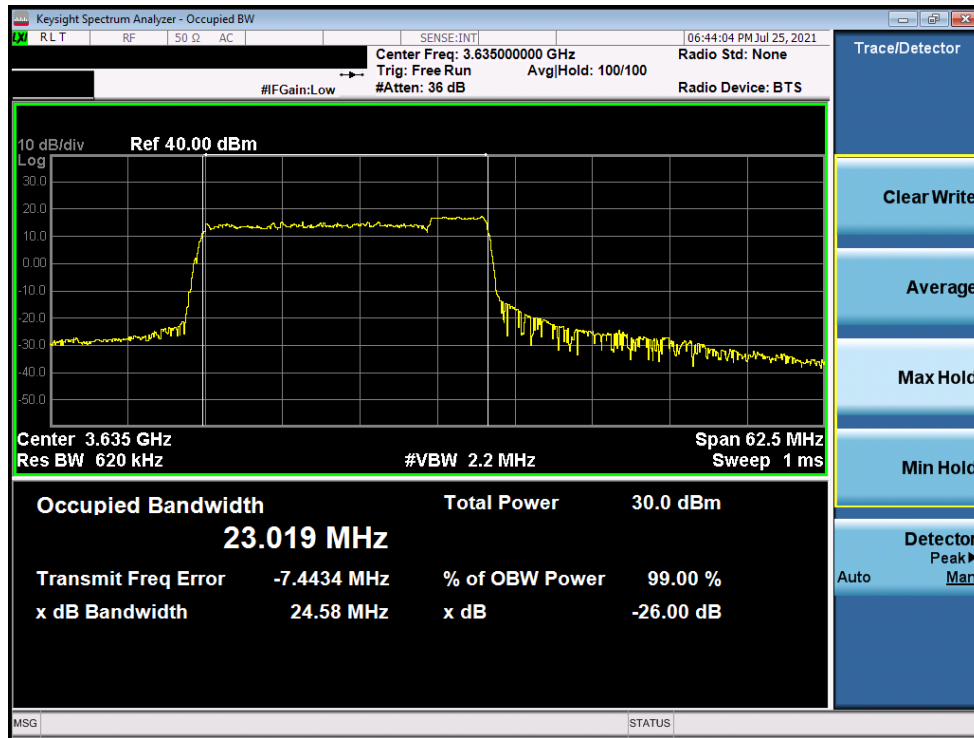
Plot 7-17. Occupied Bandwidth Plot (ULCA LTE Band 48 - 20+5MHz QPSK - Full RB Configuration)
