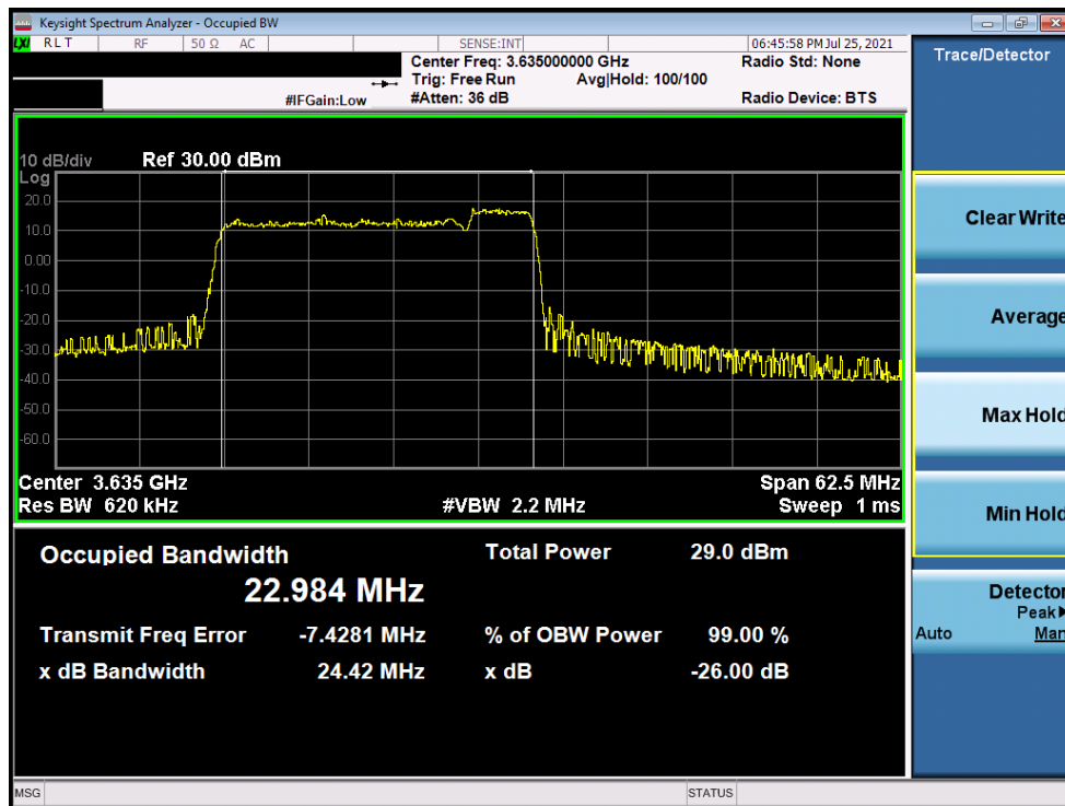
Plot 7-18. Occupied Bandwidth Plot (ULCA LTE Band 48 - 20+5MHz 16-QAM - Full RB Configuration)
