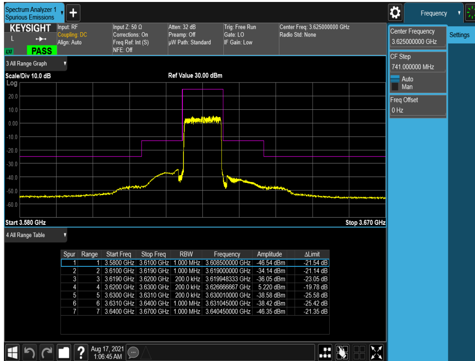
Plot 7-61. ACP Plot (LTE Band 48 - 10MHz QPSK - Mid Channel)
