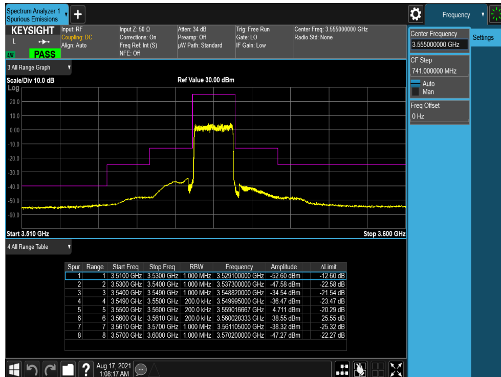
Plot 7-60. ACP Plot (LTE Band 48 - 10MHz QPSK - Low Channel)
