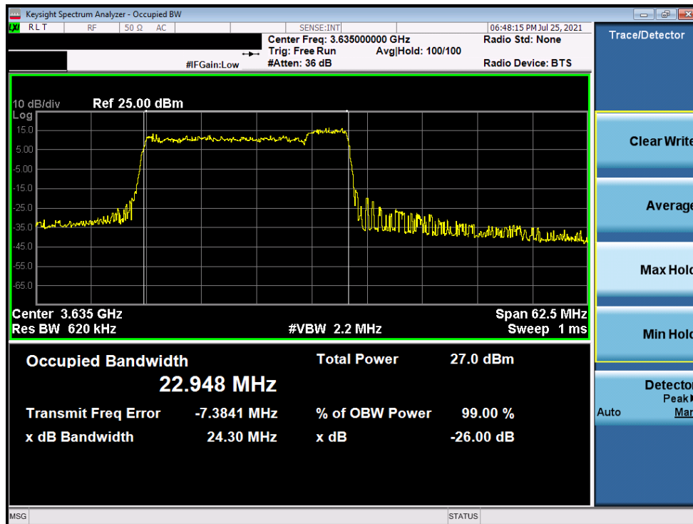
Plot 7-20. Occupied Bandwidth Plot (ULCA LTE Band 48 - 20+5MHz 256-QAM - Full RB Configuration)
