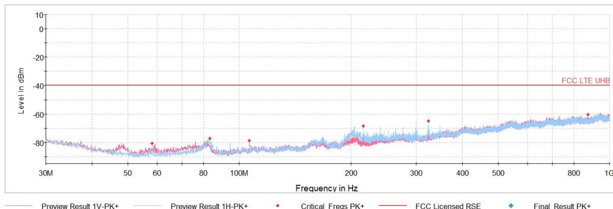
Plot 7-78. Radiated Spurious Emissions – Simultaneous Transmission 30MHz – 1GHz
