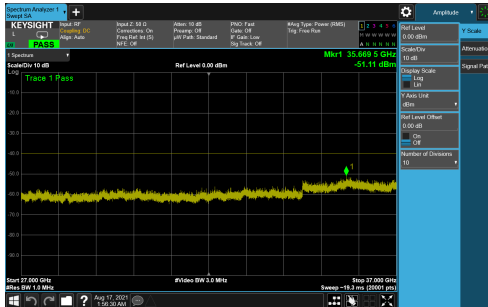
Plot 7-52. Conducted Spurious Plot (ULCA LTE Band 48 - 20+20MHz QPSK - Mid Channel)
