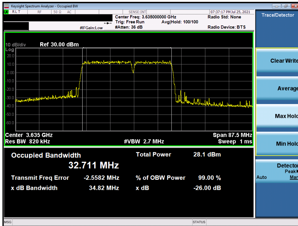
Plot 7-27. Occupied Bandwidth Plot (ULCA LTE Band 48 - 20+15MHz 64-QAM - Full RB Configuration)
