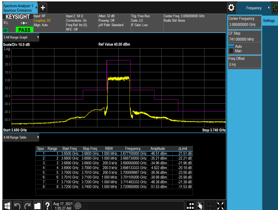
Plot 7-62. ACP Plot (LTE Band 48 - 10MHz QPSK - High Channel)
