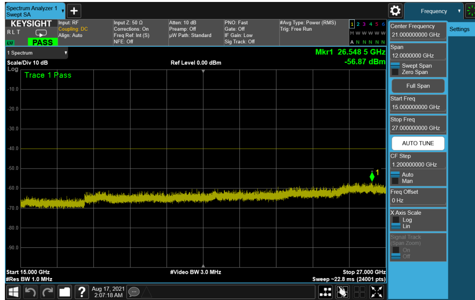
Plot 7-55. Conducted Spurious Plot (ULCA LTE Band 48 - 20+20MHz QPSK - High Channel)
