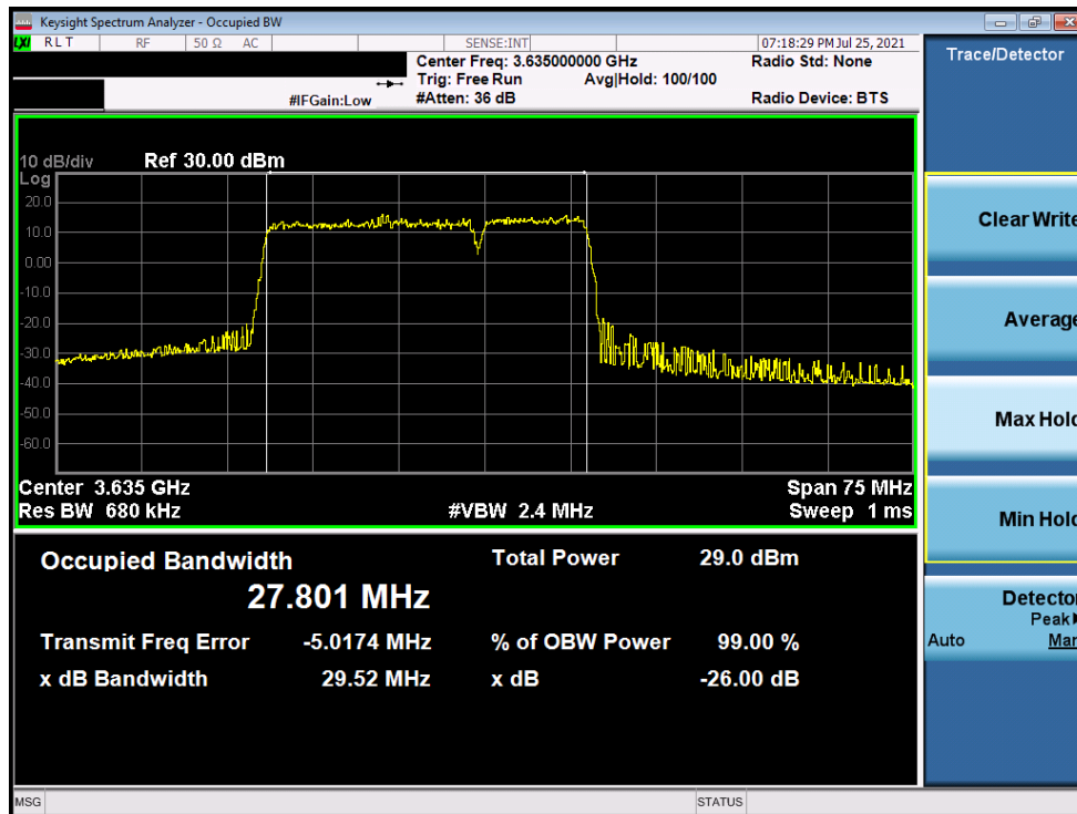
Plot 7-22. Occupied Bandwidth Plot (ULCA LTE Band 48 - 20+10MHz 16-QAM - Full RB Configuration)
