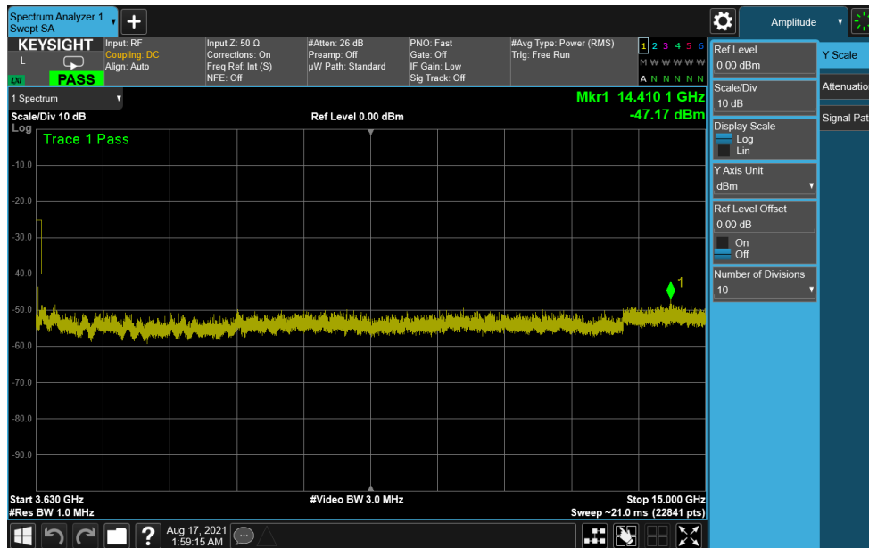
Plot 7-46. Conducted Spurious Plot (ULCA LTE Band 48 - 20+20MHz QPSK - Low Channel)
