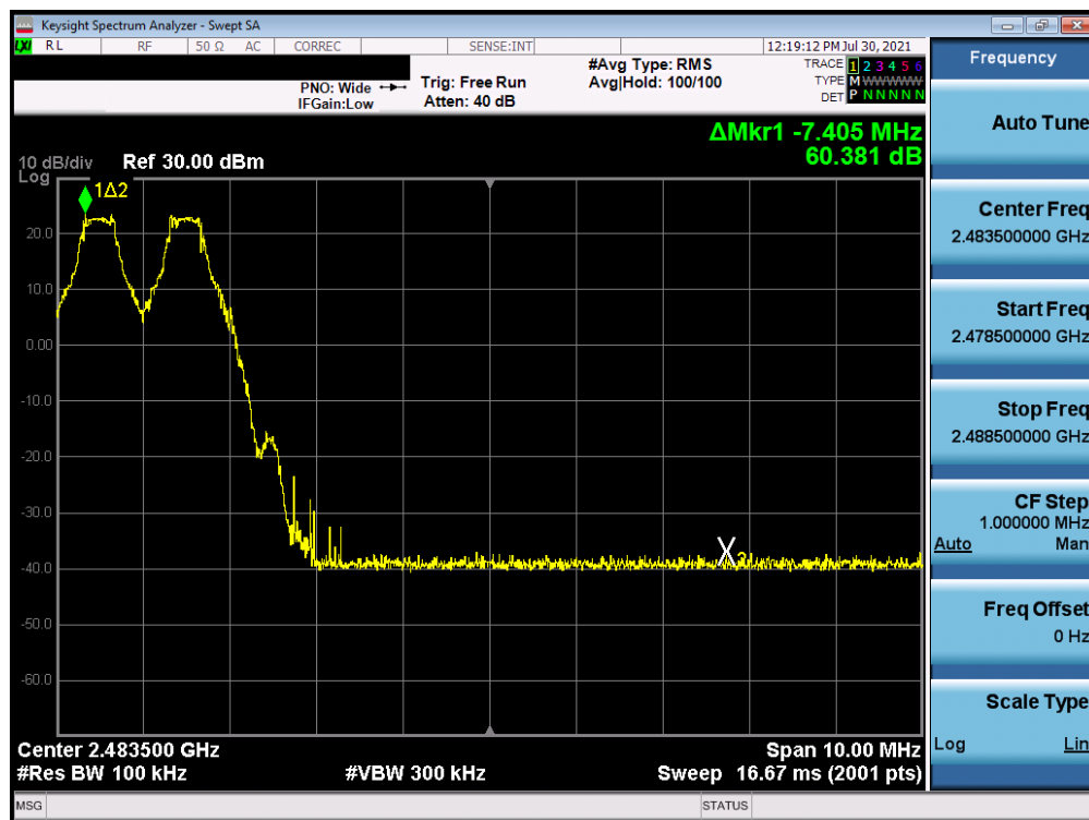
Plot 7-24. Band Edge Plot Antenna WF7 (Bluetooth with Hopping Enabled, GFSK, ePA)
