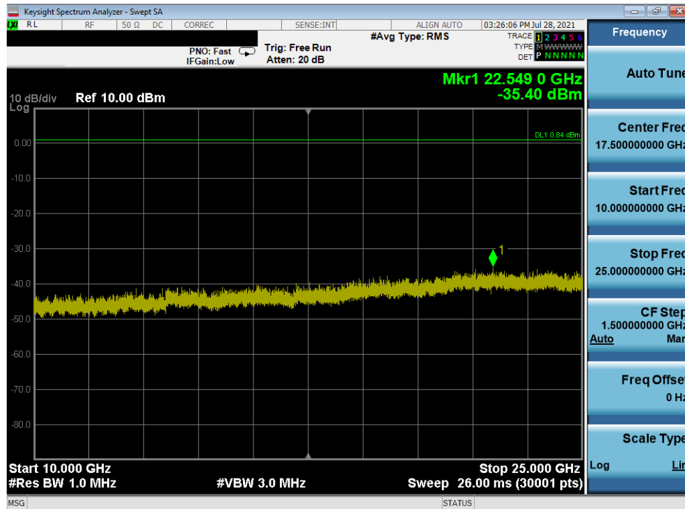
Plot 7-52. Conducted Spurious Plot Antenna WF7 (Bluetooth, GFSK, ePA – Ch. 0)
