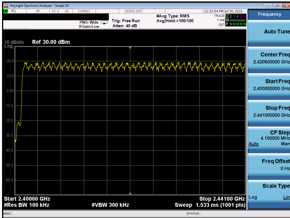
Plot 7-43. Low End Spectrum Channel Hopping Plot Antenna WF7 (Bluetooth, 8DPSK, ePA)
