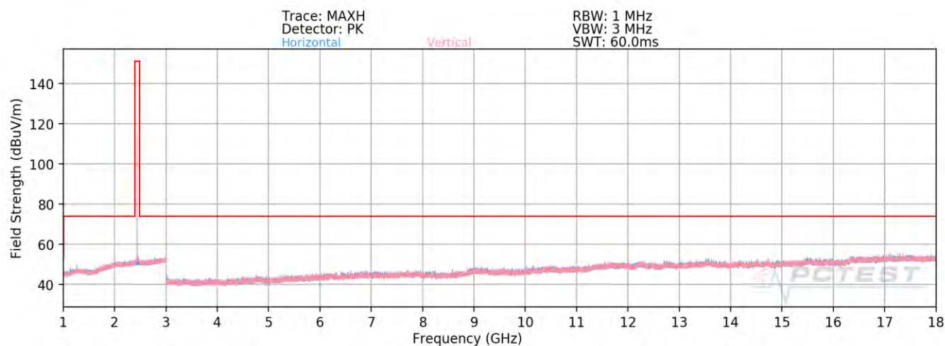
Plot 7-58. Radiated Spurious Emissions above 1GHz Antenna WF8 (BT GFSK ePA – Ch. 39)
