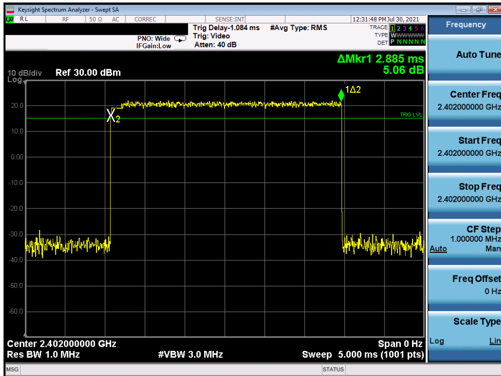
Plot 7-36. Time of Occupancy Plot Antenna WF7 (Bluetooth, 8DPSK, ePA)
