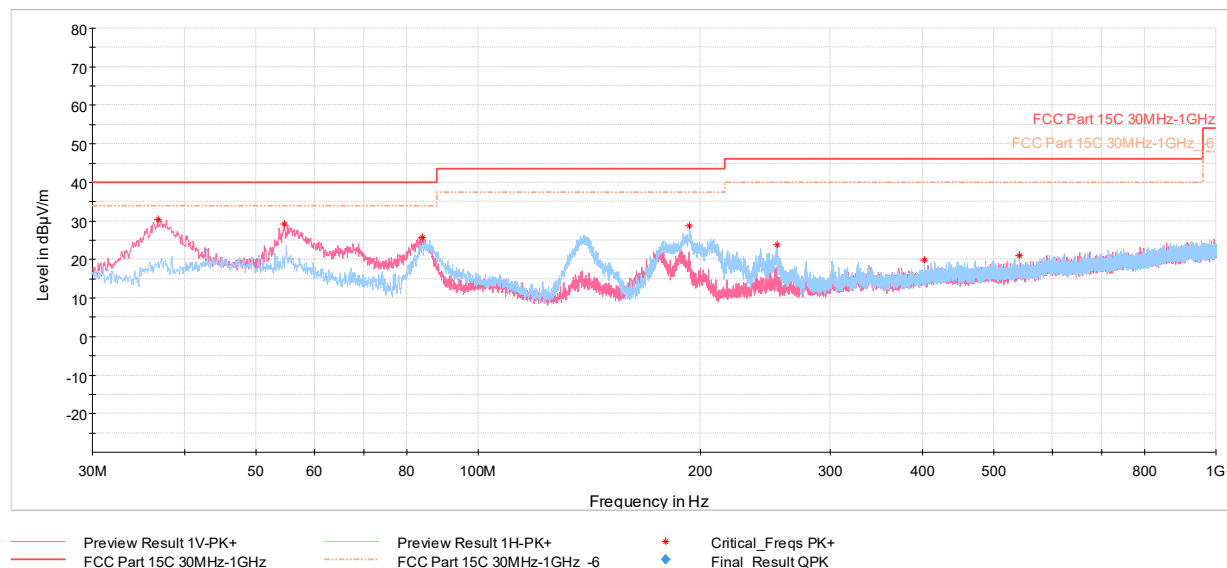
Plot 7-80. Radiated Spurious Emissions below 1GHz TxBF (GFSK ePA – Ch.39, with AC/DC Adapter)
