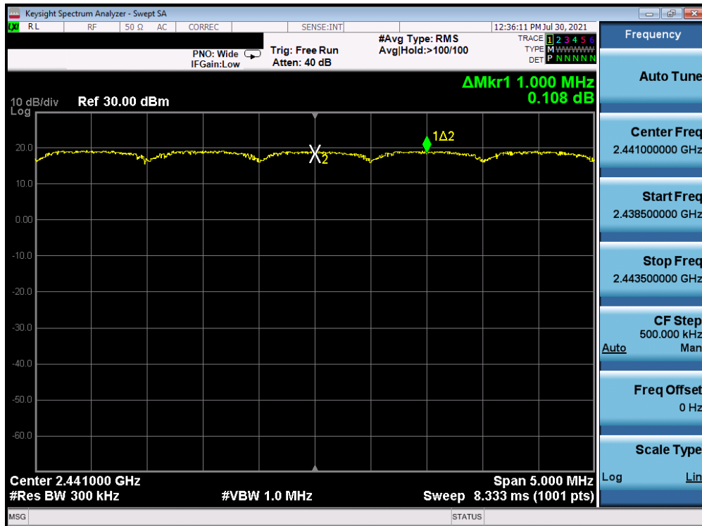
Plot 7-32. Channel Spacing Plot Antenna WF7 (Bluetooth, 8DPSK, ePA)
