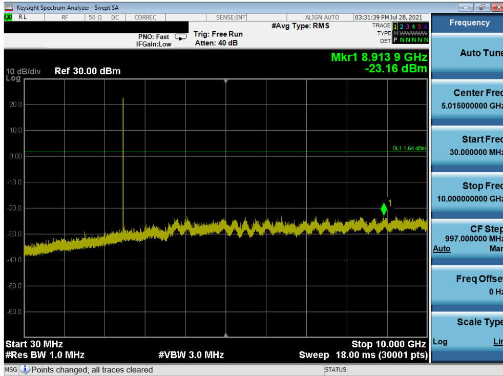
Plot 7-55. Conducted Spurious Plot Antenna WF7 (Bluetooth, GFSK, ePA – Ch. 78)
