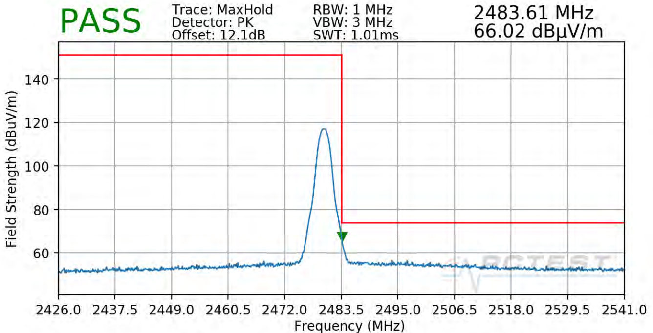
Plot 7-75. Radiated Restricted Upper Band Edge Measurement Antenna WF7 (Peak)
