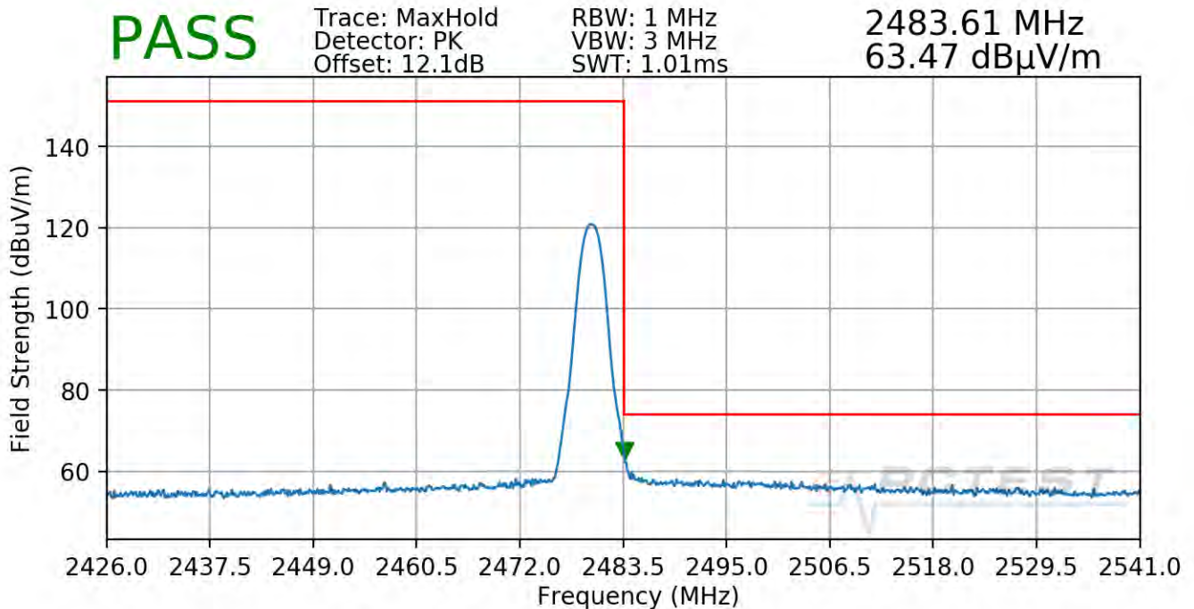
Plot 7-79. Radiated Restricted Upper Band Edge Measurement TxBF (Peak)
