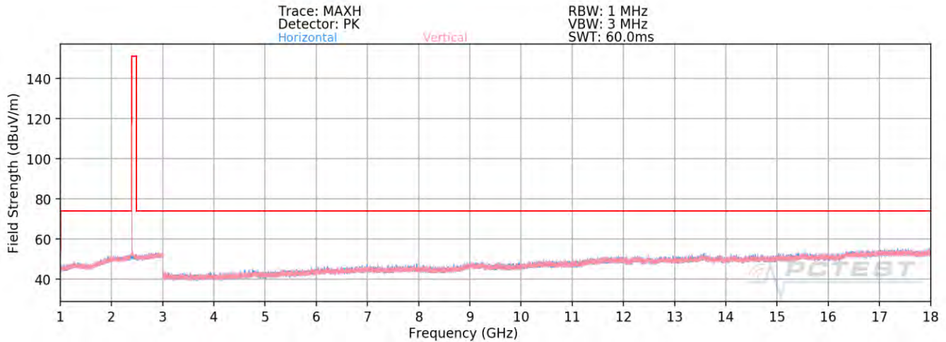
Plot 7-63. Radiated Spurious Emissions above 1GHz TxBF (BT GFSK ePA – Ch. 0)
