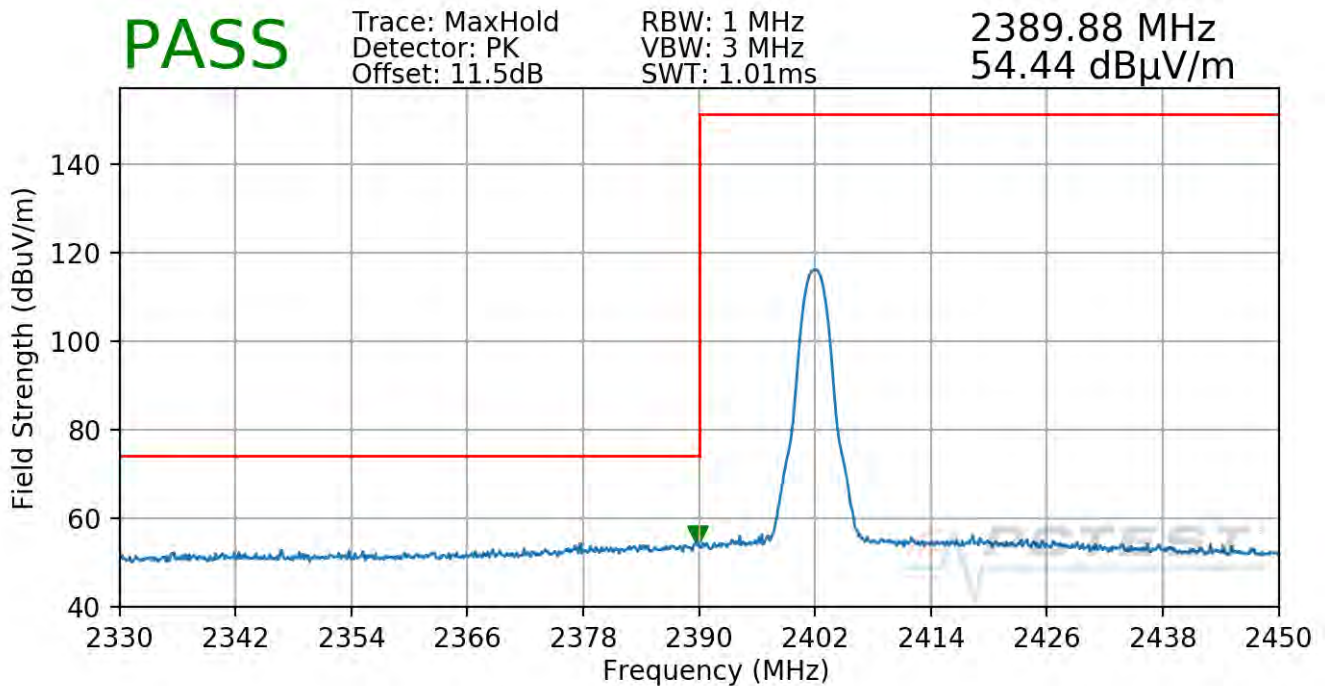
Plot 7-69. Radiated Restricted Lower Band Edge Measurement Antenna WF8 (Peak)
