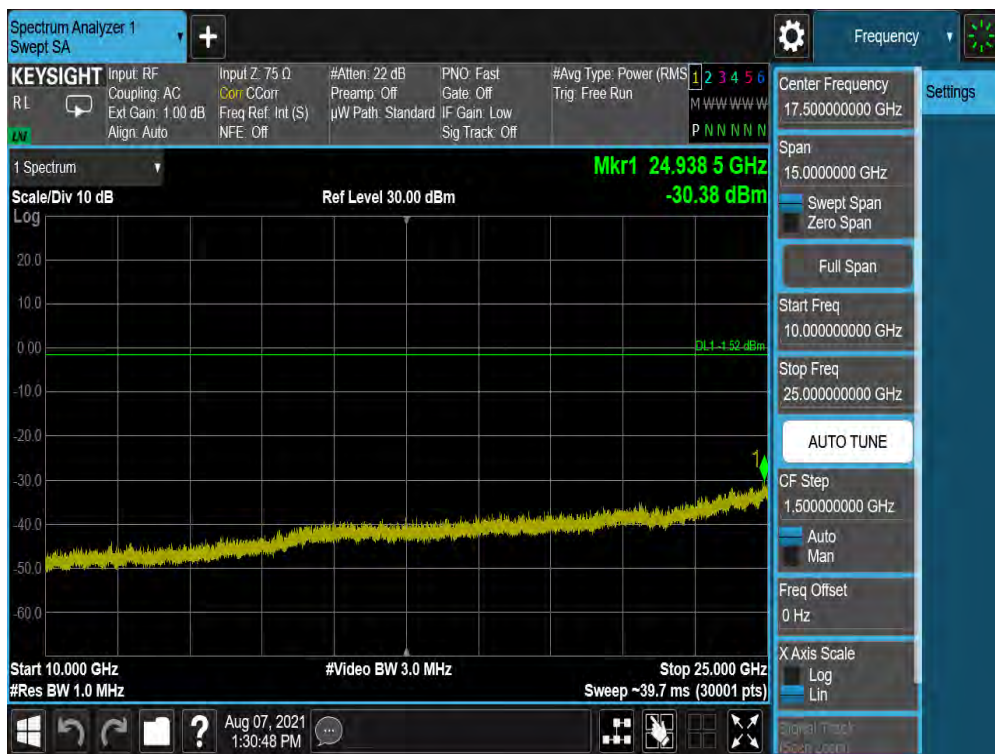
Plot 7-54. Conducted Spurious Plot Antenna WF7 (Bluetooth, GFSK, ePA Ch. 39)
