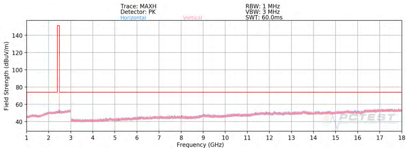
Plot 7-62. Radiated Spurious Emissions above 1GHz Antenna WF7 (BT GFSK ePA – Ch. 78)
