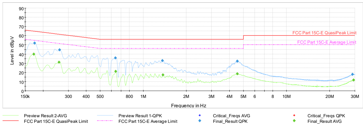
Plot 7-82. AC Line-Conducted Test Plot TxBF (N, GFSK ePA – Ch.39, with AC/DC Adapter)
