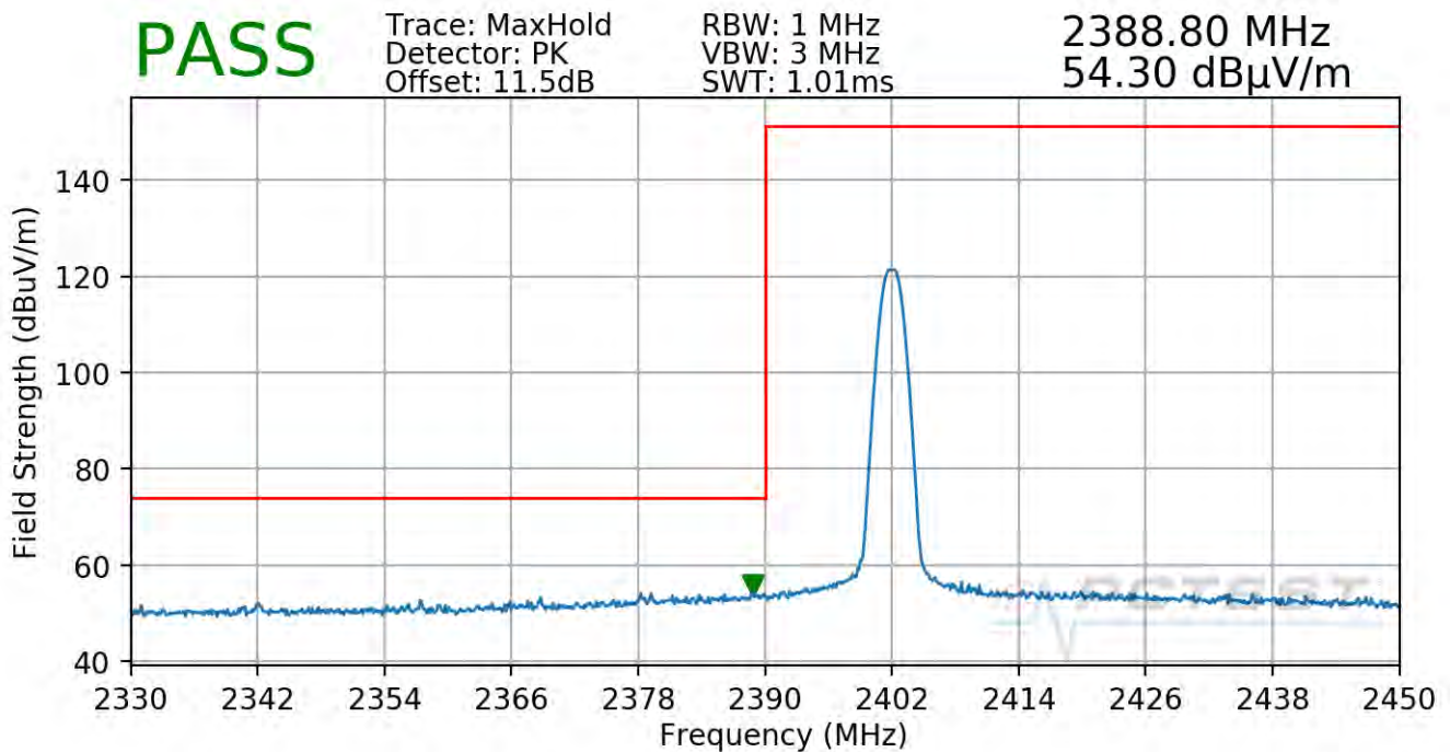
Plot 7-76. Radiated Restricted Lower Band Edge Measurement TxBF (Peak)
