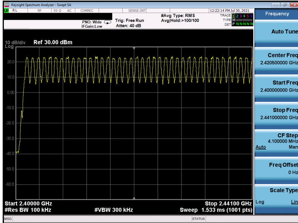
Plot 7-41. Low End Spectrum Channel Hopping Plot Antenna WF7 (Bluetooth, GFSK, ePA)
