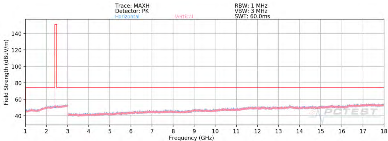
Plot 7-57. Radiated Spurious Emissions above 1GHz Antenna WF8 (BT GFSK ePA – Ch. 0)
