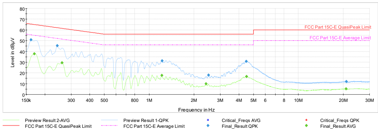
Plot 7-81. AC Line-Conducted Test Plot TxBF (L1, GFSK ePA – Ch.39, with AC/DC Adapter)
