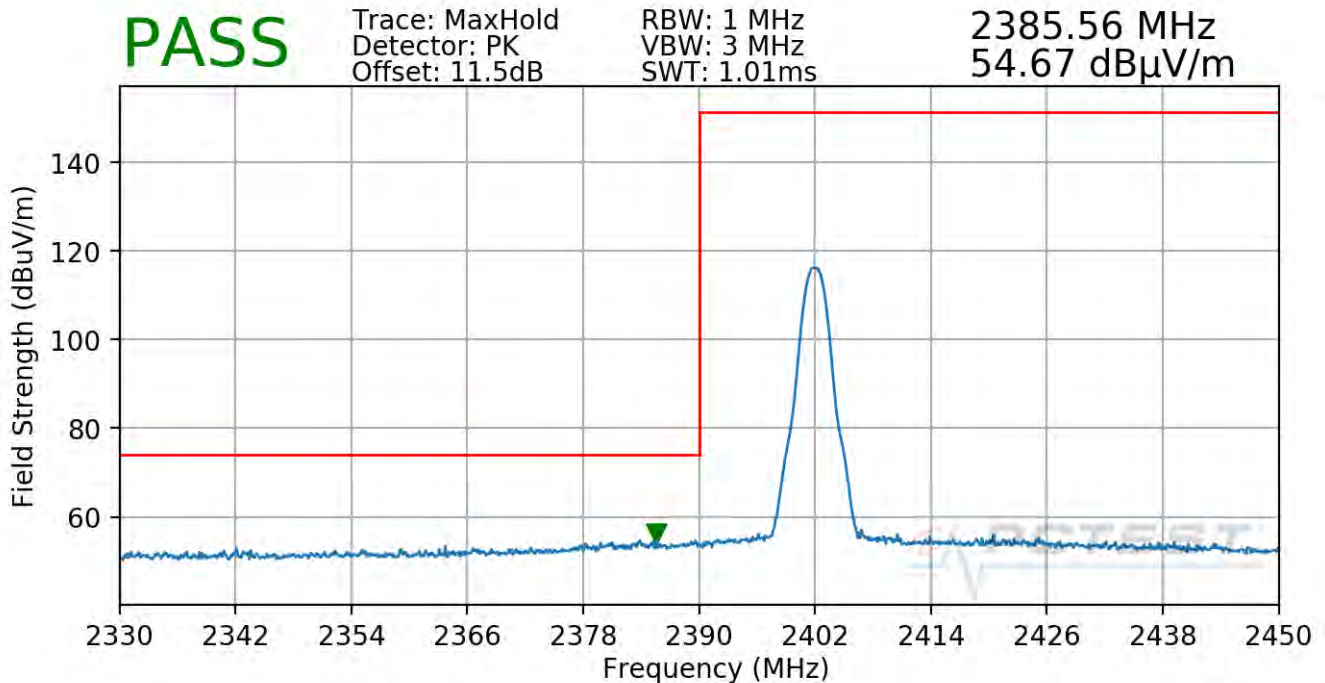
Plot 7-73. Radiated Restricted Lower Band Edge Measurement Antenna WF7 (Peak)
