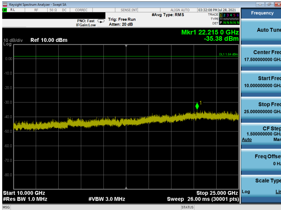
Plot 7-56. Conducted Spurious Plot Antenna WF7 (Bluetooth, GFSK, ePA – Ch. 78)
