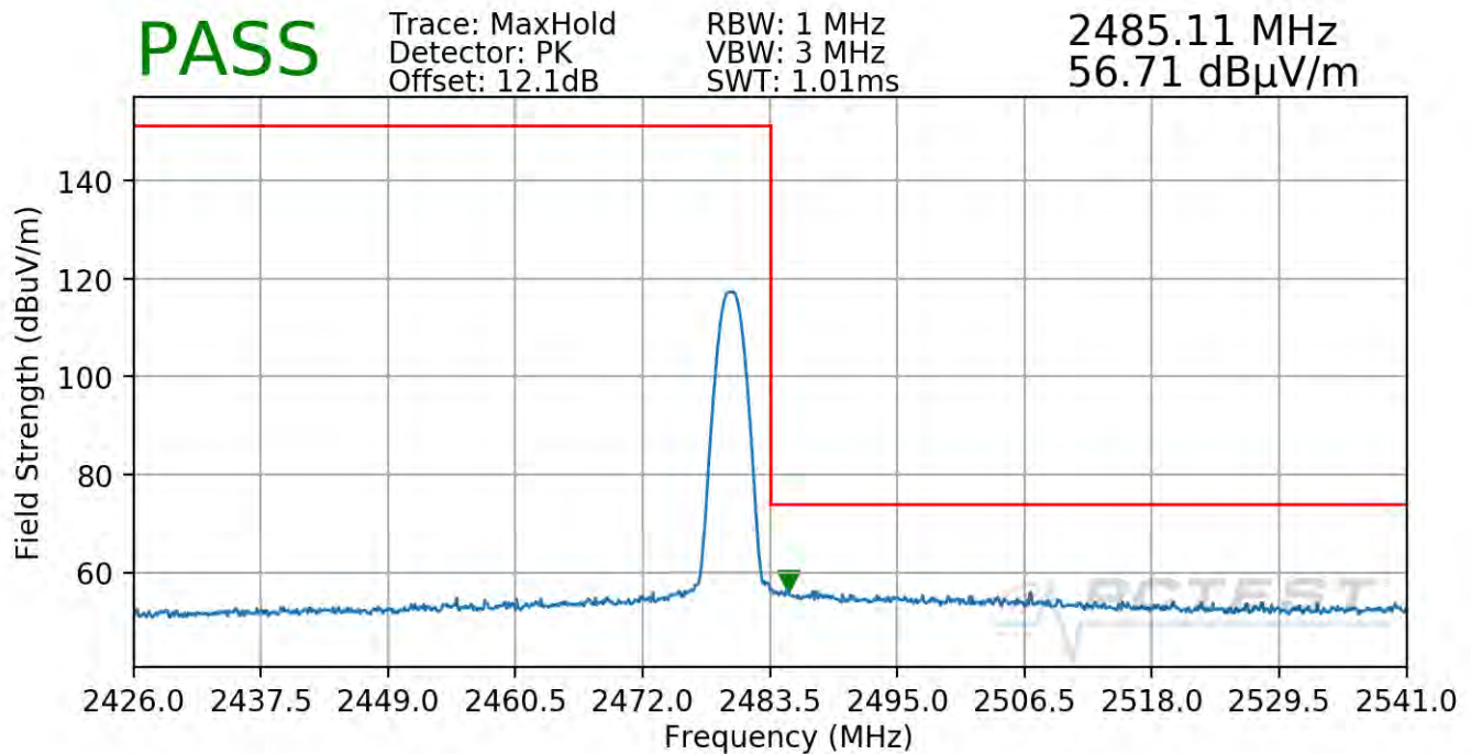
Plot 7-74. Radiated Restricted Upper Band Edge Measurement Antenna WF7 (Peak)
