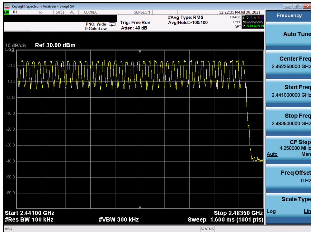
Plot 7-42. High End Spectrum Channel Hopping Plot Antenna WF7 (Bluetooth, GFSK, ePA)
