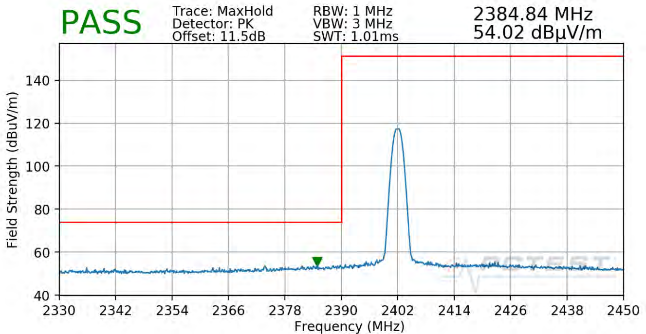
Plot 7-68. Radiated Restricted Lower Band Edge Measurement Antenna WF8 (Peak)
