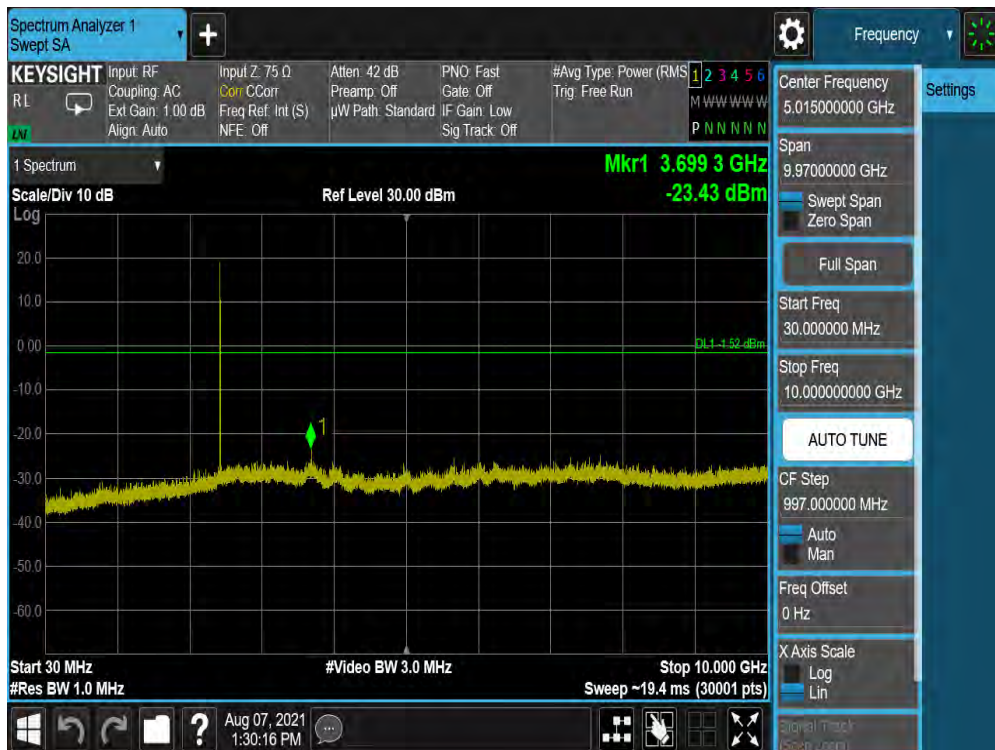
Plot 7-53. Conducted Spurious Plot Antenna WF7 (Bluetooth, GFSK, ePA – Ch. 39)
