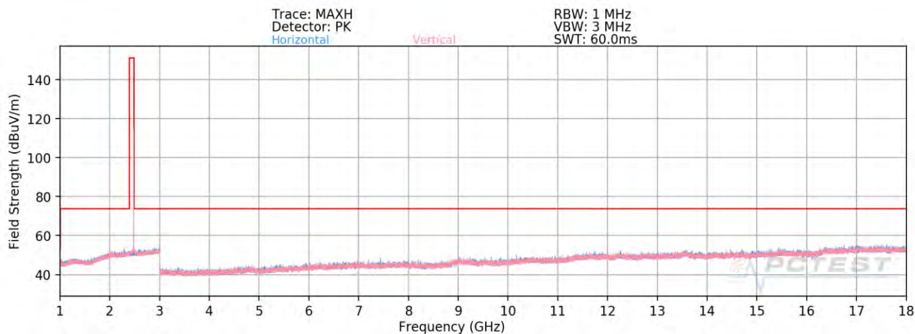
Plot 7-59. Radiated Spurious Emissions above 1GHz Antenna WF8 (BT GFSK ePA – Ch. 78)
