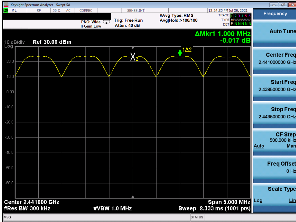
Plot 7-31. Channel Spacing Plot Antenna WF7 (Bluetooth, GFSK, ePA)
