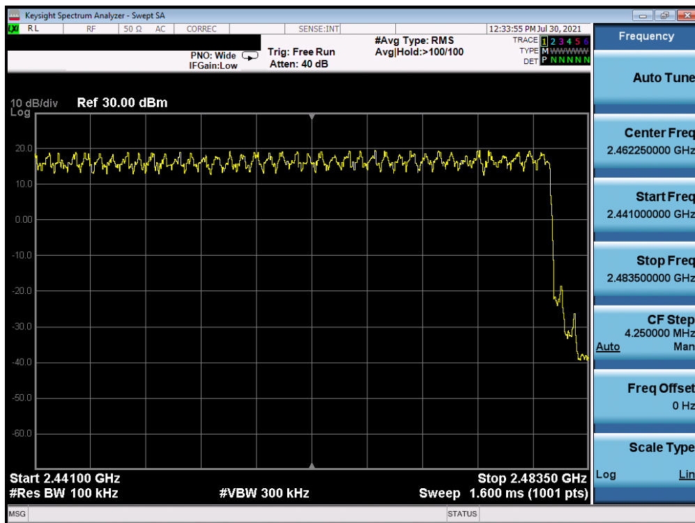
Plot 7-44. High End Spectrum Channel Hopping Plot Antenna WF7 (Bluetooth, 8DPSK, ePA)
