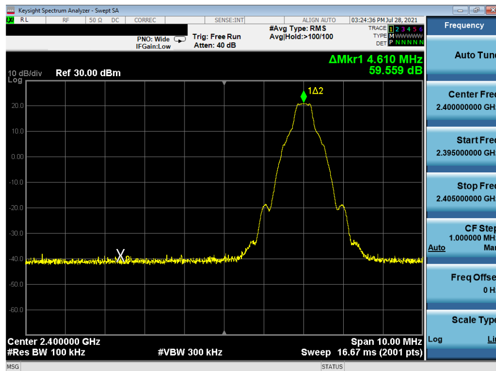
Plot 7-21. Band Edge Plot Antenna WF7 (Bluetooth with Hopping Disabled, GFSK, ePA – Ch. 0)
