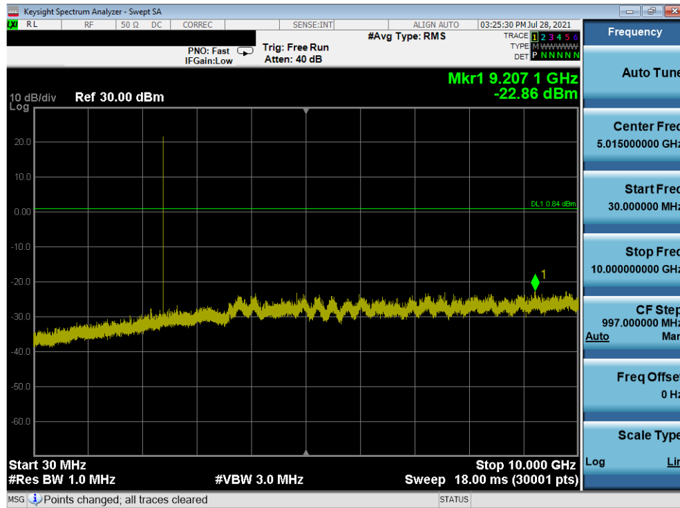
Plot 7-51. Conducted Spurious Plot Antenna WF7 (Bluetooth, GFSK, ePA – Ch. 0)
