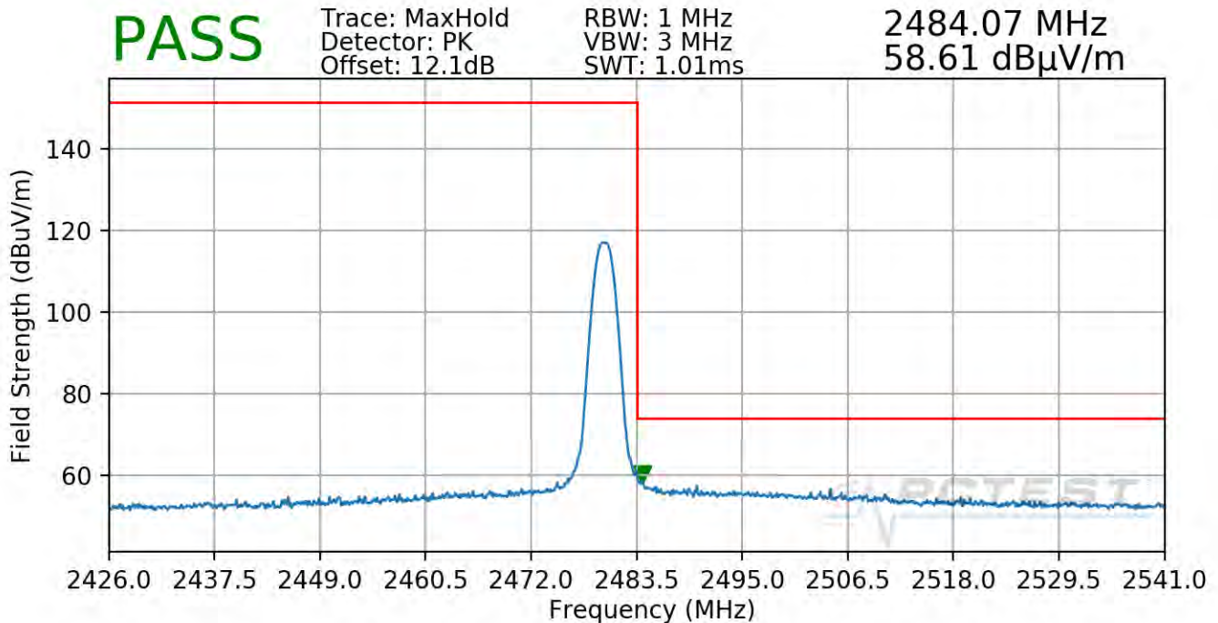
Plot 7-70. Radiated Restricted Upper Band Edge Measurement Antenna WF8 (Peak)
