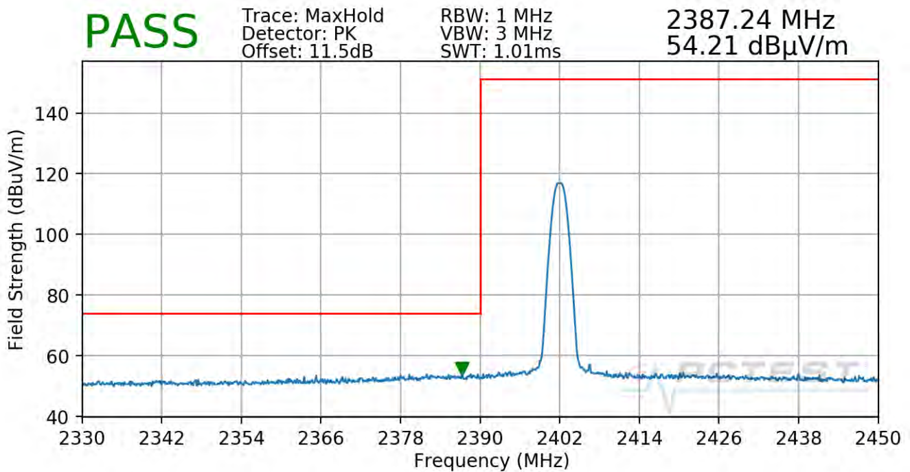
Plot 7-72. Radiated Restricted Lower Band Edge Measurement Antenna WF7 (Peak)
