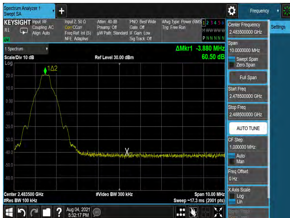
Plot 7-22. Band Edge Plot Antenna WF7 (Bluetooth with Hopping Disabled, GFSK, ePA – Ch. 78)
