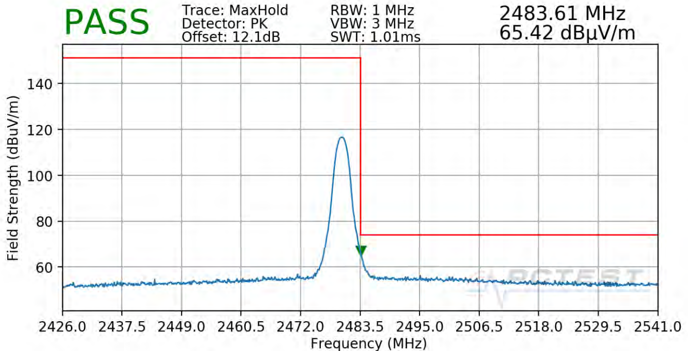
Plot 7-71. Radiated Restricted Upper Band Edge Measurement Antenna WF8 (Peak)
