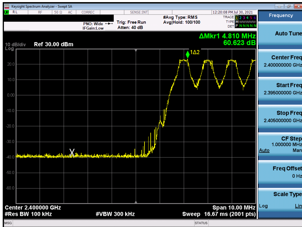
Plot 7-23. Band Edge Plot Antenna WF7 (Bluetooth with Hopping Enabled, GFSK, ePA)
