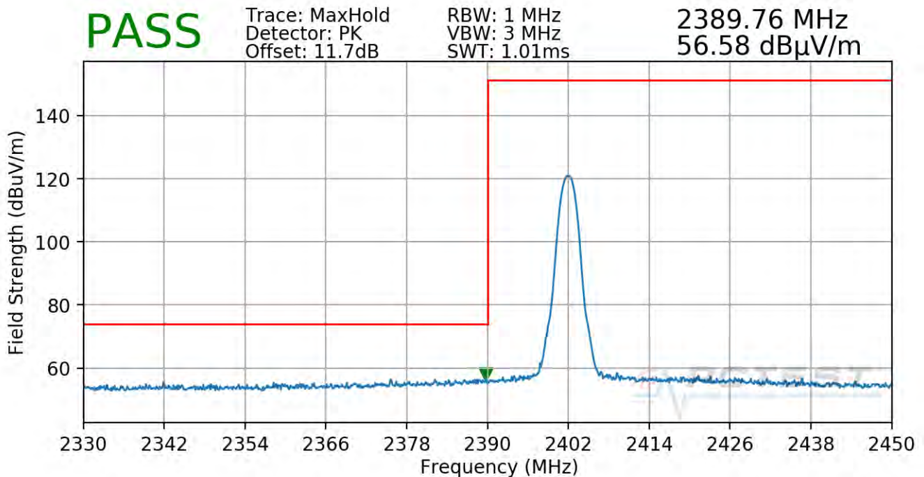
Plot 7-77. Radiated Restricted Lower Band Edge Measurement TxBF (Peak)
