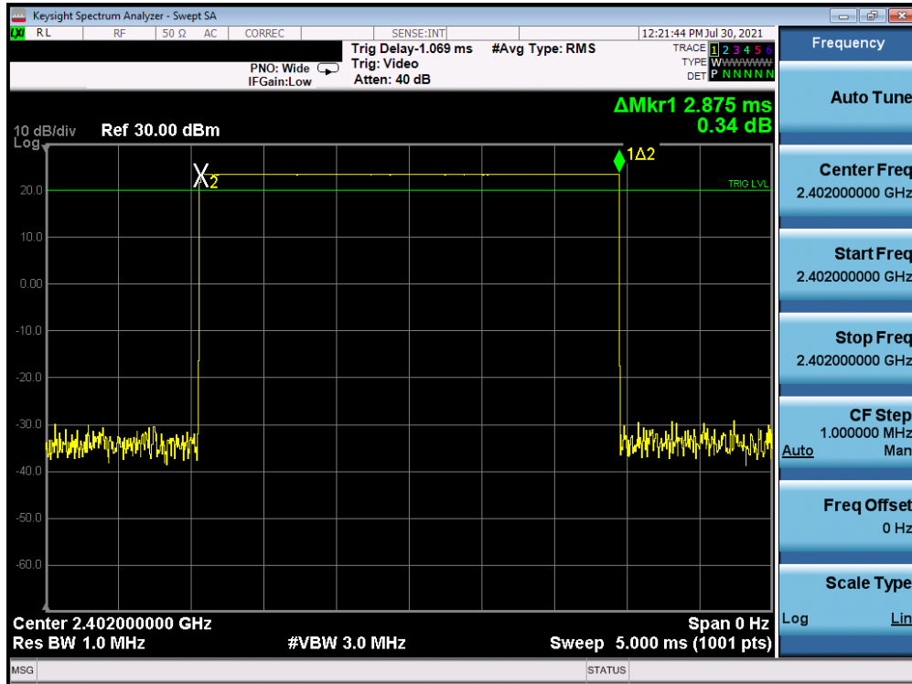
Plot 7-35. Time of Occupancy Plot Antenna WF7 (Bluetooth, GFSK, ePA)
