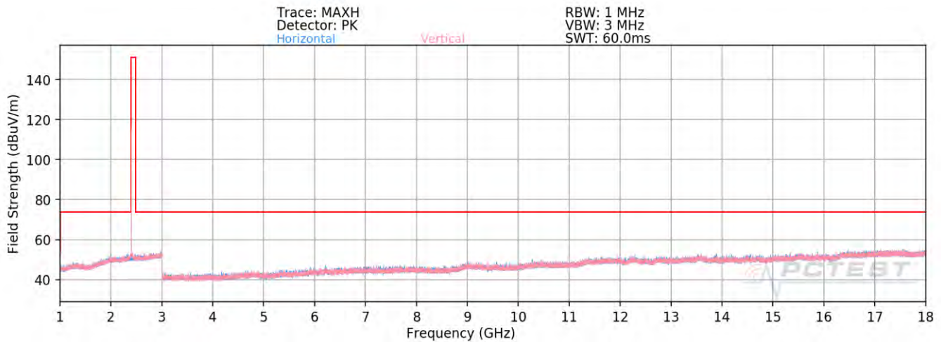
Plot 7-60. Radiated Spurious Emissions above 1GHz Antenna WF7 (BT GFSK ePA – Ch. 0)
