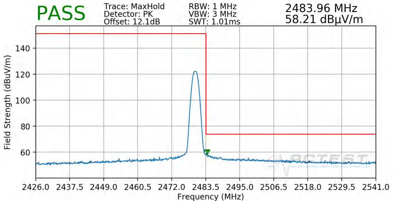
Plot 7-78. Radiated Restricted Upper Band Edge Measurement TxBF (Peak)
