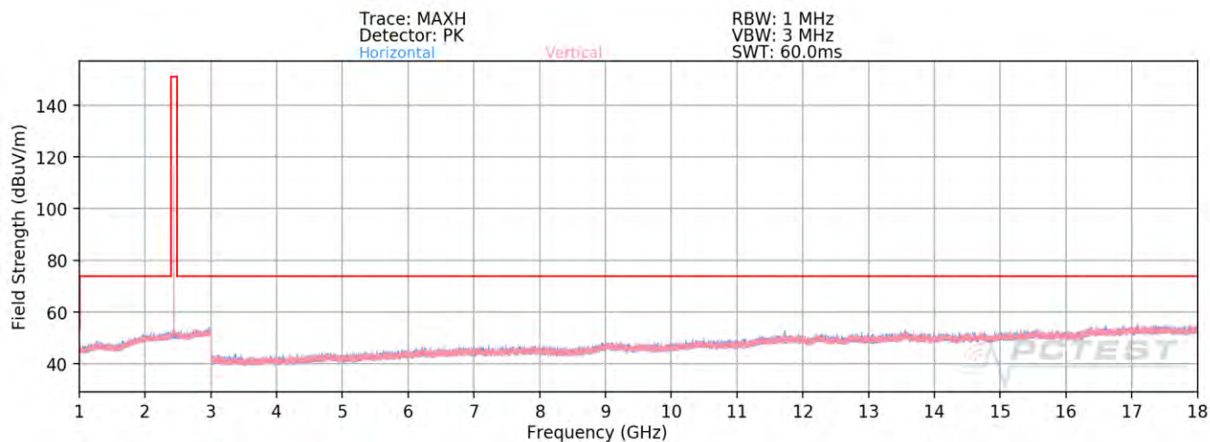
Plot 7-61. Radiated Spurious Emissions above 1GHz Antenna WF7 (BT GFSK ePA – Ch. 39)
