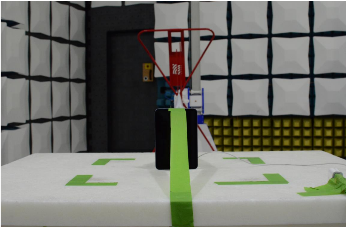
Figure 16: 30MHz-1GHz Test Setup (Rear View)
