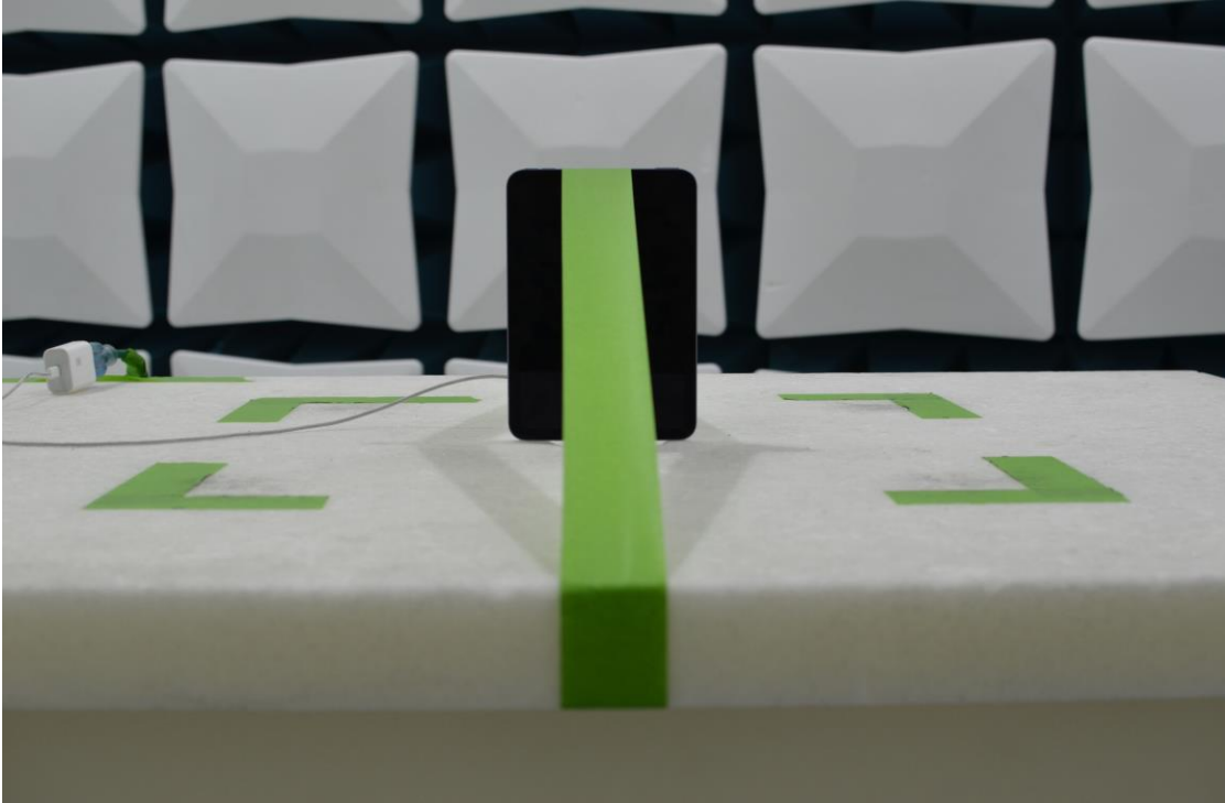
Figure 15: 30MHz-1GHz Test Setup (Front View)
