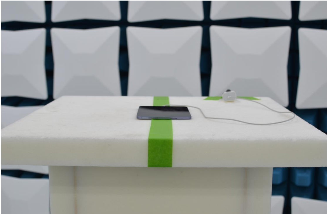
Figure 5: 1-18GHz Test Setup (Front View)
