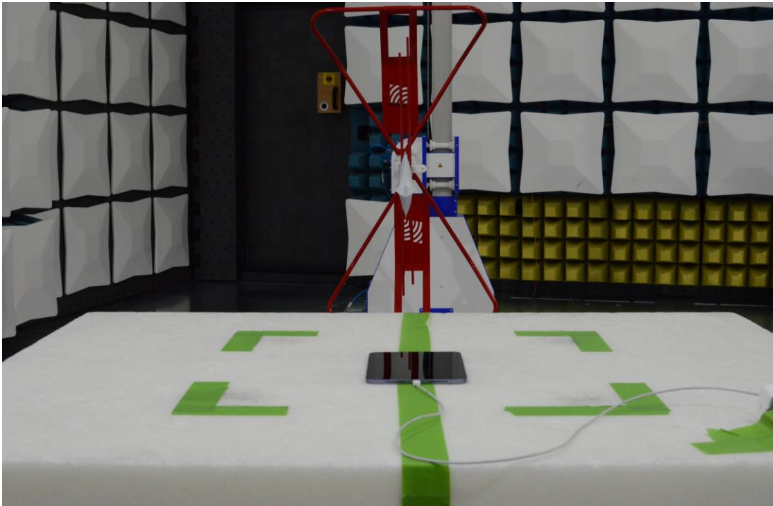
Figure 12: 30MHz-1GHz Test Setup (Rear View)
