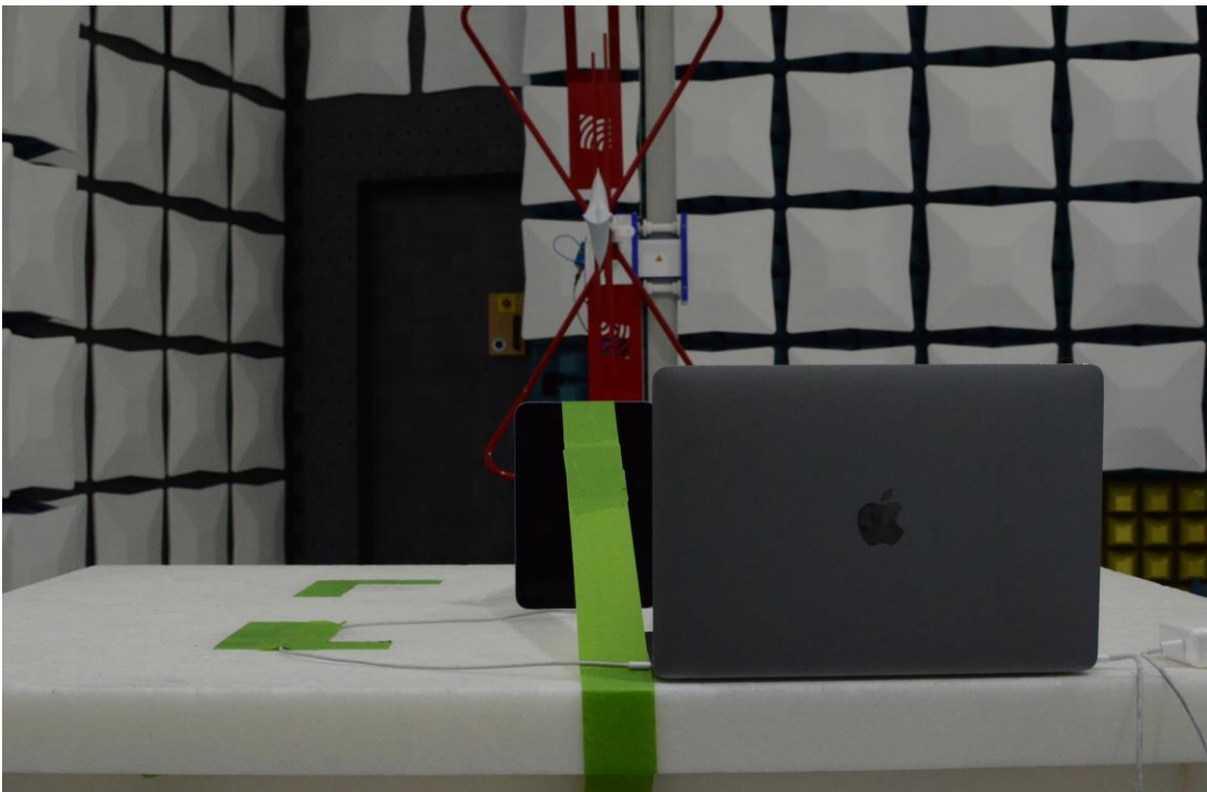
Figure 22: 30MHz-1GHz Test Setup (Rear View)
