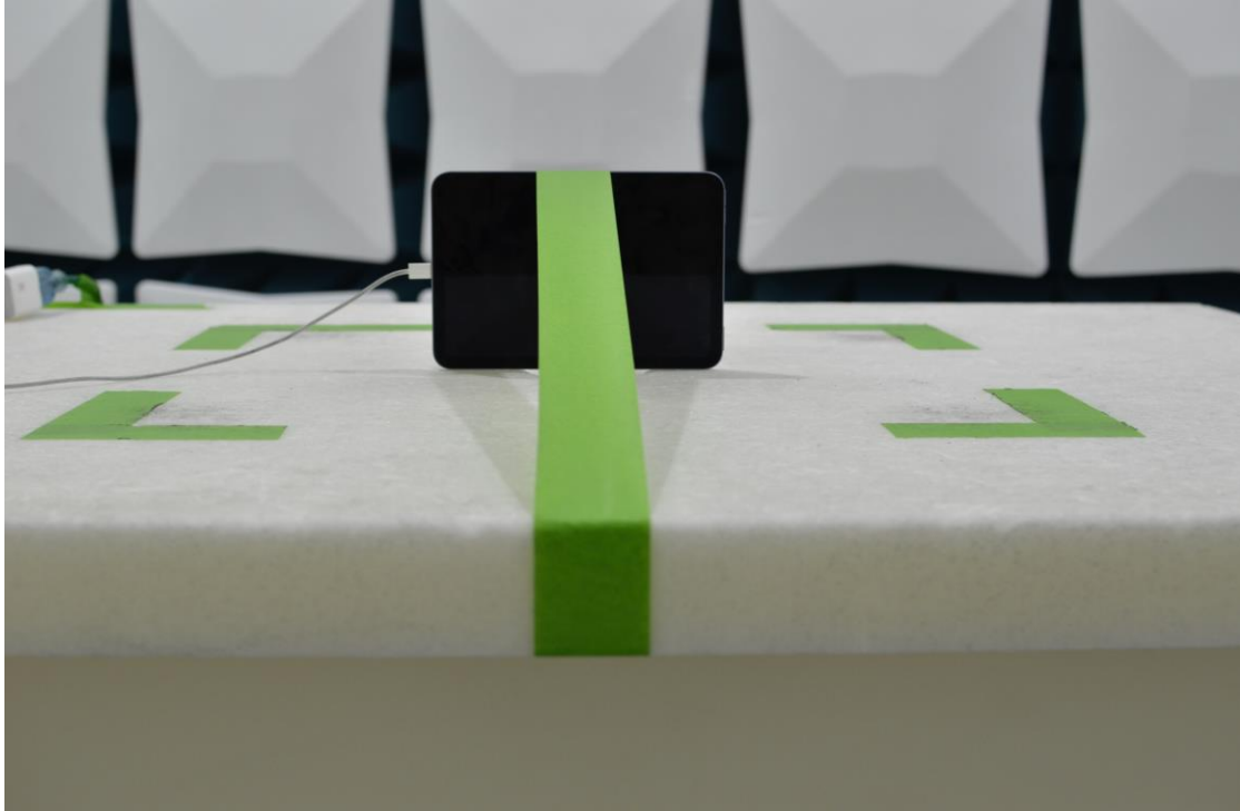
Figure 13: 30MHz-1GHz Test Setup (Front View)
