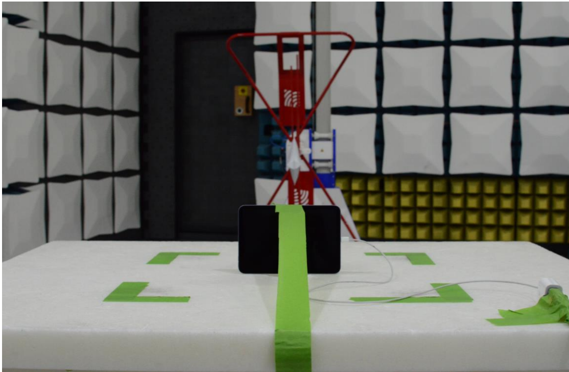
Figure 14: 30MHz-1GHz Test Setup (Rear View)
