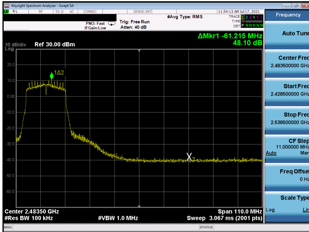
Plot 7-318. Band Edge Plot Antenna WF7 (802.11n (2.4GHz) - Ch. 7) - MCS2
