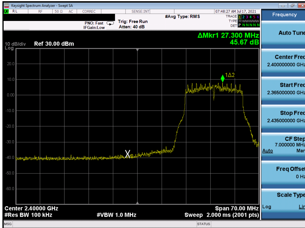
Plot 7-386. Band Edge Plot Antenna WF7 (802.11g- Ch. 3) – 36Mbps
