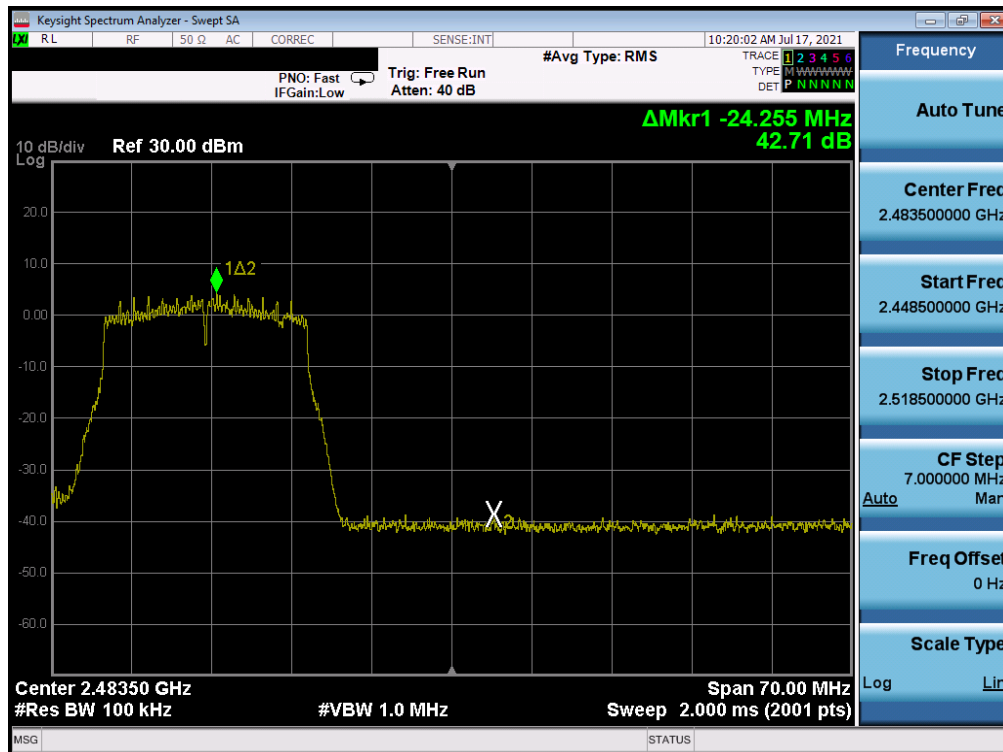
Plot 7-359. Band Edge Plot Antenna WF7 (802.11n (2.4GHz) - Ch. 11) - MCS4
