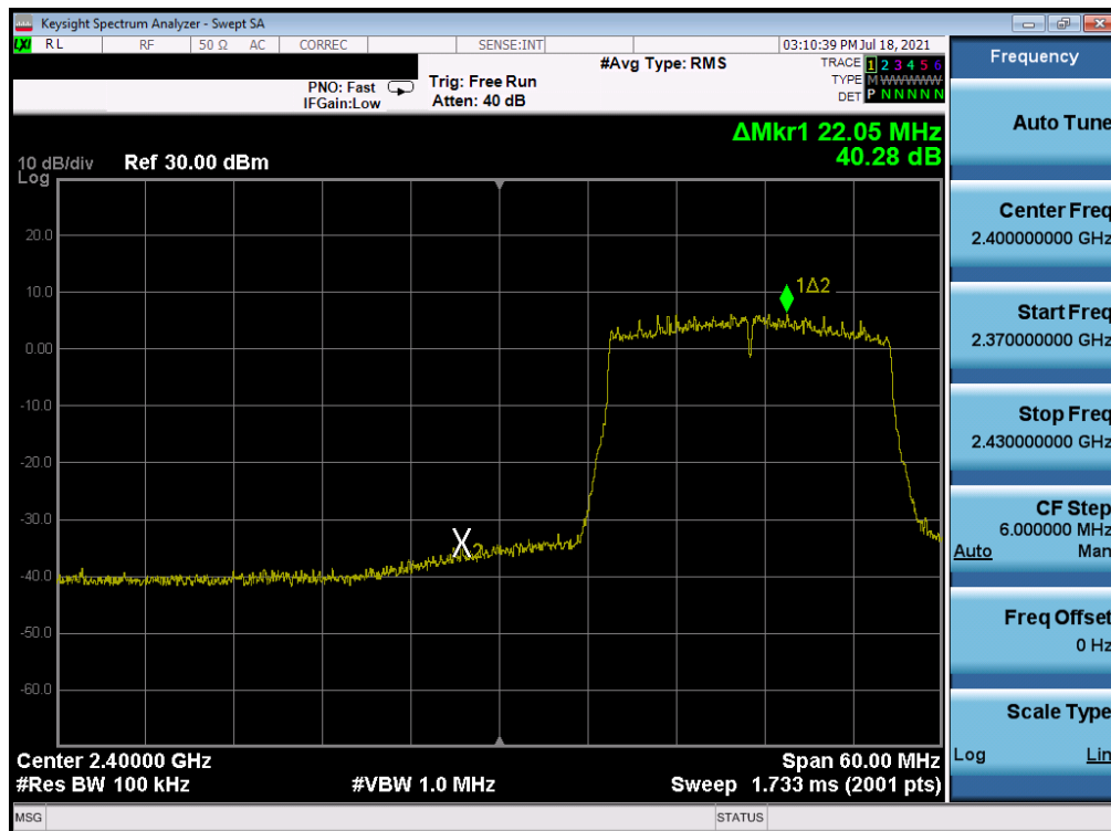
Plot 7-363. Band Edge Plot Antenna WF7 (802.11ax (SU - 2.4GHz) – Ch. 2) – MCS4
