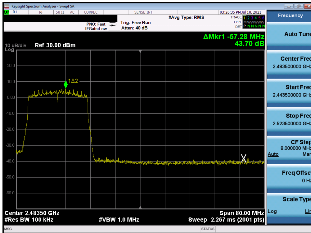
Plot 7-372. Band Edge Plot Antenna WF7 (802.11ax (SU - 2.4GHz) – Ch. 10) – MCS4
