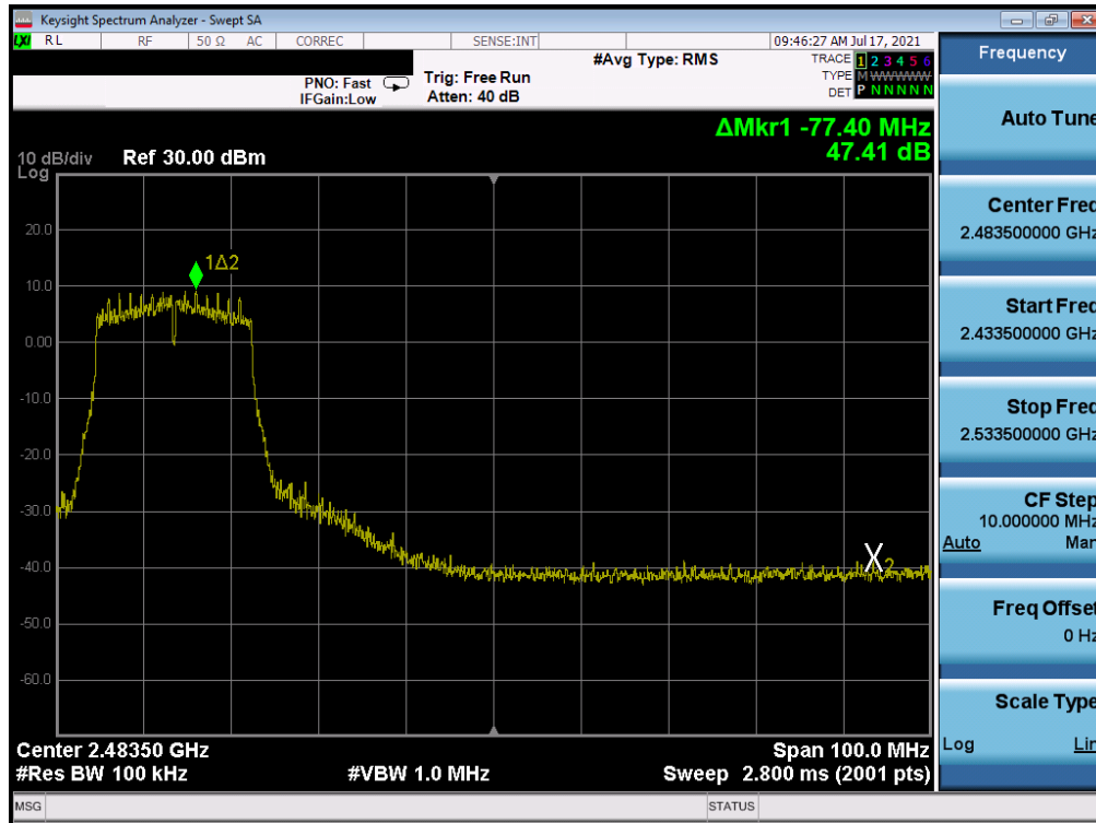
Plot 7-356. Band Edge Plot Antenna WF7 (802.11n (2.4GHz) - Ch. 8) - MCS4
