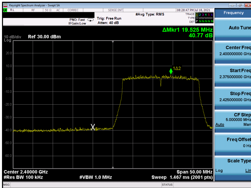
Plot 7-287. Band Edge Plot Antenna WF8 (802.11ax (SU - 2.4GHz) – Ch. 1) – MCS5
