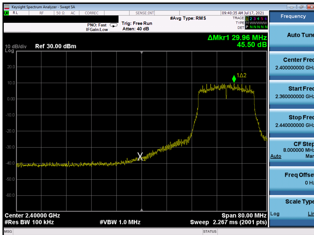
Plot 7-353. Band Edge Plot Antenna WF7 (802.11n (2.4GHz) - Ch. 4) - MCS4
