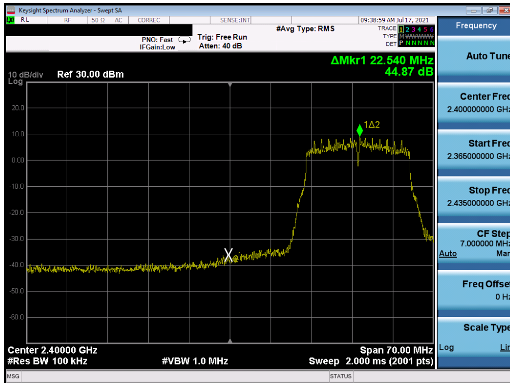
Plot 7-352. Band Edge Plot Antenna WF7 (802.11n (2.4GHz) - Ch. 3) - MCS4
