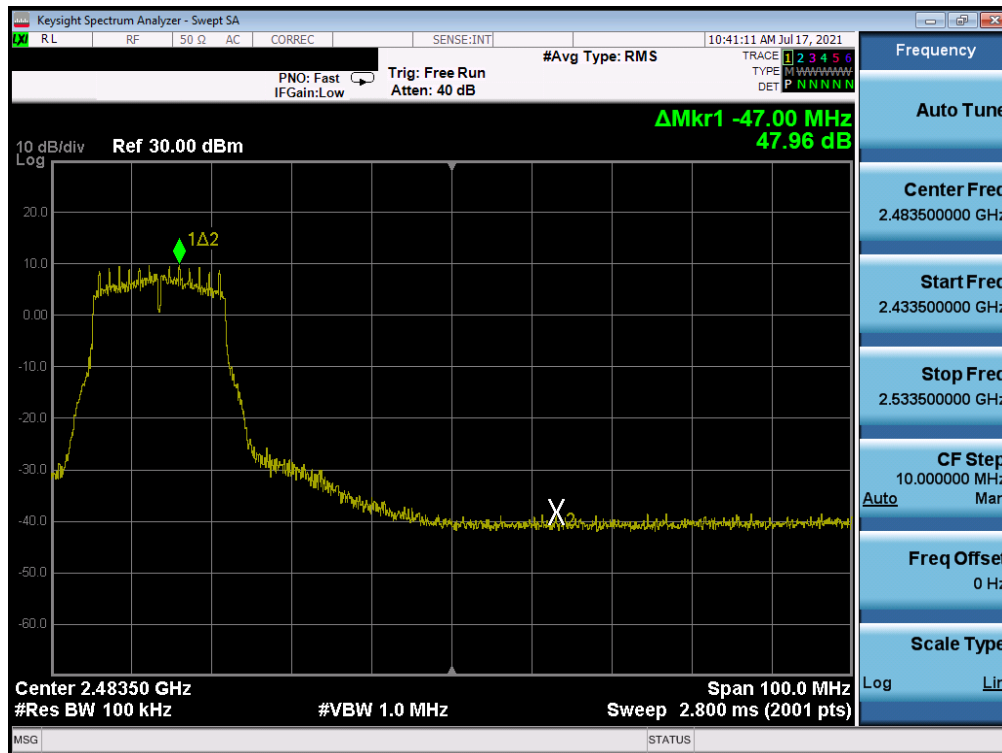
Plot 7-308. Band Edge Plot Antenna WF7 (802.11g - Ch. 8) - 12Mbps
