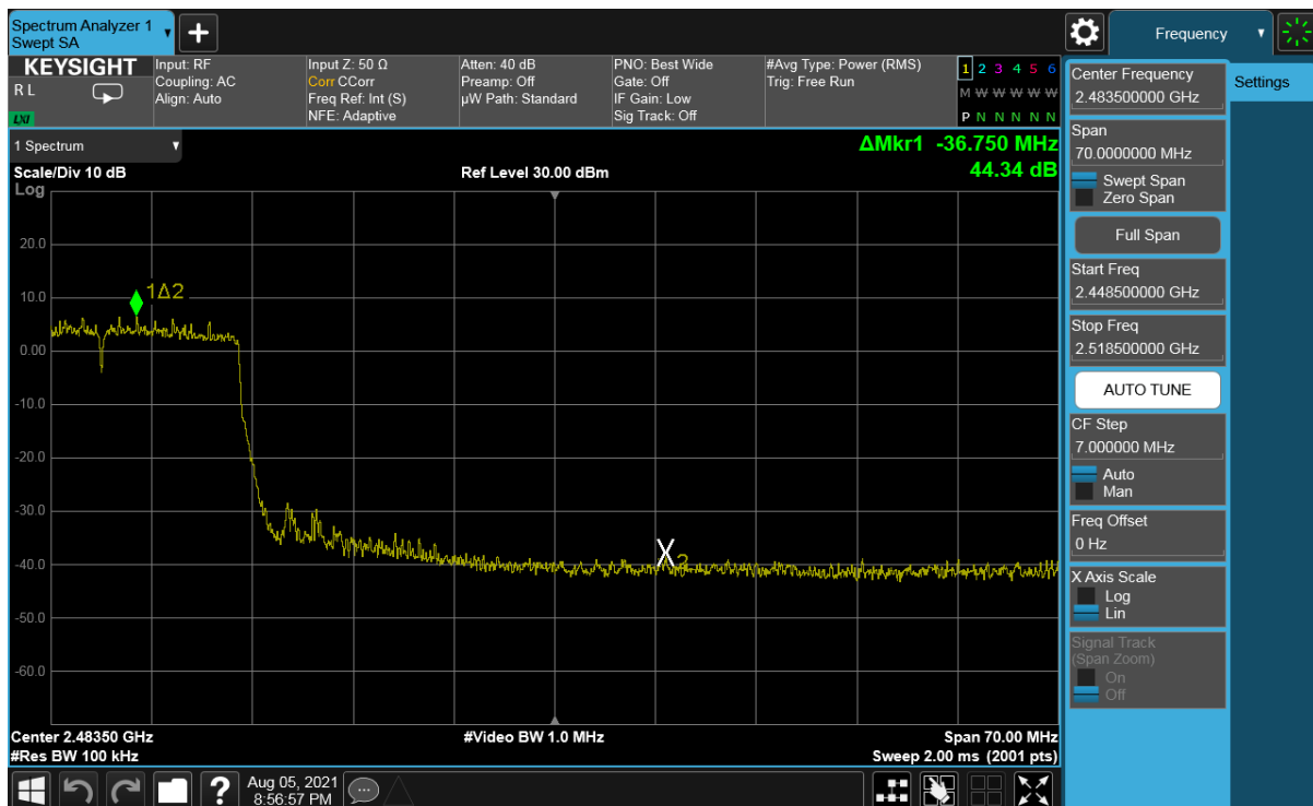
Plot 7-296. Band Edge Plot Antenna WF8 (802.11ax (SU - 2.4GHz) – Ch. 9) – MCS5
