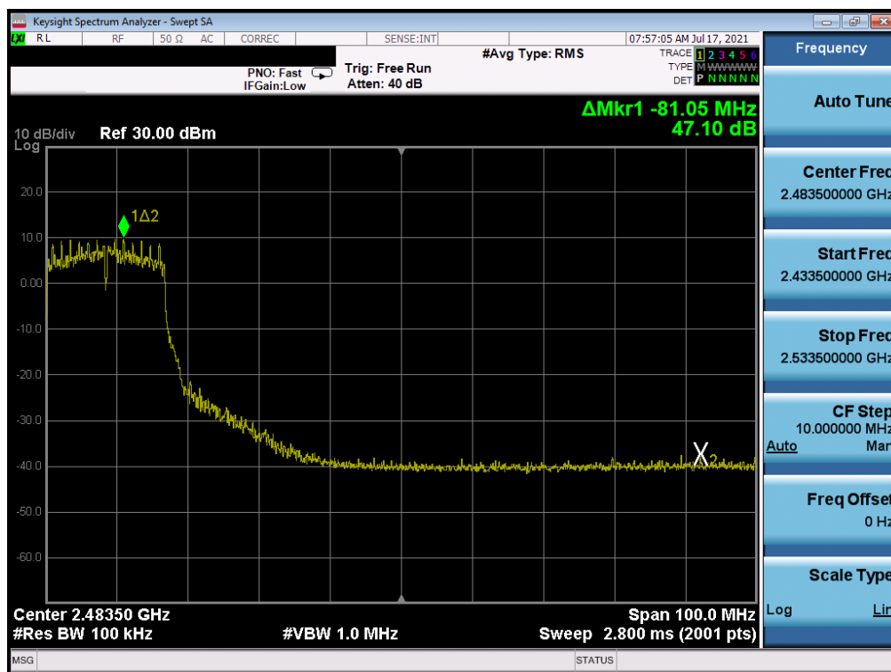
Plot 7-391. Band Edge Plot Antenna WF7 (802.11g - Ch. 7) - 36Mbps
