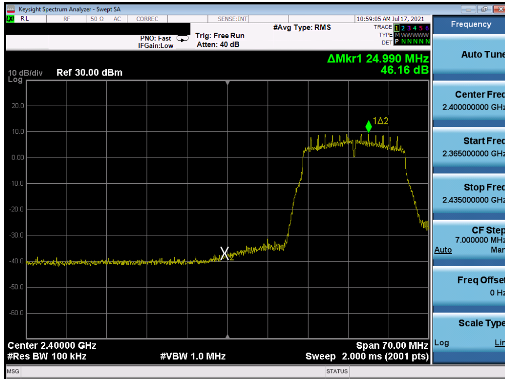
Plot 7-316. Band Edge Plot Antenna WF7 (802.11n (2.4GHz) - Ch. 3) - MCS2
