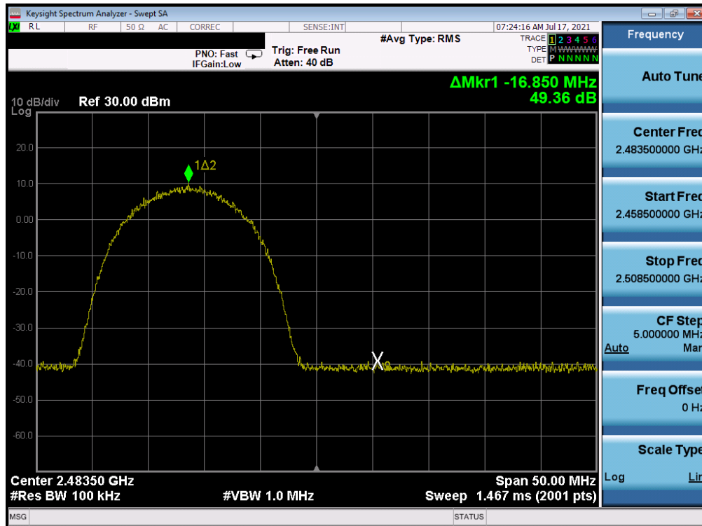
Plot 7-383. Band Edge Plot Antenna WF7 (802.11b – Ch. 13) – 11Mbps
