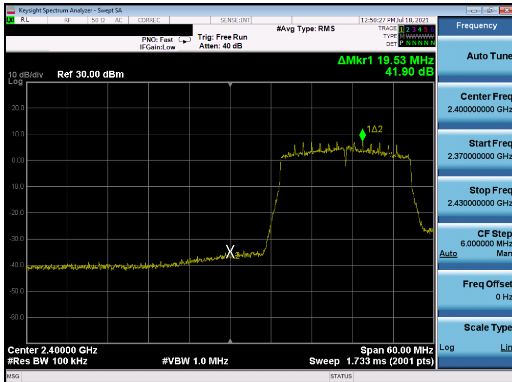
Plot 7-326. Band Edge Plot Antenna WF7 (802.11ax (SU - 2.4GHz) – Ch. 2) – MCS2
