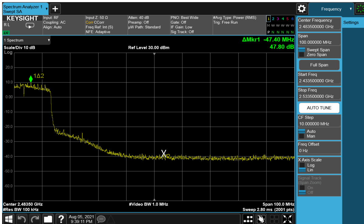
Plot 7-368. Band Edge Plot Antenna WF7 (802.11ax (SU - 2.4GHz) – Ch. 6(High)) – MCS4
