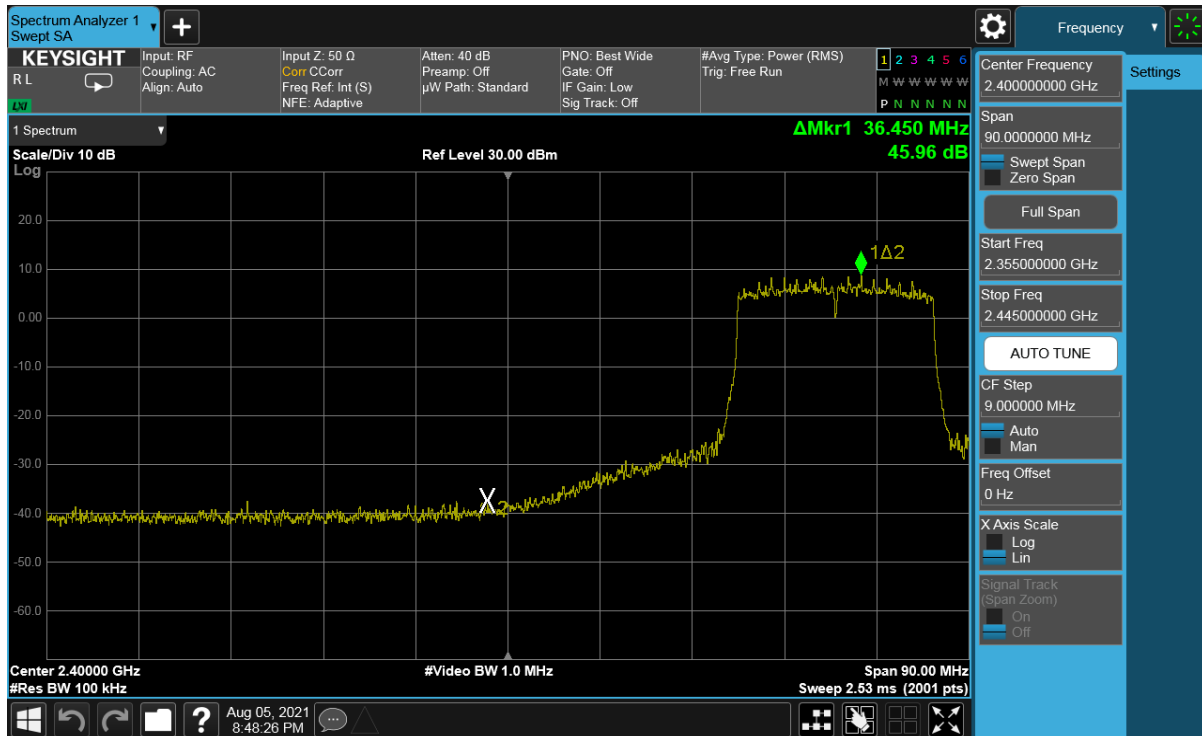
Plot 7-291. Band Edge Plot Antenna WF8 (802.11ax (SU - 2.4GHz) – Ch. 5) – MCS5
