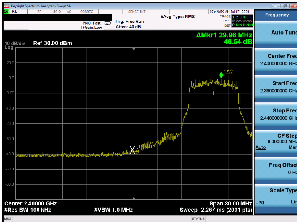
Plot 7-387. Band Edge Plot Antenna WF7 (802.11g- Ch. 4) – 36Mbps
