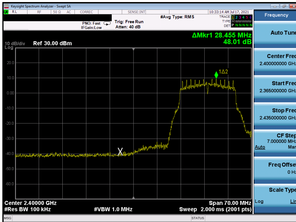
Plot 7-302. Band Edge Plot Antenna WF7 (802.11g- Ch. 3) - 12Mbps
