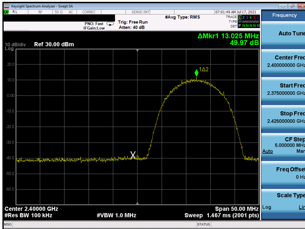
Plot 7-375. Band Edge Plot Antenna WF7 (802.11b – Ch. 1) – 11Mbps
