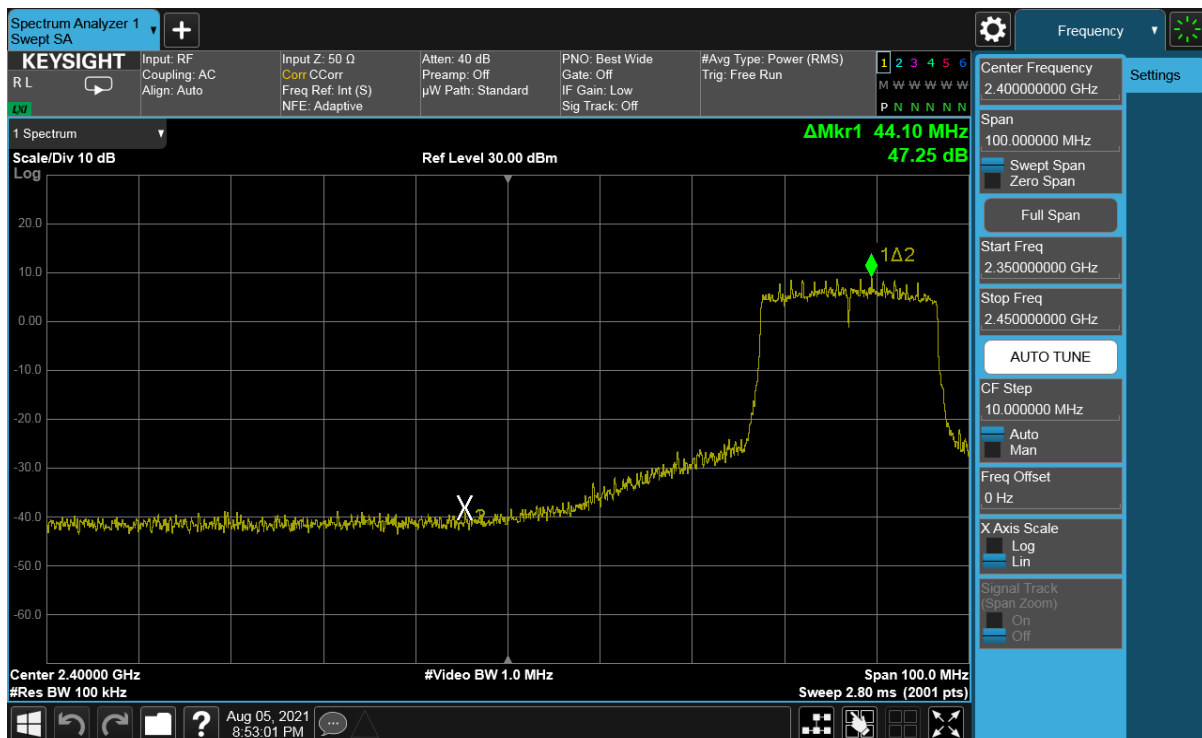
Plot 7-292. Band Edge Plot Antenna WF8 (802.11ax (SU - 2.4GHz) – Ch. 6 (Low)) – MCS5
