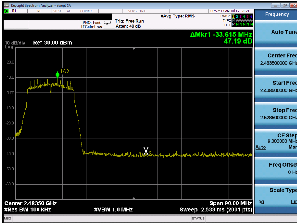
Plot 7-320. Band Edge Plot Antenna WF7 (802.11n (2.4GHz) - Ch. 9) - MCS2
