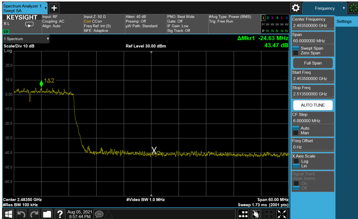
Plot 7-297. Band Edge Plot Antenna WF8 (802.11ax (SU - 2.4GHz) – Ch. 10) – MCS5
