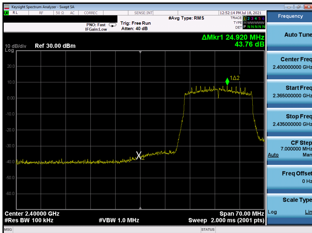
Plot 7-327. Band Edge Plot Antenna WF7 (802.11ax (SU - 2.4GHz) – Ch. 3) – MCS2
