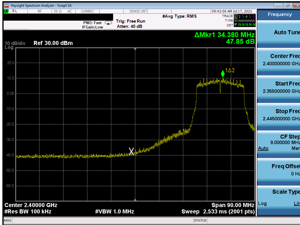
Plot 7-354. Band Edge Plot Antenna WF7 (802.11n (2.4GHz) - Ch. 5) - MCS4
