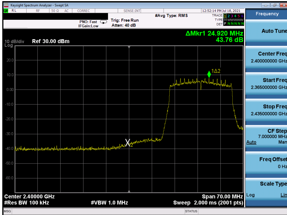
Plot 7-328. Band Edge Plot Antenna WF7 (802.11ax (SU - 2.4GHz) – Ch. 4) – MCS2
