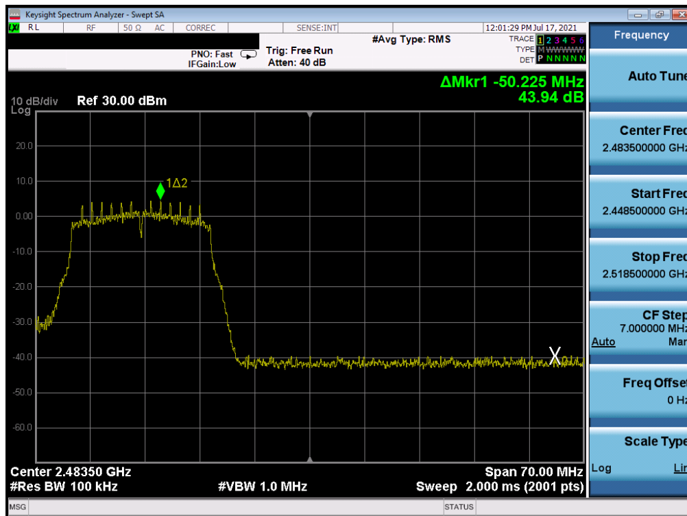
Plot 7-322. Band Edge Plot Antenna WF7 (802.11n (2.4GHz) – Ch. 11) – MCS2
