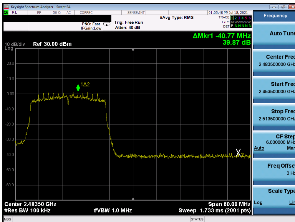
Plot 7-335. Band Edge Plot Antenna WF7 (802.11ax (SU - 2.4GHz) – Ch. 12) – MCS2
