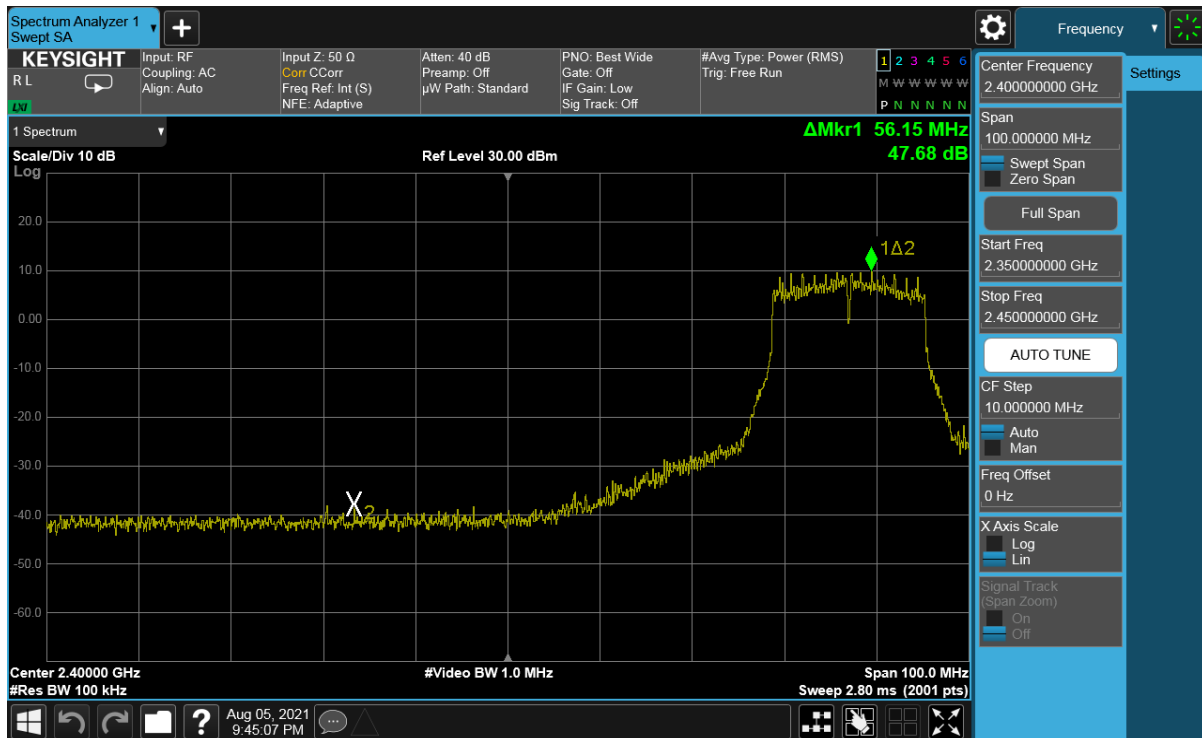
Plot 7-341. Band Edge Plot Antenna WF7 (802.11g- Ch. 6(Low)) – 24Mbps
