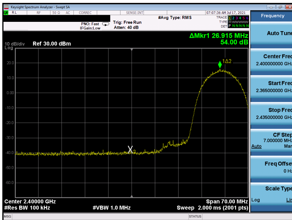
Plot 7-378. Band Edge Plot Antenna WF7 (802.11b – Ch. 4) – 11Mbps
