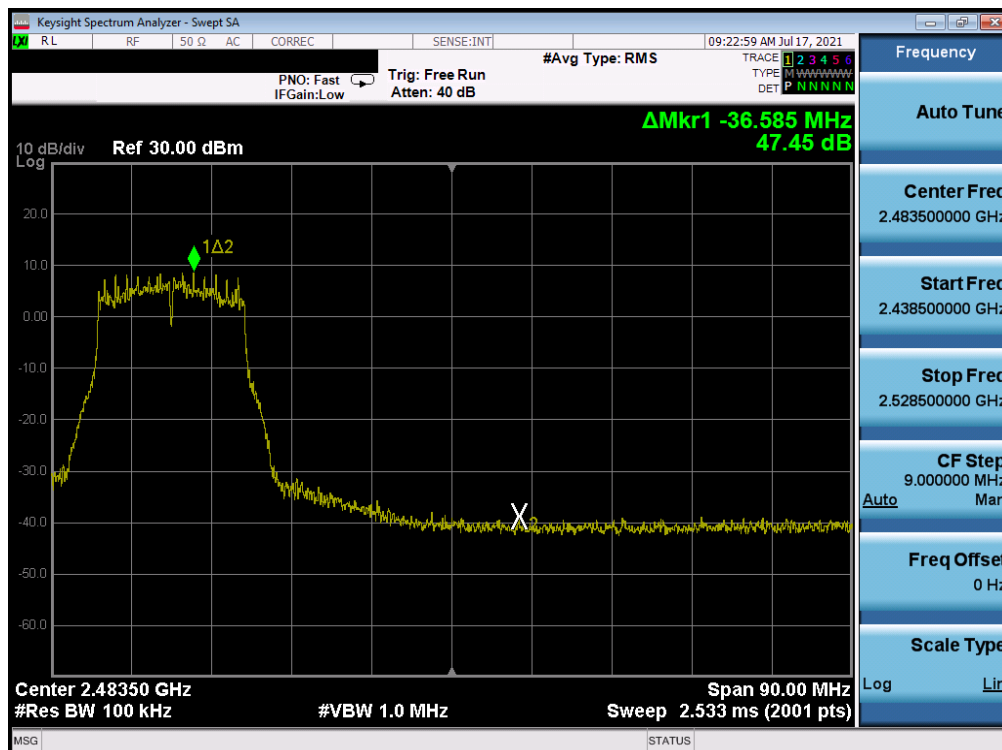
Plot 7-345. Band Edge Plot Antenna WF7 (802.11g - Ch. 9) - 24Mbps
