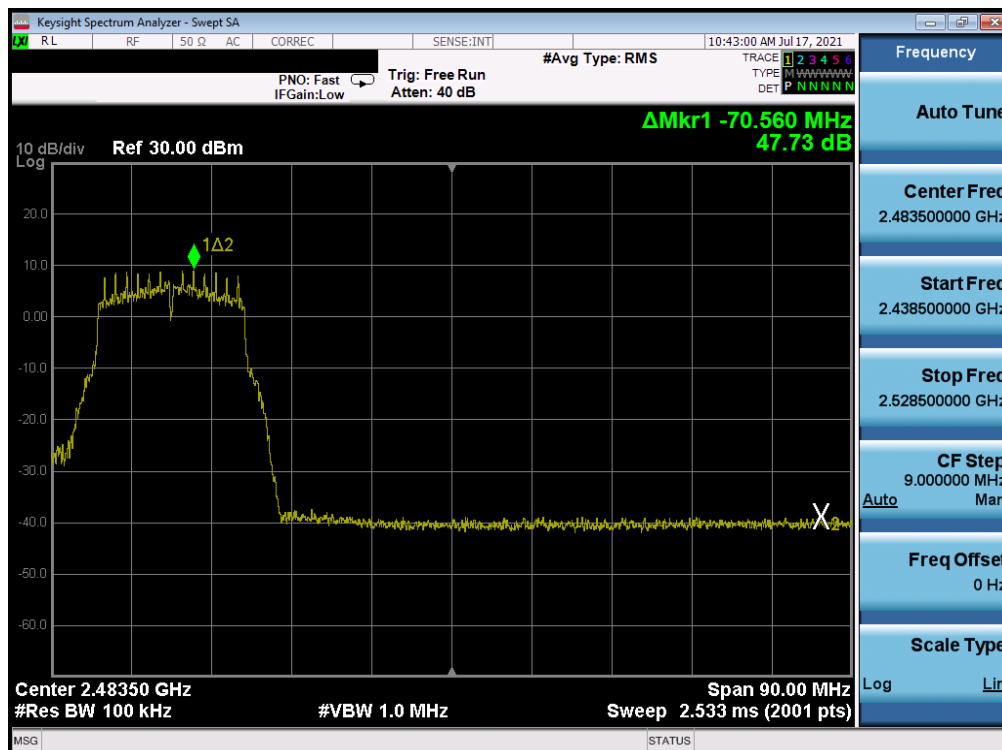
Plot 7-309. Band Edge Plot Antenna WF7 (802.11g - Ch. 9) - 12Mbps
