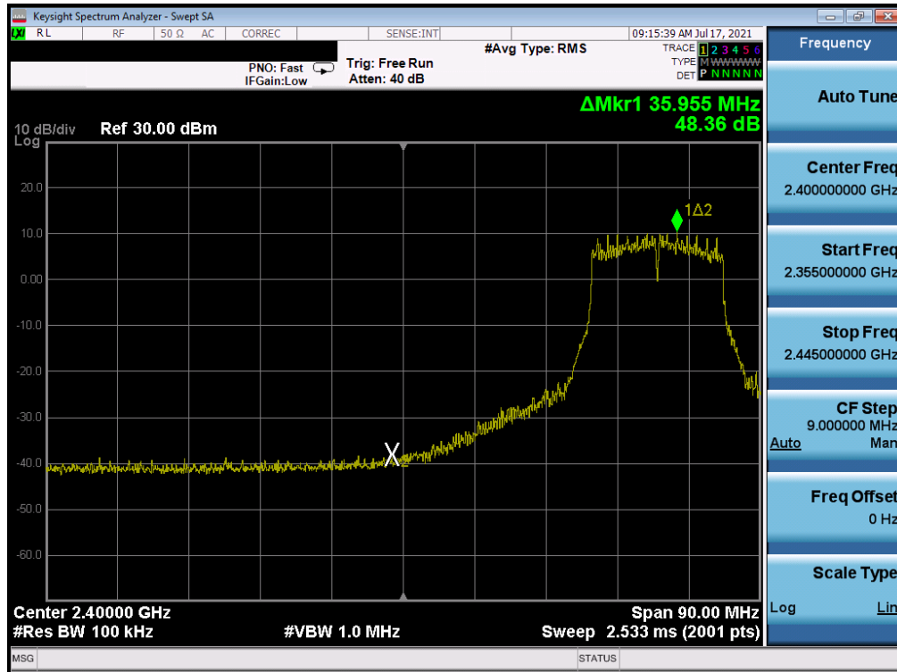
Plot 7-340. Band Edge Plot Antenna WF7 (802.11g- Ch. 5) – 24Mbps
