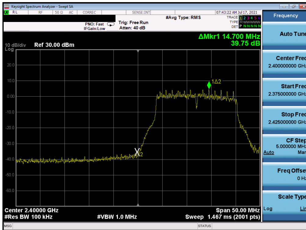
Plot 7-384. Band Edge Plot Antenna WF7 (802.11g- Ch. 1) - 36Mbps
