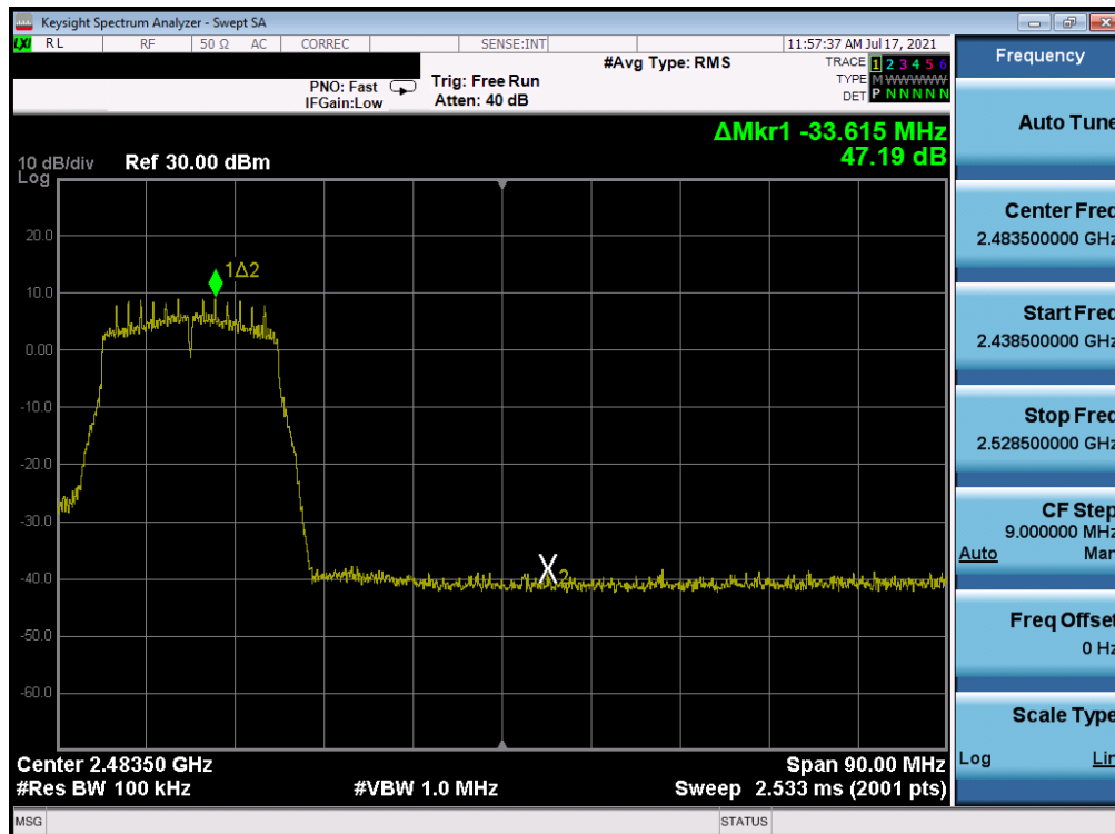
Plot 7-319. Band Edge Plot Antenna WF7 (802.11n (2.4GHz) - Ch. 8) - MCS2
