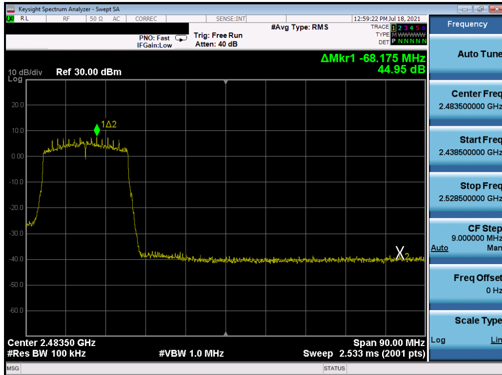
Plot 7-332. Band Edge Plot Antenna WF7 (802.11ax (SU - 2.4GHz) – Ch. 9) – MCS2
