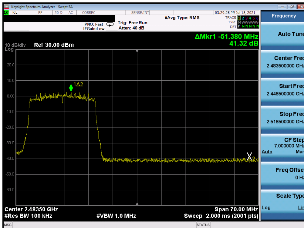
Plot 7-373. Band Edge Plot Antenna WF7 (802.11ax (SU - 2.4GHz) – Ch. 11) – MCS4
