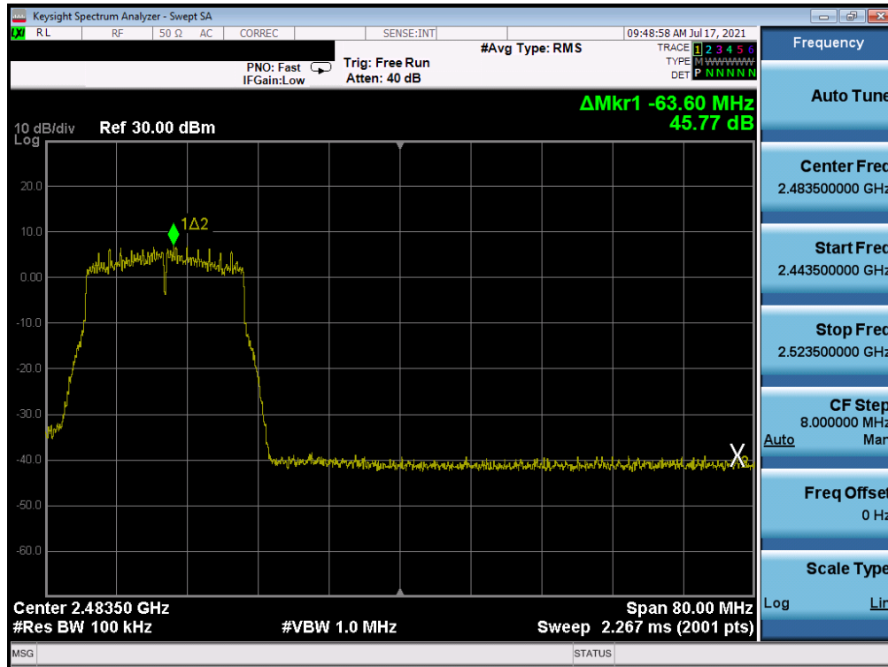
Plot 7-358. Band Edge Plot Antenna WF7 (802.11n (2.4GHz) - Ch. 10) - MCS4
