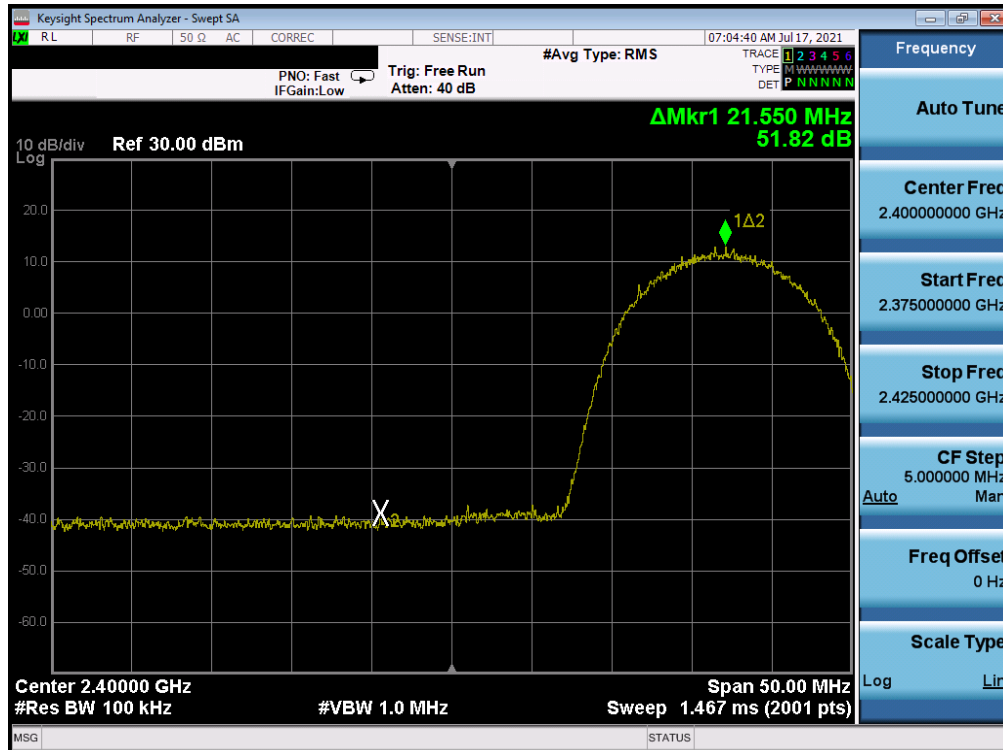
Plot 7-376. Band Edge Plot Antenna WF7 (802.11b – Ch. 2) – 11Mbps
