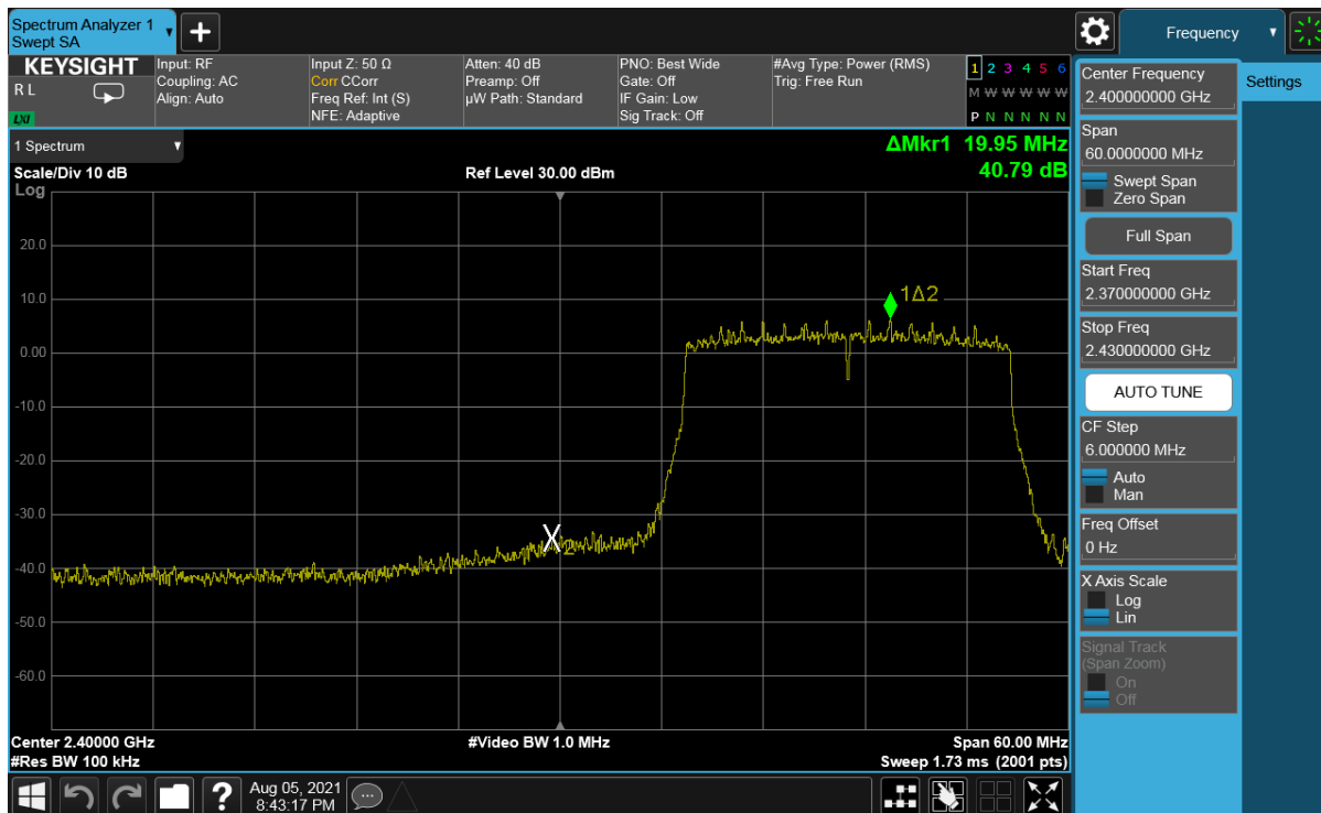
Plot 7-288. Band Edge Plot Antenna WF8 (802.11ax (SU - 2.4GHz) – Ch. 2) – MCS5
