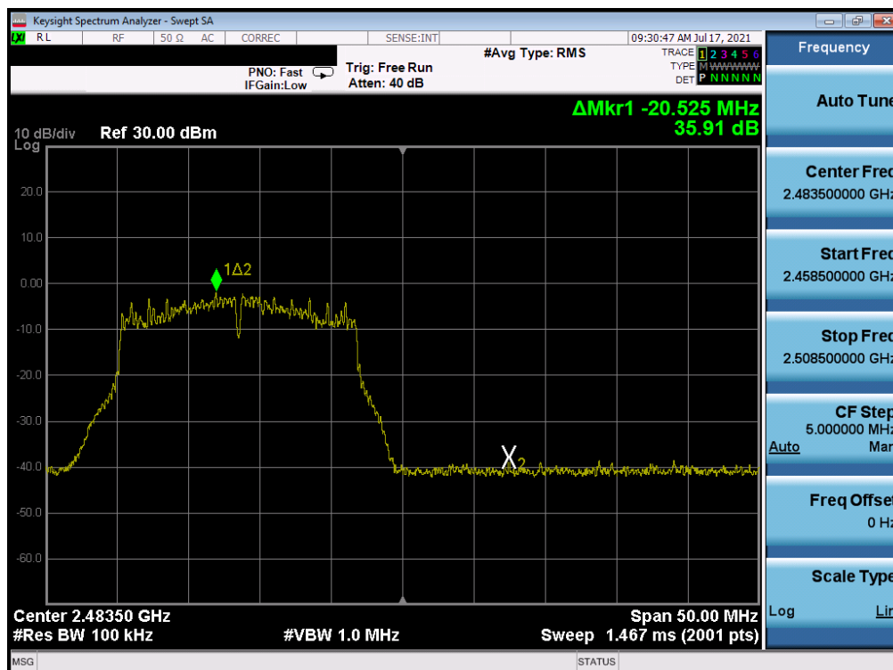
Plot 7-349. Band Edge Plot Antenna WF7 (802.11g - Ch. 13) - 24Mbps
