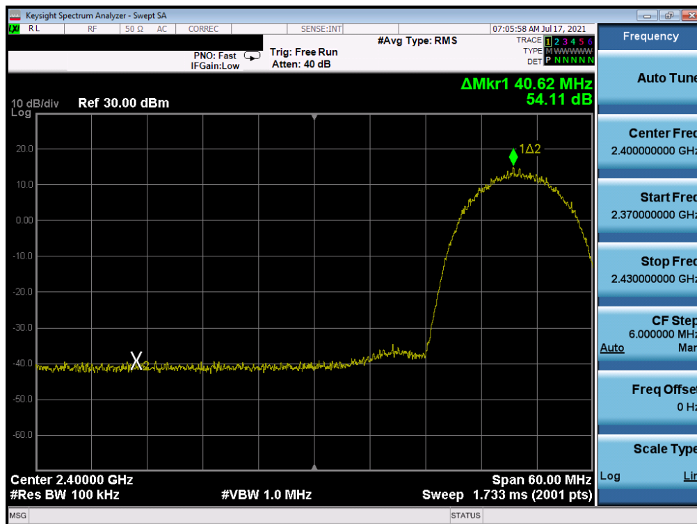
Plot 7-377. Band Edge Plot Antenna WF7 (802.11b – Ch. 3) – 11Mbps
