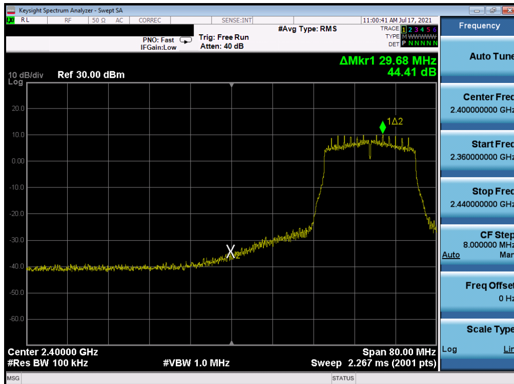
Plot 7-317. Band Edge Plot Antenna WF7 (802.11n (2.4GHz) - Ch. 4) - MCS2
