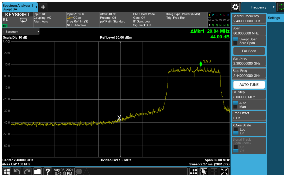
Plot 7-290. Band Edge Plot Antenna WF8 (802.11ax (SU - 2.4GHz) – Ch. 4) – MCS5
