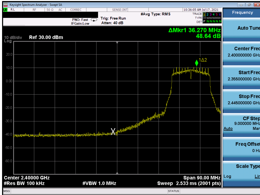
Plot 7-304. Band Edge Plot Antenna WF7 (802.11g- Ch. 5) – 12Mbps
