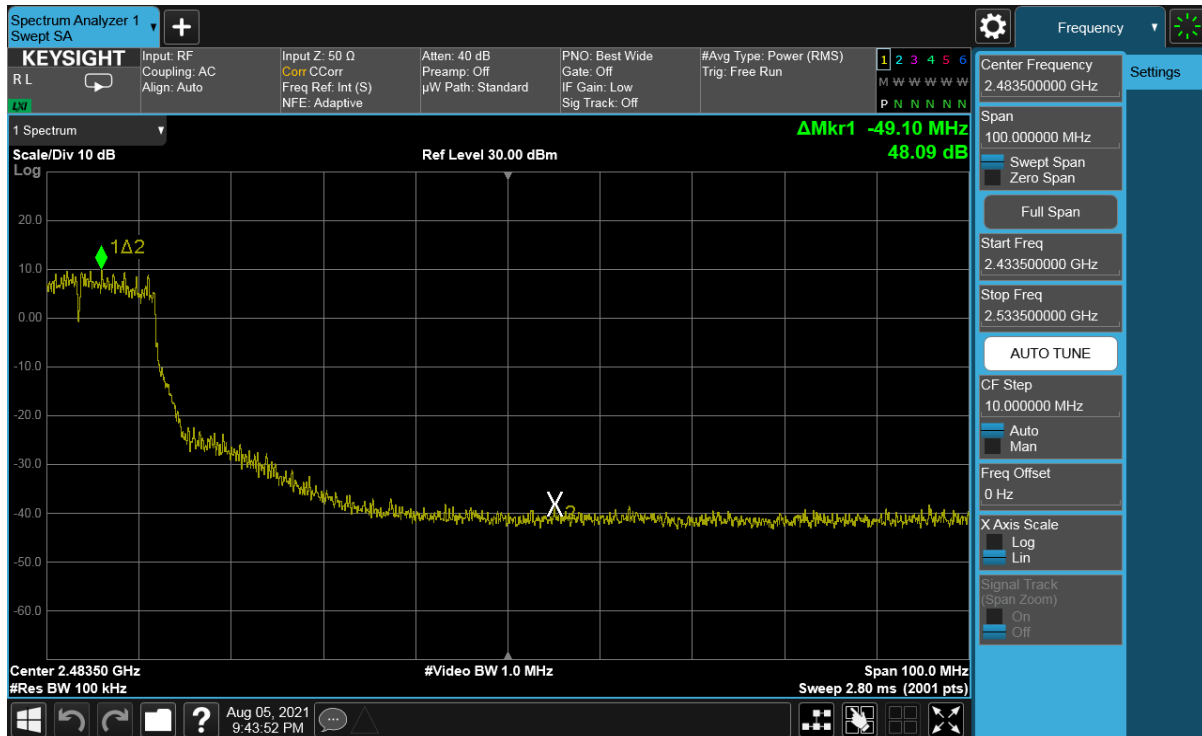
Plot 7-342. Band Edge Plot Antenna WF7 (802.11g - Ch. 6(High)) - 24Mbps
