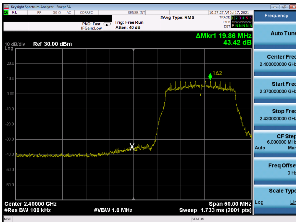
Plot 7-315. Band Edge Plot Antenna WF7 (802.11n (2.4GHz) – Ch. 2) – MCS2
