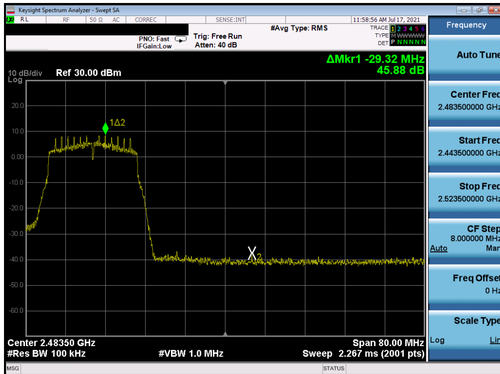
Plot 7-321. Band Edge Plot Antenna WF7 (802.11n (2.4GHz) - Ch. 10) - MCS2
