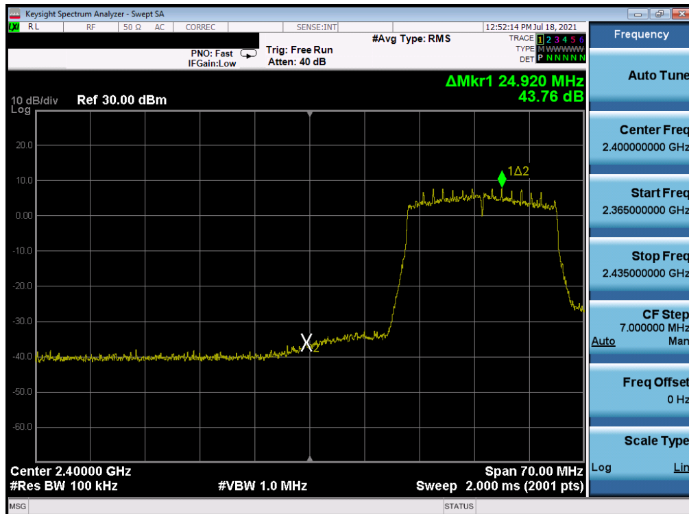
Plot 7-329. Band Edge Plot Antenna WF7 (802.11ax (SU - 2.4GHz) – Ch. 5) – MCS2
