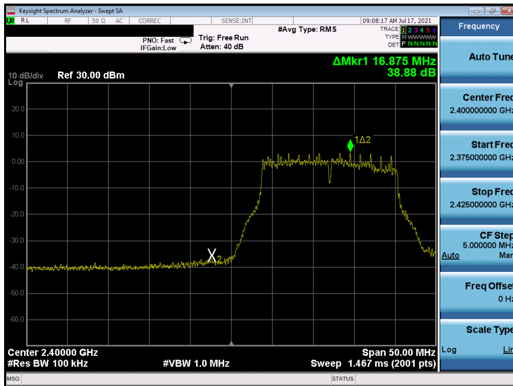
Plot 7-336. Band Edge Plot Antenna WF7 (802.11g- Ch. 1) – 24Mbps
