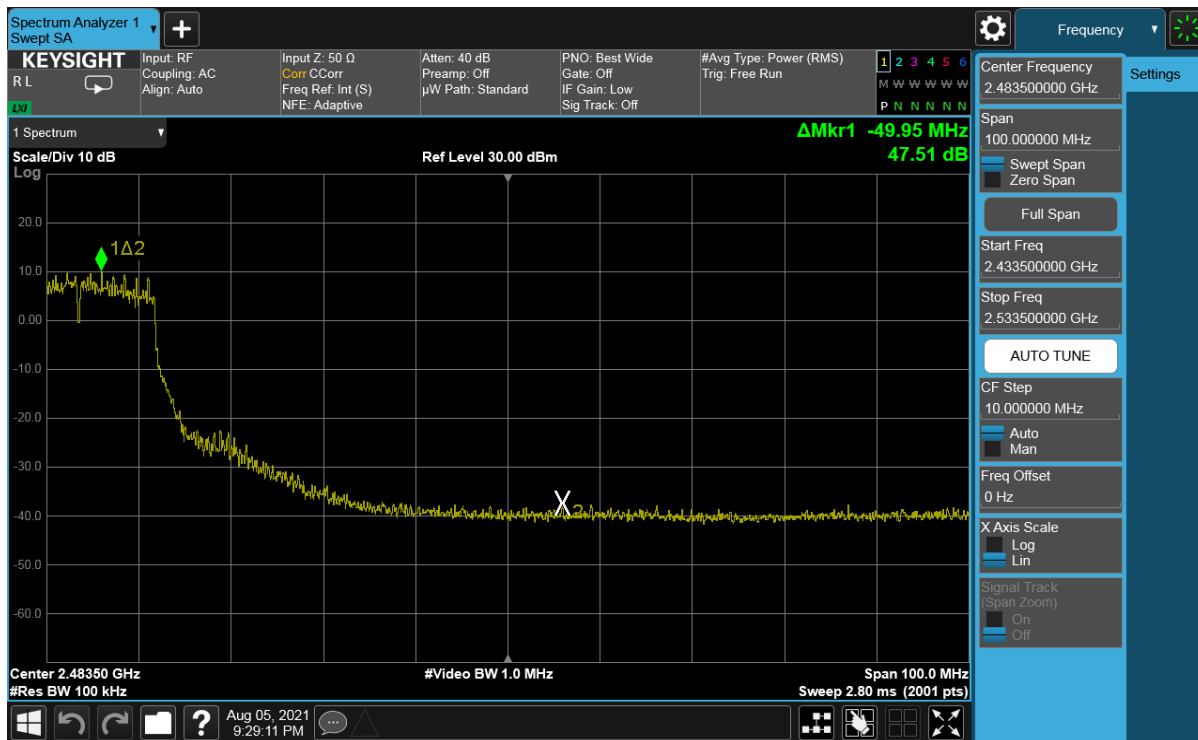
Plot 7-390. Band Edge Plot Antenna WF7 (802.11g - Ch. 6(High)) - 36Mbps
