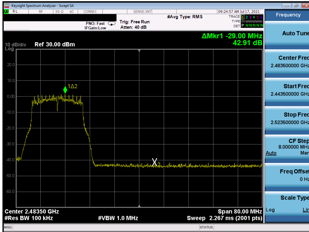
Plot 7-346. Band Edge Plot Antenna WF7 (802.11g - Ch. 10) - 24Mbps
