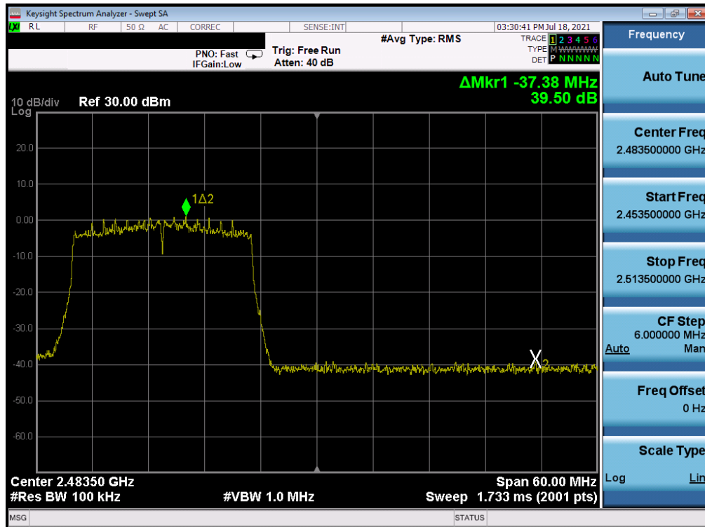
Plot 7-374. Band Edge Plot Antenna WF7 (802.11ax (SU - 2.4GHz) – Ch. 12) – MCS4
