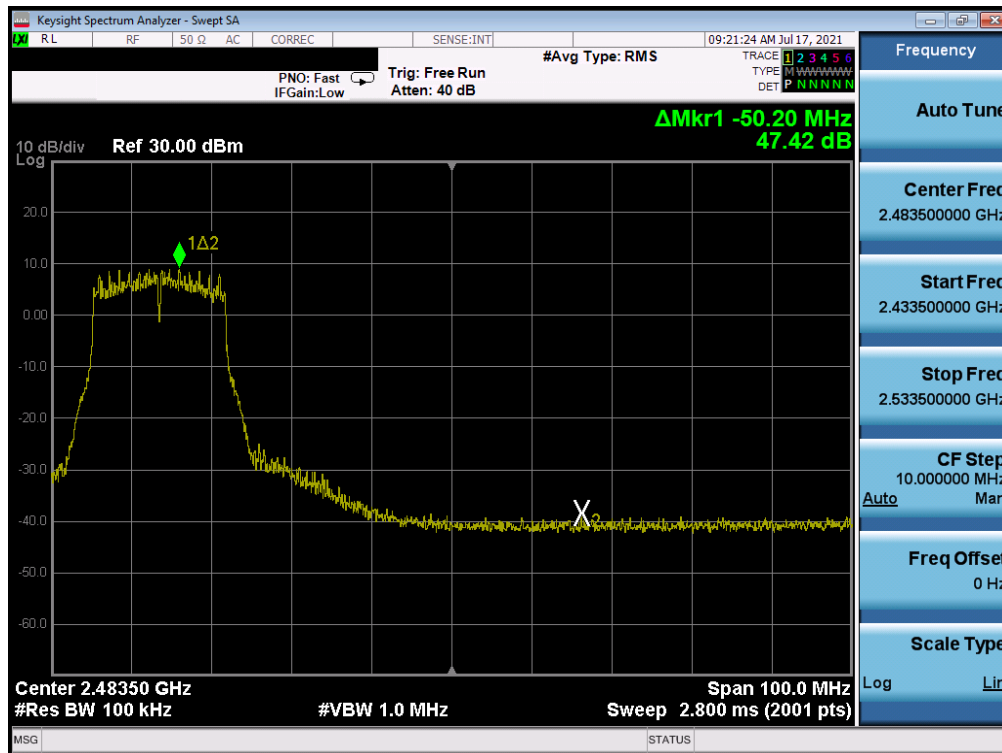
Plot 7-344. Band Edge Plot Antenna WF7 (802.11g - Ch. 8) - 24Mbps
