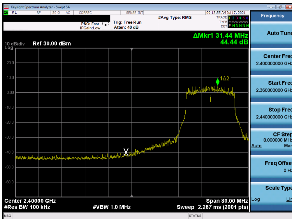
Plot 7-339. Band Edge Plot Antenna WF7 (802.11g- Ch. 4) – 24Mbps
