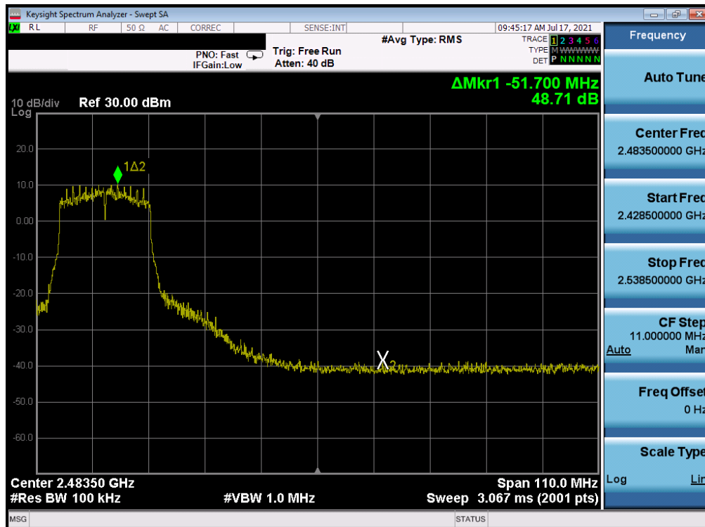
Plot 7-355. Band Edge Plot Antenna WF7 (802.11n (2.4GHz) - Ch. 7) - MCS4
