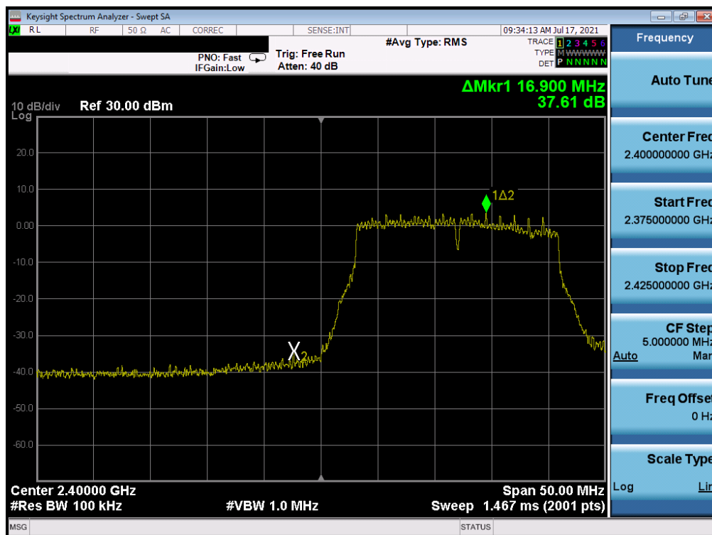
Plot 7-350. Band Edge Plot Antenna WF7 (802.11n (2.4GHz) – Ch. 1) – MCS4
