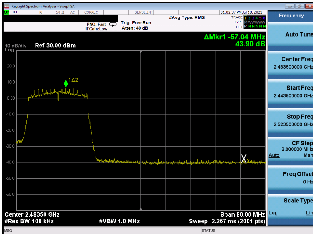
Plot 7-333. Band Edge Plot Antenna WF7 (802.11ax (SU - 2.4GHz) – Ch. 10) – MCS2
