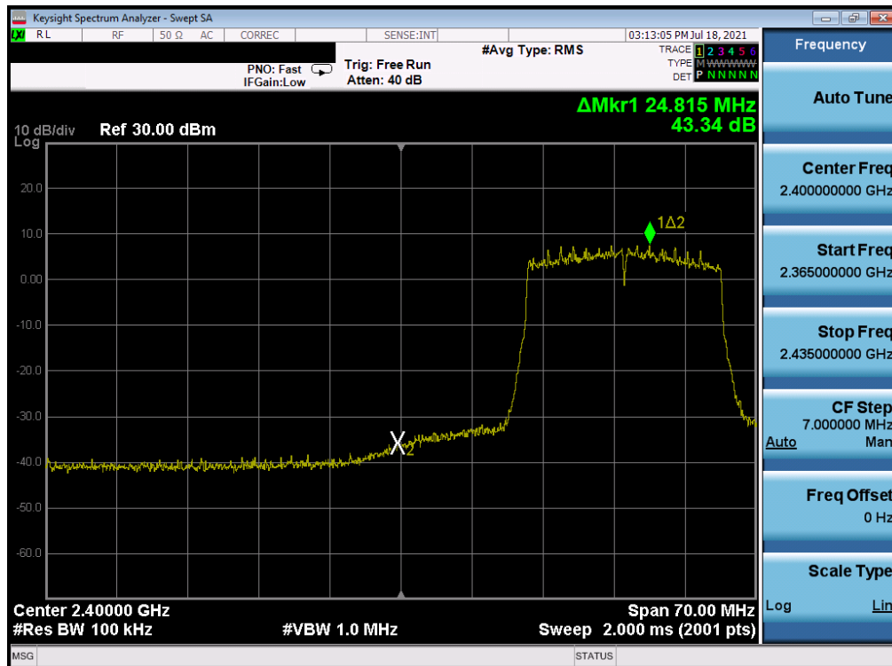
Plot 7-364. Band Edge Plot Antenna WF7 (802.11ax (SU - 2.4GHz) – Ch. 3) – MCS4
