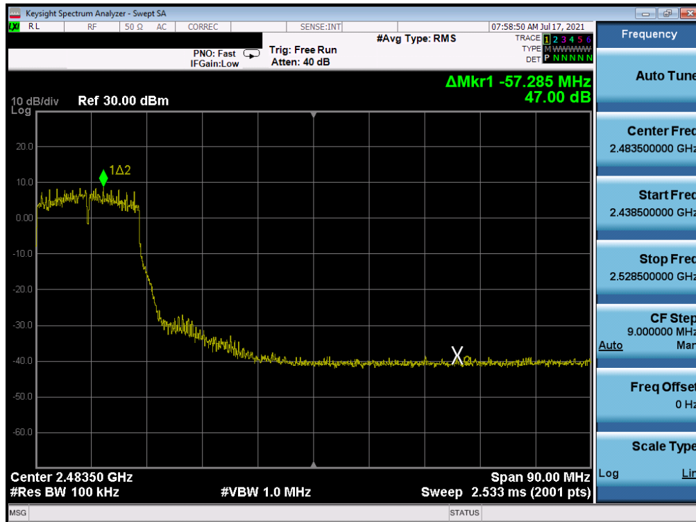
Plot 7-392. Band Edge Plot Antenna WF7 (802.11g - Ch. 8) - 36Mbps
