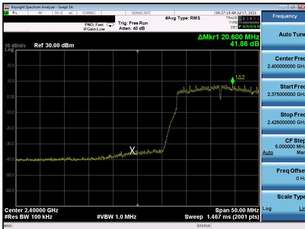
Plot 7-351. Band Edge Plot Antenna WF7 (802.11n (2.4GHz) – Ch. 2) – MCS4
