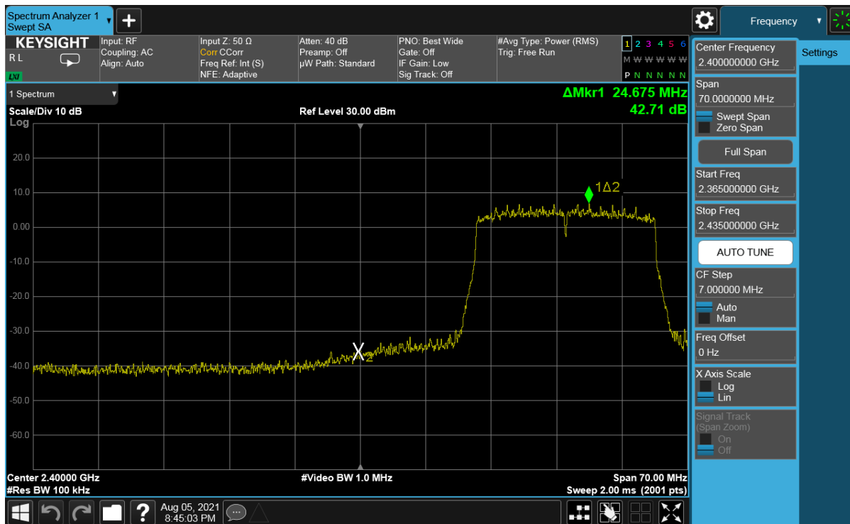
Plot 7-289. Band Edge Plot Antenna WF8 (802.11ax (SU - 2.4GHz) – Ch. 3) – MCS5
