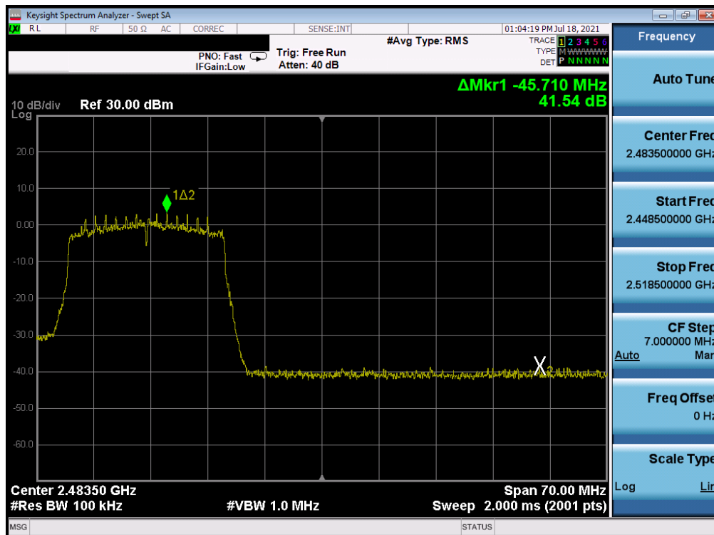
Plot 7-334. Band Edge Plot Antenna WF7 (802.11ax (SU - 2.4GHz) – Ch. 11) – MCS2
