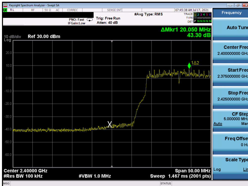
Plot 7-385. Band Edge Plot Antenna WF7 (802.11g- Ch. 2) - 36Mbps
