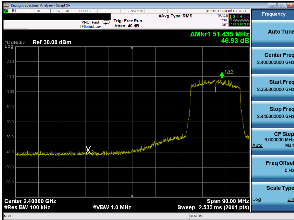
Plot 7-366. Band Edge Plot Antenna WF7 (802.11ax (SU - 2.4GHz) – Ch. 5) – MCS4
