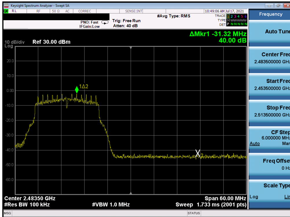
Plot 7-312. Band Edge Plot Antenna WF7 (802.11g - Ch. 12) - 12Mbps
