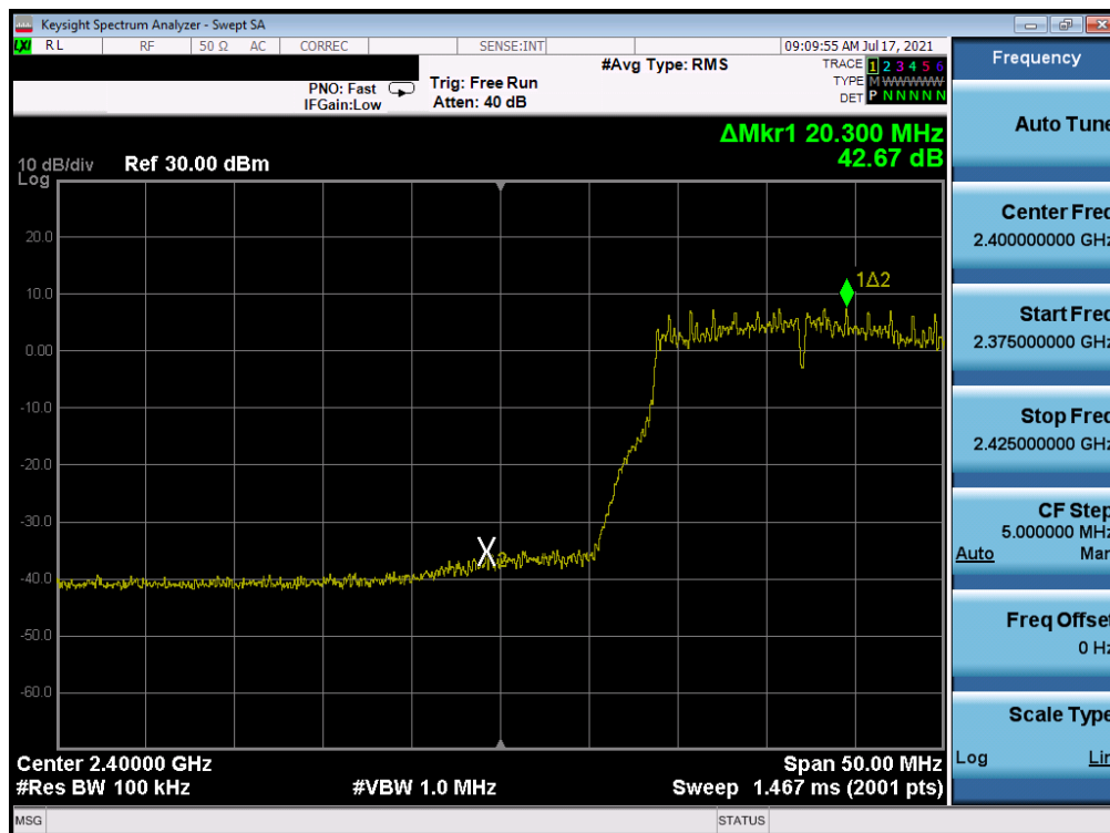
Plot 7-337. Band Edge Plot Antenna WF7 (802.11g- Ch. 2) – 24Mbps
