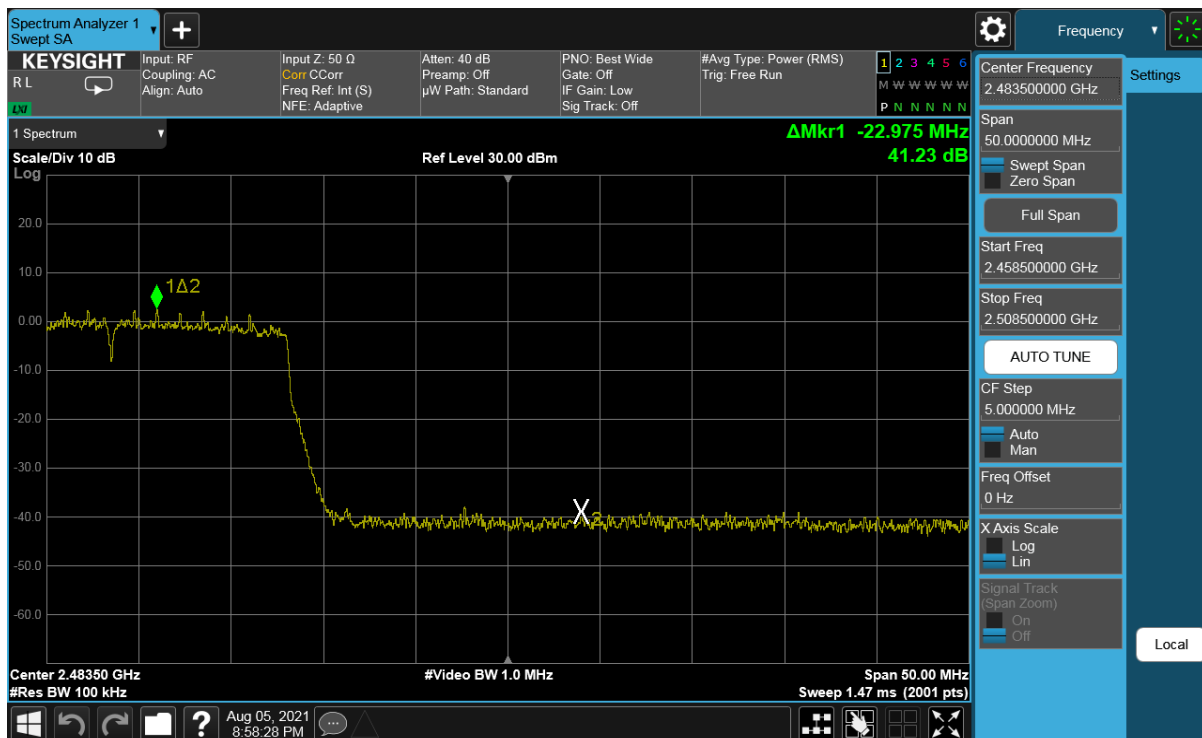
Plot 7-298. Band Edge Plot Antenna WF8 (802.11ax (SU - 2.4GHz) – Ch. 11) – MCS5
