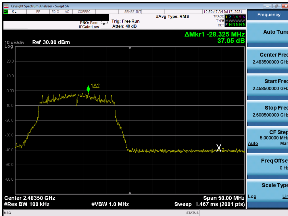
Plot 7-313. Band Edge Plot Antenna WF7 (802.11g - Ch. 13) - 12Mbps
