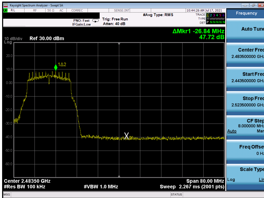
Plot 7-310. Band Edge Plot Antenna WF7 (802.11g - Ch. 10) - 12Mbps
