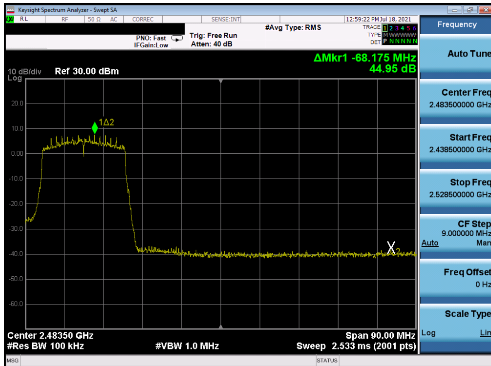
Plot 7-331. Band Edge Plot Antenna WF7 (802.11ax (SU - 2.4GHz) – Ch. 8) – MCS2
