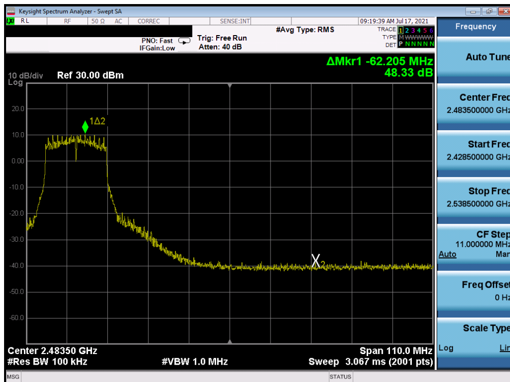
Plot 7-343. Band Edge Plot Antenna WF7 (802.11g - Ch. 7) - 24Mbps
