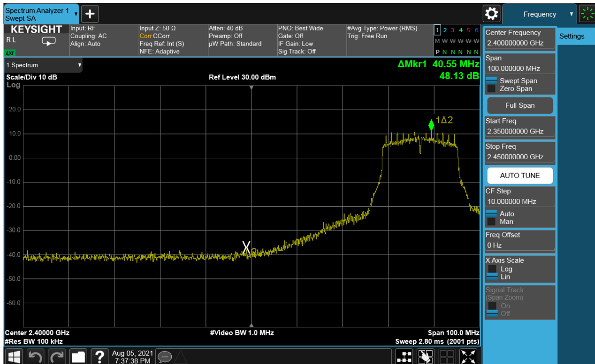
Plot 7-305. Band Edge Plot Antenna WF7 (802.11g- Ch. 6(Low)) – 12Mbps
