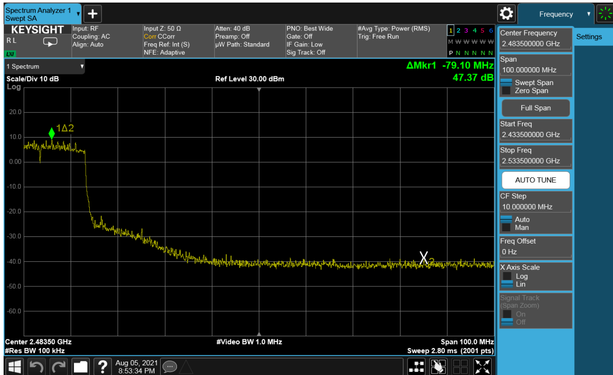
Plot 7-293. Band Edge Plot Antenna WF8 (802.11ax (SU - 2.4GHz) – Ch. 6(High)) – MCS5
