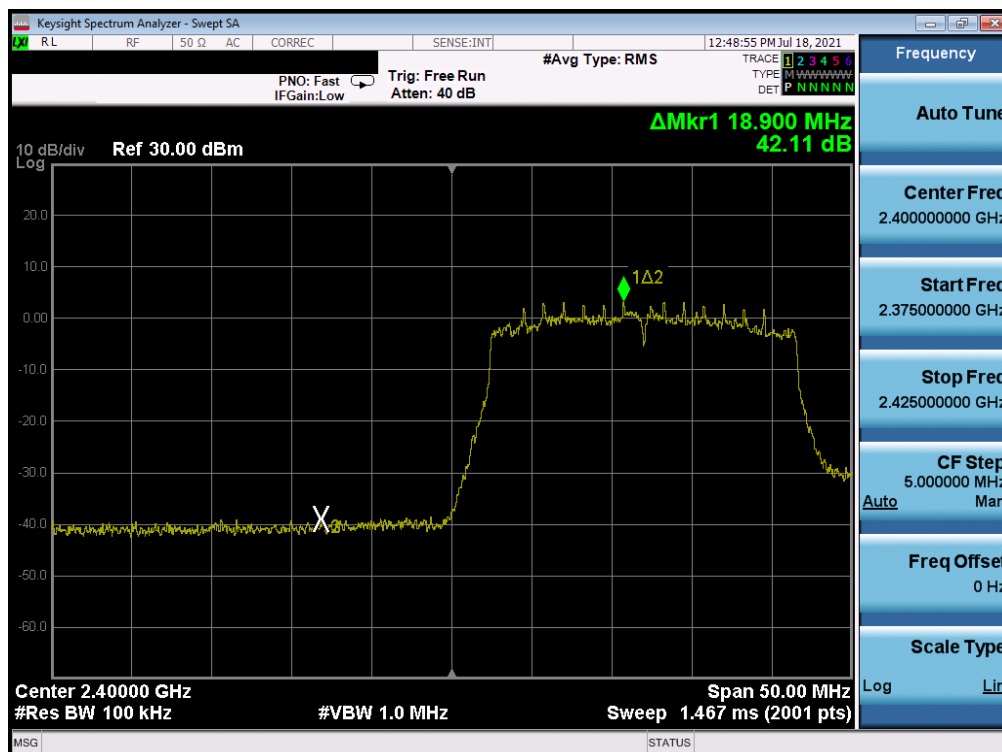
Plot 7-325. Band Edge Plot Antenna WF7 (802.11ax (SU - 2.4GHz) – Ch. 1) – MCS2
