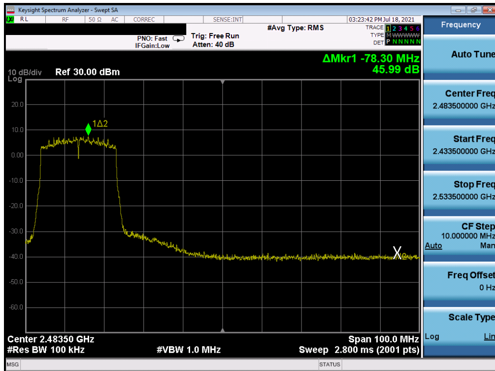
Plot 7-370. Band Edge Plot Antenna WF7 (802.11ax (SU - 2.4GHz) – Ch. 8) – MCS4
