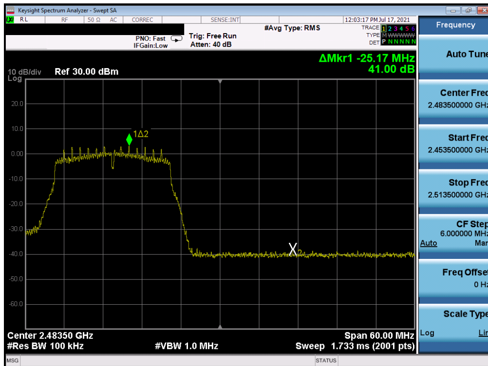
Plot 7-323. Band Edge Plot Antenna WF7 (802.11n (2.4GHz) – Ch. 12) – MCS2
