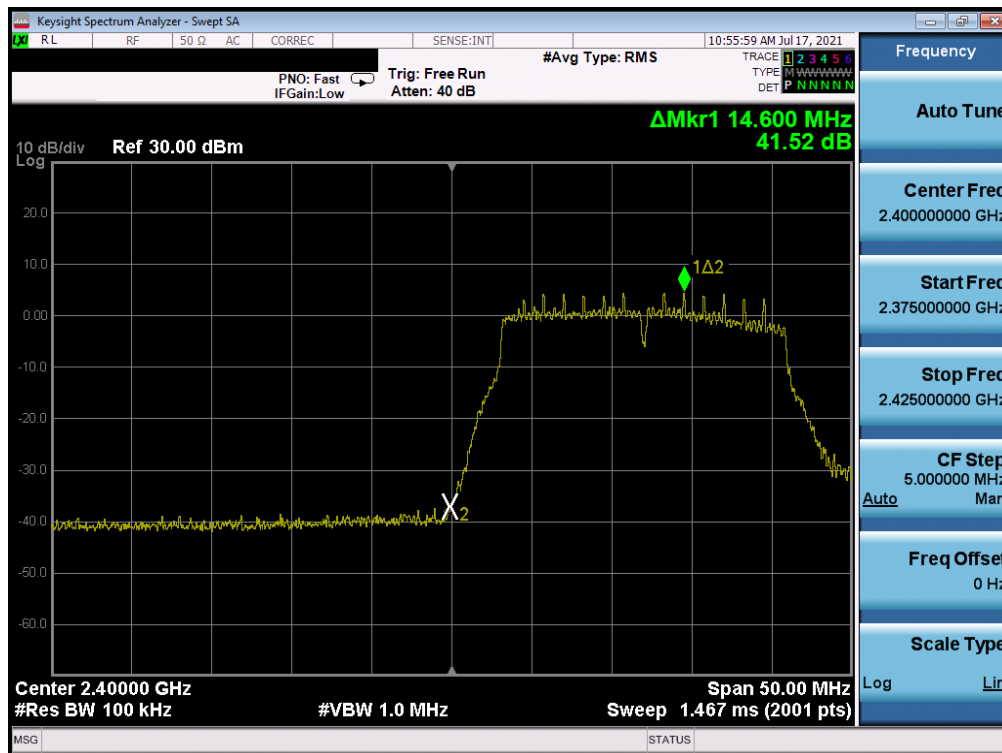
Plot 7-314. Band Edge Plot Antenna WF7 (802.11n (2.4GHz) – Ch. 1) – MCS2
