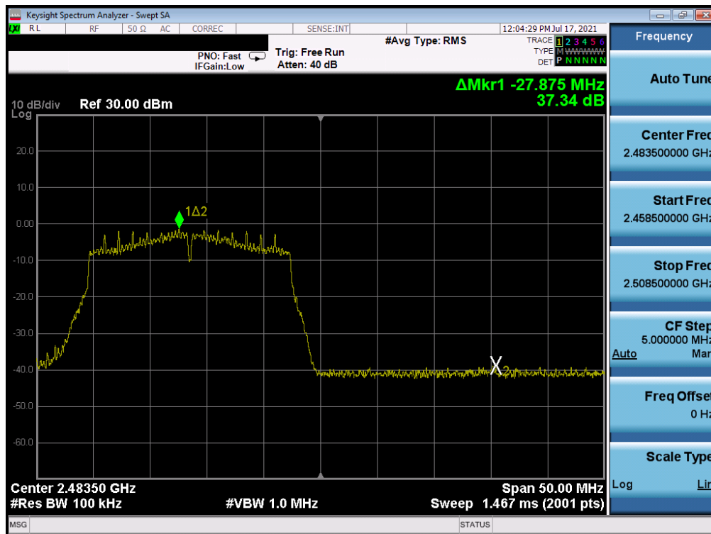
Plot 7-324. Band Edge Plot Antenna WF7 (802.11n (2.4GHz) – Ch. 13) – MCS2
