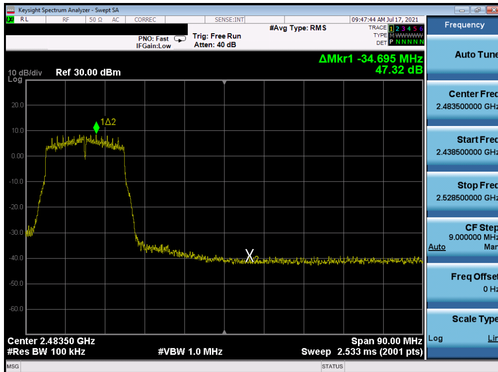
Plot 7-357. Band Edge Plot Antenna WF7 (802.11n (2.4GHz) - Ch. 9) - MCS4
