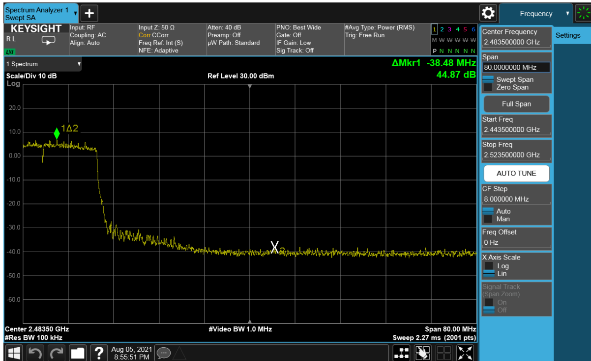
Plot 7-295. Band Edge Plot Antenna WF8 (802.11ax (SU - 2.4GHz) – Ch. 8) – MCS5
