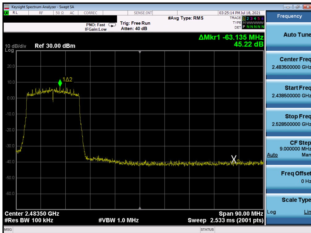
Plot 7-371. Band Edge Plot Antenna WF7 (802.11ax (SU - 2.4GHz) – Ch. 9) – MCS4
