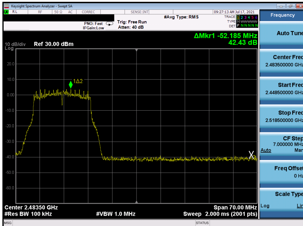
Plot 7-347. Band Edge Plot Antenna WF7 (802.11g - Ch. 11) - 24Mbps
