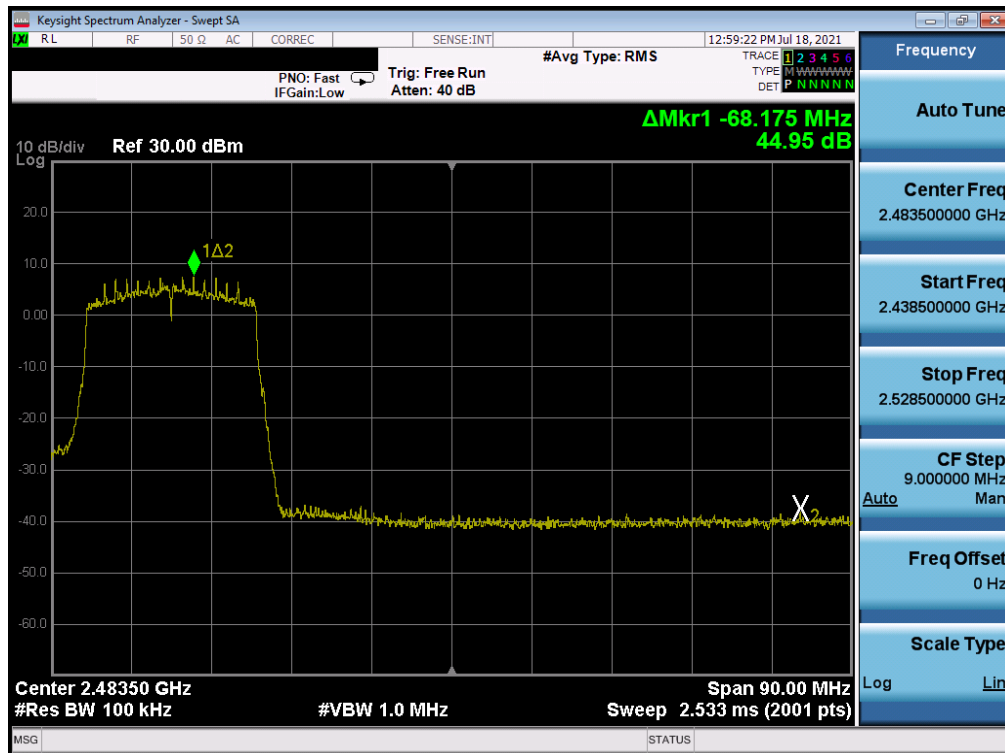
Plot 7-330. Band Edge Plot Antenna WF7 (802.11ax (SU - 2.4GHz) – Ch. 7) – MCS2
