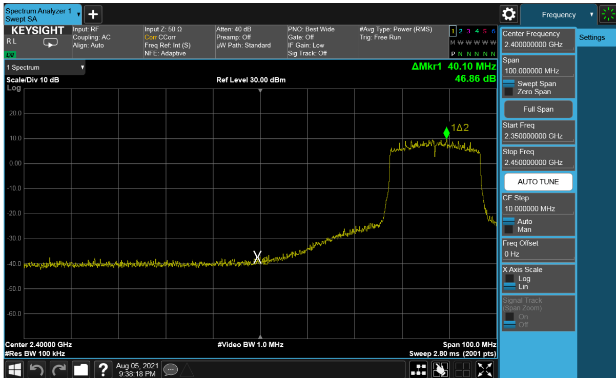
Plot 7-367. Band Edge Plot Antenna WF7 (802.11ax (SU - 2.4GHz) – Ch. 6(Low)) – MCS4
