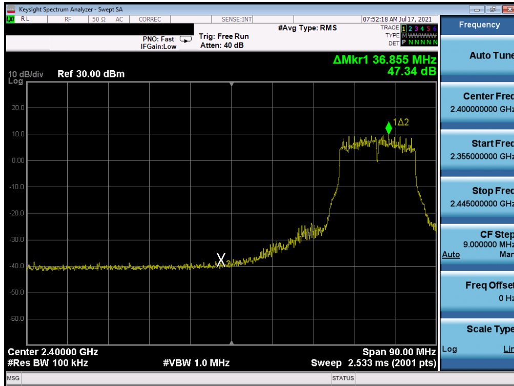
Plot 7-388. Band Edge Plot Antenna WF7 (802.11g- Ch. 5) – 36Mbps
