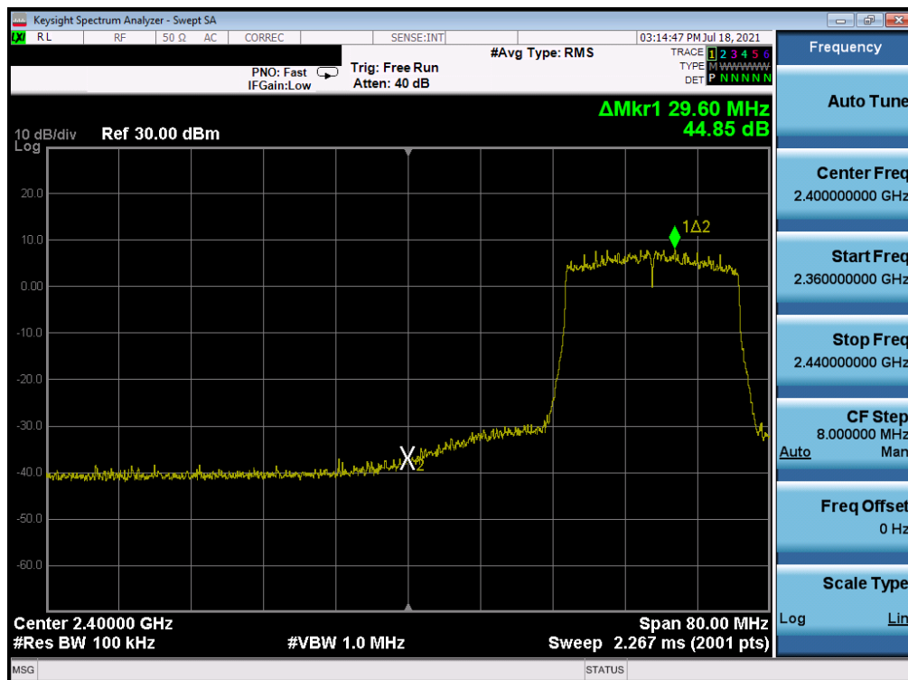
Plot 7-365. Band Edge Plot Antenna WF7 (802.11ax (SU - 2.4GHz) – Ch. 4) – MCS4
