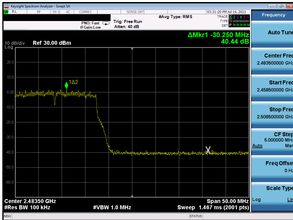
Plot 7-285. Band Edge Plot Antenna WF8 (802.11n (2.4GHz) – Ch. 12) – MCS5
