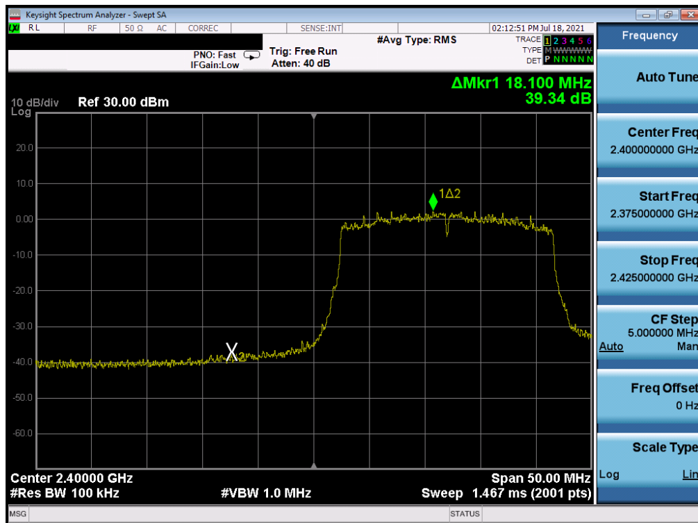
Plot 7-362. Band Edge Plot Antenna WF7 (802.11ax (SU - 2.4GHz) – Ch. 1) – MCS4
