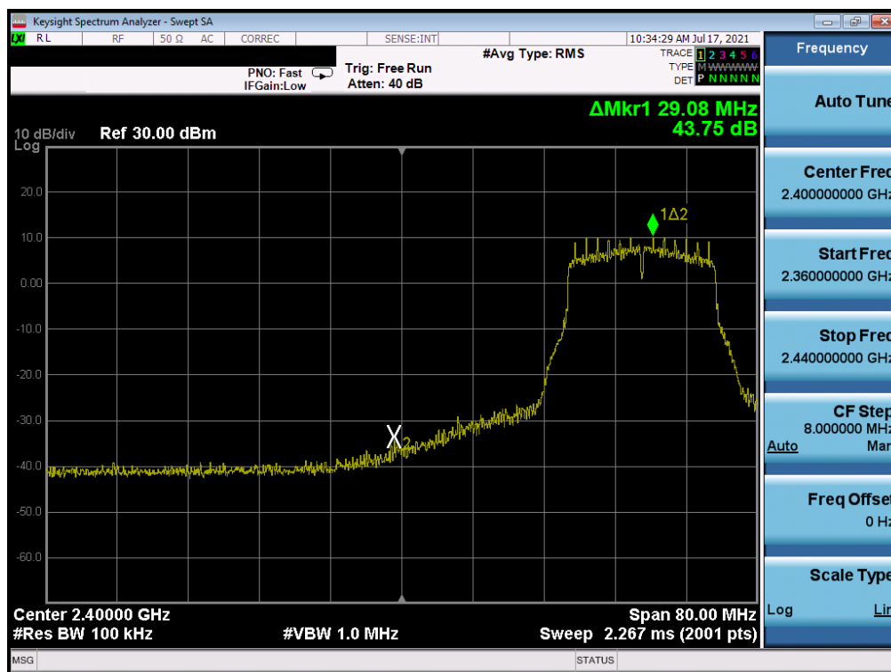
Plot 7-303. Band Edge Plot Antenna WF7 (802.11g- Ch. 4) - 12Mbps
