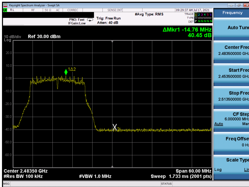
Plot 7-348. Band Edge Plot Antenna WF7 (802.11g - Ch. 12) - 24Mbps
