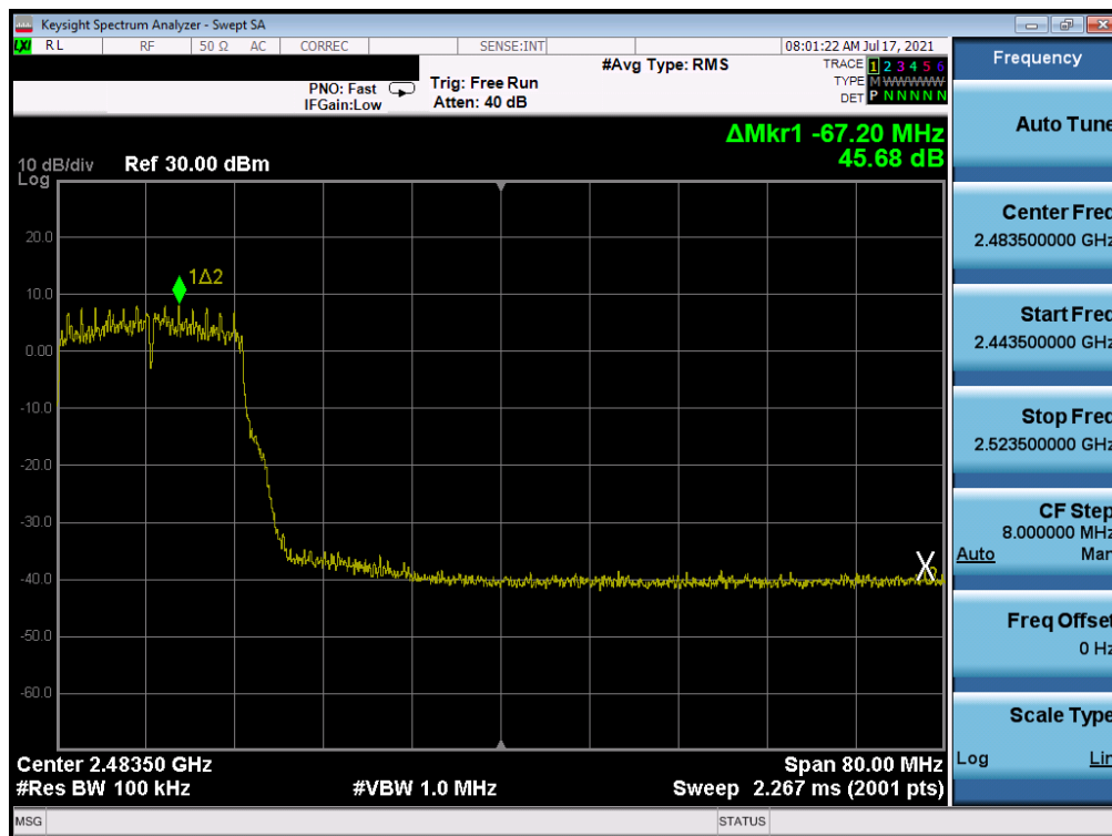
Plot 7-393. Band Edge Plot Antenna WF7 (802.11g - Ch. 9) - 36Mbps
