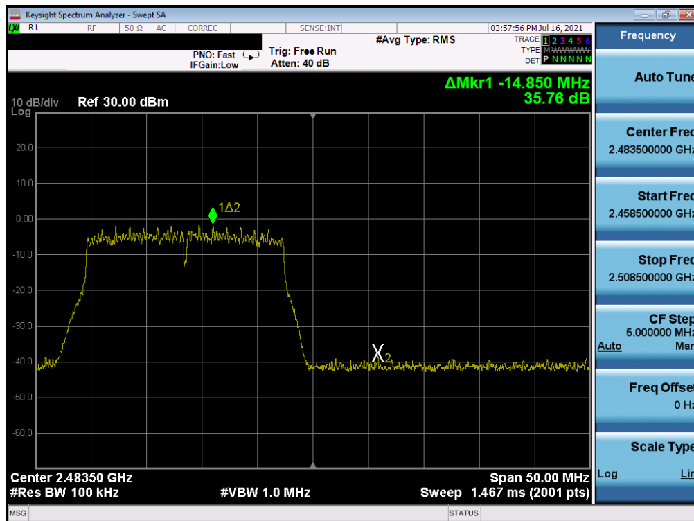
Plot 7-286. Band Edge Plot Antenna WF8 (802.11n (2.4GHz) – Ch. 13) – MCS5
