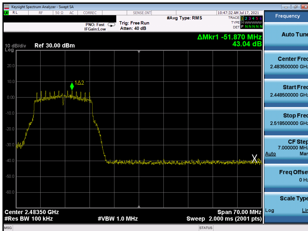
Plot 7-311. Band Edge Plot Antenna WF7 (802.11g - Ch. 11) - 12Mbps
