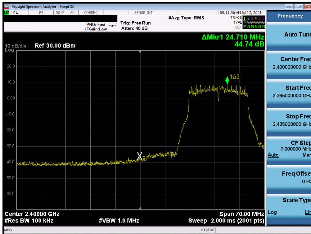
Plot 7-338. Band Edge Plot Antenna WF7 (802.11g- Ch. 3) – 24Mbps
