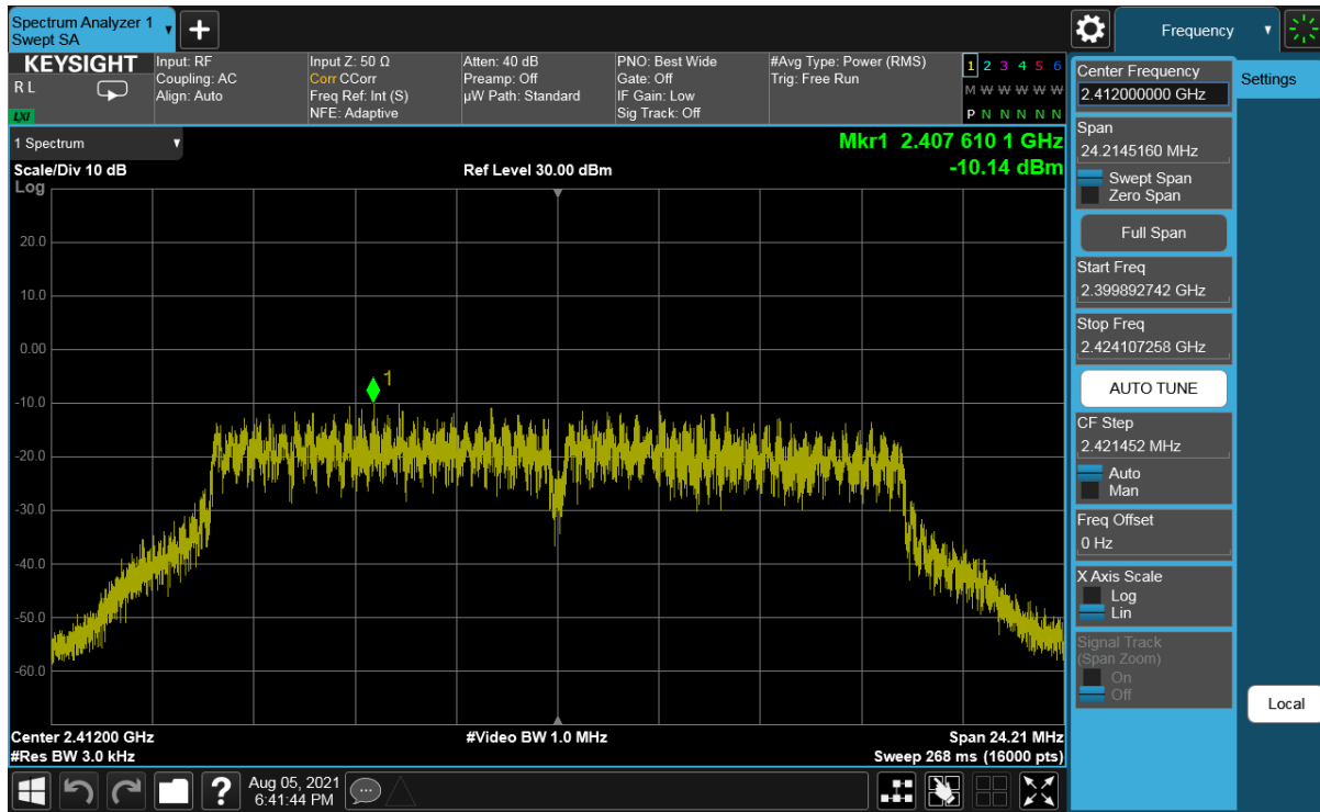
Plot 7-70. Power Spectral Density Plot Antenna WF8 (802.11g – Ch. 1) – 24Mbps
