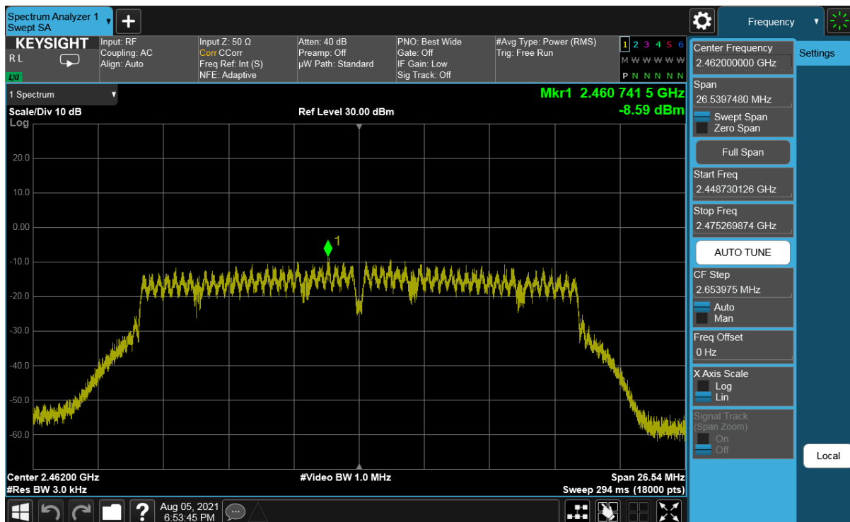
Plot 7-75. Power Spectral Density Plot Antenna WF8 (802.11n (2.4GHz) – Ch. 11) – MCS4
