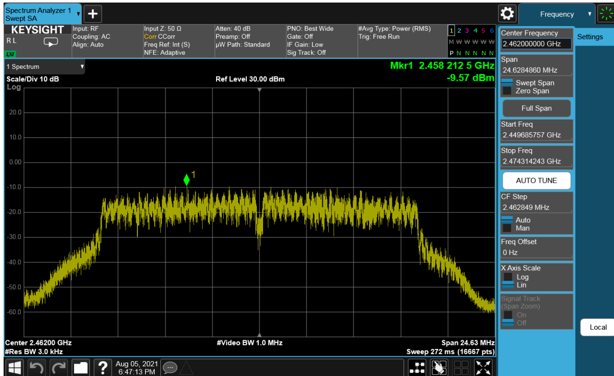
Plot 7-72. Power Spectral Density Plot Antenna WF8 (802.11g - Ch. 11) - 24Mbps
