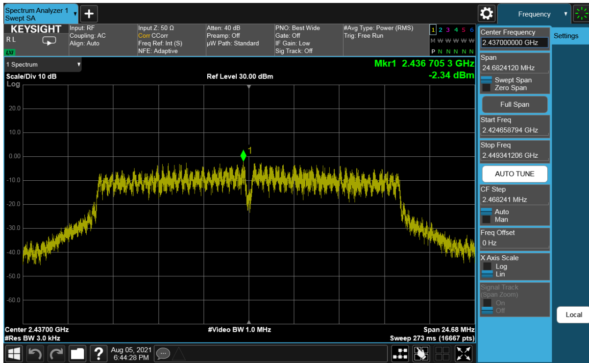
Plot 7-71. Power Spectral Density Plot Antenna WF8 (802.11g – Ch. 6) – 24Mbps
