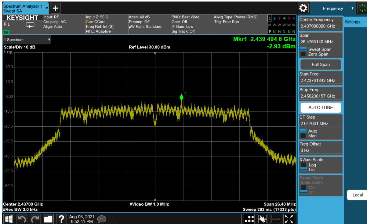
Plot 7-74. Power Spectral Density Plot Antenna WF8 (802.11n (2.4GHz) – Ch. 6) – MCS4
