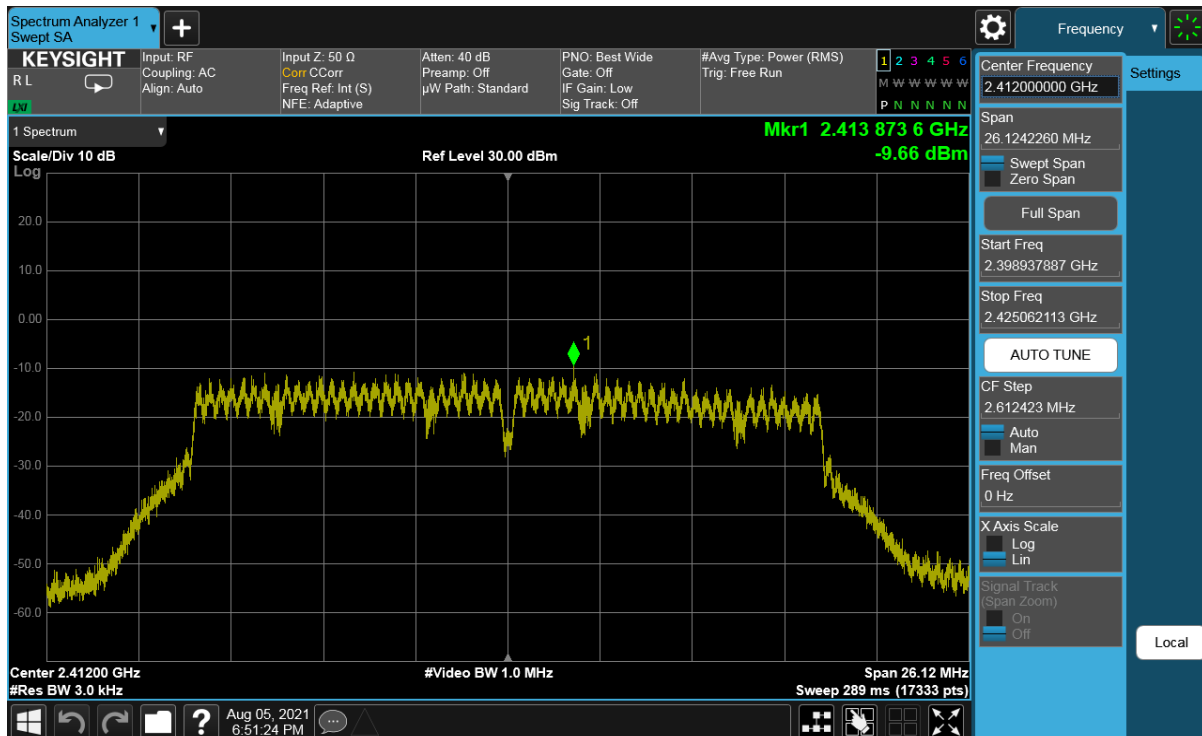
Plot 7-73. Power Spectral Density Plot Antenna WF8 (802.11n (2.4GHz) - Ch. 1) - MCS4
