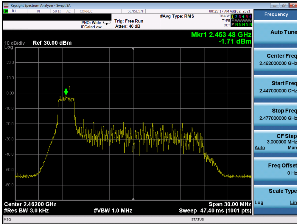
Plot 7-43. Power Spectral Density Plot Antenna WF7 (802.11ax OFDMA – RU26 Index 0 – Ch. 11)
