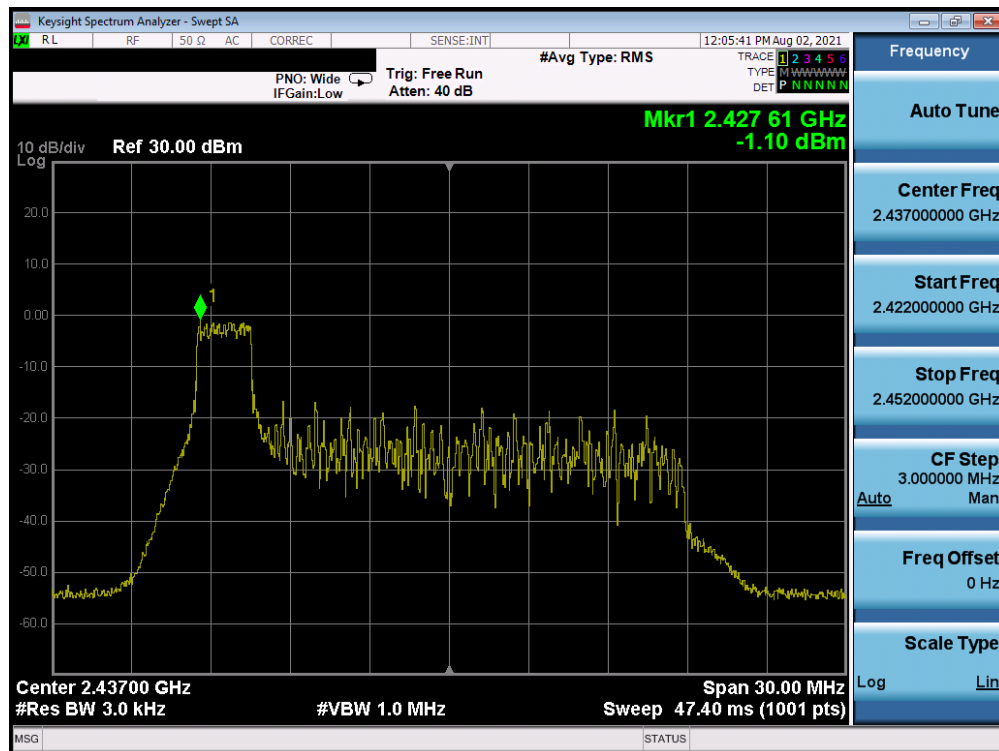
Plot 7-56. Power Spectral Density Plot CDD Antenna WF7 (802.11ax OFDMA – RU26 Index 0 – Ch. 6)
