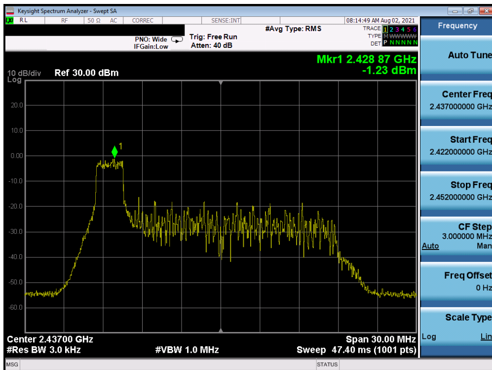
Plot 7-40. Power Spectral Density Plot Antenna WF7 (802.11ax OFDMA – RU26 Index 0 – Ch. 6)
