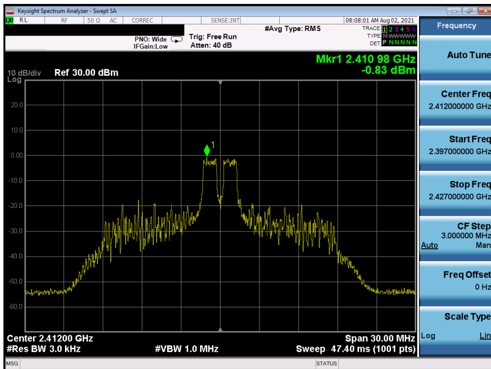
Plot 7-38. Power Spectral Density Plot Antenna WF7 (802.11ax OFDMA – RU26 Index 4 – Ch. 1)
