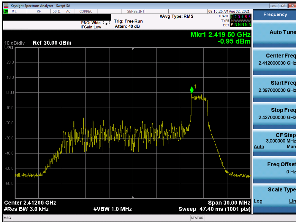
Plot 7-39. Power Spectral Density Plot Antenna WF7 (802.11ax OFDMA – RU26 Index 8 – Ch. 1)
