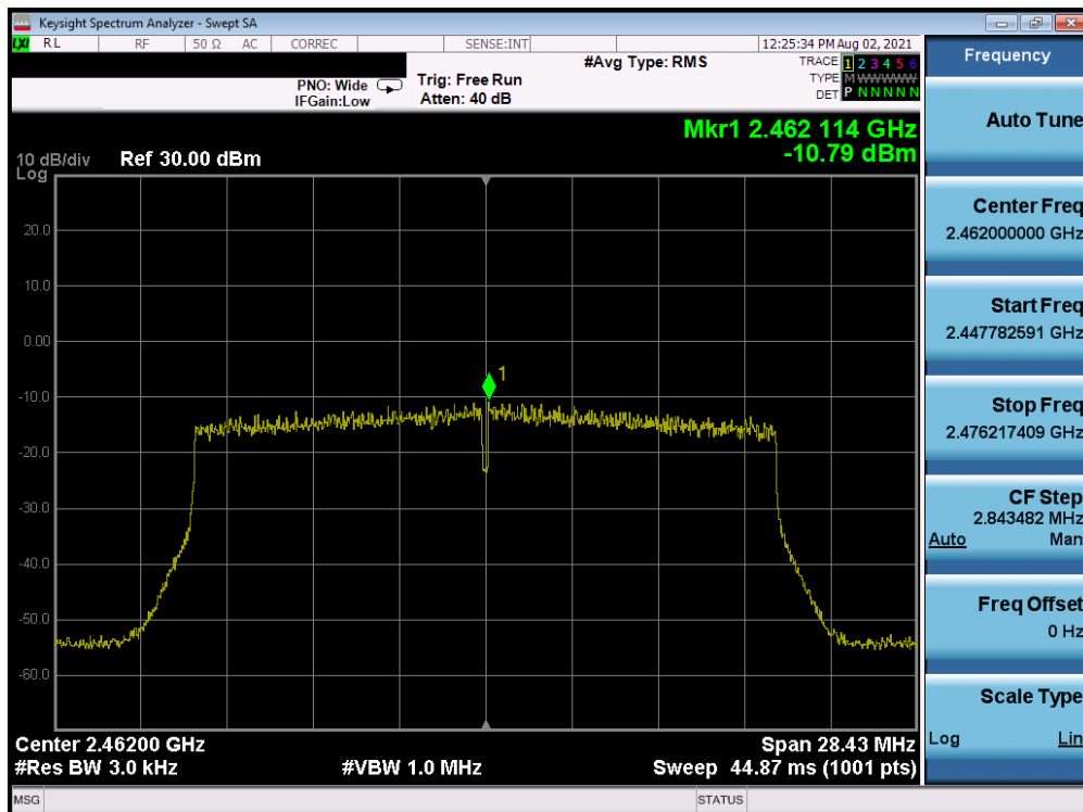
Plot 7-72. Power Spectral Density Plot CDD Antenna WF7 (802.11ax OFDMA – RU242 – Ch. 11)
