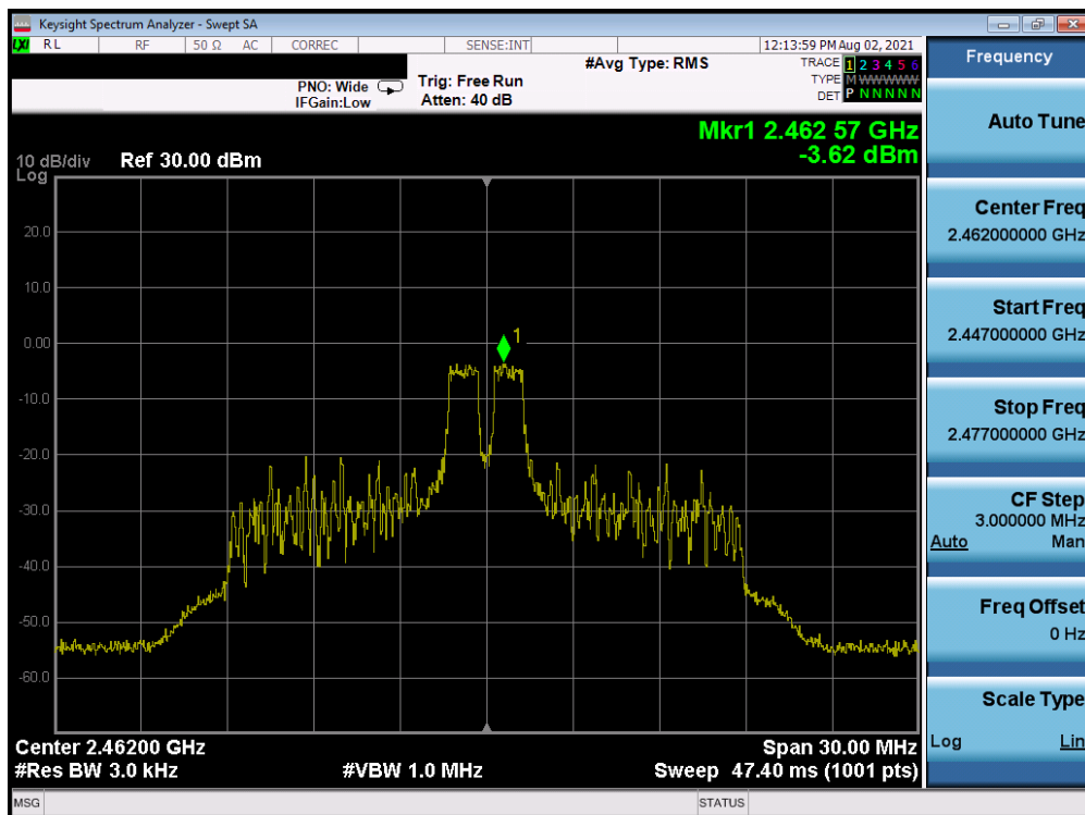
Plot 7-64. Power Spectral Density Plot CDD Antenna WF7 (802.11ax OFDMA – RU26 Index 4 – Ch. 11)
