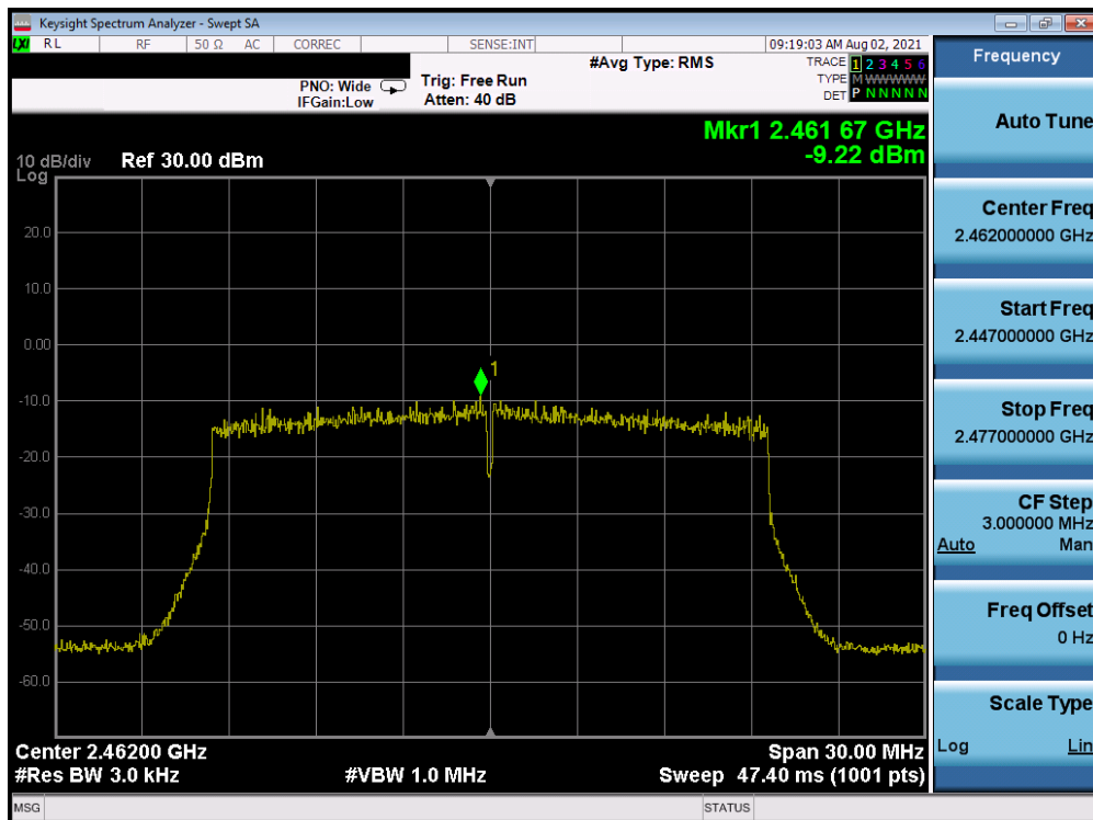
Plot 7-48. Power Spectral Density Plot Antenna WF7 (802.11ax OFDMA – RU242 – Ch. 11)
