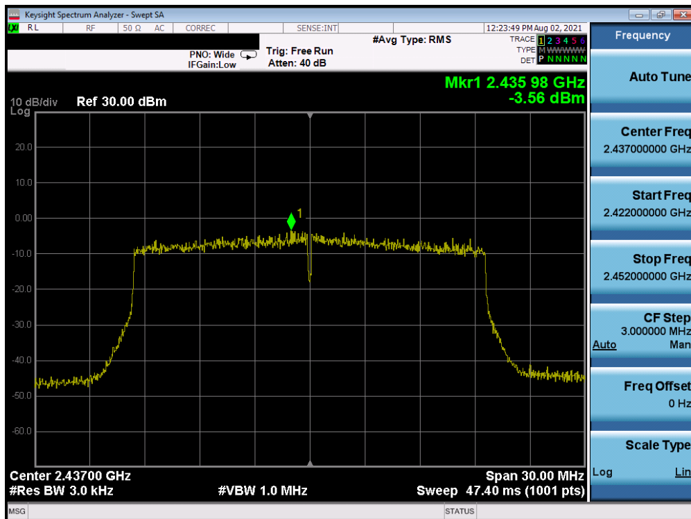
Plot 7-70. Power Spectral Density Plot CDD Antenna WF7 (802.11ax OFDMA – RU242 – Ch. 6)
