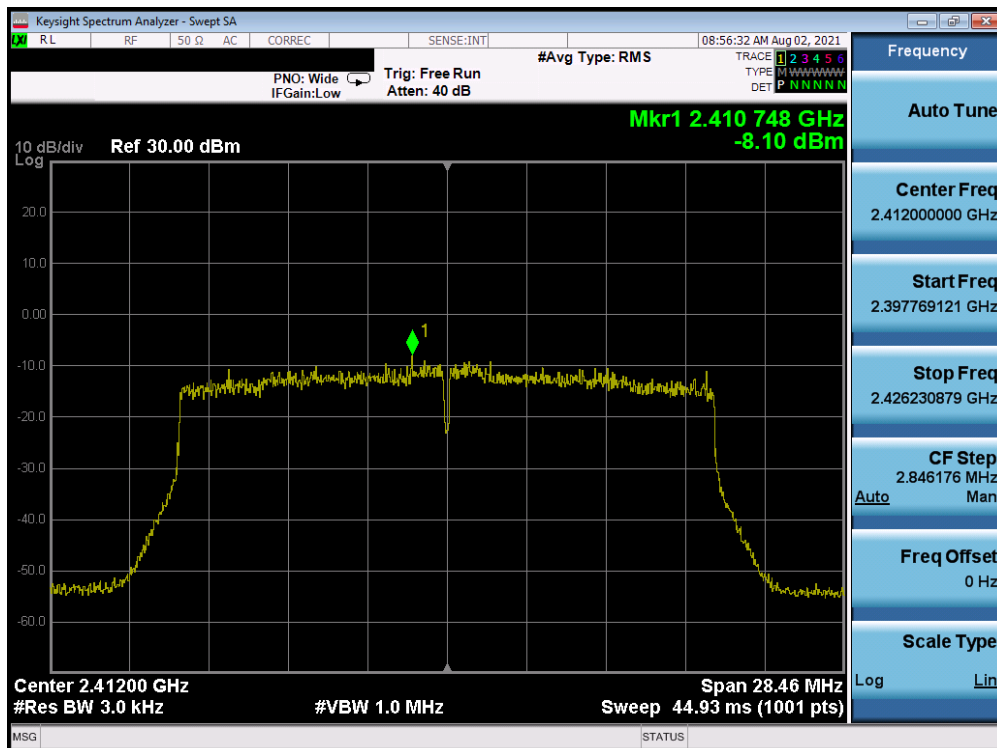
Plot 7-46. Power Spectral Density Plot Antenna WF7 (802.11ax OFDMA – RU242 – Ch. 1)
