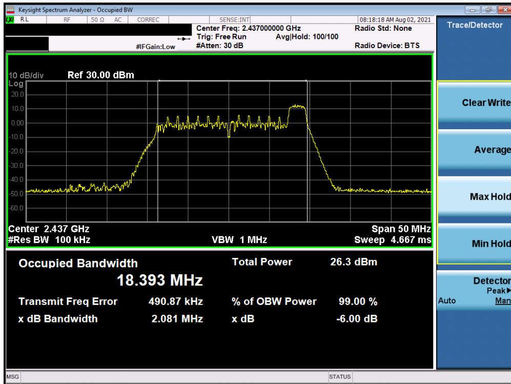
Plot 7-18. 6dB BW & 99% OBW Plot Antenna WF7 (802.11ax OFDMA – RU26 Index 8 – Ch. 6)
