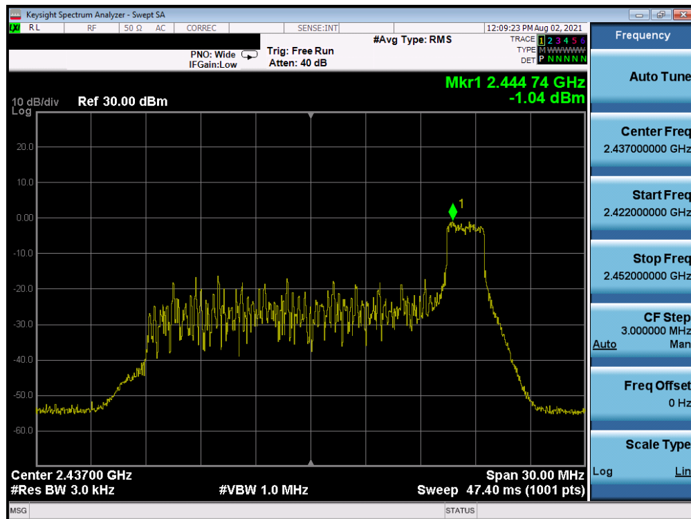
Plot 7-60. Power Spectral Density Plot CDD Antenna WF7 (802.11ax OFDMA – RU26 Index 8 – Ch. 6)
