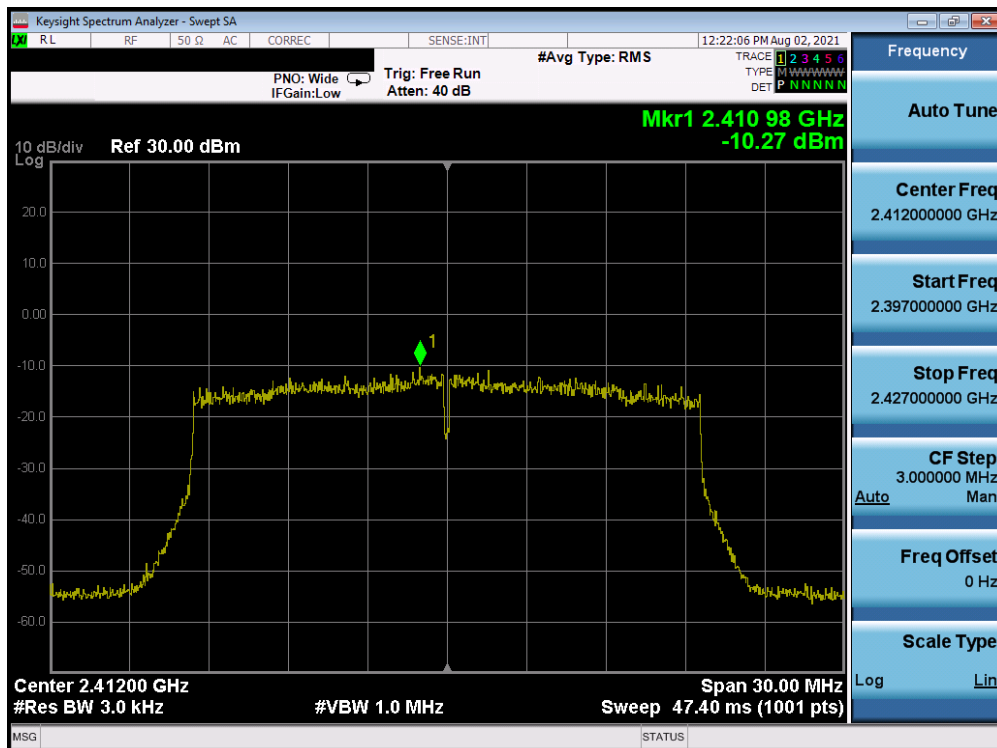
Plot 7-68. Power Spectral Density Plot CDD Antenna WF7 (802.11ax OFDMA – RU242 – Ch. 1)
