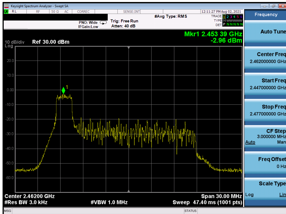
Plot 7-62. Power Spectral Density Plot CDD Antenna WF7 (802.11ax OFDMA – RU26 Index 0 – Ch. 11)
