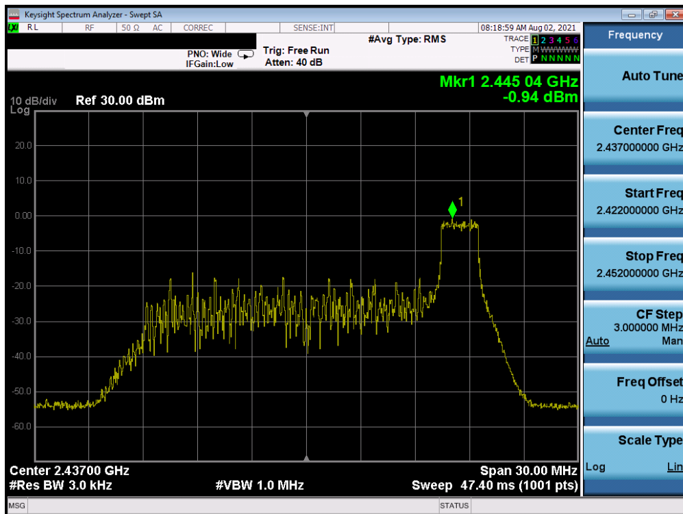
Plot 7-42. Power Spectral Density Plot Antenna WF7 (802.11ax OFDMA – RU26 Index 8 – Ch. 6)
