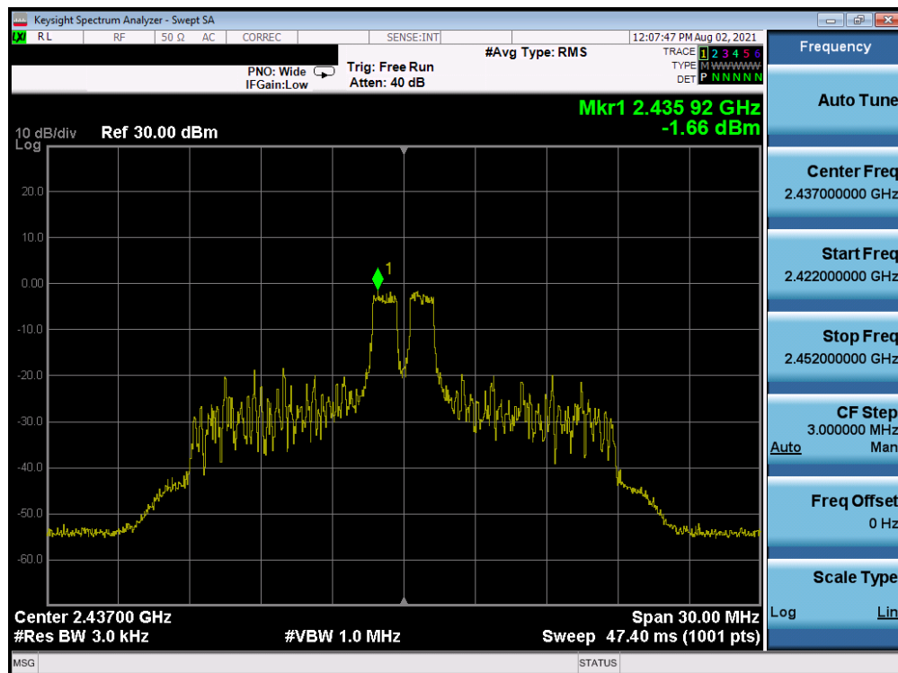
Plot 7-58. Power Spectral Density Plot CDD Antenna WF7 (802.11ax OFDMA – RU26 Index 4 – Ch. 6)
