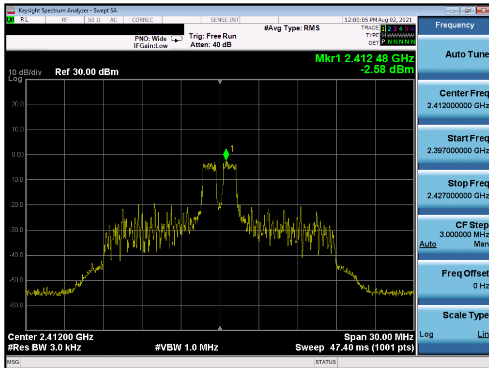
Plot 7-52. Power Spectral Density Plot CDD Antenna WF7 (802.11ax OFDMA – RU26 Index 4 – Ch. 1)
