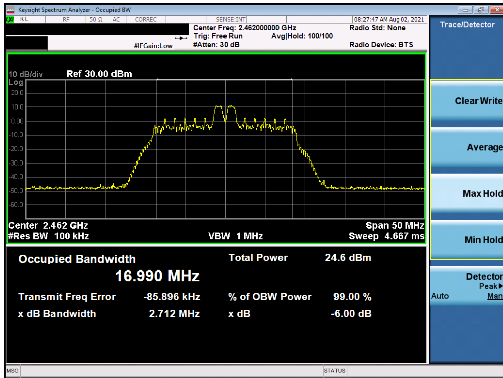
Plot 7-20. 6dB BW & 99% OBW Plot Antenna WF7 (802.11ax OFDMA – RU26 Index 4 – Ch. 11)
