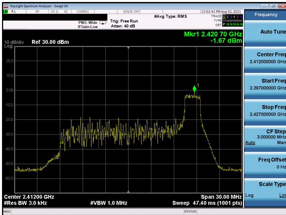
Plot 7-54. Power Spectral Density Plot CDD Antenna WF7 (802.11ax OFDMA – RU26 Index 8 – Ch. 1)
