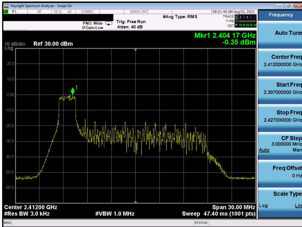
Plot 7-37. Power Spectral Density Plot Antenna WF7 (802.11ax OFDMA – RU26 Index 0 – Ch. 1)
