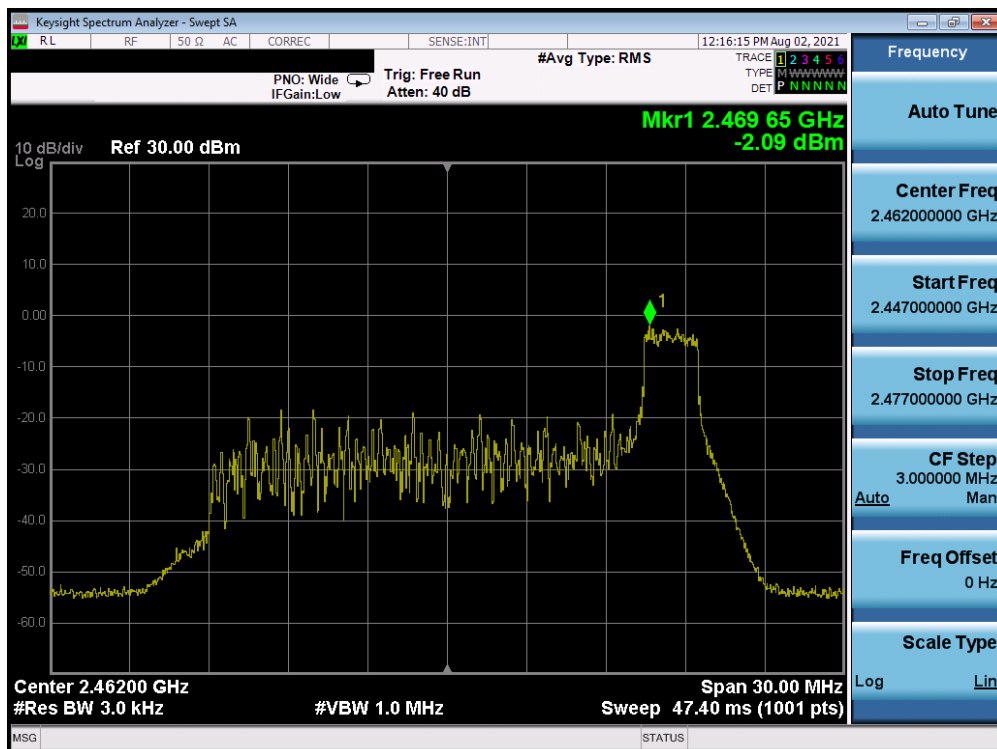
Plot 7-66. Power Spectral Density Plot CDD Antenna WF7 (802.11ax OFDMA – RU26 Index 8 – Ch. 11)
