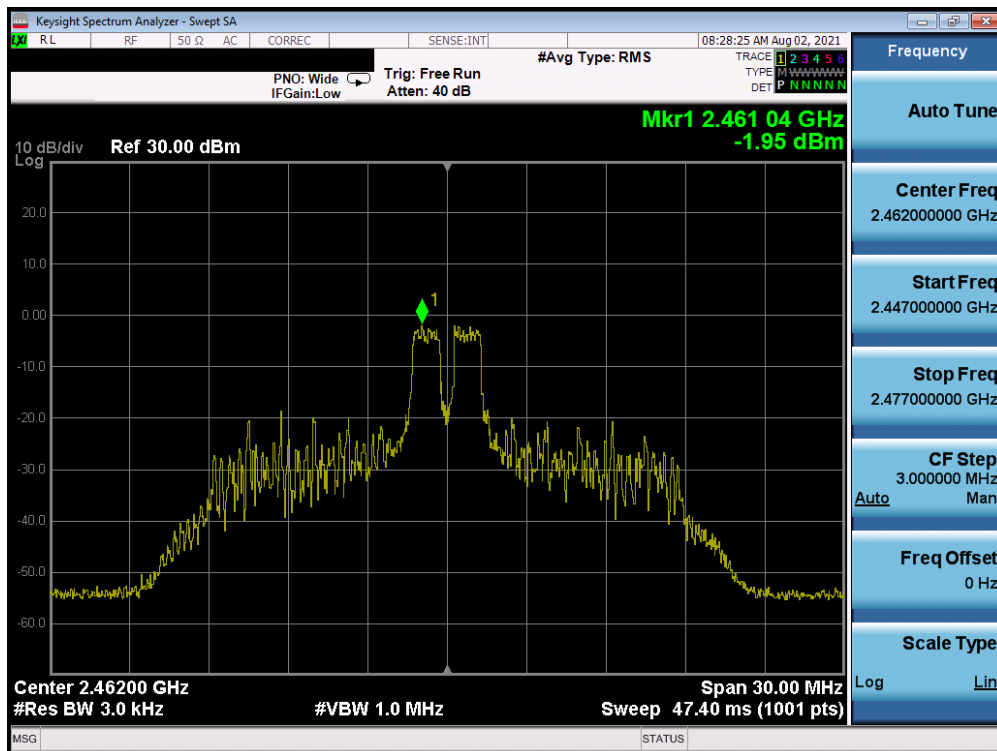
Plot 7-44. Power Spectral Density Plot Antenna WF7 (802.11ax OFDMA – RU26 Index 4 – Ch. 11)
