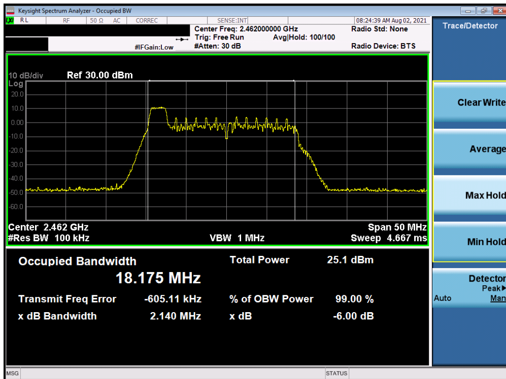
Plot 7-19. 6dB BW & 99% OBW Plot Antenna WF7 (802.11ax OFDMA – RU26 Index 0 – Ch. 11)
