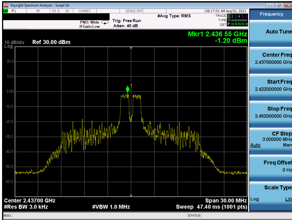
Plot 7-41. Power Spectral Density Plot Antenna WF7 (802.11ax OFDMA – RU26 Index 4 – Ch. 6)
