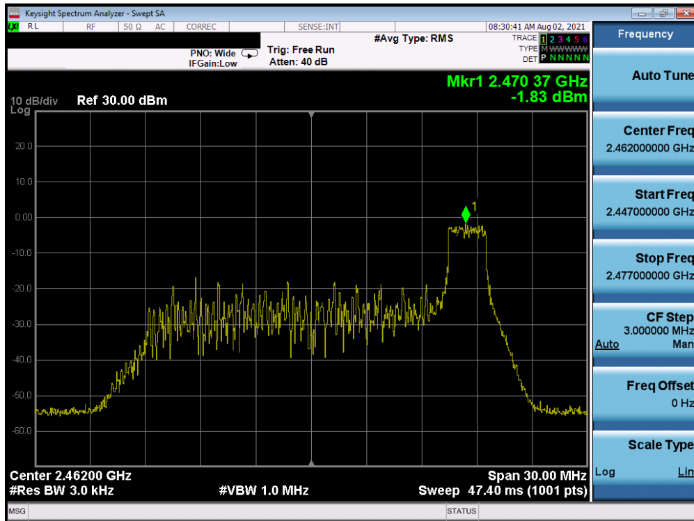
Plot 7-45. Power Spectral Density Plot Antenna WF7 (802.11ax OFDMA – RU26 Index 8 – Ch. 11)
