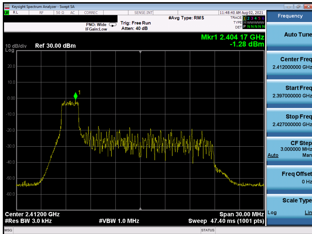
Plot 7-50. Power Spectral Density Plot CDD Antenna WF7 (802.11ax OFDMA – RU26 Index 0 – Ch. 1)
