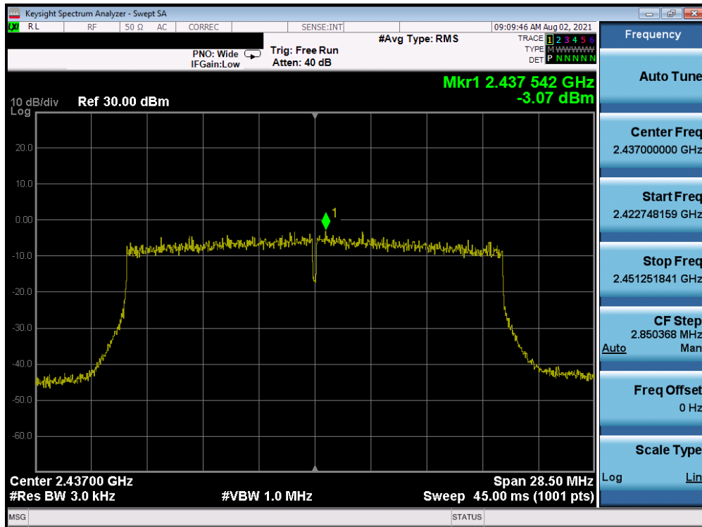
Plot 7-47. Power Spectral Density Plot Antenna WF7 (802.11ax OFDMA – RU242 – Ch. 6)
