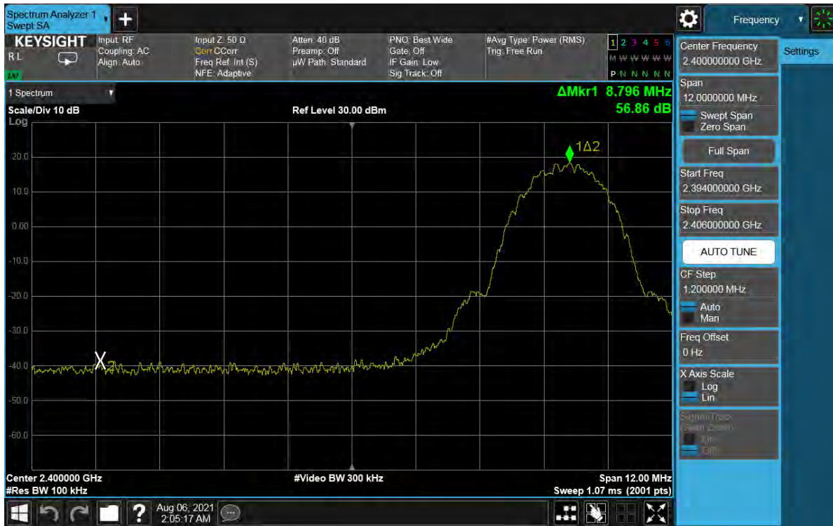
Plot 7-63. Band Edge Plot Antenna WF8 (Bluetooth (LE), 2Mbps, ePA – Ch. 1)
