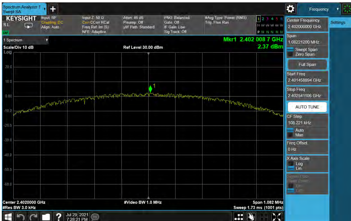
Plot 7-38. Power Spectral Density Plot Antenna WF7 (Bluetooth (LE), 1Mbps, ePA – Ch. 0)
