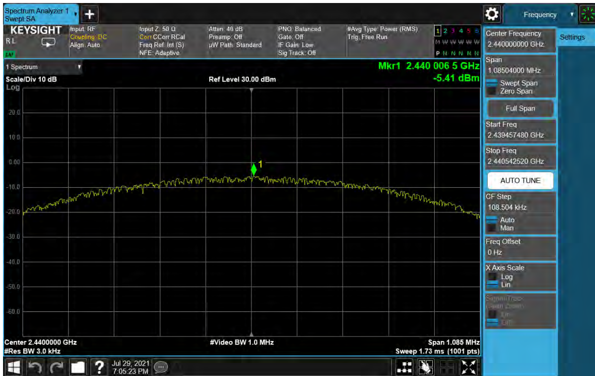
Plot 7-45. Power Spectral Density Plot Antenna WF8 (Bluetooth (LE), 1Mbps, iPA – Ch. 19)
