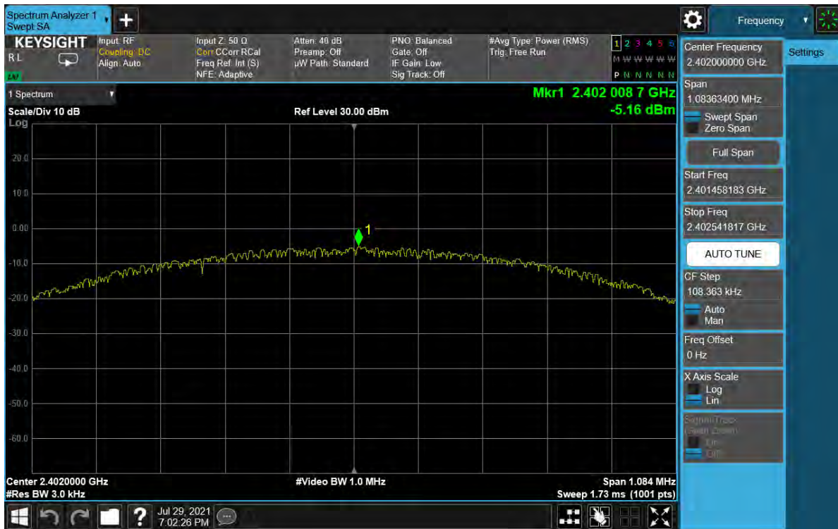
Plot 7-43. Power Spectral Density Plot Antenna WF8 (Bluetooth (LE), 1Mbps, iPA – Ch. 0)
