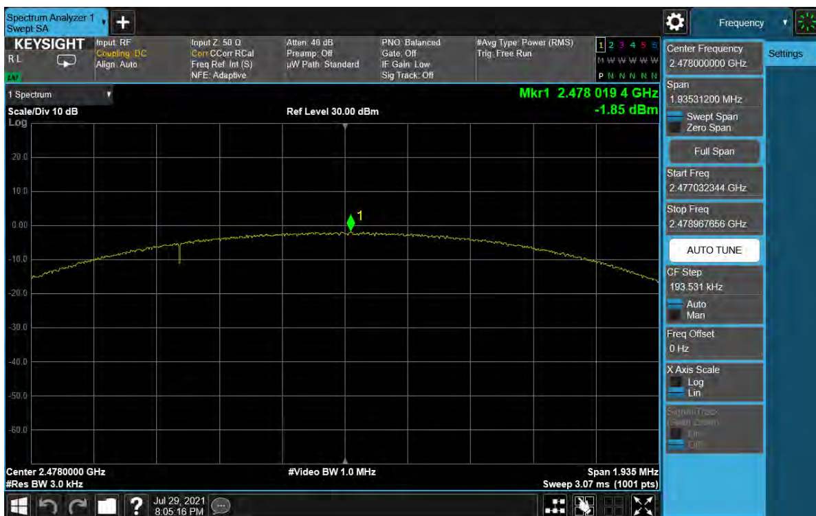
Plot 7-54. Power Spectral Density Plot Antenna WF7 (Bluetooth (LE), 2Mbps, ePA – Ch. 38)
