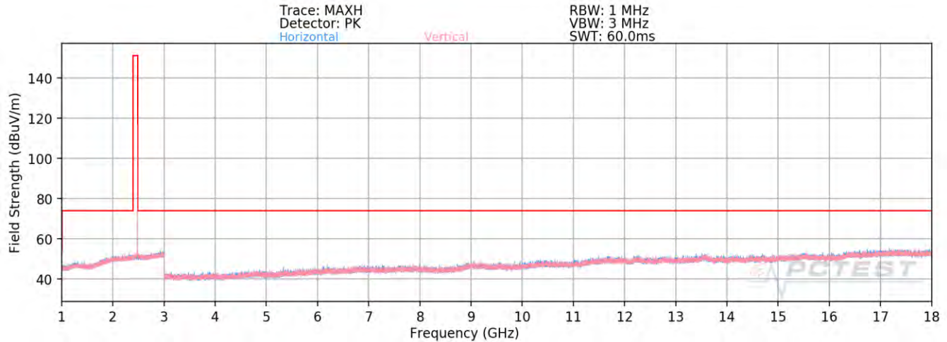
Plot 7-86. Radiated Spurious Plot Above 1GHz Antenna WF7 (1Mbps, ePA – Ch. 39)
