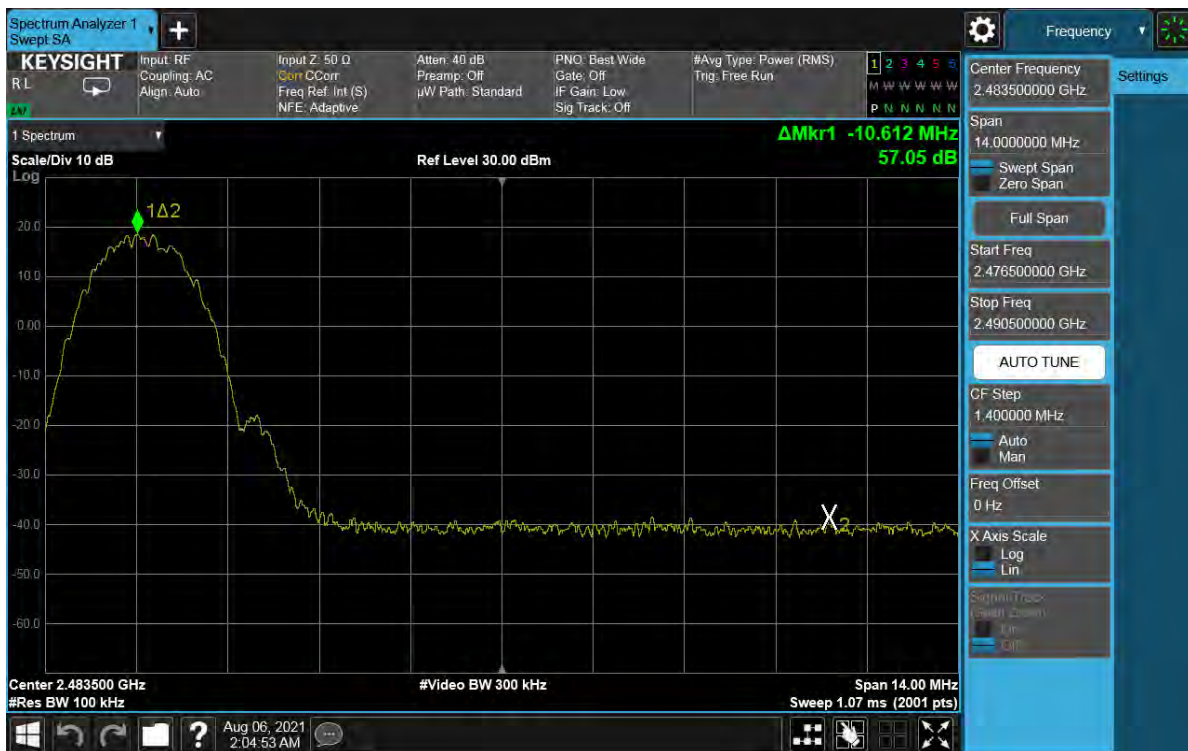
Plot 7-64. Band Edge Plot Antenna WF8 (Bluetooth (LE), 2Mbps, ePA – Ch. 38)
