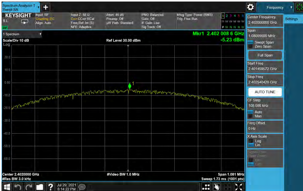
Plot 7-44. Power Spectral Density Plot Antenna WF7 (Bluetooth (LE), 1Mbps, iPA – Ch. 0)
