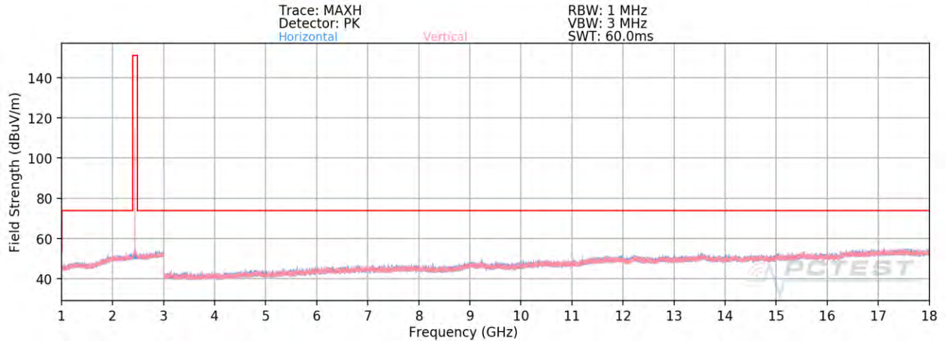
Plot 7-82. Radiated Spurious Plot Above 1GHz Antenna WF8 (1Mbps, ePA – Ch. 19)
