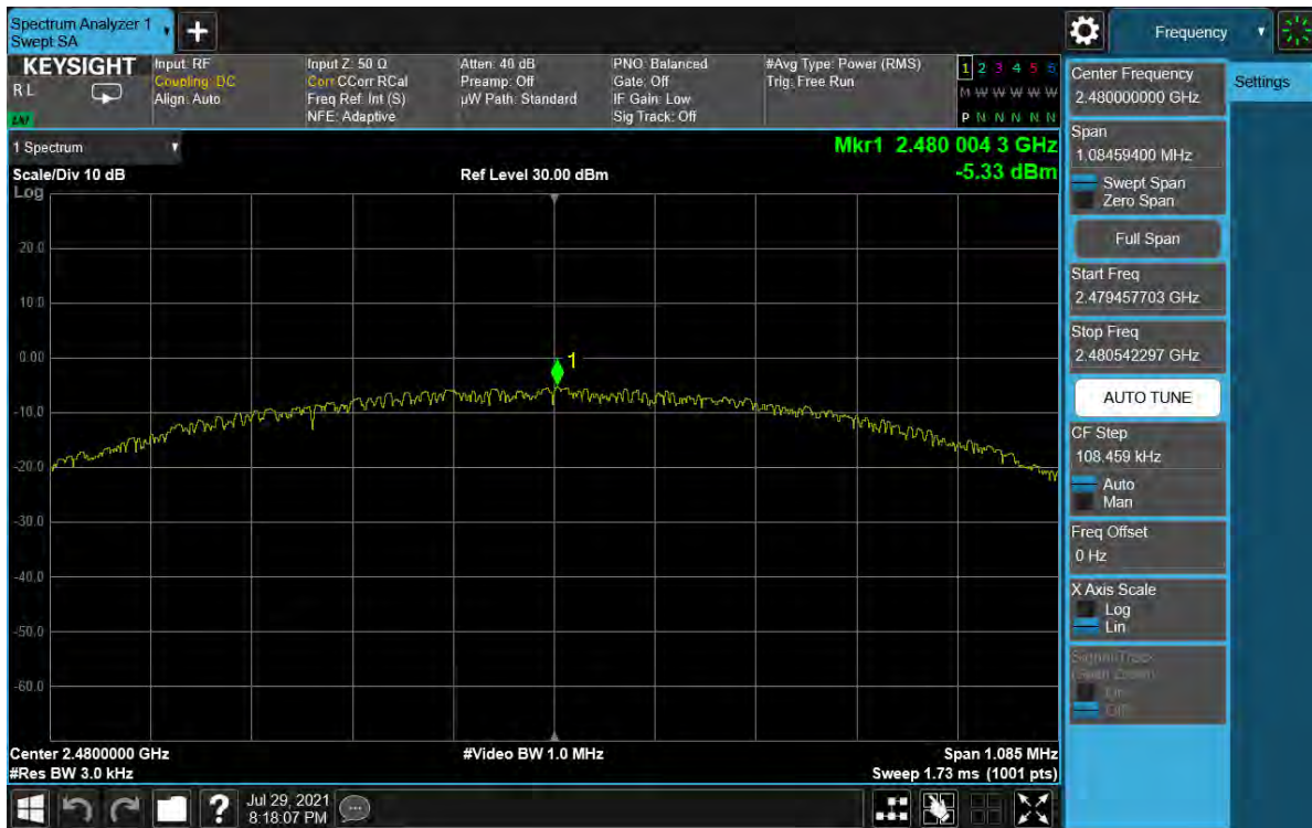
Plot 7-48. Power Spectral Density Plot Antenna WF7 (Bluetooth (LE), 1Mbps, iPA – Ch. 39)
