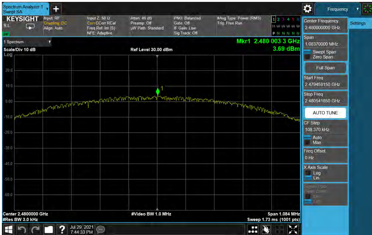
Plot 7-42. Power Spectral Density Plot Antenna WF7 (Bluetooth (LE), 1Mbps, ePA – Ch. 39)
