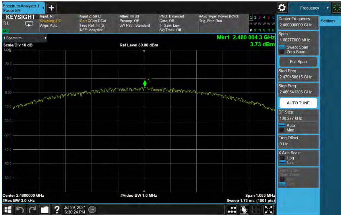
Plot 7-41. Power Spectral Density Plot Antenna WF8 (Bluetooth (LE), 1Mbps, ePA – Ch. 39)
