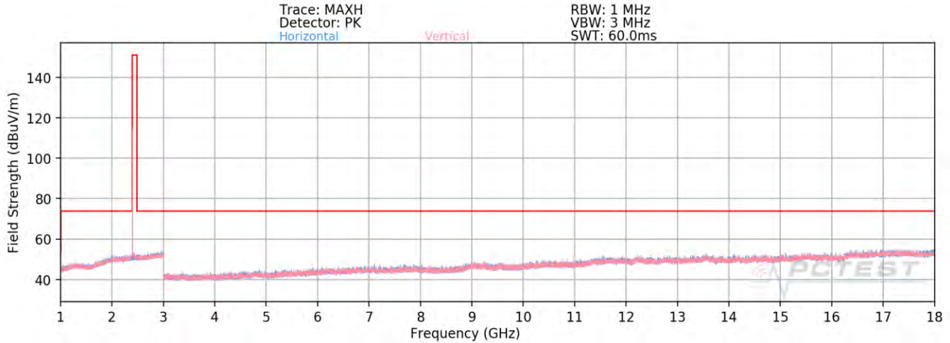
Plot 7-81. Radiated Spurious Plot Above 1GHz Antenna WF8 (1Mbps, ePA – Ch. 0)
