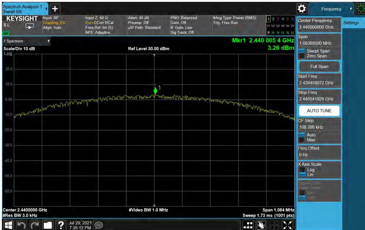
Plot 7-40. Power Spectral Density Plot Antenna WF7 (Bluetooth (LE), 1Mbps, ePA – Ch. 19)
