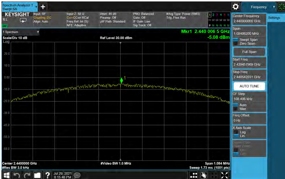
Plot 7-46. Power Spectral Density Plot Antenna WF7 (Bluetooth (LE), 1Mbps, iPA – Ch. 19)
