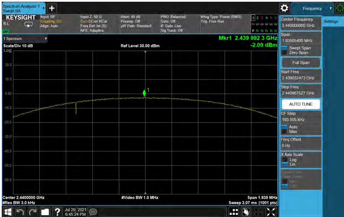
Plot 7-51. Power Spectral Density Plot Antenna WF8 (Bluetooth (LE), 2Mbps, ePA – Ch. 19)
