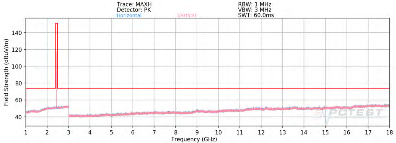
Plot 7-85. Radiated Spurious Plot Above 1GHz Antenna WF7 (1Mbps, ePA – Ch. 19)
