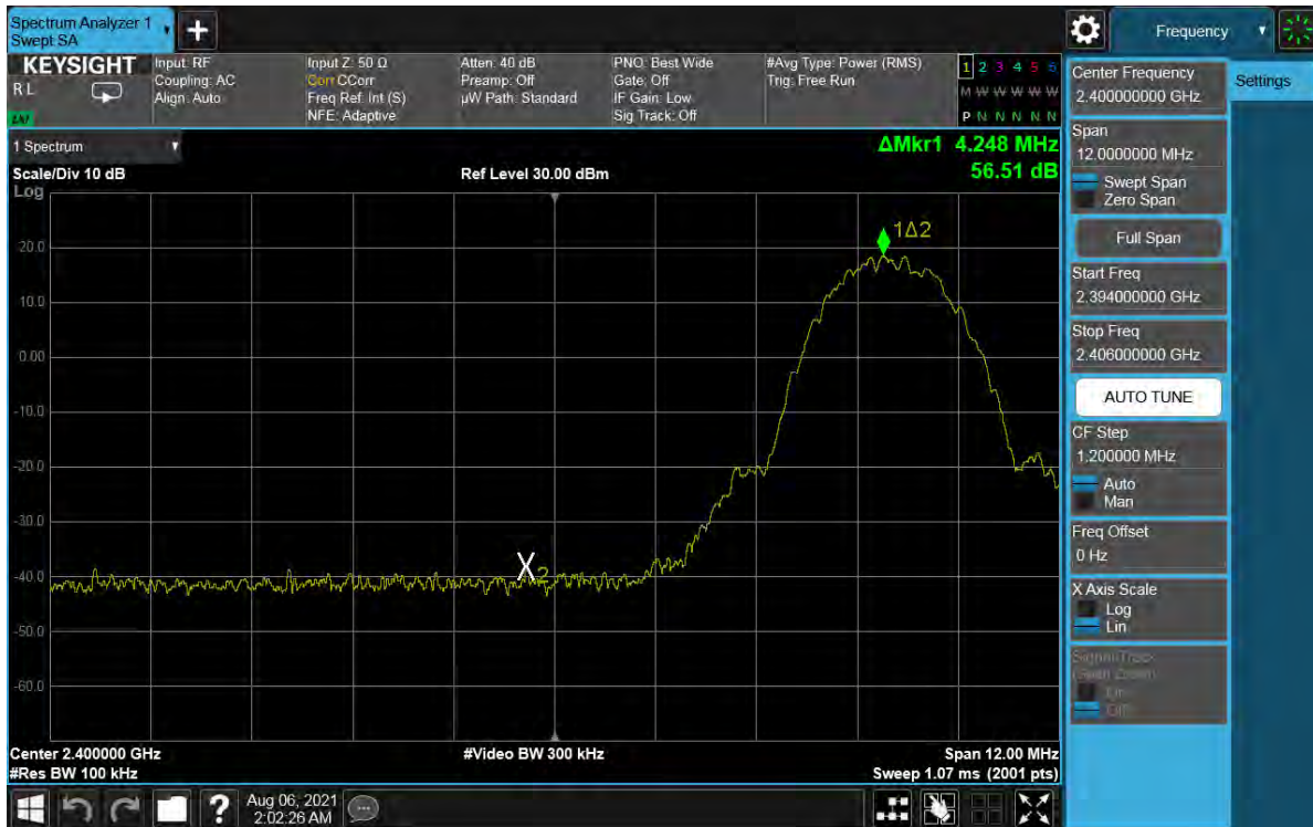
Plot 7-67. Band Edge Plot Antenna WF7 (Bluetooth (LE), 2Mbps, ePA – Ch. 1)
