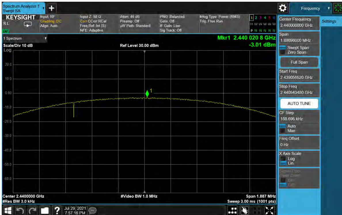
Plot 7-52. Power Spectral Density Plot Antenna WF7 (Bluetooth (LE), 2Mbps, ePA – Ch. 19)
