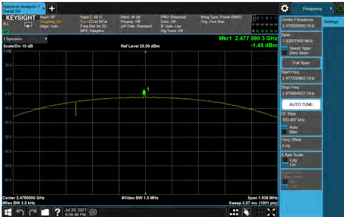
Plot 7-53. Power Spectral Density Plot Antenna WF8 (Bluetooth (LE), 2Mbps, ePA – Ch. 38)
