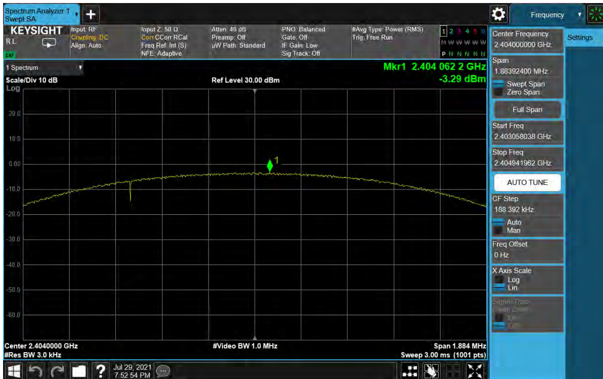
Plot 7-50. Power Spectral Density Plot Antenna WF7 (Bluetooth (LE), 2Mbps, ePA – Ch. 1)
