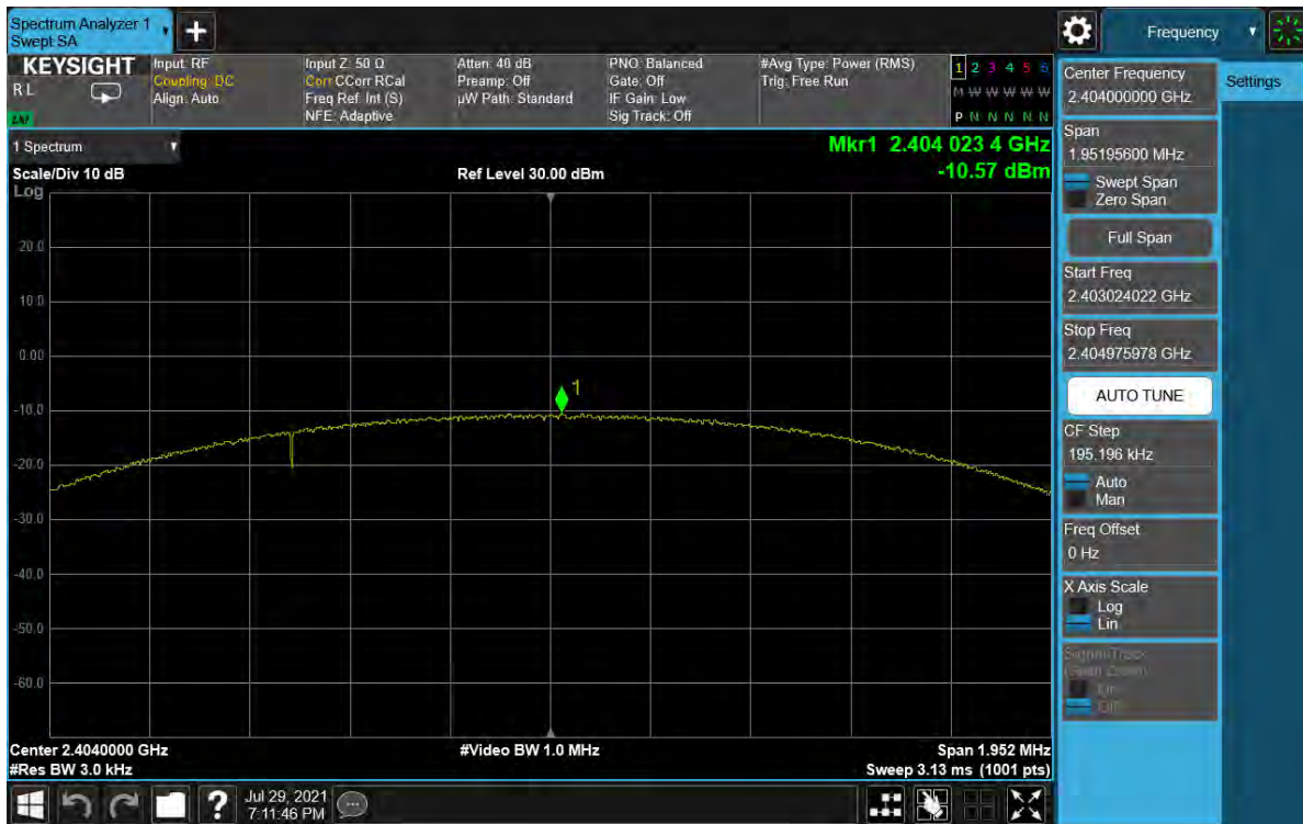
Plot 7-55. Power Spectral Density Plot Antenna WF8 (Bluetooth (LE), 2Mbps, iPA – Ch. 1)
