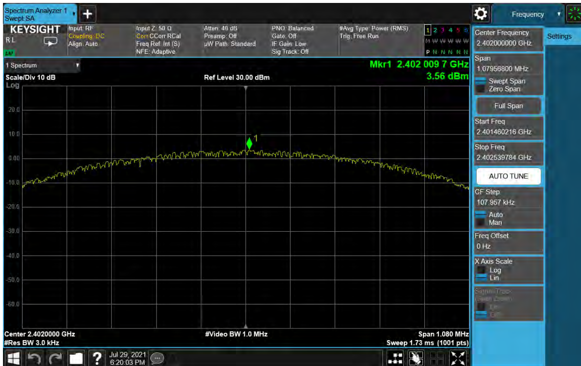
Plot 7-37. Power Spectral Density Plot Antenna WF8 (Bluetooth (LE), 1Mbps, ePA – Ch. 0)
