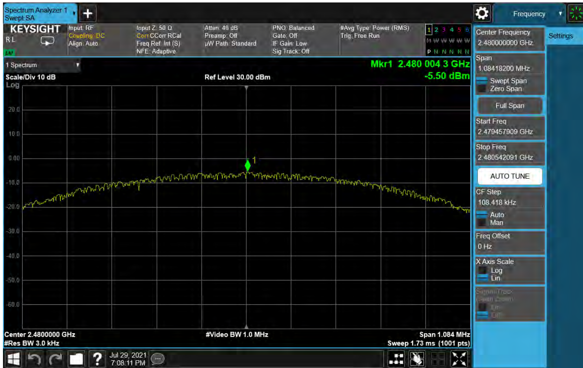
Plot 7-47. Power Spectral Density Plot Antenna WF8 (Bluetooth (LE), 1Mbps, iPA – Ch. 39)
