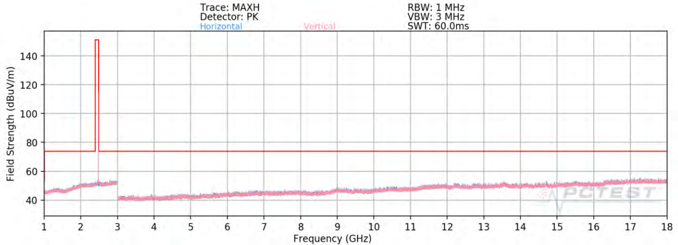
Plot 7-83. Radiated Spurious Plot Above 1GHz Antenna WF8 (1Mbps ePA – Ch. 39)
