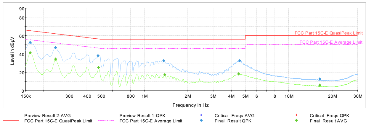
Plot 7-106. AC Line Conducted Plot with Bluetooth HDR Antenna WF8 (N, 4Mbps ePA - Ch.38 with AC/DC Adapter)
