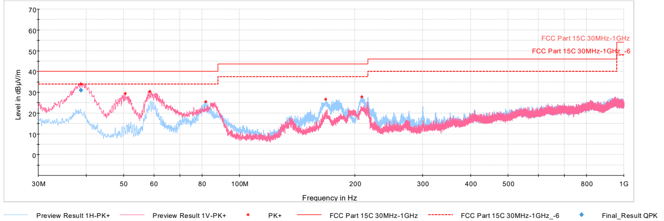
Plot 7-104. Radiated Spurious Emissions below 1GHz Ant WF8 (4Mbps, ePA – Ch.38 with AC/DC Adapter)
