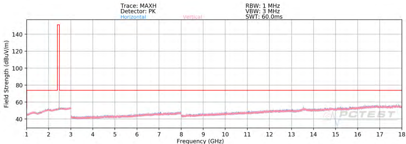
Plot 7-88. Radiated Spurious Emissions Above 1GHz Antenna WF7 (4Mbps, HDR4, ePA – Ch. 73)
