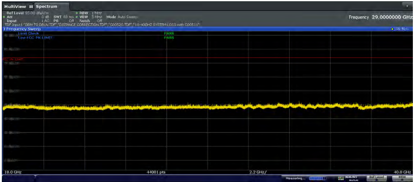
Plot 7-84. Radiated Spurious Emissions Above 18GHz Antenna WF8 (4Mbps – Ch.38, ePA, Ant. Pol. V)
