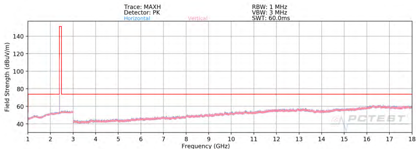
Plot 7-86. Radiated Spurious Emissions Above 1GHz Antenna WF7 (4Mbps, HDR4, ePA – Ch. 1)
