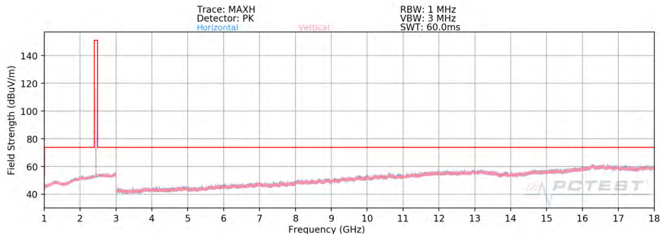
Plot 7-90. Radiated Spurious Emissions Above 1GHz TxBF (4Mbps, HDR4, ePA – Ch. 38)
