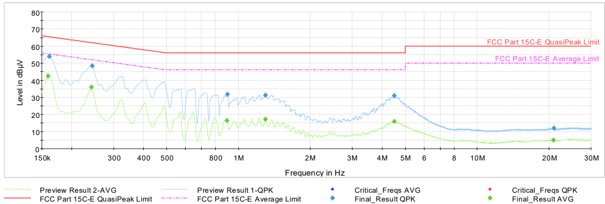
Plot 7-105. AC Line Conducted Plot with Bluetooth HDR Antenna WF8 (L1, 4Mbps ePA - Ch.38 with AC/DC Adapter)
