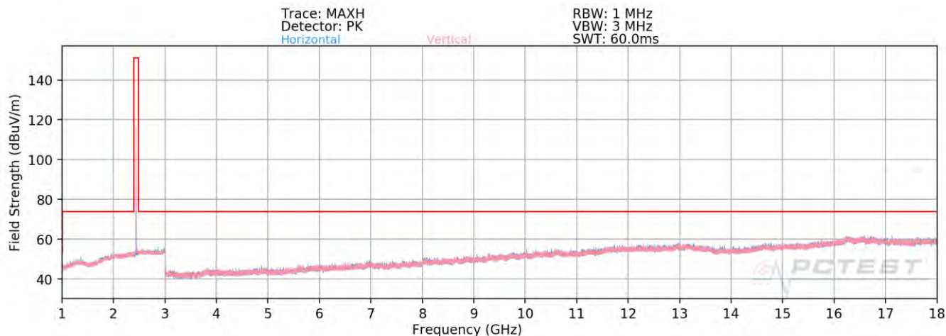
Plot 7-87. Radiated Spurious Emissions Above 1GHz Antenna WF7 (4Mbps, HDR4, ePA – Ch. 38)
