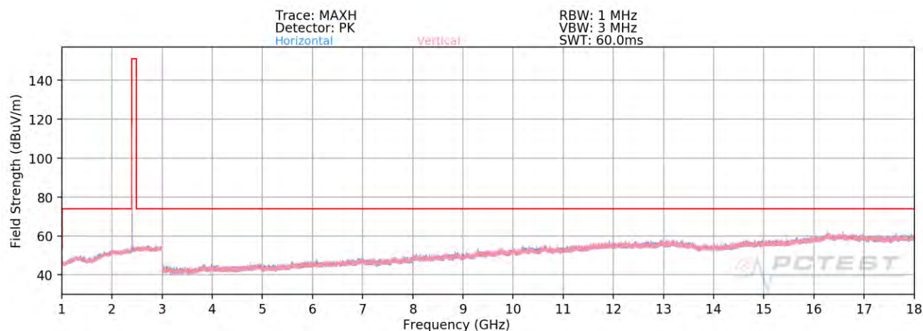
Plot 7-89. Radiated Spurious Emissions Above 1GHz TxBF (4Mbps, HDR4, ePA – Ch. 1)
