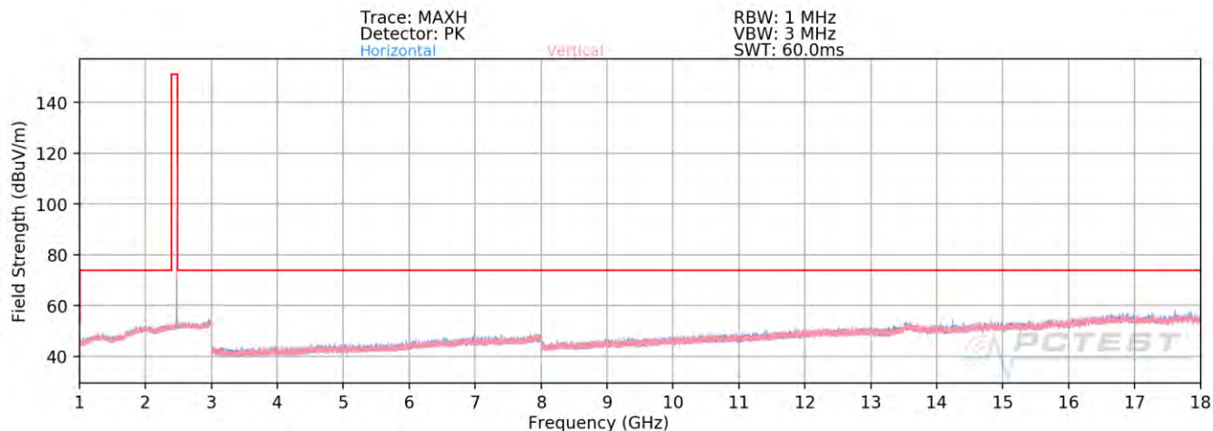
Plot 7-85. Radiated Spurious Emissions Above 1GHz Antenna WF8 (4Mbps, HDR4, ePA – Ch. 73)
