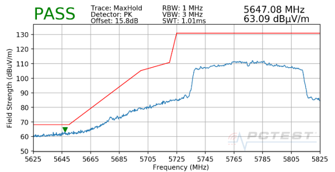
Plot 7-743. Antenna WF5T (Pk, Ch.155, 802.11ac, MCS3)
