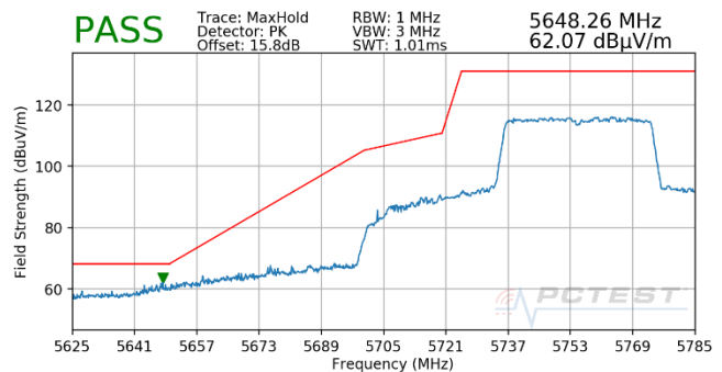
Plot 7-722. Antenna WF5T (Pk, Ch.151, 802.11ax(SU), MCS3)
