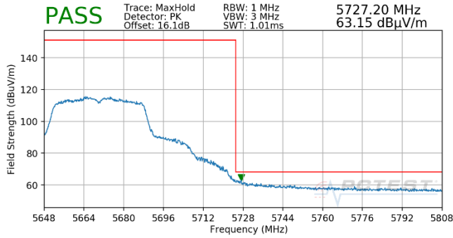
Plot 7-684. Antenna WF5T (Pk, Ch.134, 802.11n, MCS2)
