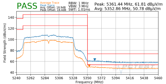
Plot 7-730. Antenna WF5T (Pk & Avg, Ch.58, 802.11ac, MCS2)
