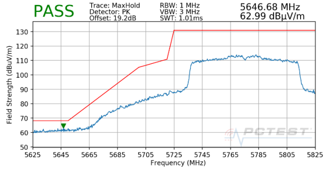
Plot 7-742. Antenna WF5T (Pk, Ch.155, 802.11ac, MCS2)
