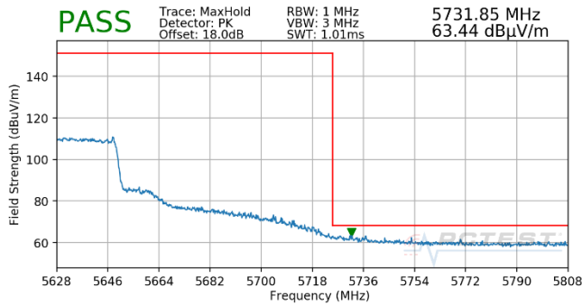
Plot 7-761. (FCC Only) Antenna WF5T (Pk, Ch.122, 802.11ax(SU), MCS3)
