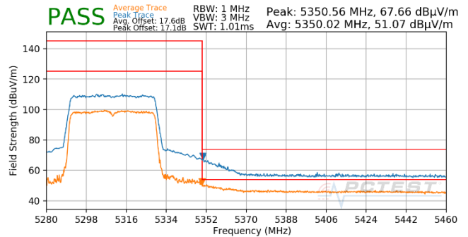
Plot 7-704. Antenna WF5T (Pk & Avg, Ch.62, 802.11ax(SU), MCS5)
