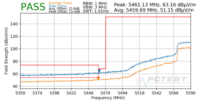
Plot 7-736. (FCC Only) Antenna WF5T (Pk & Avg, Ch.122, 802.11ac, MCS2)
