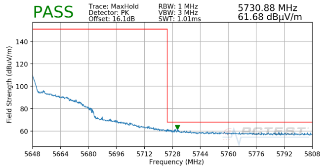
Plot 7-682. (FCC Only) Antenna WF5T (Pk, Ch.126, 802.11n, MCS3)
