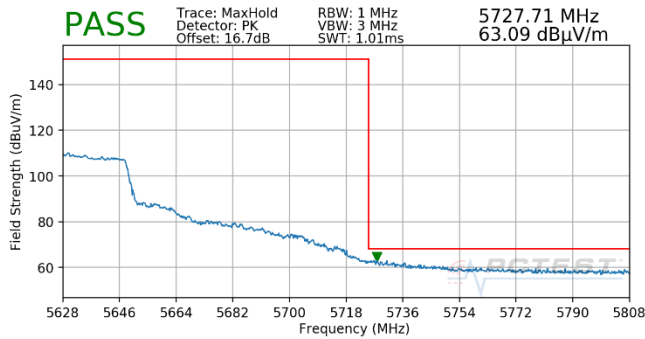
Plot 7-740. (FCC Only) Antenna WF5T (Pk, Ch.122, 802.11ac, MCS3)
