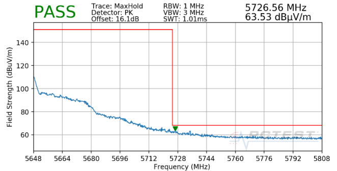
Plot 7-683. (FCC Only) Antenna WF5T (Pk, Ch.126, 802.11n, MCS5)
