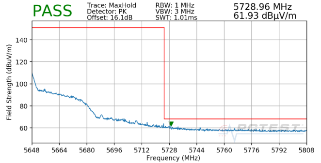
Plot 7-681. (FCC Only) Antenna WF5T (Pk, Ch.126, 802.11n, MCS2)
