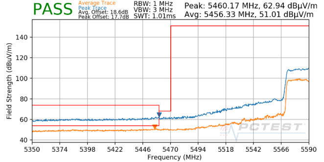
Plot 7-759. (FCC Only) Antenna WF5T (Pk & Avg, Ch.122, 802.11ax(SU), MCS5)
