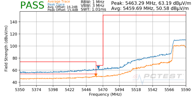
Plot 7-738. (FCC Only) Antenna WF5T (Pk & Avg, Ch.122, 802.11ac, MCS5)
