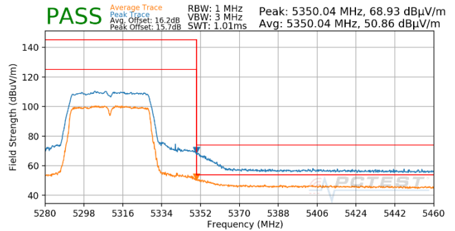
Plot 7-671. Antenna WF5T (Pk & Avg, Ch.62, 802.11n, MCS5)
