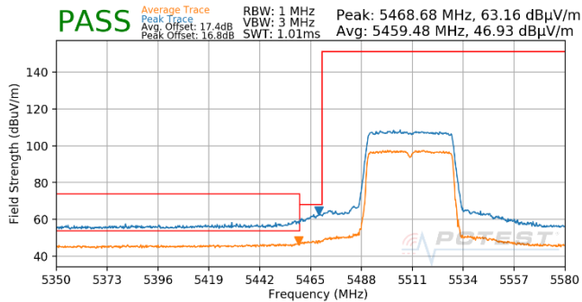
Plot 7-707. Antenna WF5T (Pk & Avg, Ch.102, 802.11ax(SU), MCS5)
