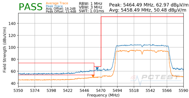
Plot 7-735. Antenna WF5T (Pk & Avg, Ch.106, 802.11ac, MCS5)
