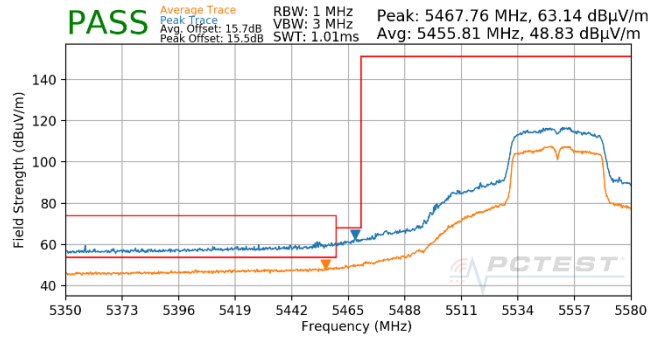
Plot 7-675. Antenna WF5T (Pk & Avg, Ch.110, 802.11n, MCS2)
