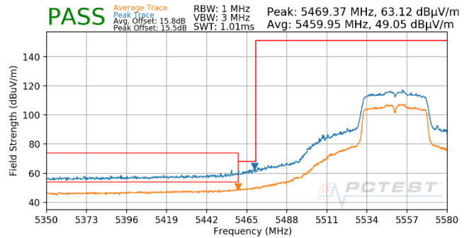
Plot 7-676. Antenna WF5T (Pk & Avg, Ch.110, 802.11n, MCS3)
