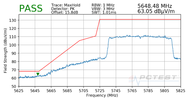
Plot 7-765. Antenna WF5T (Pk, Ch.155, 802.11ax(SU), MCS5)
