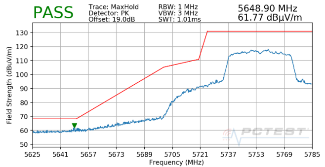
Plot 7-688. Antenna WF5T (Pk, Ch.151, 802.11n, MCS3)
