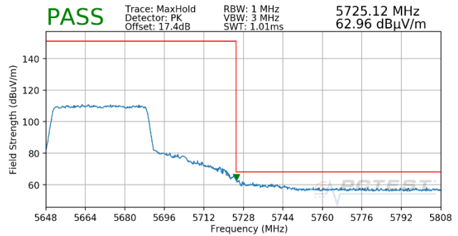
Plot 7-720. Antenna WF5T (Pk, Ch.134, 802.11ax(SU), MCS5)
