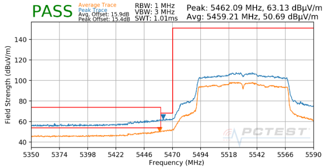
Plot 7-733. Antenna WF5T (Pk & Avg, Ch.106, 802.11ac, MCS2)
