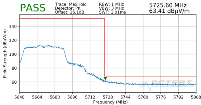
Plot 7-685. Antenna WF5T (Pk, Ch.134, 802.11n, MCS3)
