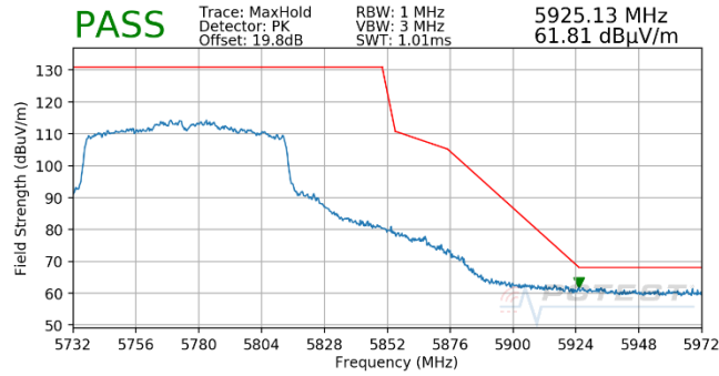
Plot 7-745. Antenna WF5T (Pk, Ch.155, 802.11ac, MCS2)
