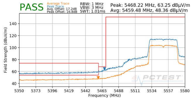
Plot 7-709. Antenna WF5T (Pk & Avg, Ch.110, 802.11ax(SU), MCS3)
