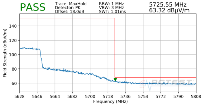
Plot 7-762. (FCC Only) Antenna WF5T (Pk, Ch.122, 802.11ax(SU), MCS5)
