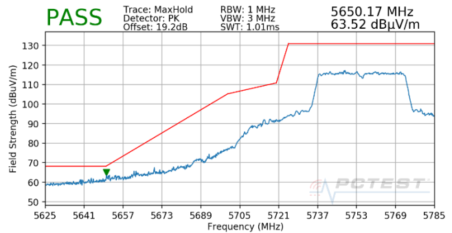
Plot 7-689. Antenna WF5T (Pk, Ch.151, 802.11n, MCS5)
