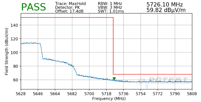
Plot 7-716. (FCC Only) Antenna WF5T (Pk, Ch.126, 802.11ax(SU), MCS3)
