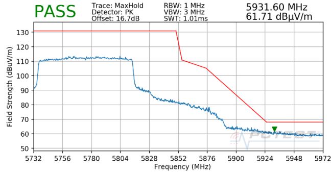
Plot 7-766. Antenna WF5T (Pk, Ch.155, 802.11ax(SU), MCS2)
