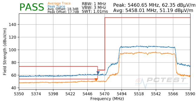
Plot 7-755. Antenna WF5T (Pk & Avg, Ch.106, 802.11ax(SU), MCS3)
