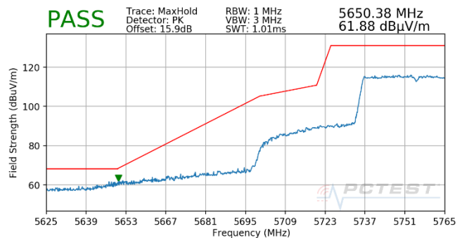
Plot 7-721. Antenna WF5T (Pk, Ch.151, 802.11ax(SU), MCS2)
