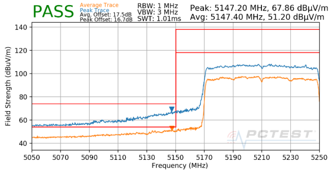
Plot 7-750. Antenna WF5T (Pk & Avg, Ch.42, 802.11ax(SU), MCS5)
