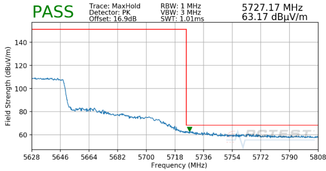
Plot 7-741. (FCC Only) Antenna WF5T (Pk, Ch.122, 802.11ac, MCS5)
