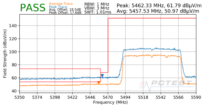
Plot 7-756. Antenna WF5T (Pk & Avg, Ch.106, 802.11ax(SU), MCS5)
