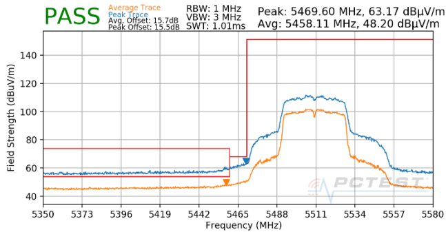
Plot 7-673. Antenna WF5T (Pk & Avg, Ch.102, 802.11n, MCS3)
