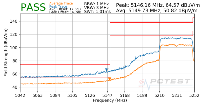
Plot 7-698. Antenna WF5T (Pk & Avg, Ch.46, 802.11ax(SU), MCS5)
