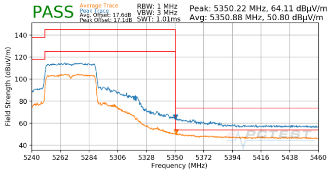
Plot 7-701. Antenna WF5T (Pk & Avg, Ch.54, 802.11ax(SU), MCS5)
