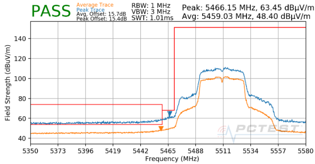
Plot 7-672. Antenna WF5T (Pk & Avg, Ch.102, 802.11n, MCS2)
