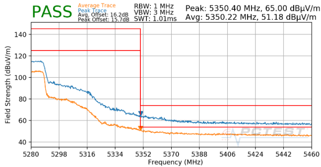
Plot 7-668. Antenna WF5T (Pk & Avg, Ch.54, 802.11n, MCS5)
