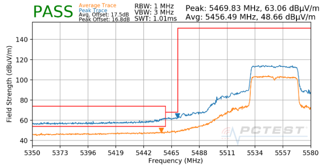
Plot 7-710. Antenna WF5T (Pk & Avg, Ch.110, 802.11ax(SU), MCS5)
