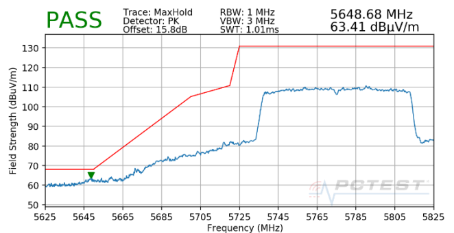
Plot 7-744. Antenna WF5T (Pk, Ch.155, 802.11ac, MCS5)
