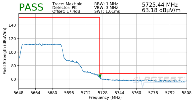
Plot 7-718. Antenna WF5T (Pk, Ch.134, 802.11ax(SU), MCS2)
