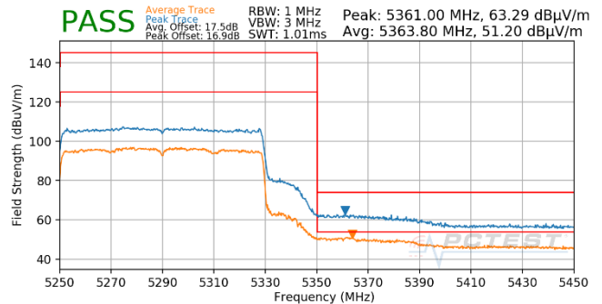
Plot 7-752. Antenna WF5T (Pk & Avg, Ch.58, 802.11ax(SU), MCS3)
