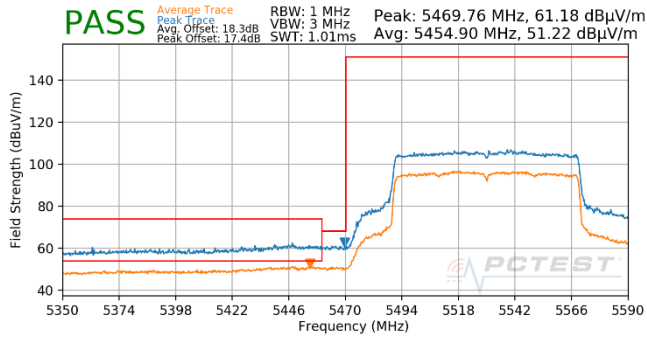
Plot 7-754. Antenna WF5T (Pk & Avg, Ch.106, 802.11ax(SU), MCS2)
