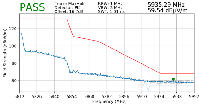
Plot 7-724. Antenna WF5T (Pk, Ch.159, 802.11ax(SU), MCS2)
