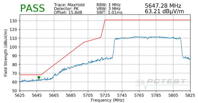
Plot 7-764. Antenna WF5T (Pk, Ch.155, 802.11ax(SU), MCS3)
