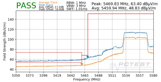
Plot 7-708. Antenna WF5T (Pk & Avg, Ch.110, 802.11ax(SU), MCS2)
