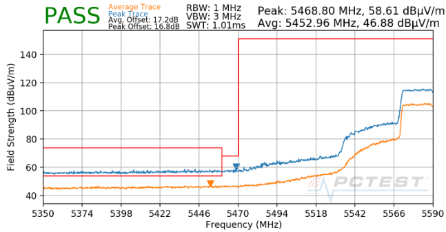
Plot 7-711. (FCC Only) Antenna WF5T (Pk & Avg, Ch.118, 802.11ax(SU), MCS2)
