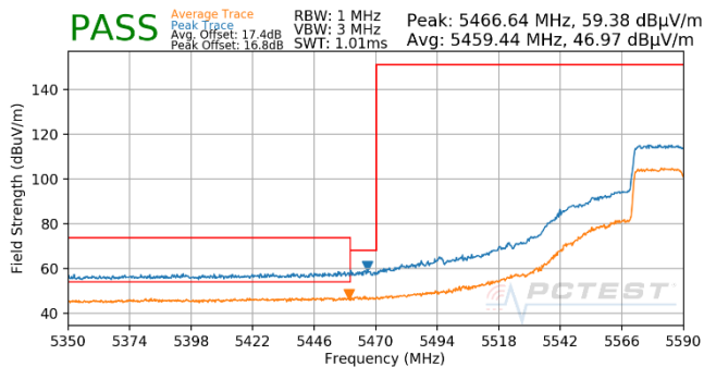
Plot 7-713. (FCC Only) Antenna WF5T (Pk & Avg, Ch.118, 802.11ax(SU), MCS5)
