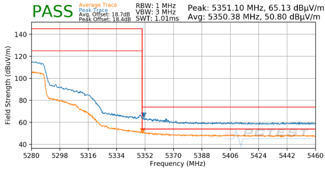
Plot 7-666. Antenna WF5T (Pk & Avg, Ch.54, 802.11n, MCS2)
