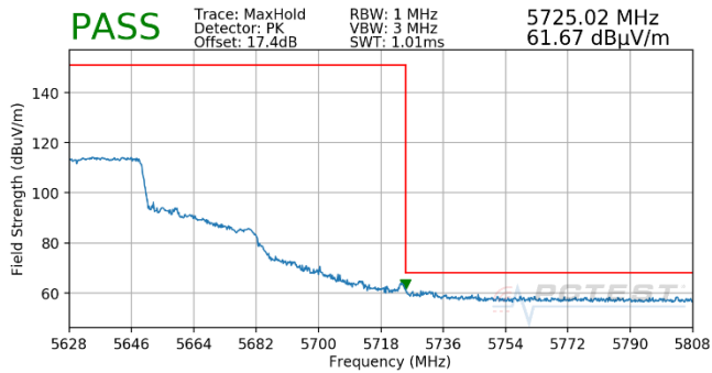
Plot 7-717. (FCC Only) Antenna WF5T (Pk, Ch.126, 802.11ax(SU), MCS5)
