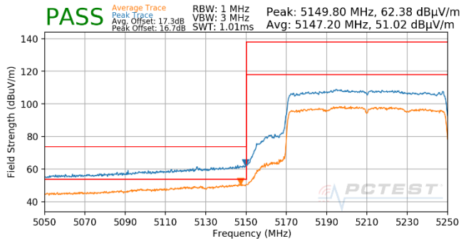
Plot 7-749. Antenna WF5T (Pk & Avg, Ch.42, 802.11ax(SU), MCS3)
