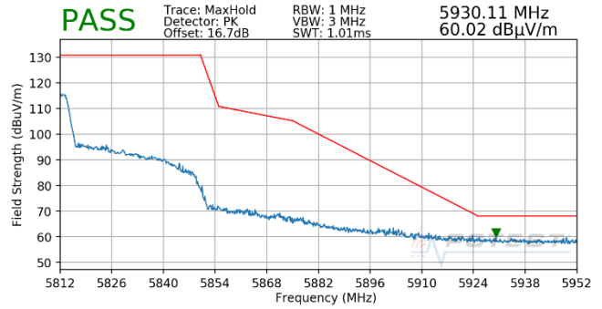
Plot 7-725. Antenna WF5T (Pk, Ch.159, 802.11ax(SU), MCS3)
