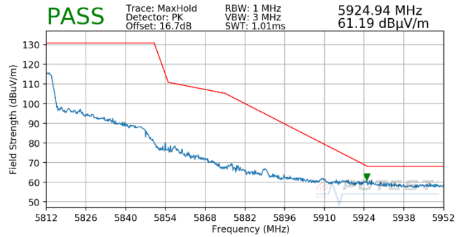
Plot 7-726. Antenna WF5T (Pk, Ch.159, 802.11ax(SU), MCS5)
