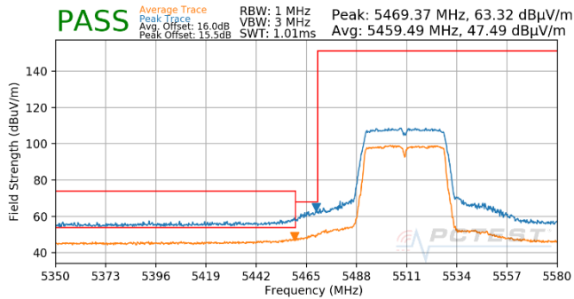
Plot 7-674. Antenna WF5T (Pk & Avg, Ch.102, 802.11n, MCS5)
