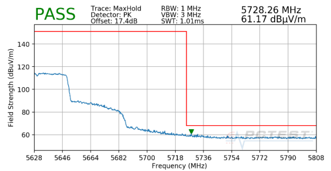
Plot 7-715. (FCC Only) Antenna WF5T (Pk, Ch.126, 802.11ax(SU), MCS2)
