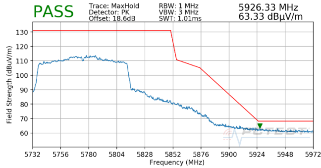
Plot 7-746. Antenna WF5T (Pk, Ch.155, 802.11ac, MCS3)
