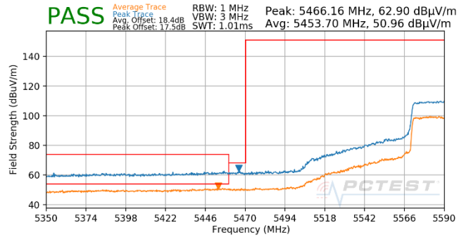
Plot 7-757. (FCC Only) Antenna WF5T (Pk & Avg, Ch.122, 802.11ax(SU), MCS2)
