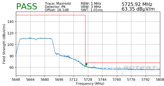
Plot 7-686. Antenna WF5T (Pk, Ch.134, 802.11n, MCS5)
