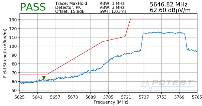
Plot 7-723. Antenna WF5T (Pk, Ch.151, 802.11ax(SU), MCS5)
