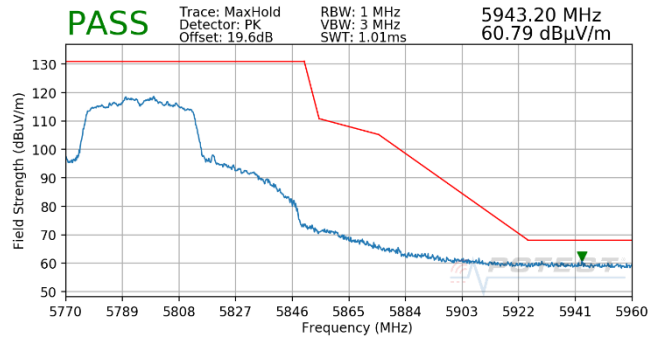
Plot 7-691. Antenna WF5T (Pk, Ch.159, 802.11n, MCS3)
