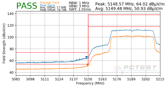
Plot 7-693. Antenna WF5T (Pk & Avg, Ch.38, 802.11ax(SU), MCS2)
