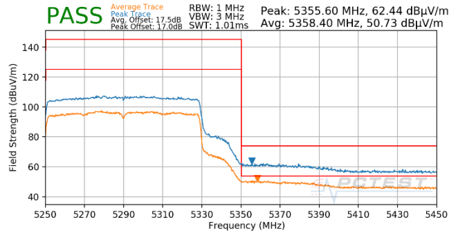
Plot 7-751. Antenna WF5T (Pk & Avg, Ch.58, 802.11ax(SU), MCS2)
