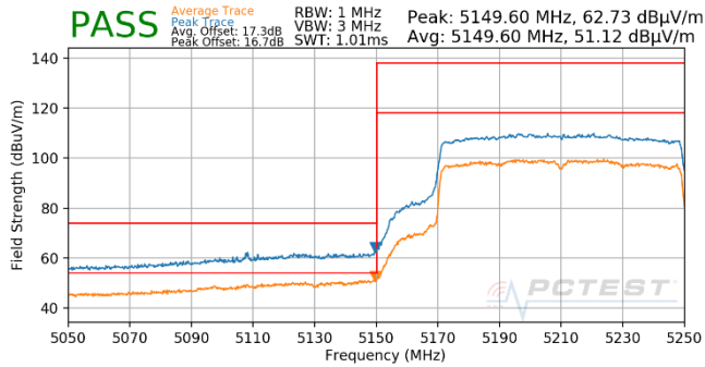
Plot 7-748. Antenna WF5T (Pk & Avg, Ch.42, 802.11ax(SU), MCS2)
