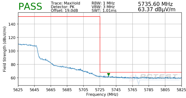
Plot 7-739. (FCC Only) Antenna WF5T (Pk, Ch.122, 802.11ac, MCS2)
