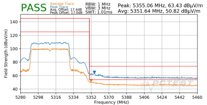
Plot 7-703. Antenna WF5T (Pk & Avg, Ch.62, 802.11ax(SU), MCS3)
