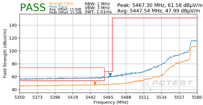
Plot 7-680. (FCC Only) Antenna WF5T (Pk & Avg, Ch.118, 802.11n, MCS5)
