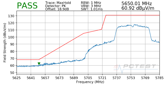
Plot 7-687. Antenna WF5T (Pk, Ch.151, 802.11n, MCS2)
