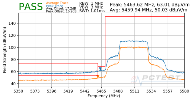
Plot 7-705. Antenna WF5T (Pk & Avg, Ch.102, 802.11ax(SU), MCS2)
