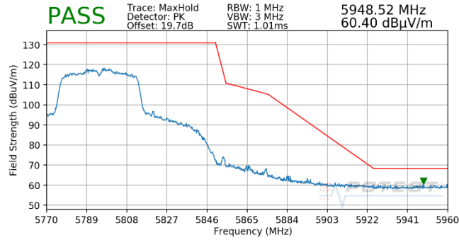
Plot 7-690. Antenna WF5T (Pk, Ch.159, 802.11n, MCS2)
