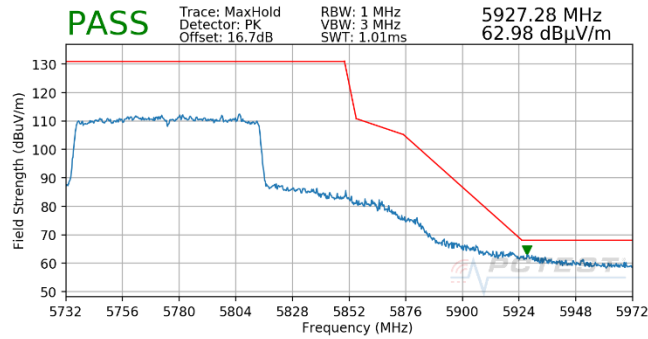
Plot 7-768. Antenna WF5T (Pk, Ch.155, 802.11ax(SU), MCS5)
