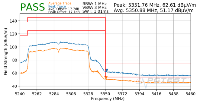
Plot 7-731. Antenna WF5T (Pk & Avg, Ch.58, 802.11ac, MCS3)
