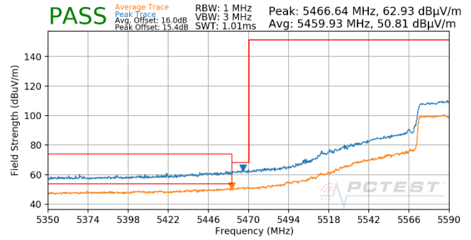
Plot 7-737. (FCC Only) Antenna WF5T (Pk & Avg, Ch.122, 802.11ac, MCS3)
