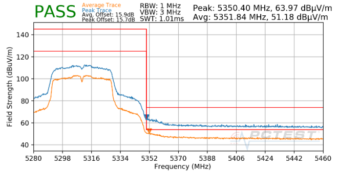
Plot 7-669. Antenna WF5T (Pk & Avg, Ch.62, 802.11n, MCS2)
