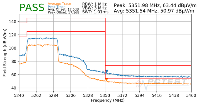
Plot 7-700. Antenna WF5T (Pk & Avg, Ch.54, 802.11ax(SU), MCS3)
