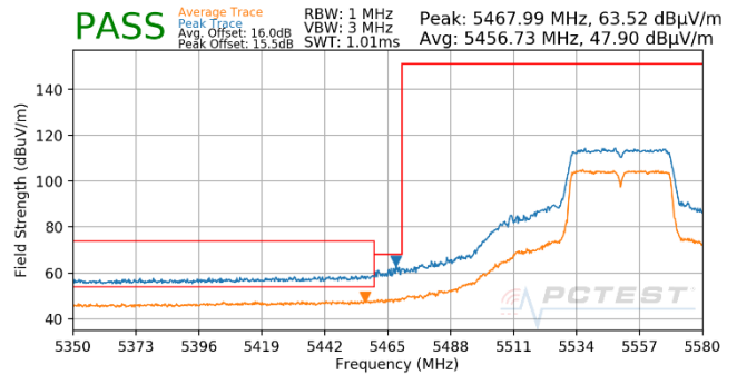
Plot 7-677. Antenna WF5T (Pk & Avg, Ch.110, 802.11n, MCS5)
