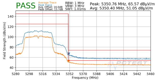
Plot 7-670. Antenna WF5T (Pk & Avg, Ch.62, 802.11n, MCS3)
