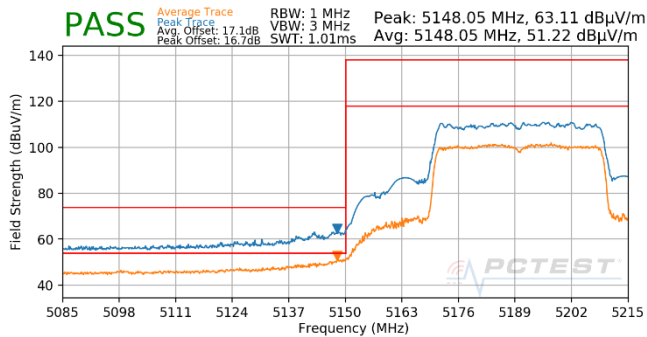
Plot 7-694. Antenna WF5T (Pk & Avg, Ch.38, 802.11ax(SU), MCS3)
