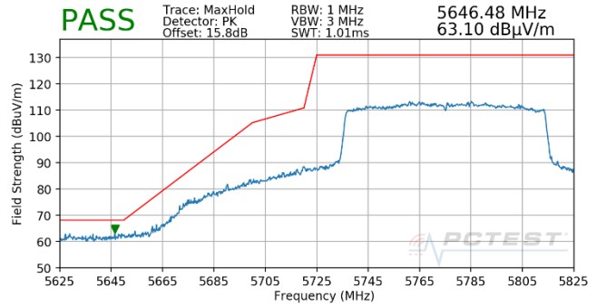
Plot 7-763. Antenna WF5T (Pk, Ch.155, 802.11ax(SU), MCS2)
