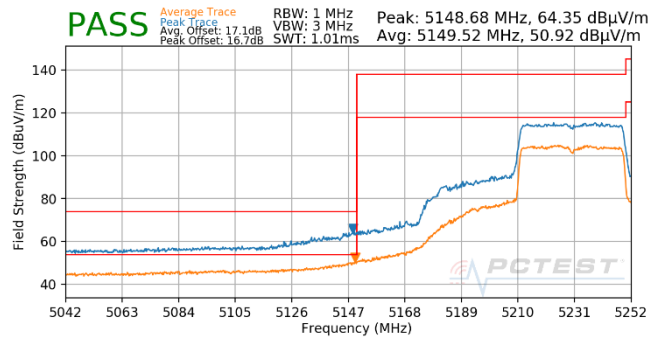
Plot 7-697. Antenna WF5T (Pk & Avg, Ch.46, 802.11ax(SU), MCS3)
