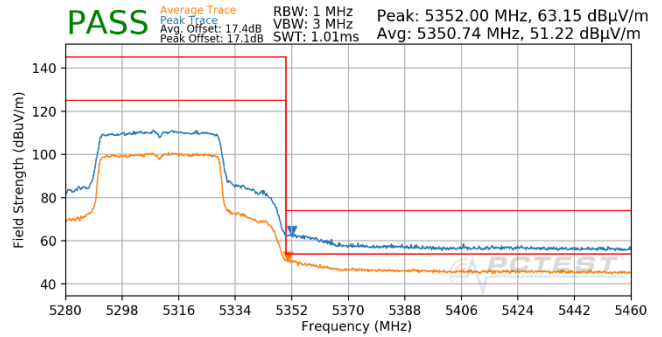
Plot 7-702. Antenna WF5T (Pk & Avg, Ch.62, 802.11ax(SU), MCS2)
