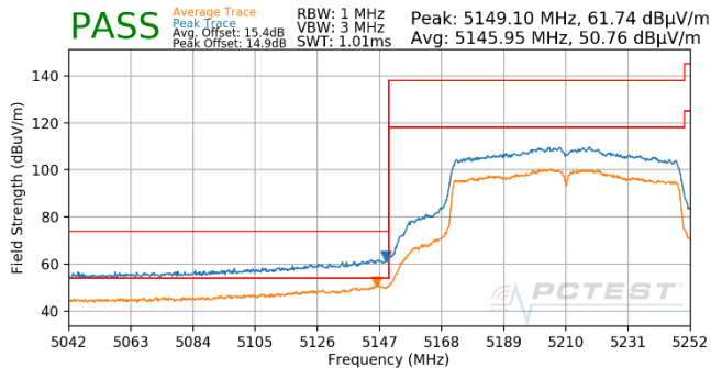
Plot 7-727. Antenna WF5T (Pk & Avg, Ch.42, 802.11ac, MCS2)
