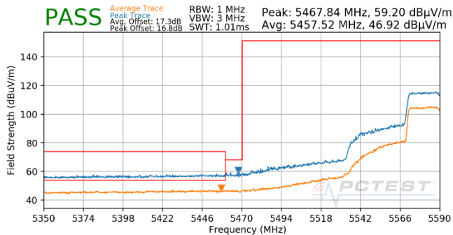
Plot 7-712. (FCC Only) Antenna WF5T (Pk & Avg, Ch.118, 802.11ax(SU), MCS3)
