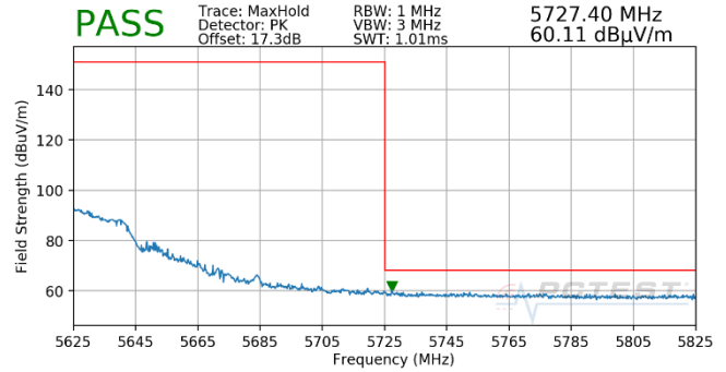
Plot 7-714. (FCC Only) Antenna WF5T (Pk, Ch.118, 802.11ax(SU), MCS5)
