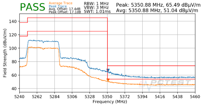
Plot 7-699. Antenna WF5T (Pk & Avg, Ch.54, 802.11ax(SU), MCS2)
