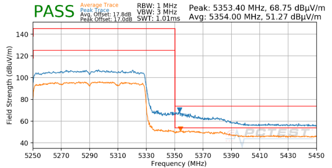
Plot 7-753. Antenna WF5T (Pk & Avg, Ch.58, 802.11ax(SU), MCS5)
