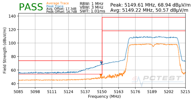
Plot 7-695. Antenna WF5T (Pk & Avg, Ch.38, 802.11ax(SU), MCS5)
