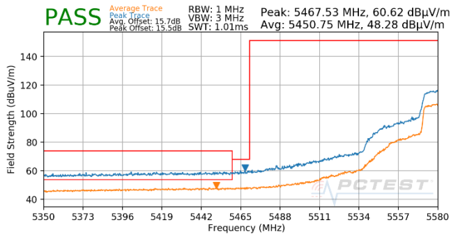
Plot 7-679. (FCC Only) Antenna WF5T (Pk & Avg, Ch.118, 802.11n, MCS3)
