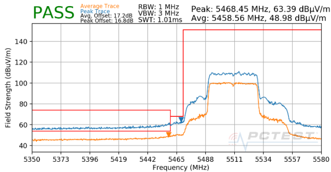
Plot 7-706. Antenna WF5T (Pk & Avg, Ch.102, 802.11ax(SU), MCS3)
