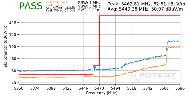
Plot 7-758. (FCC Only) Antenna WF5T (Pk & Avg, Ch.122, 802.11ax(SU), MCS3)
