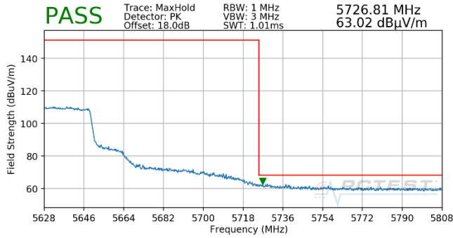
Plot 7-760. (FCC Only) Antenna WF5T (Pk, Ch.122, 802.11ax(SU), MCS2)
