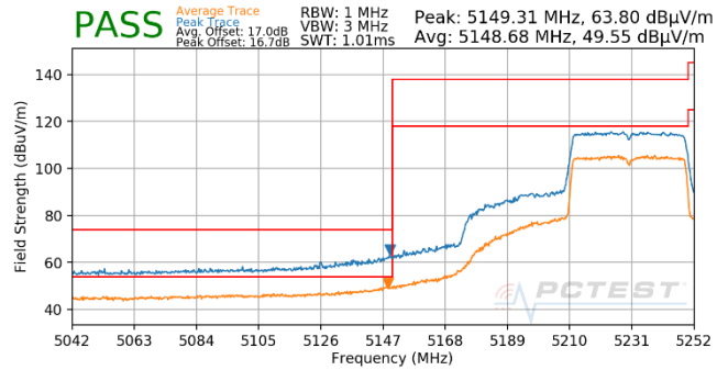
Plot 7-696. Antenna WF5T (Pk & Avg, Ch.46, 802.11ax(SU), MCS2)
