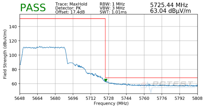
Plot 7-719. Antenna WF5T (Pk, Ch.134, 802.11ax(SU), MCS3)
