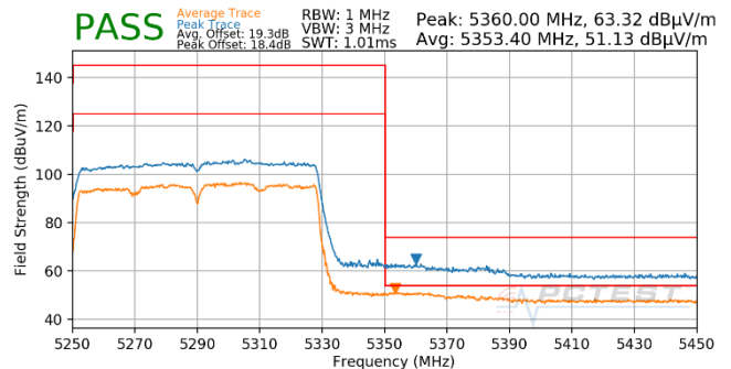
Plot 7-732. Antenna WF5T (Pk & Avg, Ch.58, 802.11ac, MCS5)
