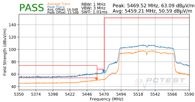
Plot 7-734. Antenna WF5T (Pk & Avg, Ch.106, 802.11ac, MCS3)
