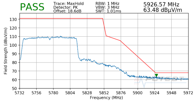
Plot 7-747. Antenna WF5T (Pk, Ch.155, 802.11ac, MCS5)
