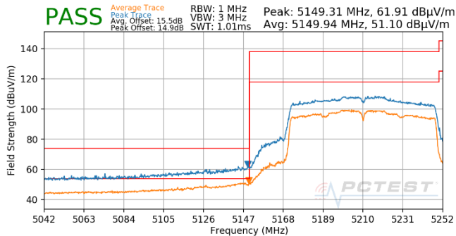
Plot 7-728. Antenna WF5T (Pk & Avg, Ch.42, 802.11ac, MCS3)
