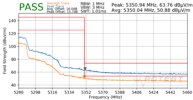
Plot 7-667. Antenna WF5T (Pk & Avg, Ch.54, 802.11n, MCS3)
