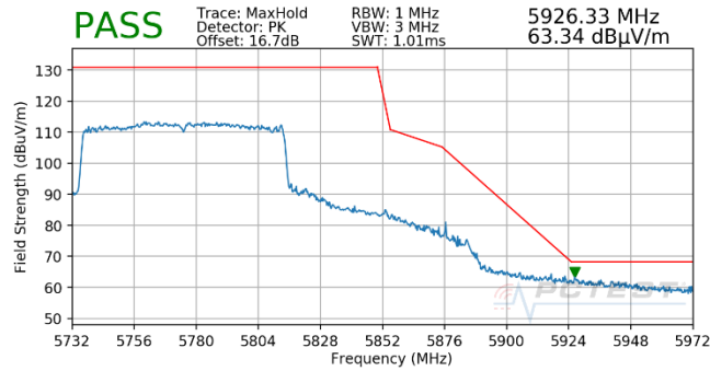
Plot 7-767. Antenna WF5T (Pk, Ch.155, 802.11ax(SU), MCS3)
