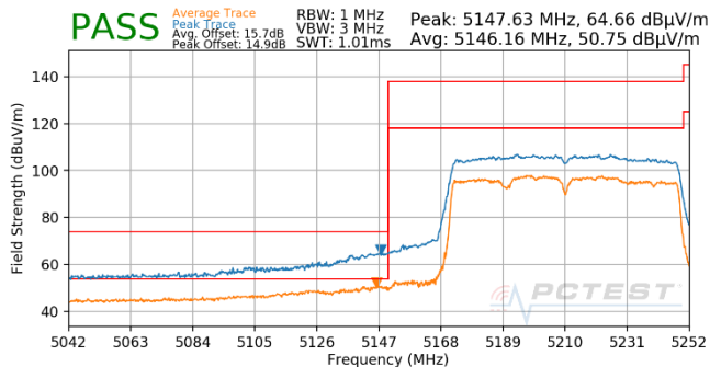
Plot 7-729. Antenna WF5T (Pk & Avg, Ch.42, 802.11ac, MCS5)
