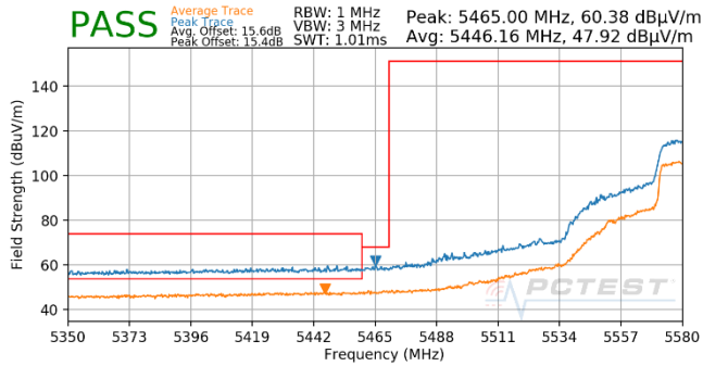
Plot 7-678. (FCC Only) Antenna WF5T (Pk & Avg, Ch.118, 802.11n, MCS2)
