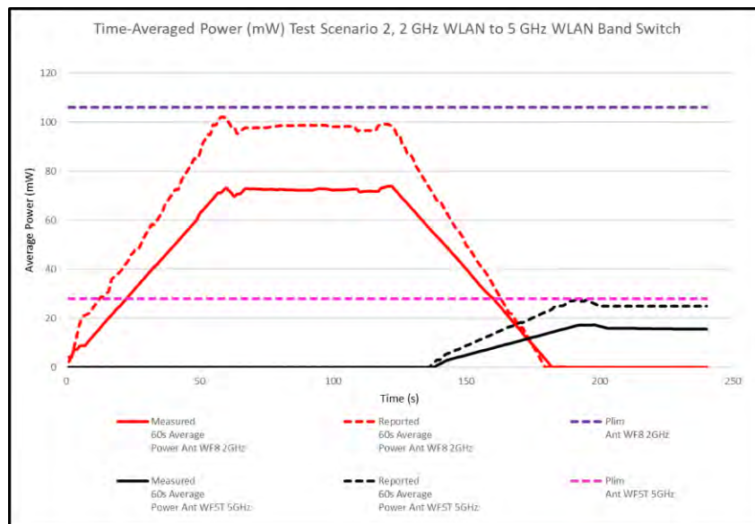
Figure G-6 60s Average Power vs. Time during Band Switch
