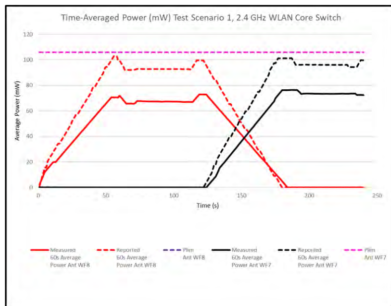
Figure G-2 60s Average Power vs. Time, 2.4 GHz
