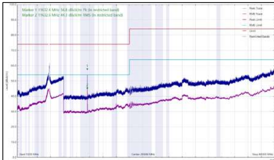
Figure 1076 - 5825 MHz (CH165), HE20, RU26-0, Core 0 + Core 1, 1 GHz to 40 GHz, Horizontal
