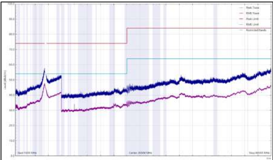
Figure 1054 - U-NII-2C - 5500 MHz (CH100), HT20, CDD, Core 0 + Core 1, 1 GHz to 40 GHz, Vertical
