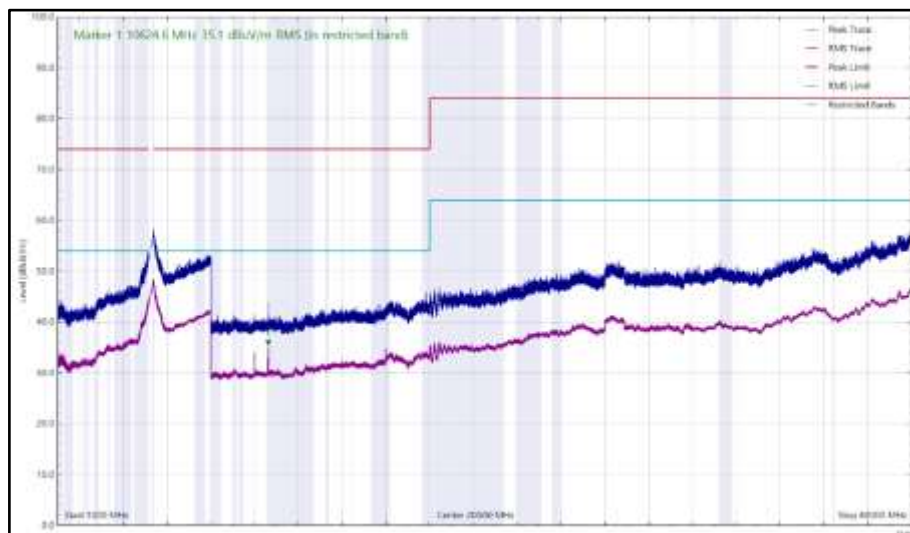
Figure 1068 - 5320 MHz (CH64), HE20, RU52-37, Core 0 + Core 1, 1 GHz to 40 GHz, Vertical
