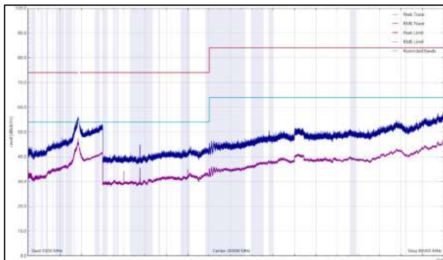
Figure 1058 - U-NII-3 - 5745 MHz (CH149), HT20, CDD, Core 0 + Core 1, 1 GHz to 40 GHz, Vertical
