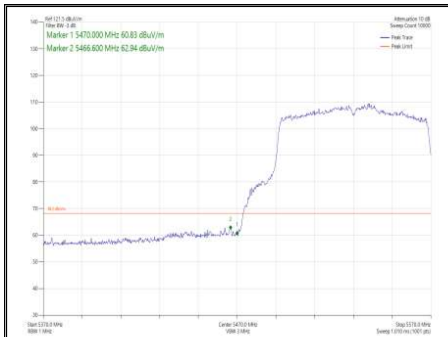
Figure 1011 - 802.11ac VHT80 Core 1 - 5530 MHz Band Edge Frequency 5470 MHz
