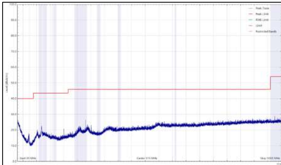
Figure 1059 - U-NII-3 - 5825 MHz (CH165), HT20, CDD, Core 0 + Core 1, 30 MHz to 1 GHz, Horizontal
