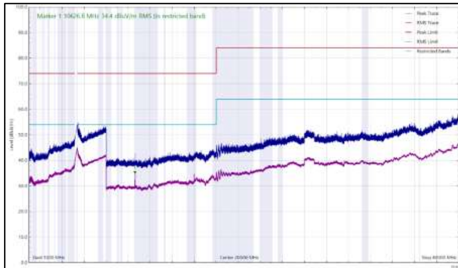
Figure 1067 - 5320 MHz (CH64), HE20, RU52-37, Core 0 + Core 1, 1 GHz to 40 GHz, Horizontal
