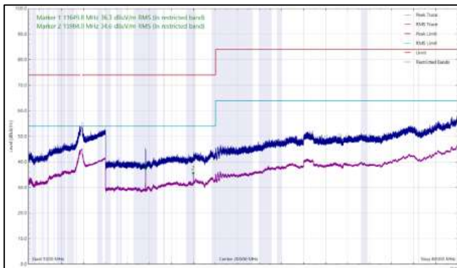
Figure 1060 - U-NII-3 - 5825 MHz (CH165), HT20, CDD, Core 0 + Core 1, 1 GHz to 40 GHz, Horizontal
