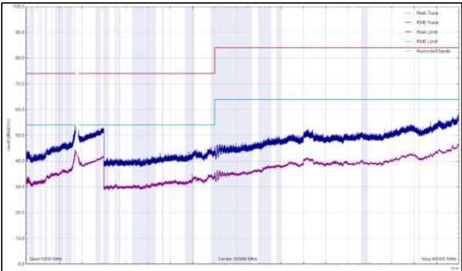
Figure 1053 - U-NII-2C - 5500 MHz (CH100), HT20, CDD, Core 0 + Core 1, 1 GHz to 40 GHz, Horizontal
