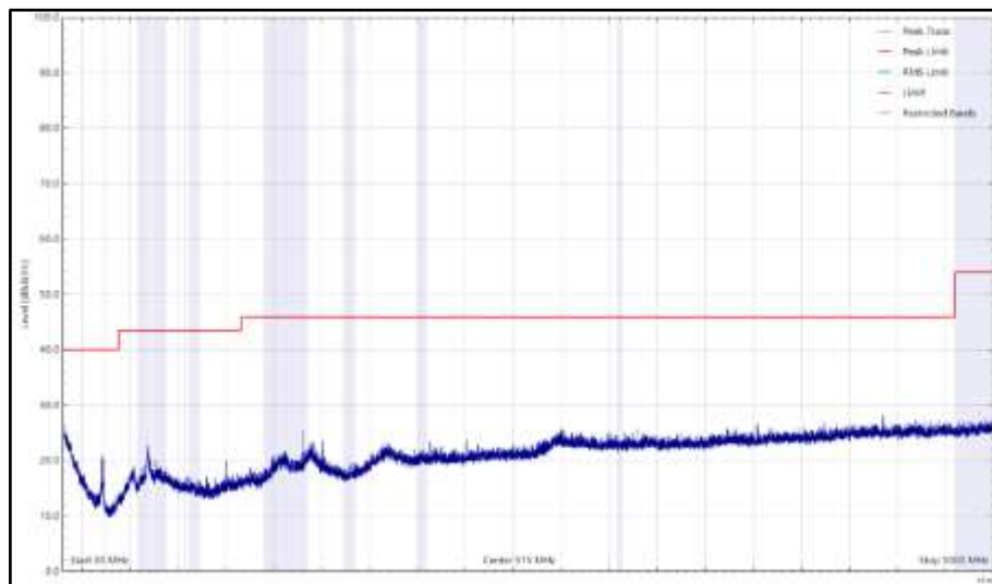
Figure 1075 - 5825 MHz (CH165), HE20, RU26-0, Core 0 + Core 1, 30 MHz to 1 GHz, Horizontal
