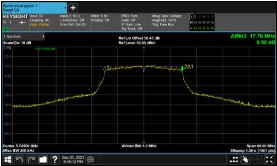
Figure 903 - Core 0 (A) 5745 MHz (CH149) 99% Bandwidth
