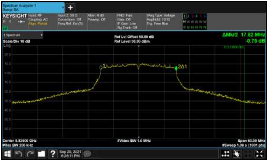
Figure 913 - Core 1 (B) 5825 MHz (CH165) 99% Bandwidth
