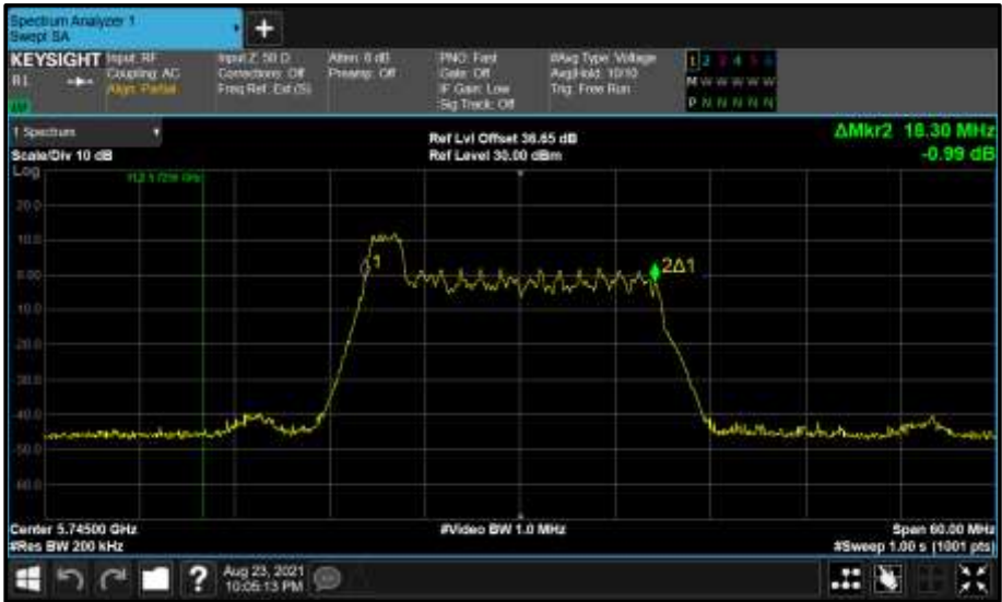
Figure 747 - Core 1 (B) 5745 MHz (CH149) 99% Bandwidth
