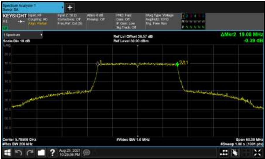
Figure 731 - Core 0 (A) 5785 MHz (CH157) 99% Bandwidth
