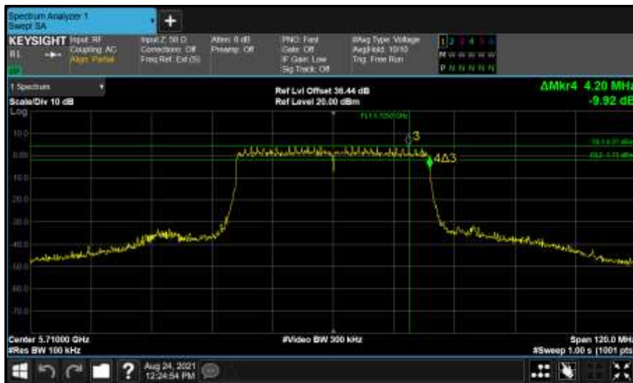
Figure 868 - Core 0 (A) 5710 MHz (CH142) 6 dB Bandwidth
