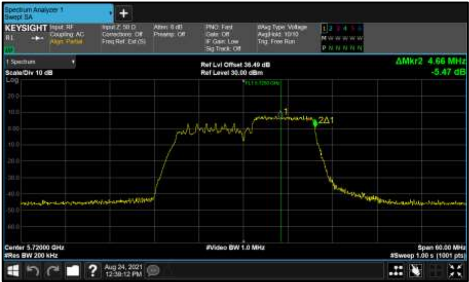
Figure 833 - Core 0 (A) 5720 MHz (CH144) 99% Bandwidth
