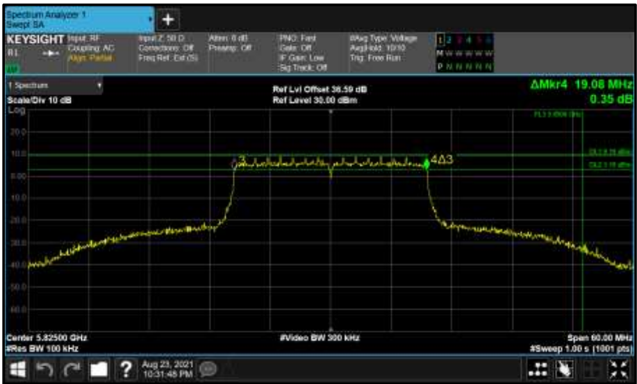
Figure 738 - Core 1 (B) 5825 MHz (CH165) 6 dB Bandwidth
