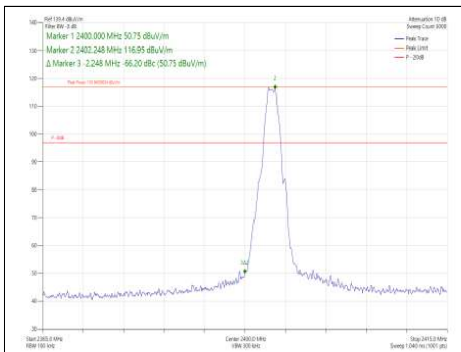
Figure 238 - GFSK/DH1- 2402 MHz – Band Edge Frequency 2400.0 MHz
