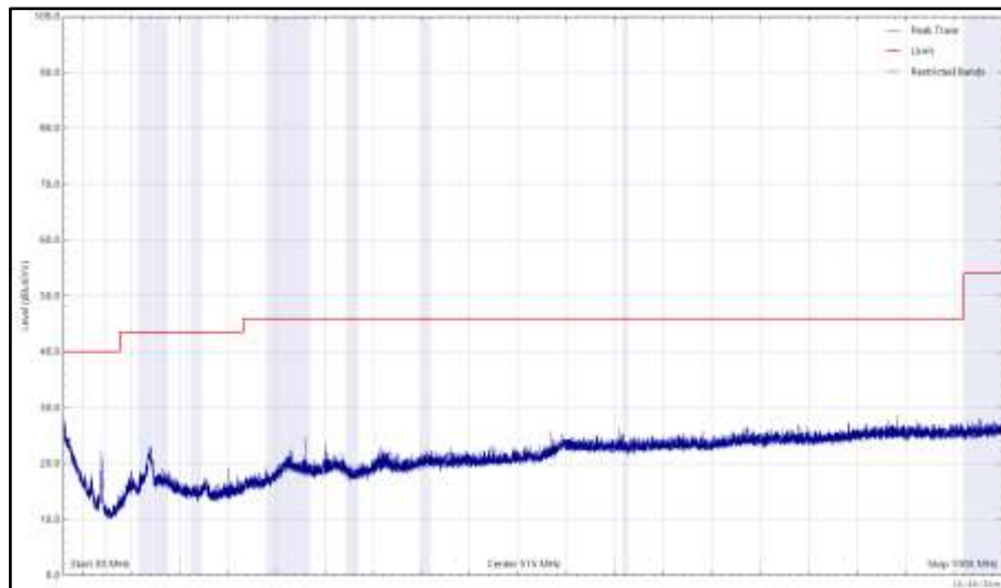
Figure 220 - 2440 MHz (CH17), LE1M, iPA, Core 0 + Core 1, 30 MHz to 1 GHz, Horizontal (Peak)
