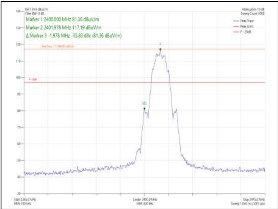
Figure 239 - GFSK/DH1- 2402 MHz – Band Edge Frequency 2400.0 MHz
