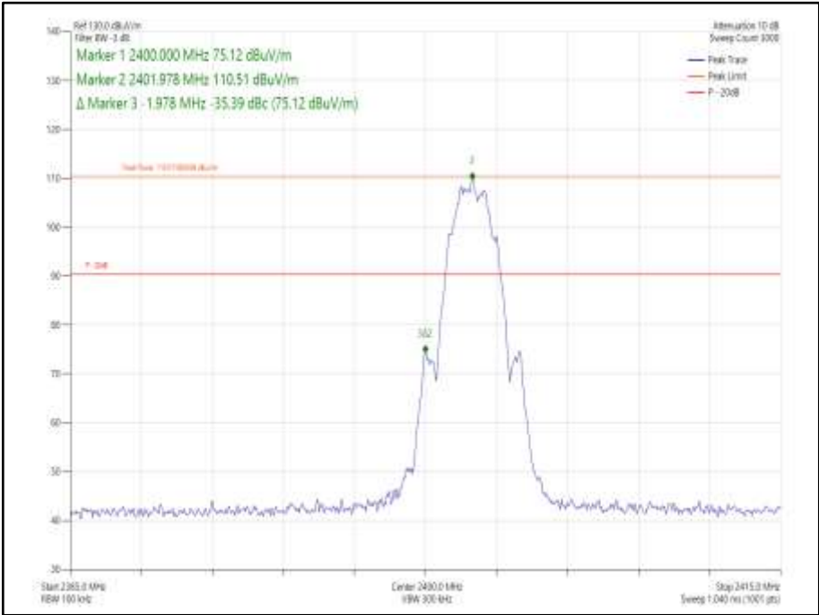
Figure 240 - GFSK/DH1- 2402 MHz – Band Edge Frequency 2400.0 MHz
