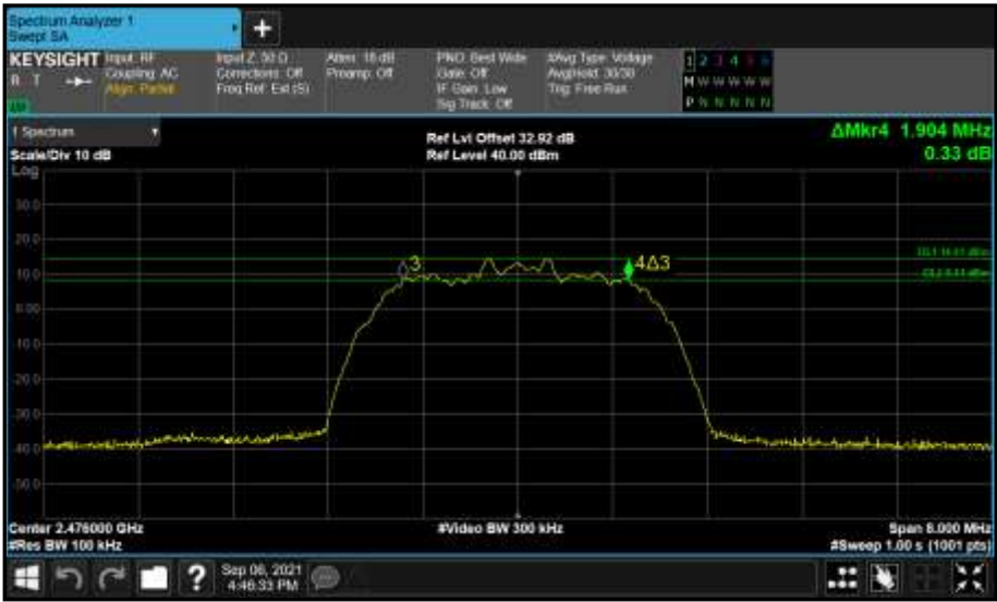
Figure 62 - Core 0 (A) 2476 MHz (CH74) 6 dB Bandwidth
