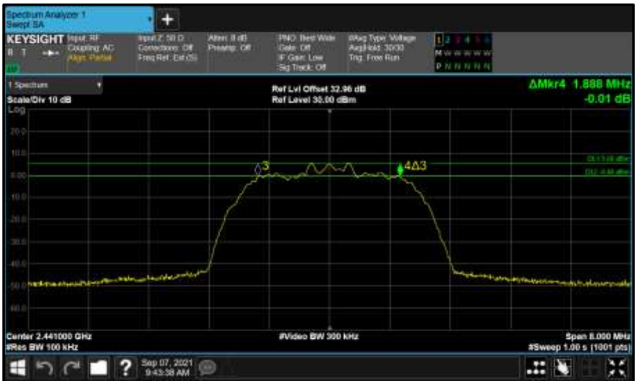
Figure 128 - Core 2 (C) 2441 MHz (CH39) 6 dB Bandwidth
