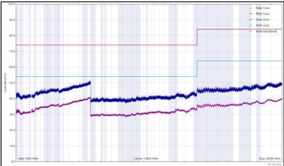
Figure 216 - 2480 MHz (CH39), LE1M, ePA, Core 0 + Core 1, 1 GHz to 26 GHz, Horizontal
