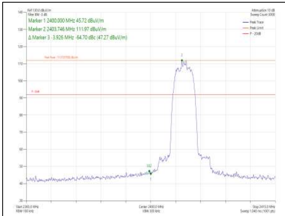
Figure 244 Core 0- GFSK/DH1- 2402 MHz – Band Edge Frequency 2400.0 MHz
