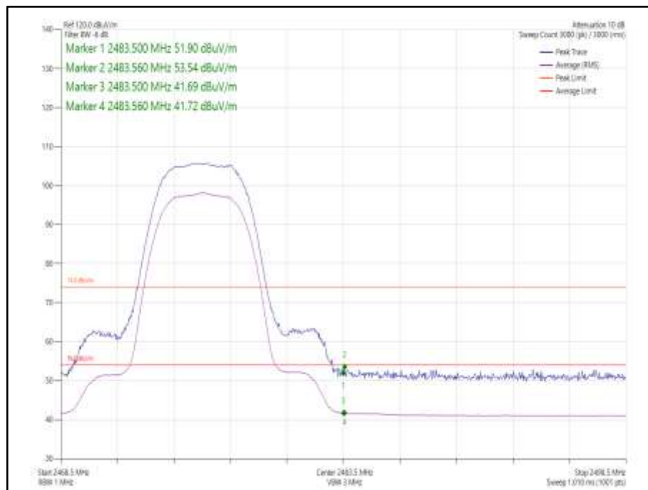
Figure 32 - Static - GFSK/4DH5 - 2476 MHz - Band Edge Frequency 2483.5 MHz
