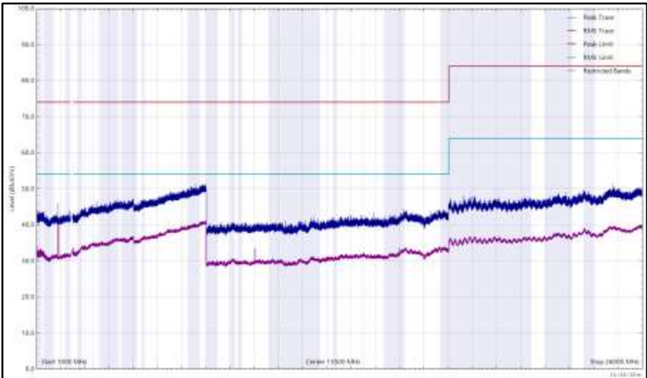
Figure 233 - 2480 MHz (CH39), LE1M, iPA, Core 2, 1 GHz to 26 GHz, Vertical
