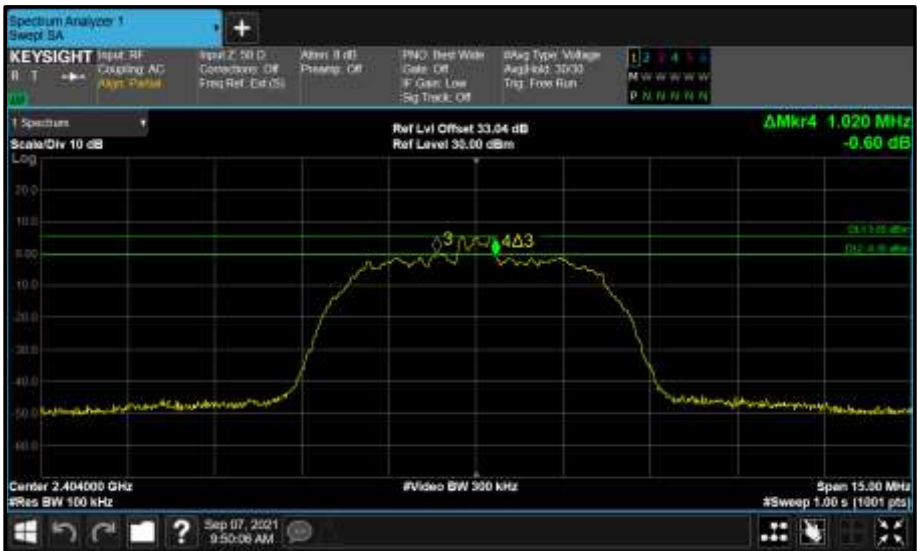
Figure 132 - Core 2 (C) 2404 MHz (CH2) 6 dB Bandwidth
