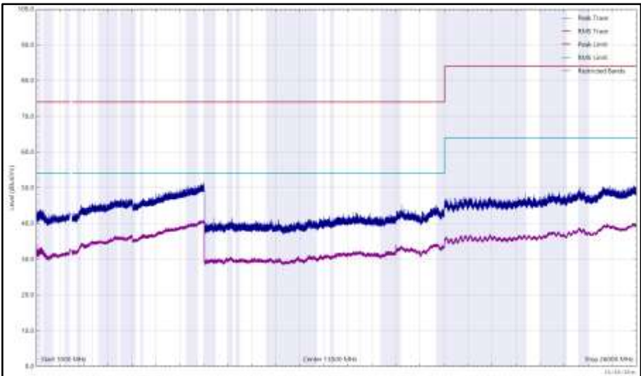
Figure 218 - 2402 MHz (CH37), LE1M, iPA, Core 0 + Core 1, 1 GHz to 26 GHz, Horizontal
