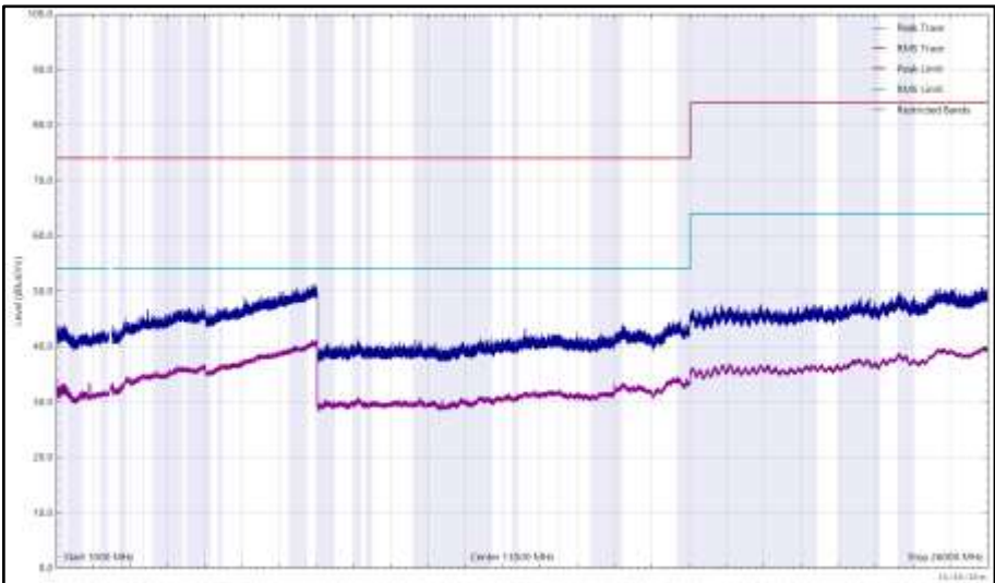
Figure 224 - 2480 MHz (CH39), LE1M, iPA, Core 0 + Core 1, 1 GHz to 26 GHz, Horizontal
