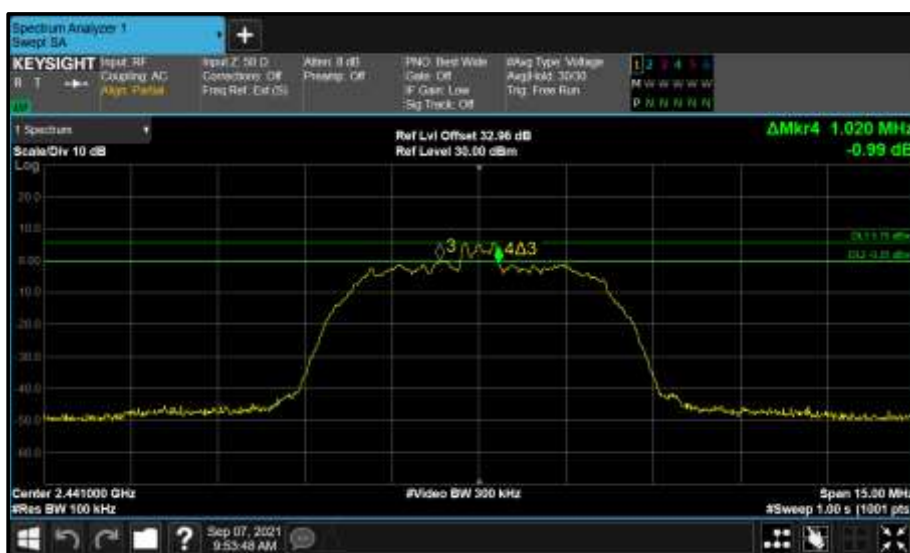
Figure 134 - Core 2 (C) 2441 MHz (CH39) 6 dB Bandwidth
