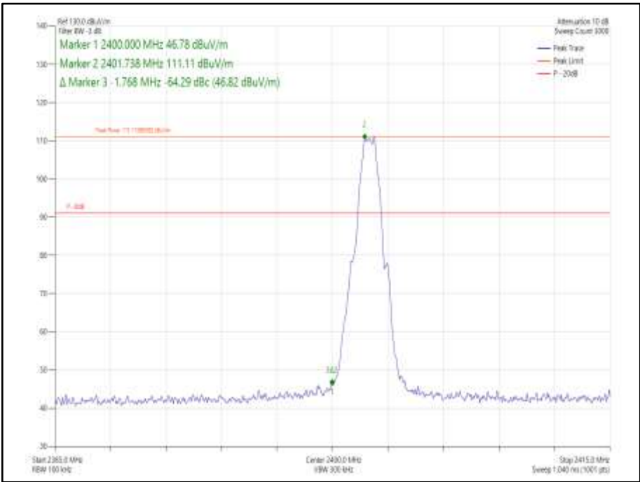
Figure 235 - GFSK/DH1- 2402 MHz – Band Edge Frequency 2400.0 MHz
