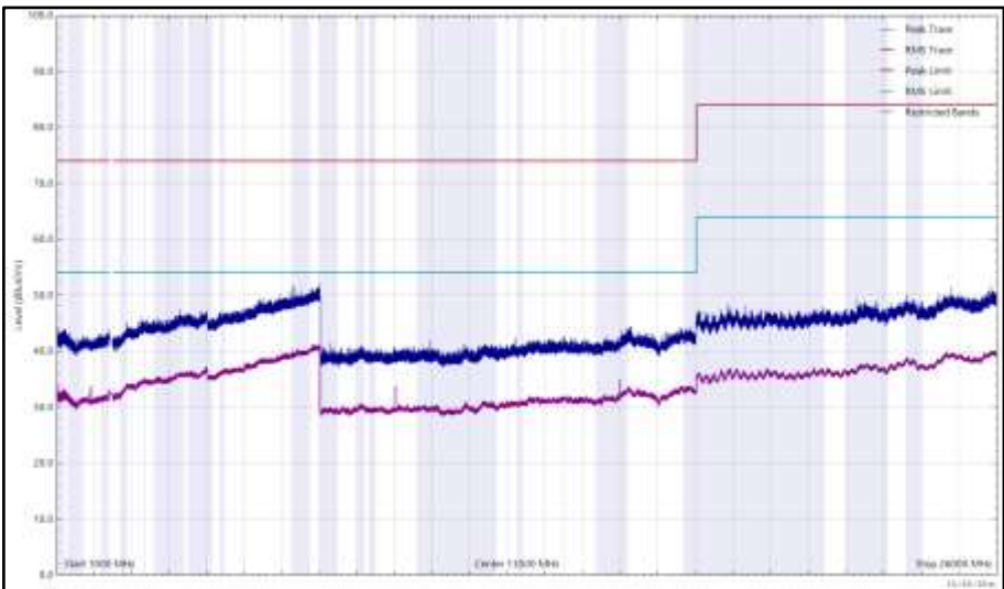
Figure 227 - 2402 MHz (CH37), LE1M, iPA, Core 2, 1 GHz to 26 GHz, Vertical
