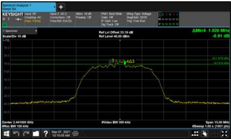
Figure 50 - Core 1 (B) 2441 MHz (CH39) 6 dB Bandwidth
