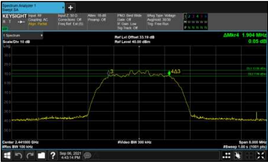
Figure 60 - Core 1 (B) 2441 MHz (CH39) 6 dB Bandwidth
