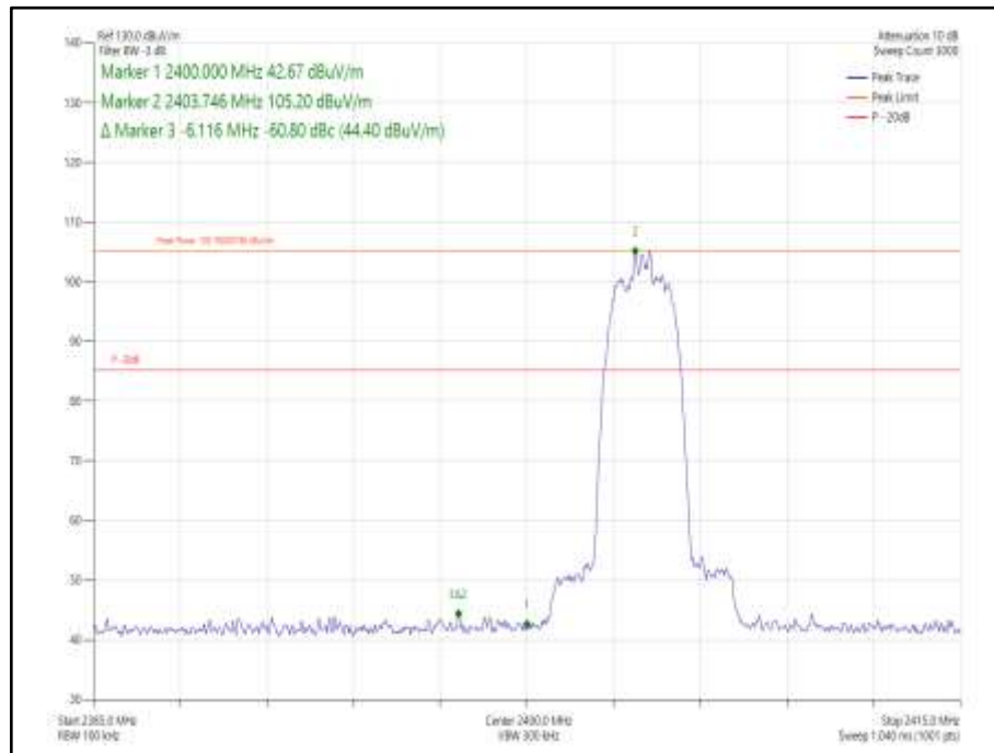
Figure 245 Core 0- GFSK/DH1- 2402 MHz – Band Edge Frequency 2400.0 MHz
