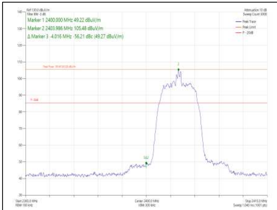
Figure 251 Core 0- GFSK/DH1- 2402 MHz – Band Edge Frequency 2400.0 MHz
