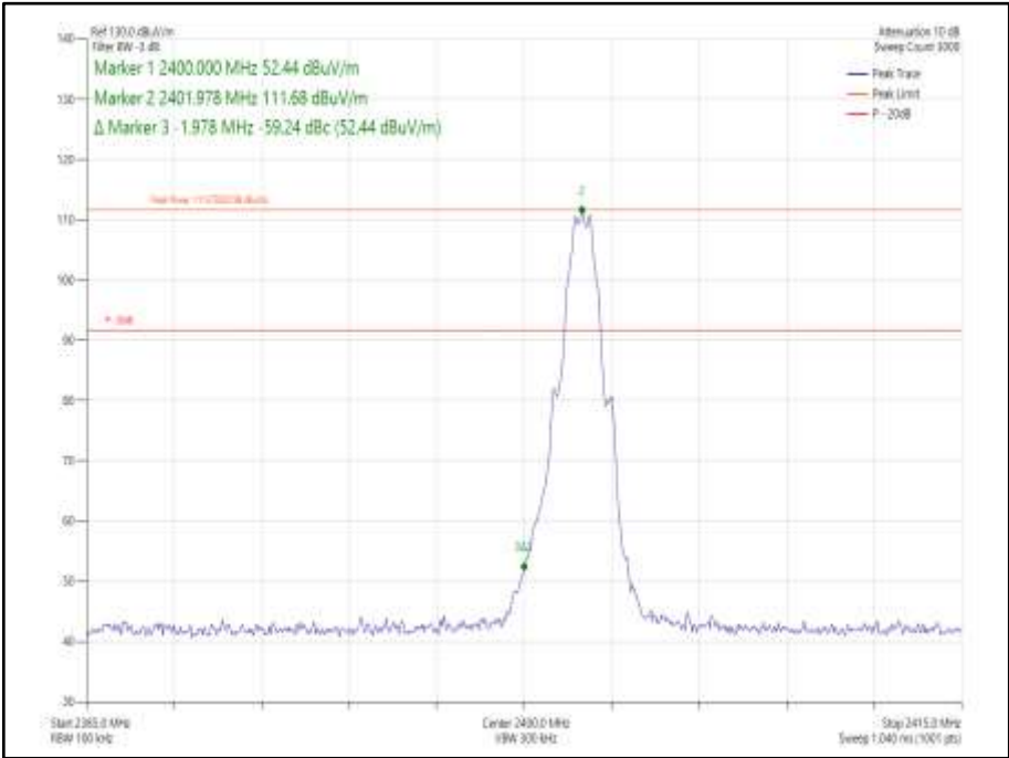
Figure 236 - GFSK/DH1- 2402 MHz – Band Edge Frequency 2400.0 MHz
