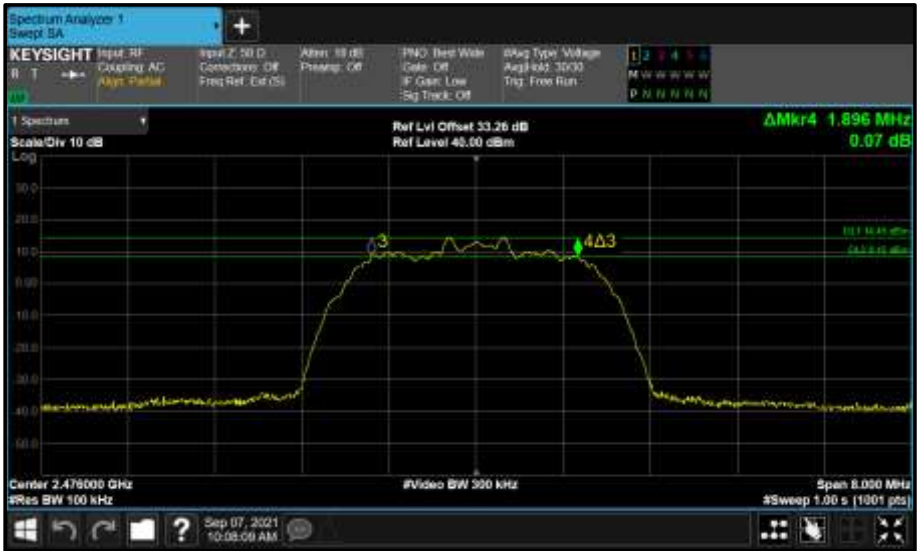
Figure 46 - Core 1 (B) 2476 MHz (CH74) 6 dB Bandwidth
