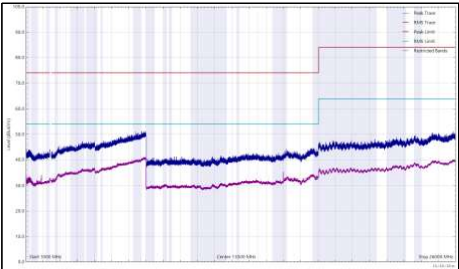
Figure 226 - 2402 MHz (CH37), LE1M, iPA, Core 2, 1 GHz to 26 GHz, Horizontal
