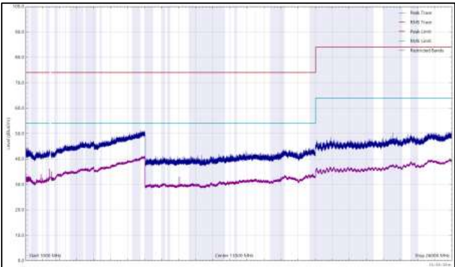
Figure 223 - 2440 MHz (CH17), LE1M, iPA, Core 0 + Core 1, 1 GHz to 26 GHz, Vertical
