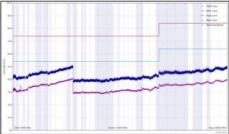
Figure 229 - 2440 MHz (CH17), LE1M, iPA, Core 2, 1 GHz to 26 GHz, Horizontal
