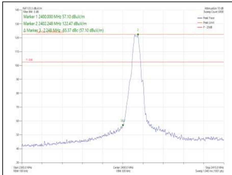
Figure 237 - GFSK/DH1- 2402 MHz – Band Edge Frequency 2400.0 MHz
