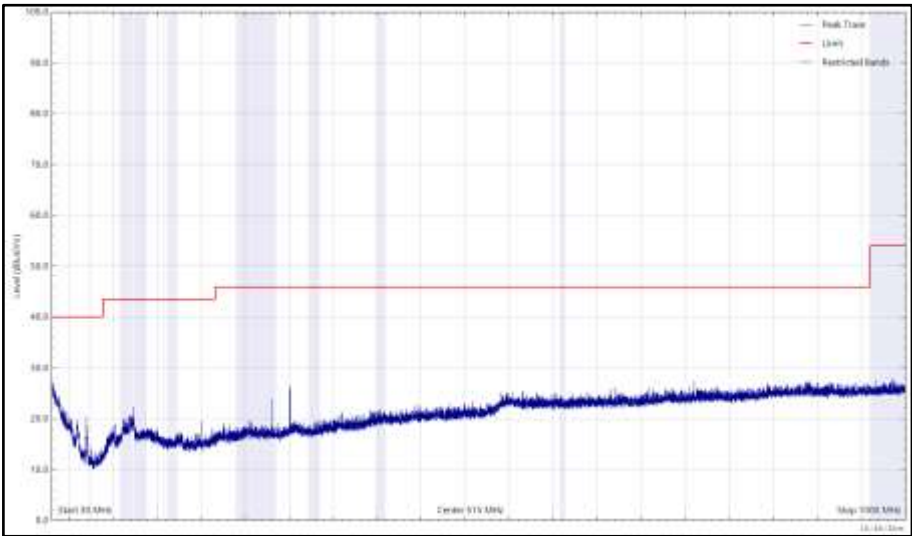
Figure 230 - 2440 MHz (CH17), LE1M, iPA, Core 2, 30 MHz to 1 GHz, Vertical (Peak)
