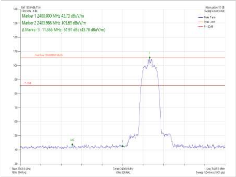
Figure 246 Core 0- GFSK/DH1- 2402 MHz – Band Edge Frequency 2400.0 MHz
