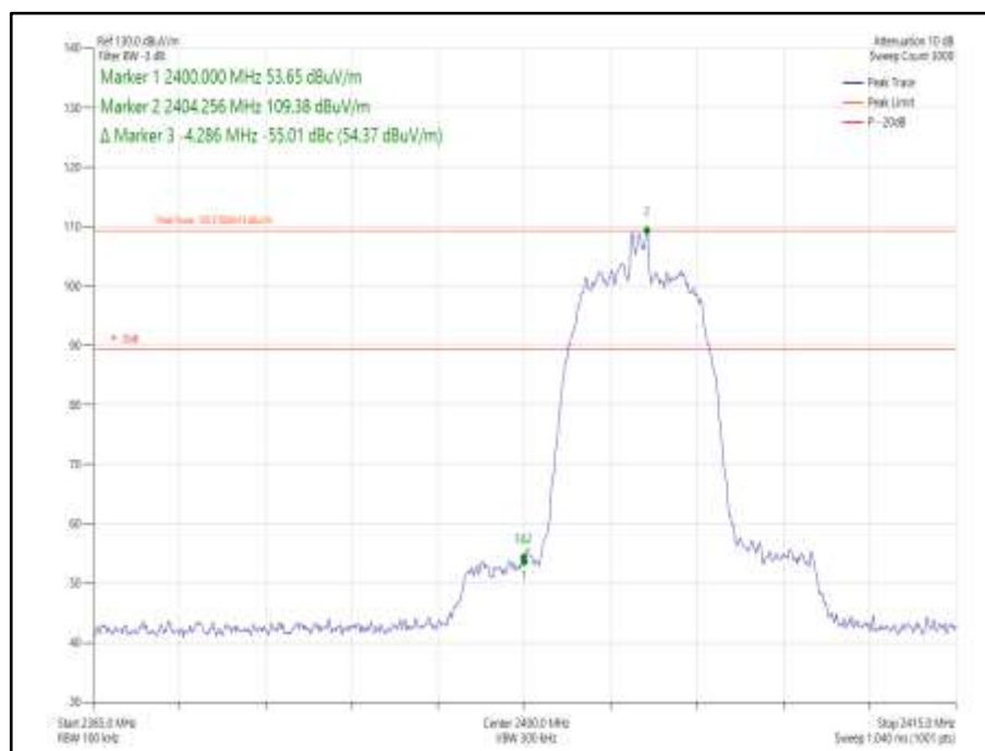
Figure 253 Core 0- GFSK/DH1- 2402 MHz – Band Edge Frequency 2400.0 MHz
