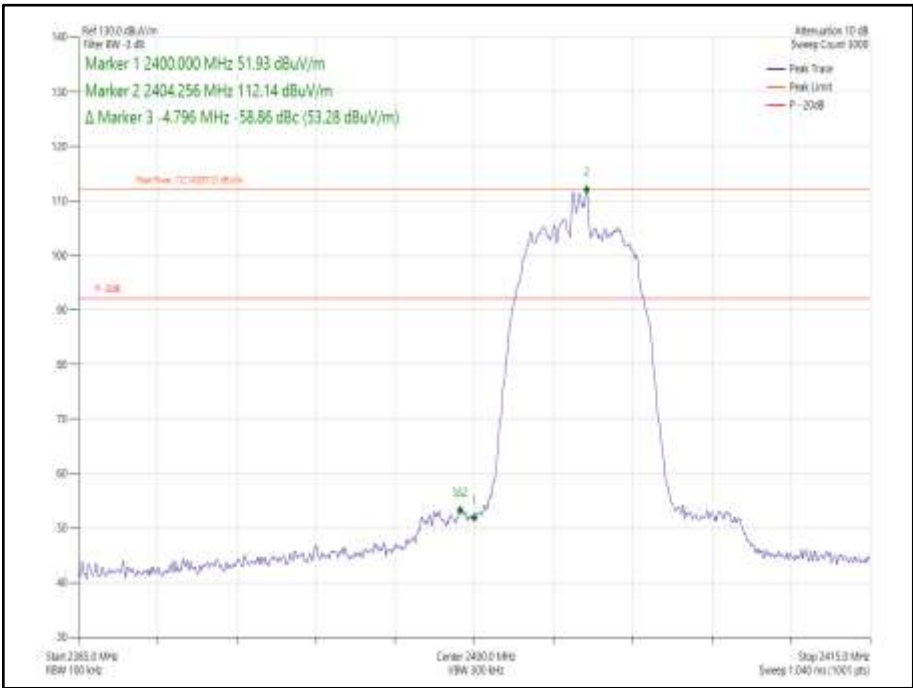
Figure 249 Core 0- GFSK/DH1- 2402 MHz – Band Edge Frequency 2400.0 MHz
