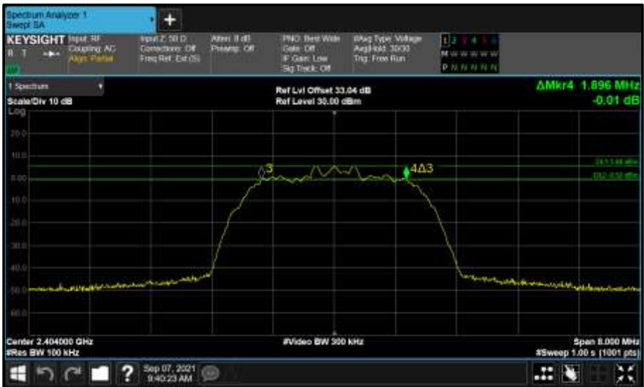
Figure 126 - Core 2 (C) 2404 MHz (CH2) 6 dB Bandwidth
