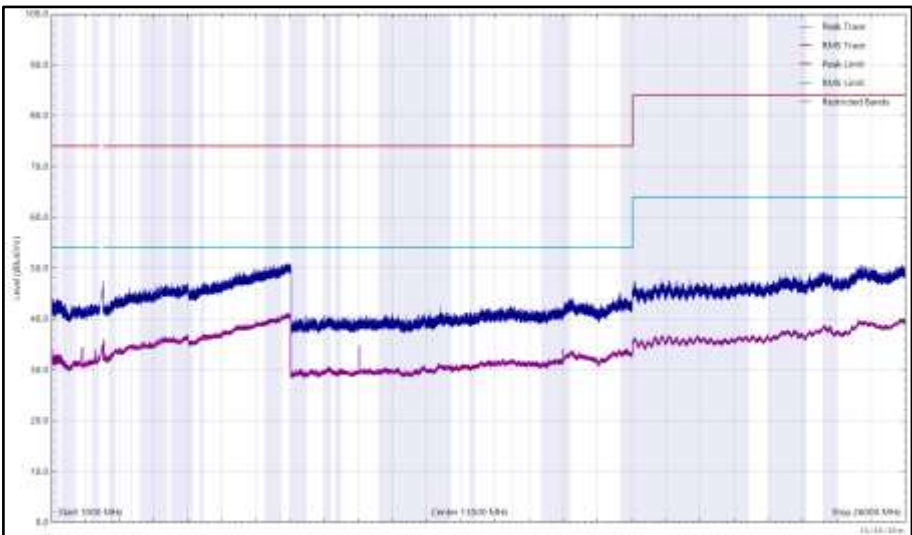
Figure 225 - 2480 MHz (CH39), LE1M, iPA, Core 0 + Core 1, 1 GHz to 26 GHz, Vertical
