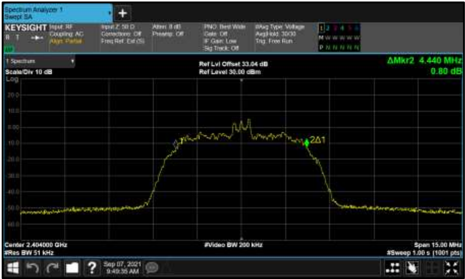
Figure 131 - Core 2 (C) 2404 MHz (CH2) 99% Bandwidth
