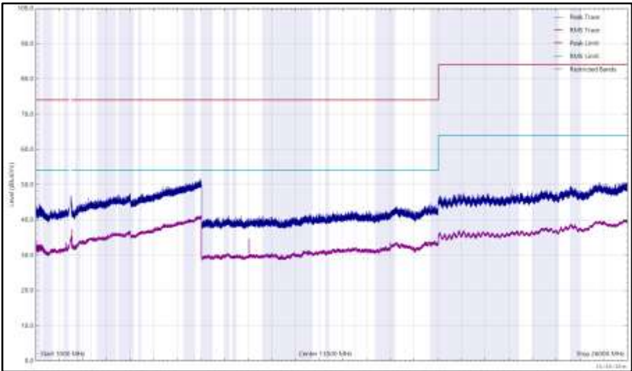
Figure 217 - 2480 MHz (CH39), LE1M, ePA, Core 0 + Core 1, 1 GHz to 26 GHz, Vertical
