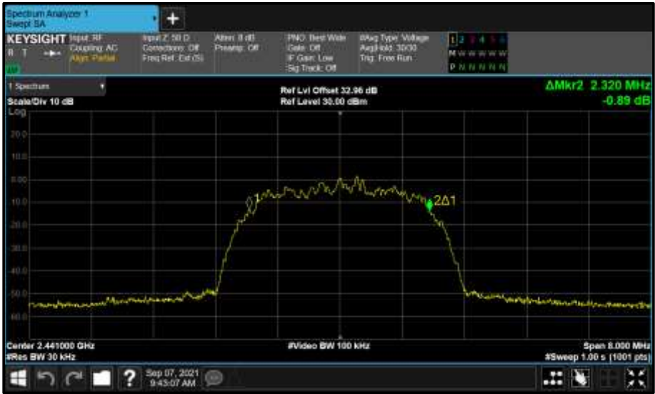
Figure 127 - Core 2 (C) 2441 MHz (CH39) 99% Bandwidth
