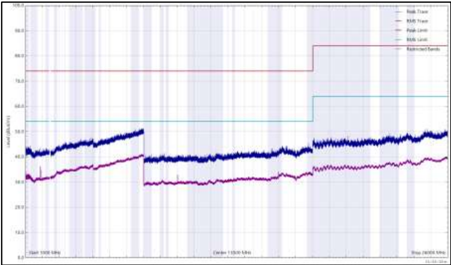
Figure 231 - 2440 MHz (CH17), LE1M, iPA, Core 2, 1 GHz to 26 GHz, Vertical
