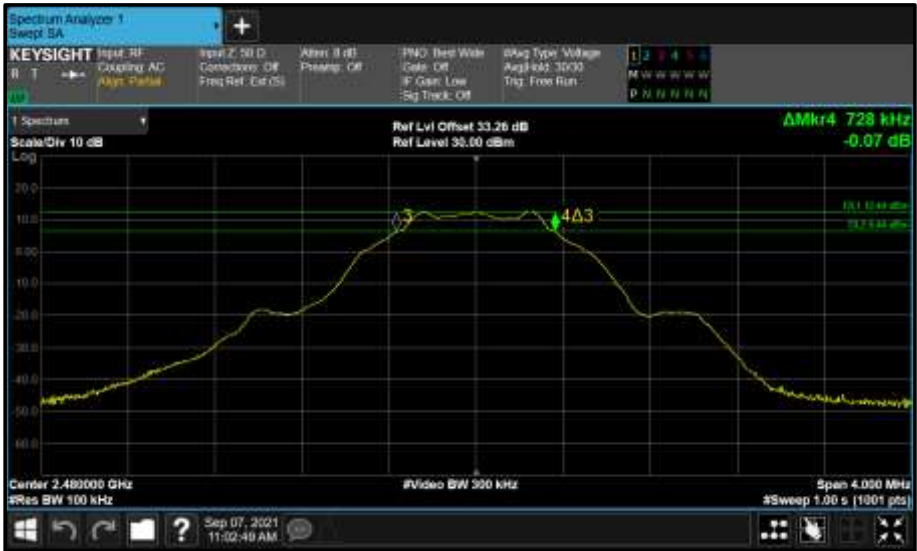
Figure 82 - Core 1 (B) 2480 MHz (CH39) 6 dB Bandwidth
