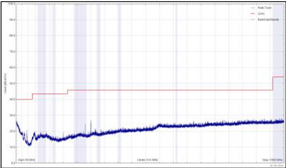
Figure 222 - 2440 MHz (CH17), LE1M, iPA, Core 0 + Core 1, 30 MHz to 1 GHz, Vertical (Peak)
