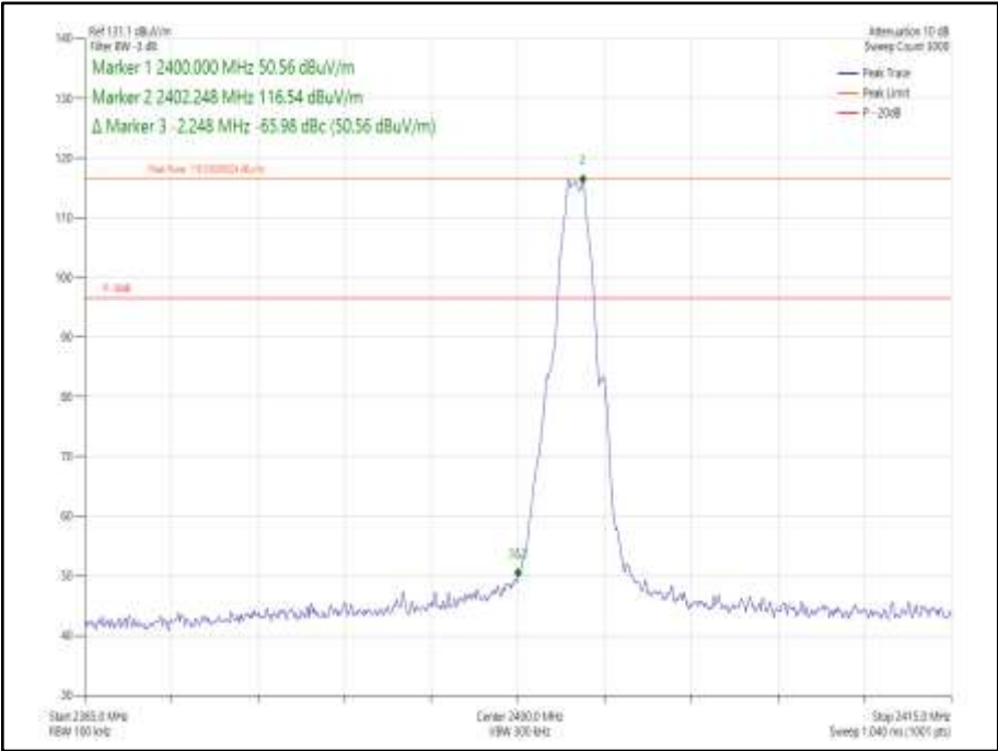
Figure 234 - GFSK/DH1- 2402 MHz – Band Edge Frequency 2400.0 MHz
