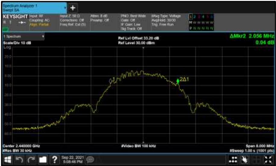
Figure 107 - Core 1 (B) 2440 MHz (CH17) 99% Bandwidth
