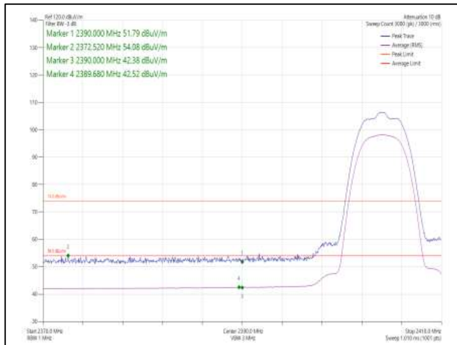
Figure 31 - Static - GFSK/4DH5 - 2404 MHz - Band Edge Frequency 2390.0 MHz
