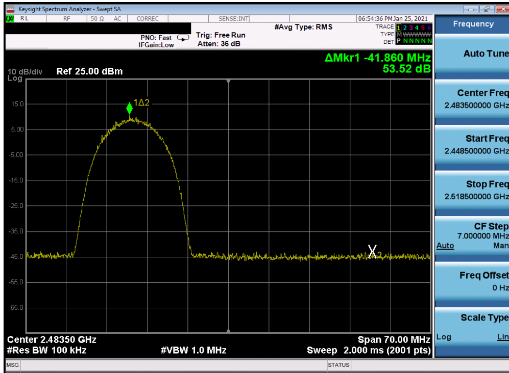
Plot 7-296. Band Edge Plot Antenna 2a (802.11b – Ch. 12) – 11Mbps
