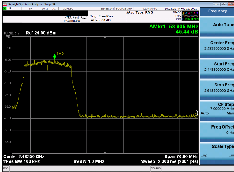
Plot 7-211. Band Edge Plot Antenna 4a (802.11n (2.4GHz) - Ch. 11) - MCS3
