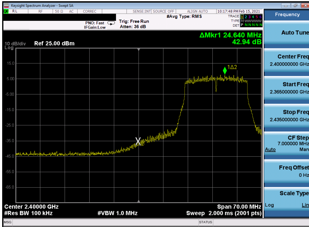
Plot 7-235. Band Edge Plot Antenna 4a (802.11n (2.4GHz) – Ch. 3) – MCS7
