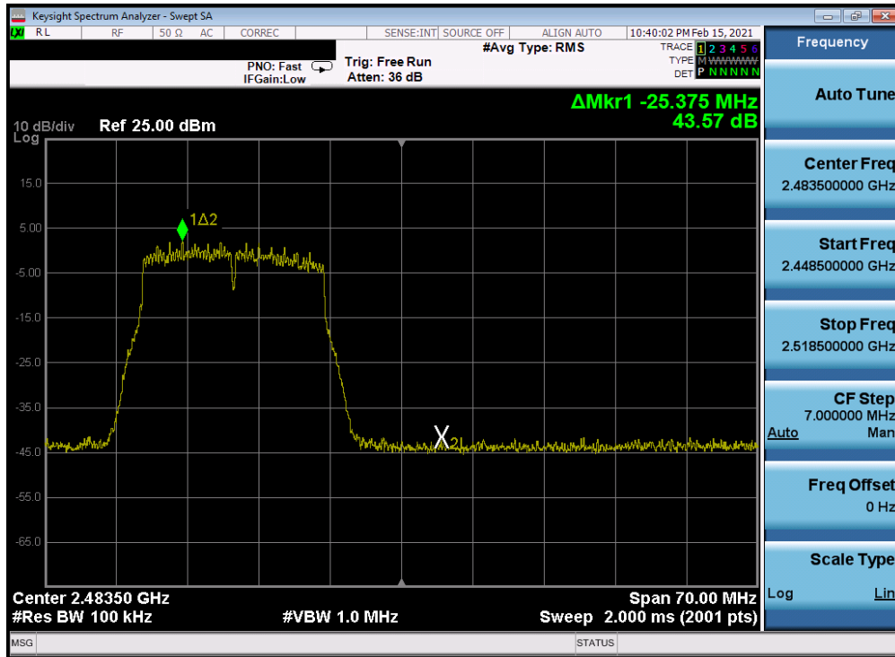
Plot 7-239. Band Edge Plot Antenna 4a (802.11n (2.4GHz) - Ch. 12) - MCS7
