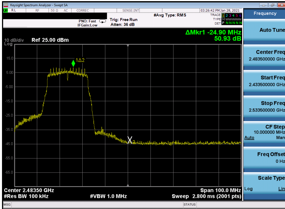
Plot 7-260. Band Edge Plot Antenna 2a (802.11n (2.4GHz) - Ch. 10) - MCS0
