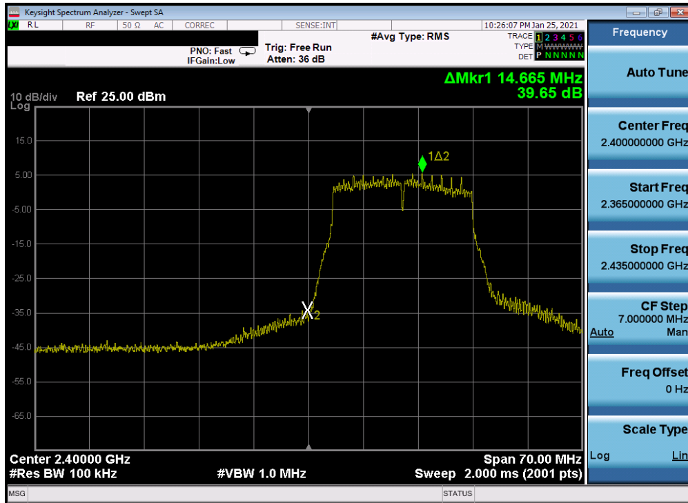
Plot 7-279. Band Edge Plot Antenna 2a (802.11n (2.4GHz) – Ch. 1) – MCS3
