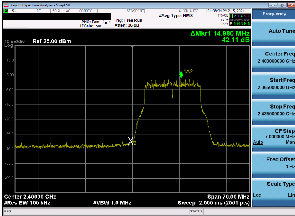
Plot 7-225. Band Edge Plot Antenna 4a (802.11g– Ch. 1) – 54Mbps
