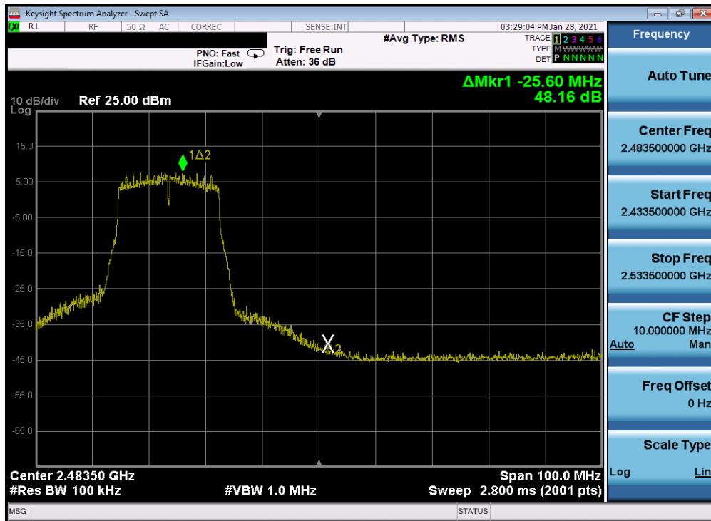
Plot 7-283. Band Edge Plot Antenna 2a (802.11n (2.4GHz) - Ch. 10) - MCS3
