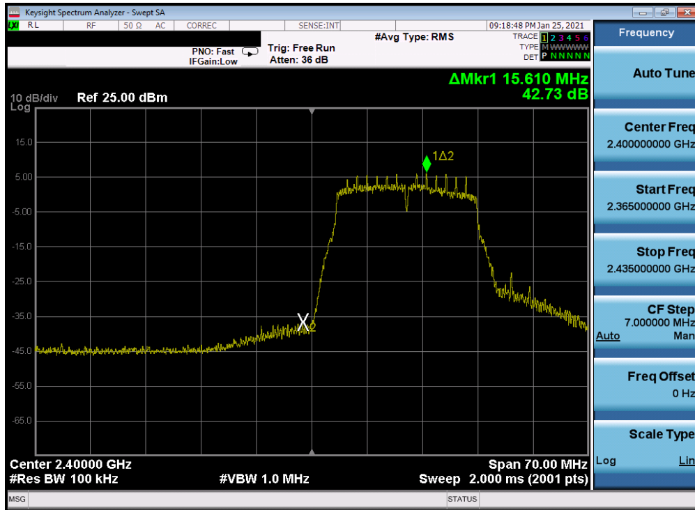
Plot 7-256. Band Edge Plot Antenna 2a (802.11n (2.4GHz) - Ch. 1) - MCS0
