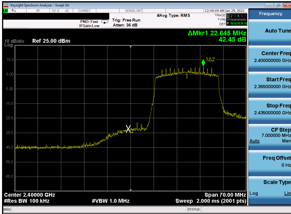
Plot 7-266. Band Edge Plot Antenna 2a (802.11ax (SU - 2.4GHz) – Ch. 3) – MCS0
