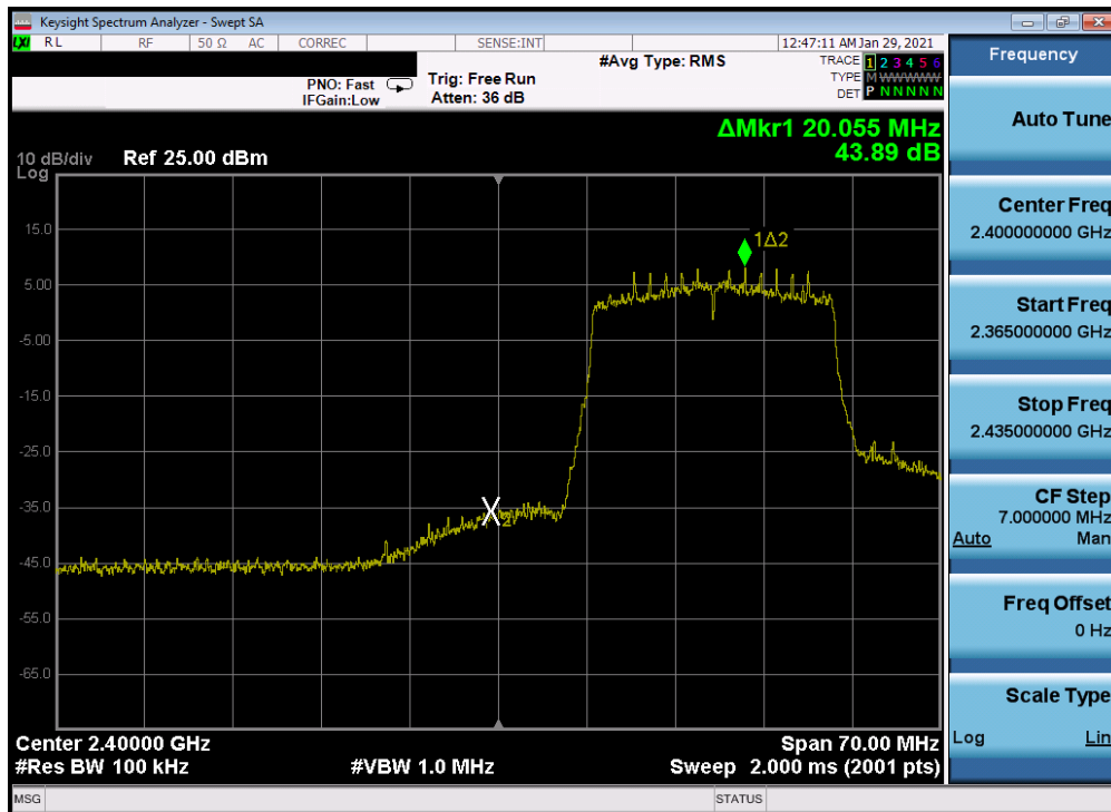
Plot 7-265. Band Edge Plot Antenna 2a (802.11ax (SU - 2.4GHz) – Ch. 2) – MCS0
