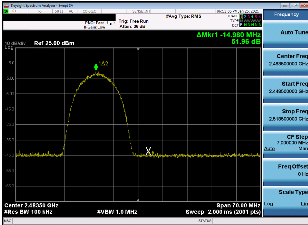
Plot 7-297. Band Edge Plot Antenna 2a (802.11b – Ch. 13) – 11Mbps
