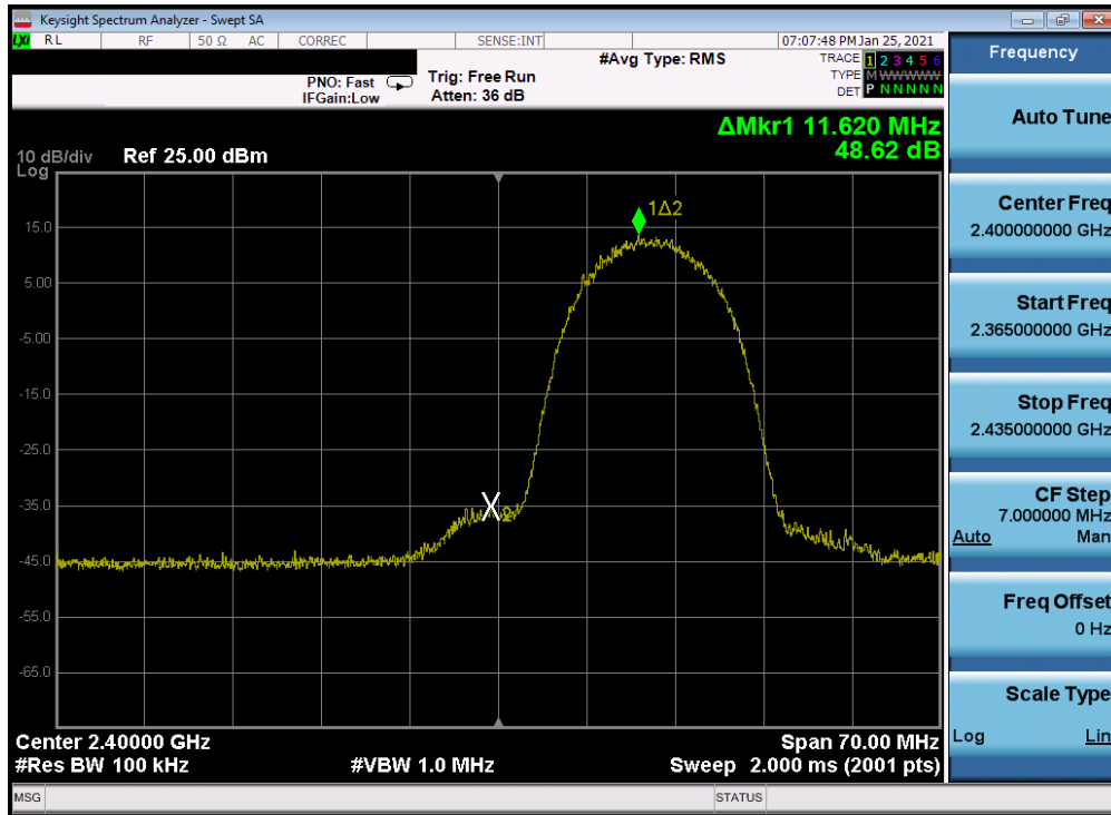
Plot 7-294. Band Edge Plot Antenna 2a (802.11b – Ch. 1) – 11Mbps
