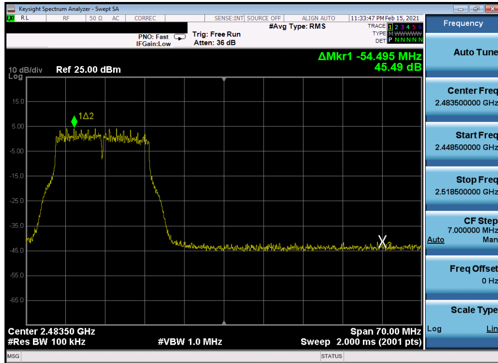
Plot 7-303. Band Edge Plot Antenna 2a (802.11g – Ch. 11) – 54Mbps
