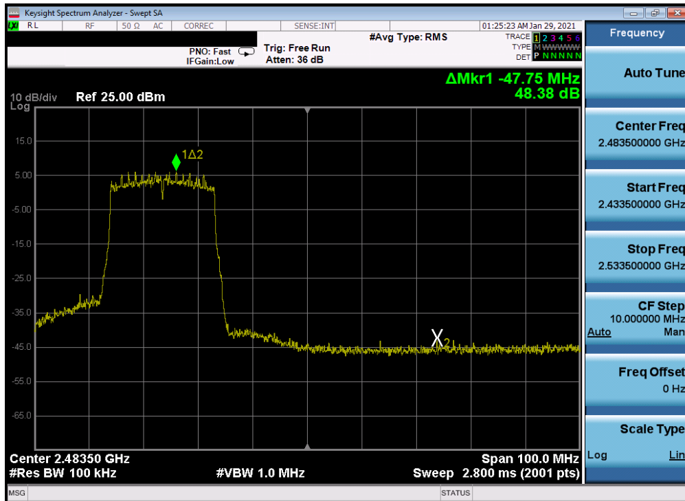
Plot 7-291. Band Edge Plot Antenna 2a (802.11ax (SU - 2.4GHz) – Ch. 10) – MCS3
