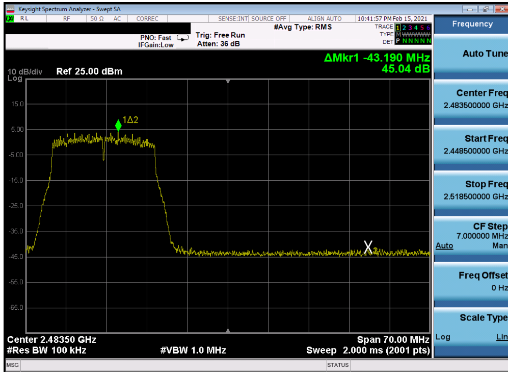
Plot 7-238. Band Edge Plot Antenna 4a (802.11n (2.4GHz) - Ch. 11) - MCS7
