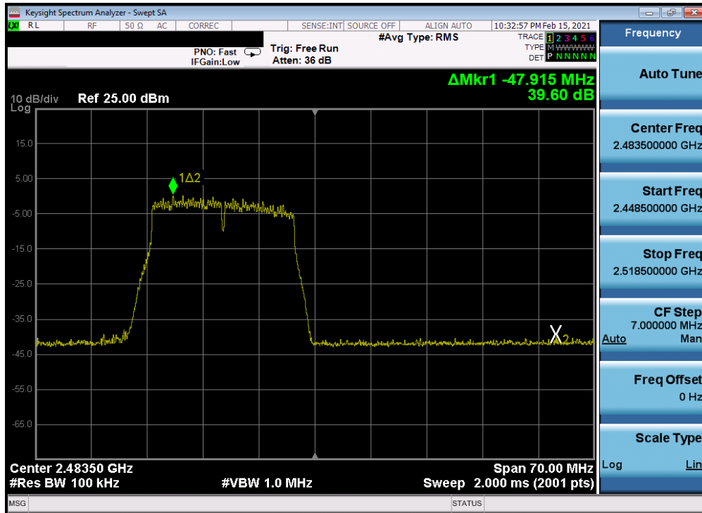
Plot 7-240. Band Edge Plot Antenna 4a (802.11n (2.4GHz) - Ch. 13) - MCS7
