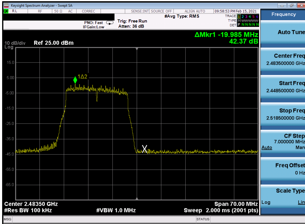
Plot 7-213. Band Edge Plot Antenna 4a (802.11n (2.4GHz) – Ch. 13) – MCS3
