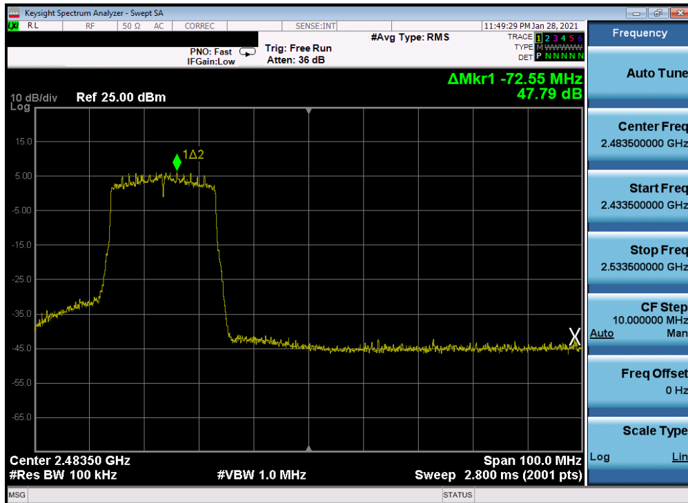
Plot 7-218. Band Edge Plot Antenna 4a (802.11ax (SU - 2.4GHz) – Ch. 10) – MCS3
