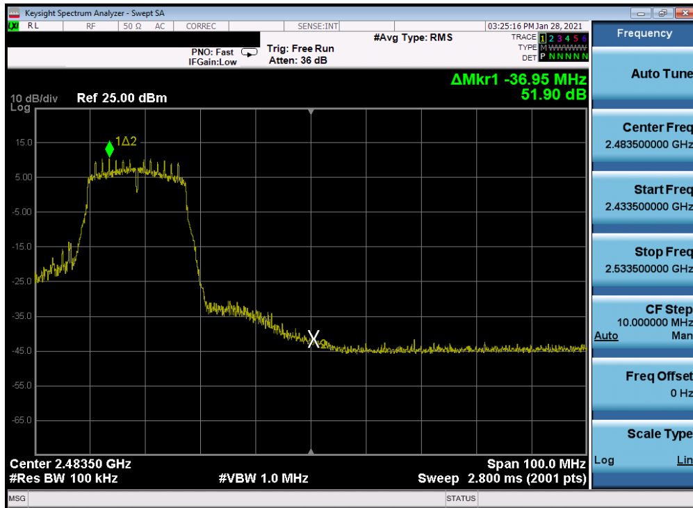
Plot 7-259. Band Edge Plot Antenna 2a (802.11n (2.4GHz) – Ch. 9) – MCS0
