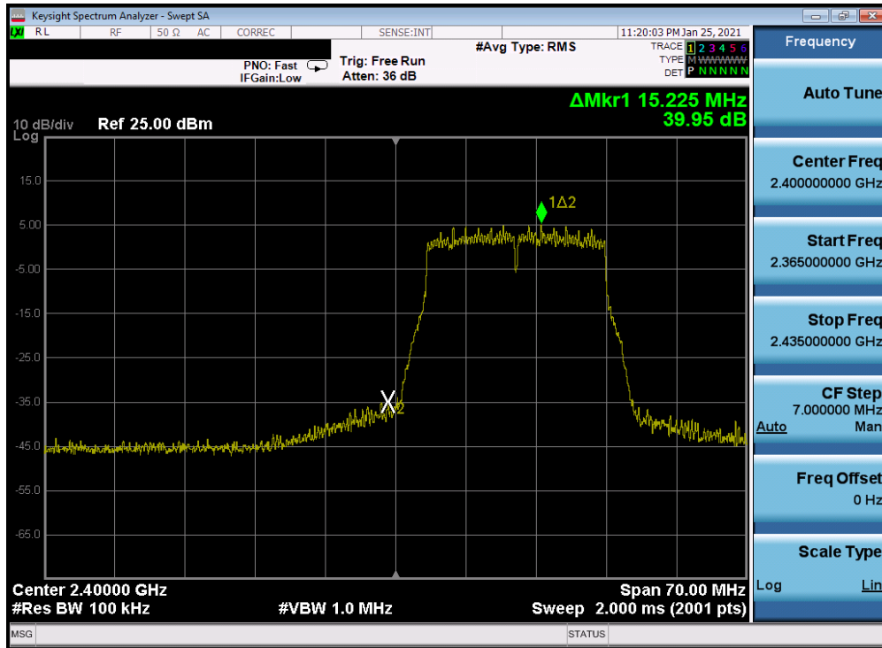
Plot 7-306. Band Edge Plot Antenna 2a (802.11n (2.4GHz) - Ch. 1) - MCS7
