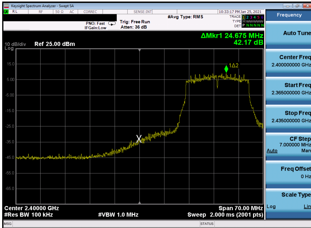
Plot 7-281. Band Edge Plot Antenna 2a (802.11n (2.4GHz) - Ch. 3) - MCS3
