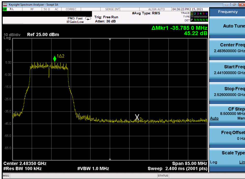
Plot 7-229. Band Edge Plot Antenna 4a (802.11g – Ch. 10) – 54Mbps
