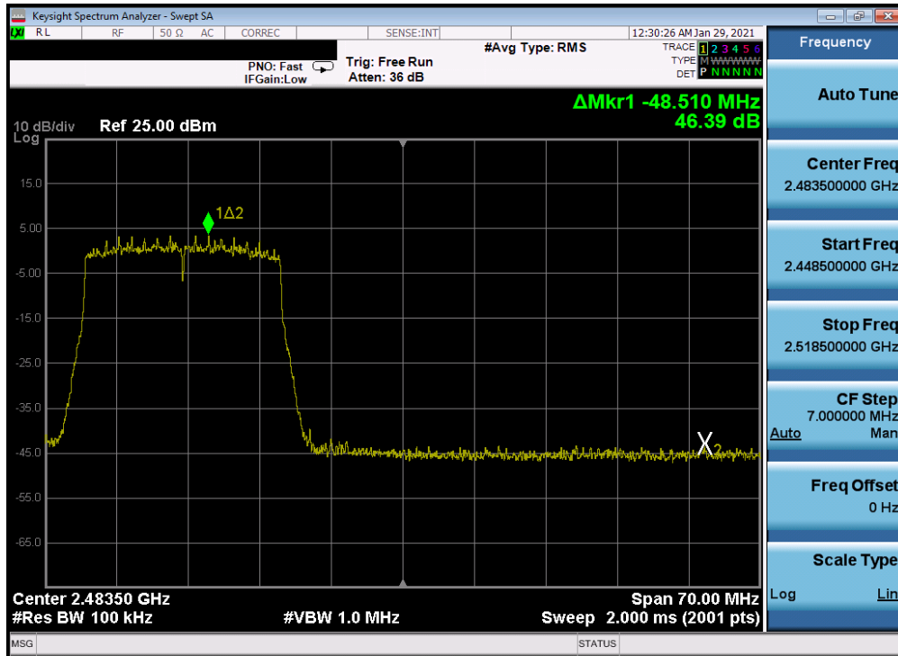
Plot 7-246. Band Edge Plot Antenna 4a (802.11ax (SU - 2.4GHz) – Ch. 11) – MCS5
