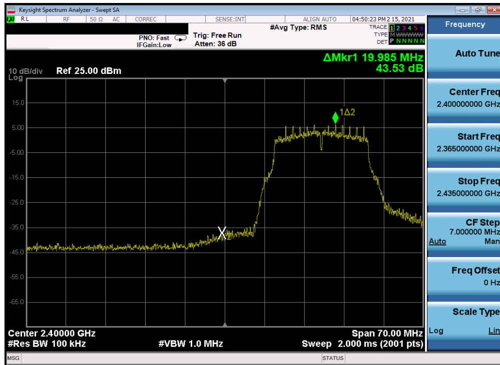
Plot 7-249. Band Edge Plot Antenna 2a (802.11g- Ch. 2) – 6Mbps
