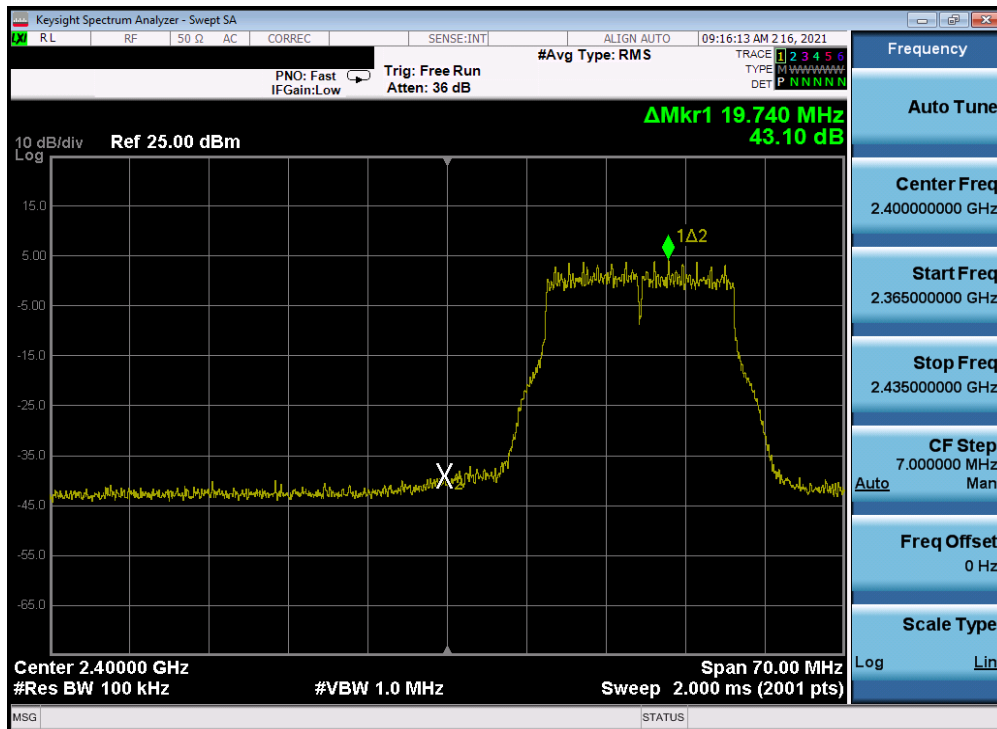
Plot 7-299. Band Edge Plot Antenna 2a (802.11g– Ch. 2) – 54Mbps
