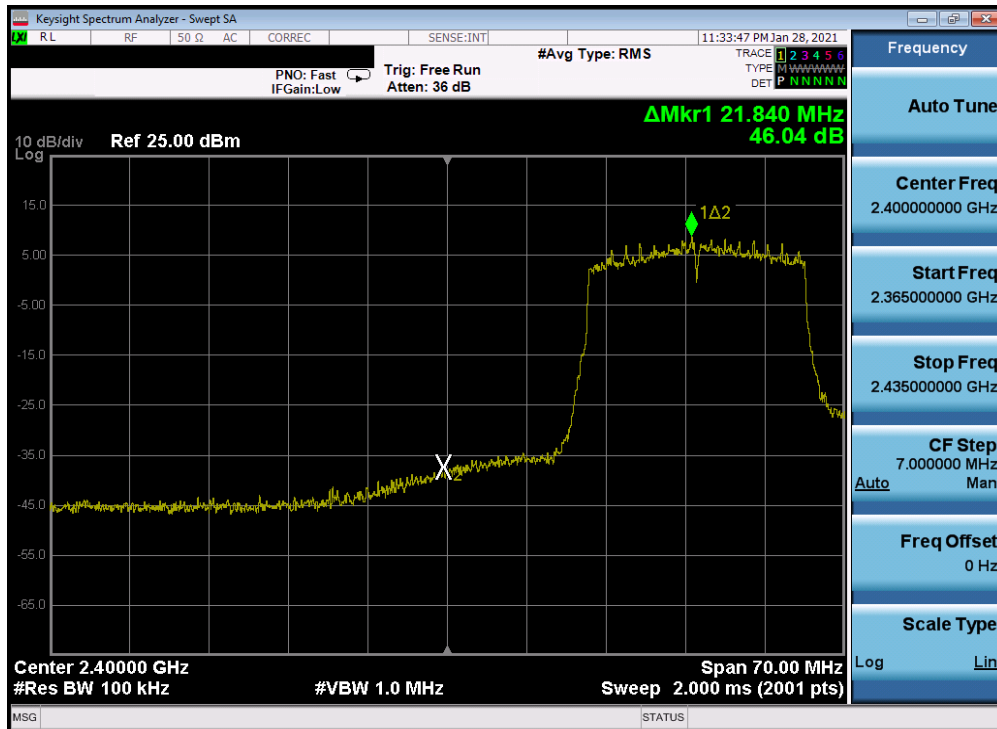
Plot 7-216. Band Edge Plot Antenna 4a (802.11ax (SU - 2.4GHz) – Ch. 3) – MCS3
