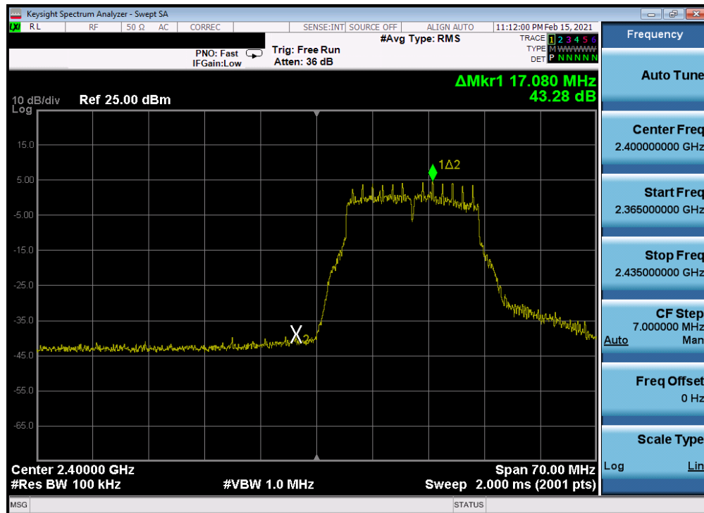
Plot 7-271. Band Edge Plot Antenna 2a (802.11g– Ch. 1) – 18Mbps
