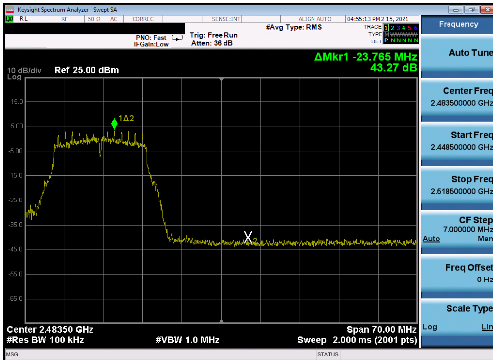
Plot 7-253. Band Edge Plot Antenna 2a (802.11g – Ch. 11) – 6Mbps
