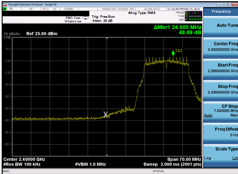
Plot 7-273. Band Edge Plot Antenna 2a (802.11g– Ch. 3) – 18Mbps
