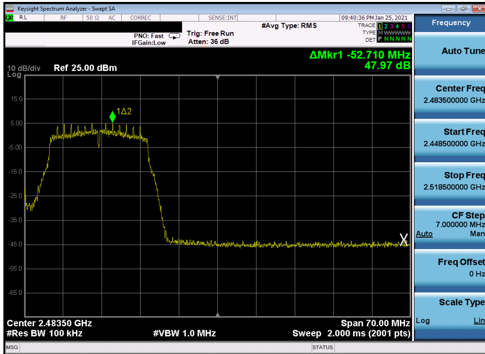
Plot 7-261. Band Edge Plot Antenna 2a (802.11n (2.4GHz) - Ch. 11) - MCS0
