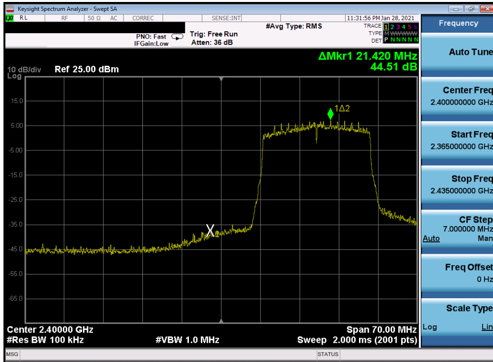
Plot 7-215. Band Edge Plot Antenna 4a (802.11ax (SU - 2.4GHz) – Ch. 2) – MCS3
