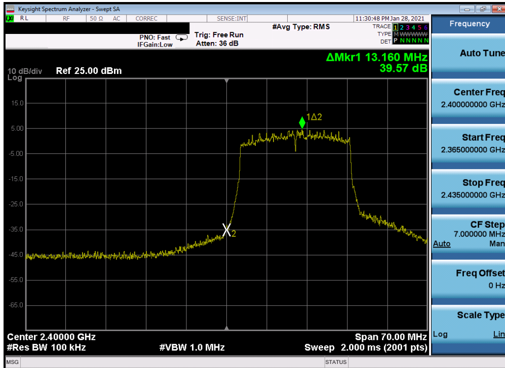
Plot 7-214. Band Edge Plot Antenna 4a (802.11ax (SU - 2.4GHz) – Ch. 1) – MCS3
