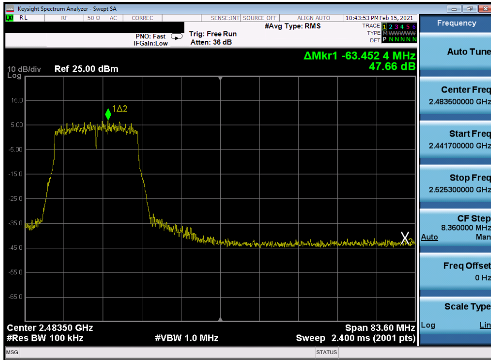
Plot 7-237. Band Edge Plot Antenna 4a (802.11n (2.4GHz) - Ch. 10) - MCS7
