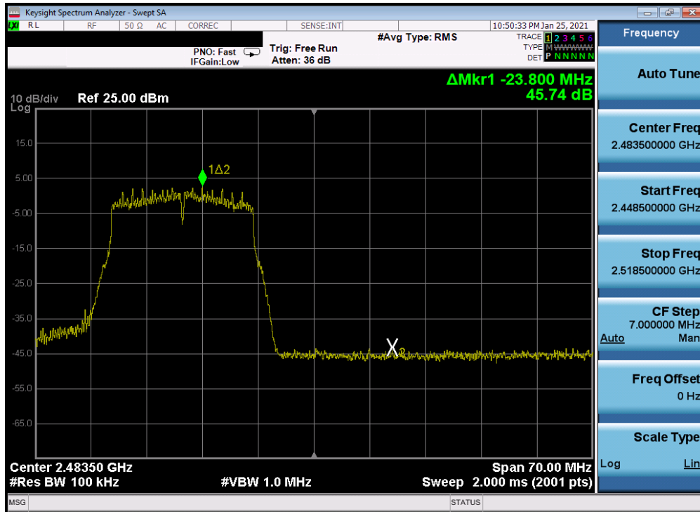
Plot 7-285. Band Edge Plot Antenna 2a (802.11n (2.4GHz) - Ch. 12) - MCS3
