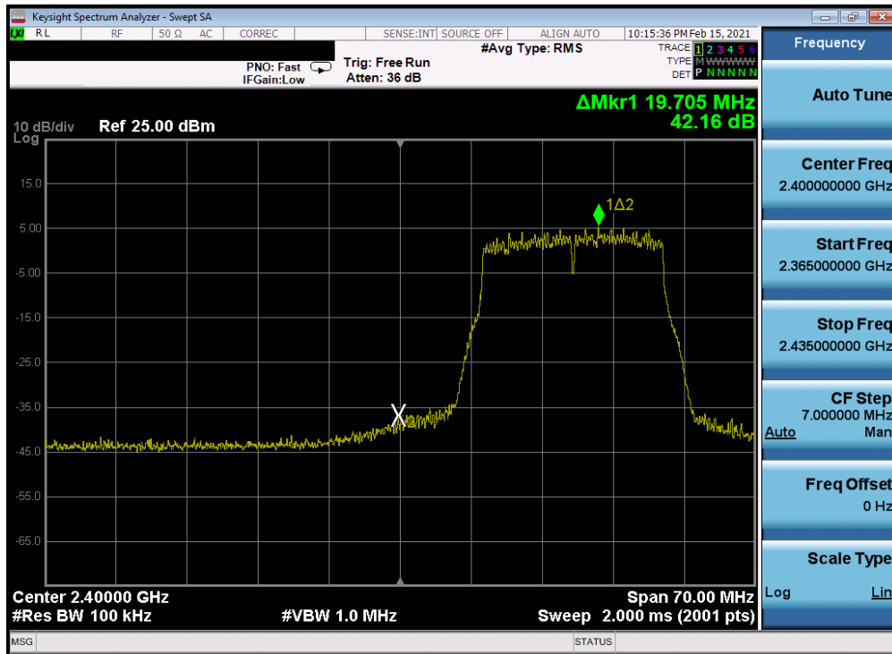
Plot 7-234. Band Edge Plot Antenna 4a (802.11n (2.4GHz) – Ch. 2) – MCS7
