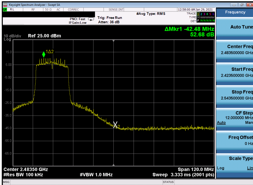
Plot 7-267. Band Edge Plot Antenna 2a (802.11ax (SU - 2.4GHz) – Ch. 9) – MCS0
