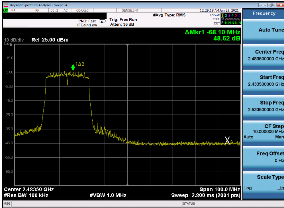
Plot 7-245. Band Edge Plot Antenna 4a (802.11ax (SU - 2.4GHz) – Ch. 10) – MCS5
