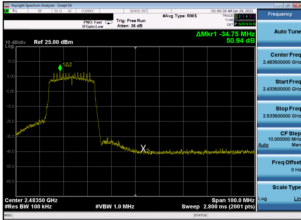
Plot 7-268. Band Edge Plot Antenna 2a (802.11ax (SU - 2.4GHz) – Ch. 10) – MCS0
