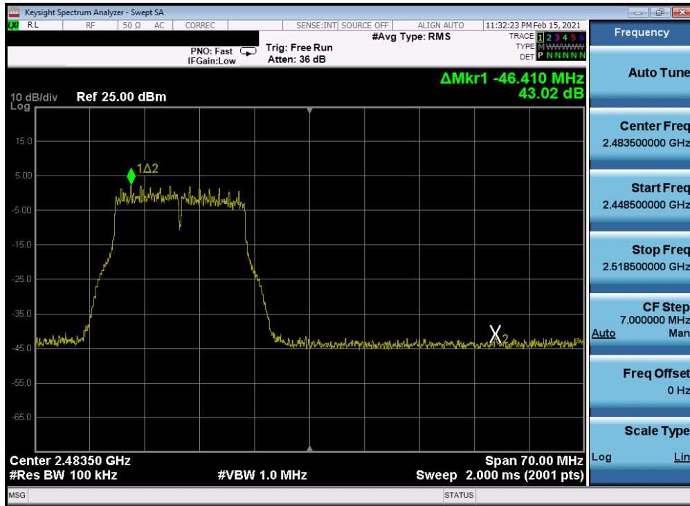
Plot 7-304. Band Edge Plot Antenna 2a (802.11g – Ch. 12) – 54Mbps
