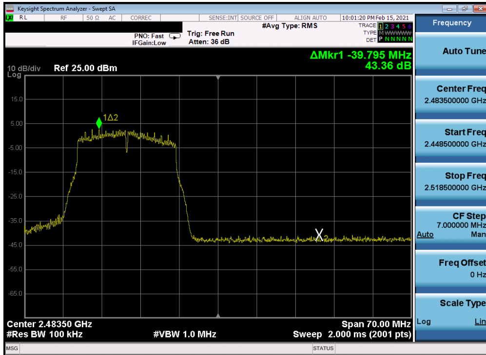
Plot 7-212. Band Edge Plot Antenna 4a (802.11n (2.4GHz) - Ch. 12) - MCS3
