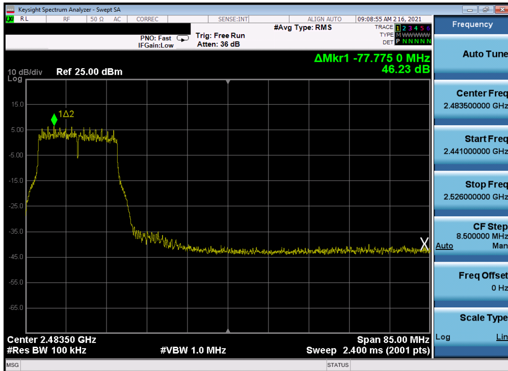
Plot 7-301. Band Edge Plot Antenna 2a (802.11g – Ch. 9) – 54Mbps
