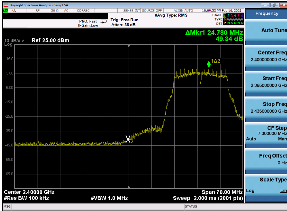
Plot 7-250. Band Edge Plot Antenna 2a (802.11g - Ch. 3) - 6Mbps
