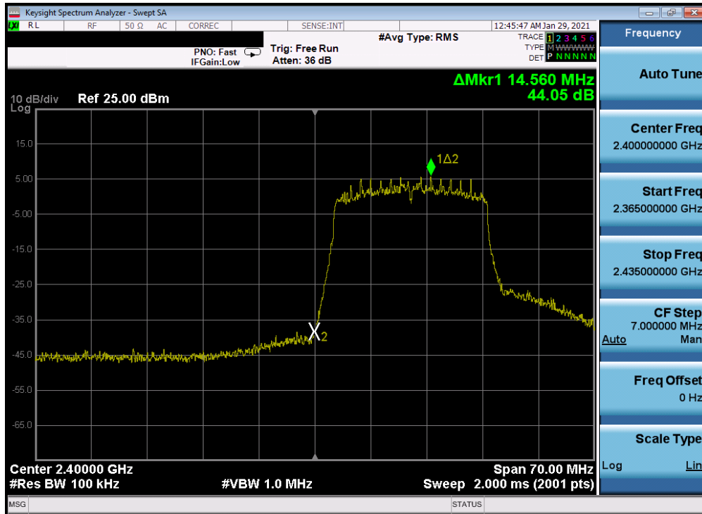
Plot 7-264. Band Edge Plot Antenna 2a (802.11ax (SU - 2.4GHz) – Ch. 1) – MCS0
