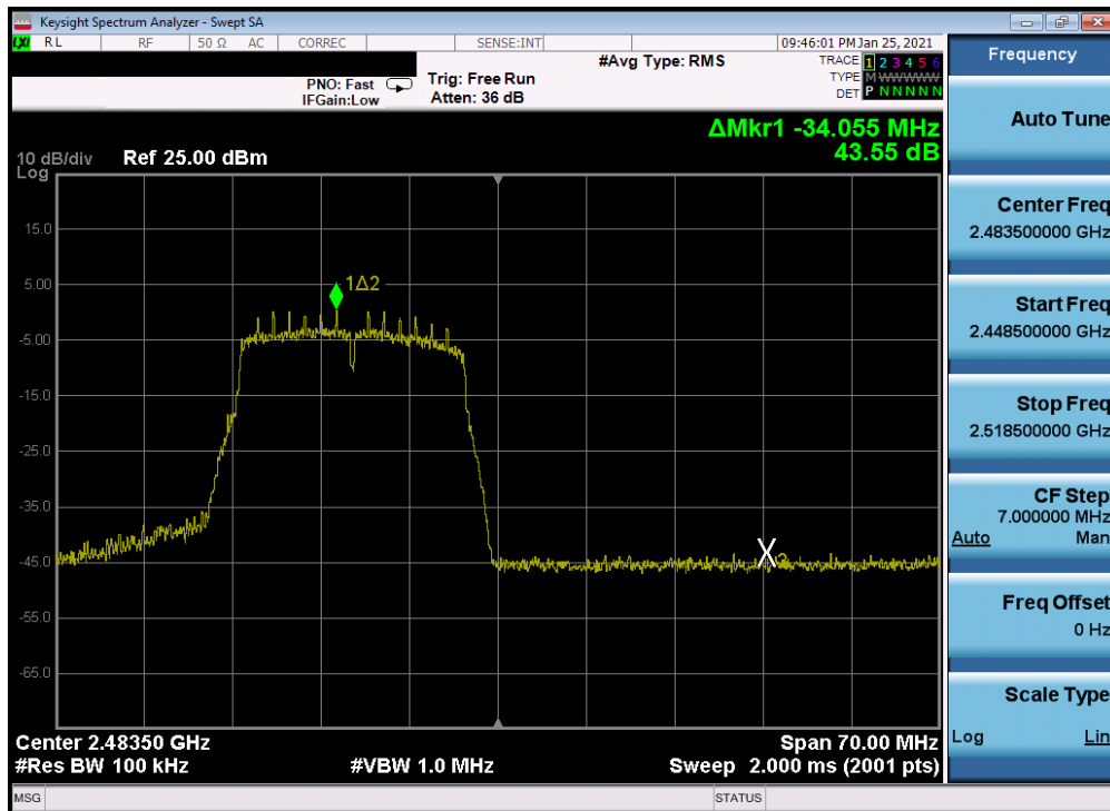
Plot 7-263. Band Edge Plot Antenna 2a (802.11n (2.4GHz) – Ch. 13) – MCS0
