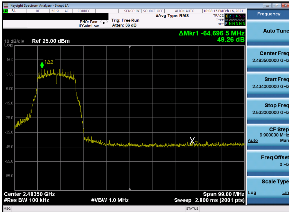
Plot 7-251. Band Edge Plot Antenna 2a (802.11g - Ch. 9) - 6Mbps
