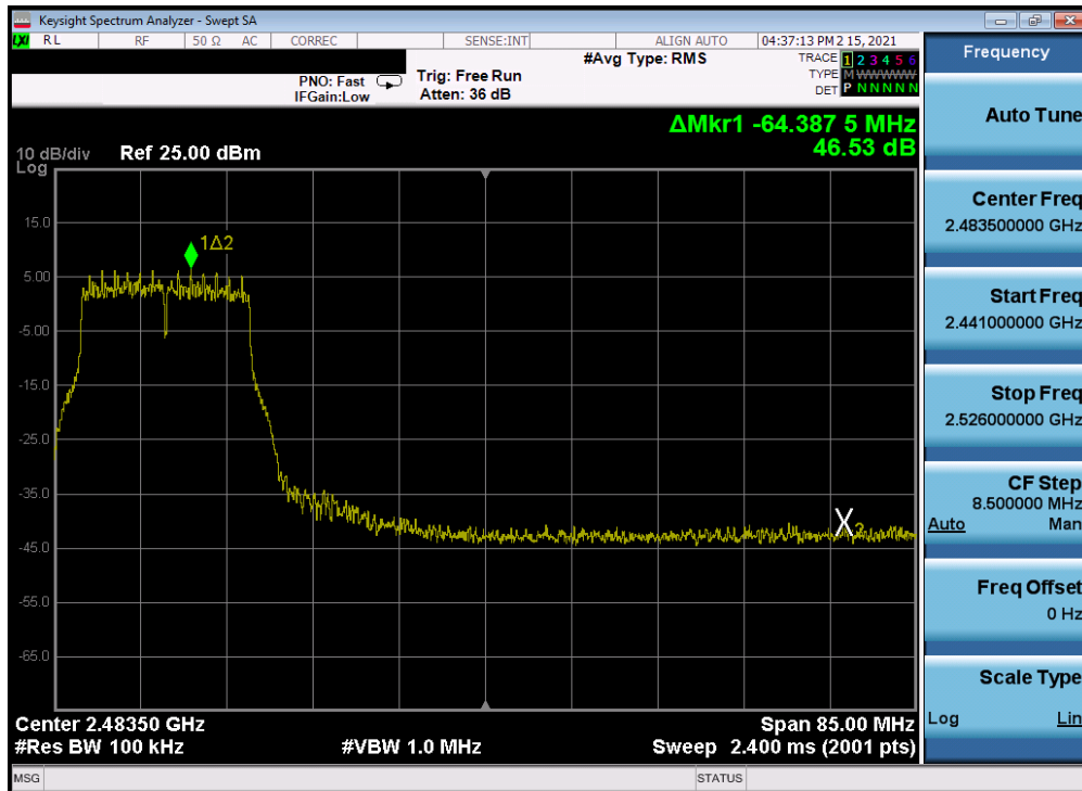
Plot 7-228. Band Edge Plot Antenna 4a (802.11g – Ch. 9) – 54Mbps
