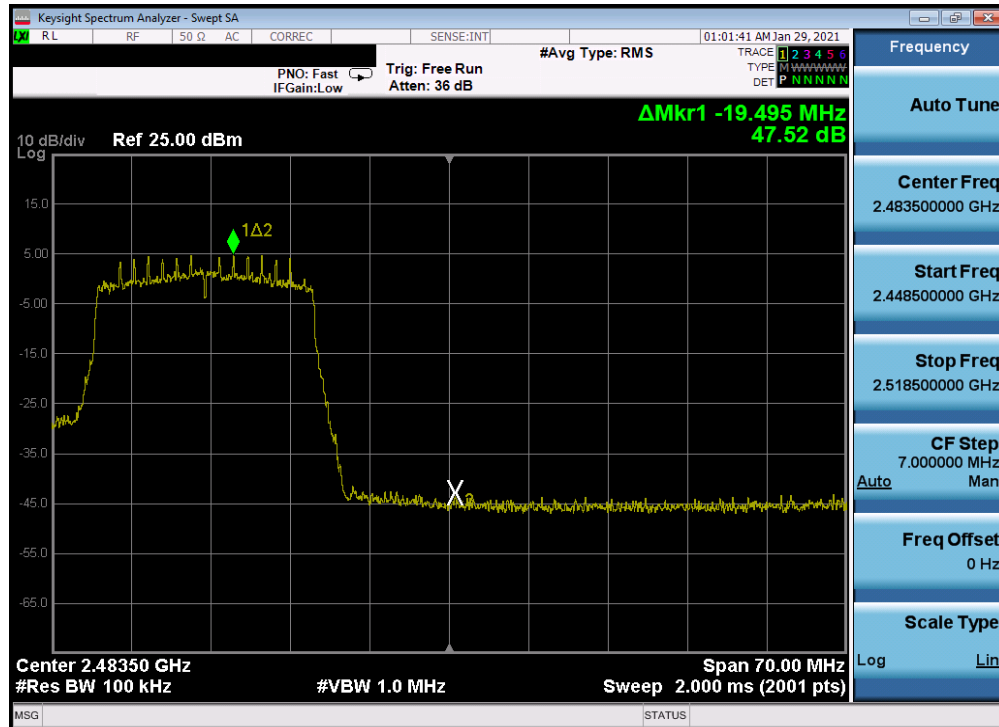
Plot 7-269. Band Edge Plot Antenna 2a (802.11ax (SU - 2.4GHz) – Ch. 11) – MCS0
