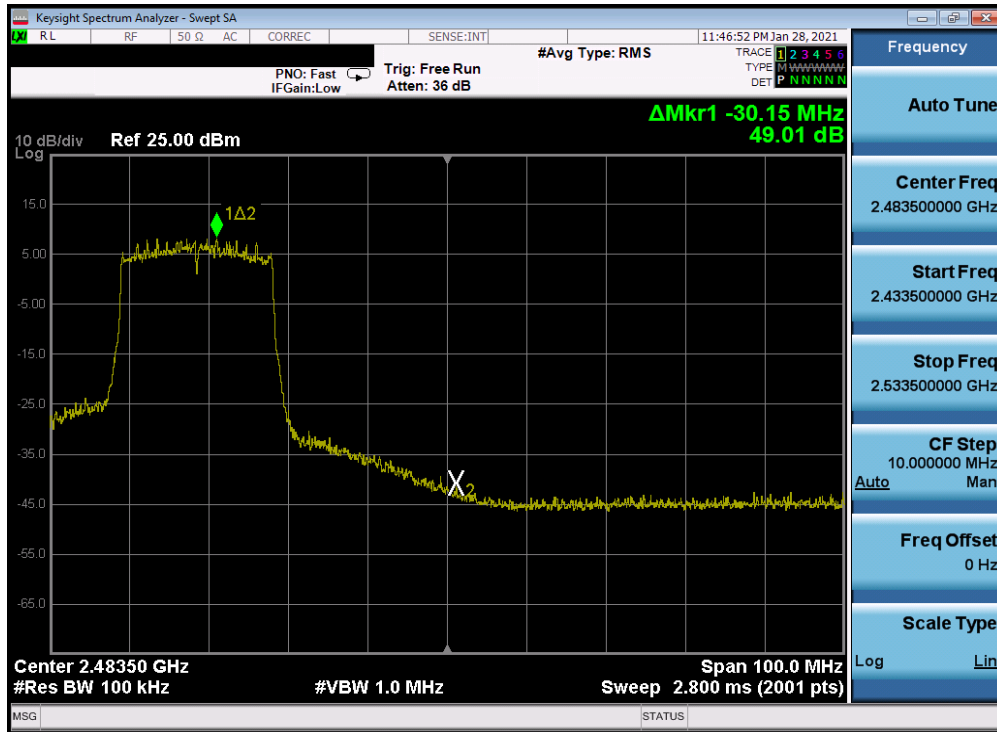
Plot 7-217. Band Edge Plot Antenna 4a (802.11ax (SU - 2.4GHz) – Ch. 9) – MCS3
