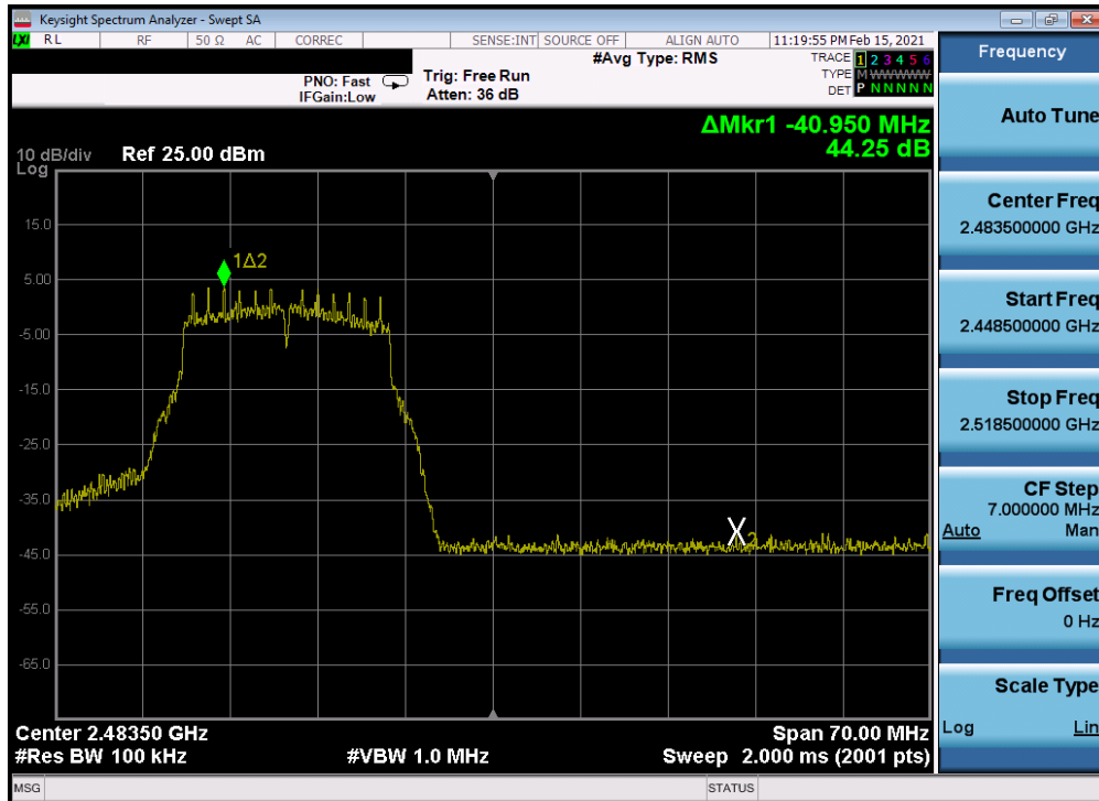
Plot 7-277. Band Edge Plot Antenna 2a (802.11g - Ch. 12) - 18Mbps
