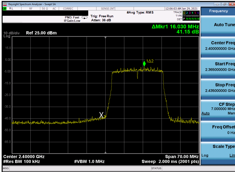
Plot 7-241. Band Edge Plot Antenna 4a (802.11ax (SU - 2.4GHz) – Ch. 1) – MCS5
