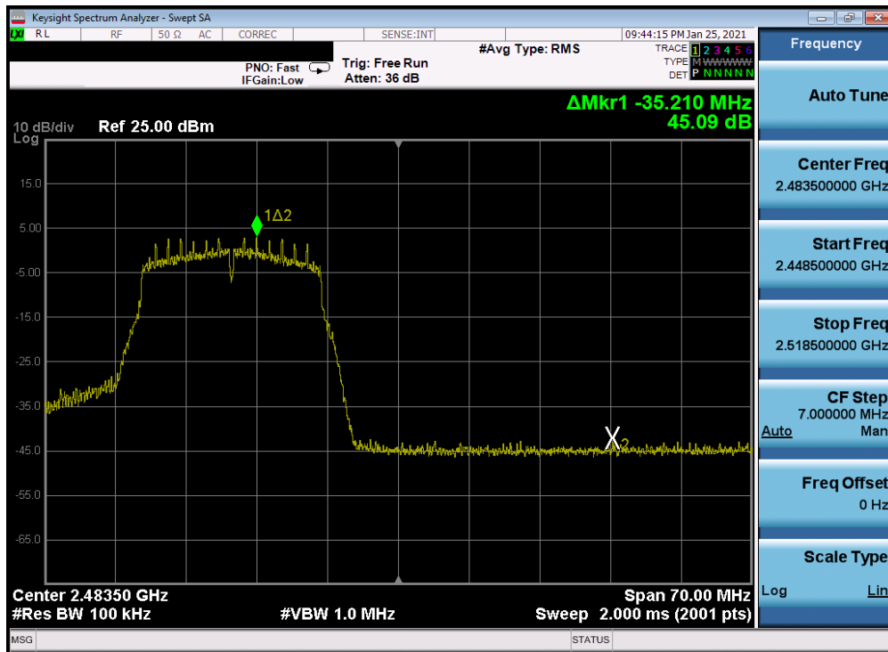
Plot 7-262. Band Edge Plot Antenna 2a (802.11n (2.4GHz) – Ch. 12) – MCS0
