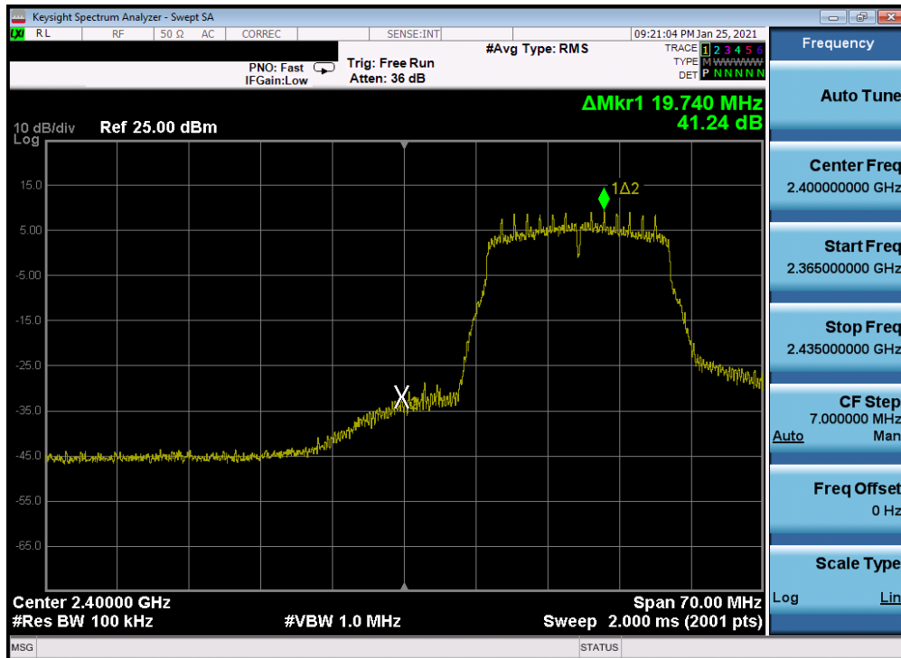
Plot 7-257. Band Edge Plot Antenna 2a (802.11n (2.4GHz) - Ch. 2) - MCS0
