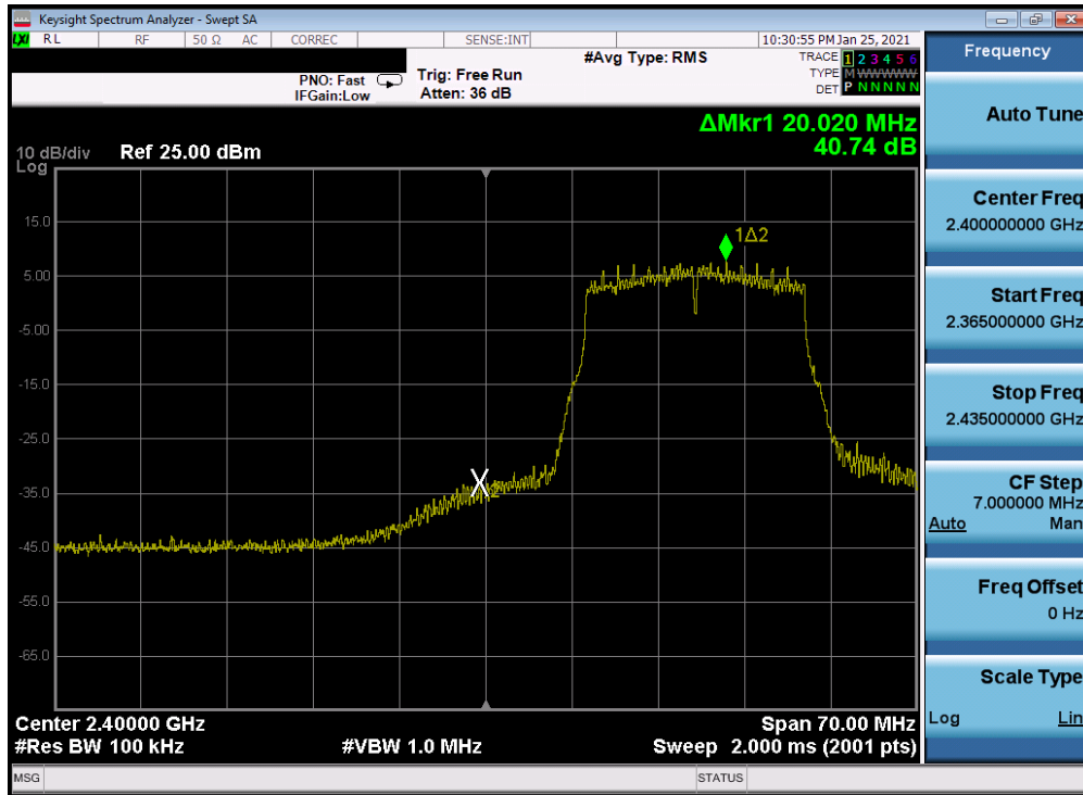
Plot 7-280. Band Edge Plot Antenna 2a (802.11n (2.4GHz) - Ch. 2) - MCS3
