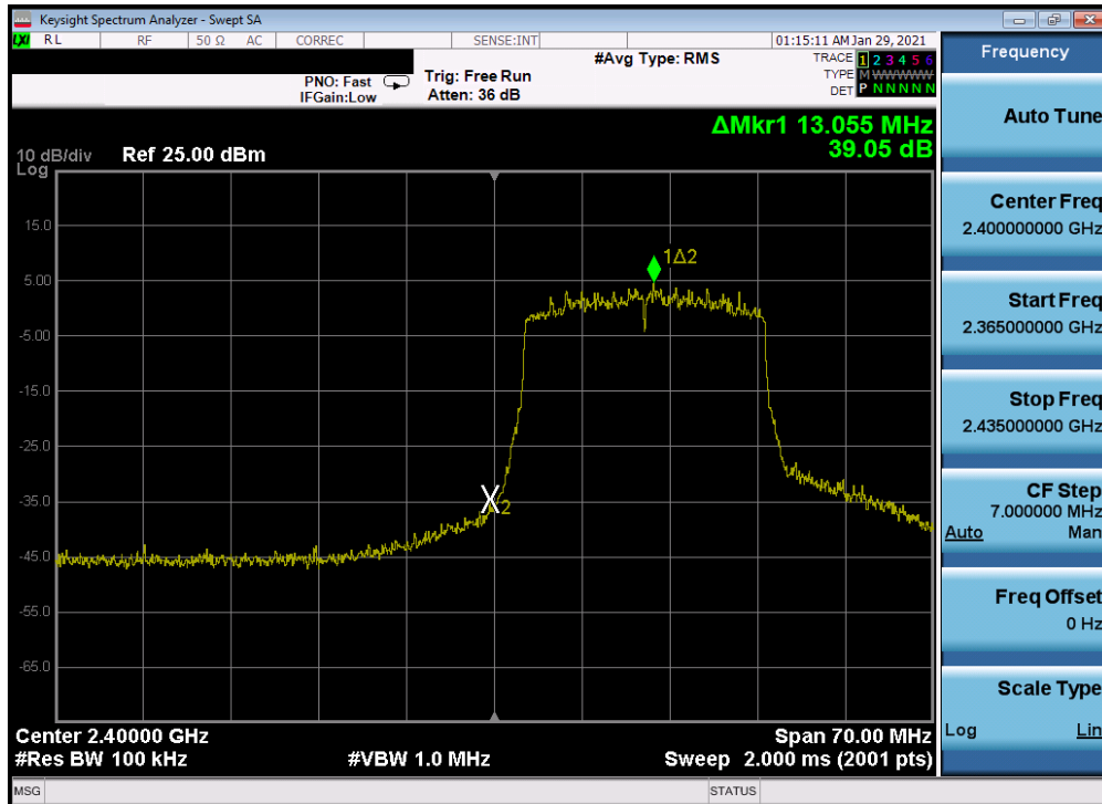
Plot 7-287. Band Edge Plot Antenna 2a (802.11ax (SU - 2.4GHz) - Ch. 1) - MCS3
