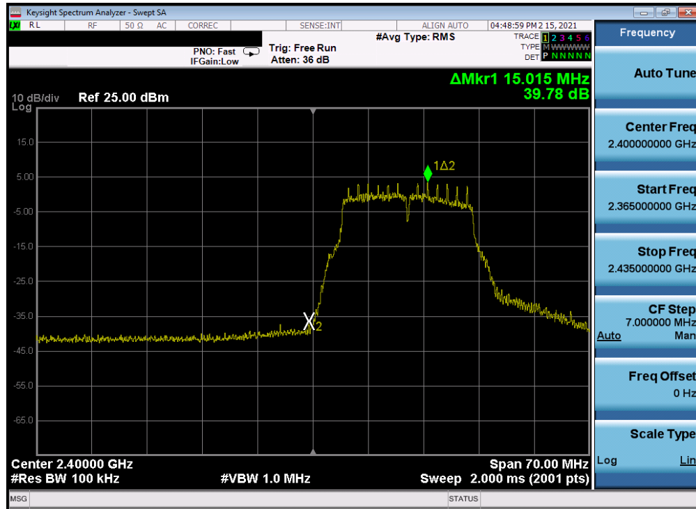
Plot 7-248. Band Edge Plot Antenna 2a (802.11g- Ch. 1) – 6Mbps
