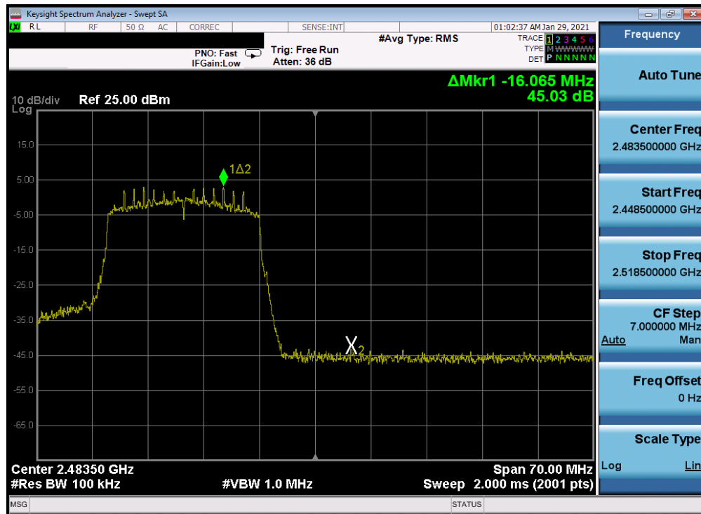
Plot 7-270. Band Edge Plot Antenna 2a (802.11ax (SU - 2.4GHz) – Ch. 12) – MCS0
