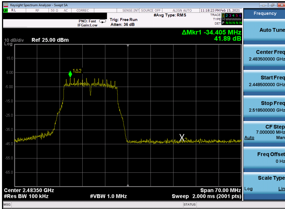
Plot 7-278. Band Edge Plot Antenna 2a (802.11g – Ch. 13) – 18Mbps
