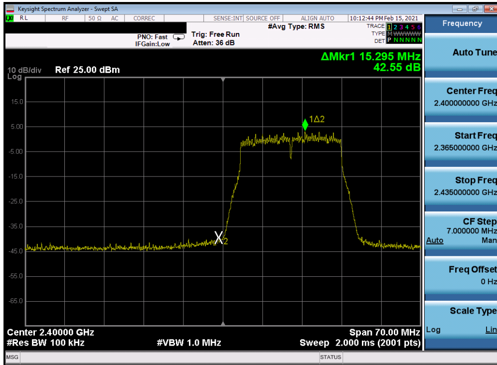
Plot 7-233. Band Edge Plot Antenna 4a (802.11n (2.4GHz) – Ch. 1) – MCS7
