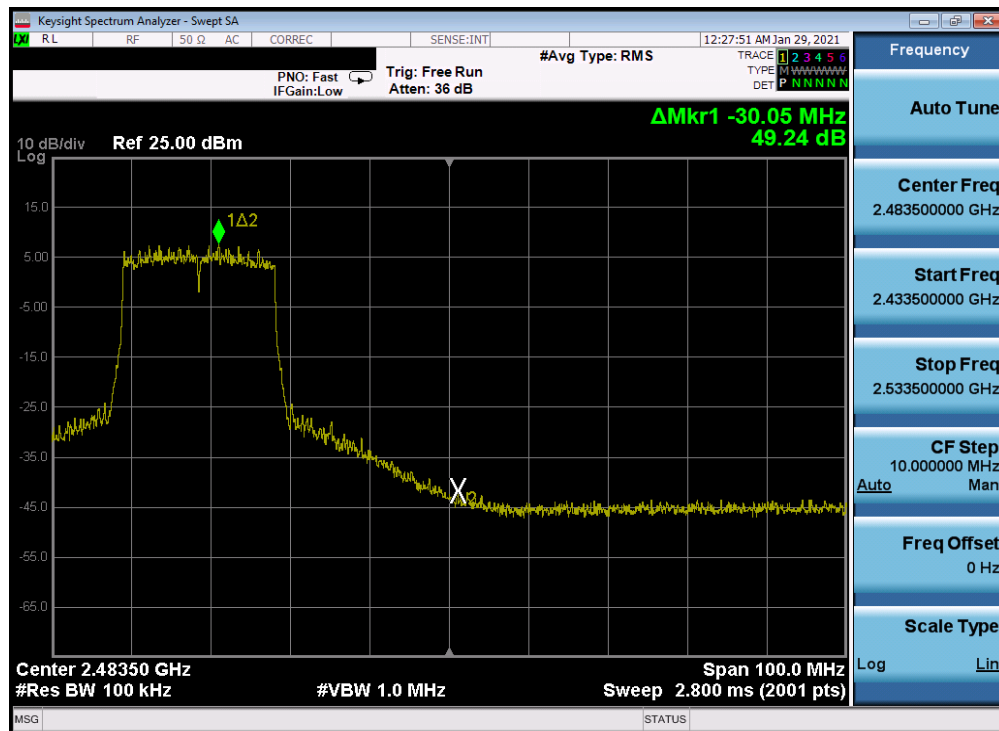
Plot 7-244. Band Edge Plot Antenna 4a (802.11ax (SU - 2.4GHz) – Ch. 9) – MCS5
