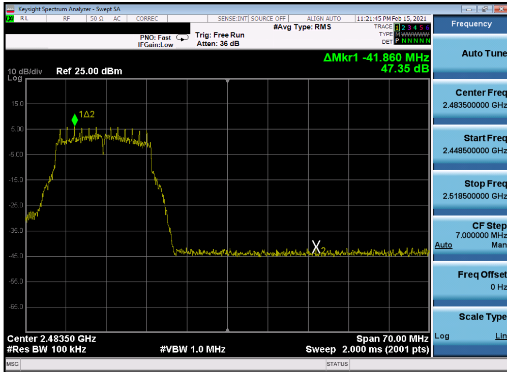
Plot 7-276. Band Edge Plot Antenna 2a (802.11g - Ch. 11) - 18Mbps
