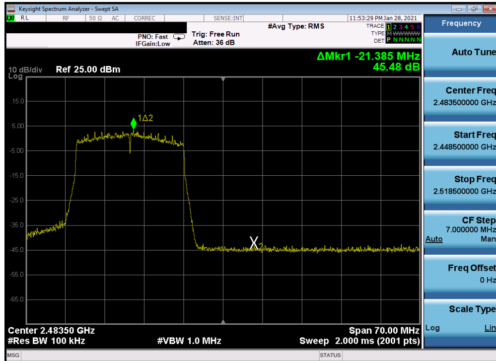
Plot 7-220. Band Edge Plot Antenna 4a (802.11ax (SU - 2.4GHz) – Ch. 12) – MCS3
