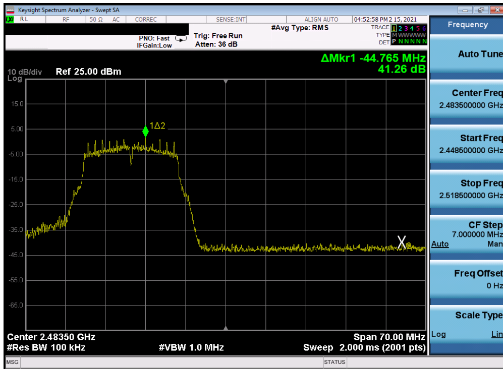
Plot 7-254. Band Edge Plot Antenna 2a (802.11g – Ch. 12) – 6Mbps
