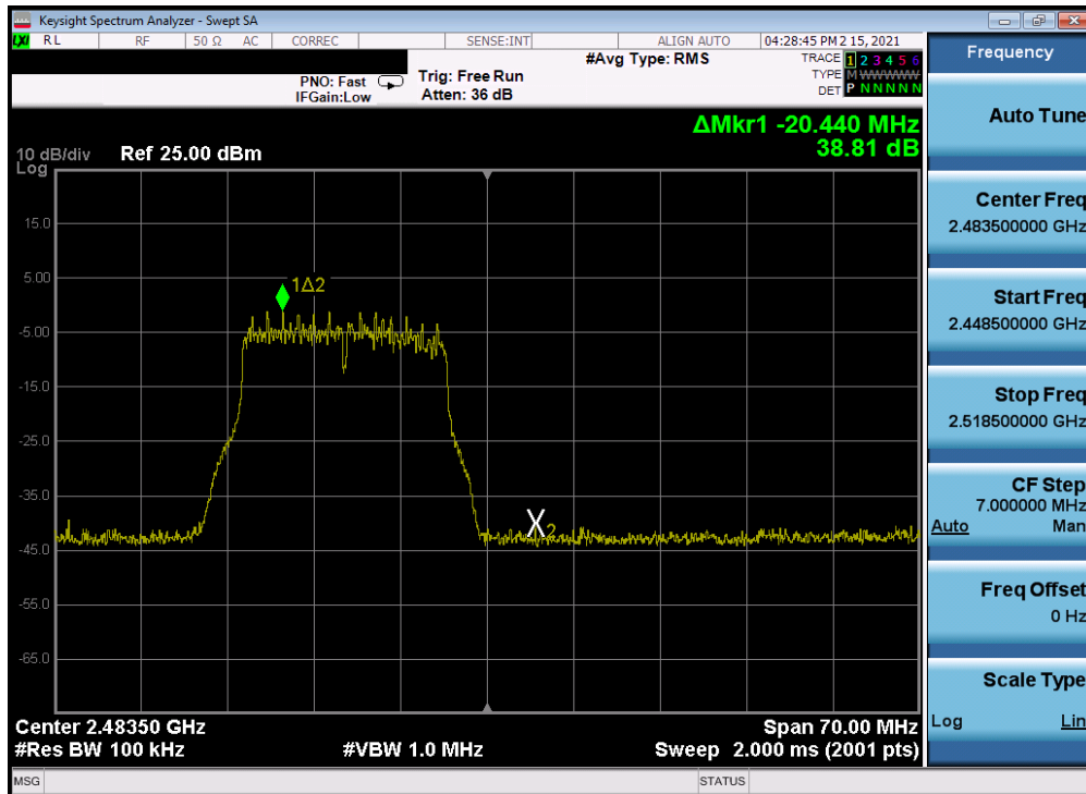
Plot 7-232. Band Edge Plot Antenna 4a (802.11g – Ch. 13) – 54Mbps
