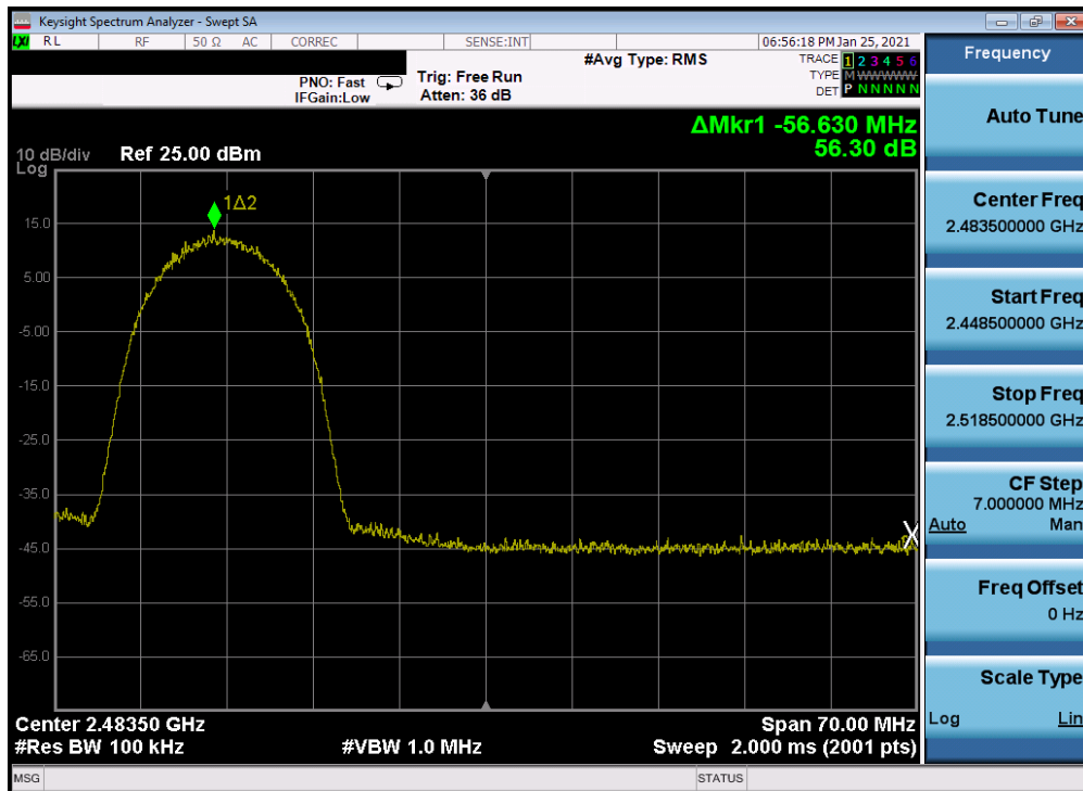
Plot 7-295. Band Edge Plot Antenna 2a (802.11b – Ch. 11) – 11Mbps
