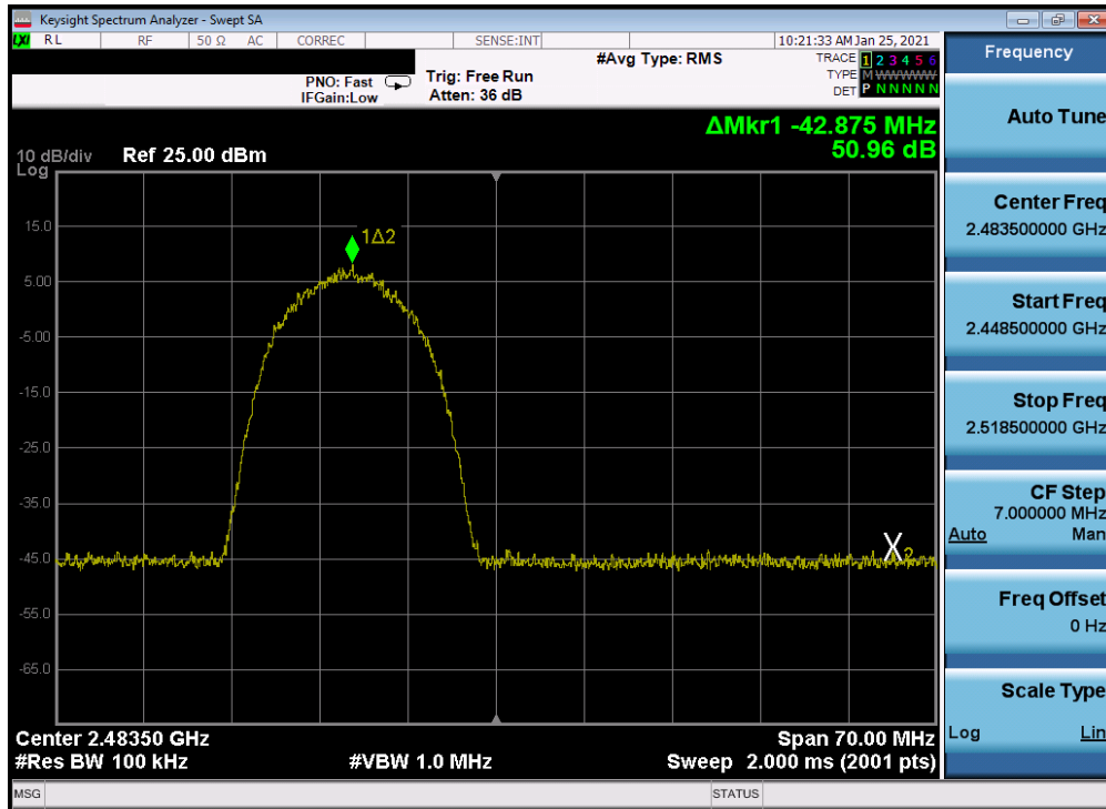
Plot 7-224. Band Edge Plot Antenna 4a (802.11b – Ch. 13) – 11Mbps
