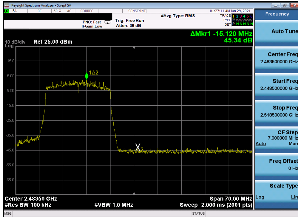
Plot 7-293. Band Edge Plot Antenna 2a (802.11ax (SU - 2.4GHz) – Ch. 12) – MCS3
