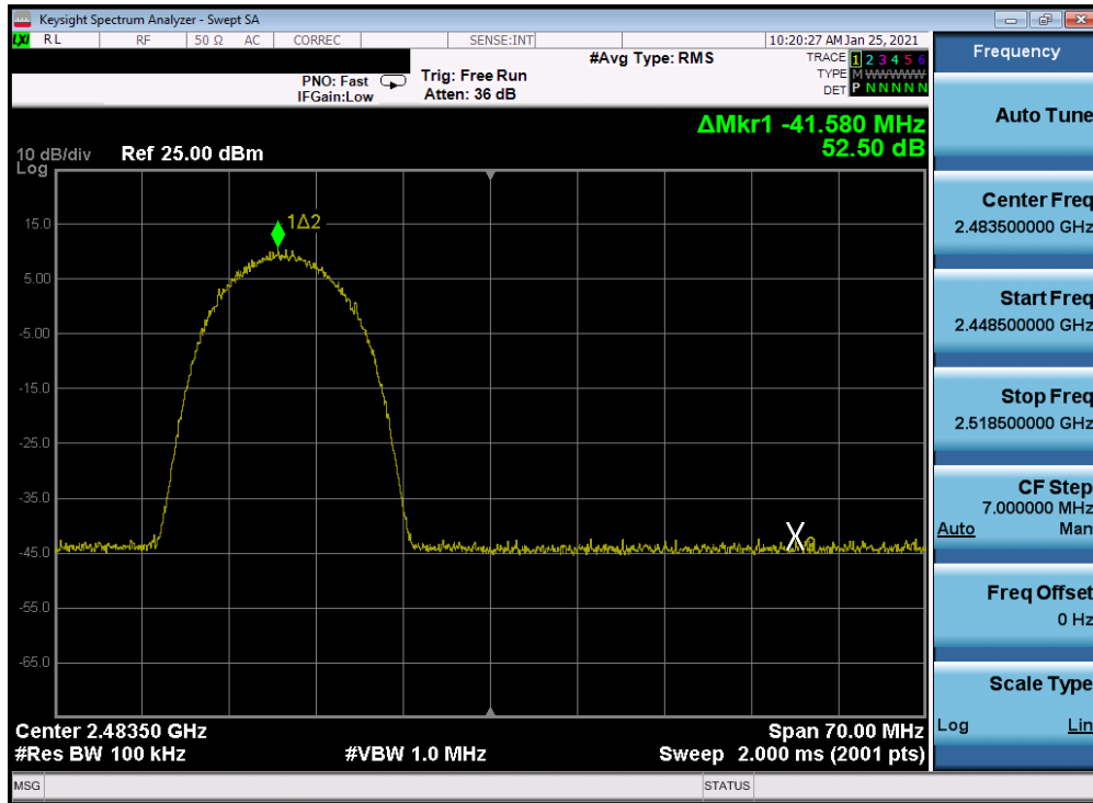
Plot 7-223. Band Edge Plot Antenna 4a (802.11b – Ch. 12) – 11Mbps
