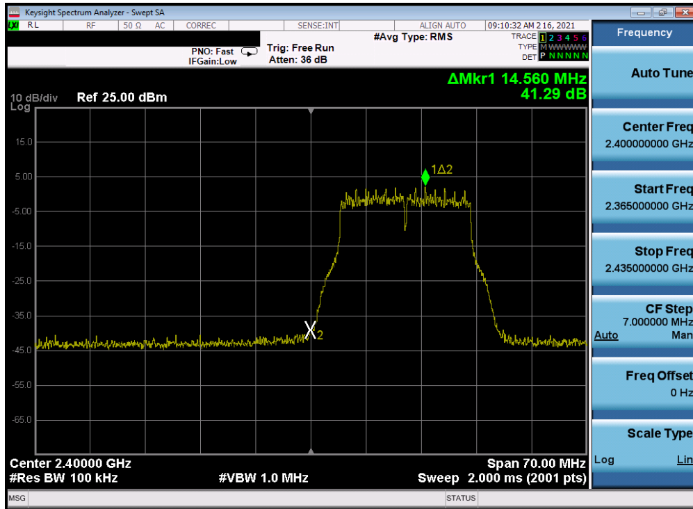
Plot 7-298. Band Edge Plot Antenna 2a (802.11g– Ch. 1) – 54Mbps
