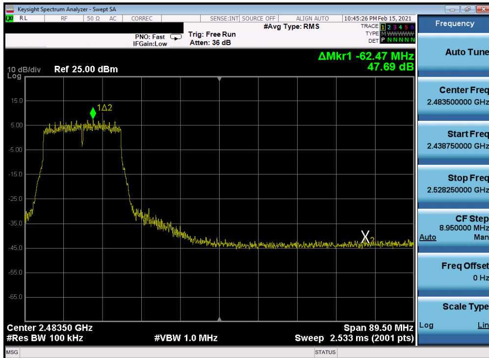
Plot 7-236. Band Edge Plot Antenna 4a (802.11n (2.4GHz) – Ch. 9) – MCS7
