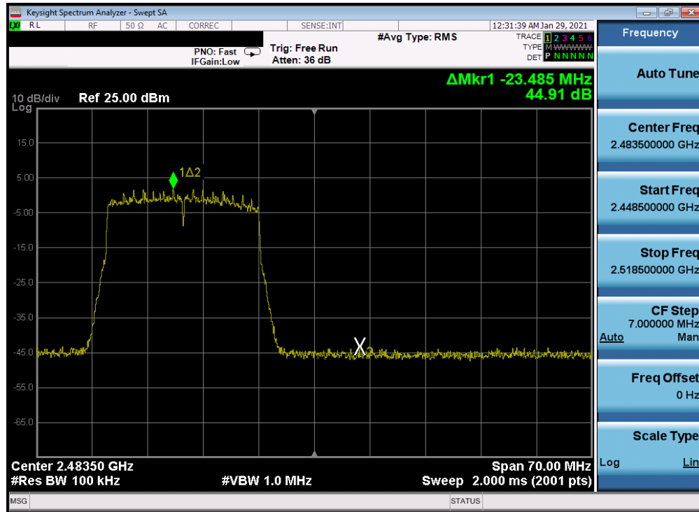
Plot 7-247. Band Edge Plot Antenna 4a (802.11ax (SU - 2.4GHz) – Ch. 12) – MCS5
