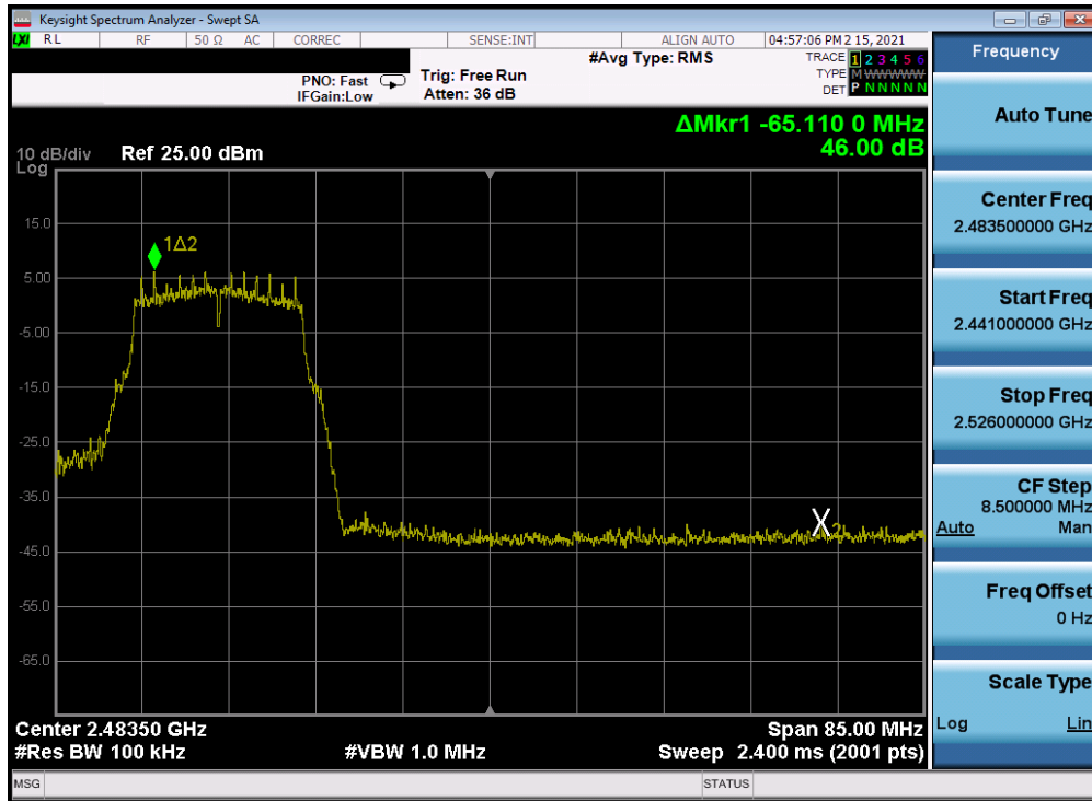
Plot 7-252. Band Edge Plot Antenna 2a (802.11g – Ch. 10) – 6Mbps
