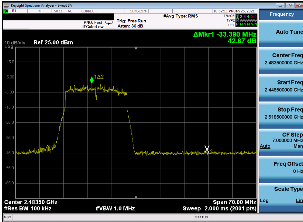
Plot 7-286. Band Edge Plot Antenna 2a (802.11n (2.4GHz) - Ch. 13) - MCS3
