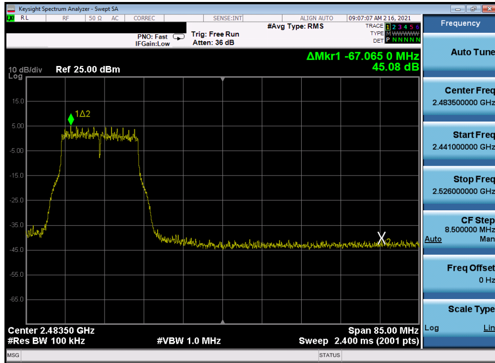
Plot 7-302. Band Edge Plot Antenna 2a (802.11g – Ch. 10) – 54Mbps
