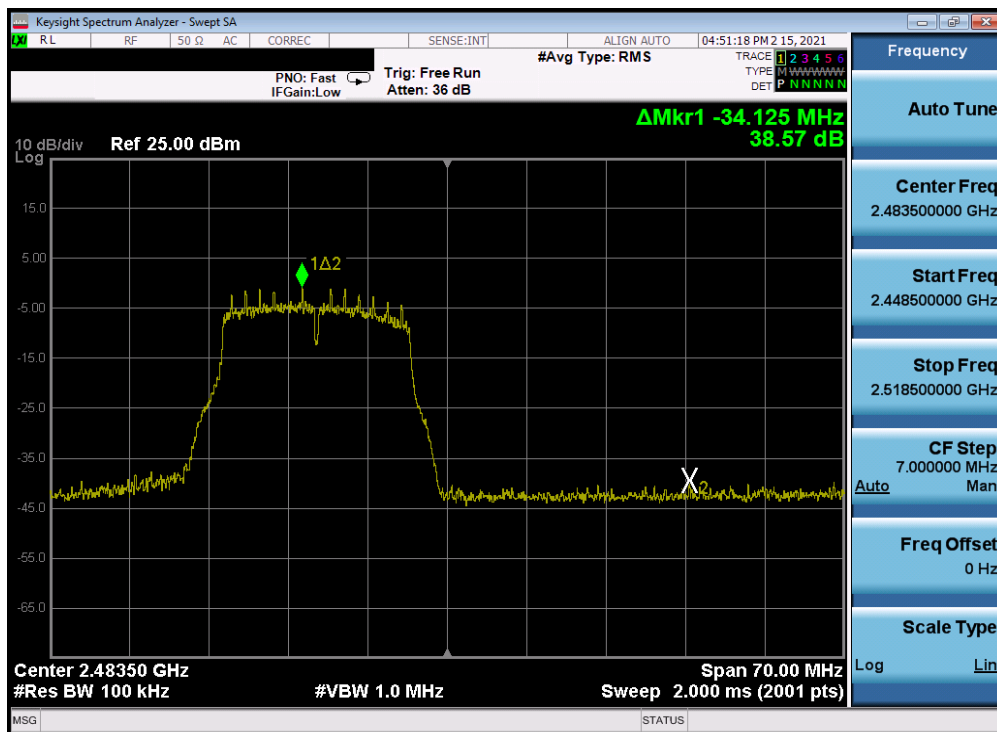
Plot 7-255. Band Edge Plot Antenna 2a (802.11g – Ch. 13) – 6Mbps
