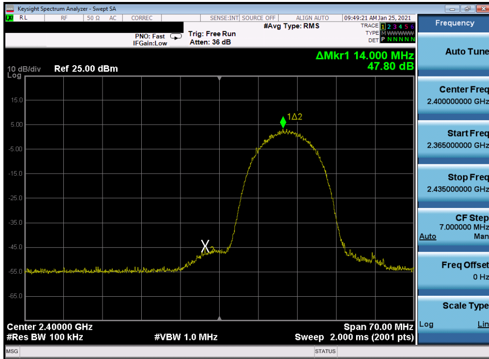
Plot 7-221. Band Edge Plot Antenna 4a (802.11b – Ch. 1) – 11Mbps
