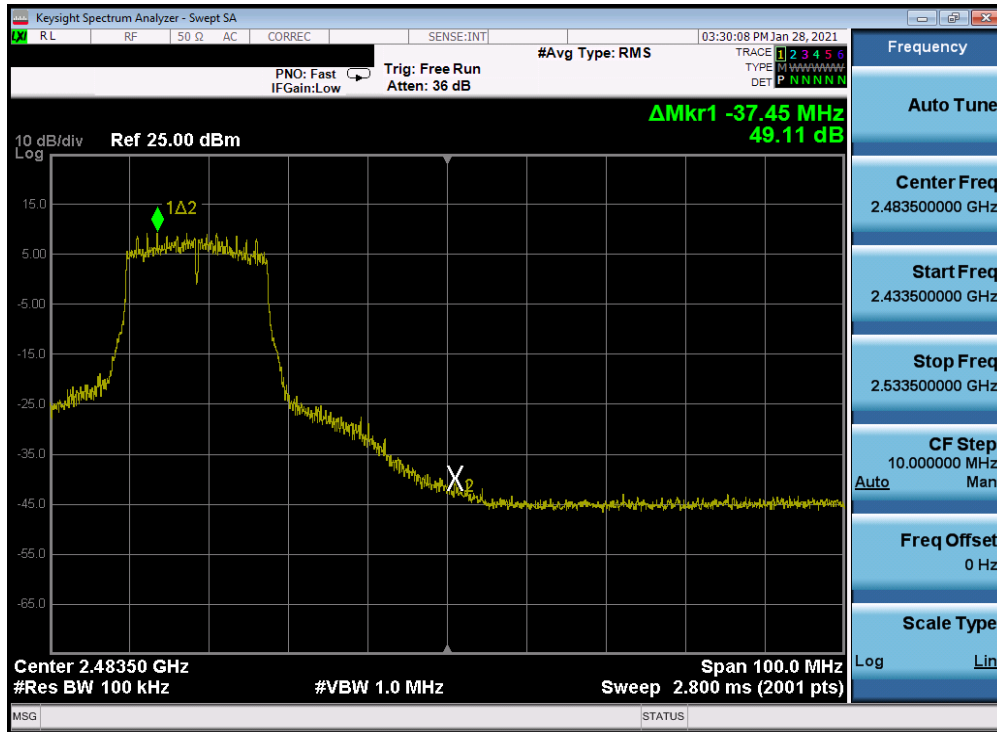
Plot 7-282. Band Edge Plot Antenna 2a (802.11n (2.4GHz) - Ch. 9) - MCS3
