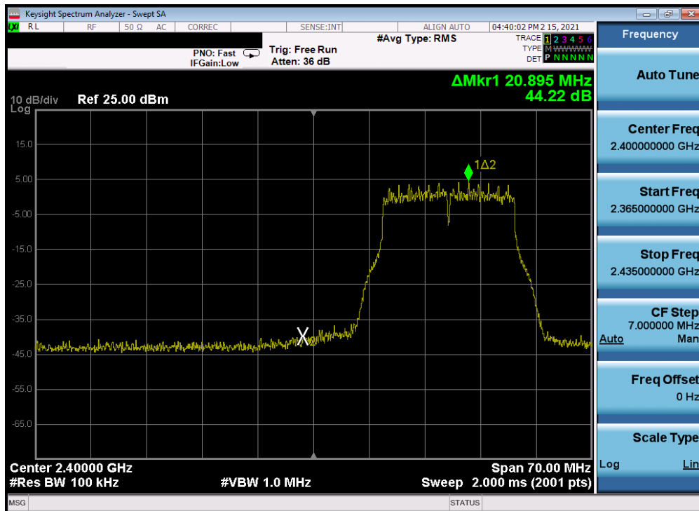
Plot 7-226. Band Edge Plot Antenna 4a (802.11g– Ch. 2) – 54Mbps
