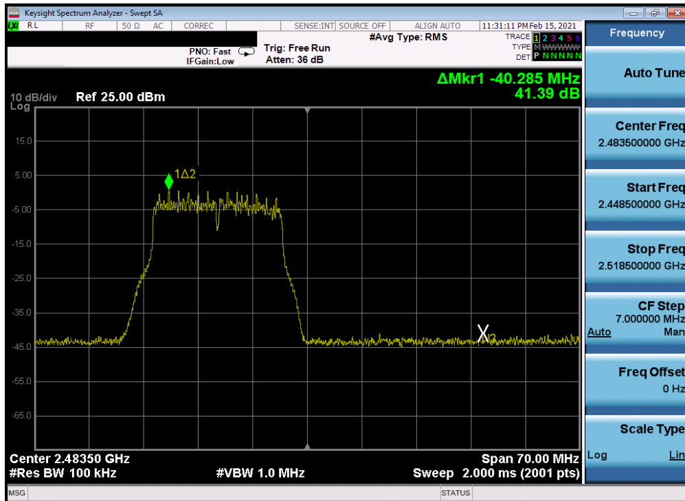
Plot 7-305. Band Edge Plot Antenna 2a (802.11g – Ch. 13) – 54Mbps
