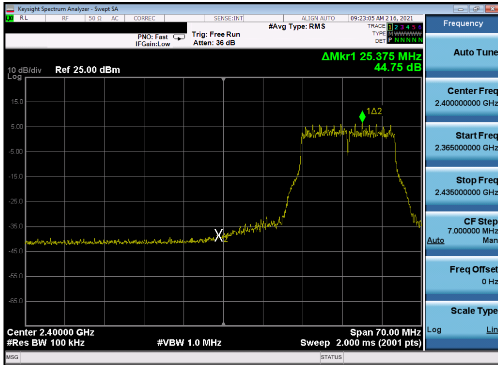
Plot 7-300. Band Edge Plot Antenna 2a (802.11g- Ch. 3) – 54Mbps
