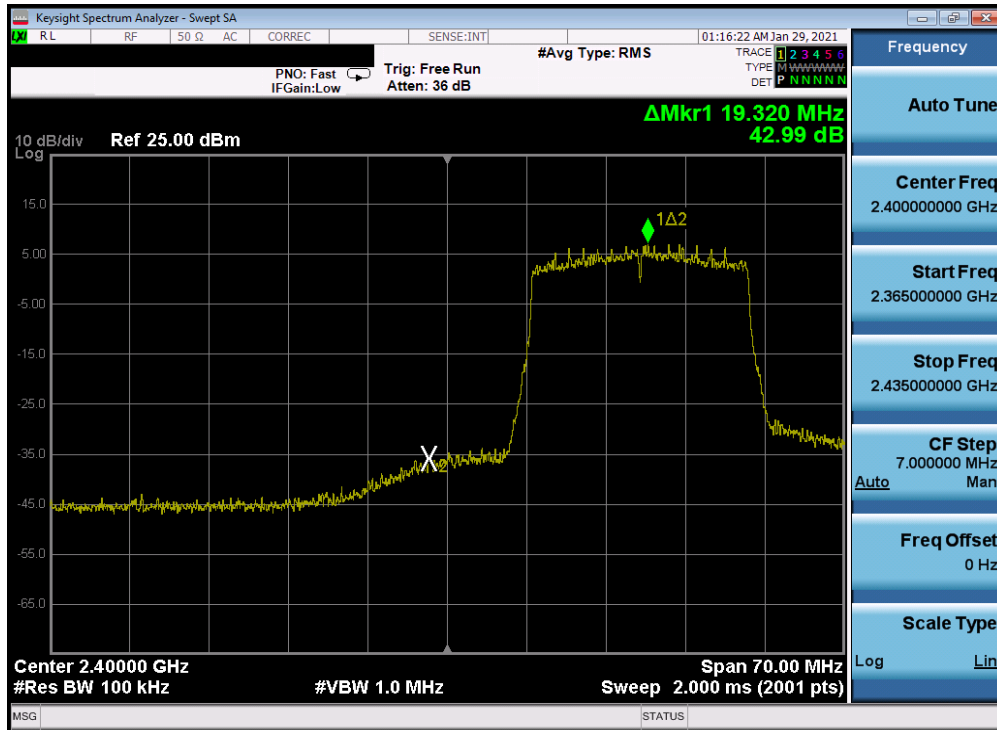
Plot 7-288. Band Edge Plot Antenna 2a (802.11ax (SU - 2.4GHz) – Ch. 2) – MCS3
