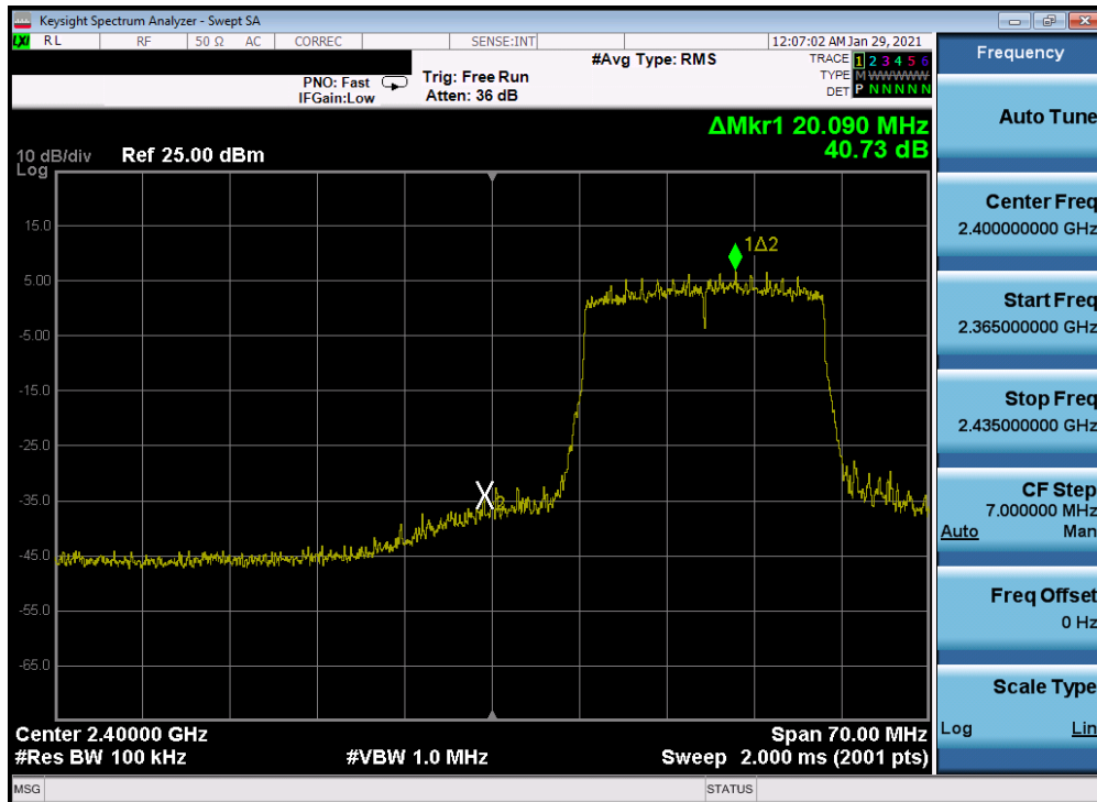
Plot 7-242. Band Edge Plot Antenna 4a (802.11ax (SU - 2.4GHz) – Ch. 2) – MCS5
