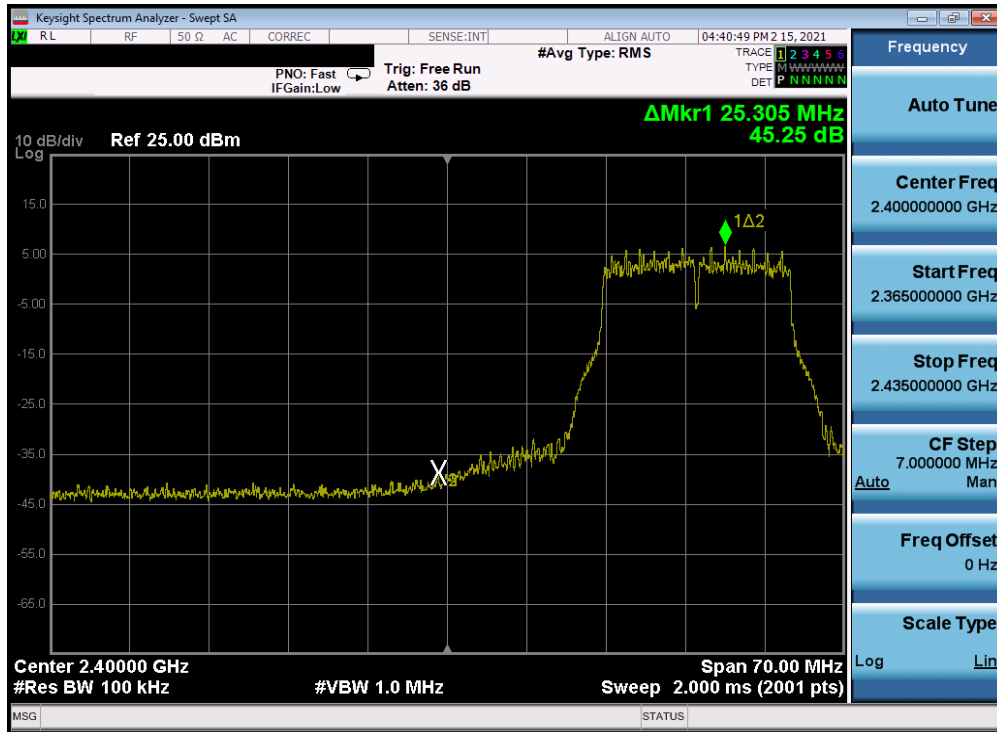
Plot 7-227. Band Edge Plot Antenna 4a (802.11g- Ch. 3) – 54Mbps
