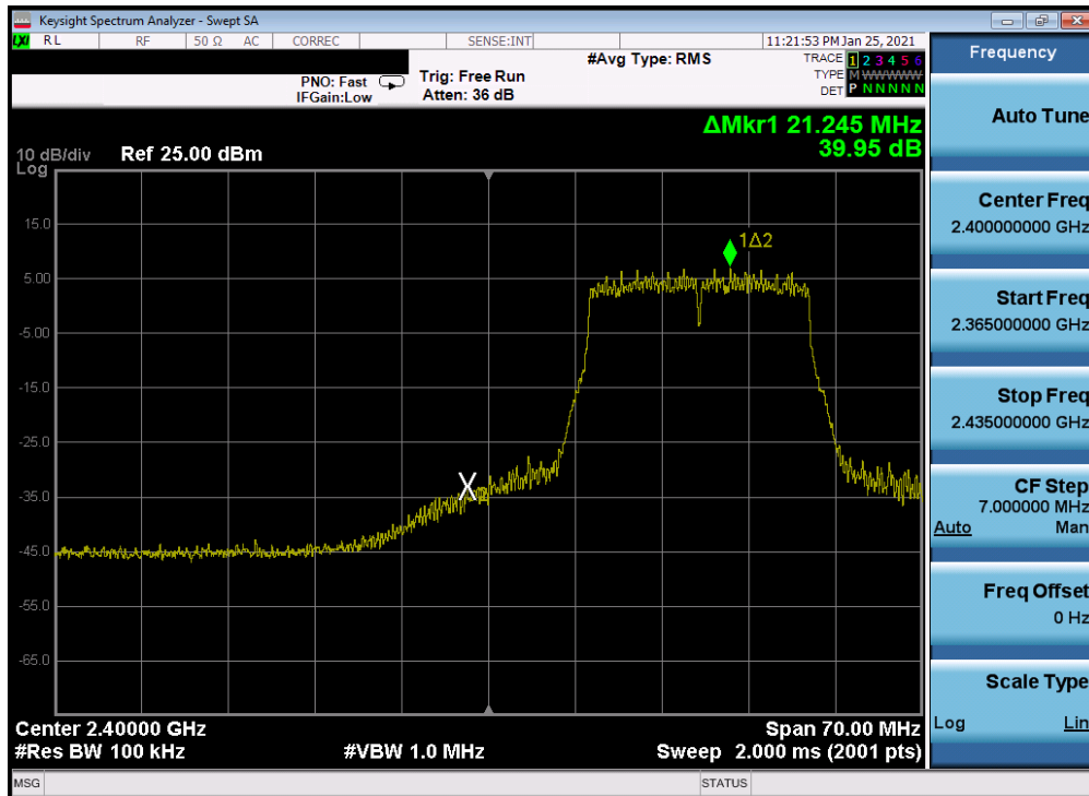
Plot 7-307. Band Edge Plot Antenna 2a (802.11n (2.4GHz) - Ch. 2) - MCS7
