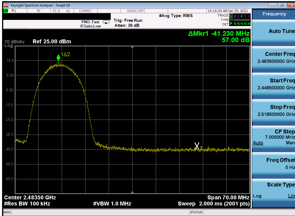
Plot 7-222. Band Edge Plot Antenna 4a (802.11b – Ch. 11) – 11Mbps
