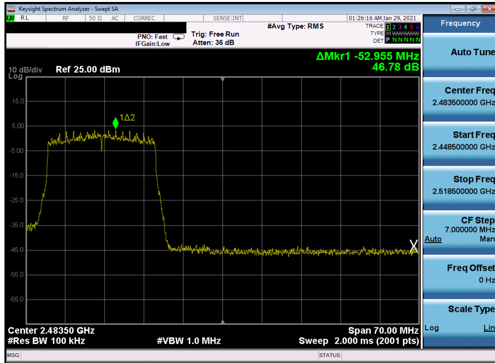
Plot 7-292. Band Edge Plot Antenna 2a (802.11ax (SU - 2.4GHz) – Ch. 11) – MCS3
