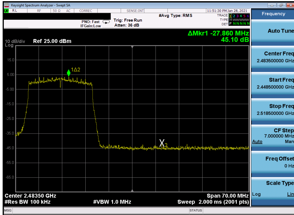
Plot 7-219. Band Edge Plot Antenna 4a (802.11ax (SU - 2.4GHz) – Ch. 11) – MCS3
