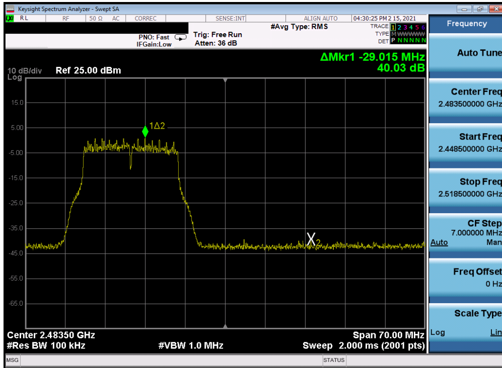
Plot 7-231. Band Edge Plot Antenna 4a (802.11g – Ch. 12) – 54Mbps
