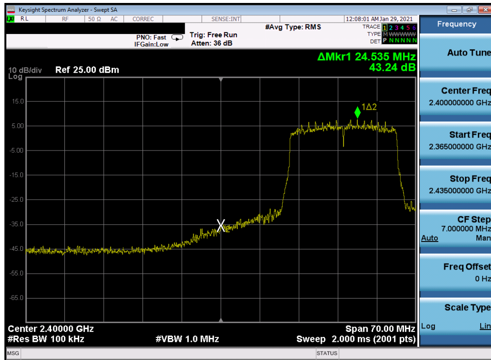
Plot 7-243. Band Edge Plot Antenna 4a (802.11ax (SU - 2.4GHz) – Ch. 3) – MCS5
