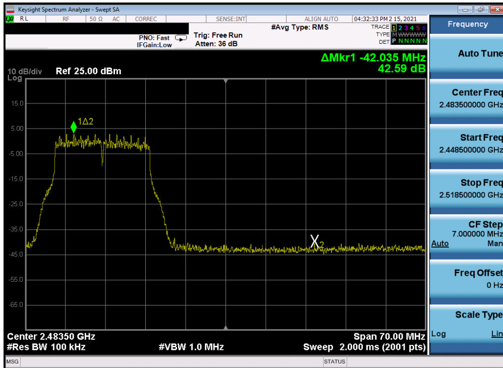
Plot 7-230. Band Edge Plot Antenna 4a (802.11g – Ch. 11) – 54Mbps
