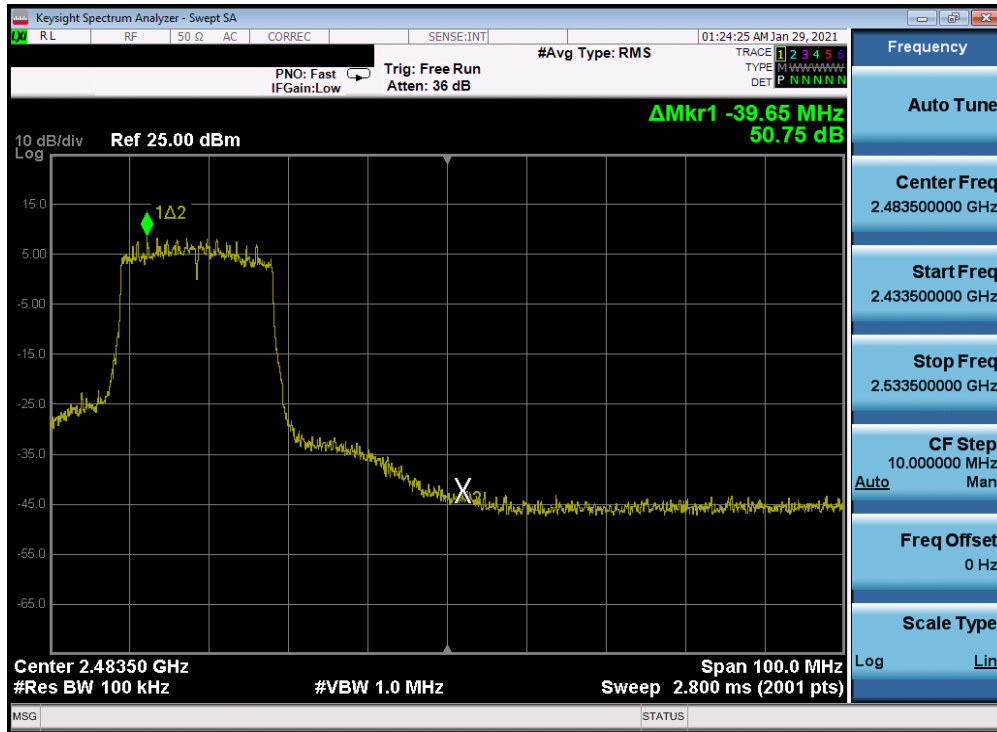
Plot 7-290. Band Edge Plot Antenna 2a (802.11ax (SU - 2.4GHz) – Ch. 9) – MCS3
