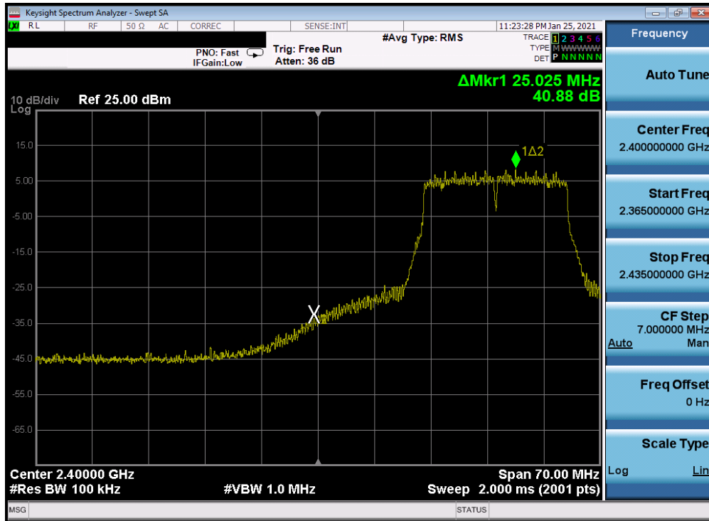
Plot 7-308. Band Edge Plot Antenna 2a (802.11n (2.4GHz) – Ch. 3) – MCS7
