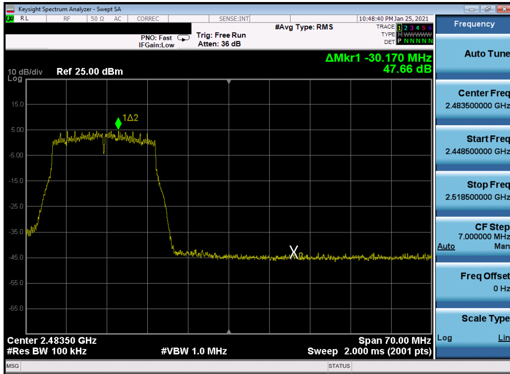
Plot 7-284. Band Edge Plot Antenna 2a (802.11n (2.4GHz) - Ch. 11) - MCS3
