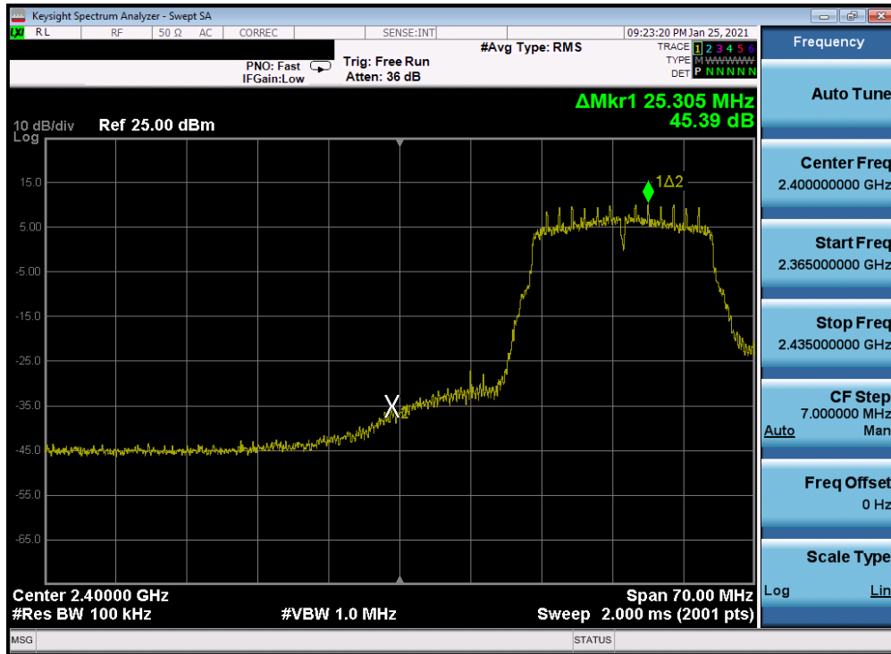
Plot 7-258. Band Edge Plot Antenna 2a (802.11n (2.4GHz) – Ch. 3) – MCS0
