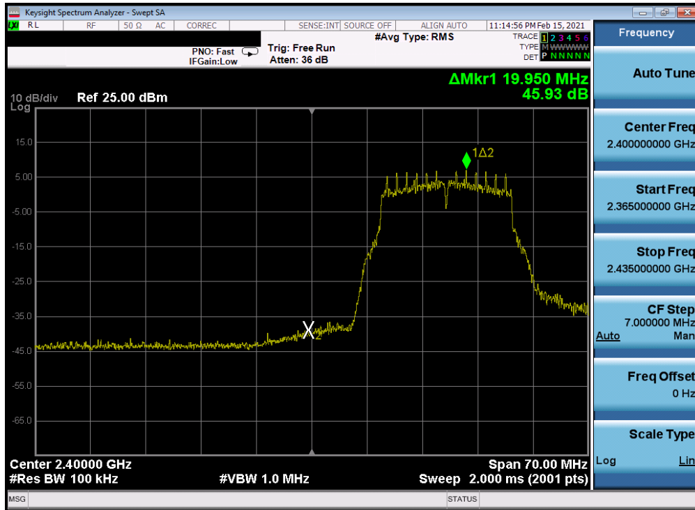
Plot 7-272. Band Edge Plot Antenna 2a (802.11g– Ch. 2) – 18Mbps
