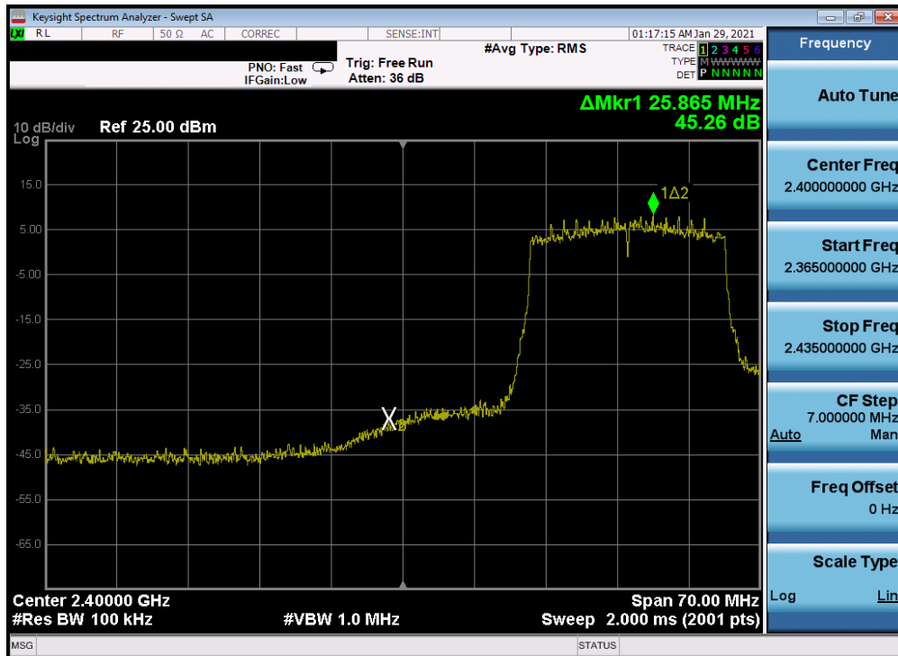
Plot 7-289. Band Edge Plot Antenna 2a (802.11ax (SU - 2.4GHz) – Ch. 3) – MCS3
