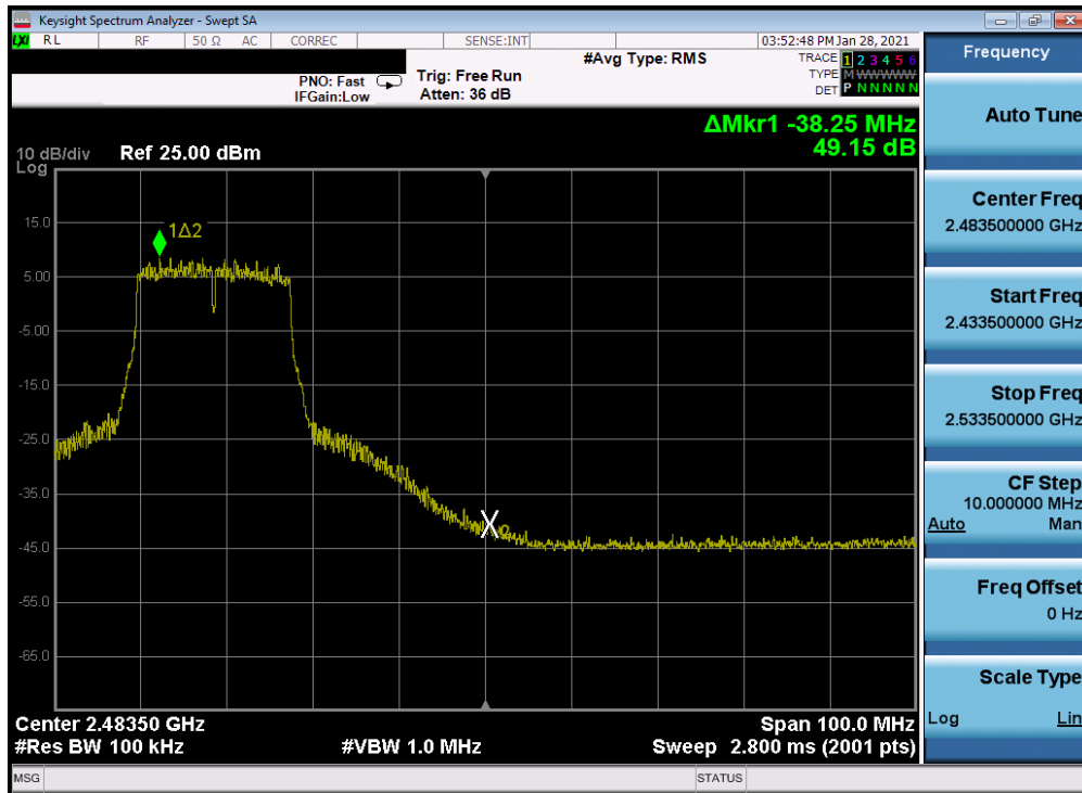
Plot 7-309. Band Edge Plot Antenna 2a (802.11n (2.4GHz) – Ch. 9) – MCS7
