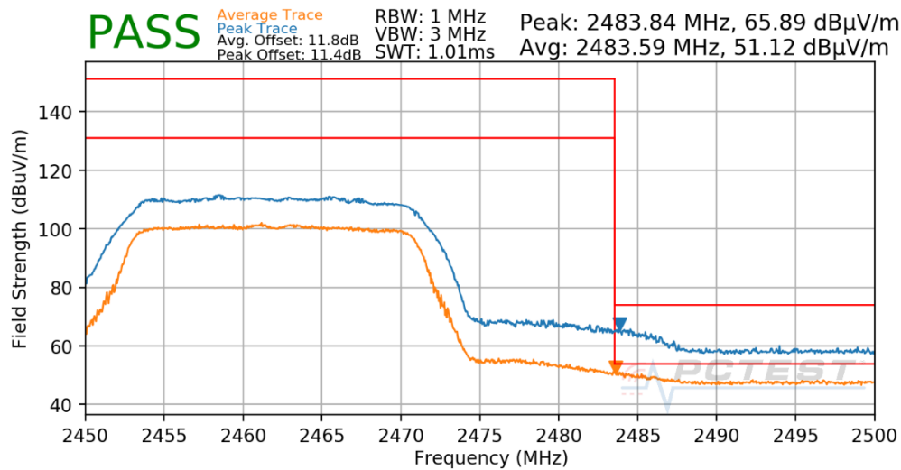
Plot 7-78. Radiated Restricted Upper Band Edge Measurement CDD
