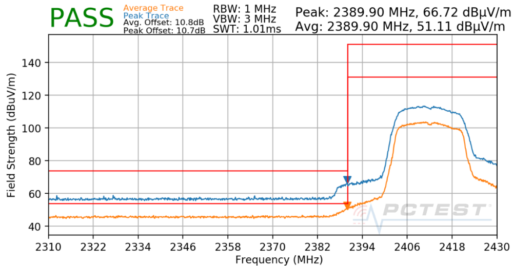
Plot 7-62. Radiated Restricted Lower Band Edge Measurement CDD
