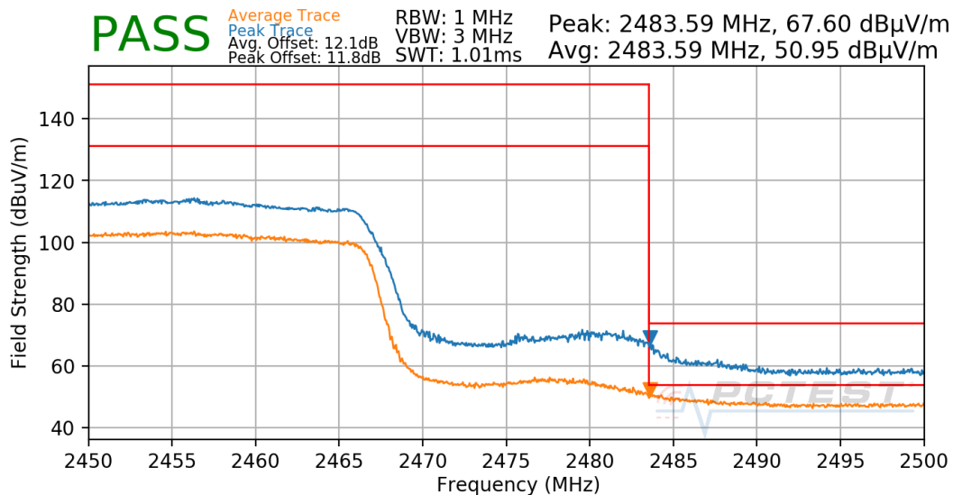
Plot 7-54. Radiated Restricted Upper Band Edge Measurement Antenna 4a
