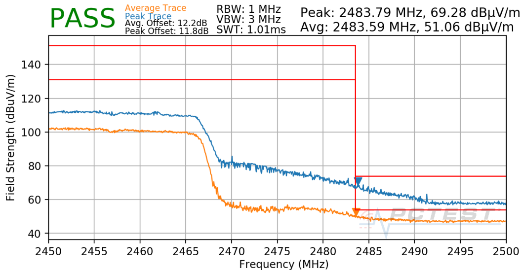
Plot 7-55. Radiated Restricted Upper Band Edge Measurement Antenna 4a
