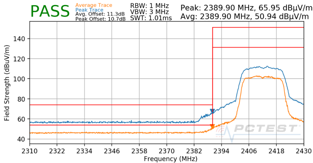
Plot 7-64. Radiated Restricted Lower Band Edge Measurement CDD
