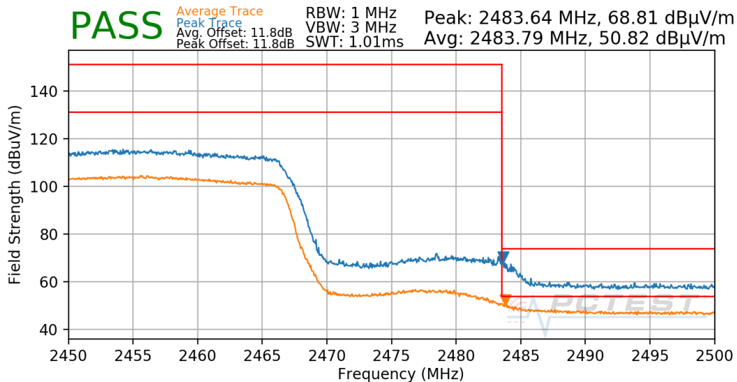
Plot 7-53. Radiated Restricted Upper Band Edge Measurement Antenna 4a
