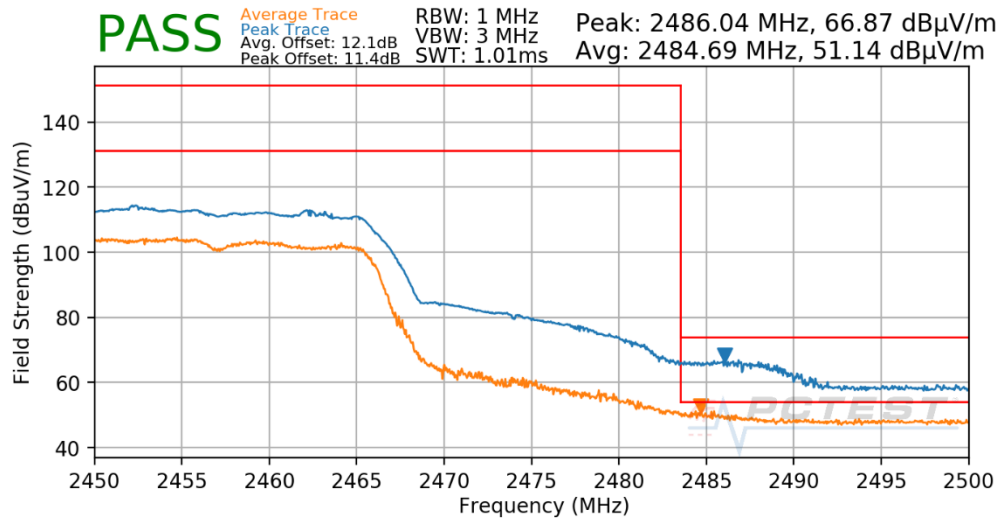
Plot 7-76. Radiated Restricted Upper Band Edge Measurement CDD
