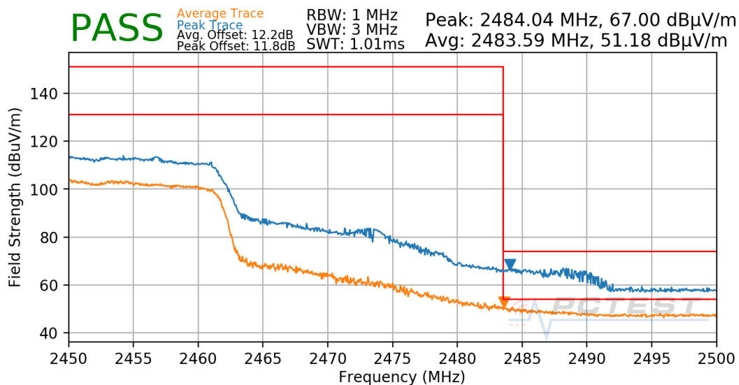
Plot 7-52. Radiated Restricted Upper Band Edge Measurement Antenna 4a
