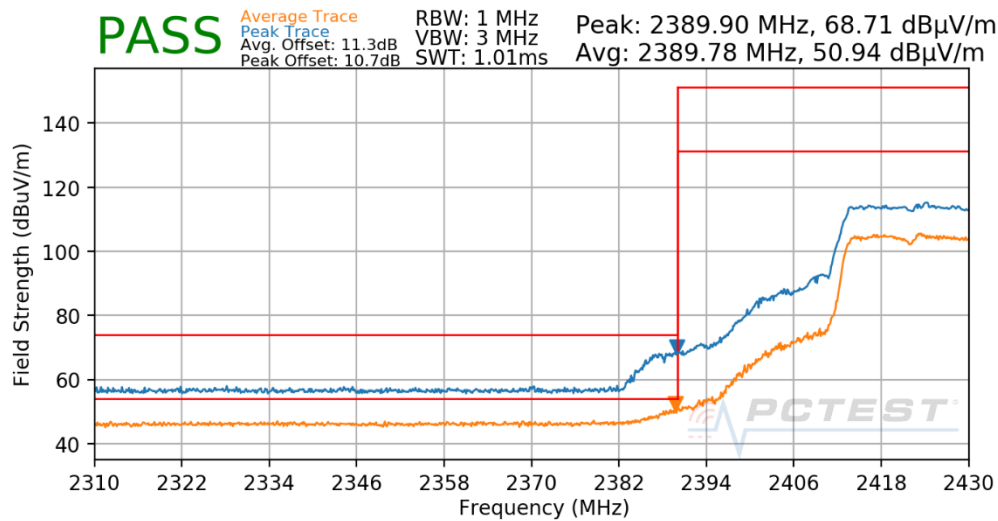
Plot 7-70. Radiated Restricted Lower Band Edge Measurement CDD
