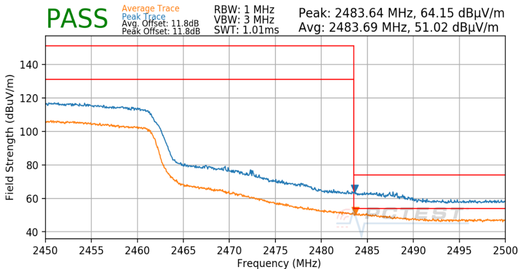
Plot 7-50. Radiated Restricted Upper Band Edge Measurement Antenna 4a
