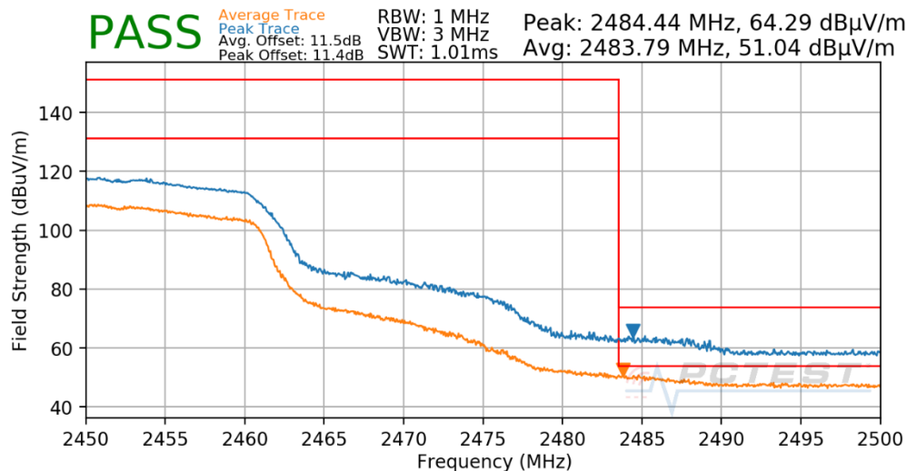
Plot 7-71. Radiated Restricted Upper Band Edge Measurement CDD
