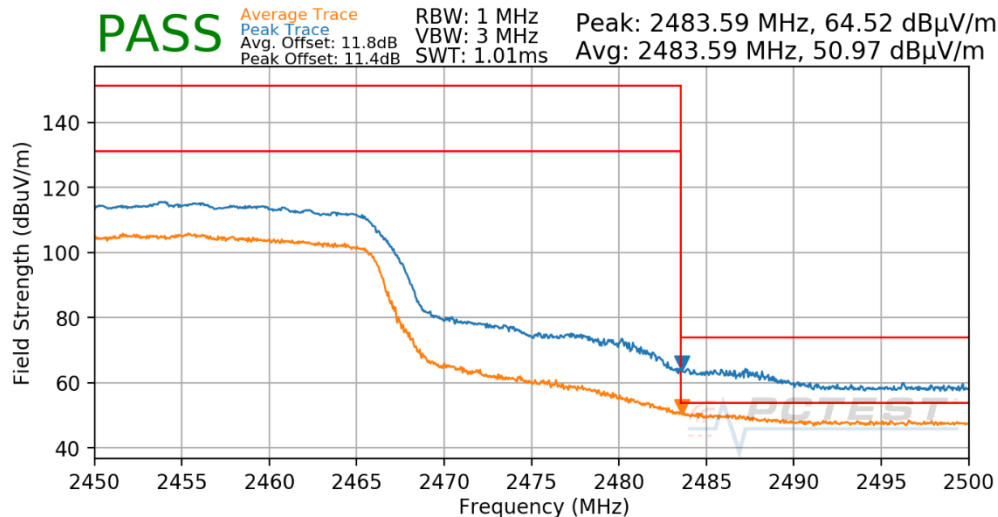
Plot 7-75. Radiated Restricted Upper Band Edge Measurement CDD
