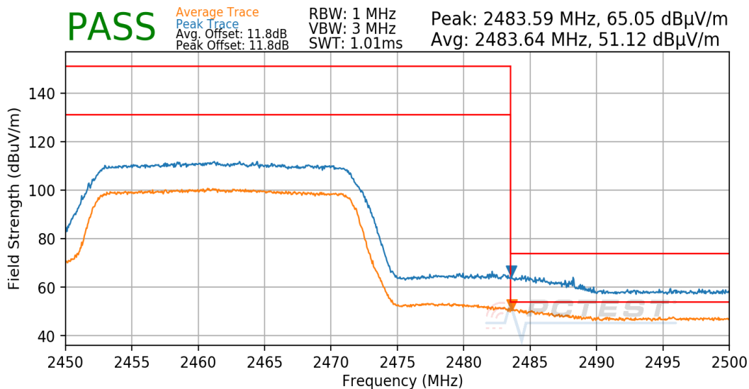
Plot 7-56. Radiated Restricted Upper Band Edge Measurement Antenna 4a
