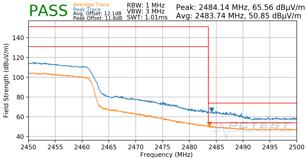
Plot 7-51. Radiated Restricted Upper Band Edge Measurement Antenna 4a
