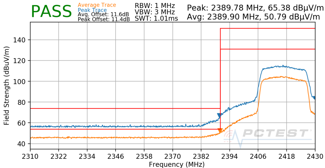
Plot 7-45. Radiated Restricted Lower Band Edge Measurement Antenna 4a
