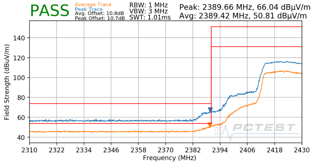
Plot 7-68. Radiated Restricted Lower Band Edge Measurement CDD
