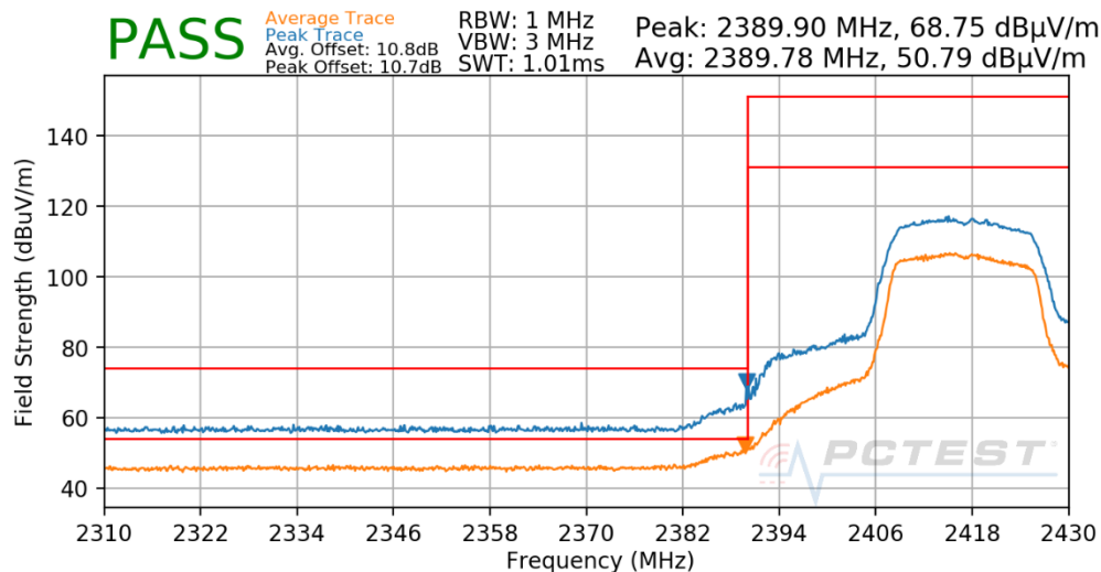
Plot 7-65. Radiated Restricted Lower Band Edge Measurement CDD
