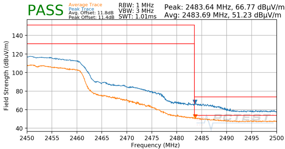
Plot 7-72. Radiated Restricted Upper Band Edge Measurement CDD
