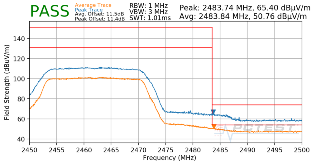
Plot 7-77. Radiated Restricted Upper Band Edge Measurement CDD
