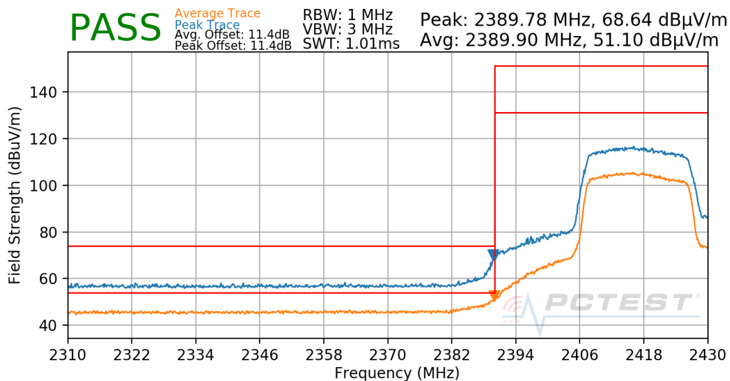
Plot 7-44. Radiated Restricted Lower Band Edge Measurement Antenna 4a
