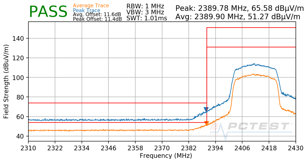
Plot 7-42. Radiated Restricted Lower Band Edge Measurement Antenna 4a
