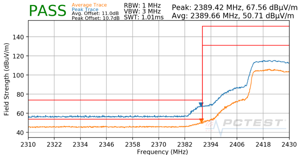
Plot 7-69. Radiated Restricted Lower Band Edge Measurement CDD
