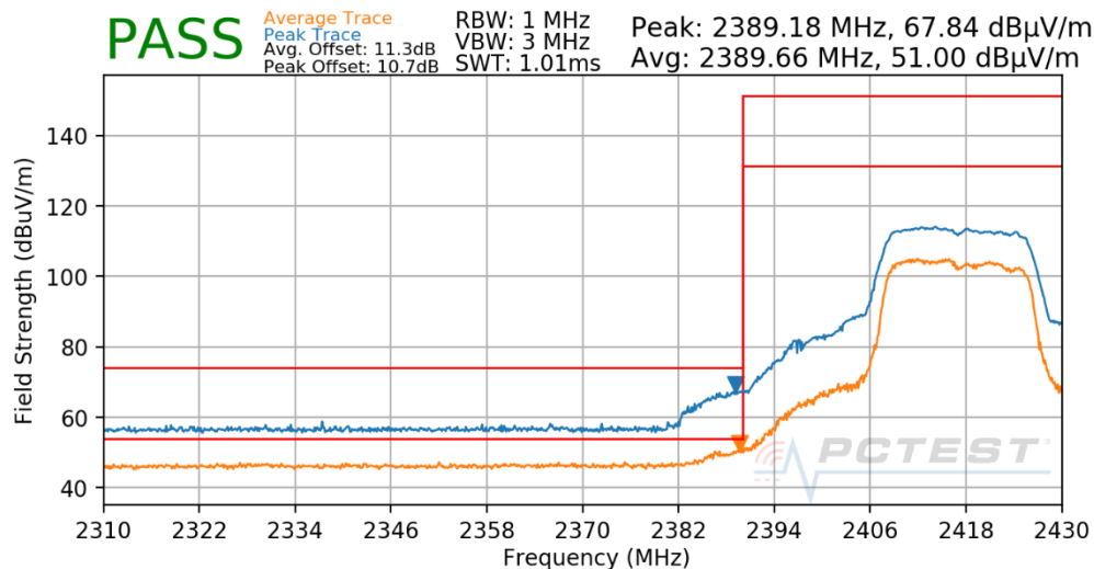
Plot 7-67. Radiated Restricted Lower Band Edge Measurement CDD
