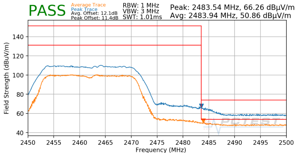
Plot 7-79. Radiated Restricted Upper Band Edge Measurement CDD
