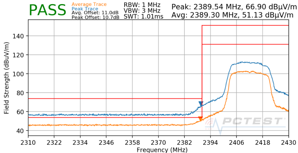
Plot 7-63. Radiated Restricted Lower Band Edge Measurement CDD
