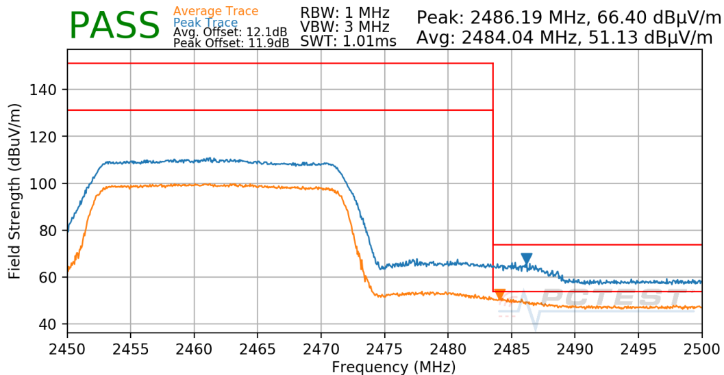
Plot 7-57. Radiated Restricted Upper Band Edge Measurement Antenna 4a
