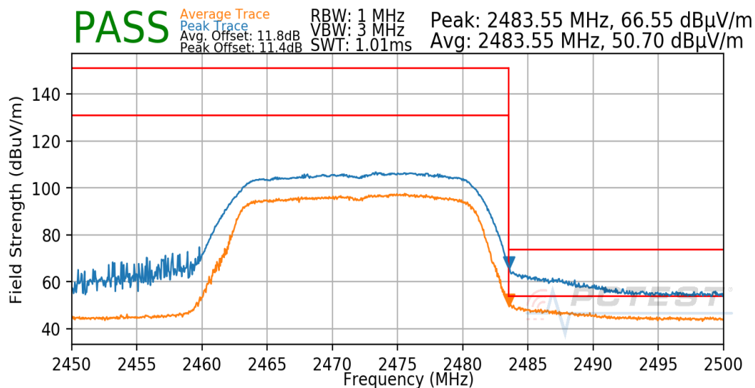
Plot 7-40. Radiated Restricted Upper Band Edge Measurement Antenna 4a
