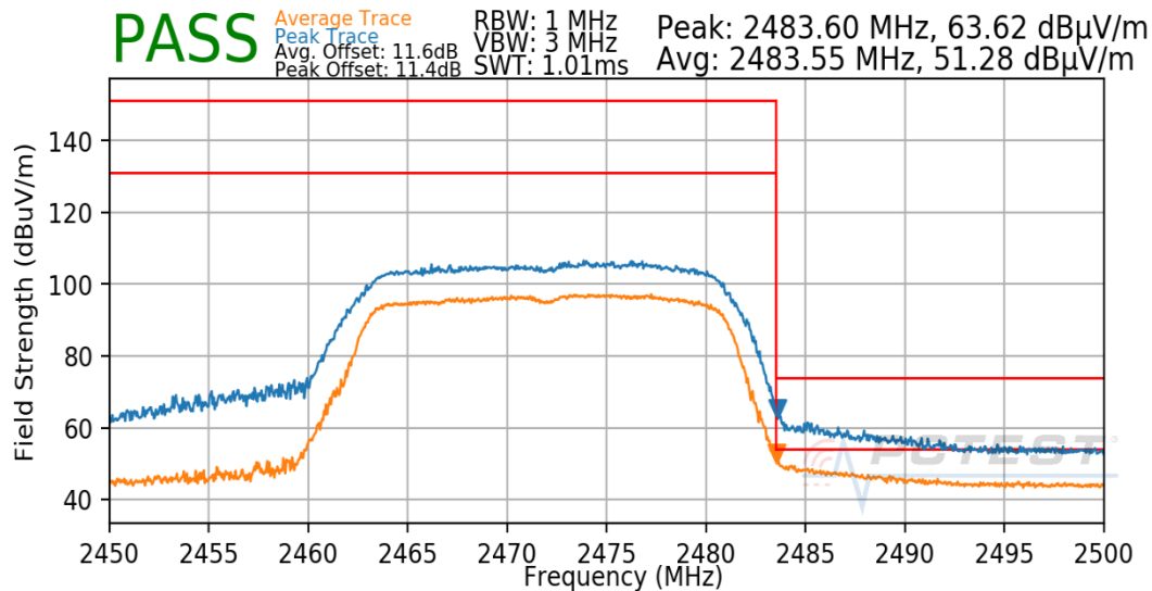
Plot 7-39. Radiated Restricted Upper Band Edge Measurement Antenna 4a
