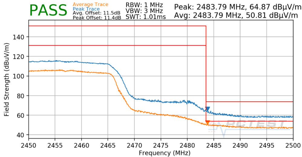
Plot 7-74. Radiated Restricted Upper Band Edge Measurement CDD
