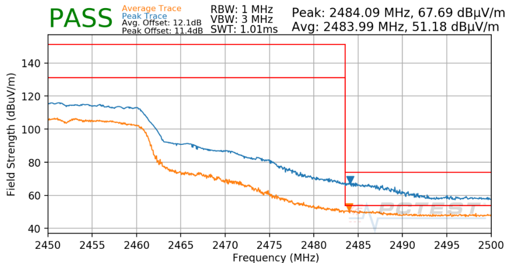
Plot 7-73. Radiated Restricted Upper Band Edge Measurement CDD
