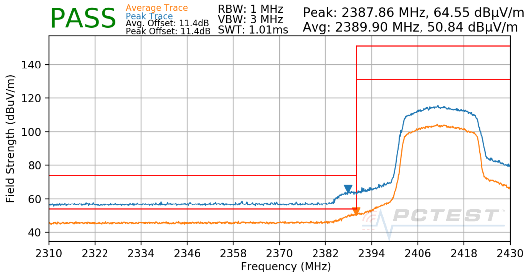
Plot 7-41. Radiated Restricted Lower Band Edge Measurement Antenna 4a
