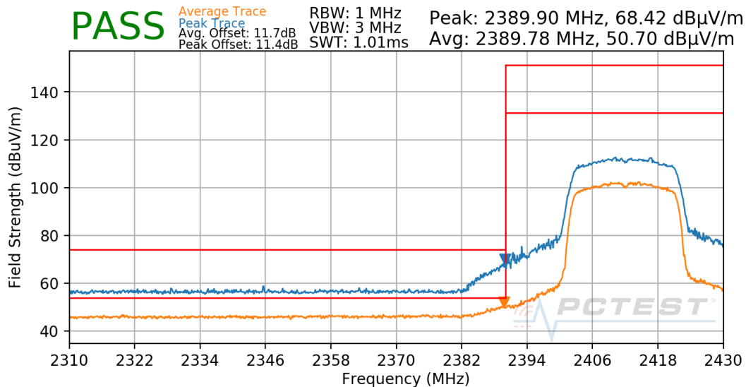
Plot 7-43. Radiated Restricted Lower Band Edge Measurement Antenna 4a
