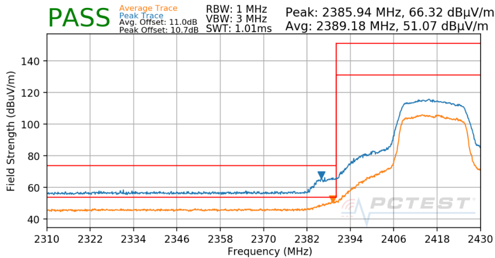
Plot 7-66. Radiated Restricted Lower Band Edge Measurement CDD
