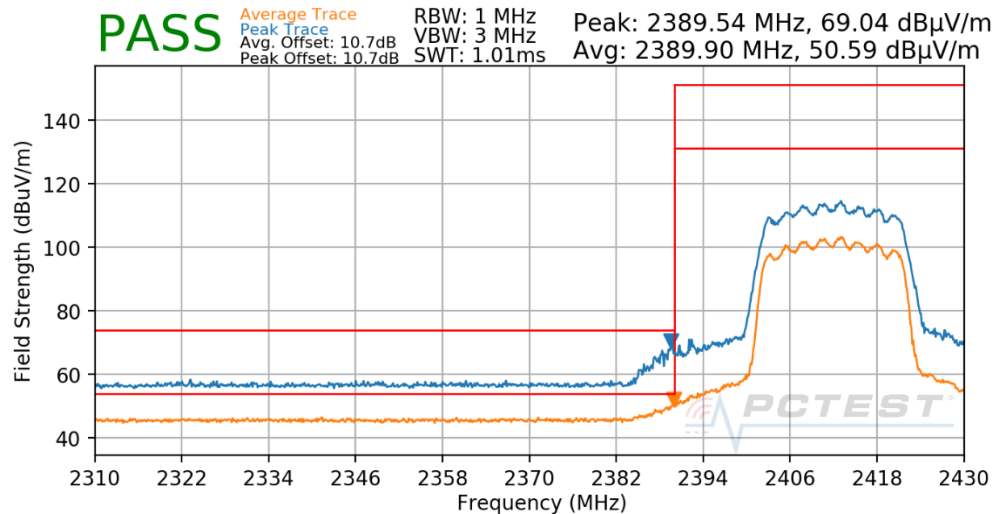
Plot 8-35: Radiated Restricted Lower Band Edge Measurement CDD (Average & Peak – RU242)
