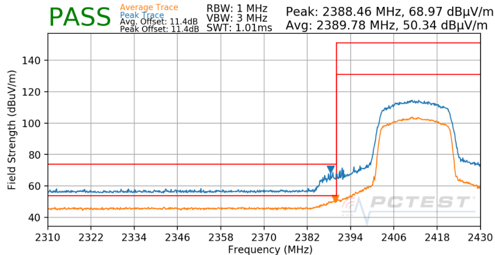
Plot 8-21. Radiated Restricted Lower Band Edge Measurement Antenna 4a (Average & Peak – RU242)
