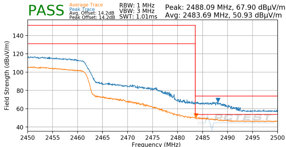
Plot 8-24: Radiated Restricted Upper Band Edge Measurement Antenna 4a (Average & Peak – RU242)
