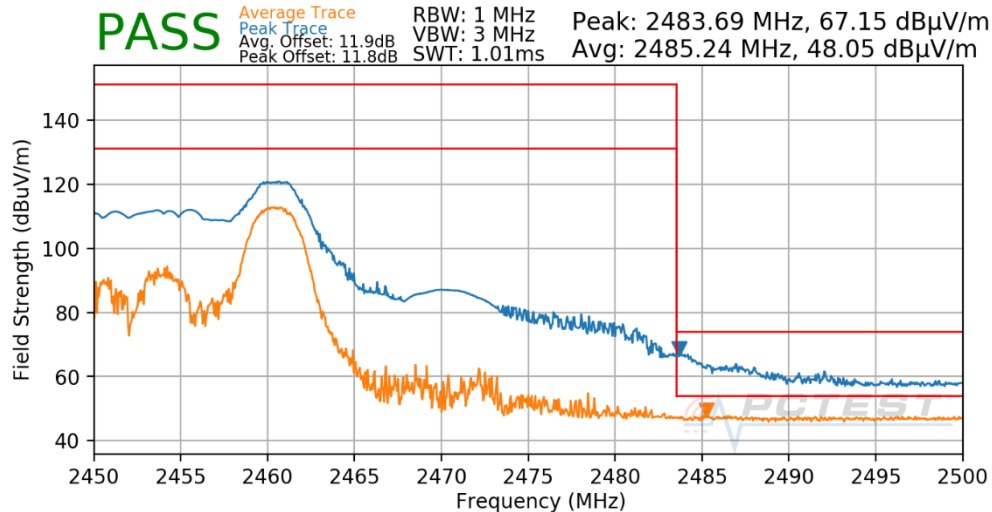
Plot 8-17. Radiated Restricted Upper Band Edge Measurement Antenna 4a (Average & Peak – RU26)
