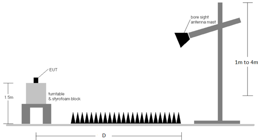
Figure 8-1. Radiated Test Setup >1GHz
