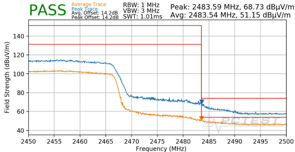
Plot 8-25: Radiated Restricted Upper Band Edge Measurement Antenna 4a (Average & Peak – RU242)
