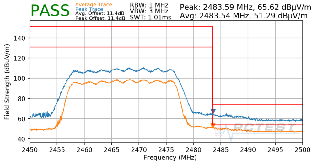
Plot 8-41: Radiated Restricted Upper Band Edge Measurement CDD (Average & Peak – RU242)
