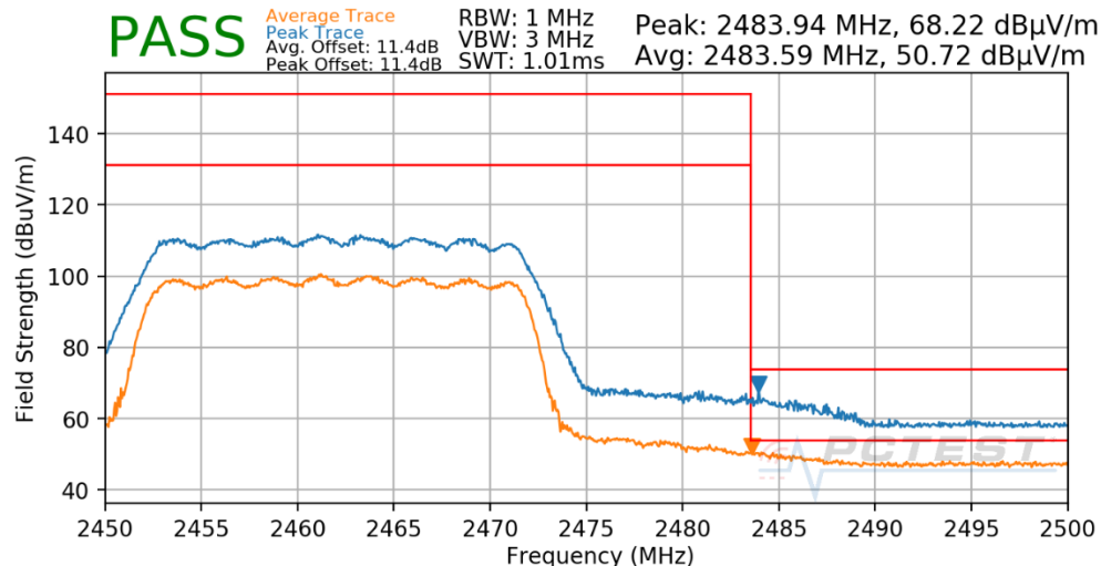
Plot 8-40: Radiated Restricted Upper Band Edge Measurement CDD (Average & Peak – RU242)
