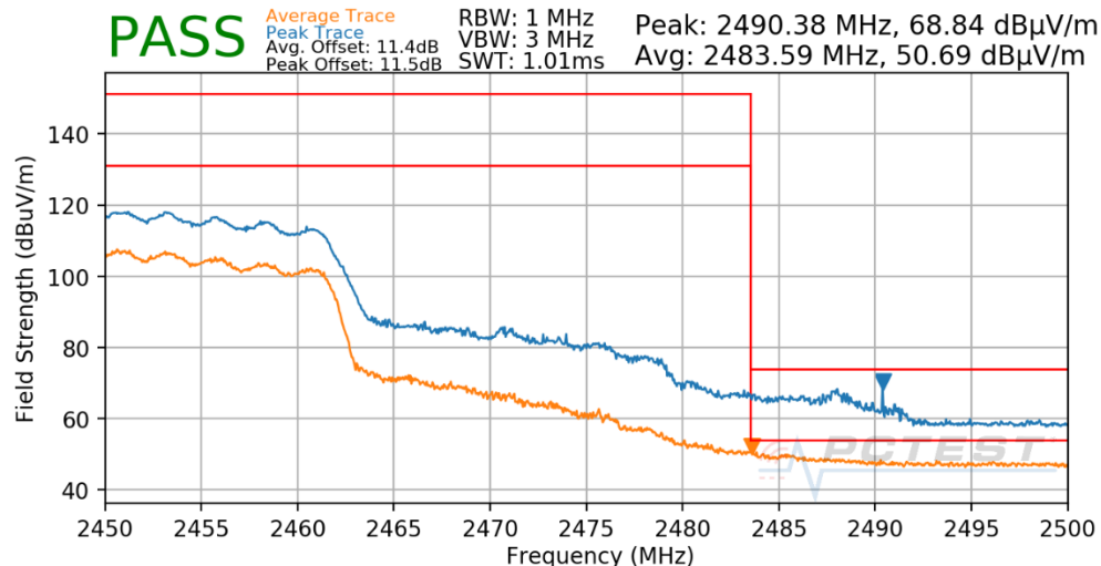
Plot 8-38: Radiated Restricted Upper Band Edge Measurement CDD (Average & Peak – RU242)
