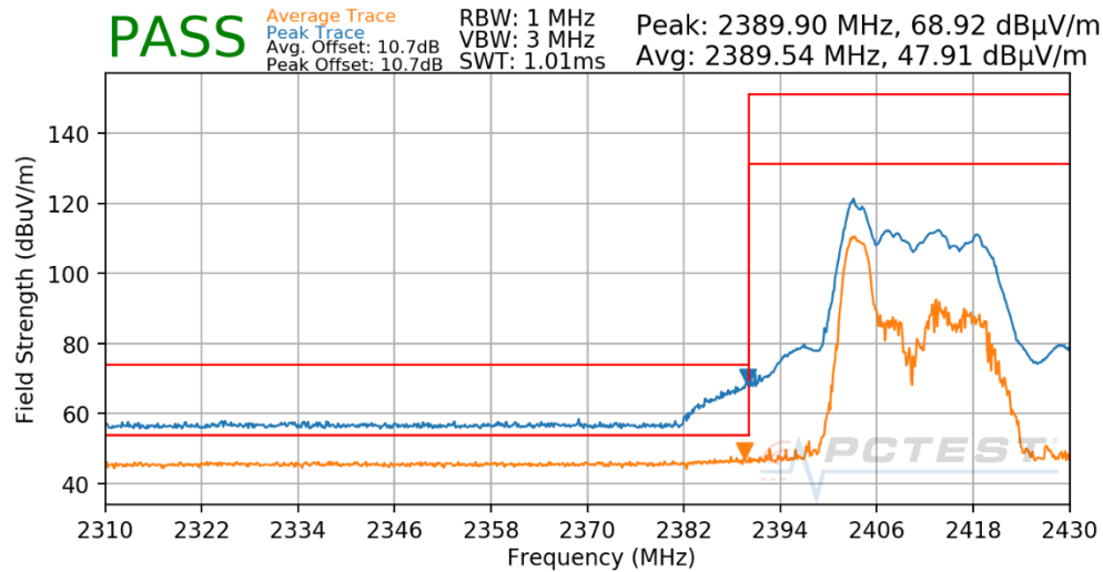
Plot 8-28: Radiated Restricted Lower Band Edge Measurement CDD (Average & Peak – RU26)
