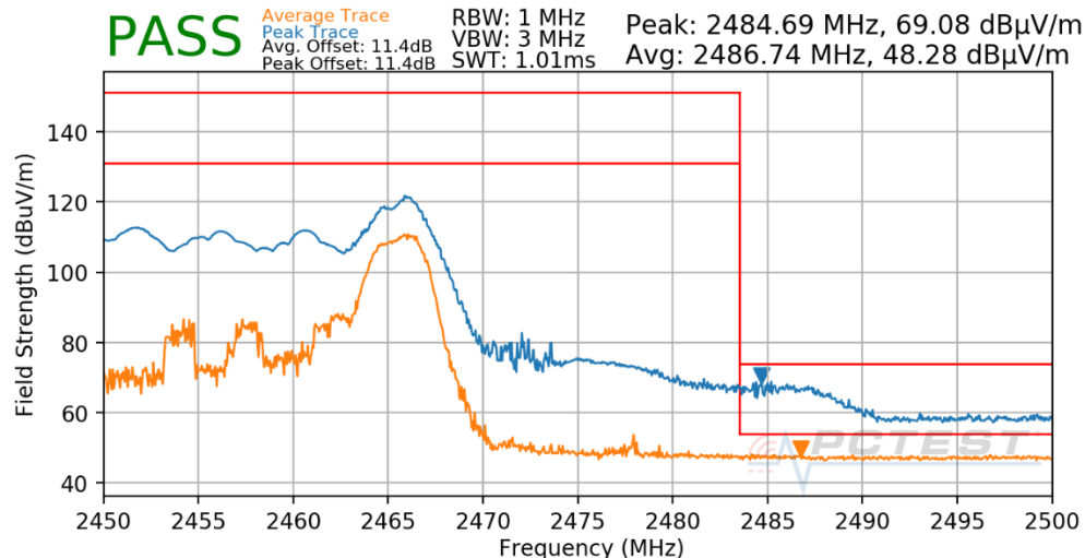
Plot 8-32: Radiated Restricted Upper Band Edge Measurement CDD (Average & Peak – RU26)
