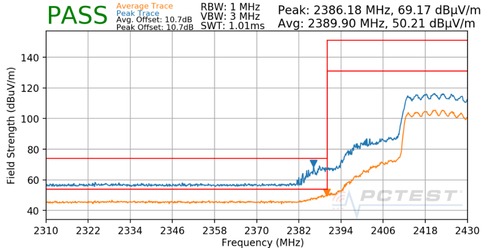
Plot 8-37: Radiated Restricted Lower Band Edge Measurement CDD (Average & Peak – RU242)
