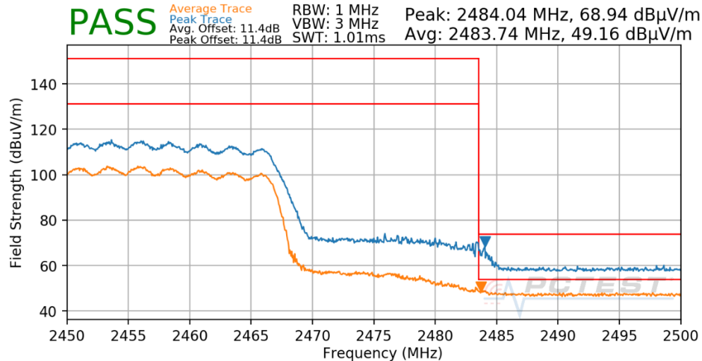
Plot 8-39: Radiated Restricted Upper Band Edge Measurement CDD (Average & Peak – RU242)
