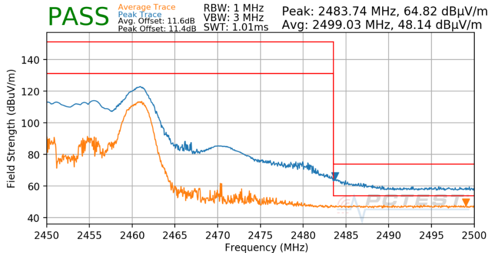
Plot 8-31: Radiated Restricted Upper Band Edge Measurement CDD (Average & Peak – RU26)
