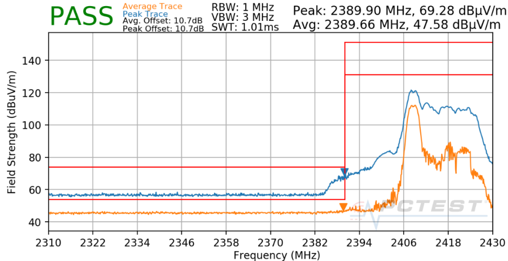
Plot 8-29: Radiated Restricted Lower Band Edge Measurement CDD (Average & Peak – RU26)
