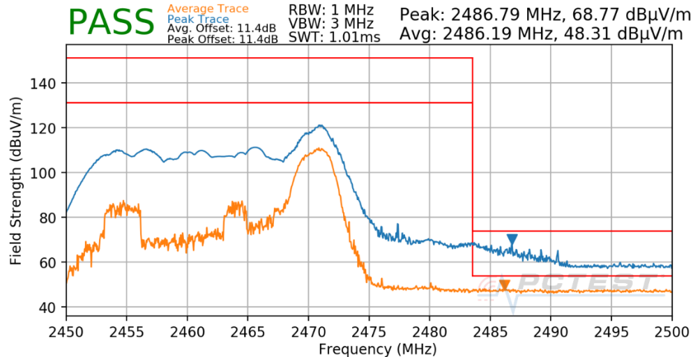
Plot 8-33: Radiated Restricted Upper Band Edge Measurement CDD (Average & Peak – RU26)
