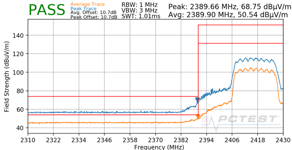
Plot 8-36: Radiated Restricted Lower Band Edge Measurement CDD (Average & Peak – RU242)
