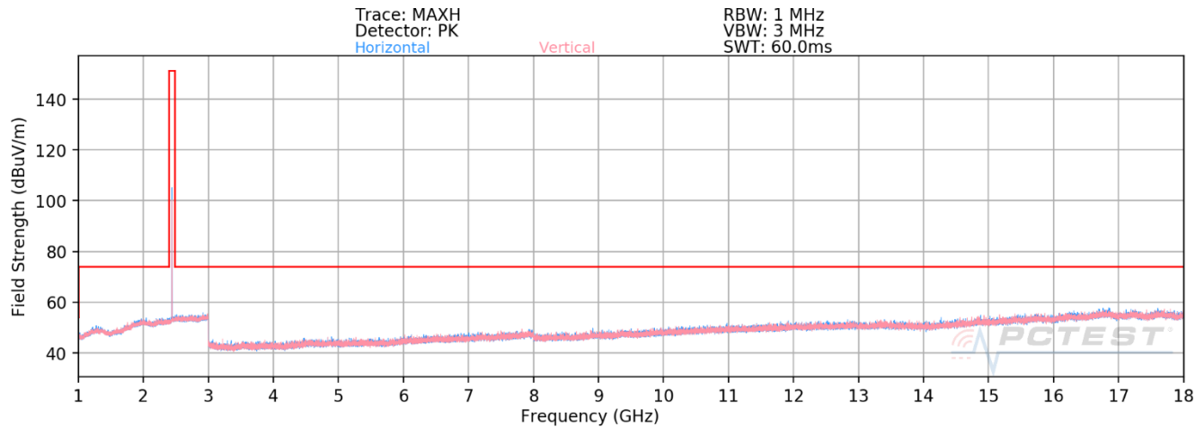
Plot 7-1. Radiated Spurious Emissions Above 1GHz TxBF (4Mbps, HDR4, ePA – Ch. 38)
