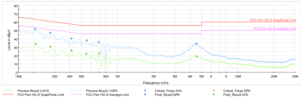
Plot 7-106. AC Line Conducted Plot with Bluetooth LE TxBF (1Mbps, ePA – Ch.19, N, with AC/DC Adapter)
