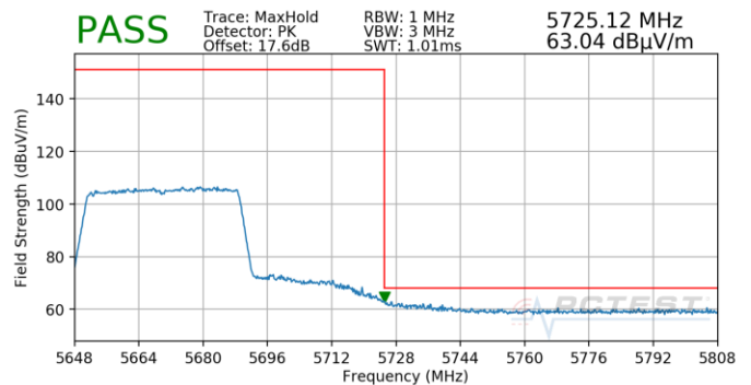
Plot 7-888. Antenna 4b (Pk, Ch.134, 80.11ax(SU), MCS3)
