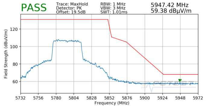
Plot 7-895. Antenna 4b (Pk, Ch.159, 80.11ax(SU), MCS11)
