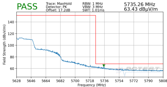
Plot 7-848. (FCC Only) Antenna 4b (Pk, Ch.126, 802.11n, MCS0)
