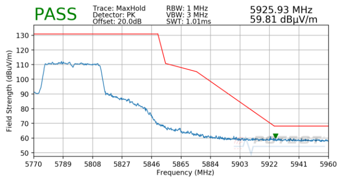
Plot 7-859. Antenna 4b (Pk, Ch.159, 802.11n, MCS5)
