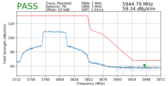
Plot 7-894. Antenna 4b (Pk, Ch.159, 80.11ax(SU), MCS3)
