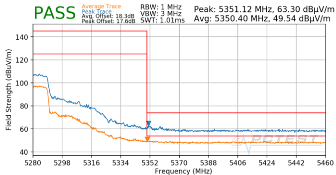
Plot 7-868. Antenna 4b (Pk & Avg, Ch.54, 80.11ax(SU), MCS11)
