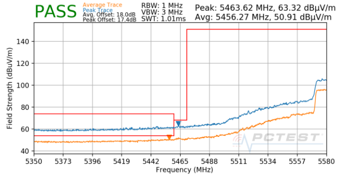
Plot 7-906. (FCC Only) Antenna 4b (Pk & Avg, Ch.122, 802.11ac, MCS3)
