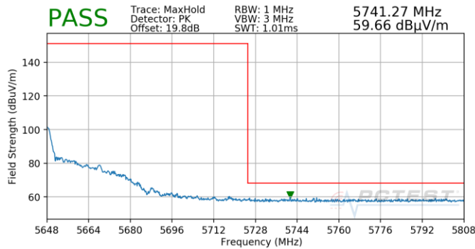
Plot 7-886. (FCC Only) Antenna 4b (Pk, Ch.126, 80.11ax(SU), MCS11)
