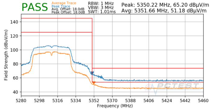
Plot 7-838. Antenna 4b (Pk & Avg, Ch.62, 802.11n, MCS0)
