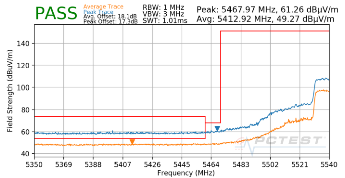
Plot 7-877. Antenna 4b (Pk & Avg, Ch.110, 80.11ax(SU), MCS11)
