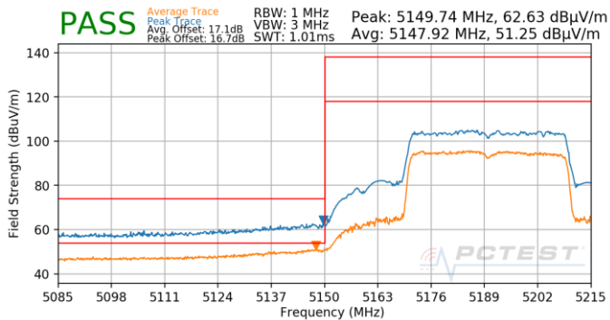
Plot 7-861. Antenna 4b (Pk & Avg, Ch.38, 80.11ax(SU), MCS3)
