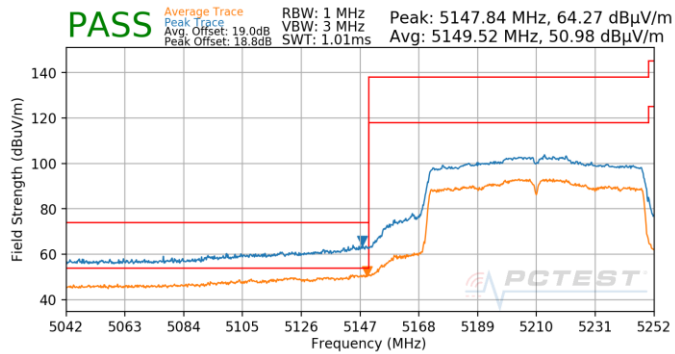
Plot 7-896. Antenna 4b (Pk & Avg, Ch.42, 802.11ac, MCS0)
