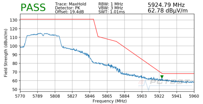
Plot 7-857. Antenna 4b (Pk, Ch.159, 802.11n, MCS0)
