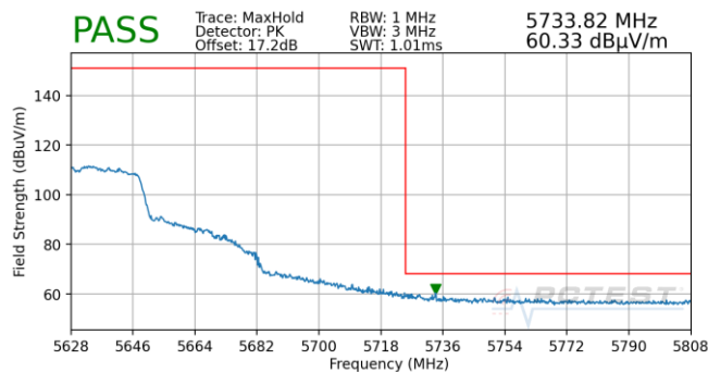
Plot 7-849. (FCC Only) Antenna 4b (Pk, Ch.126, 802.11n, MCS3)
