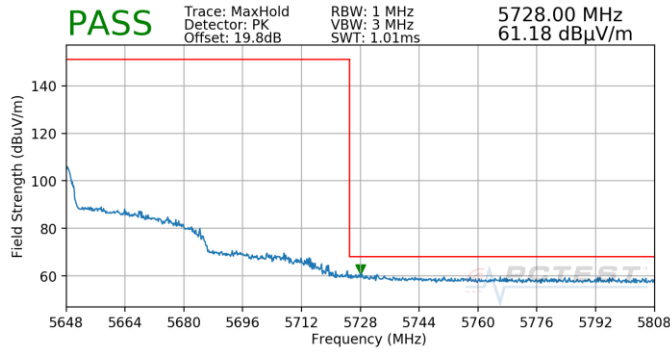
Plot 7-884. (FCC Only) Antenna 4b (Pk, Ch.126, 80.11ax(SU), MCS0)
