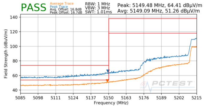
Plot 7-863. Antenna 4b (Pk & Avg, Ch.46, 80.11ax(SU), MCS0)
