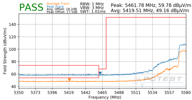
Plot 7-880. (FCC Only) Antenna 4b (Pk & Avg, Ch.118, 80.11ax(SU), MCS11)
