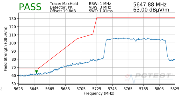
Plot 7-913. Antenna 4b (Pk, Ch.155, 802.11ac, MCS5)
