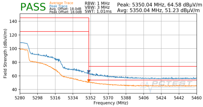
Plot 7-835. Antenna 4b (Pk & Avg, Ch.54, 802.11n, MCS0)
