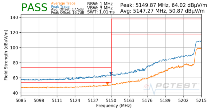
Plot 7-865. Antenna 4b (Pk & Avg, Ch.46, 80.11ax(SU), MCS11)
