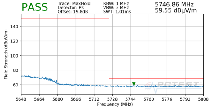
Plot 7-881. (FCC Only) Antenna 4b (Pk, Ch.118, 80.11ax(SU), MCS0)
