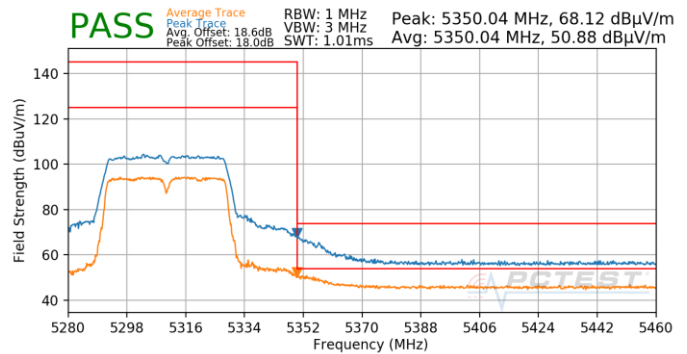
Plot 7-840. Antenna 4b (Pk & Avg, Ch.62, 802.11n, MCS5)
