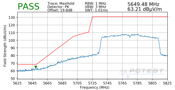
Plot 7-912. Antenna 4b (Pk, Ch.155, 802.11ac, MCS3)
