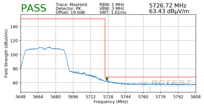
Plot 7-852. Antenna 4b (Pk, Ch.134, 802.11n, MCS3)
