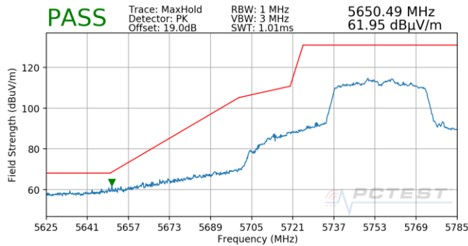
Plot 7-855. Antenna 4b (Pk, Ch.151, 802.11n, MCS3)
