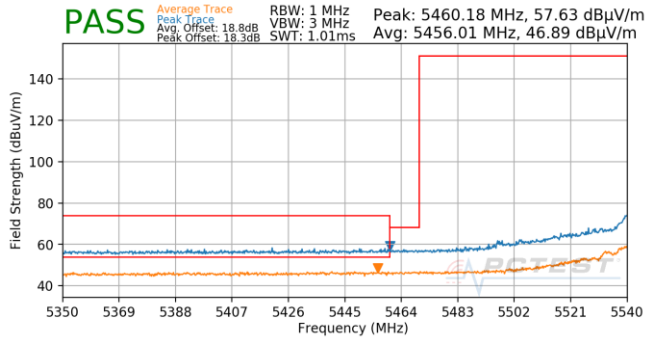
Plot 7-847. (FCC Only) Antenna 4b (Pk, Ch.118, 802.11n, MCS5)
