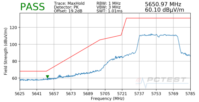
Plot 7-856. Antenna 4b (Pk, Ch.151, 802.11n, MCS5)
