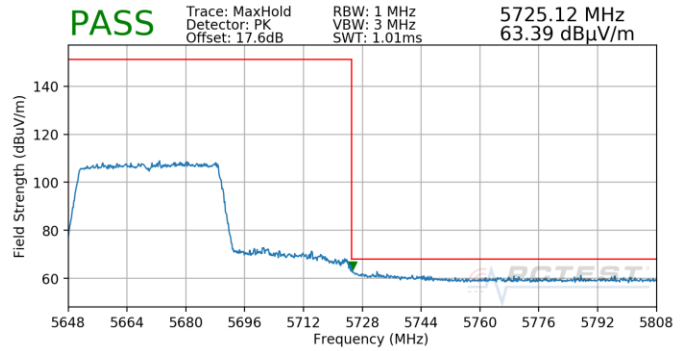
Plot 7-887. Antenna 4b (Pk, Ch.134, 80.11ax(SU), MCS0)
