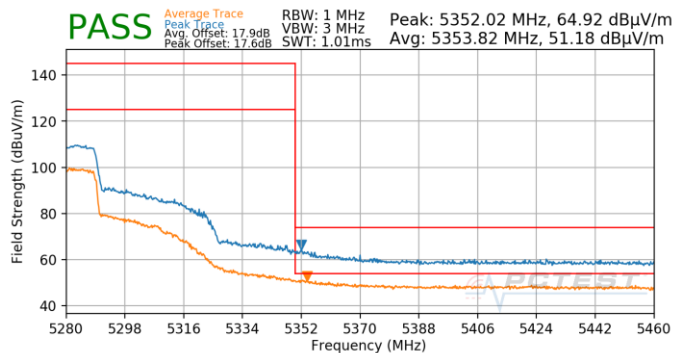
Plot 7-867. Antenna 4b (Pk & Avg, Ch.54, 80.11ax(SU), MCS3)
