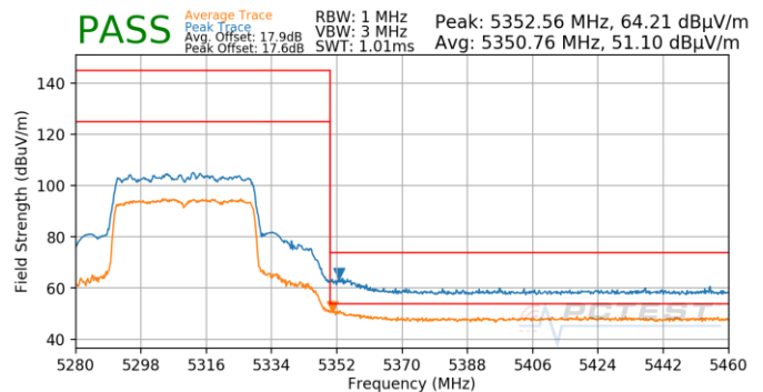
Plot 7-870. Antenna 4b (Pk & Avg, Ch.62, 80.11ax(SU), MCS3)
