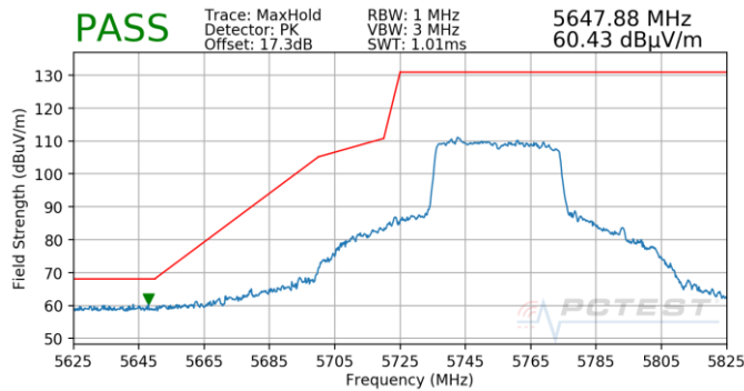
Plot 7-892. Antenna 4b (Pk, Ch.151, 80.11ax(SU), MCS11)
