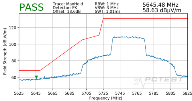
Plot 7-891. Antenna 4b (Pk, Ch.151, 80.11ax(SU), MCS3)
