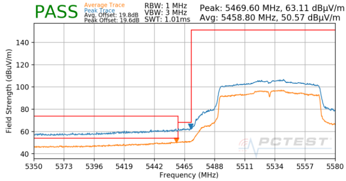
Plot 7-902. Antenna 4b (Pk & Avg, Ch.106, 802.11ac, MCS0)
