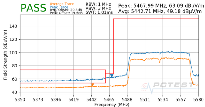
Plot 7-904. Antenna 4b (Pk & Avg, Ch.106, 802.11ac, MCS5)
