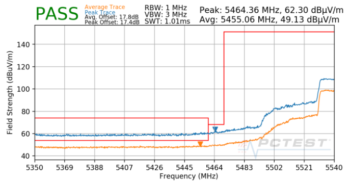
Plot 7-876. Antenna 4b (Pk & Avg, Ch.110, 80.11ax(SU), MCS3)
