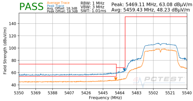
Plot 7-841. Antenna 4b (Pk & Avg, Ch.102, 802.11n, MCS0)
