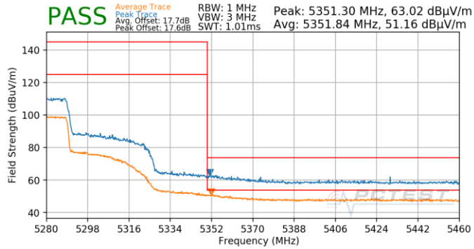
Plot 7-866. Antenna 4b (Pk & Avg, Ch.54, 80.11ax(SU), MCS0)
