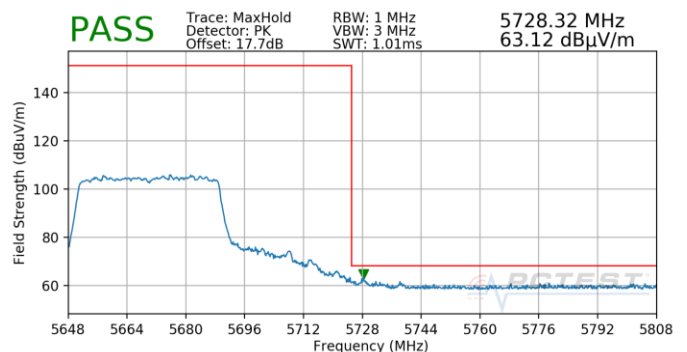
Plot 7-889. Antenna 4b (Pk, Ch.134, 80.11ax(SU), MCS11)
