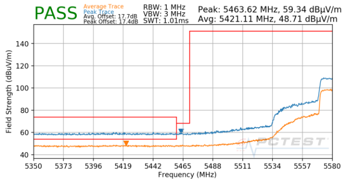
Plot 7-879. (FCC Only) Antenna 4b (Pk & Avg, Ch.118, 80.11ax(SU), MCS3)
