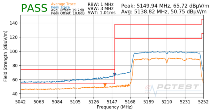
Plot 7-898. Antenna 4b (Pk & Avg, Ch.42, 802.11ac, MCS5)
