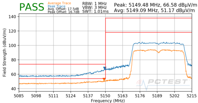
Plot 7-862. Antenna 4b (Pk & Avg, Ch.38, 80.11ax(SU), MCS11)
