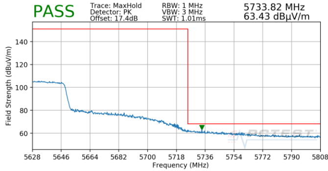
Plot 7-908. (FCC Only) Antenna 4b (Pk, Ch.122, 802.11ac, MCS0)
