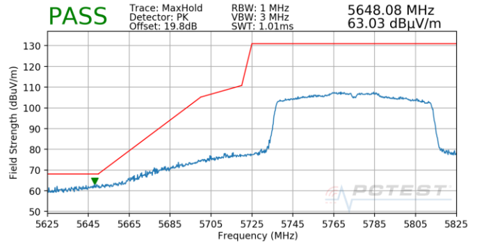
Plot 7-911. Antenna 4b (Pk, Ch.155, 802.11ac, MCS0)
