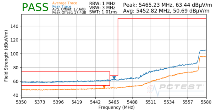
Plot 7-905. (FCC Only) Antenna 4b (Pk & Avg, Ch.122, 802.11ac, MCS0)
