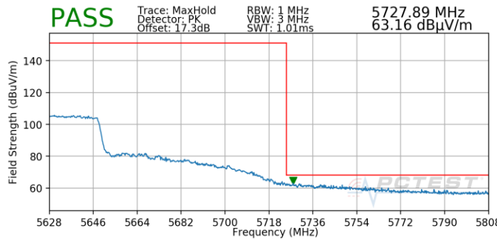
Plot 7-910. (FCC Only) Antenna 4b (Pk, Ch.122, 802.11ac, MCS5)
