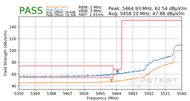
Plot 7-845. Antenna 4b (Pk & Avg, Ch.110, 802.11n, MCS3)
