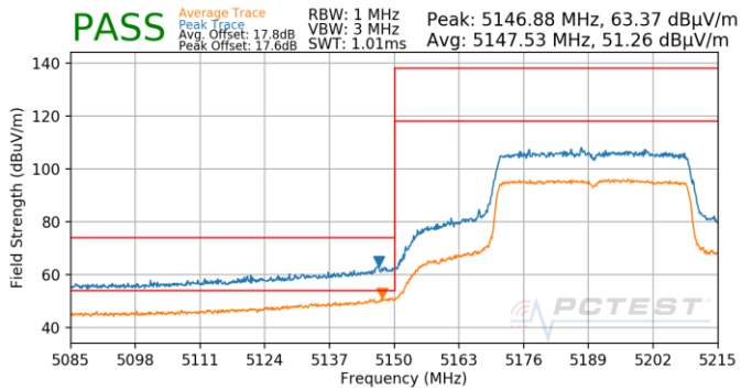
Plot 7-860. Antenna 4b (Pk & Avg, Ch.38, 80.11ax(SU), MCS0)
