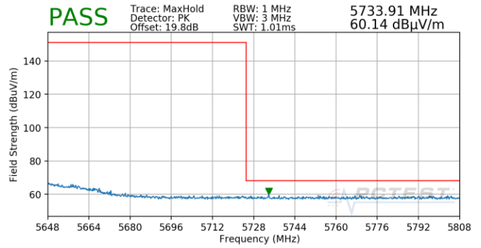
Plot 7-882. (FCC Only) Antenna 4b (Pk, Ch.118, 80.11ax(SU), MCS3)
