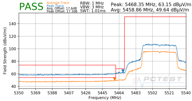
Plot 7-872. Antenna 4b (Pk & Avg, Ch.102, 80.11ax(SU), MCS0)
