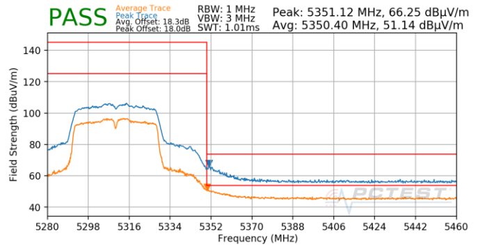
Plot 7-839. Antenna 4b (Pk & Avg, Ch.62, 802.11n, MCS3)
