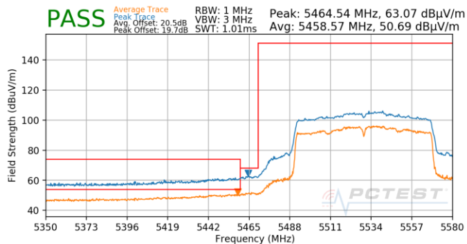
Plot 7-903. Antenna 4b (Pk & Avg, Ch.106, 802.11ac, MCS3)
