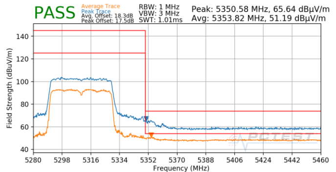
Plot 7-871. Antenna 4b (Pk & Avg, Ch.62, 80.11ax(SU), MCS11)
