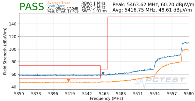
Plot 7-878. (FCC Only) Antenna 4b (Pk & Avg, Ch.118, 80.11ax(SU), MCS0)
