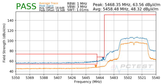
Plot 7-842. Antenna 4b (Pk & Avg, Ch.102, 802.11n, MCS3)
