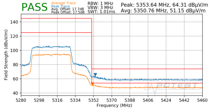
Plot 7-869. Antenna 4b (Pk & Avg, Ch.62, 80.11ax(SU), MCS0)
