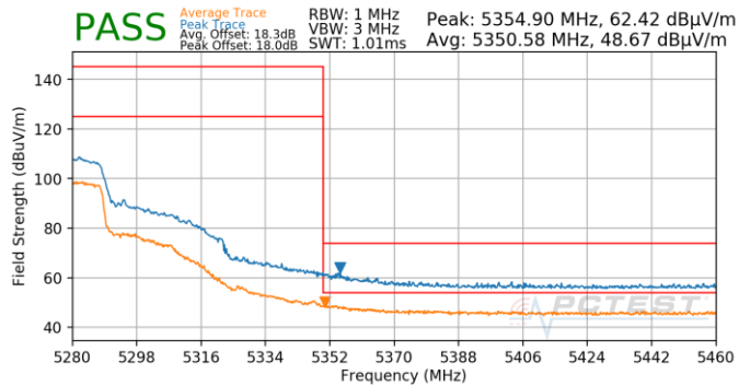
Plot 7-836. Antenna 4b (Pk & Avg, Ch.54, 802.11n, MCS3)
