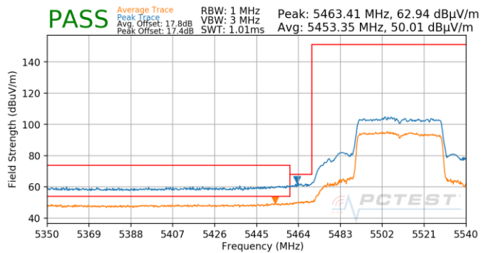
Plot 7-873. Antenna 4b (Pk & Avg, Ch.102, 80.11ax(SU), MCS3)
