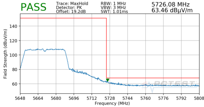
Plot 7-853. Antenna 4b (Pk, Ch.134, 802.11n, MCS5)
