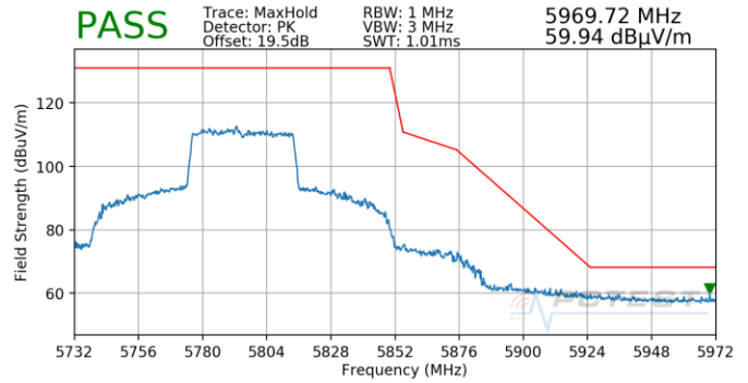
Plot 7-893. Antenna 4b (Pk, Ch.159, 80.11ax(SU), MCS0)
