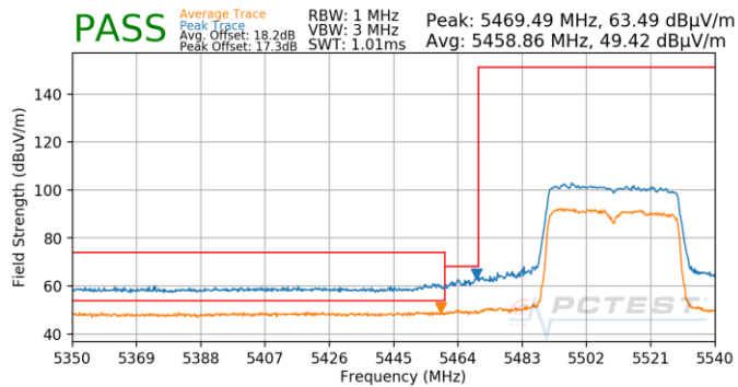
Plot 7-874. Antenna 4b (Pk & Avg, Ch.102, 80.11ax(SU), MCS11)
