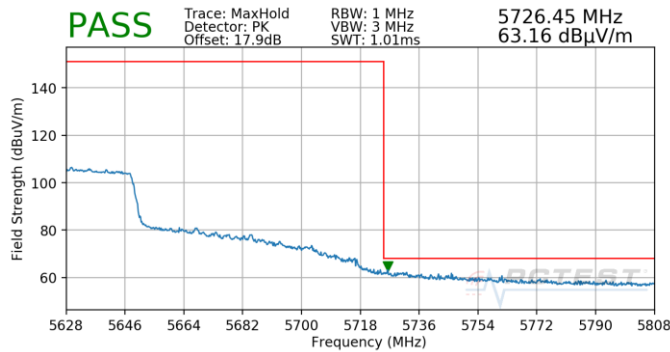
Plot 7-909. (FCC Only) Antenna 4b (Pk, Ch.122, 802.11ac, MCS3)
