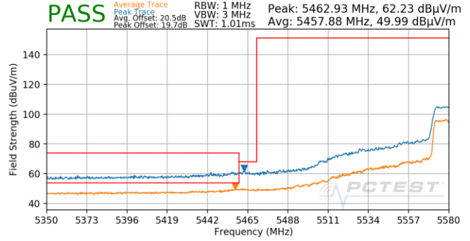
Plot 7-907. (FCC Only) Antenna 4b (Pk & Avg, Ch.122, 802.11ac, MCS5)
