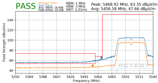
Plot 7-843. Antenna 4b (Pk & Avg, Ch.102, 802.11n, MCS5)
