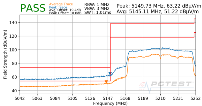
Plot 7-897. Antenna 4b (Pk & Avg, Ch.42, 802.11ac, MCS3)
