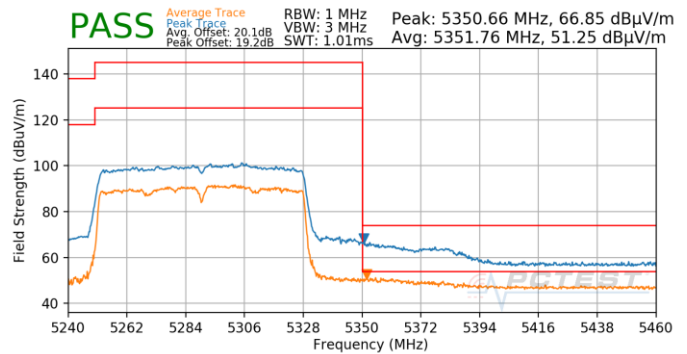
Plot 7-901. Antenna 4b (Pk & Avg, Ch.58, 802.11ac, MCS5)
