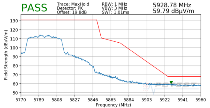
Plot 7-858. Antenna 4b (Pk, Ch.159, 802.11n, MCS3)
