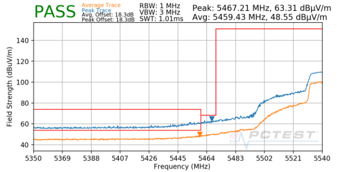
Plot 7-844. Antenna 4b (Pk & Avg, Ch.110, 802.11n, MCS0)
