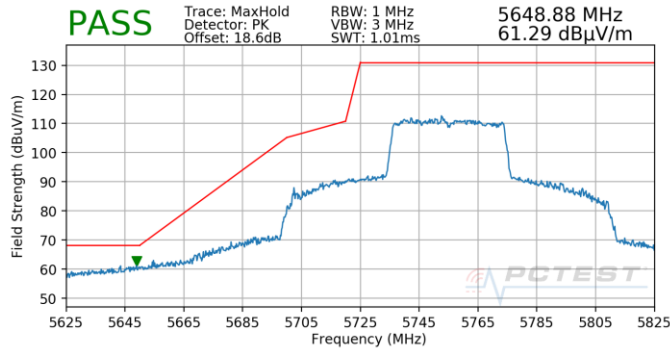
Plot 7-890. Antenna 4b (Pk, Ch.151, 80.11ax(SU), MCS0)
