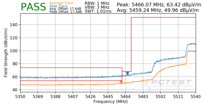
Plot 7-875. Antenna 4b (Pk & Avg, Ch.110, 80.11ax(SU), MCS0)
