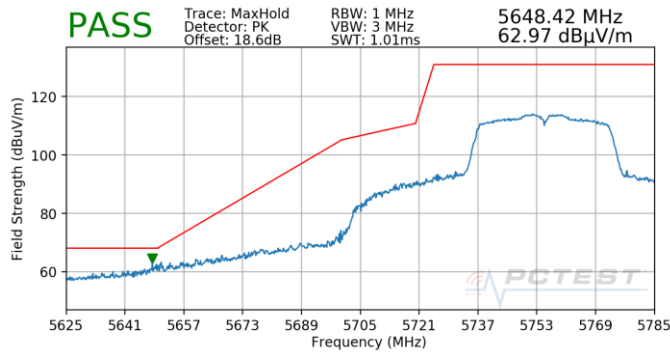
Plot 7-854. Antenna 4b (Pk, Ch.151, 802.11n, MCS0)
