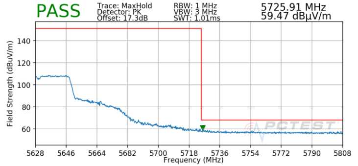
Plot 7-850. (FCC Only) Antenna 4b (Pk, Ch.126, 802.11n, MCS5)
