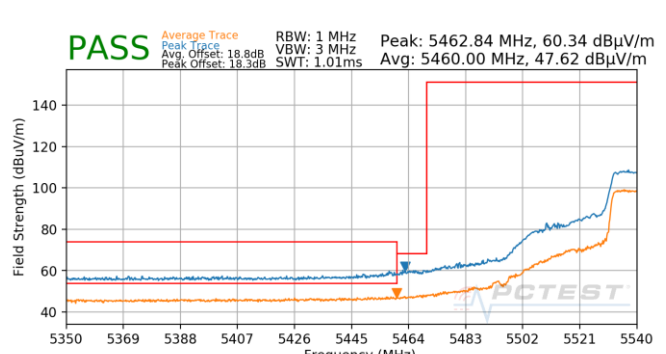
Plot 7-846. Antenna 4b (Pk & Avg, Ch.110, 802.11n, MCS5)
