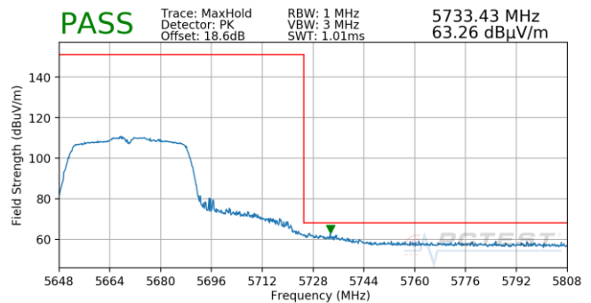
Plot 7-851. Antenna 4b (Pk, Ch.134, 802.11n, MCS0)
