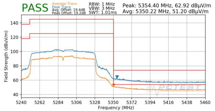
Plot 7-899. Antenna 4b (Pk & Avg, Ch.58, 802.11ac, MCS0)
