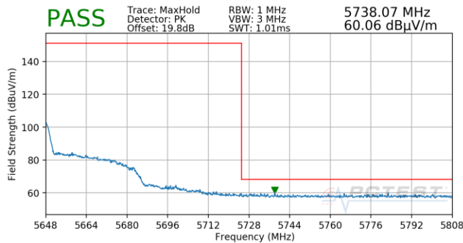
Plot 7-885. (FCC Only) Antenna 4b (Pk, Ch.126, 80.11ax(SU), MCS3)
