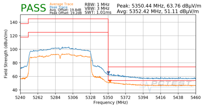
Plot 7-900. Antenna 4b (Pk & Avg, Ch.58, 802.11ac, MCS3)
