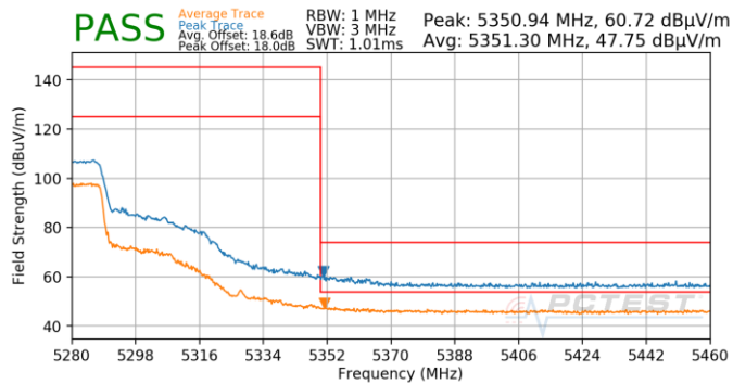
Plot 7-837. Antenna 4b (Pk & Avg, Ch.54, 802.11n, MCS5)
