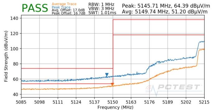
Plot 7-864. Antenna 4b (Pk & Avg, Ch.46, 80.11ax(SU), MCS3)
