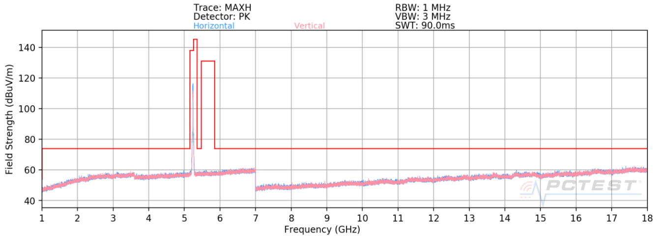
Plot 7-557. Radiated Spurious Emissions above 1GHz CDD (802.11n – Ch. 48)
