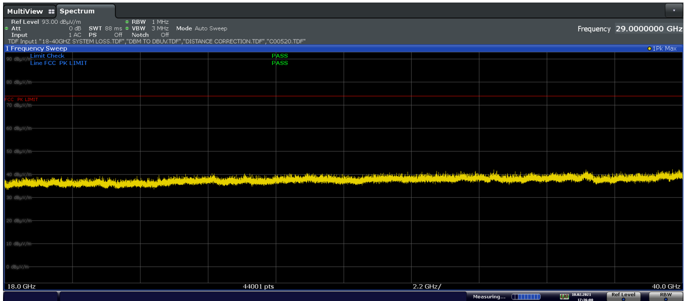
Plot 7-565. Radiated Spurious Emissions 18GHz - 40GHz CDD (802.11n – Ch.116, Pol. H)
