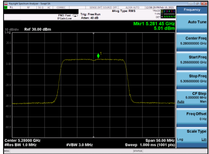
Plot 7-340. PSD CDD Antenna 4b (20MHz BW 802.11ax(SU) – Ch. 56, MCS0)
