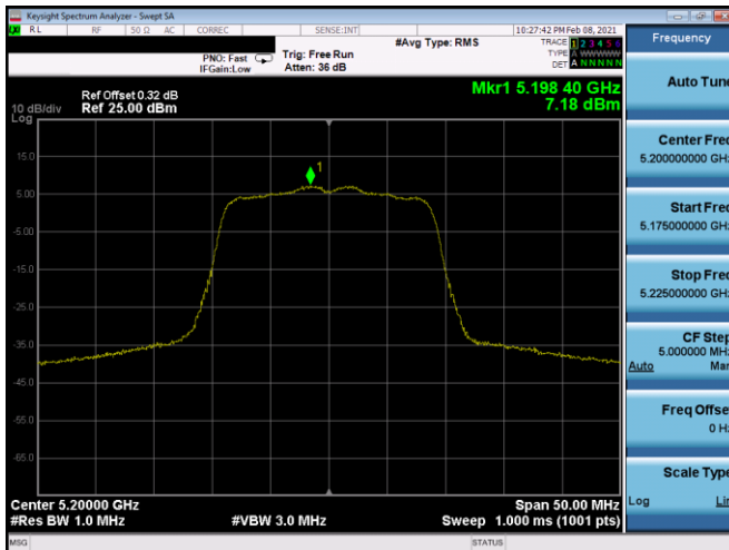
Plot 7-362. PSD CDD Antenna 4b (20MHz BW 802.11n – Ch. 40, MCS11)
