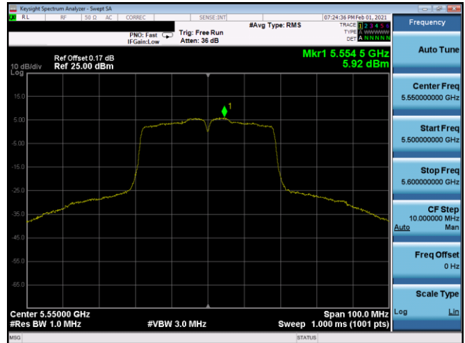
Plot 7-353. PSD CDD Antenna 5b (40MHz BW 802.11n – Ch. 110, MCS8)
