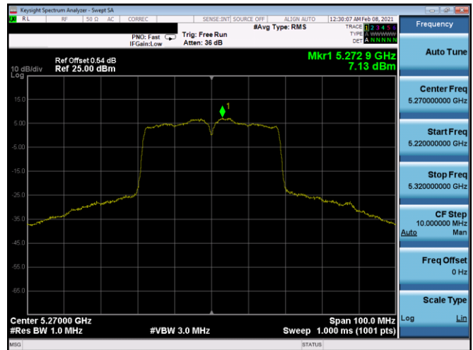
Plot 7-378. PSD CDD Antenna 4b (40MHz BW 802.11n – Ch. 54, MCS11)
