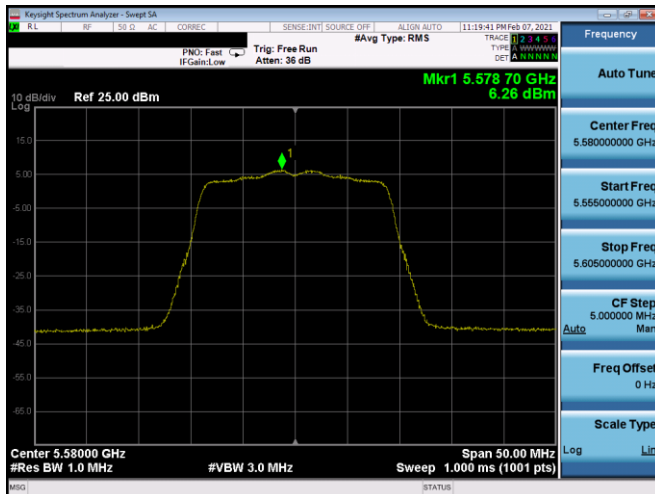
Plot 7-350. PSD CDD Antenna 4b (20MHz BW 802.11n – Ch. 116, MCS8)
