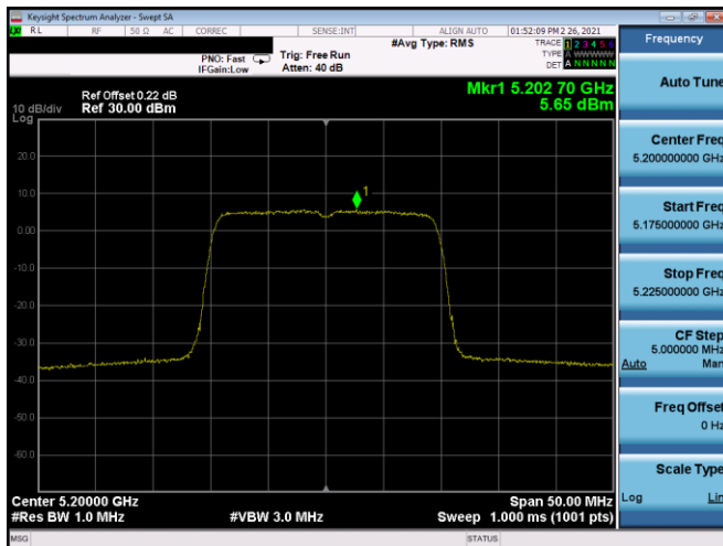
Plot 7-363. PSD CDD Antenna 5b (20MHz BW 802.11ax(SU) – Ch. 40, MCS3)
