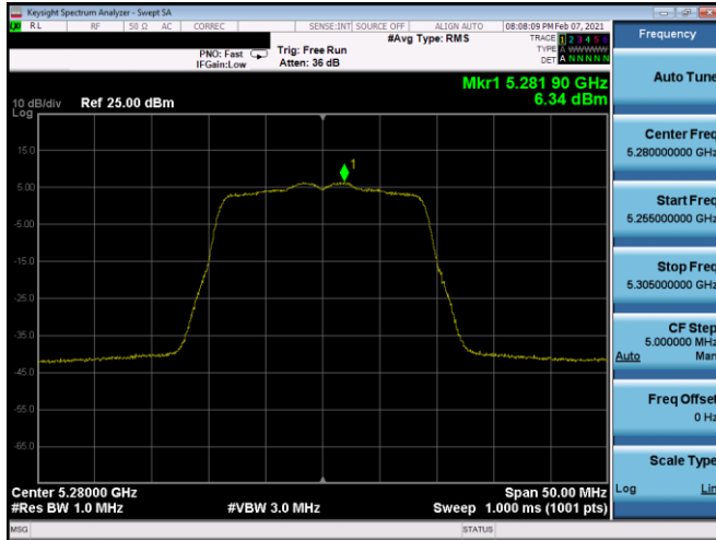
Plot 7-337. PSD CDD Antenna 5b (20MHz BW 802.11n – Ch. 56, MCS8)
