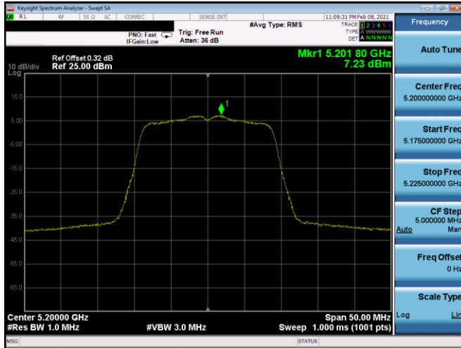
Plot 7-361. PSD CDD Antenna 5b (20MHz BW 802.11n – Ch. 40, MCS11)
