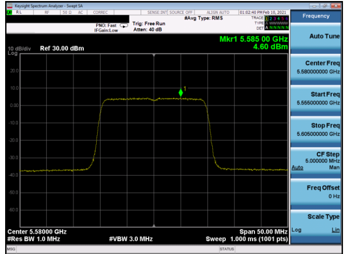
Plot 7-352. PSD CDD Antenna 4b (20MHz BW 802.11ax(SU) – Ch. 116, MCS0)
