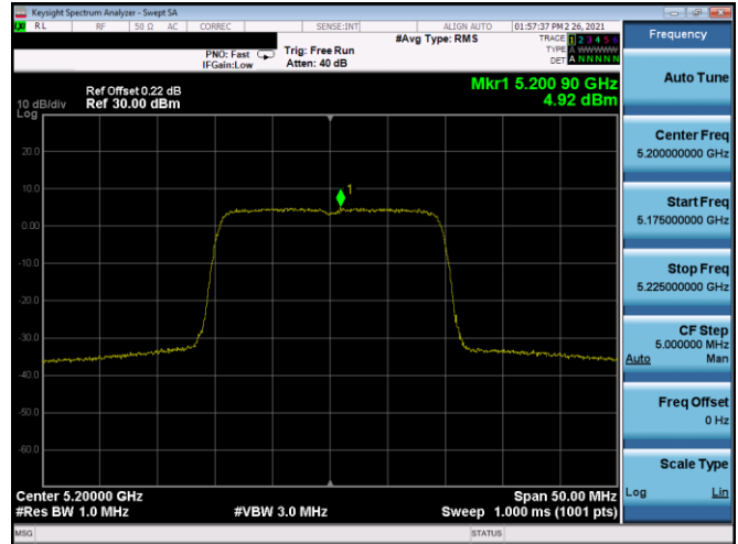
Plot 7-364. PSD CDD Antenna 4b (20MHz BW 802.11ax(SU) – Ch. 40, MCS3)
