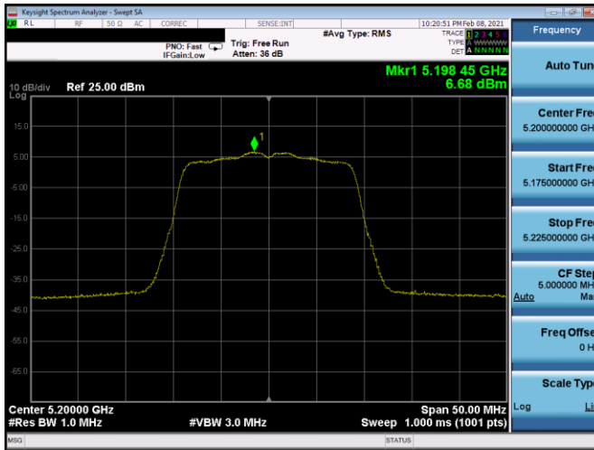
Plot 7-326. PSD CDD Antenna 4b (20MHz BW 802.11n – Ch. 40, MCS8)
