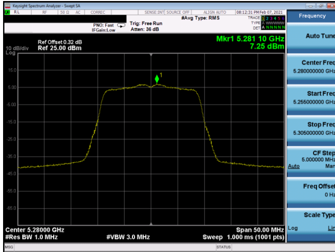
Plot 7-373. PSD CDD Antenna 5b (20MHz BW 802.11n – Ch. 56, MCS11)
