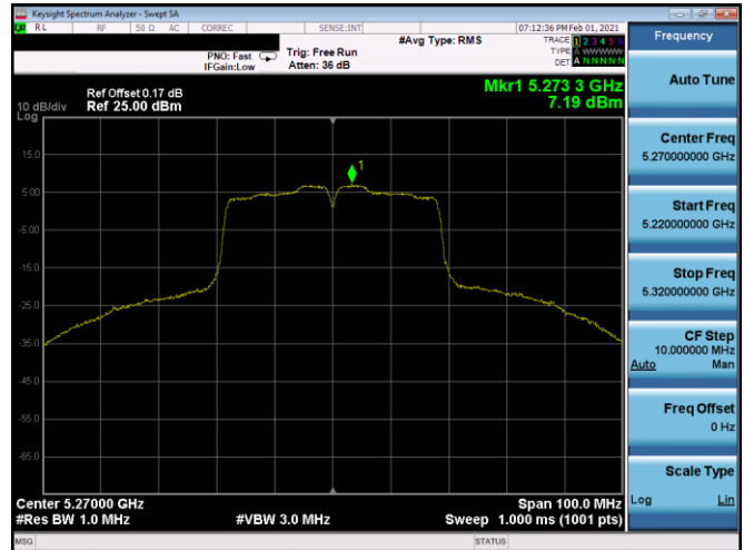
Plot 7-341. PSD CDD Antenna 5b (40MHz BW 802.11n – Ch. 54, MCS8)
