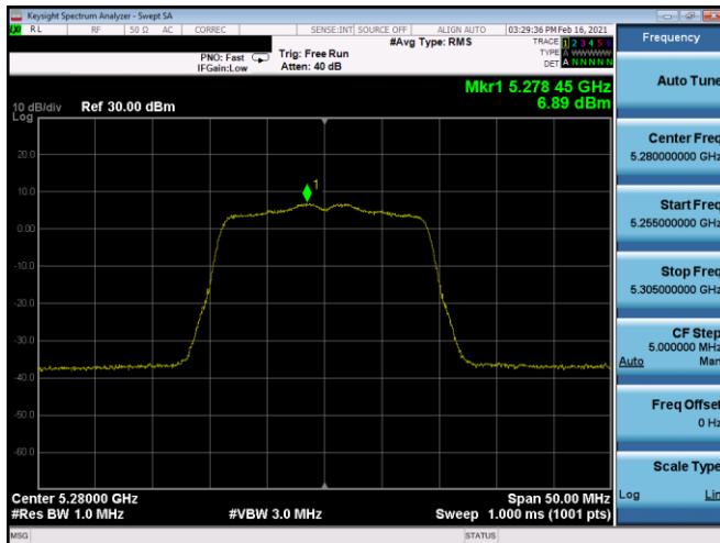
Plot 7-338. PSD CDD Antenna 4b (20MHz BW 802.11n – Ch. 56, MCS8)
