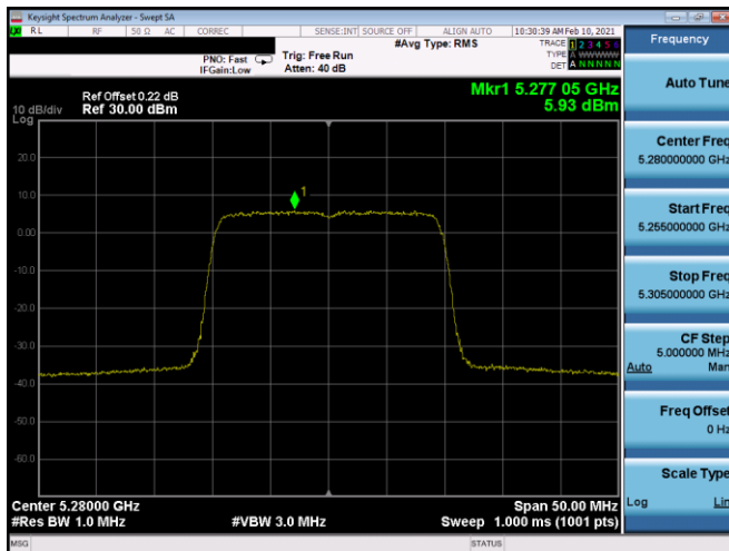
Plot 7-375. PSD CDD Antenna 5b (20MHz BW 802.11ax(SU) – Ch. 56, MCS3)
