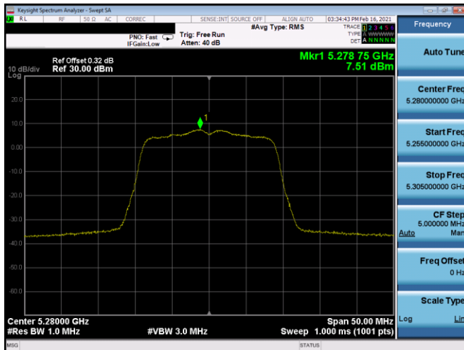
Plot 7-374. PSD CDD Antenna 4b (20MHz BW 802.11n – Ch. 56, MCS11)
