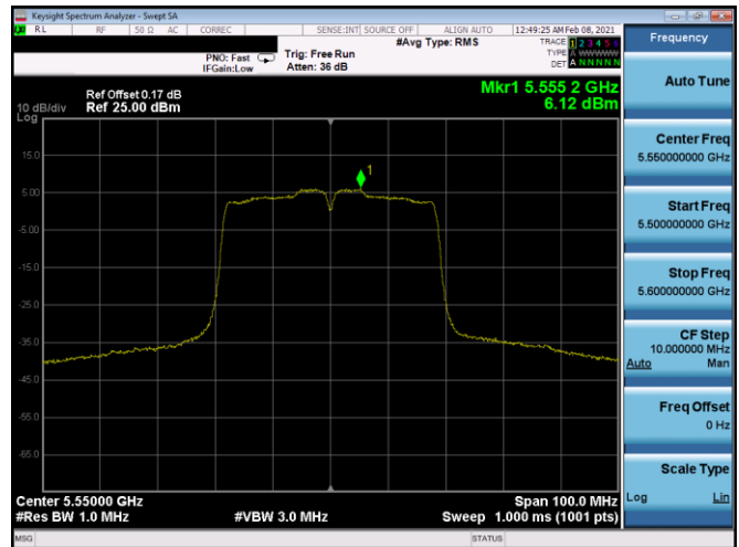
Plot 7-354. PSD CDD Antenna 4b (40MHz BW 802.11n – Ch. 110, MCS8)
