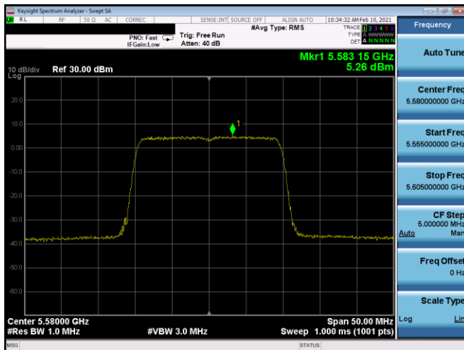
Plot 7-351. PSD CDD Antenna 5b (20MHz BW 802.11ax(SU) – Ch. 116, MCS0)
