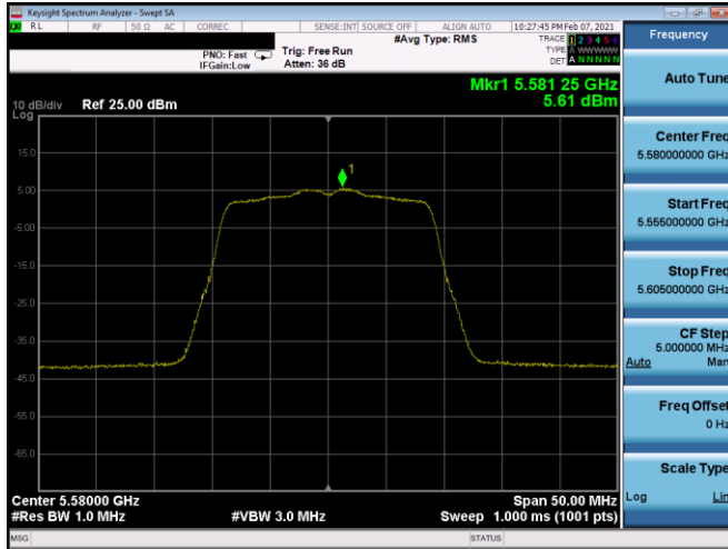
Plot 7-349. PSD CDD Antenna 5b (20MHz BW 802.11n – Ch. 116, MCS8)
