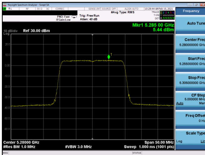
Plot 7-339. PSD CDD Antenna 5b (20MHz BW 802.11ax(SU) – Ch. 56, MCS0)
