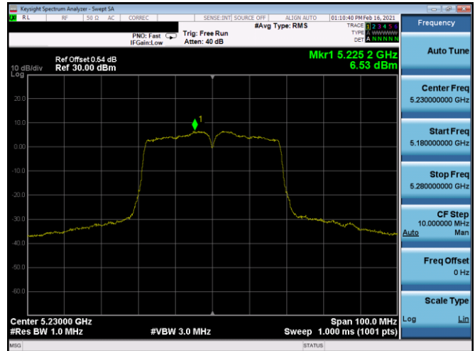
Plot 7-365. PSD CDD Antenna 5b (40MHz BW 802.11n – Ch. 46, MCS11)
