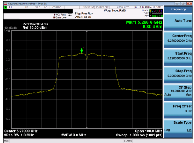
Plot 7-377. PSD CDD Antenna 5b (40MHz BW 802.11n – Ch. 54, MCS11)
