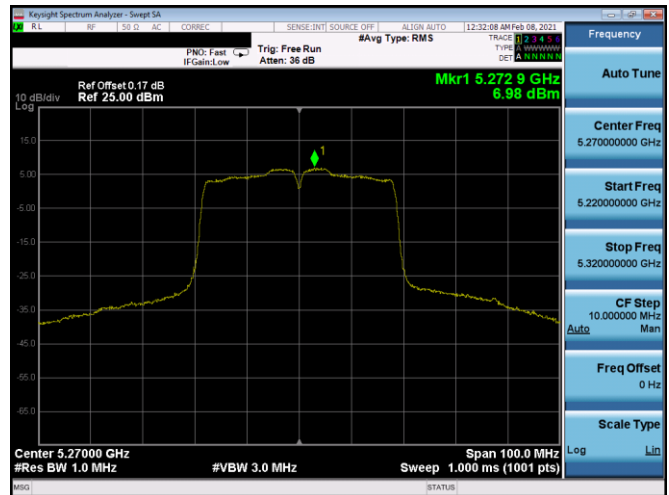
Plot 7-342. PSD CDD Antenna 4b (40MHz BW 802.11n – Ch. 54, MCS8)
