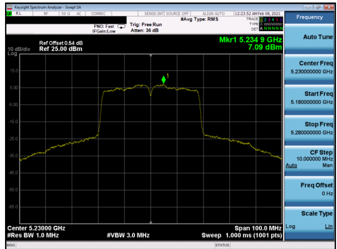
Plot 7-366. PSD CDD Antenna 4b (40MHz BW 802.11n – Ch. 46, MCS11)
