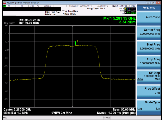
Plot 7-376. PSD CDD Antenna 4b (20MHz BW 802.11ax(SU) – Ch. 56, MCS3)
