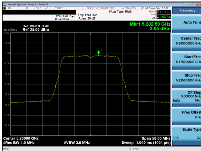
Plot 7-229. ISED PSD Antenna 5b (20MHz BW 11n – Ch.40, MCS5)
