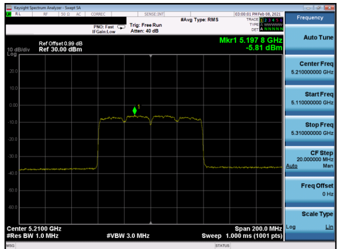
Plot 7-234. ISED PSD Antenna 5b (80MHz BW 11ax(SU) – Ch.42, MCS11)
