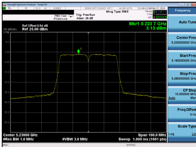
Plot 7-231. ISED PSD Antenna 5b (40MHz BW 11n – Ch.46, MCS5)
