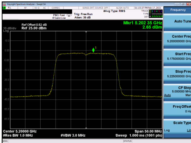
Plot 7-230. ISED PSD Antenna 5b (20MHz BW 11ax(SU) – Ch.40, MCS11)
