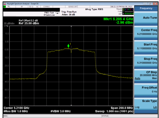
Plot 7-239. PSD Antenna 4b (80MHz BW 802.11ax – Ch. 42, MCS0)
