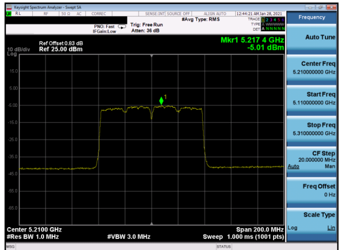
Plot 7-233. ISED PSD Antenna 5b (80MHz BW 11ac – Ch.42, MCS5)
