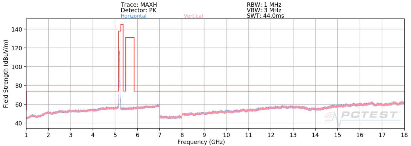
Plot 7-1. RSE above 1GHz CDD (11ax(SU) – Ch.40)
