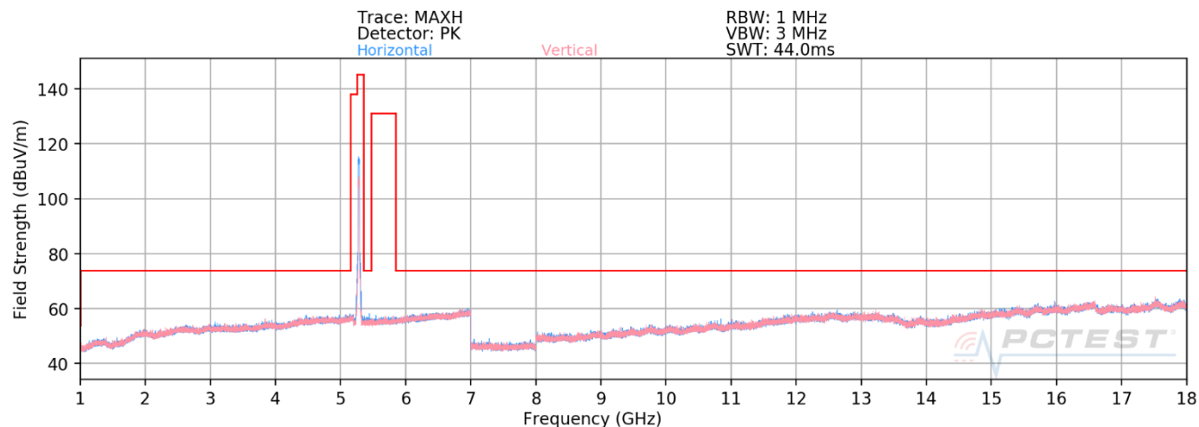
Plot 7-2. RSE above 1GHz CDD (11ax(SU) – Ch.56)
