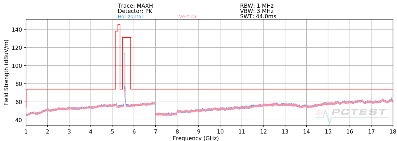
Plot 7-3. RSE above 1GHz CDD (11ax(SU) – Ch.116)
