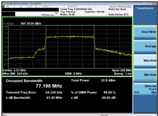
Plot 7-36. 26dB BW & 99% OBW Antenna 5b (80MHz BW 802.11ax(SU) – Ch. 106, MCS3)
