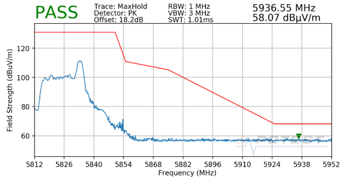
Plot 7-482. Antenna 4b (Pk, RU26, Index 8, Ch.165, MCS11)
