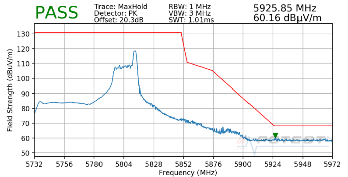
Plot 7-518. Antenna 4b (Pk, RU26, Index 36, Ch.155, MCS11)
