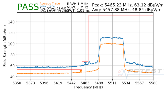
Plot 7-456. Antenna 5b (Pk & Avg, RU484, Index 65, Ch.102, MCS11)
