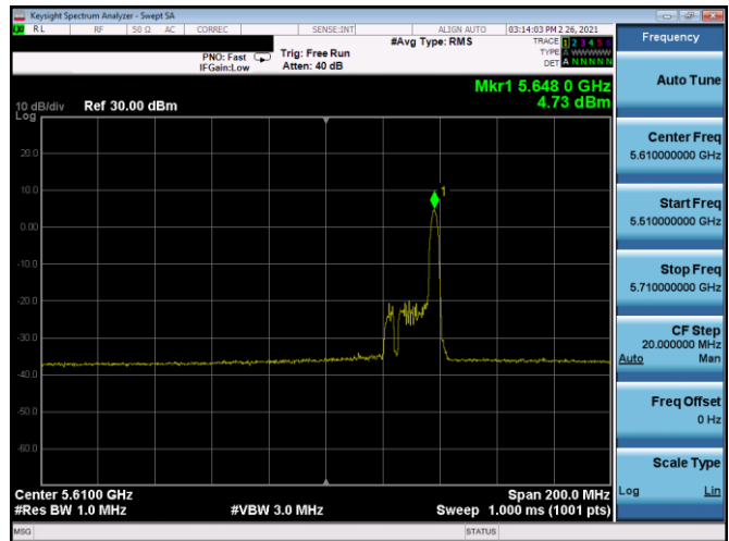
Plot 7-286. PSD CDD Antenna 4b (80MHz BW 11ax Index 36 – RU26 – Ch.122)
