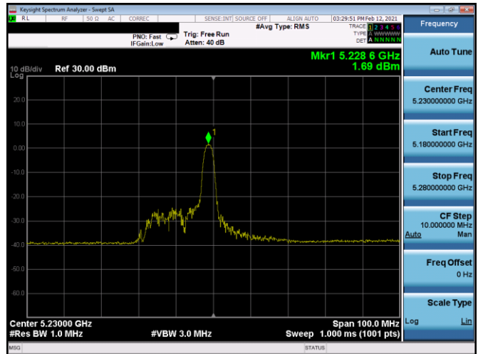
Plot 7-323. ISD PSD SDM Antenna 5b (40MHz BW 11ax Index 8 - RU26 - Ch.46)
