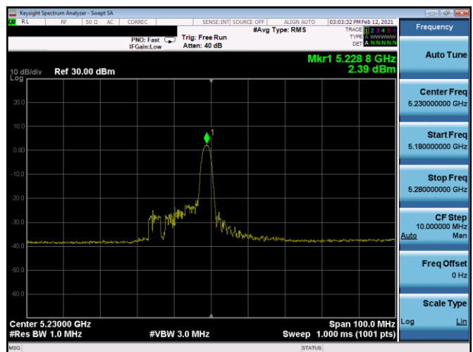
Plot 7-324. ISD PSD SDM Antenna 4b (40MHz BW 11ax Index 8 - RU26 - Ch.46)
