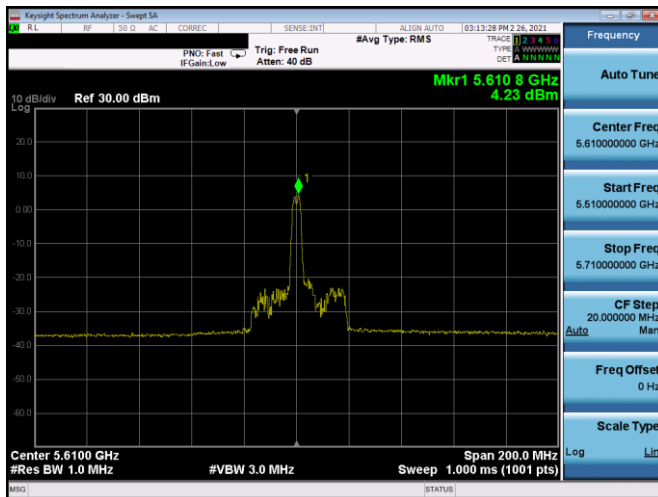
Plot 7-284. PSD CDD Antenna 4b (80MHz BW 11ax Index 18 – RU26 – Ch.122)
