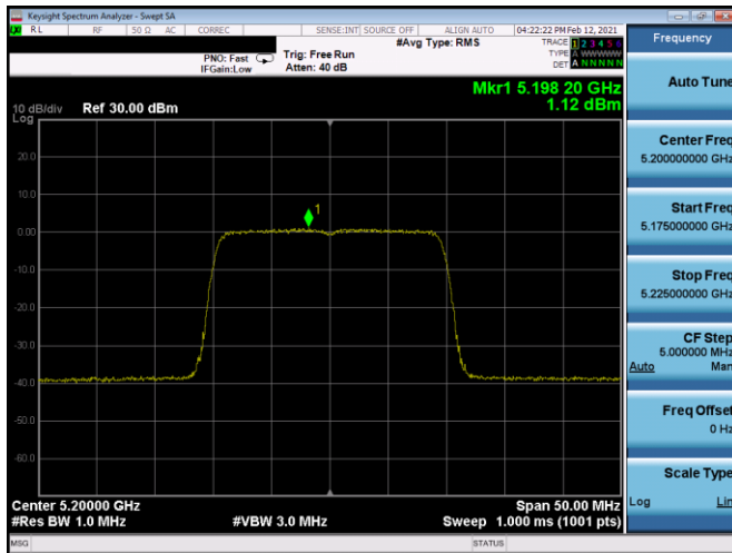
Plot 7-319. ISD PSD SDM Antenna 5b (20MHz BW 11ax- RU242 - Ch.40)
