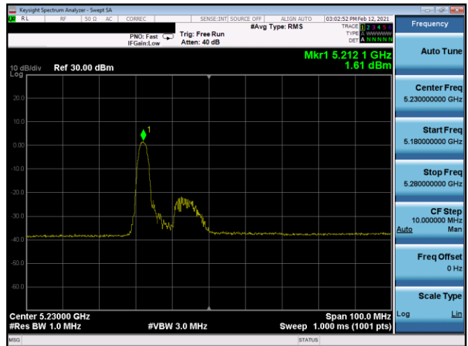
Plot 7-322. ISD PSD SDM Antenna 4b (40MHz BW 11ax Index 0 - RU26 - Ch.46)
