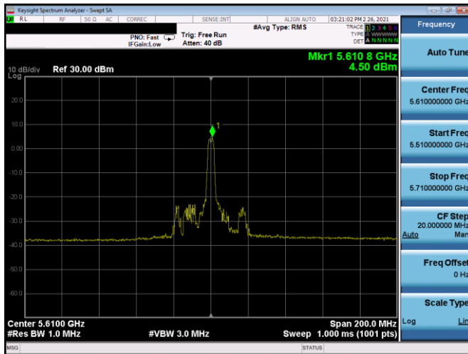
Plot 7-283. PSD CDD Antenna 5b (80MHz BW 11ax Index 18 – RU26 – Ch.122)
