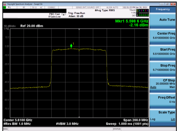
Plot 7-287. PSD CDD Antenna 5b (80MHz BW 11ax – RU996 – Ch.122)
