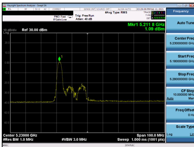
Plot 7-321. ISD PSD SDM Antenna 5b (40MHz BW 11ax Index 0 - RU26 - Ch.46)
