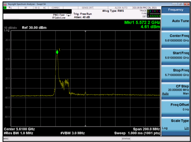
Plot 7-281. PSD CDD Antenna 5b (80MHz BW 11ax Index 0 – RU26 – Ch.122)
