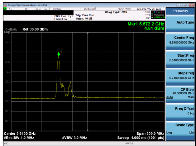
Plot 7-282. PSD CDD Antenna 4b (80MHz BW 11ax Index 0 – RU26 – Ch.122)
