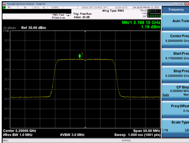
Plot 7-320. ISD PSD SDM Antenna 4b (20MHz BW 11ax- RU242 - Ch.40)
