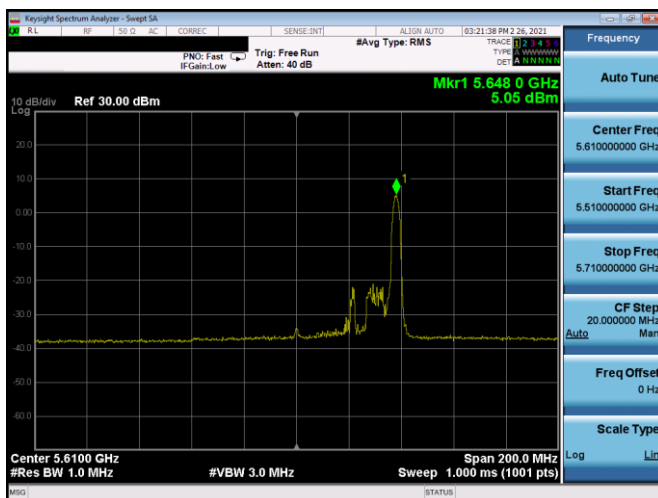
Plot 7-285. PSD CDD Antenna 5b (80MHz BW 11ax Index 36 – RU26 – Ch.122)
