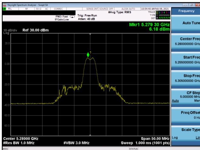
Plot 7-243. PSD CDD Antenna 5b (20MHz BW 11ax Index 4 – RU26 – Ch.56)
