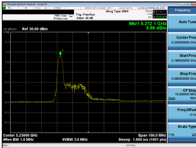
Plot 7-225. PSD CDD Antenna 5b (40MHz BW 11ax Index 0 - RU26 - Ch.46)
