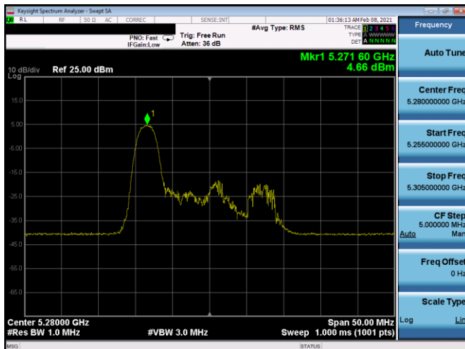
Plot 7-242. PSD CDD Antenna 4b (20MHz BW 11ax Index 0 – RU26 – Ch.56)
