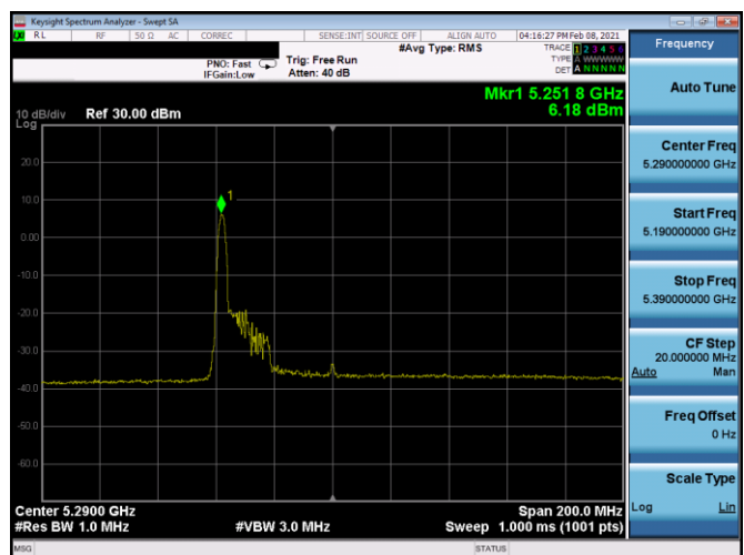
Plot 7-258. PSD CDD Antenna 4b (80MHz BW 11ax Index 0 – RU26 – Ch.58)
