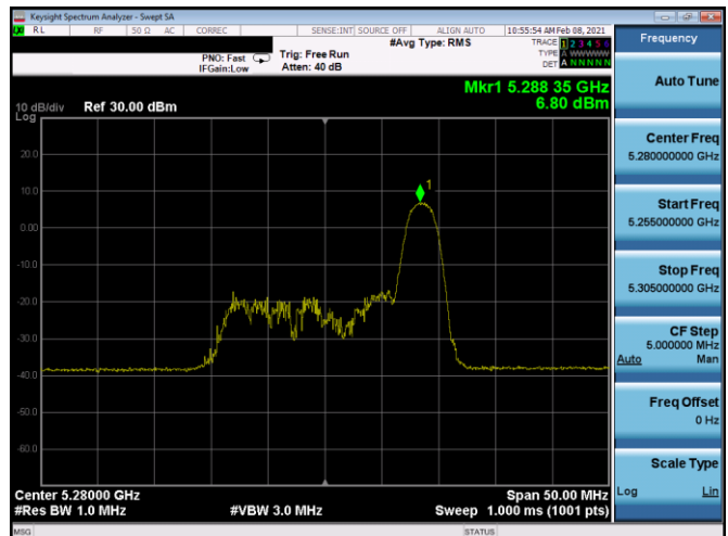
Plot 7-245. PSD CDD Antenna 5b (20MHz BW 11ax Index 8 – RU26 – Ch.56)
