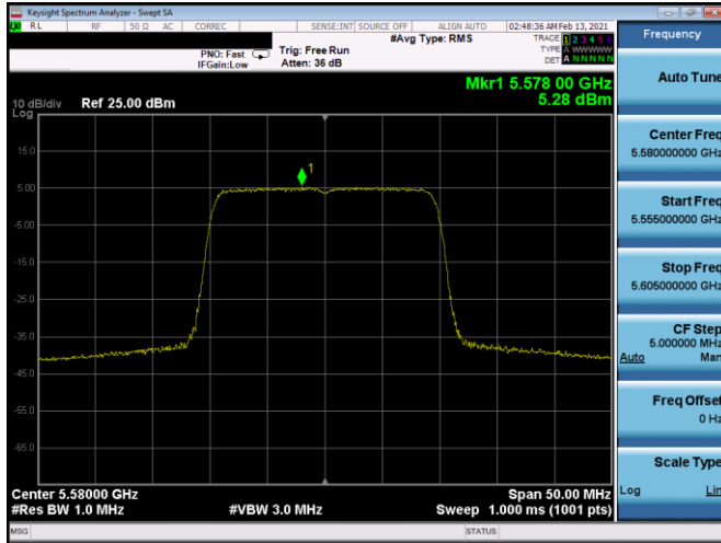
Plot 7-271. PSD CDD Antenna 5b (20MHz BW 11ax- RU242 - Ch.116)
