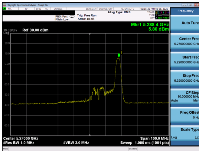
Plot 7-254. PSD CDD Antenna 4b (40MHz BW 11ax Index 17 – RU26 – Ch.54)
