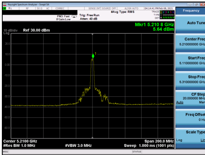
Plot 7-236. PSD CDD Antenna 4b (80MHz BW 11ax Index 18 – RU26 – Ch.42)
