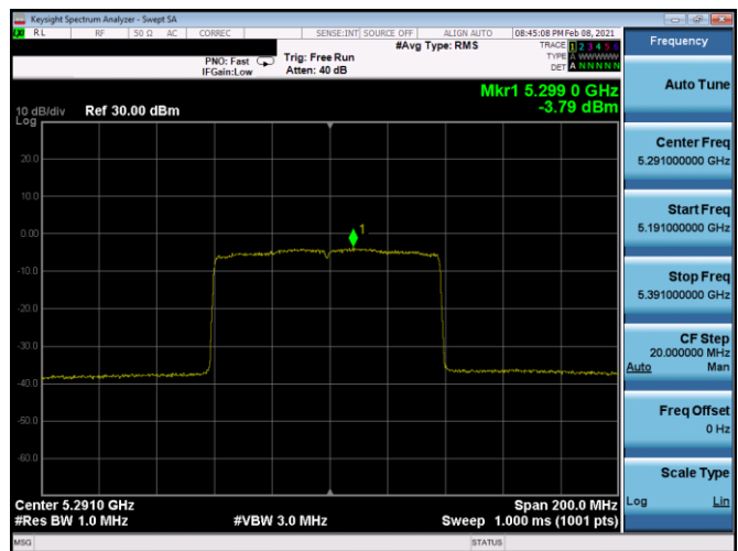
Plot 7-264. PSD CDD Antenna 4b (80MHz BW 11ax – RU996 – Ch.58)
