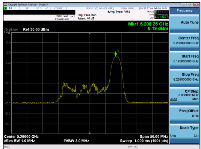
Plot 7-221. PSD CDD Antenna 5b (20MHz BW 11ax Index 8– RU26 – Ch.40)
