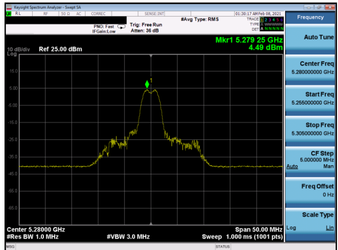
Plot 7-244. PSD CDD Antenna 4b (20MHz BW 11ax Index 4 – RU26 – Ch.56)
