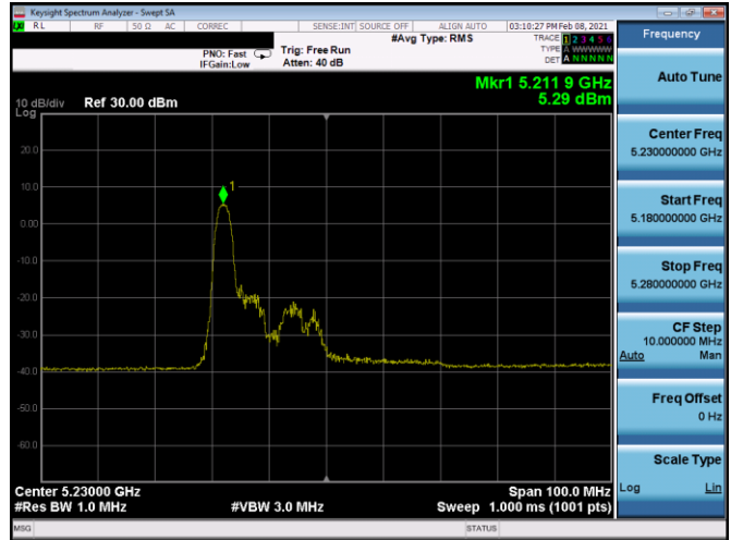
Plot 7-226. PSD CDD Antenna 4b (40MHz BW 11ax Index 0 - RU26 - Ch.46)
