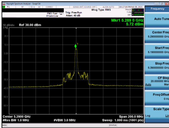
Plot 7-260. PSD CDD Antenna 4b (80MHz BW 11ax Index 18 – RU26 – Ch.58)
