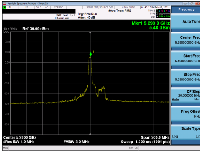
Plot 7-259. PSD CDD Antenna 5b (80MHz BW 11ax Index 18 – RU26 – Ch.58)
