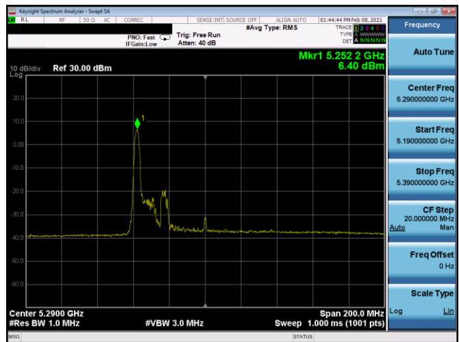
Plot 7-257. PSD CDD Antenna 5b (80MHz BW 11ax Index 0 – RU26 – Ch.58)
