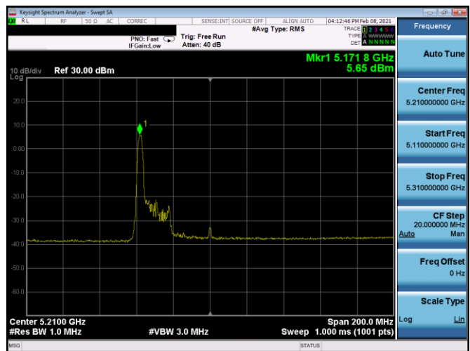
Plot 7-234. PSD CDD Antenna 4b (80MHz BW 11ax Index 0 – RU26 – Ch.42)
