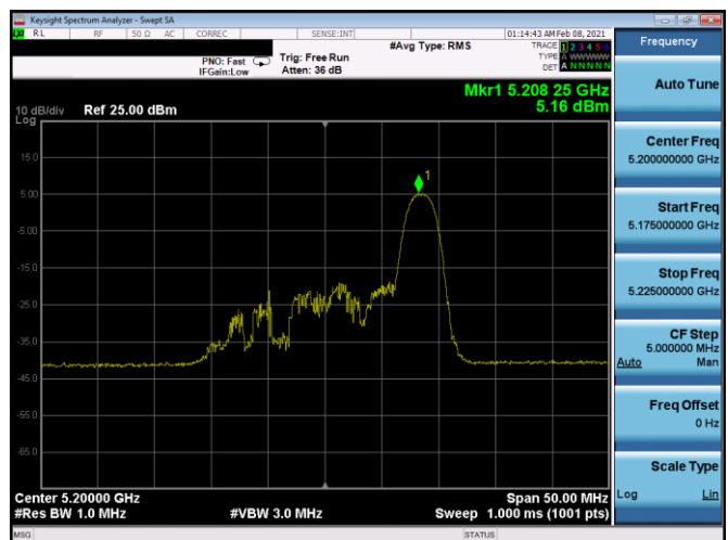
Plot 7-222. PSD CDD Antenna 4b (20MHz BW 11ax Index 8– RU26 – Ch.40)
