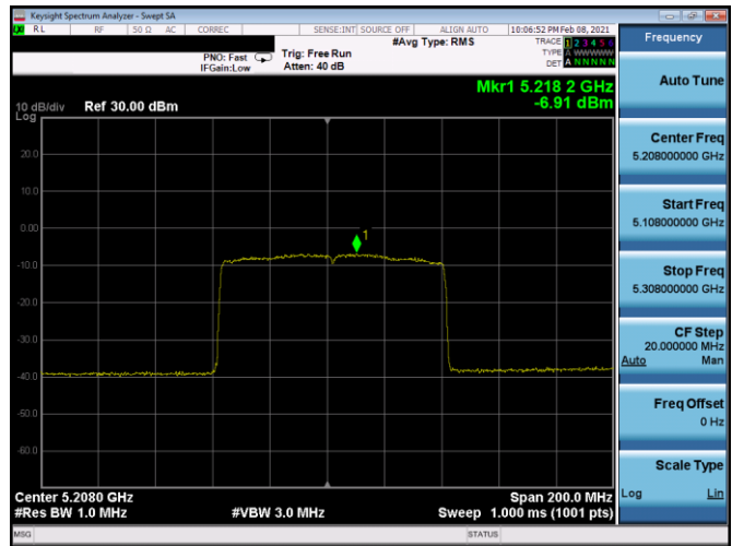
Plot 7-239. PSD CDD Antenna 5b (80MHz BW 11ax – RU996 – Ch.42)
