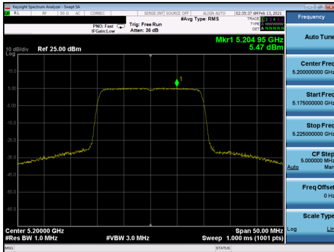
Plot 7-224. PSD CDD Antenna 4b (20MHz BW 11ax- RU242 - Ch.40)
