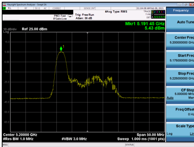
Plot 7-218. PSD CDD Antenna 4b (20MHz BW 11ax Index 0 – RU26 – Ch.40)
