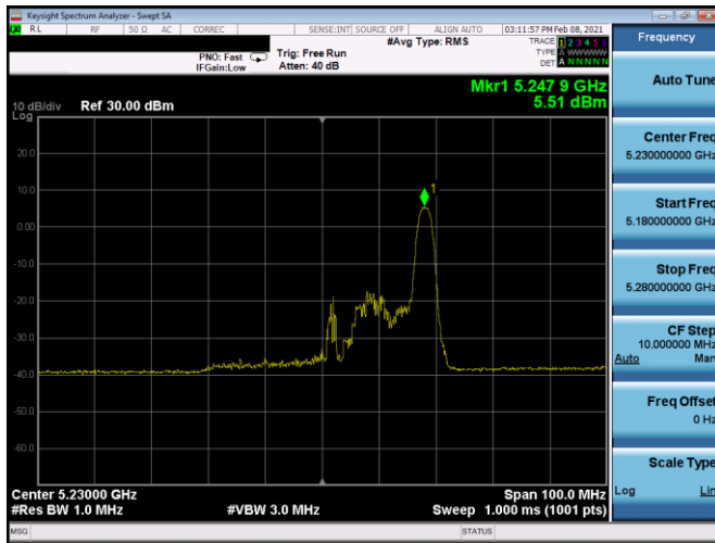
Plot 7-230. PSD CDD Antenna 4b (40MHz BW 11ax Index 17 – RU26 – Ch.46)
