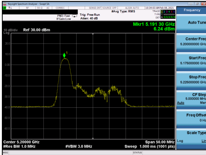
Plot 7-217. PSD CDD Antenna 5b (20MHz BW 11ax Index 0 – RU26 – Ch.40)
