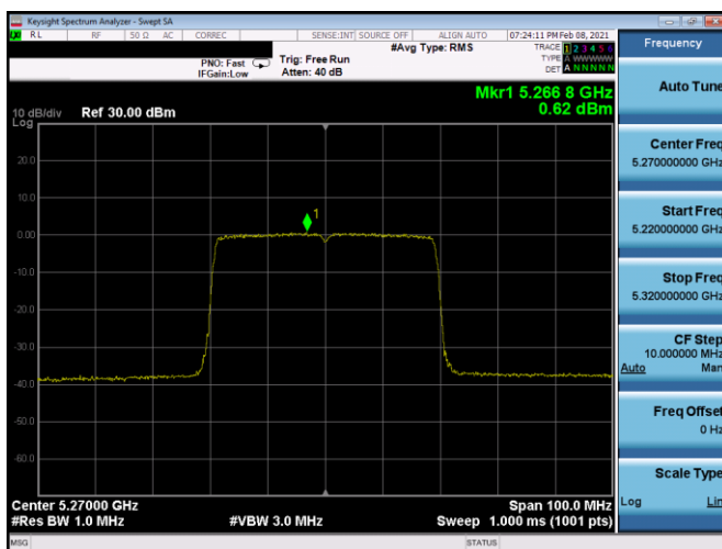
Plot 7-255. PSD CDD Antenna 5b (40MHz BW 11ax – RU484 – Ch.54)
