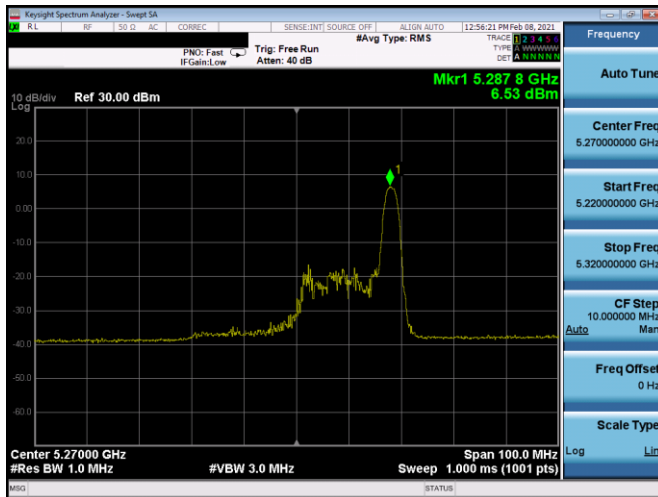
Plot 7-253. PSD CDD Antenna 5b (40MHz BW 11ax Index 17 – RU26 – Ch.54)
