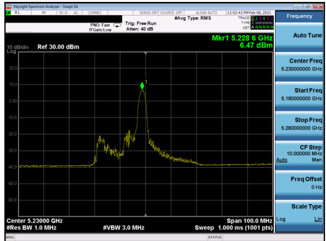
Plot 7-227. PSD CDD Antenna 5b (40MHz BW 11ax Index 8 - RU26 - Ch.46)
