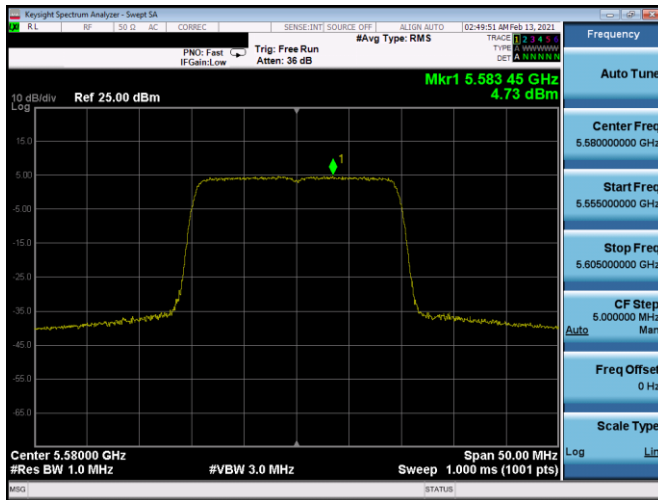
Plot 7-272. PSD CDD Antenna 4b (20MHz BW 11ax- RU242 - Ch.116)
