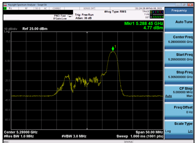
Plot 7-246. PSD CDD Antenna 4b (20MHz BW 11ax Index 8 – RU26 – Ch.56)
