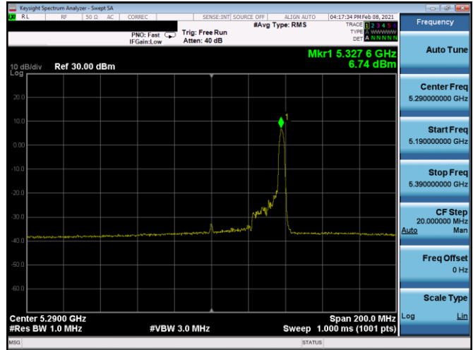
Plot 7-262. PSD CDD Antenna 4b (80MHz BW 11ax Index 36 – RU26 – Ch.58)
