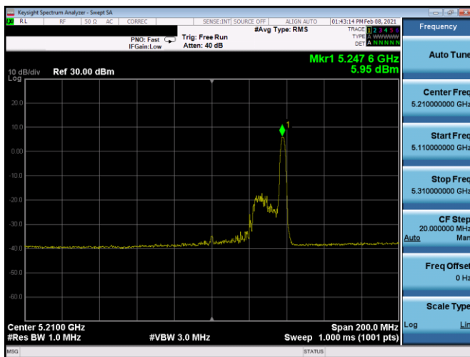
Plot 7-237. PSD CDD Antenna 5b (80MHz BW 11ax Index 36 – RU26 – Ch.42)
