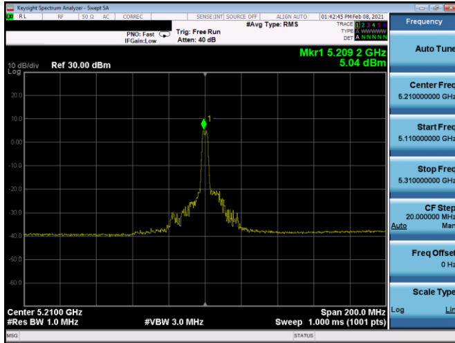
Plot 7-235. PSD CDD Antenna 5b (80MHz BW 11ax Index 18 – RU26 – Ch.42)
