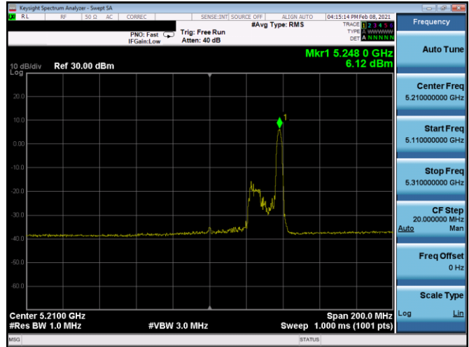
Plot 7-238. PSD CDD Antenna 4b (80MHz BW 11ax Index 36 – RU26 – Ch.42)
