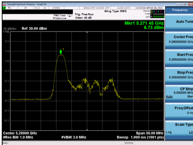
Plot 7-241. PSD CDD Antenna 5b (20MHz BW 11ax Index 0 – RU26 – Ch.56)
