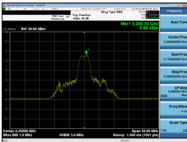
Plot 7-219. PSD CDD Antenna 5b (20MHz BW 11ax Index 4 – RU26 – Ch.40)
