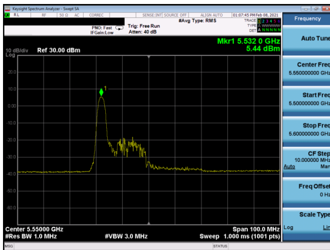
Plot 7-273. PSD CDD Antenna 5b (40MHz BW 11ax Index 0 - RU26 - Ch.110)
