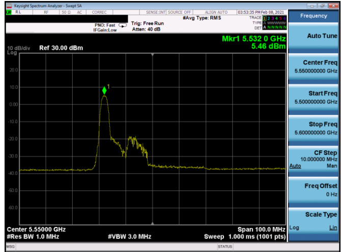
Plot 7-274. PSD CDD Antenna 4b (40MHz BW 11ax Index 0 - RU26 - Ch.110)
