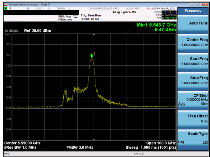
Plot 7-275. PSD CDD Antenna 5b (40MHz BW 11ax Index 8 - RU26 - Ch.110)
