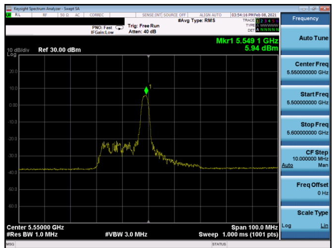
Plot 7-276. PSD CDD Antenna 4b (40MHz BW 11ax Index 8 - RU26 - Ch.110)
