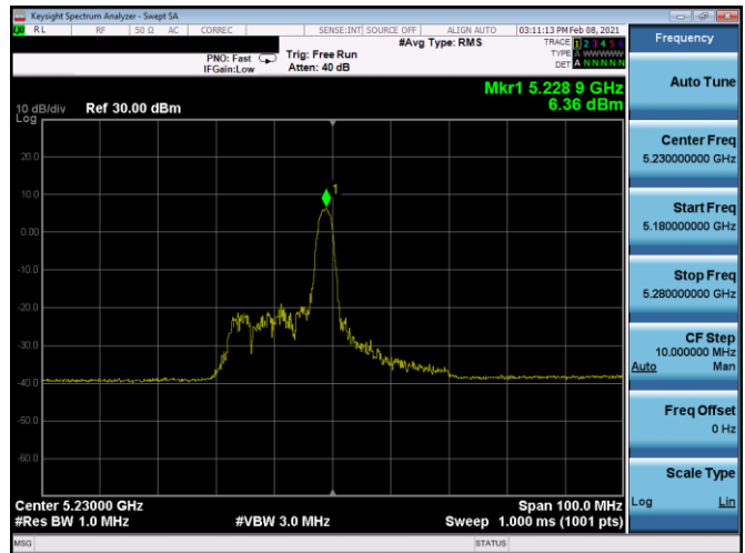
Plot 7-228. PSD CDD Antenna 4b (40MHz BW 11ax Index 8 - RU26 - Ch.46)
