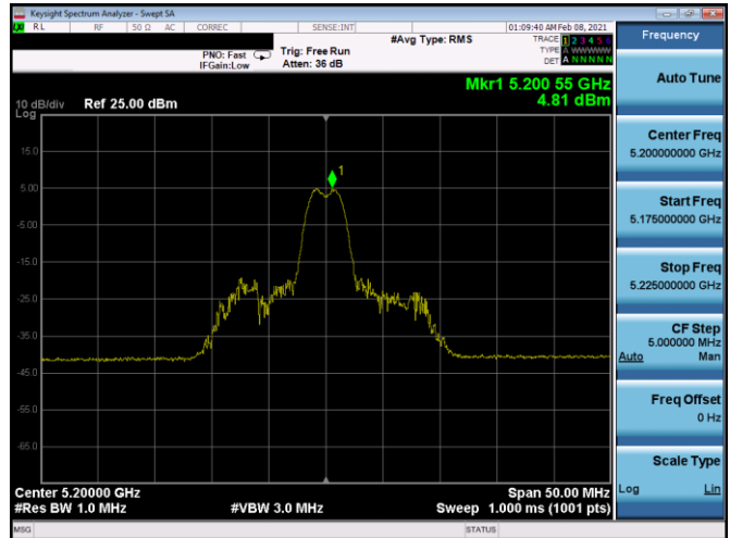
Plot 7-220. PSD CDD Antenna 4b (20MHz BW 11ax Index 4 – RU26 – Ch.40)
