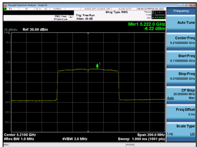
Plot 7-240. PSD CDD Antenna 4b (80MHz BW 11ax – RU996 – Ch.42)
