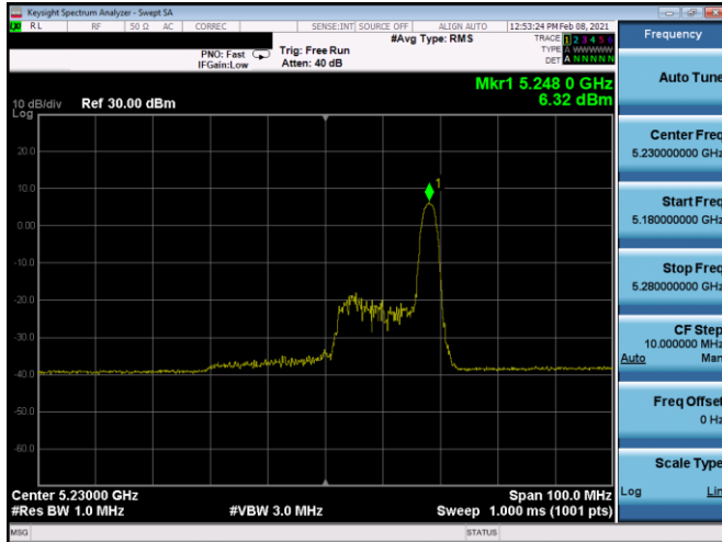
Plot 7-229. PSD CDD Antenna 5b (40MHz BW 11ax Index 17 – RU26 – Ch.46)
