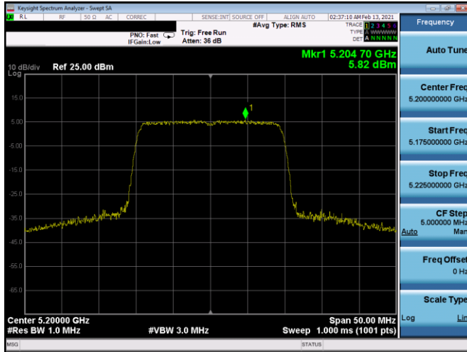
Plot 7-223. PSD CDD Antenna 5b (20MHz BW 11ax- RU242 - Ch.40)
