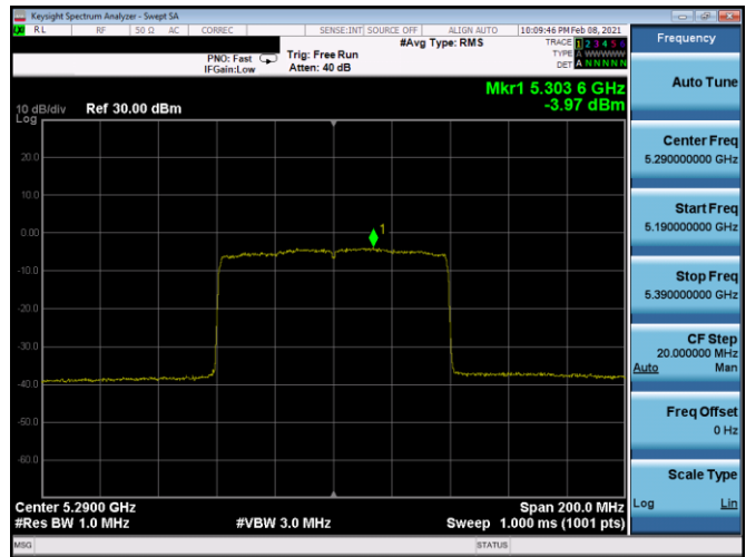
Plot 7-263. PSD CDD Antenna 5b (80MHz BW 11ax – RU996 – Ch.58)
