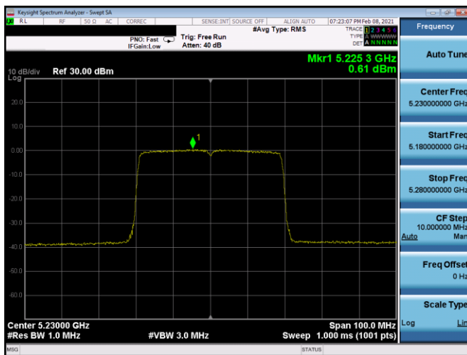
Plot 7-231. PSD CDD Antenna 5b (40MHz BW 11ax – RU484 – Ch.46)
