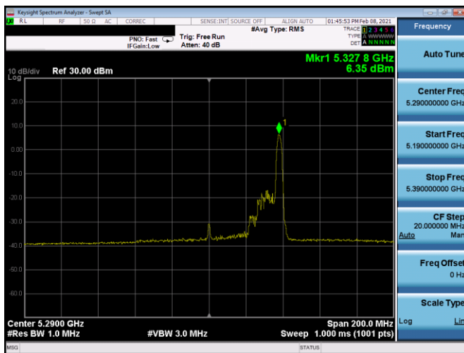
Plot 7-261. PSD CDD Antenna 5b (80MHz BW 11ax Index 36 – RU26 – Ch.58)
