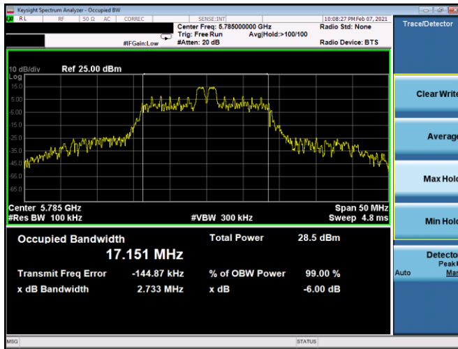
Plot 7-86. 6dB BW & 99% OBW Antenna 4b (20MHz BW 11ax Index 4 – RU26 – Ch.157)
