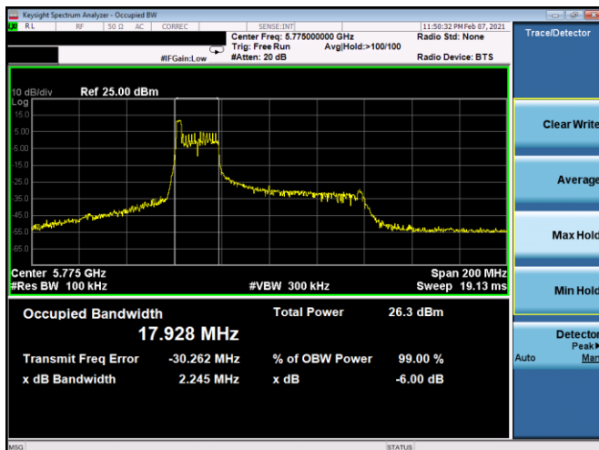
Plot 7-93. 6dB BW & 99% OBW Antenna 4b (80MHz BW 11ax Index 0 – RU26 – Ch.155)
