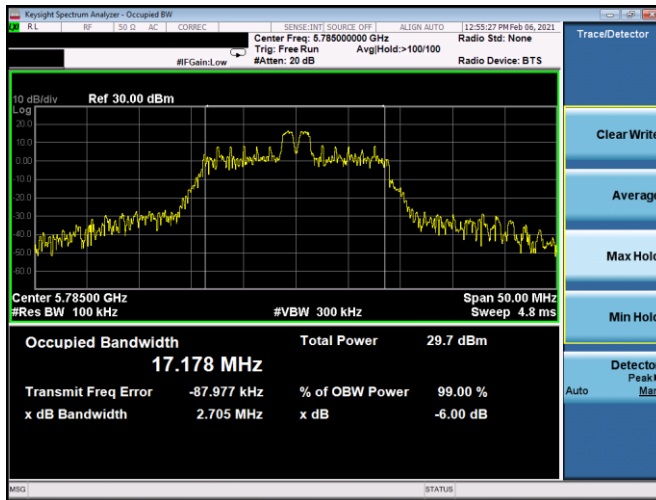
Plot 7-74. 6dB BW & 99% OBW Antenna 5b (20MHz BW 11ax Index 4 – RU26 – Ch.157)
