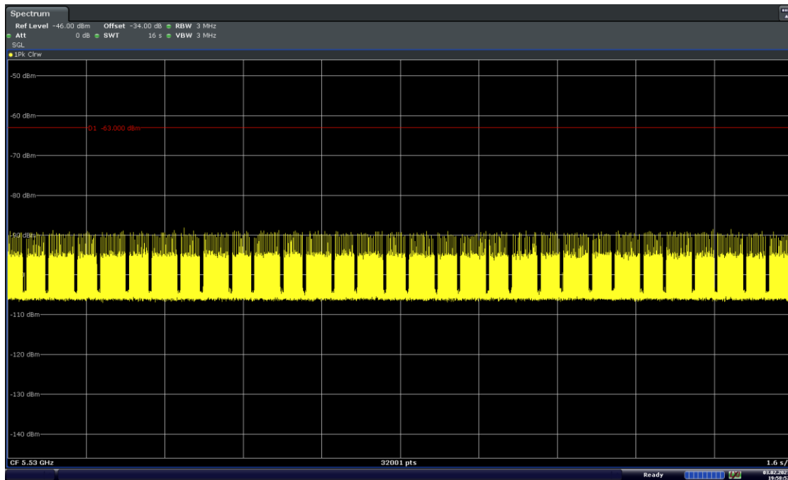
Figure 9-17. 5530MHz - Channel Loading - Mode 3 (80MHz)
