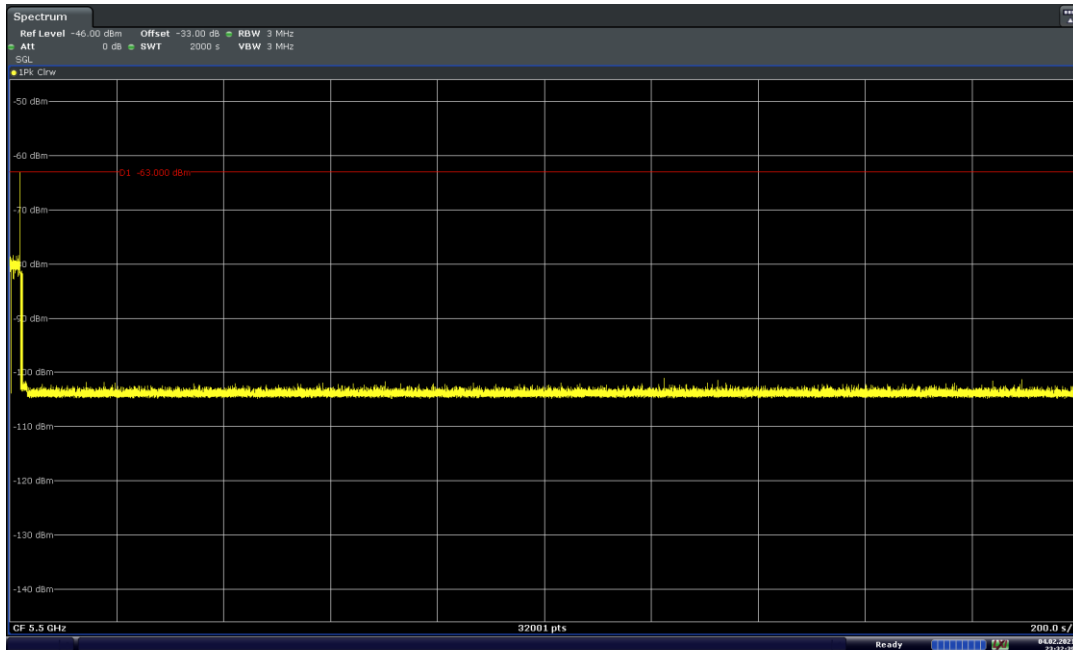
Figure 9-46. 5500MHz - Non-Occupancy Period (30 Minutes) - Mode 4 (20MHz)
