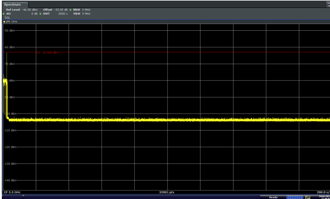
Figure 9-43. 5500MHz - Non-Occupancy Period (30 Minutes) - Mode 3 (20MHz)
