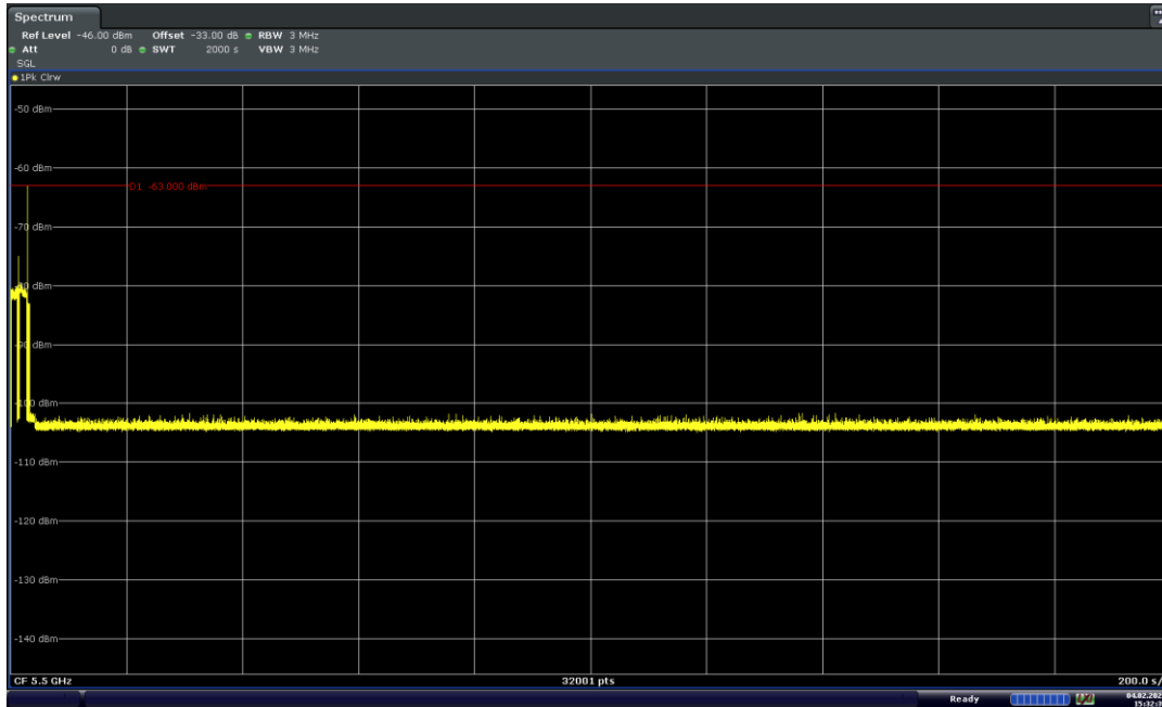
Figure 9-37. 5500MHz - Non-Occupancy Period (30 Minutes) - Mode 1 (20MHz)
