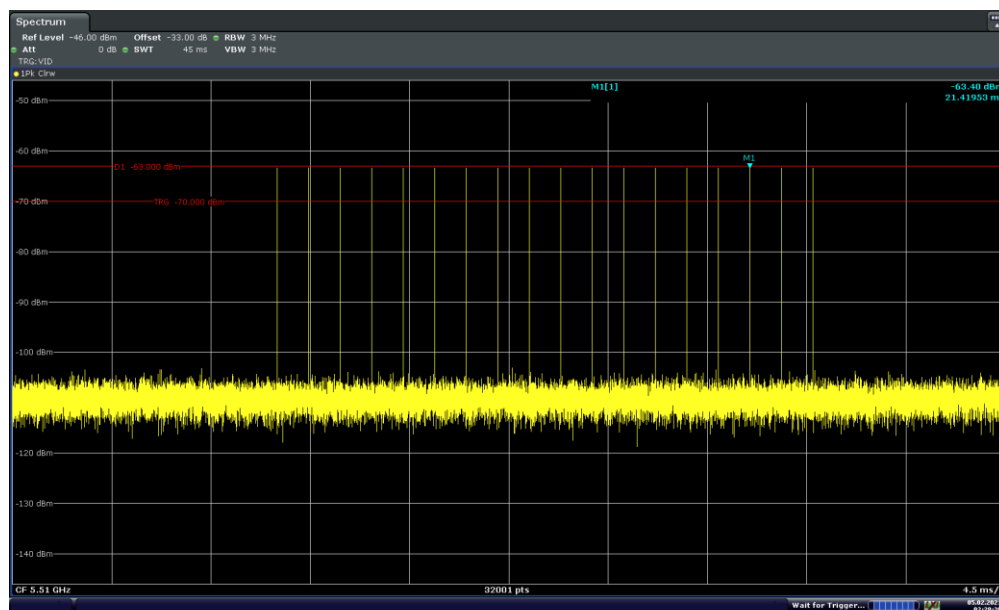
Figure 7-4. 5510MHz – Radar Pulse Type 0 (40MHz)
