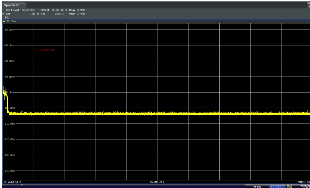
Figure 9-38. 5510MHz - Non-Occupancy Period (30 Minutes) - Mode 1 (40MHz)
