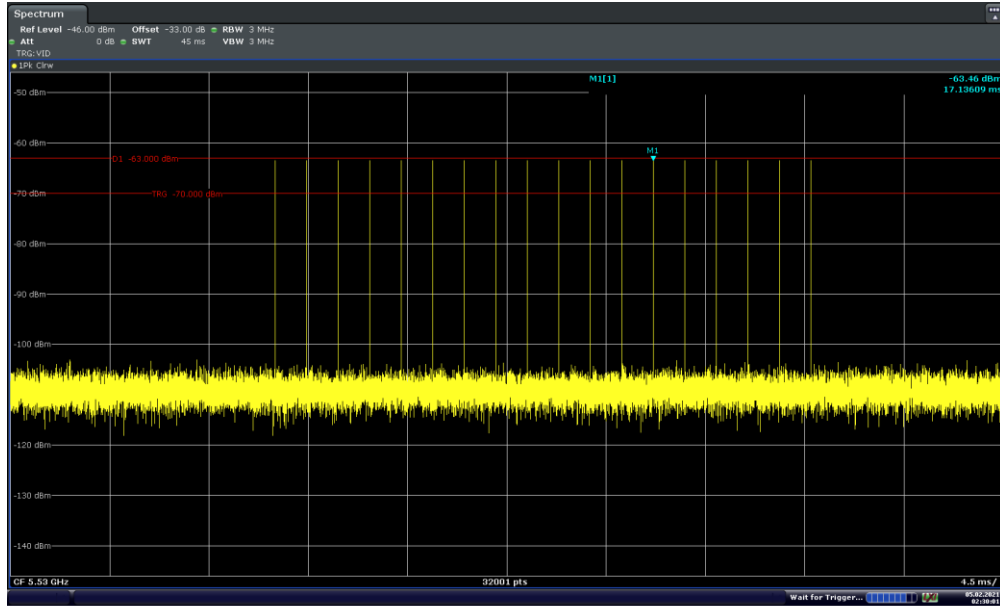
Figure 7-5. 5530MHz – Radar Pulse Type 0 (80MHz)
