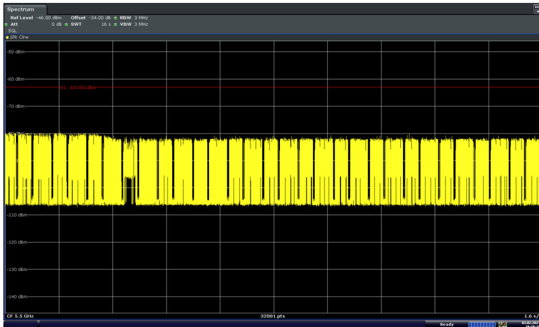
Figure 9-19. 5500 MHz - Channel Loading - Mode 4 (20MHz)
