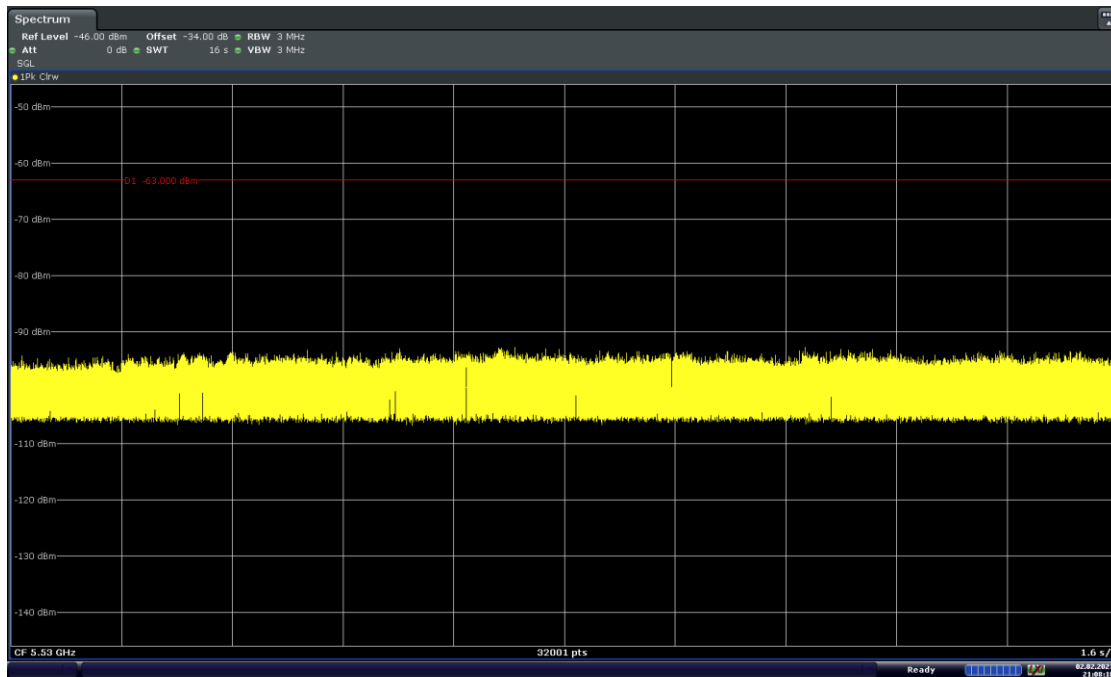
Figure 9-5. 5530MHz - Channel Loading - Mode 1 (80MHz)
