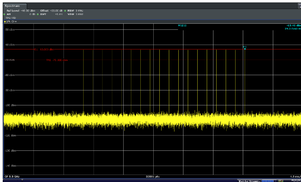
Figure 7-3. 5500MHz – Radar Pulse Type 0 (20MHz)
