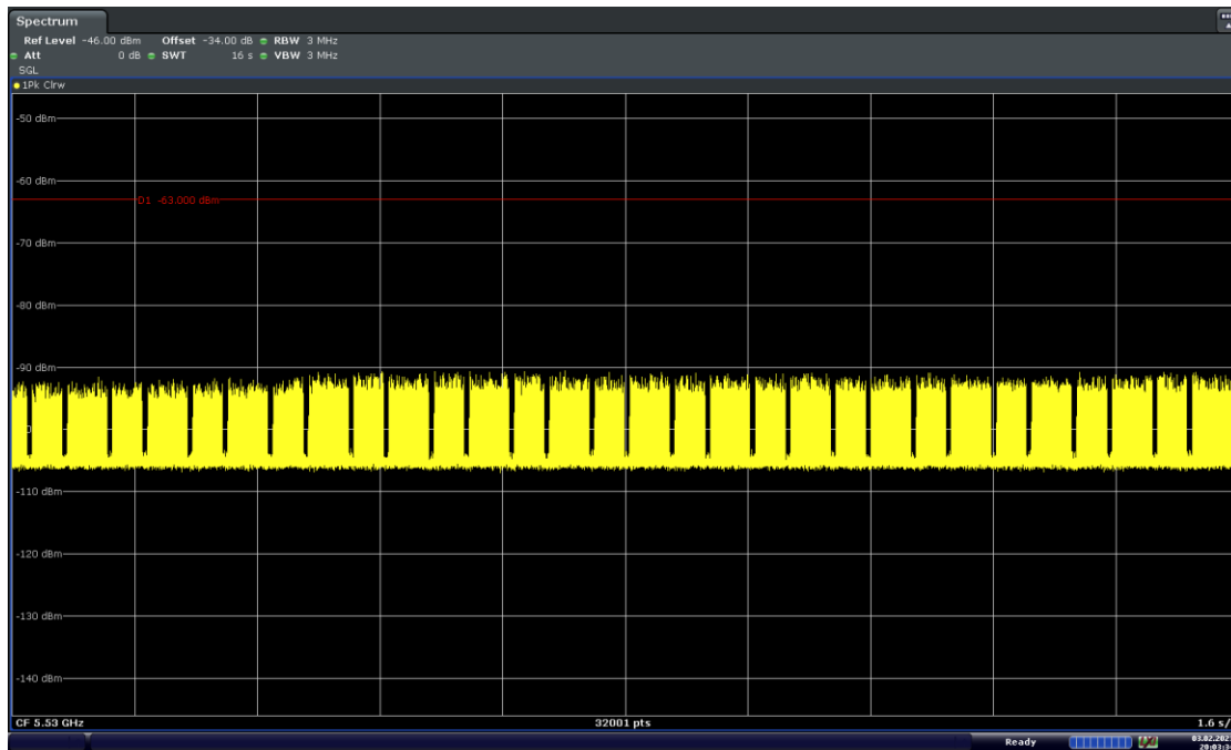
Figure 9-23. 5530MHz - Channel Loading - Mode 4 (80MHz)
