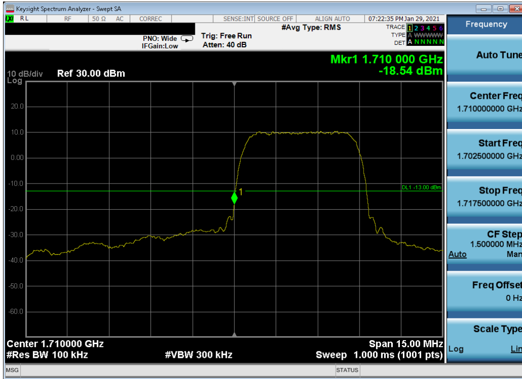
Plot 7-293. Band Edge Plot (AWS WCDMA Mode - Low Channel)
