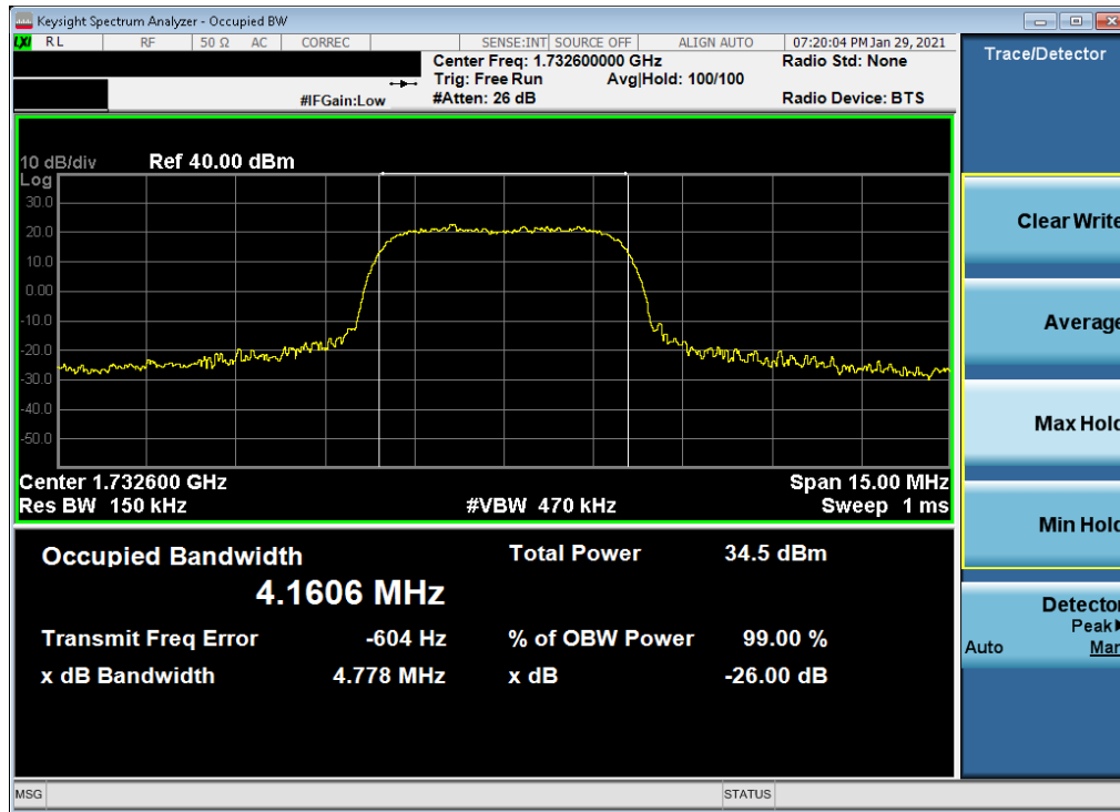
Plot 7-120. Occupied Bandwidth Plot (WCDMA, Ch. 1413)
