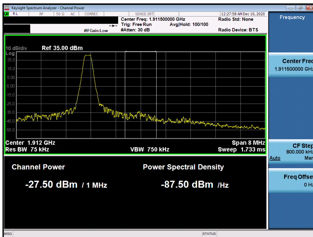
Plot 7-167. Extended Upper Band Edge Plot (GPRS PCS – Ch. 810)
