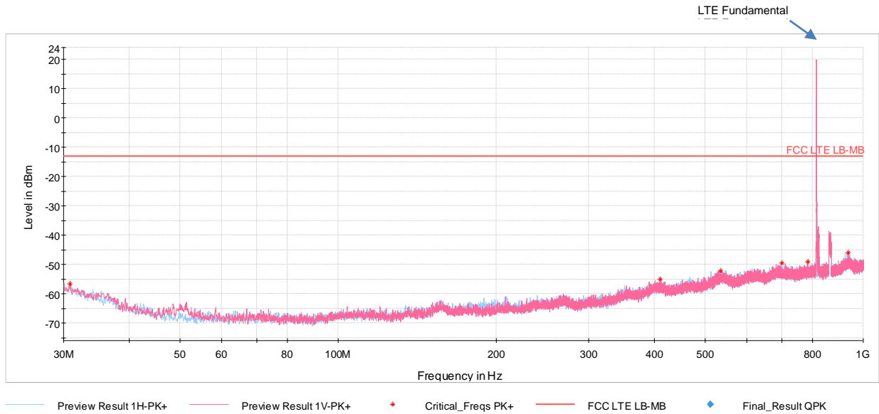
Plot 7-49. Radiated Spurious Emissions Below 1GHz (Band 26)
