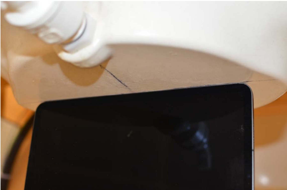
Test Setup Photo 9 – Left Edge SAR at 0 mm
