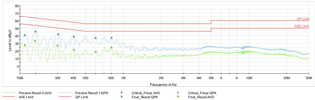
Plot 6-5. AC Line Conducted Plot (L1, Charging Rate 10C, with AC/DC Adapter)
