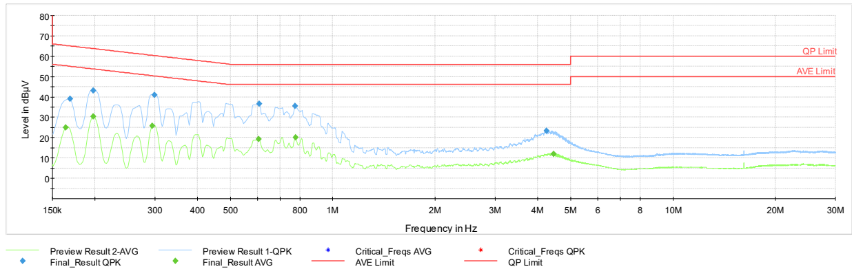
Plot 6-6. AC Line Conducted Plot (N, Charging Rate 10C, with AC/DC Adapter)
