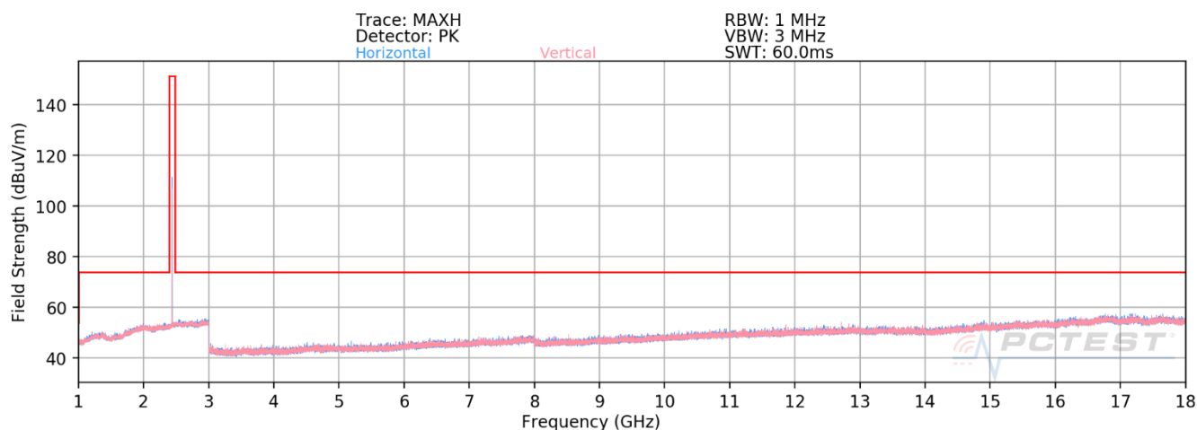
Plot 8-5. Radiated Spurious Emissions Above 1GHz TxBF (BT GFSK ePA – Ch. 39)
