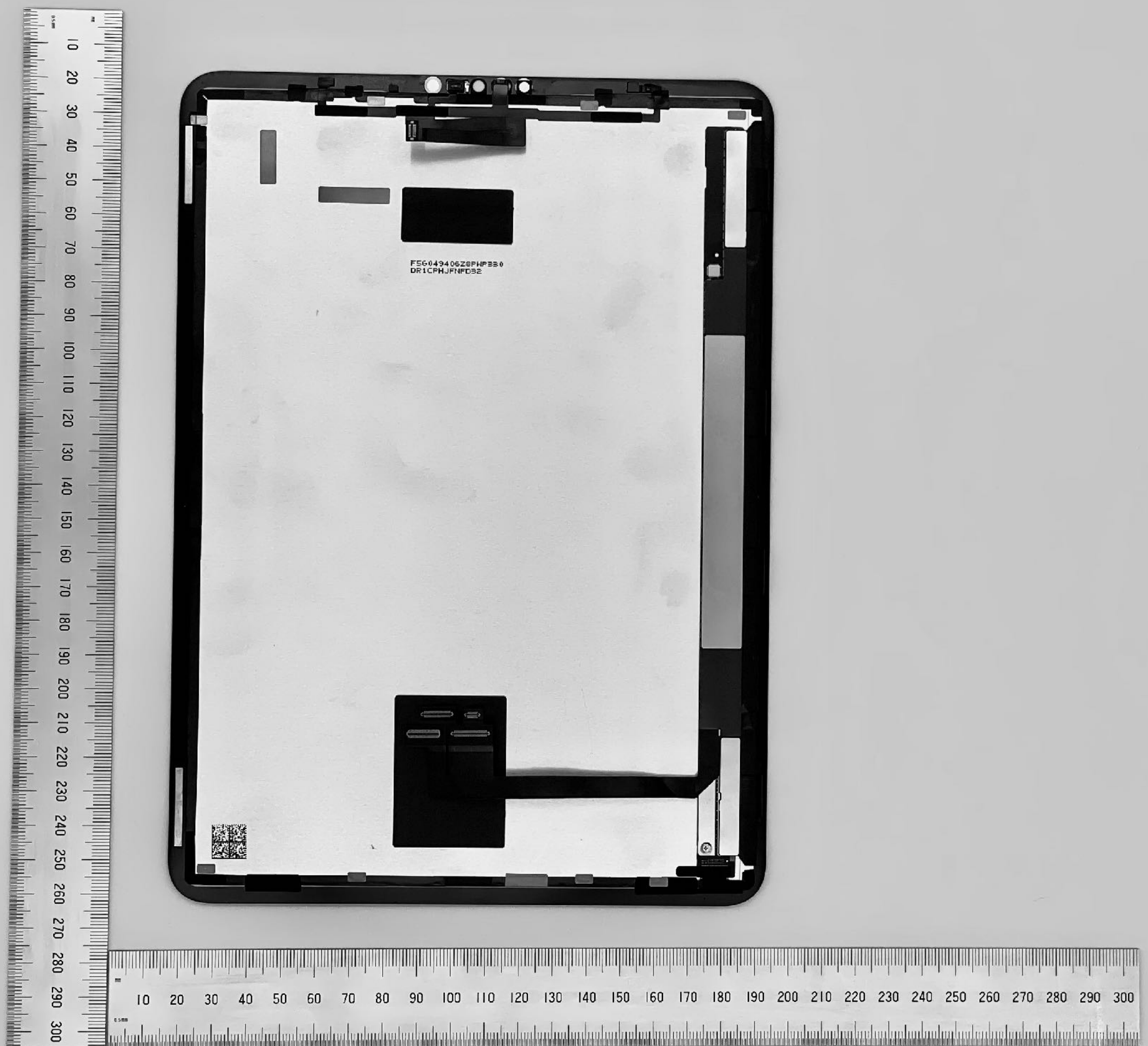
A2459, A2460 Display Panel - Back
