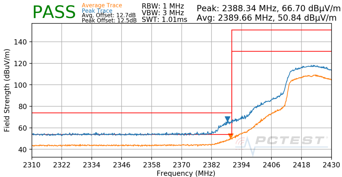
Plot 7-26. Radiated Restricted Lower Band Edge Measurement Antenna 4a
