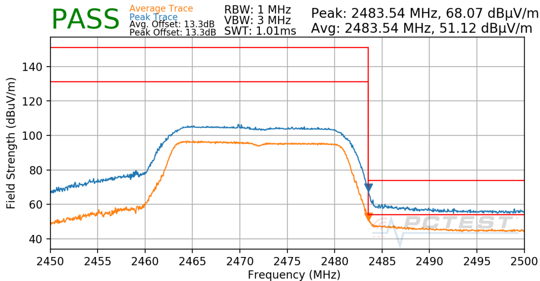
Plot 7-43. Radiated Restricted Upper Band Edge Measurement Antenna 4a
