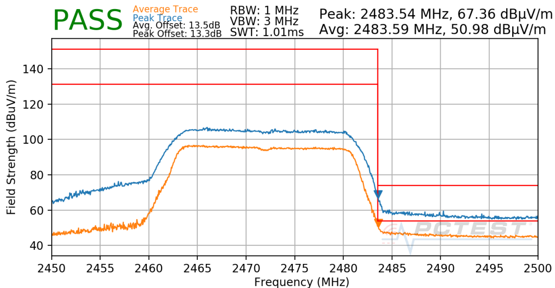
Plot 7-44. Radiated Restricted Upper Band Edge Measurement Antenna 4a
