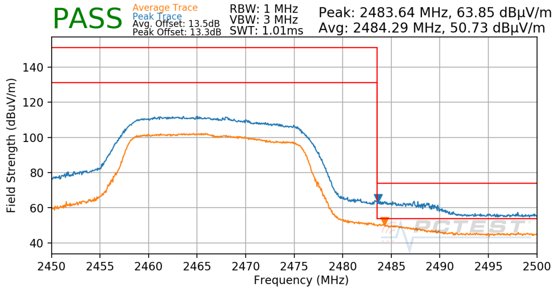
Plot 7-41. Radiated Restricted Upper Band Edge Measurement Antenna 4a
