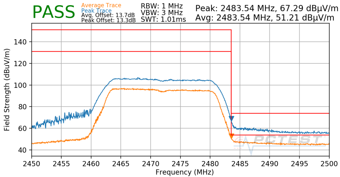
Plot 7-45. Radiated Restricted Upper Band Edge Measurement Antenna 4a
