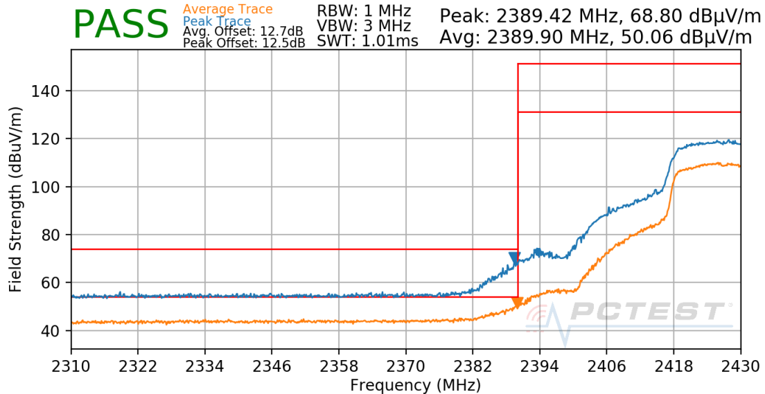
Plot 7-29. Radiated Restricted Lower Band Edge Measurement Antenna 4a
