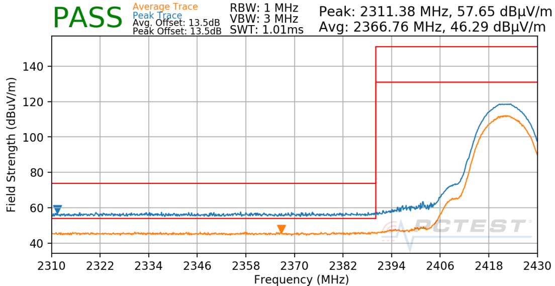
Plot 7-15. Radiated Restricted Lower Band Edge Measurement Antenna 4a
