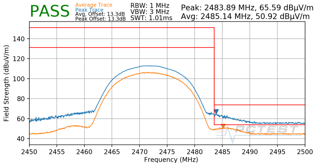
Plot 7-18. Radiated Restricted Upper Band Edge Measurement Antenna 4a
