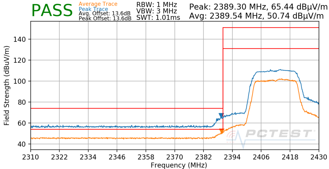
Plot 7-19. Radiated Restricted Lower Band Edge Measurement Antenna 4a
