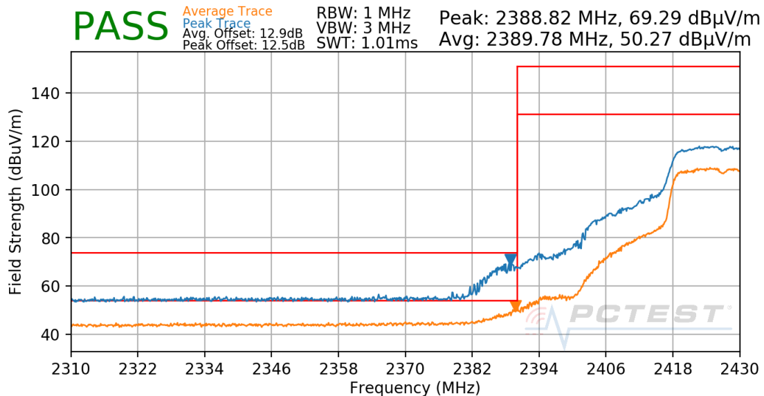
Plot 7-30. Radiated Restricted Lower Band Edge Measurement Antenna 4a
