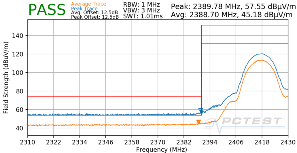
Plot 7-14. Radiated Restricted Lower Band Edge Measurement Antenna 4a
