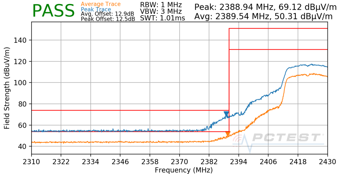
Plot 7-27. Radiated Restricted Lower Band Edge Measurement Antenna 4a
