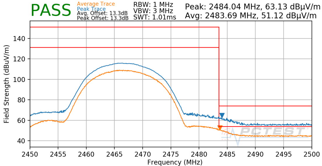
Plot 7-17. Radiated Restricted Upper Band Edge Measurement Antenna 4a
