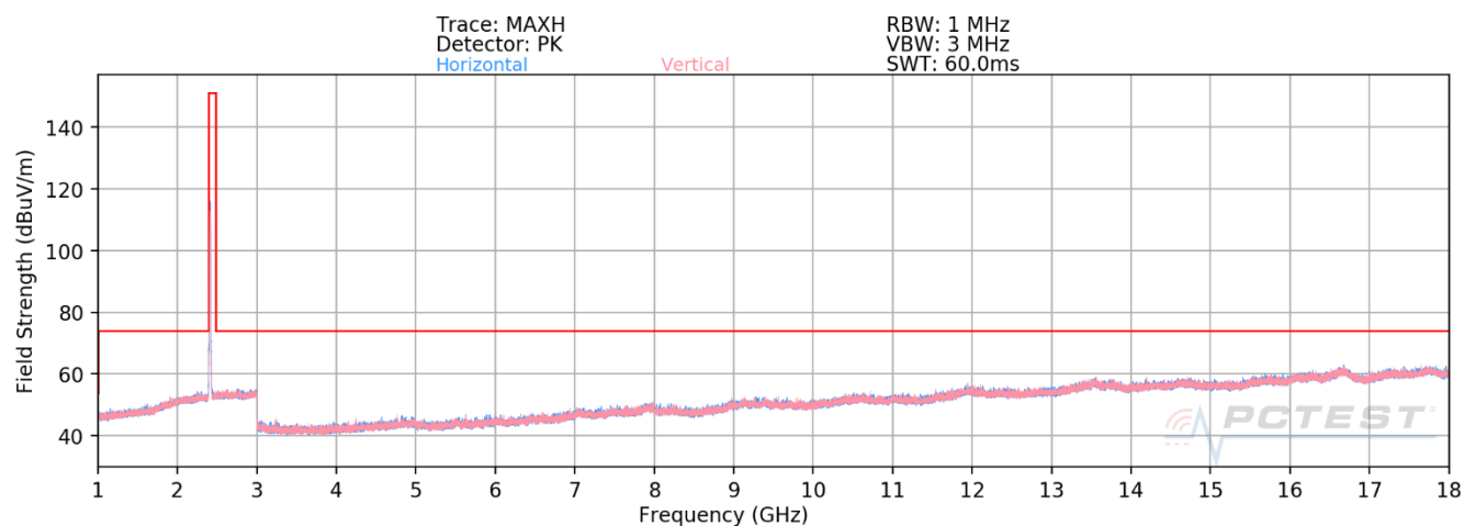
Plot 7-1. Radiated Spurious Emissions above 1GHz Antenna 4a (802.11b – Ch. 1)
