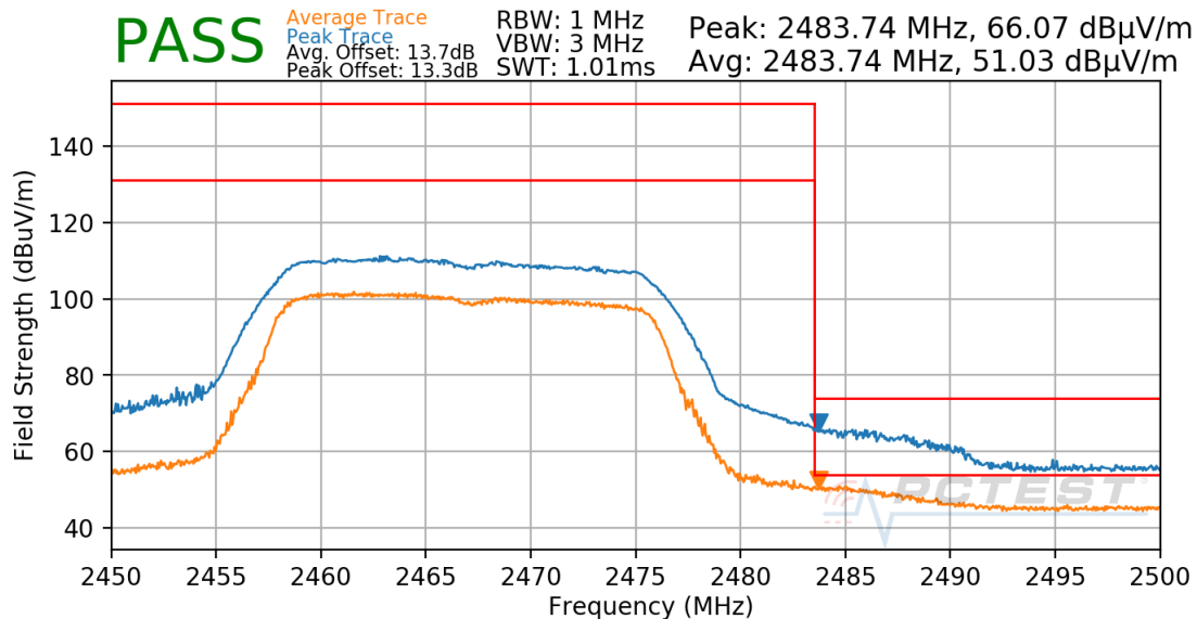
Plot 7-42. Radiated Restricted Upper Band Edge Measurement Antenna 4a
