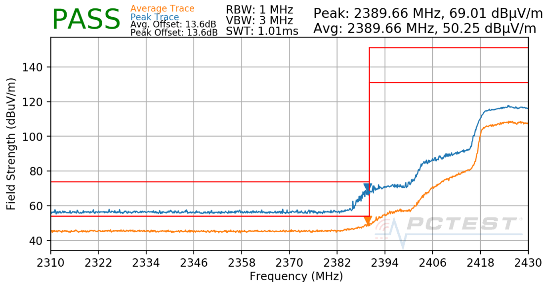
Plot 7-28. Radiated Restricted Lower Band Edge Measurement Antenna 4a
