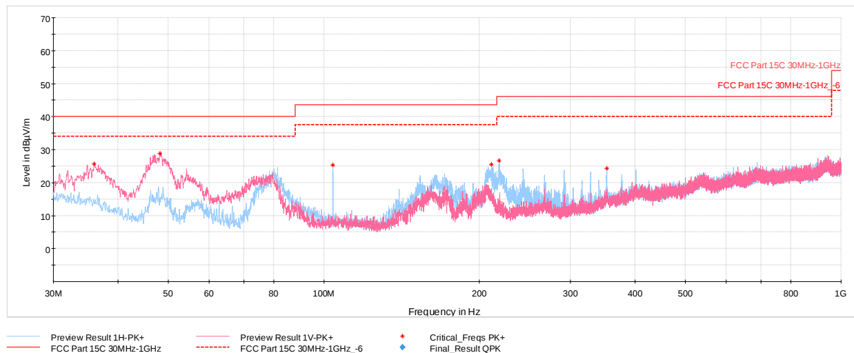
Plot 7-197. Radiated Spurious Emissions below 1GHz CDD Ch.1 (RU26), with AC/DC Adapter
