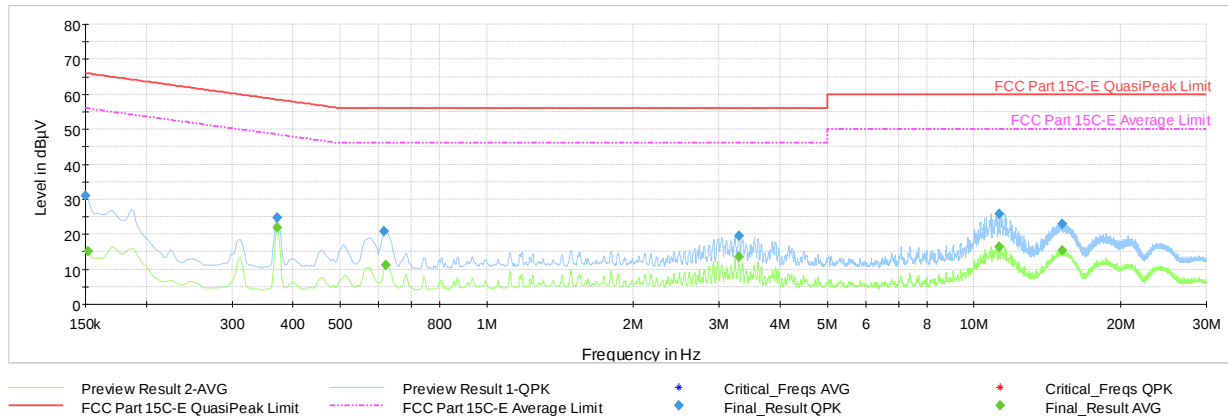
Plot 7-202. AC Line Conducted Emissions with 802.11ax (RU26) Ch.1 (N, with Laptop)
