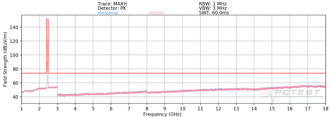
Plot 8-10. Radiated Spurious Emissions above 1GHz CDD (802.11ax OFDMA – RU26 – Ch. 11)
