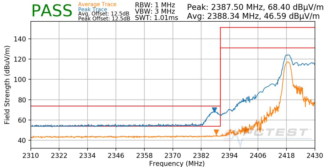
Plot 8-17. Radiated Restricted Lower Band Edge Measurement Antenna 4a (Average & Peak – RU26)
