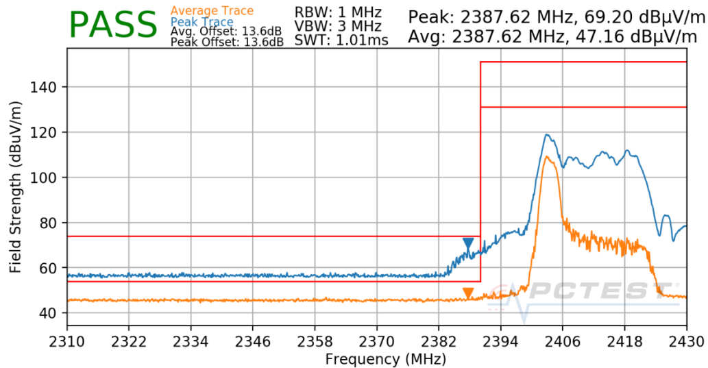
Plot 8-30: Radiated Restricted Lower Band Edge Measurement CDD (Average & Peak – RU26)
