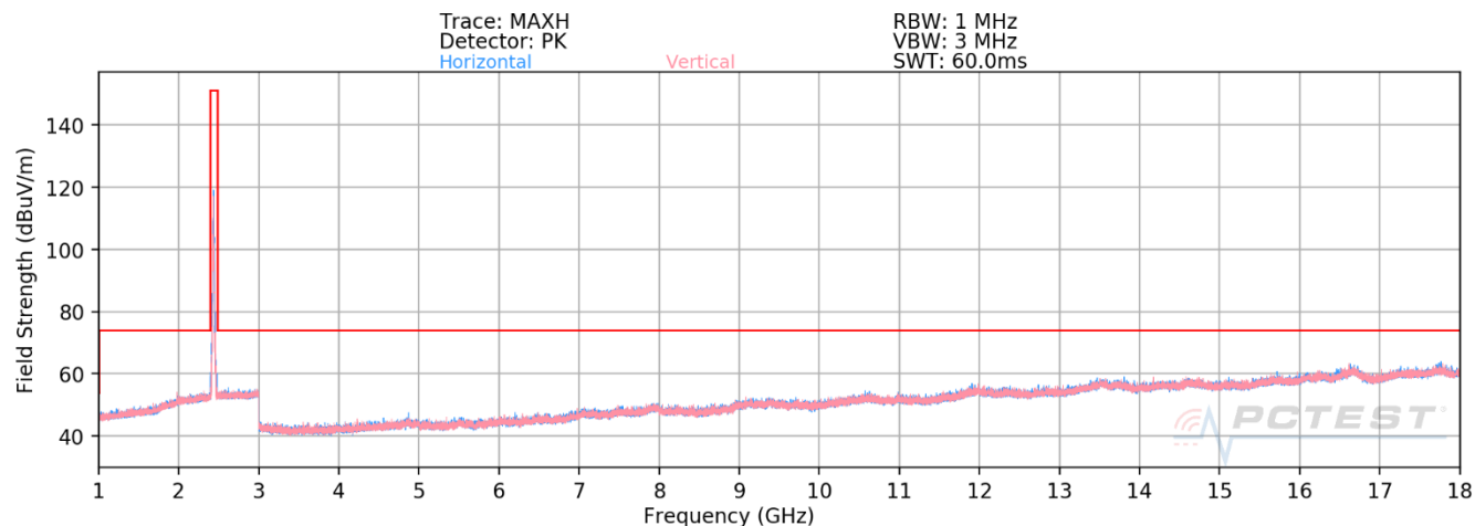
Plot 8-2. Radiated Spurious Emissions above 1GHz Antenna 4a (802.11ax OFDMA – RU26 – Ch. 6)
