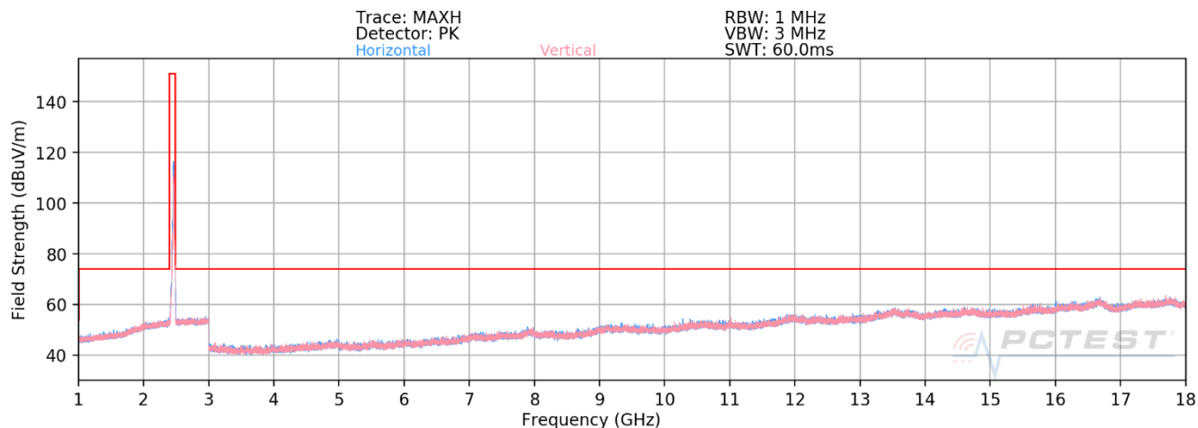
Plot 8-7: Radiated Spurious Emissions above 1GHz Antenna 4a (802.11ax OFDMA – RU242 – Ch. 11)
