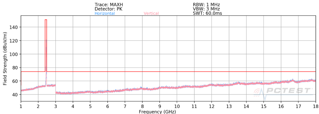
Plot 8-3. Radiated Spurious Emissions above 1GHz Antenna 4a (802.11ax OFDMA – RU26 – Ch. 11)
