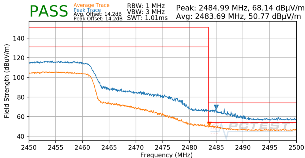
Plot 8-26: Radiated Restricted Upper Band Edge Measurement Antenna 4a (Average & Peak – RU242)
