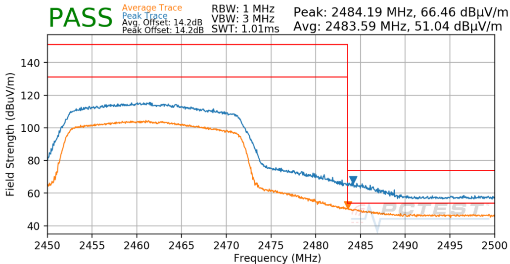
Plot 8-28: Radiated Restricted Upper Band Edge Measurement Antenna 4a (Average & Peak – RU242)
