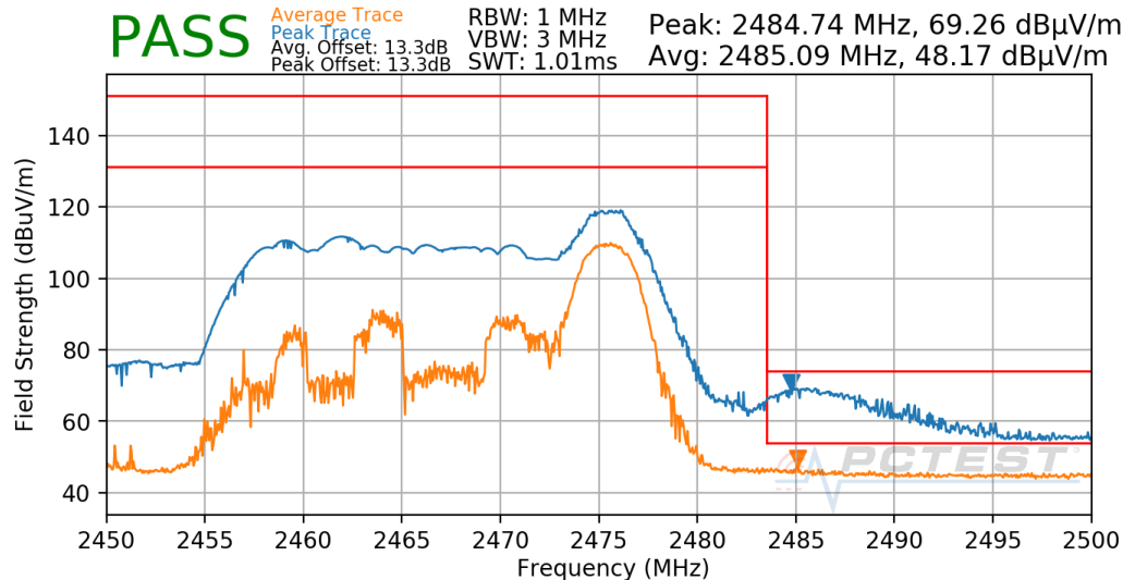
Plot 8-21. Radiated Restricted Upper Band Edge Measurement Antenna 4a (Average & Peak – RU26)
