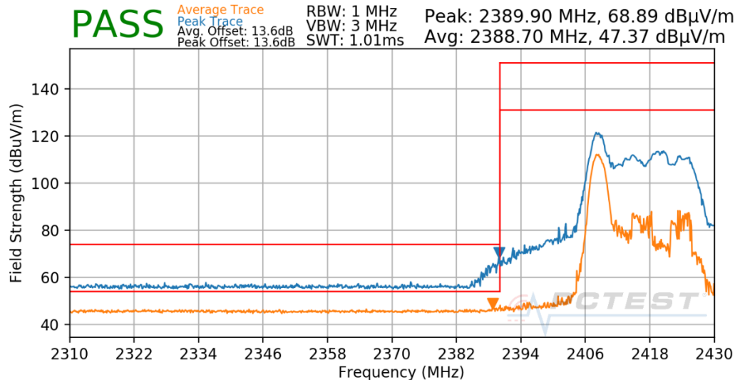
Plot 8-31: Radiated Restricted Lower Band Edge Measurement CDD (Average & Peak – RU26)
