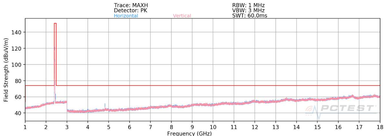
Plot 8-1. Radiated Spurious Emissions above 1GHz Antenna 4a (802.11ax OFDMA – RU26 – Ch. 1)
