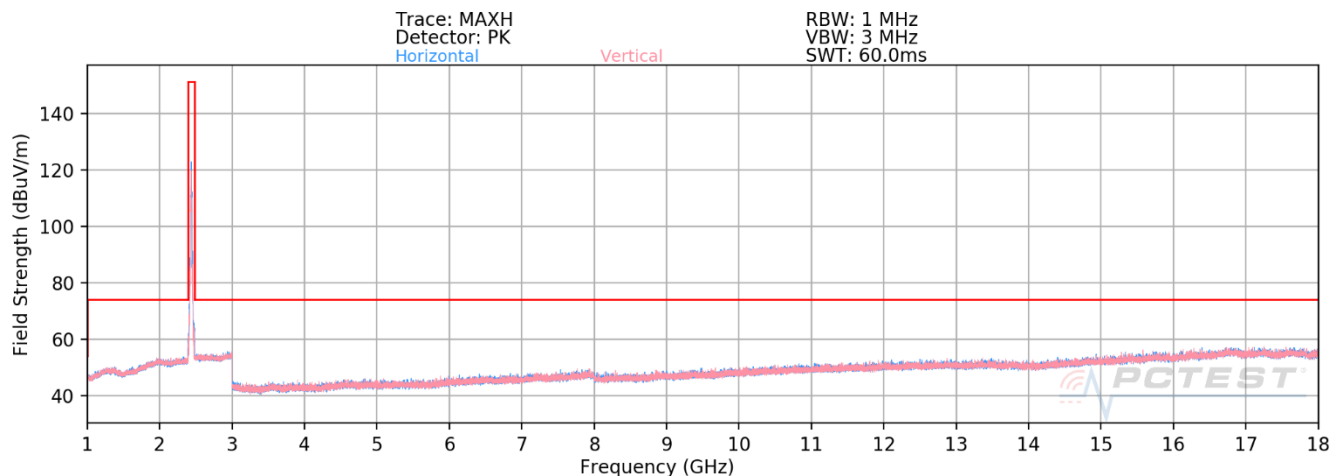
Plot 8-9. Radiated Spurious Emissions above 1GHz CDD (802.11ax OFDMA – RU26 – Ch. 6)
