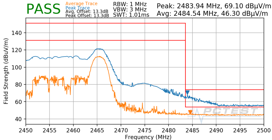
Plot 8-19. Radiated Restricted Upper Band Edge Measurement Antenna 4a (Average & Peak – RU26)
