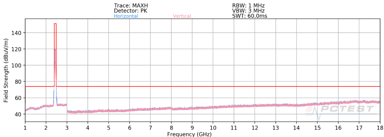
Plot 8-12. Radiated Spurious Emissions above 1GHz CDD (802.11ax OFDMA – RU242 – Ch. 6)
