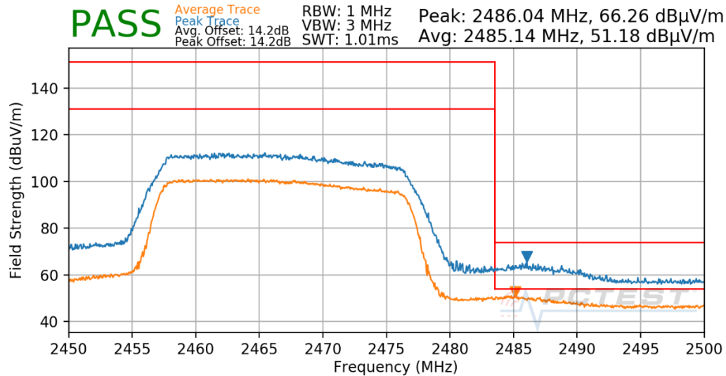
Plot 8-29: Radiated Restricted Upper Band Edge Measurement Antenna 4a (Average & Peak – RU242)
