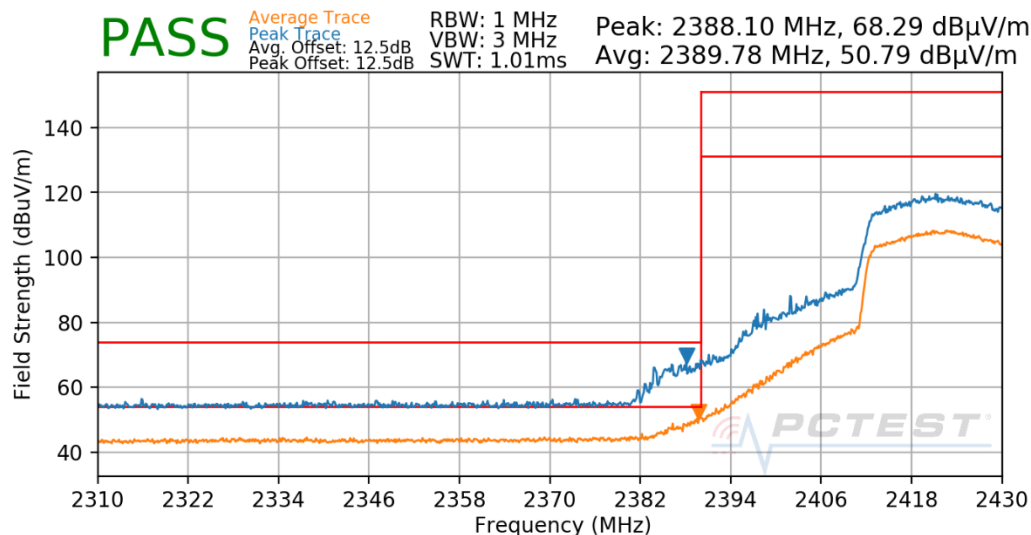
Plot 8-24: Radiated Restricted Lower Band Edge Measurement Antenna 4a (Average & Peak – RU242)
