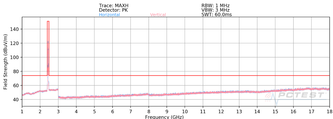
Plot 7-1: Radiated Spurious Emissions above 1GHz CDD (802.11ax OFDMA – RU26 – Ch. 6)
