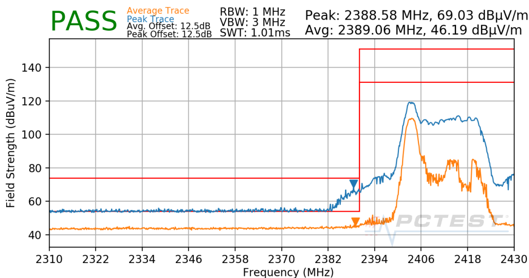
Plot 8-14. Radiated Restricted Lower Band Edge Measurement Antenna 4a (Average & Peak – RU26)
