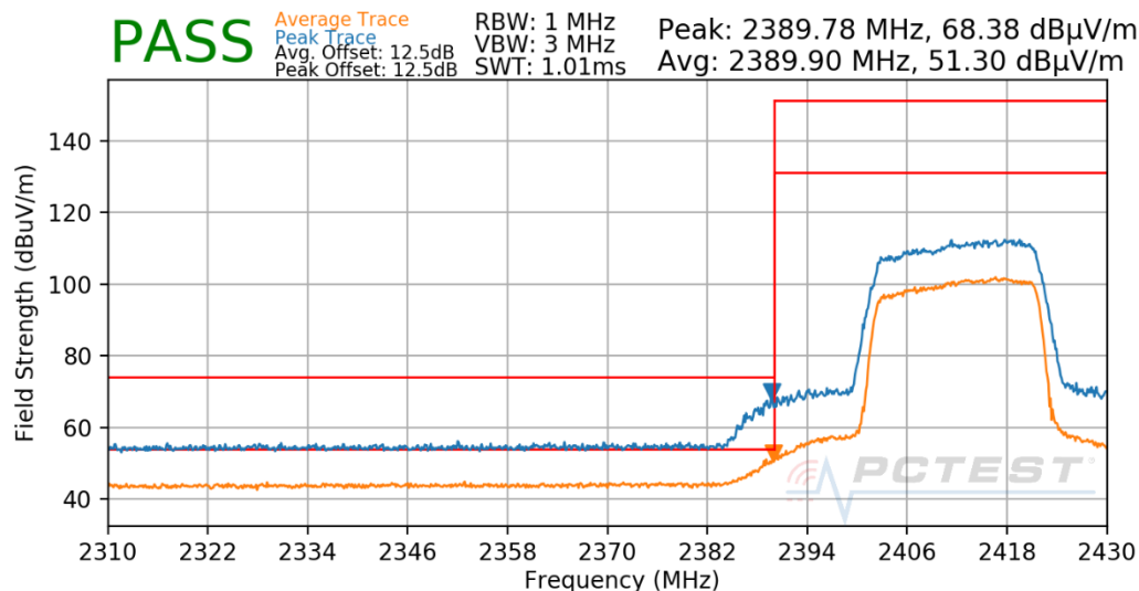
Plot 8-22. Radiated Restricted Lower Band Edge Measurement Antenna 4a (Average & Peak – RU242)
