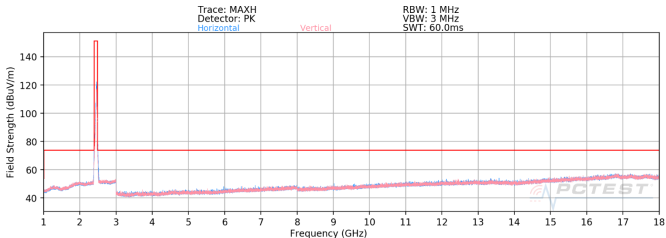
Plot 8-13. Radiated Spurious Emissions above 1GHz CDD (802.11ax OFDMA – RU242 – Ch. 11)
