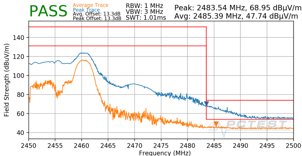
Plot 8-18. Radiated Restricted Upper Band Edge Measurement Antenna 4a (Average & Peak – RU26)
