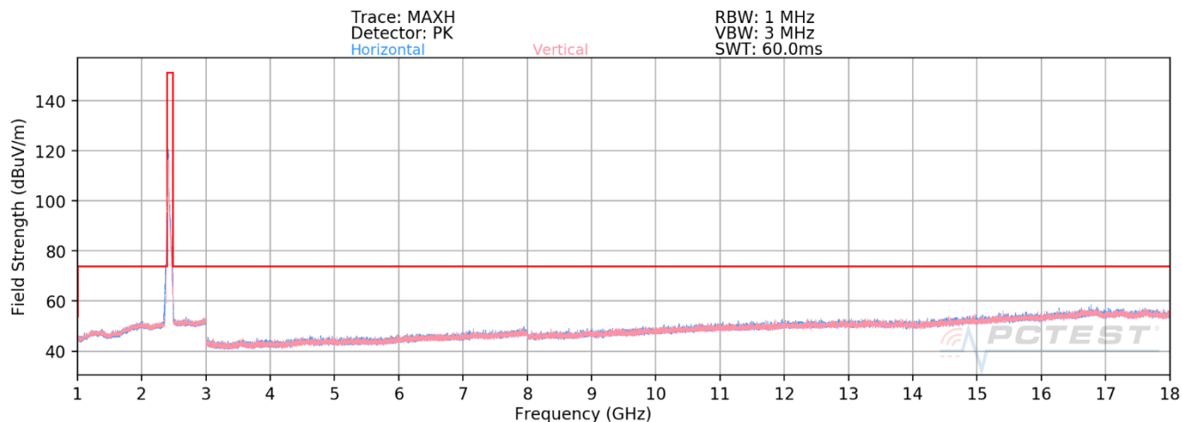
Plot 8-11. Radiated Spurious Emissions above 1GHz CDD (802.11ax OFDMA – RU242 – Ch. 1)
