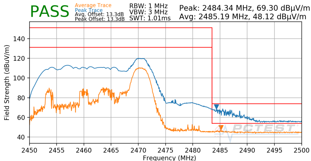
Plot 8-20. Radiated Restricted Upper Band Edge Measurement Antenna 4a (Average & Peak – RU26)
