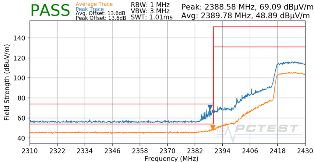
Plot 8-25: Radiated Restricted Lower Band Edge Measurement Antenna 4a (Average & Peak – RU242)
