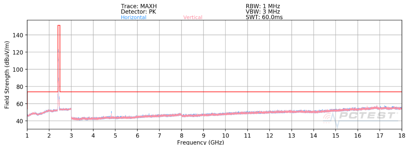
Plot 8-8. Radiated Spurious Emissions above 1GHz CDD (802.11ax OFDMA – RU26 – Ch. 1)
