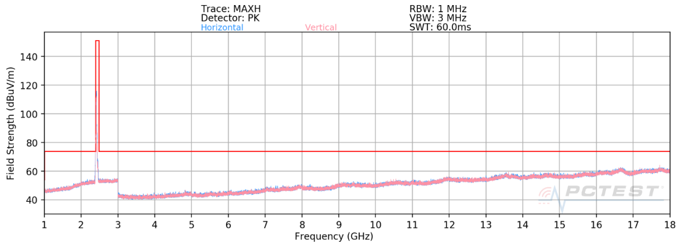
Plot 8-4: Radiated Spurious Emissions above 1GHz Antenna 4a (802.11ax OFDMA – RU242 – Ch. 1)
