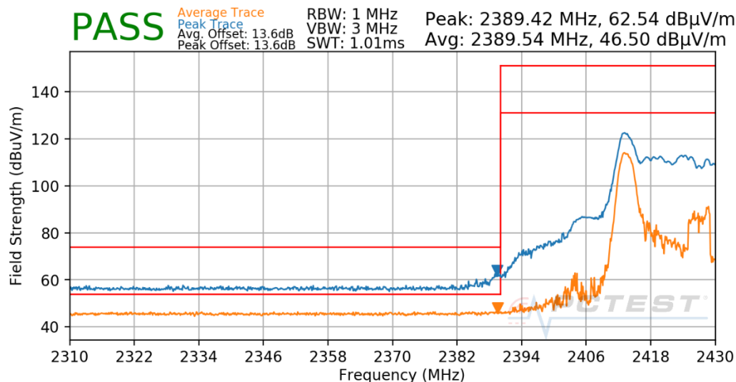
Plot 8-32: Radiated Restricted Lower Band Edge Measurement CDD (Average & Peak – RU26)
