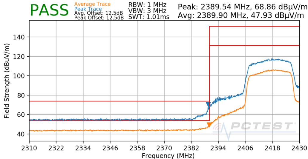
Plot 8-23: Radiated Restricted Lower Band Edge Measurement Antenna 4a (Average & Peak – RU242)
