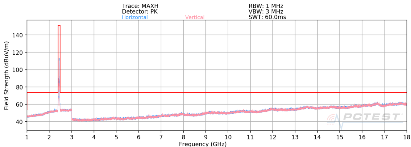
Plot 8-6: Radiated Spurious Emissions above 1GHz Antenna 4a (802.11ax OFDMA – RU242 – Ch. 6)
