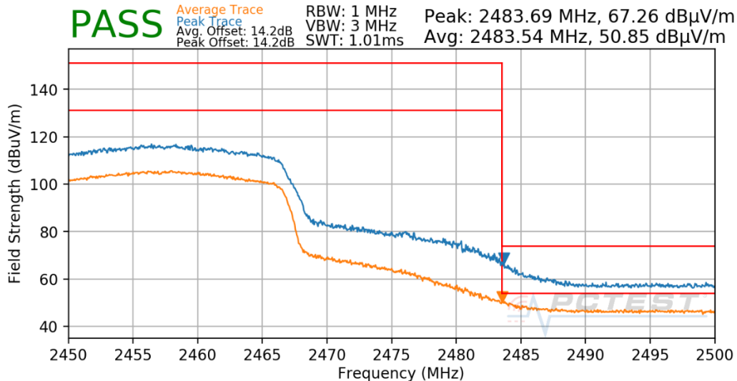
Plot 8-27: Radiated Restricted Upper Band Edge Measurement Antenna 4a (Average & Peak – RU242)
