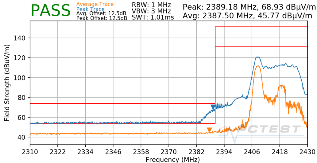
Plot 8-15. Radiated Restricted Lower Band Edge Measurement Antenna 4a (Average & Peak – RU26)
