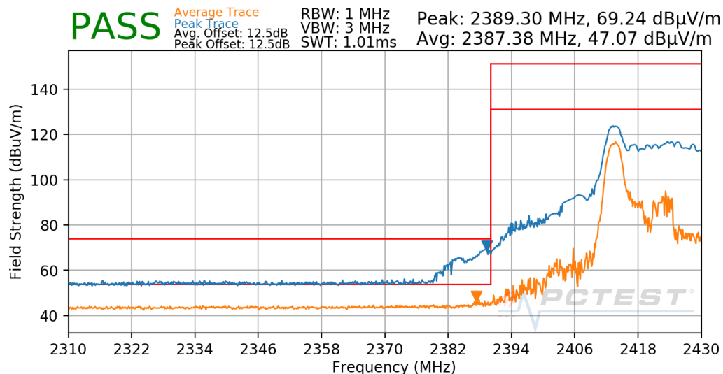
Plot 8-16. Radiated Restricted Lower Band Edge Measurement Antenna 4a (Average & Peak – RU26)
