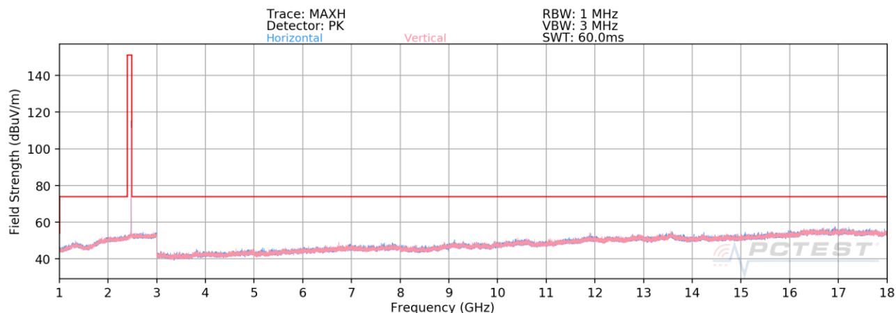
Plot 7-89. Radiated Spurious Emissions Above 1GHz TxBF (4Mbps, HDR4, ePA – Ch. 73)
