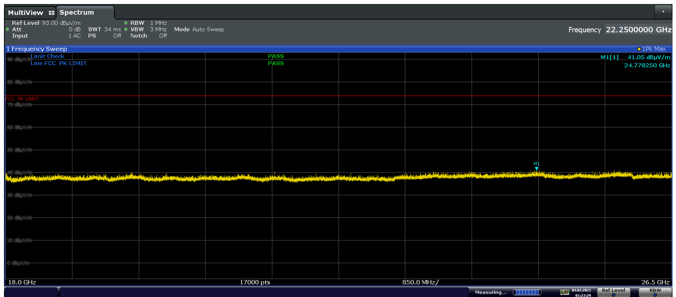
Plot 7-91. Radiated Spurious Emissions Above 18GHz TxBF (4Mbps – Ch.38, ePA, Ant. Pol. V)
