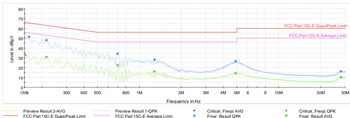
Plot 7-105. AC Line Conducted Plot with Bluetooth HDR (L1, 4Mbps ePA - Ch.38 with AC/DC Adapter)
