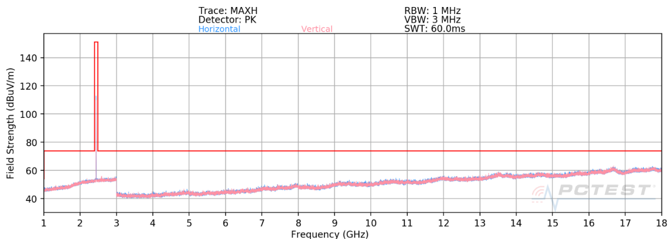
Plot 8-2. Radiated Spurious Emissions Above 1GHz Antenna 4a (4Mbps, HDR4, ePA – Ch. 38)
