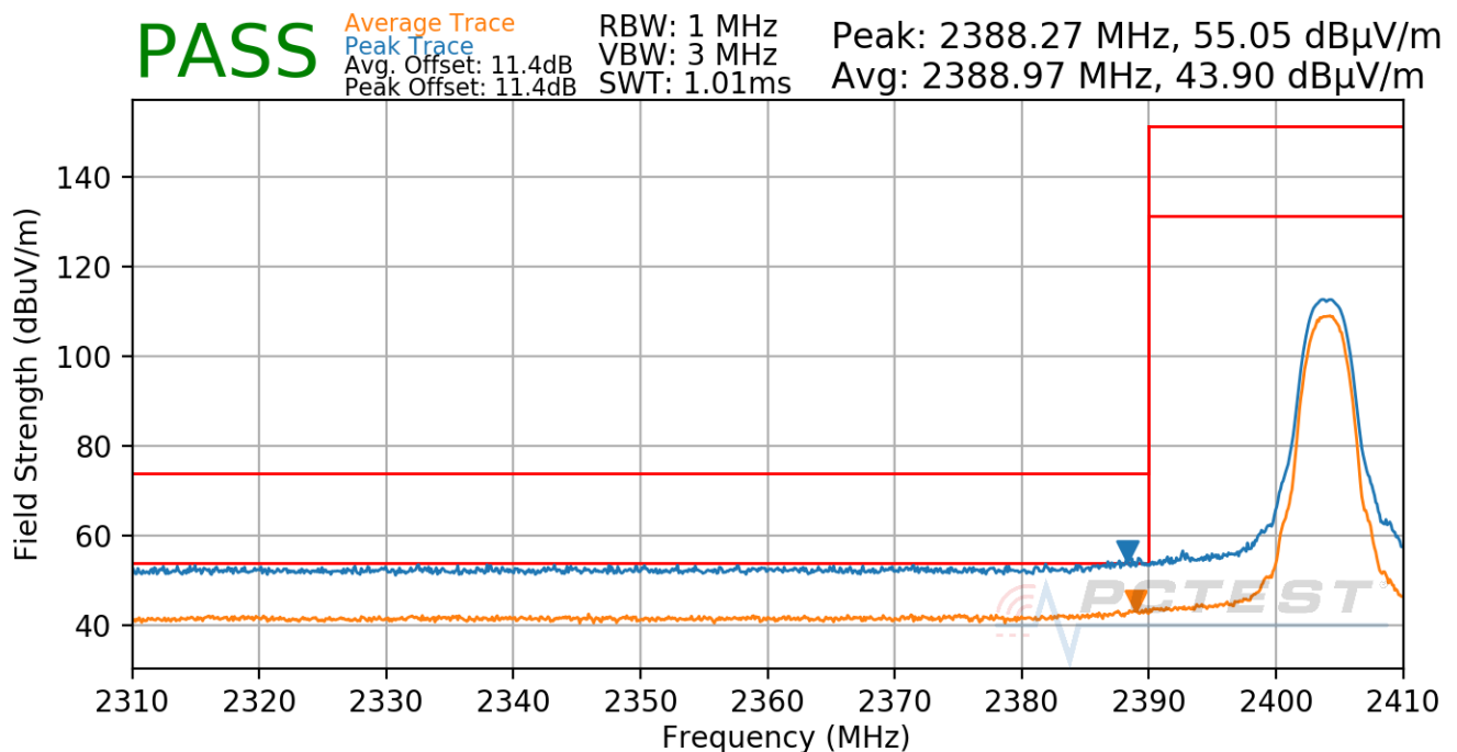
Plot 8-7. Radiated Restricted Lower Band Edge Measurement Antenna 4a (Average & Peak)
