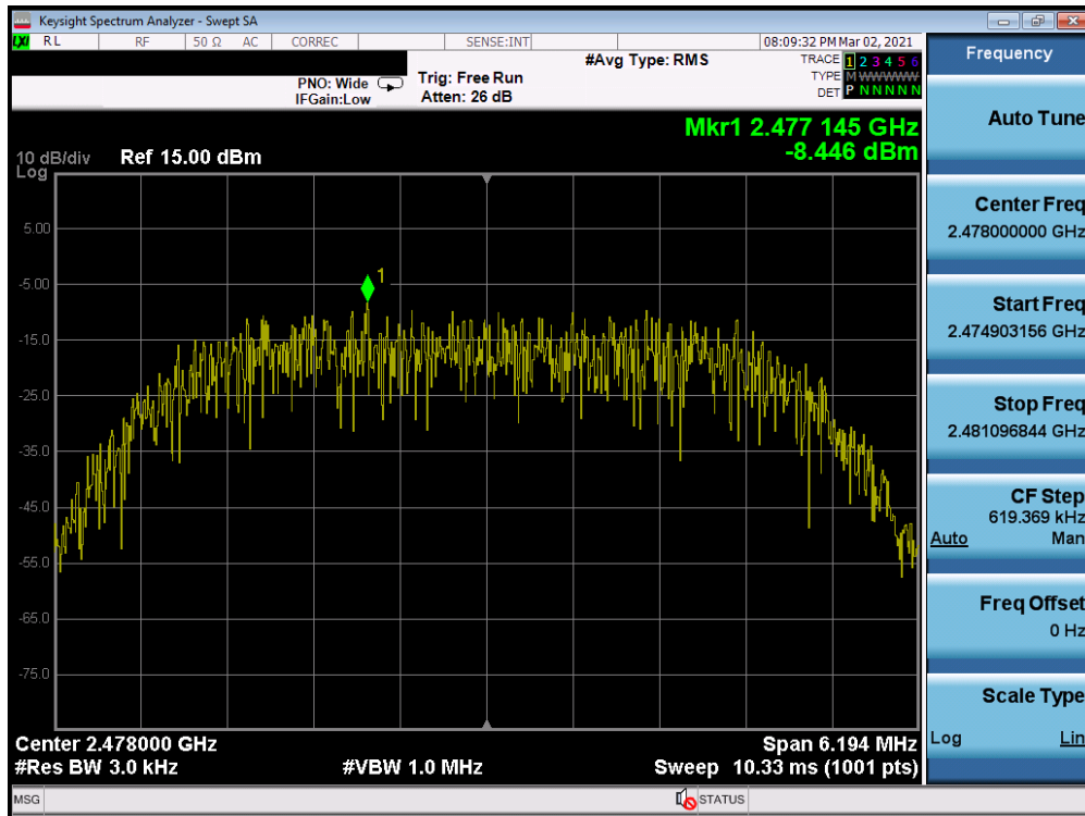
Plot 7-21. Power Spectral Density Plot Antenna 4a (Bluetooth (HDR8), 8Mbps, ePA – Ch. 73)
