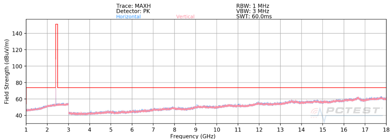
Plot 8-1. Radiated Spurious Emissions Above 1GHz Antenna 4a (4Mbps, HDR4, ePA – Ch. 1)
