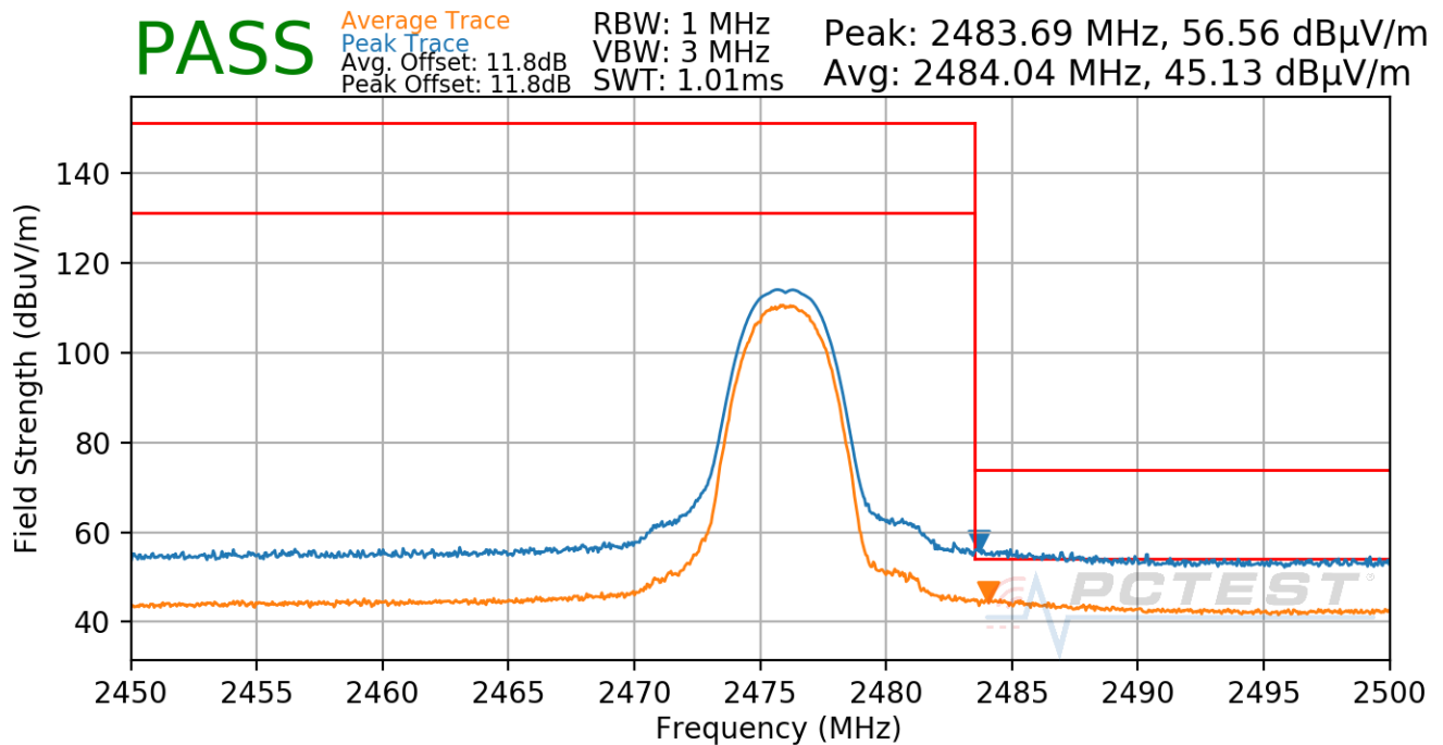
Plot 8-9. Radiated Restricted Upper Band Edge Measurement Antenna 4a (Average & Peak)
