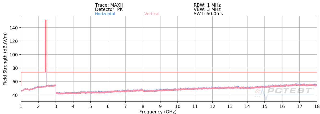
Plot 8-6. Radiated Spurious Emissions Above 1GHz TxBF (4Mbps, HDR4, ePA – Ch. 73)
