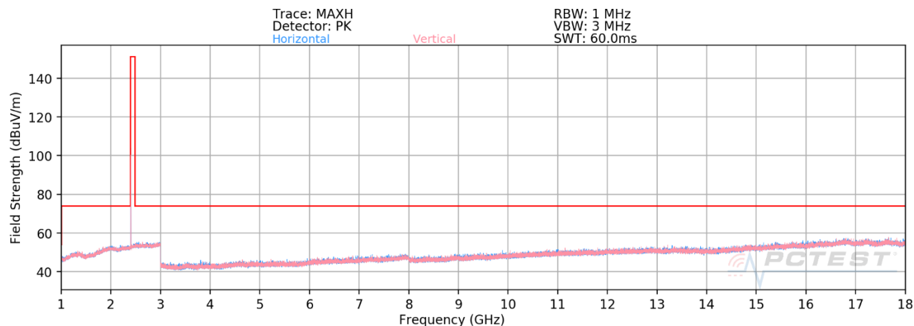
Plot 8-4. Radiated Spurious Emissions Above 1GHz TxBF (4Mbps, HDR4, ePA – Ch. 1)
