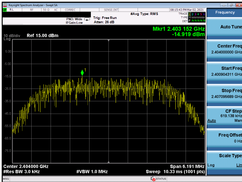
Plot 7-22. Power Spectral Density Plot Antenna 4a (Bluetooth (HDR8), 8Mbps, iPA – Ch. 1)
