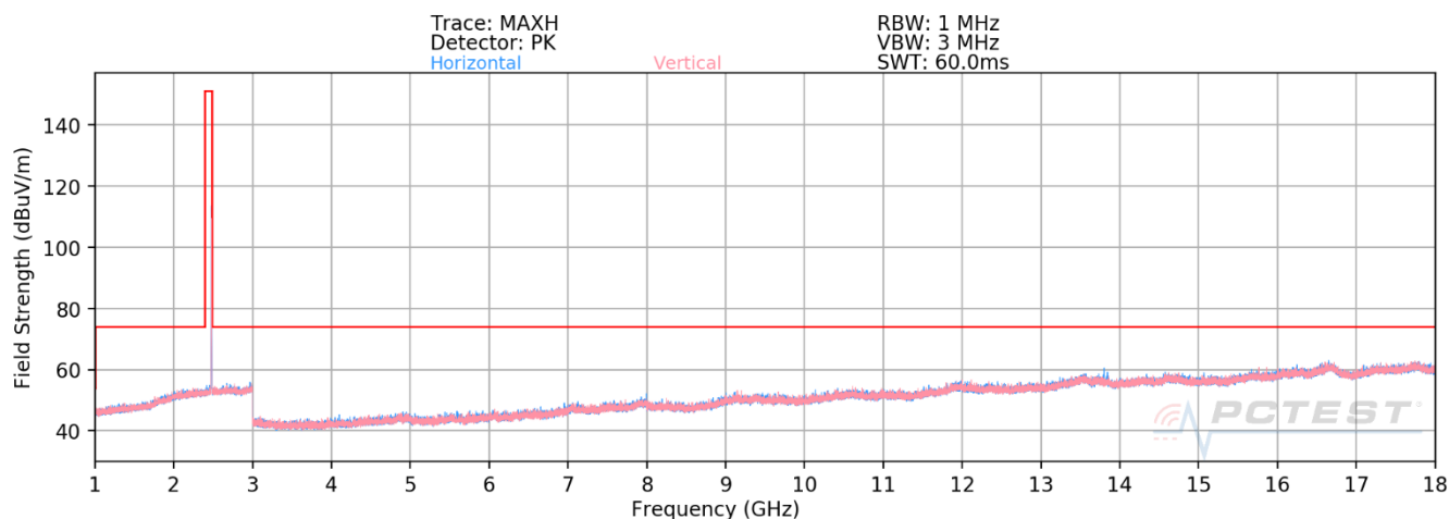
Plot 8-3. Radiated Spurious Emissions Above 1GHz Antenna 4a (4Mbps, HDR4, ePA – Ch. 73)
