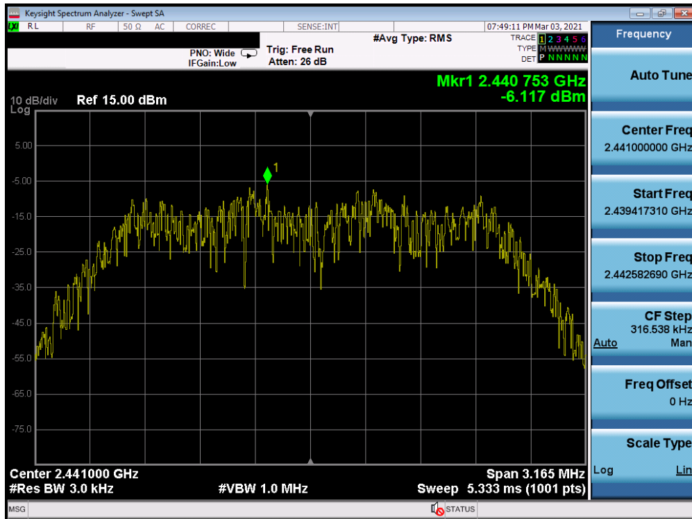
Plot 7-39. Power Spectral Density Plot Tx BF Antenna 4a (Bluetooth (HDR4), 4Mbps, ePA – Ch. 38)
