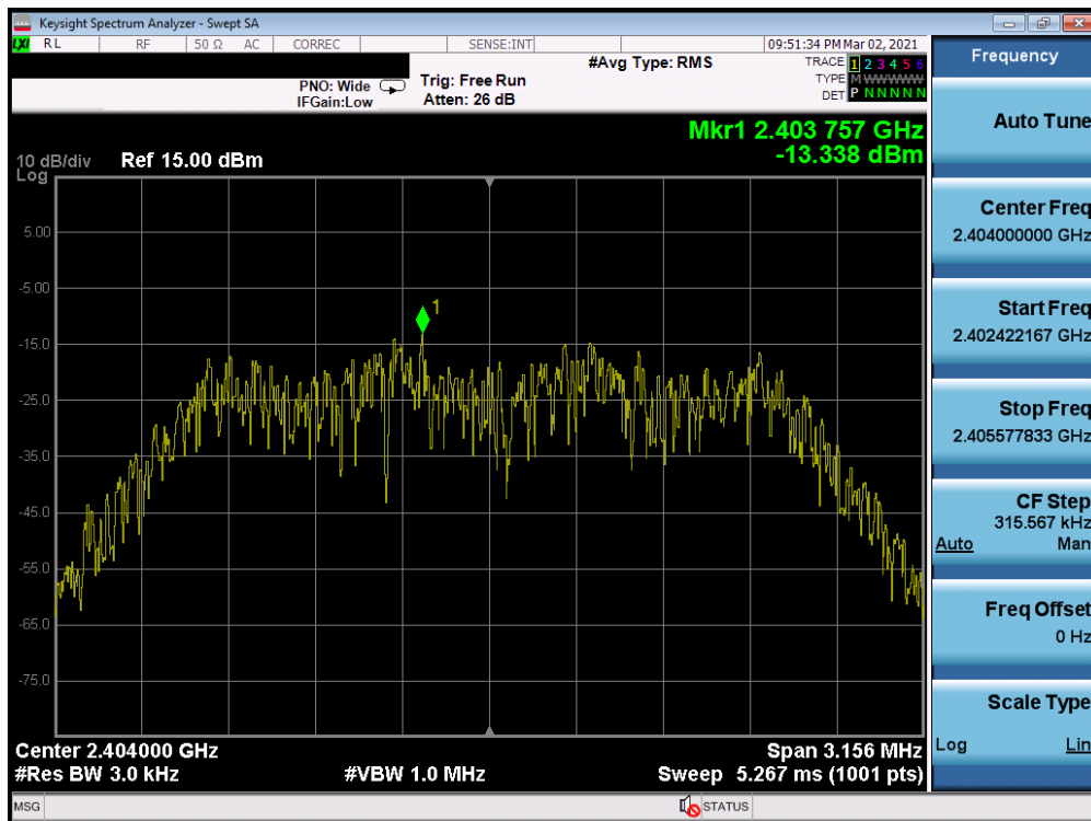
Plot 7-28. Power Spectral Density Plot Antenna 2a (Bluetooth (HDR4), 4Mbps, iPA – Ch. 1)
