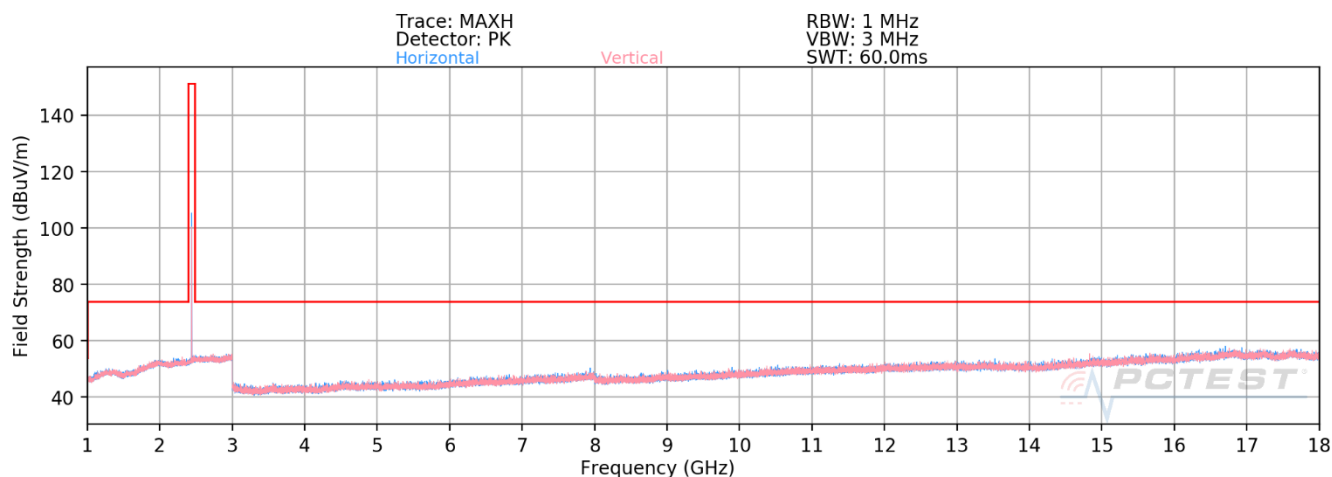
Plot 8-5. Radiated Spurious Emissions Above 1GHz TxBF (4Mbps, HDR4, ePA – Ch. 38)
