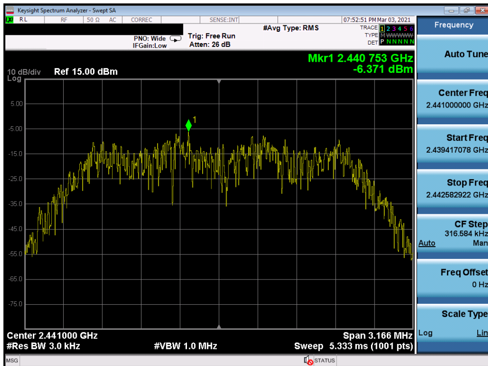
Plot 7-40. Power Spectral Density Plot Tx BF Antenna 2a (Bluetooth (HDR4), 4Mbps, ePA – Ch. 38)
