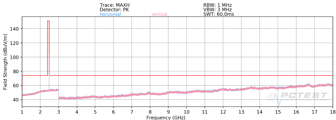
Plot 8-3. Radiated Spurious Emissions Above 1GHz Antenna 4a (1Mbps, LE, ePA – Ch. 39)
