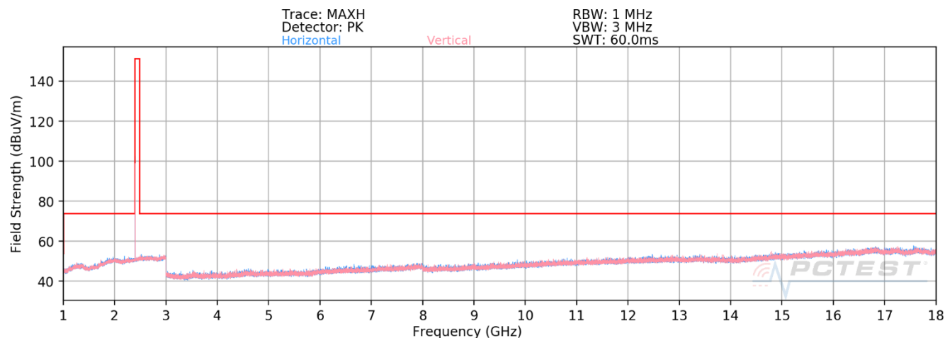
Plot 8-4. Radiated Spurious Emissions Above 1GHz TxBF (1Mbps, LE, ePA – Ch. 0)
