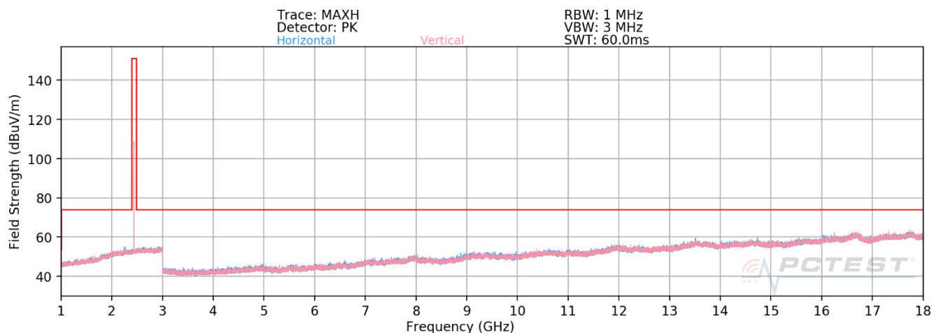
Plot 8-2. Radiated Spurious Emissions Above 1GHz Antenna 4a (1Mbps, LE, ePA – Ch. 19)
