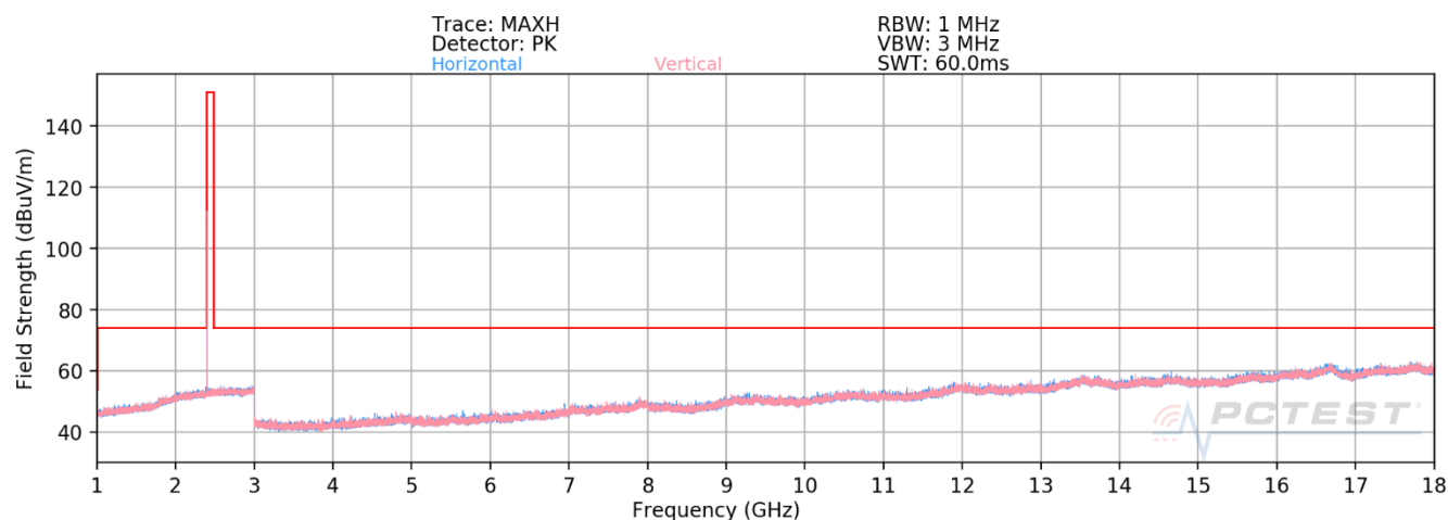
Plot 8-1. Radiated Spurious Emissions Above 1GHz Antenna 4a (1Mbps, LE, ePA – Ch. 0)
