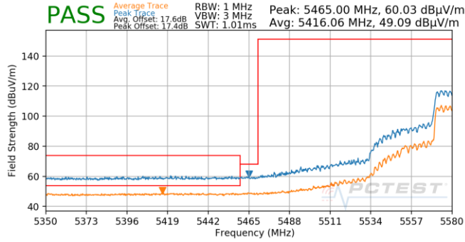
Plot 7-1053. (FCC Only) SDM (Pk & Avg, Ch.118, 802.11ax(SU), MCS3)
