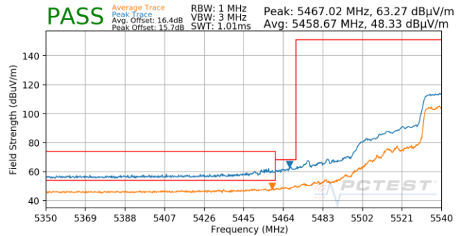
Plot 7-1020. CDD (Pk & Avg, Ch.110, 802.11n, MCS13)
