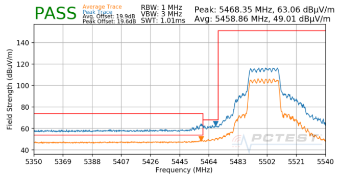
Plot 7-986. CDD (Pk & Avg, Ch.100, 802.11ax(SU), MCS3)
