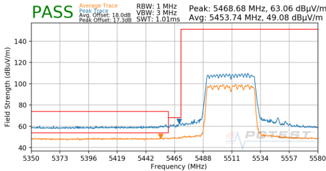
Plot 7-1049. CDD (Pk & Avg, Ch.102, 802.11ax(SU), MCS11)
