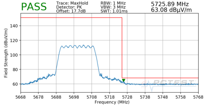
Plot 7-996. CDD (Pk, Ch.140, 802.11ax(SU), MCS11)
