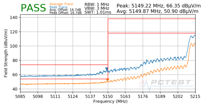
Plot 7-1038. CDD (Pk & Avg, Ch.46, 802.11ax(SU), MCS0)
