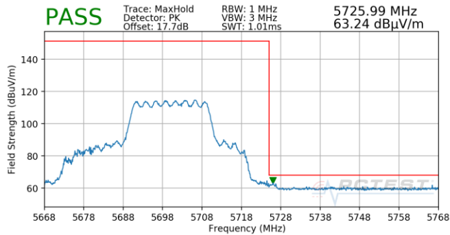
Plot 7-994. CDD (Pk, Ch.140, 802.11ax(SU), MCS0)
