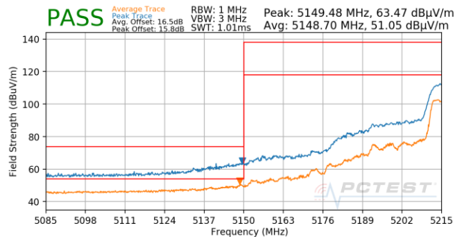
Plot 7-1008. CDD (Pk & Avg, Ch.46, 802.11n, MCS13)
