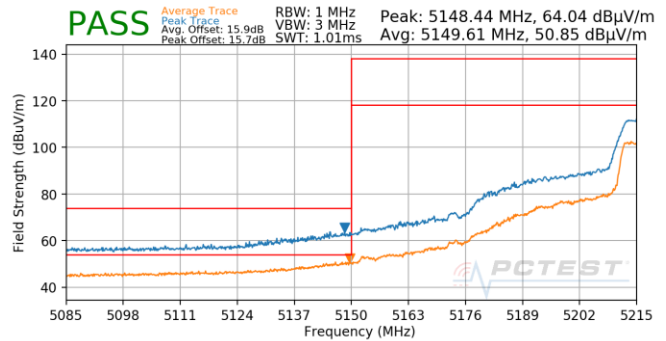
Plot 7-1006. SDM (Pk & Avg, Ch.46, 802.11n, MCS8)
