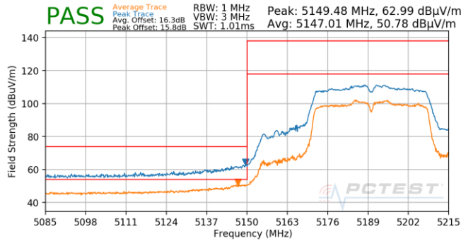
Plot 7-1004. CDD (Pk & Avg, Ch.38, 802.11n, MCS11)
