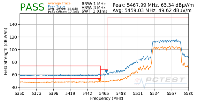
Plot 7-1052. CDD (Pk & Avg, Ch.110, 802.11ax(SU), MCS11)
