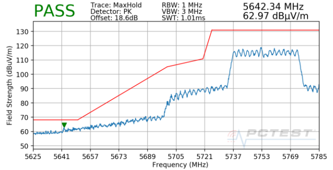
Plot 7-1062. CDD (Pk, Ch.151, 802.11ax(SU), MCS0)
