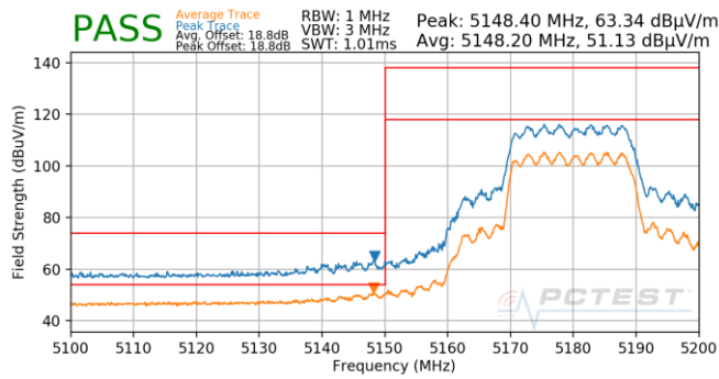
Plot 7-975. SDM (Pk & Avg, Ch.36, 802.11ax(SU), MCS0)
