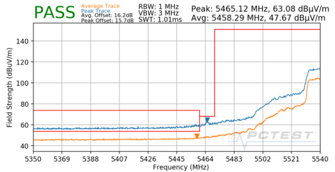
Plot 7-1019. SDM (Pk & Avg, Ch.110, 802.11n, MCS11)
