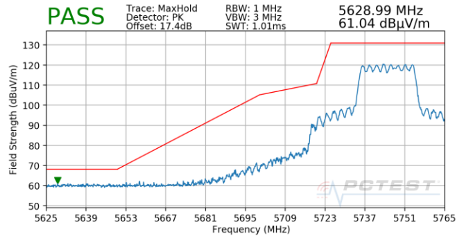
Plot 7-998. CDD (Pk, Ch.149, 802.11ax(SU), MCS3)
