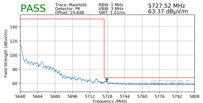
Plot 7-1058. (FCC Only) CDD (Pk, Ch.126, 802.11ax(SU), MCS11)
