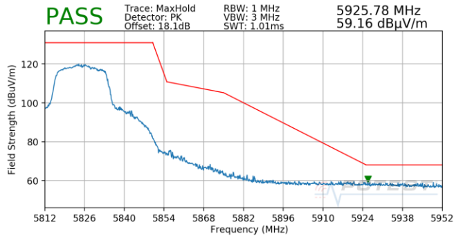
Plot 7-973. CDD (Pk, Ch.165, 802.11n, MCS11)
