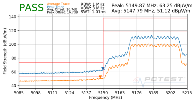
Plot 7-1035. CDD (Pk & Avg, Ch.38, 802.11ax(SU), MCS0)
