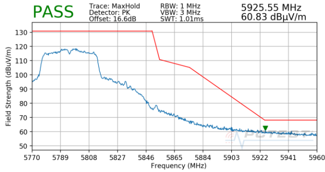
Plot 7-1033. CDD (Pk, Ch.159, 802.11n, MCS11)
