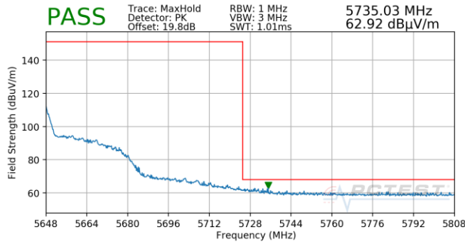
Plot 7-1023. (FCC Only) SDM (Pk, Ch.126, 802.11n, MCS8)
