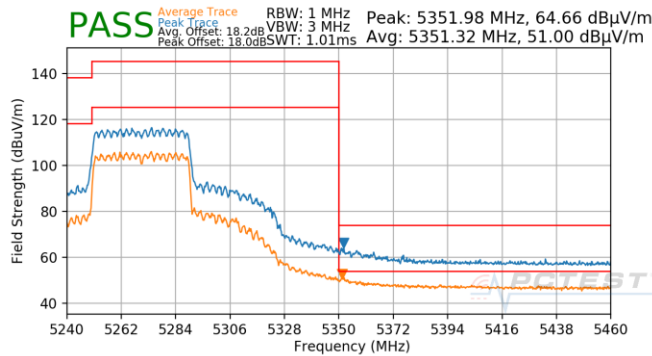
Plot 7-1042. CDD (Pk & Avg, Ch.54, 802.11ax(SU), MCS3)
