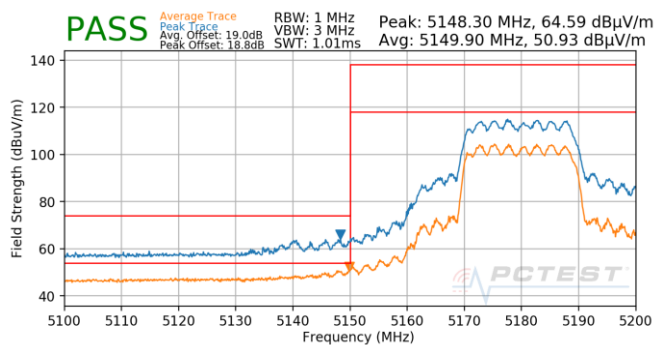
Plot 7-976. SDM (Pk & Avg, Ch.36, 802.11ax(SU), MCS3)
