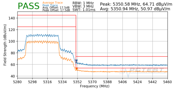
Plot 7-1044. CDD (Pk & Avg, Ch.62, 802.11ax(SU), MCS0)
