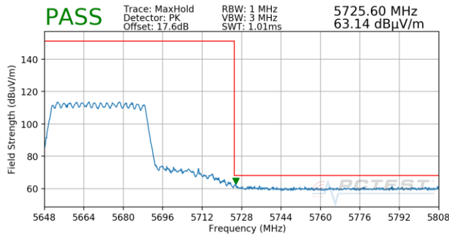
Plot 7-1060. CDD (Pk, Ch.134, 802.11ax(SU), MCS3)
