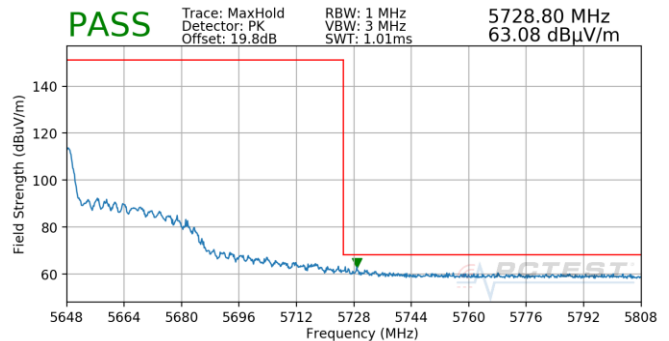
Plot 7-1057. (FCC Only) SDM (Pk, Ch.126, 802.11ax(SU), MCS3)
