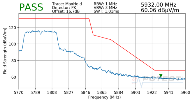
Plot 7-1034. CDD (Pk, Ch.159, 802.11n, MCS13)
