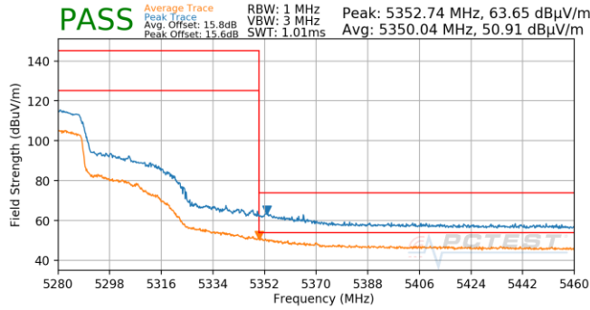
Plot 7-1009. SDM (Pk & Avg, Ch.54, 802.11n, MCS8)
