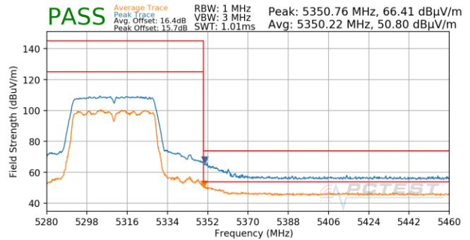
Plot 7-1014. CDD (Pk & Avg, Ch.62, 802.11n, MCS13)
