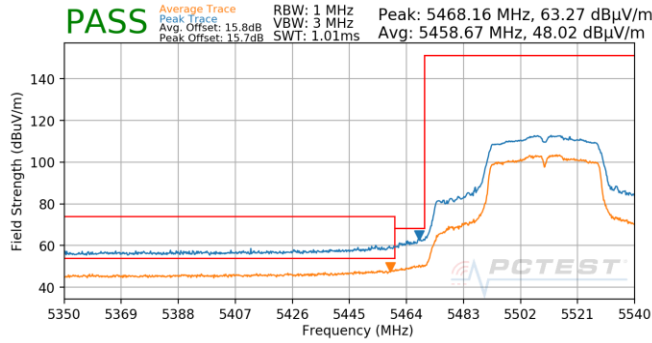
Plot 7-1015. CDD (Pk & Avg, Ch.102, 802.11n, MCS8)
