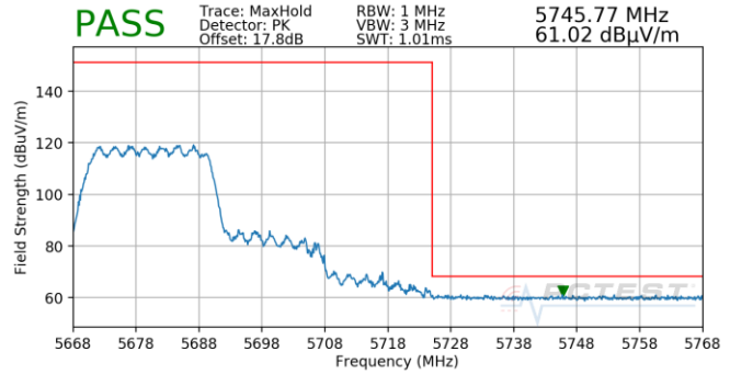
Plot 7-991. SDM (Pk, Ch.136, 802.11ax(SU), MCS0)
