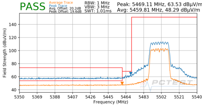
Plot 7-987. CDD (Pk & Avg, Ch.100, 802.11ax(SU), MCS11)
