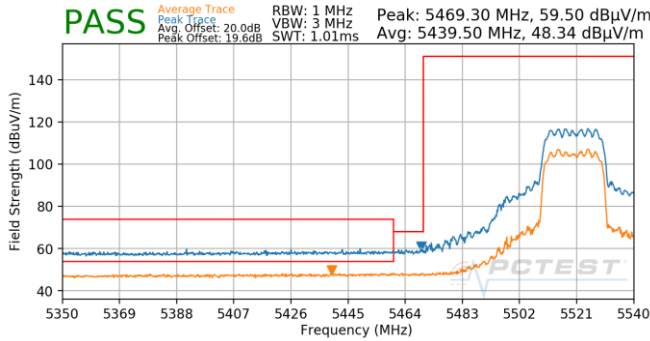
Plot 7-989. SDM (Pk & Avg, Ch.104, 802.11ax(SU), MCS11)
