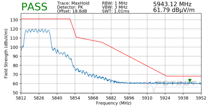
Plot 7-1002. CDD (Pk, Ch.165, 802.11ax(SU), MCS11)
