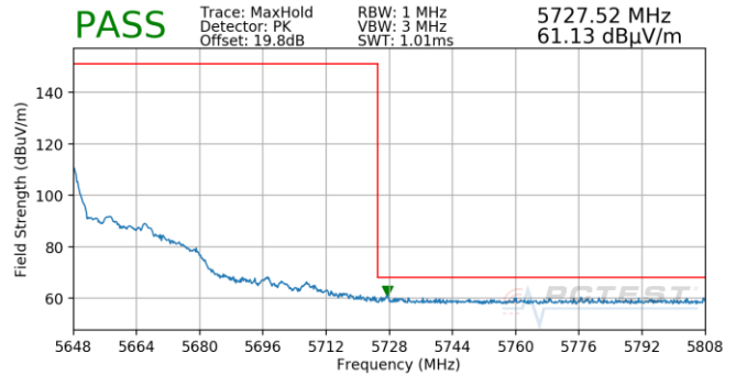
Plot 7-1025. (FCC Only) SDM (Pk, Ch.126, 802.11n, MCS13)
