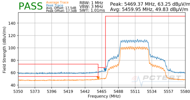
Plot 7-1047. CDD (Pk & Avg, Ch.102, 802.11ax(SU), MCS0)
