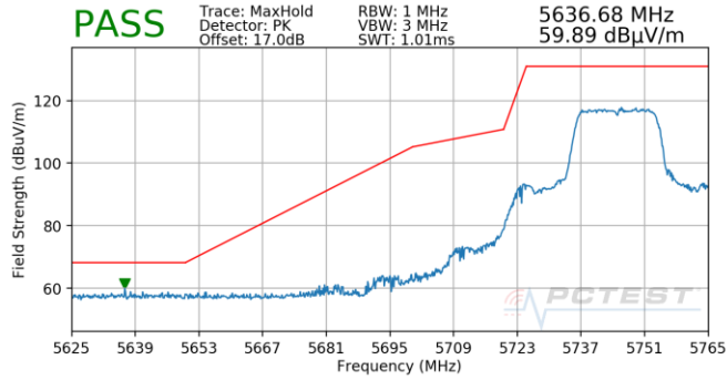
Plot 7-971. CDD (Pk, Ch.149, 802.11n, MCS13)
