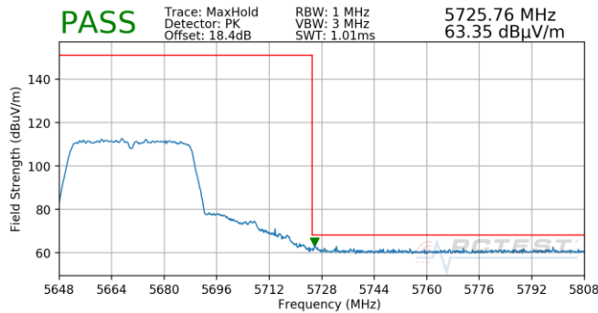
Plot 7-1028. CDD (Pk, Ch.134, 802.11n, MCS13)
