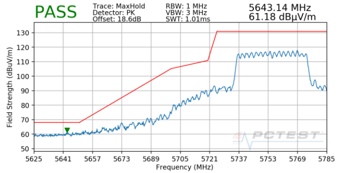
Plot 7-1064. CDD (Pk, Ch.151, 802.11ax(SU), MCS11)
