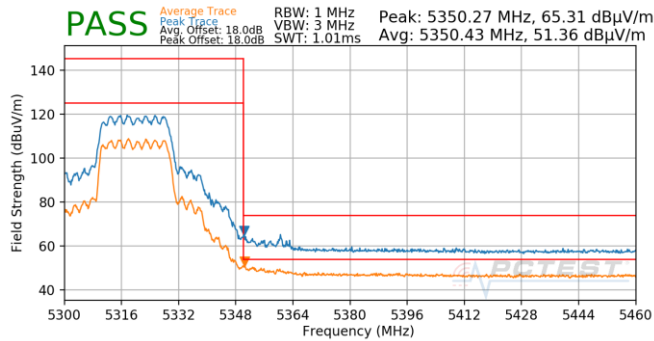
Plot 7-982. SDM (Pk & Avg, Ch.64, 802.11ax(SU), MCS0)
