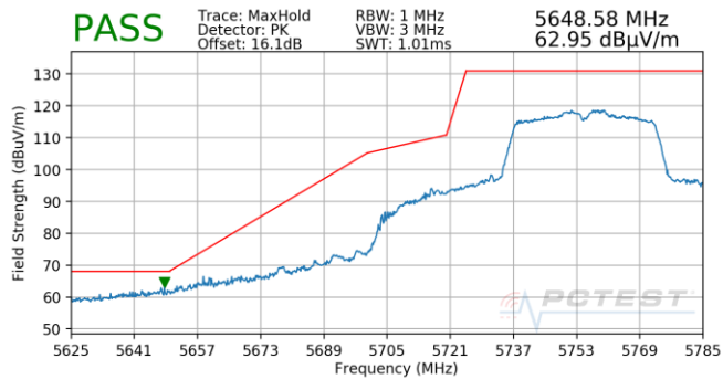
Plot 7-1029. CDD (Pk, Ch.151, 802.11n, MCS8)
