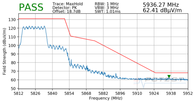
Plot 7-1000. CDD (Pk, Ch.165, 802.11ax(SU), MCS0)
