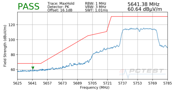
Plot 7-1031. CDD (Pk, Ch.151, 802.11n, MCS13)
