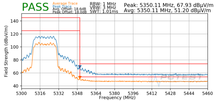
Plot 7-984. SDM (Pk & Avg, Ch.64, 802.11ax(SU), MCS11)
