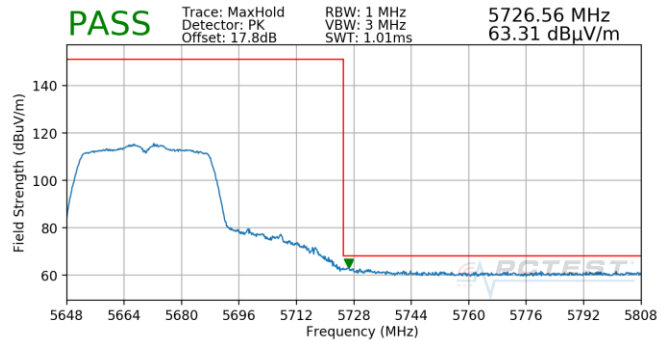
Plot 7-1026. CDD (Pk, Ch.134, 802.11n, MCS8)
