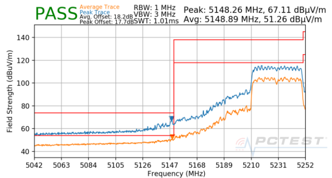
Plot 7-1040. CDD (Pk & Avg, Ch.46, 802.11ax(SU), MCS11)
