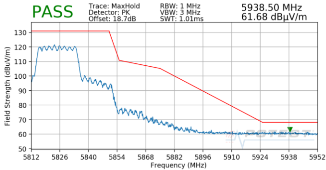
Plot 7-1001. CDD (Pk, Ch.165, 802.11ax(SU), MCS3)
