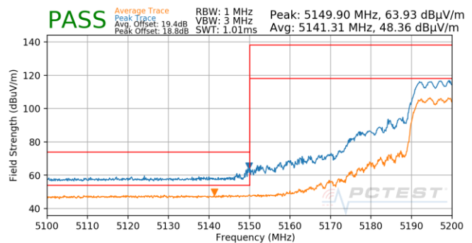
Plot 7-980. SDM (Pk & Avg, Ch.40, 802.11ax(SU), MCS11)
