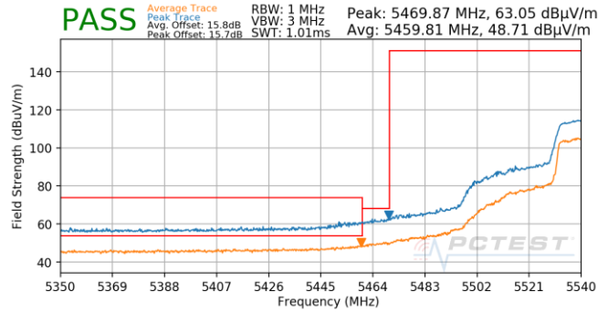
Plot 7-1018. SDM (Pk & Avg, Ch.110, 802.11n, MCS8)
