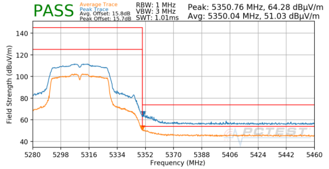
Plot 7-1012. CDD (Pk & Avg, Ch.62, 802.11n, MCS8)
