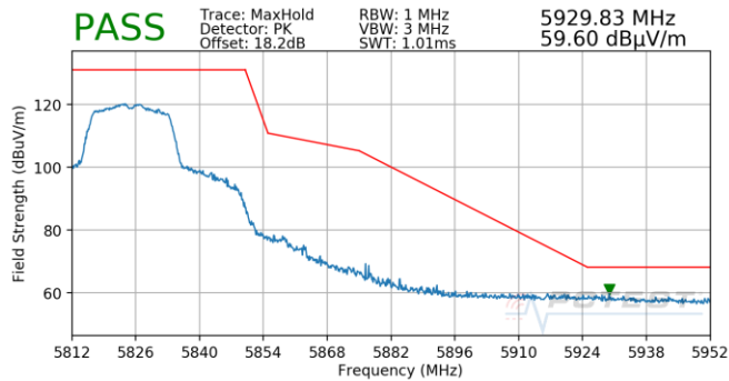
Plot 7-972. CDD (Pk, Ch.165, 802.11n, MCS8)
