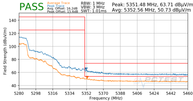
Plot 7-1010. SDM (Pk & Avg, Ch.54, 802.11n, MCS11)
