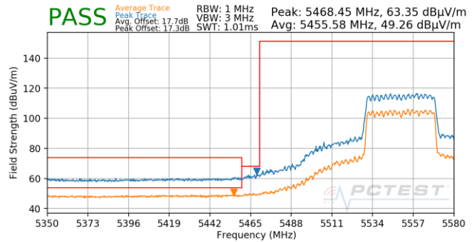
Plot 7-1051. CDD (Pk & Avg, Ch.110, 802.11ax(SU), MCS3)
