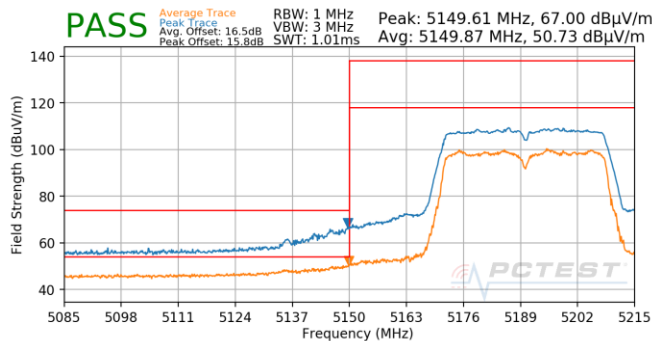
Plot 7-1005. CDD (Pk & Avg, Ch.38, 802.11n, MCS13)
