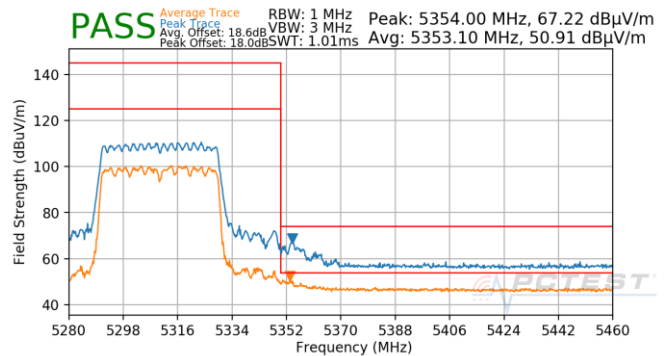
Plot 7-1046. CDD (Pk & Avg, Ch.62, 802.11ax(SU), MCS11)
