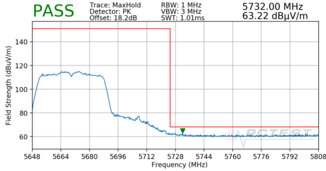
Plot 7-1027. CDD (Pk, Ch.134, 802.11n, MCS11)
