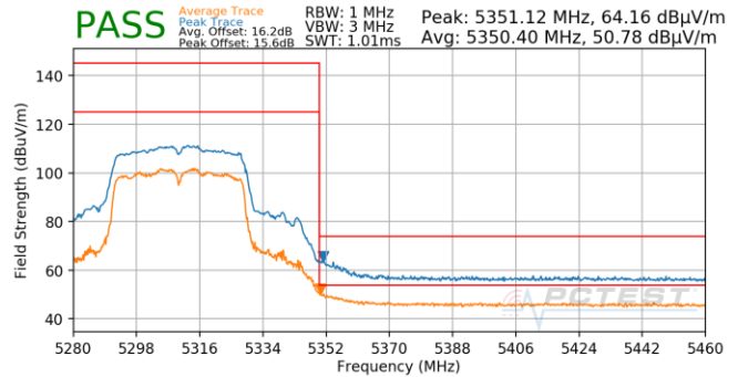
Plot 7-1013. CDD (Pk & Avg, Ch.62, 802.11n, MCS11)
