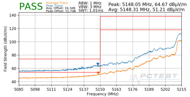
Plot 7-1007. SDM (Pk & Avg, Ch.46, 802.11n, MCS11)
