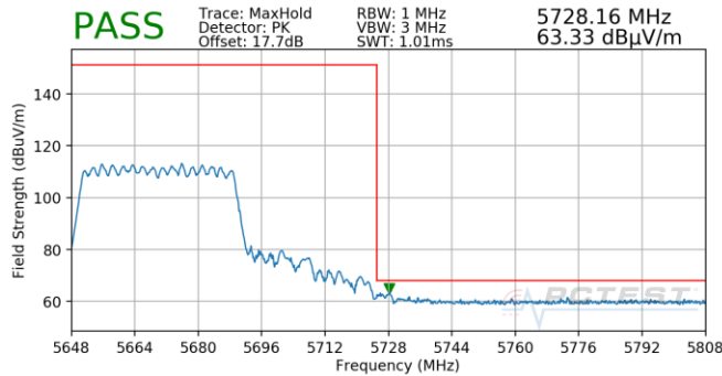
Plot 7-1061. CDD (Pk, Ch.134, 802.11ax(SU), MCS11)
