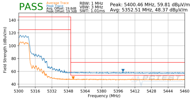
Plot 7-981. SDM (Pk & Avg, Ch.60, 802.11ax(SU), MCS11)
