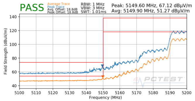
Plot 7-978. SDM (Pk & Avg, Ch.40, 802.11ax(SU), MCS0)
