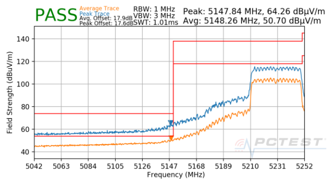
Plot 7-1039. CDD (Pk & Avg, Ch.46, 802.11ax(SU), MCS3)
