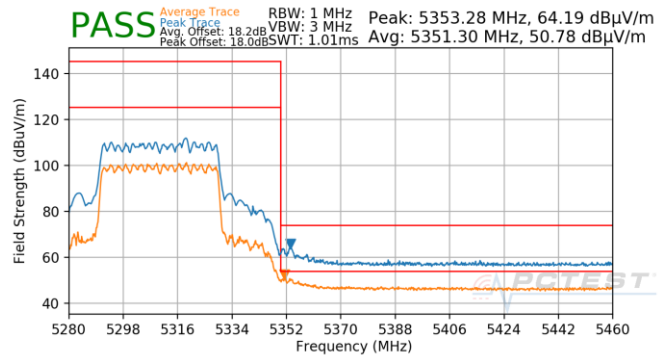
Plot 7-1045. CDD (Pk & Avg, Ch.62, 802.11ax(SU), MCS3)
