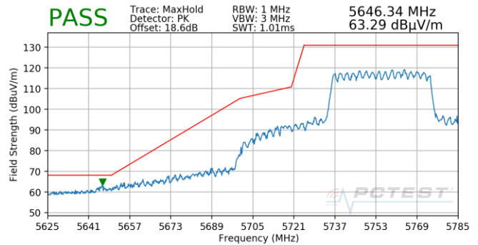
Plot 7-1063. CDD (Pk, Ch.151, 802.11ax(SU), MCS3)
