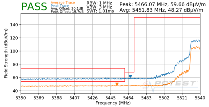
Plot 7-990. SDM (Pk & Avg, Ch.108, 802.11ax(SU), MCS11)
