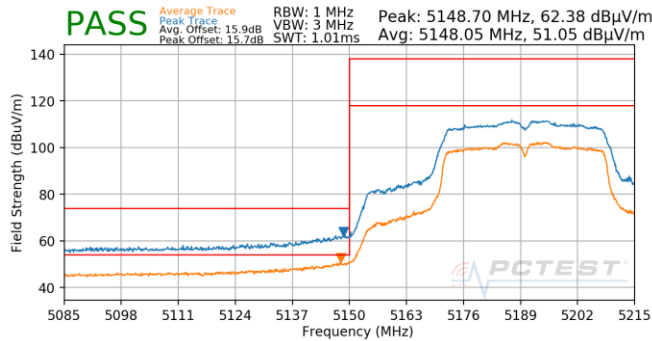
Plot 7-1003. CDD (Pk & Avg, Ch.38, 802.11n, MCS8)
