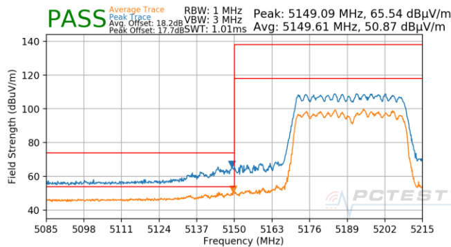
Plot 7-1037. CDD (Pk & Avg, Ch.38, 802.11ax(SU), MCS11)
