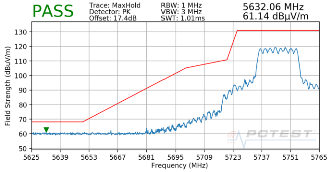
Plot 7-999. CDD (Pk, Ch.149, 802.11ax(SU), MCS11)
