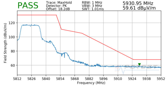
Plot 7-974. CDD (Pk, Ch.165, 802.11n, MCS13)
