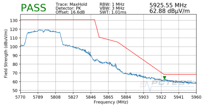
Plot 7-1032. CDD (Pk, Ch.159, 802.11n, MCS8)
