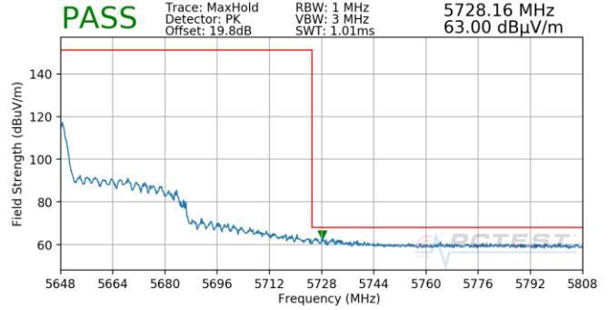
Plot 7-1056. (FCC Only) SDM (Pk, Ch.126, 802.11ax(SU), MCS0)
