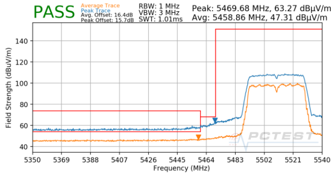
Plot 7-1017. CDD (Pk & Avg, Ch.102, 802.11n, MCS13)
