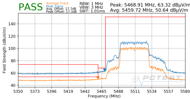
Plot 7-1048. CDD (Pk & Avg, Ch.102, 802.11ax(SU), MCS3)
