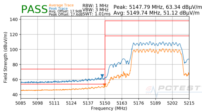
Plot 7-1036. CDD (Pk & Avg, Ch.38, 802.11ax(SU), MCS3)
