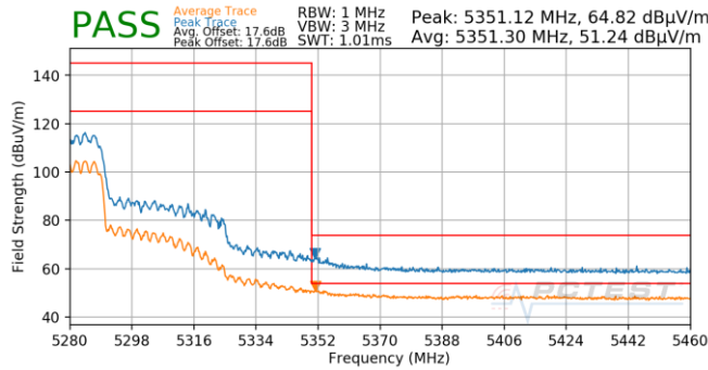
Plot 7-1041. SDM (Pk & Avg, Ch.54, 802.11ax(SU), MCS0)
