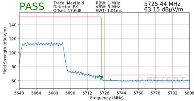
Plot 7-1059. CDD (Pk, Ch.134, 802.11ax(SU), MCS0)
