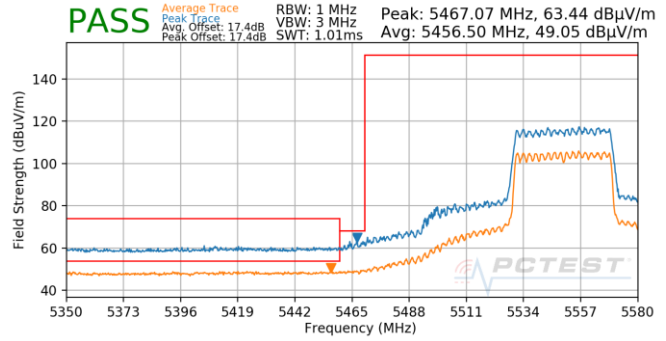
Plot 7-1050. CDD (Pk & Avg, Ch.110, 802.11ax(SU), MCS0)
