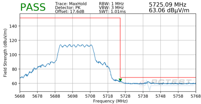
Plot 7-995. CDD (Pk, Ch.140, 802.11ax(SU), MCS3)
