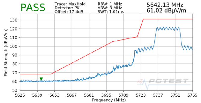
Plot 7-997. CDD (Pk, Ch.149, 802.11ax(SU), MCS0)
