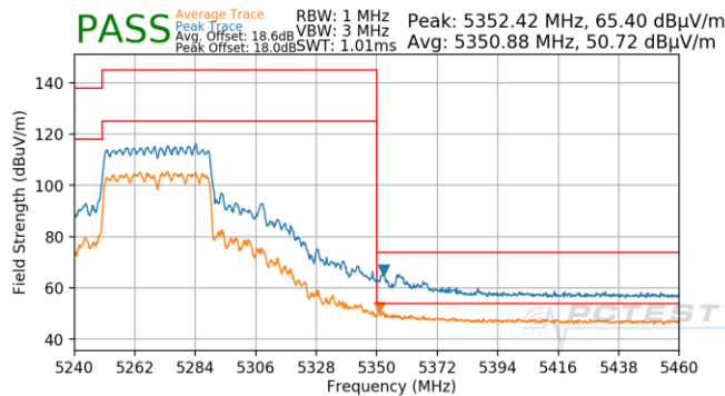
Plot 7-1043. CDD (Pk & Avg, Ch.54, 802.11ax(SU), MCS11)
