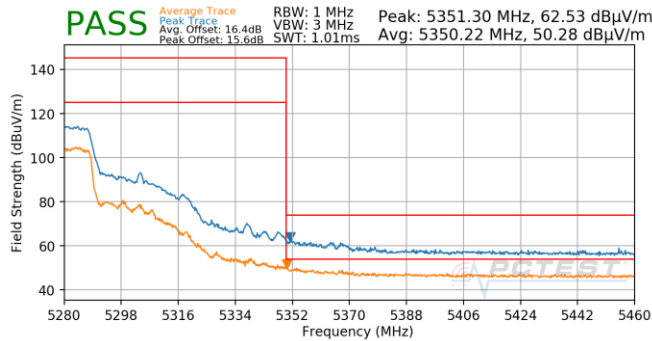
Plot 7-1011. SDM (Pk & Avg, Ch.54, 802.11n, MCS13)
