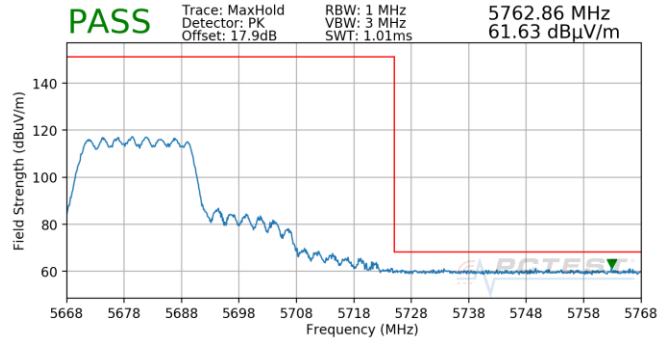
Plot 7-992. SDM (Pk, Ch.136, 802.11ax(SU), MCS3)
