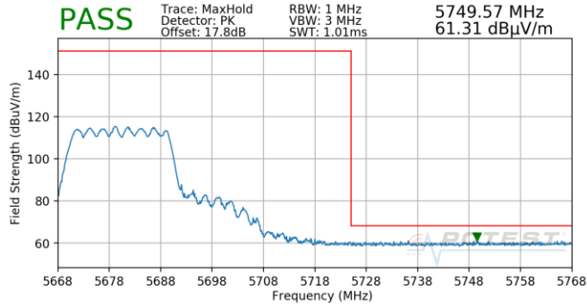
Plot 7-993. SDM (Pk, Ch.136, 802.11ax(SU), MCS11)
