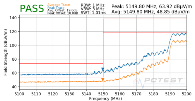
Plot 7-979. SDM (Pk & Avg, Ch.40, 802.11ax(SU), MCS3)
