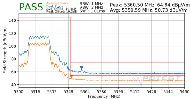
Plot 7-983. SDM (Pk & Avg, Ch.64, 802.11ax(SU), MCS3)
