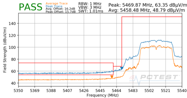
Plot 7-1016. CDD (Pk & Avg, Ch.102, 802.11n, MCS11)
