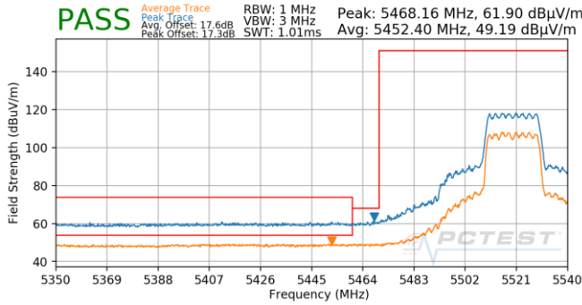
Plot 7-988. SDM (Pk & Avg, Ch.104, 802.11ax(SU), MCS3)
