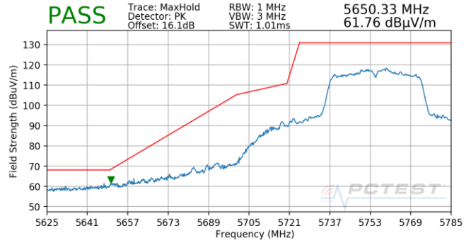
Plot 7-1030. CDD (Pk, Ch.151, 802.11n, MCS11)
