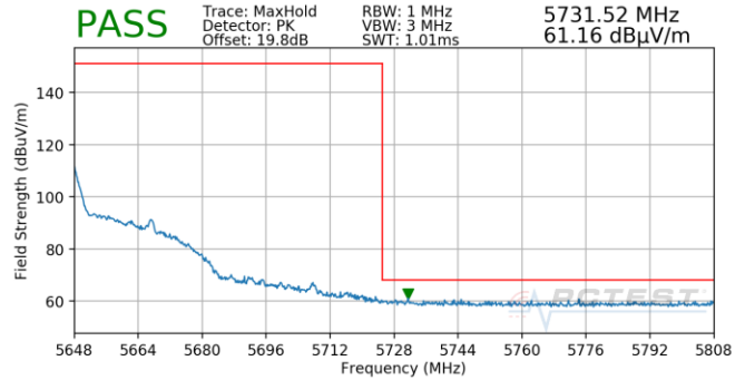
Plot 7-1024. (FCC Only) SDM (Pk, Ch.126, 802.11n, MCS11)
