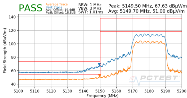
Plot 7-977. CDD (Pk & Avg, Ch.36, 802.11ax(SU), MCS11)
