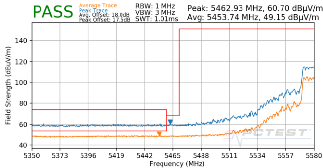
Plot 7-1054. (FCC Only) CDD (Pk & Avg, Ch.118, 802.11ax(SU), MCS11)
