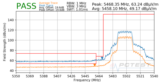
Plot 7-985. SDM (Pk & Avg, Ch.100, 802.11ax(SU), MCS0)
